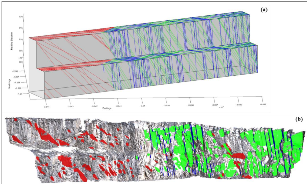
Figure 22: SiroModel fracture traces calibration (a) Simulated fracture traces within SiroModel software (b) mapped fractures on the study area
