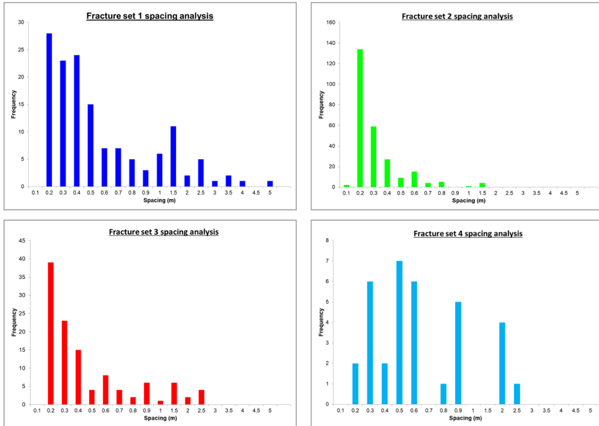
Figure 14: Fracture spacing distribution per Fracture Set
