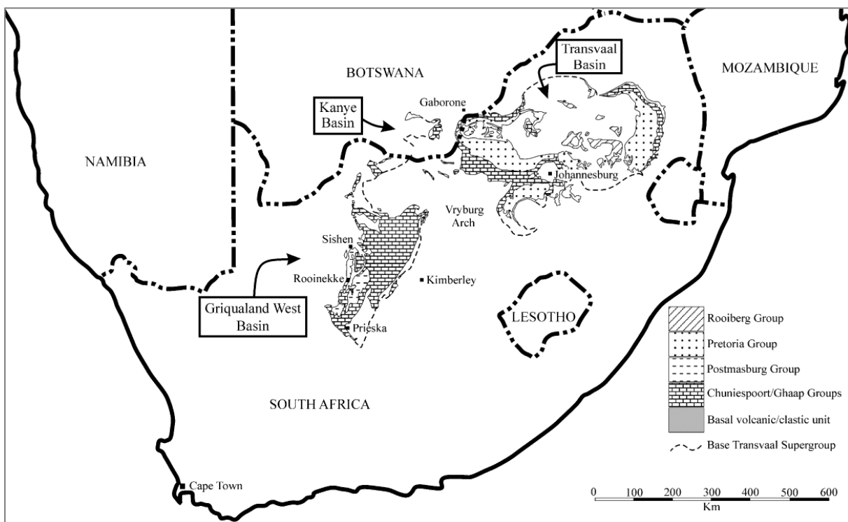
Figure 2. Locality map, showing the distribution of the major subdivisions of the Transvaal Supergroup (adapted from Moore et al. , 2001)
