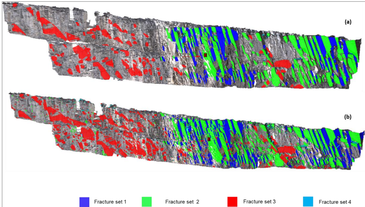
Figure 12: Cut 7 wall mapped fracture sets – (7a) is the mapping with user defined limits on area of extents (7b) shows fractures where limits were not defined, the system minimum and maximum areas of extents were used
