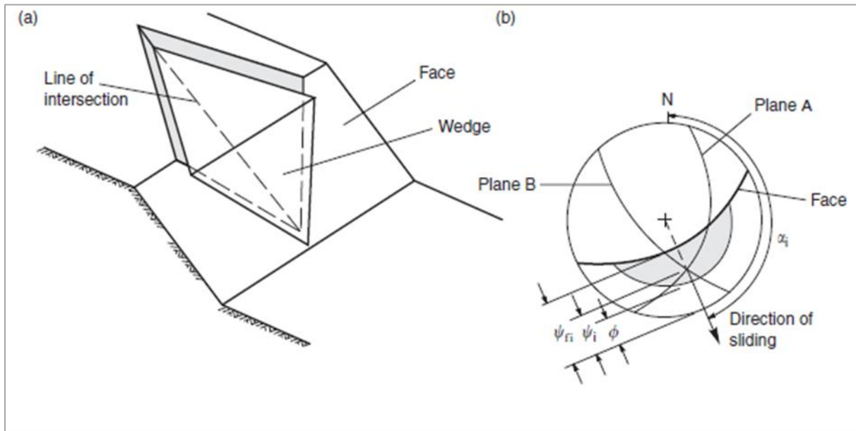
Figure 18: Geometry of wedge slope failure; (a) pictorial view of wedge slope failure; (b) Stereoplot showing the line of intersection (Rajesh, 2014)
