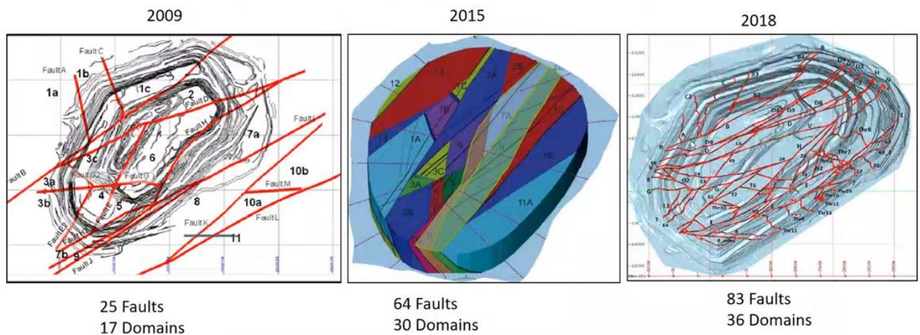
Figure 4. Chronology of Jwaneng geotechnical domains with structural model update
