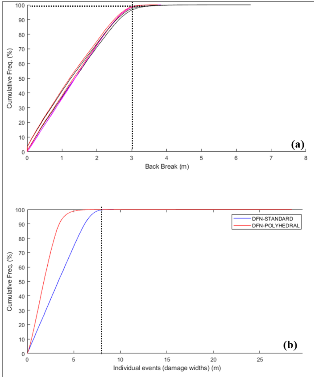
Figure 30: Back break analysis of the research area (a) Back break analysis (b) Individual events strike length analysis
