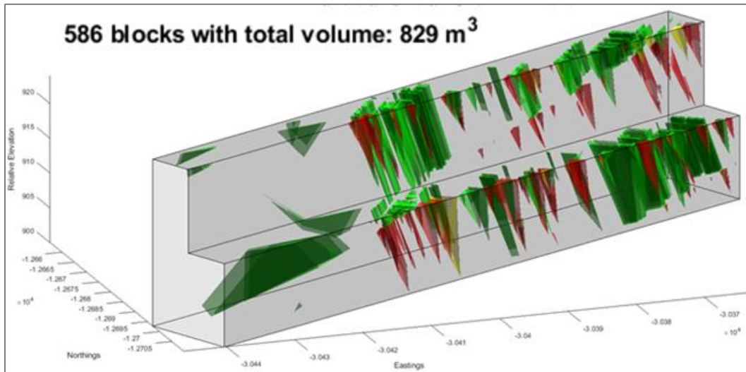
Figure 27: Block simulated from the four mapped fracture sets
