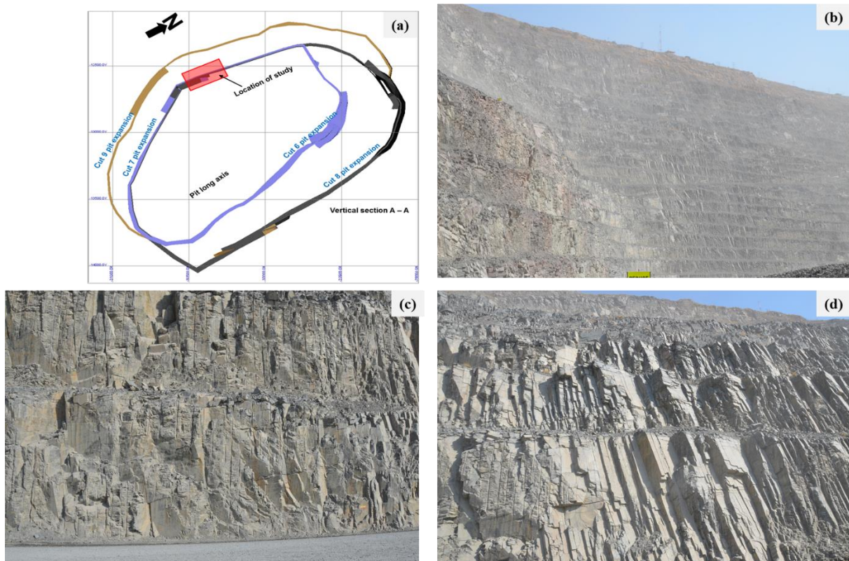
Figure 6: Research area (a) Location of research area within the Jwaneng open pit (b) Overview/large scale view of Cut 7 walls study area (c) & (d) Close-up view of typical fracture orientations/interactions within the Cut 7 research area
