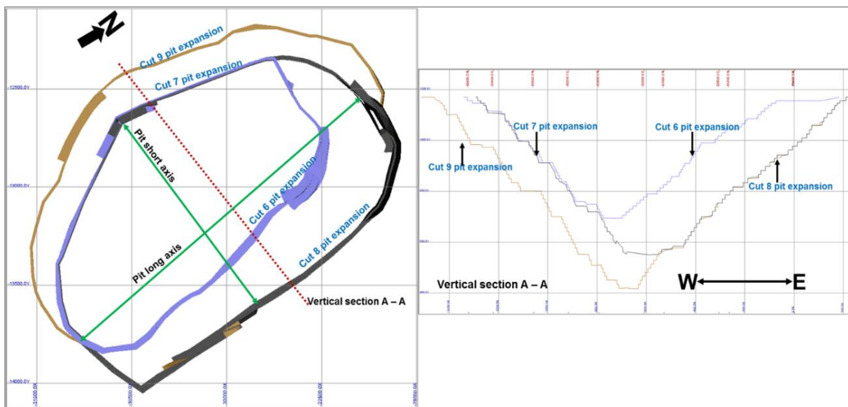
Figure 1: Jwaneng Mine open pit expansion – split shell open pit expansion adapted from (Debswana, 2017)
