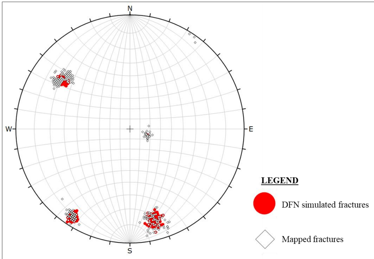
Figure 24: Stereoplot comparison of Simulated fractures and mapped fractures
