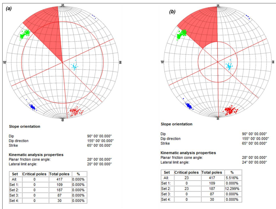
Figure 17: Cut 7 walls Planar failure analysis stereographic projection from Maptek I-site software
