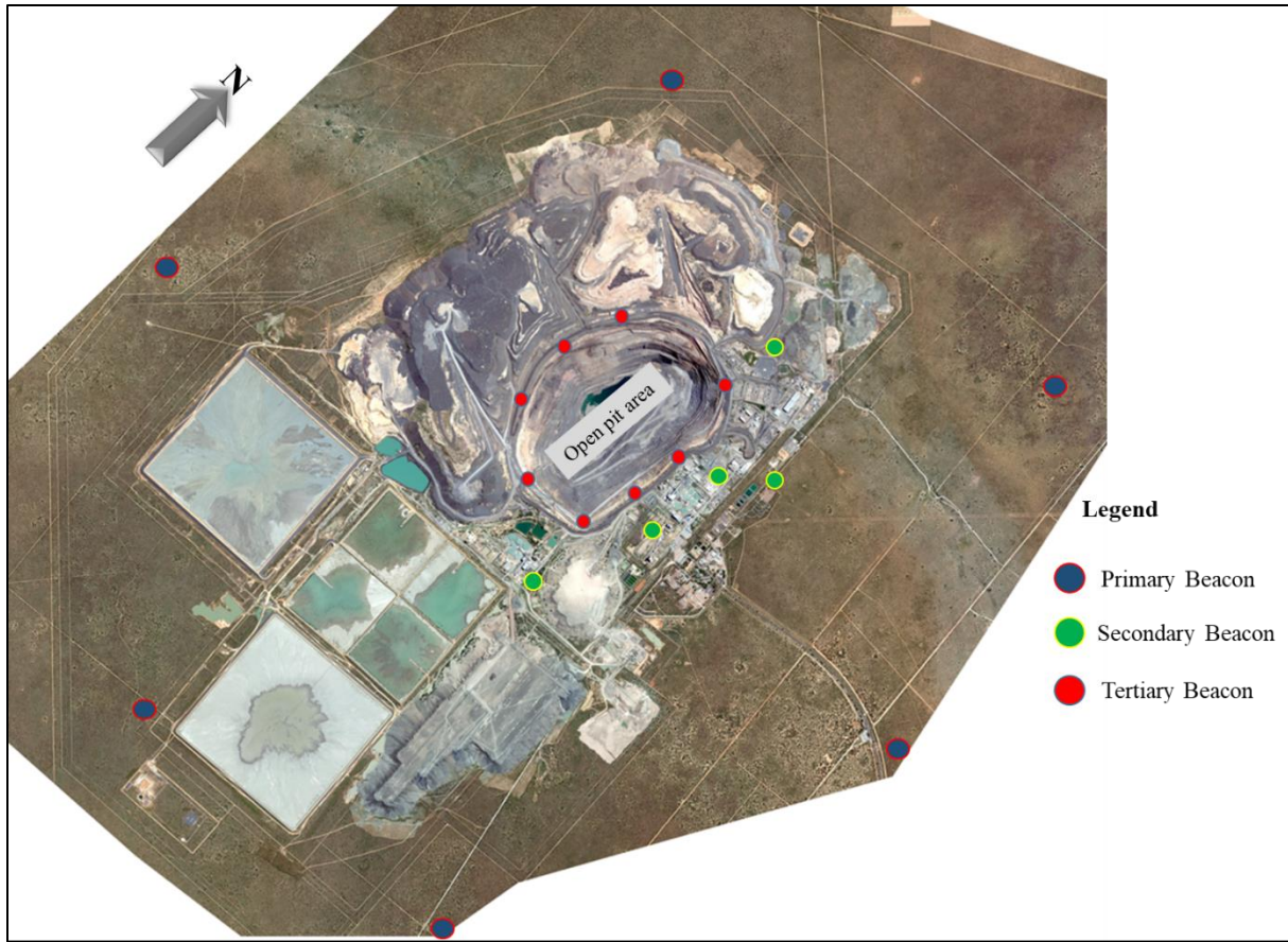
Figure 7: Jwaneng Mine Survey Control Network
