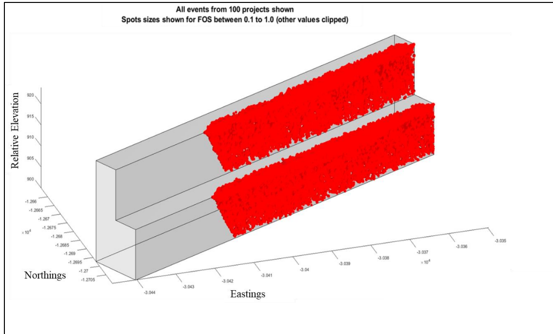
Figure 34: Potential rockfall Hazard Map of the research area
