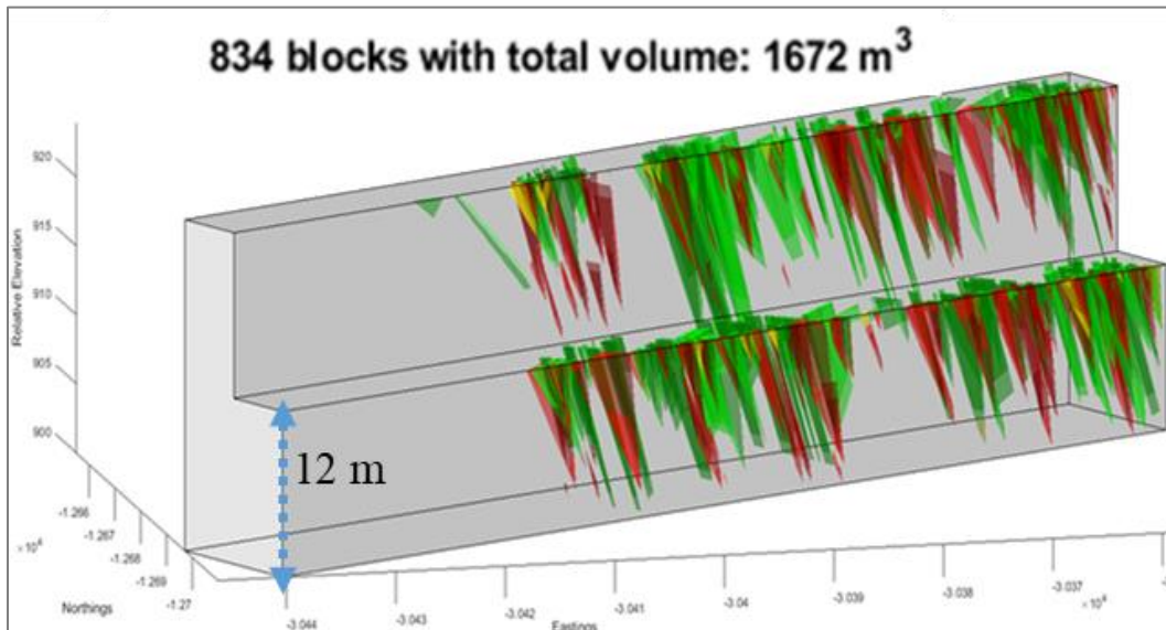
Figure 28: Block model simulations from the three stochastic fracture sets
