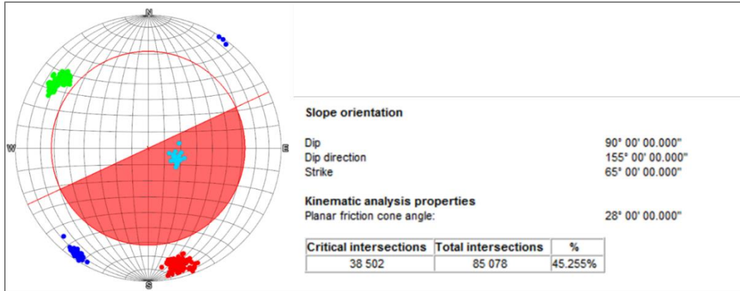
Figure 19: Cut 7 walls wedge failure analysis
