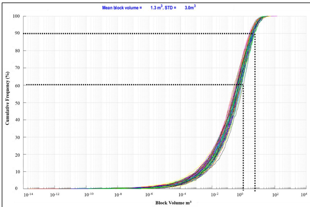
Figure 32: Potential rockfall block volume distribution within the study area
