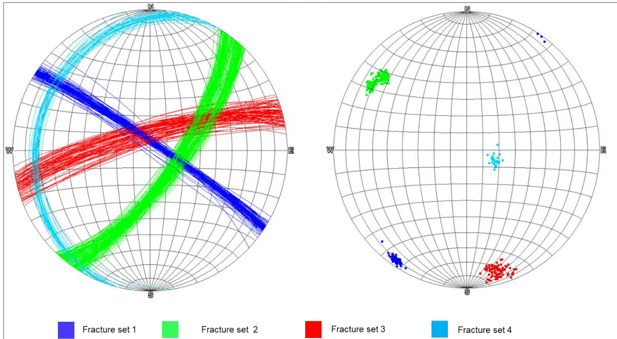
Figure 13: Stereographic plot of mapped Fracture Sets (planes and poles)
