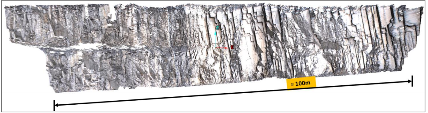
Figure 10: Cut 7 wall image produced from Maptek Maptek I-Site 8820
