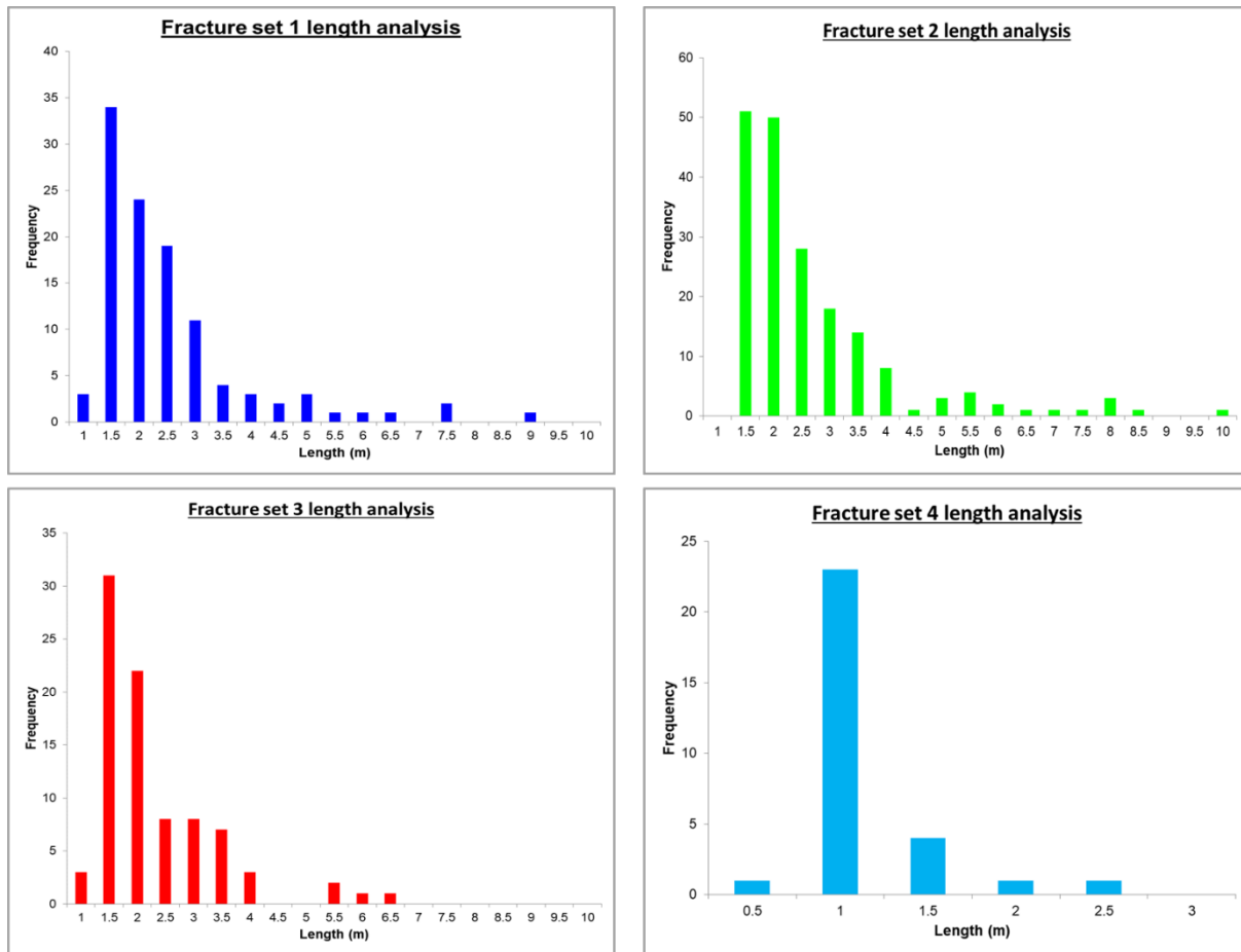
Figure 15: Fracture length distribution per set
