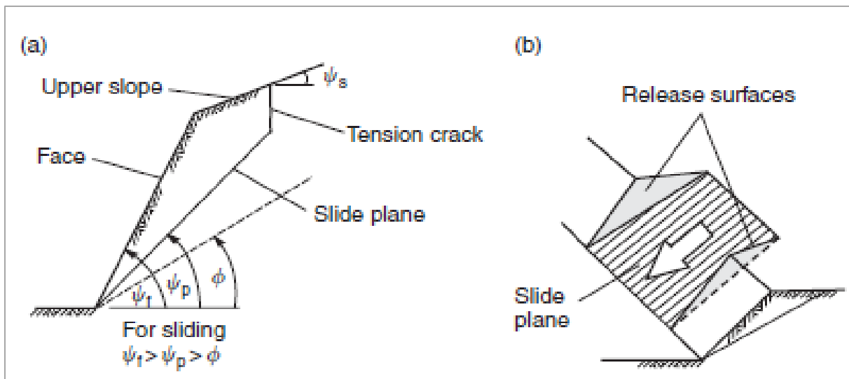
Figure 16: Geometry of plane slope failure: (a) Typical view of a plane failure; (b) release surfaces at the ends of the plane failure (Wyllie & Mah, 2004)
