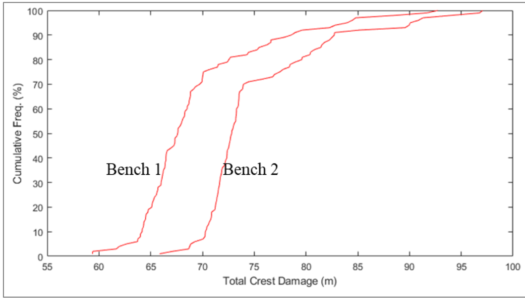
Figure 31: Total crest damage analysis (along the strike length)
