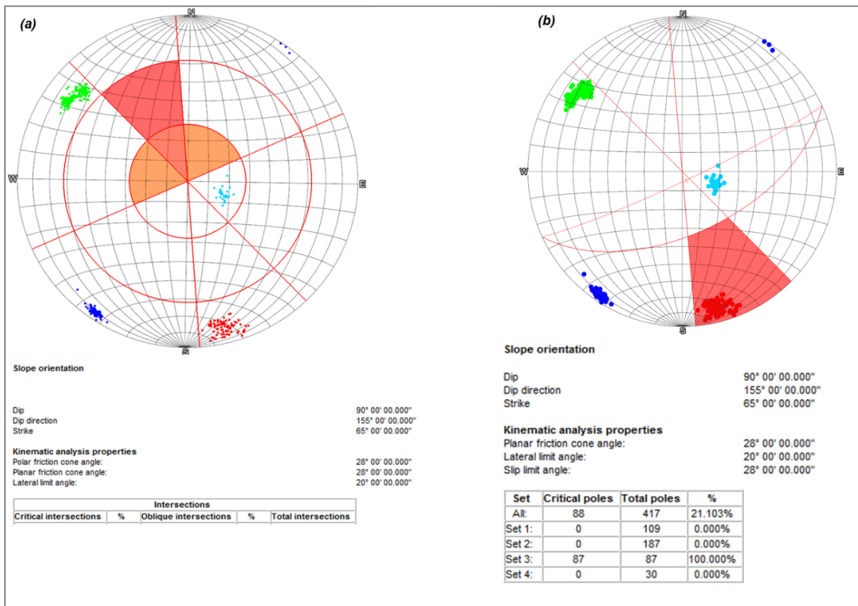
Figure 21: Cut 7 walls toppling failure analysis (a) Flexural toppling (b) Direct toppling
