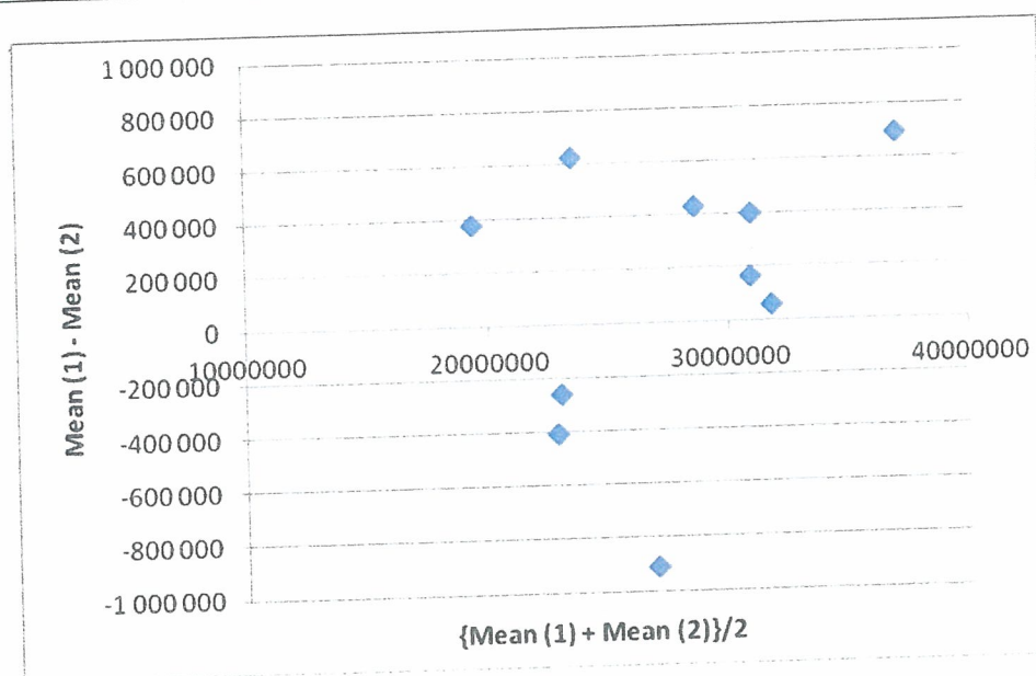
Figure 4.15 Bland-Altman plot
