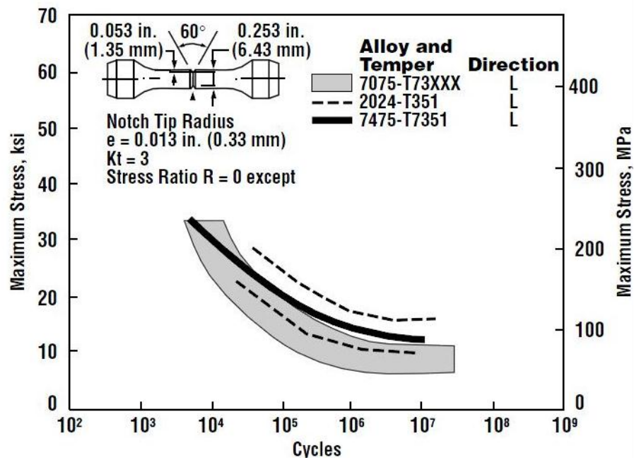
Figure 2-31: Data for AL7075 [24]
