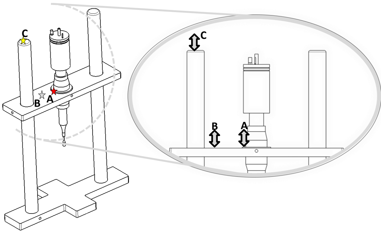
Figure 4-30: Position where vibration of Rig was investigated
