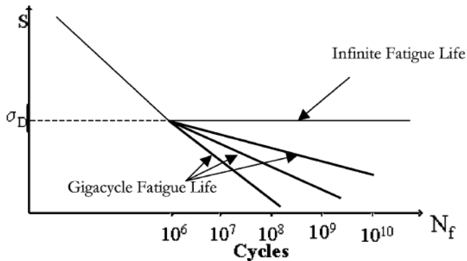
Figure 1-2: Possible material fatigue properties in giga-cycle region [1]
