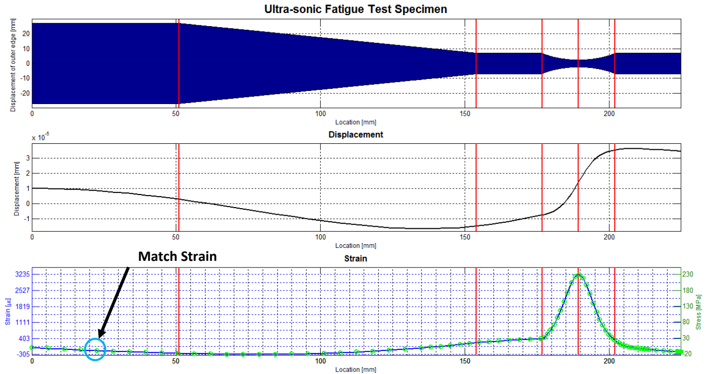
Figure 4-27: Typical displacement, strain and stress output
