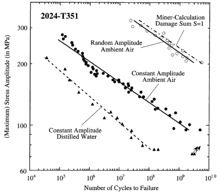
Figure 2-16: Fatigue data for aluminium 2024-T351, Stanzi [12]
