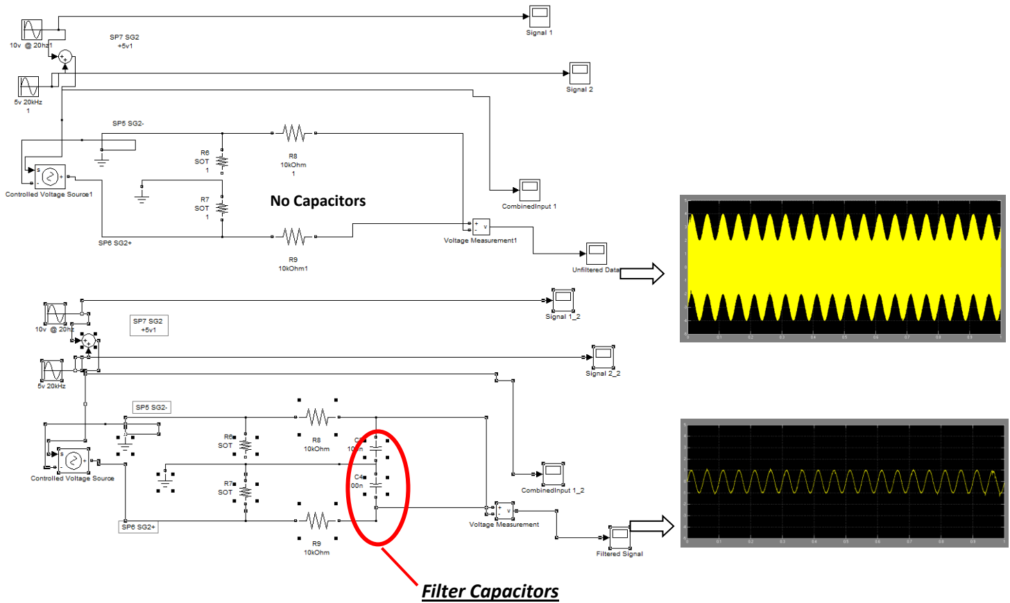
Figure D-5: Test of Circuitry
