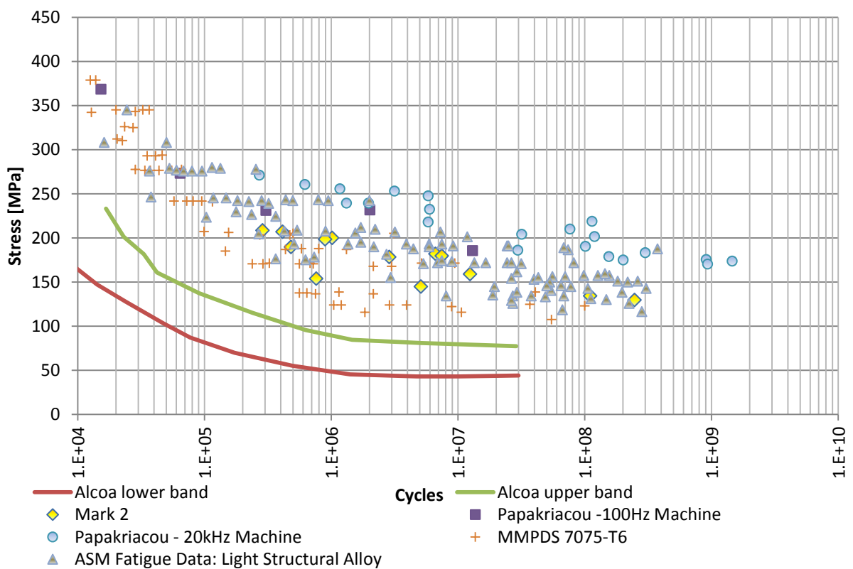
Figure 4-36: Mark 2 AL7075-T7351
