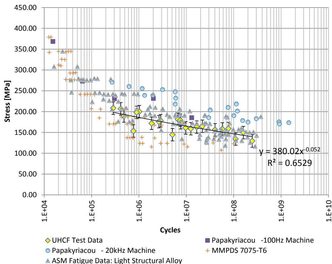
Figure 5-3: Comparison of AL7075-T7351 Data
