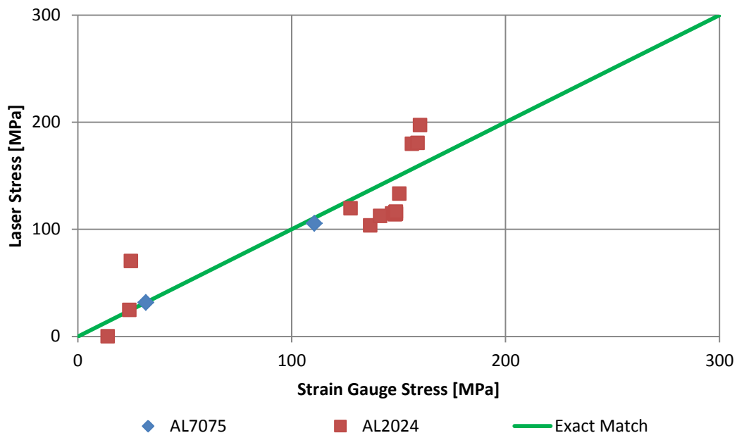
Figure 4-21: Comparison of strain gauges to laser
