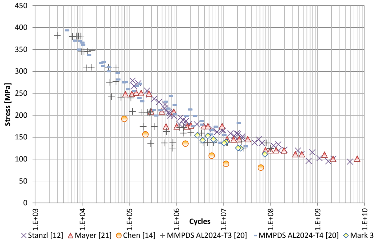
Figure 4-39: Mark 3 AL2024-T351
