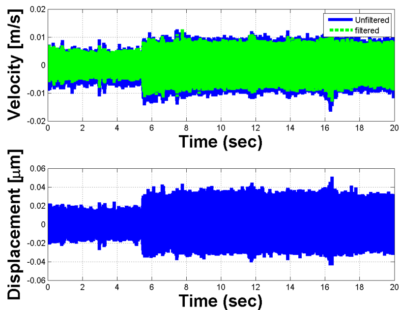
Figure 4-32: Top support displacement
