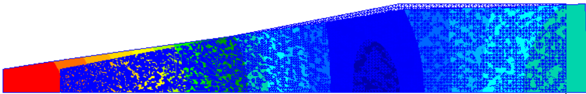
Figure 4-15: Axial resonance mode of the AL7075 horn design
