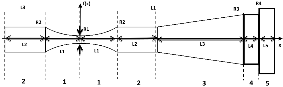
Figure A-1: General sonic fatigue specimen
