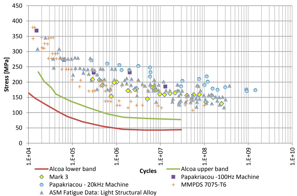
Figure 4-40: Mark 3 AL7075-T7351
