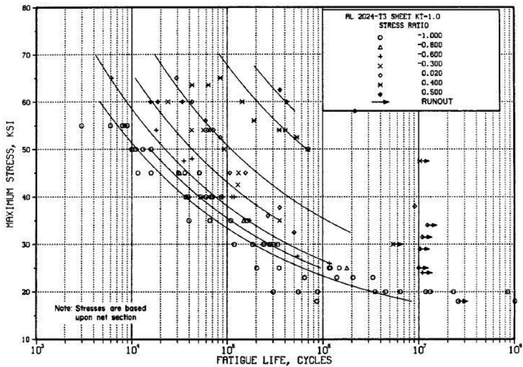
Figure 2-21: AL2024-T3 as per MMPDS [20]
