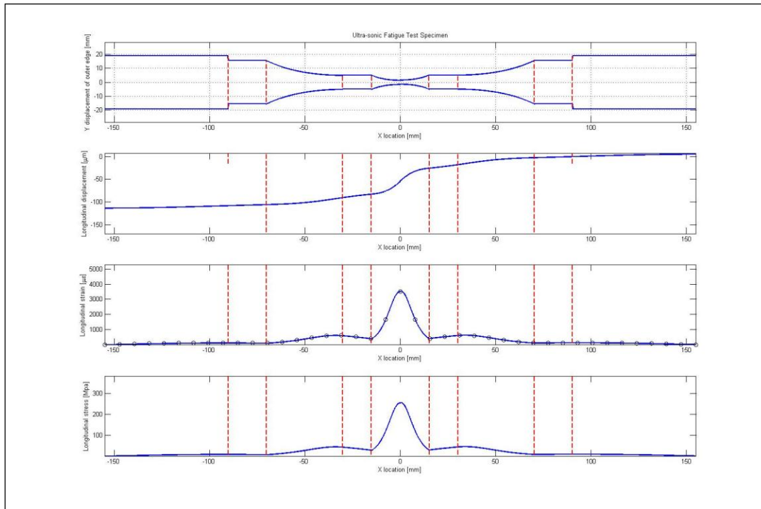
Figure A-3: Plot for 5 section specimen model fixed geometry
