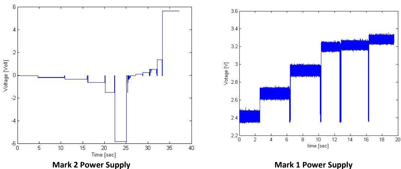
Figure 4-20: Comparison to power generator noise output
