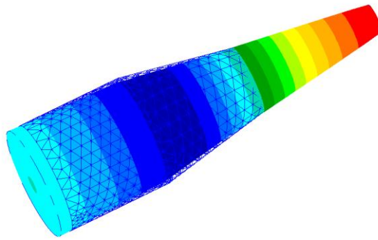
Figure 4-16: 3D FEM Tet10 horn model
