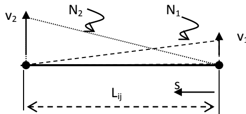
Figure C-5: Boundary displacement at a location on side 12
