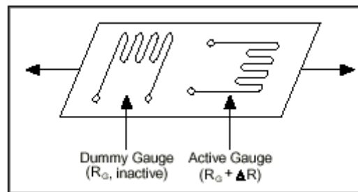
Figure B-5: Use of dummy gauge to eliminate temperature affects [26].
