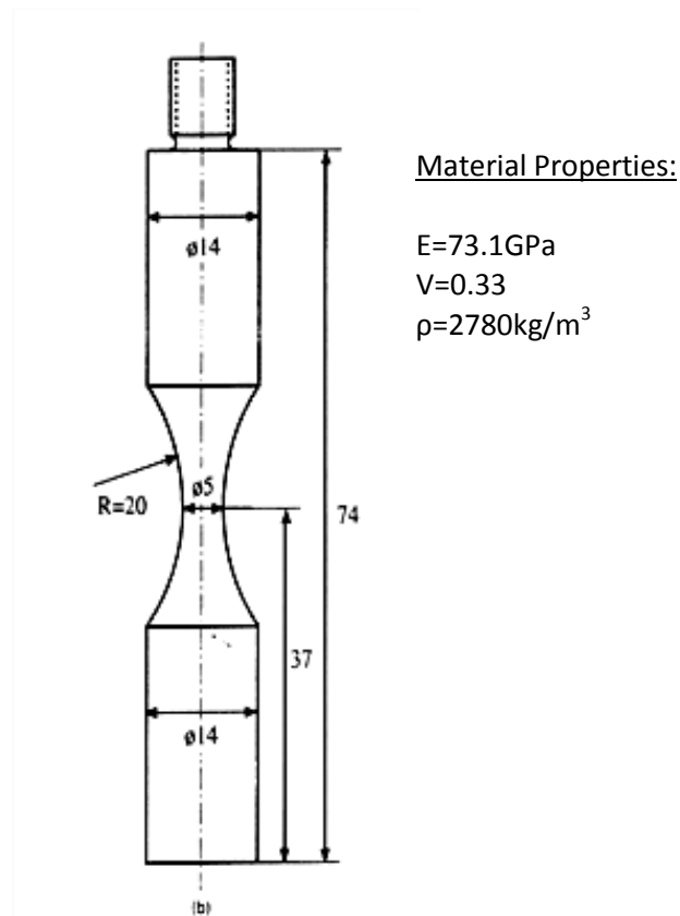
Figure 2-17: Typical aluminium 2024 specimen, Chen [14]
