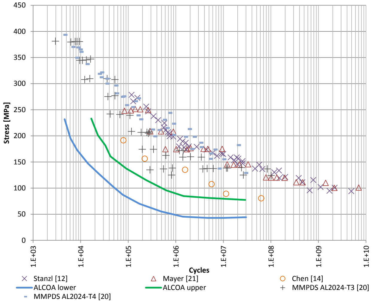
Figure 2-24: AL2024 combine data
