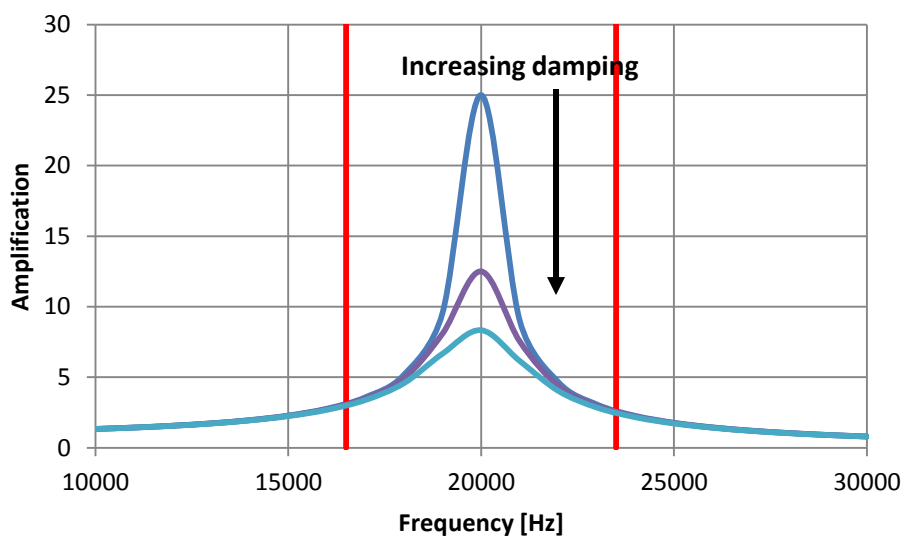
Figure 4-18: Amplification affects for one degree of freedom system
