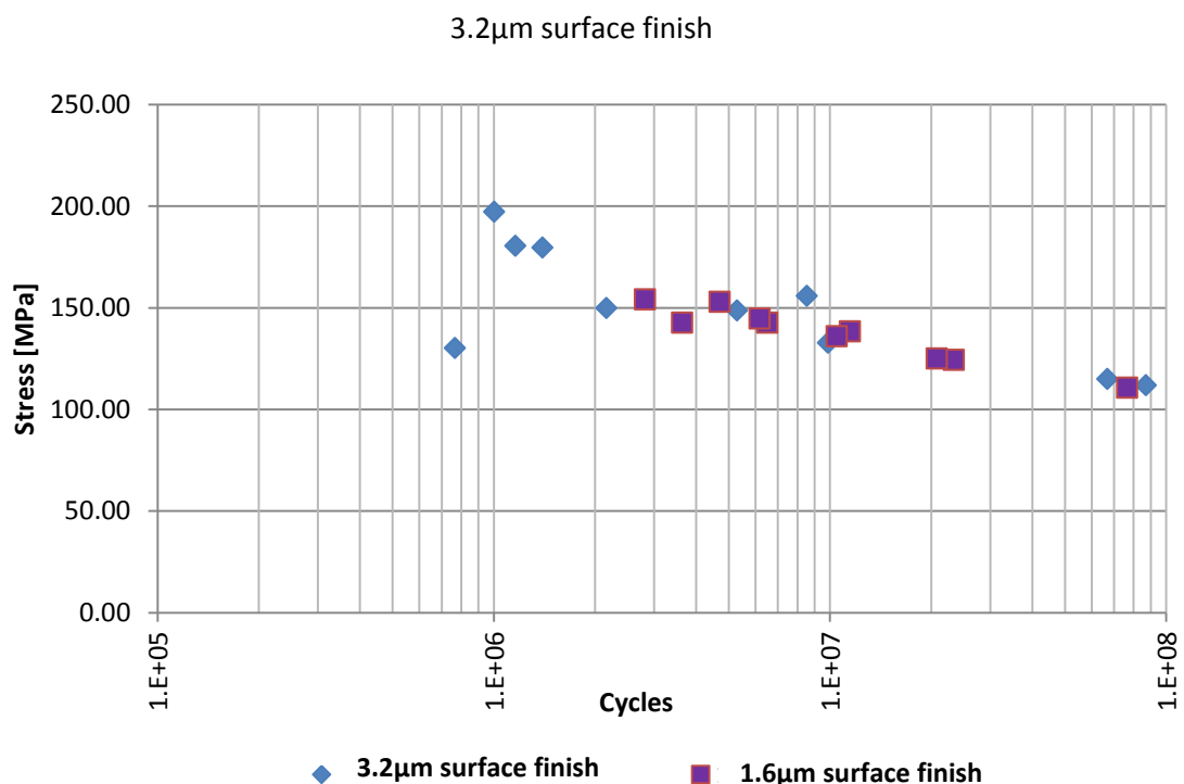
Figure 4-41: AL2024 comparison of surface finish
