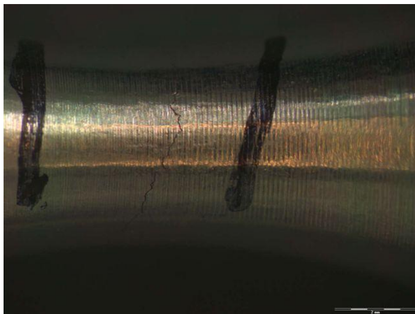
Figure 4-37: AL2024 specimen micrographic image of surface crack
