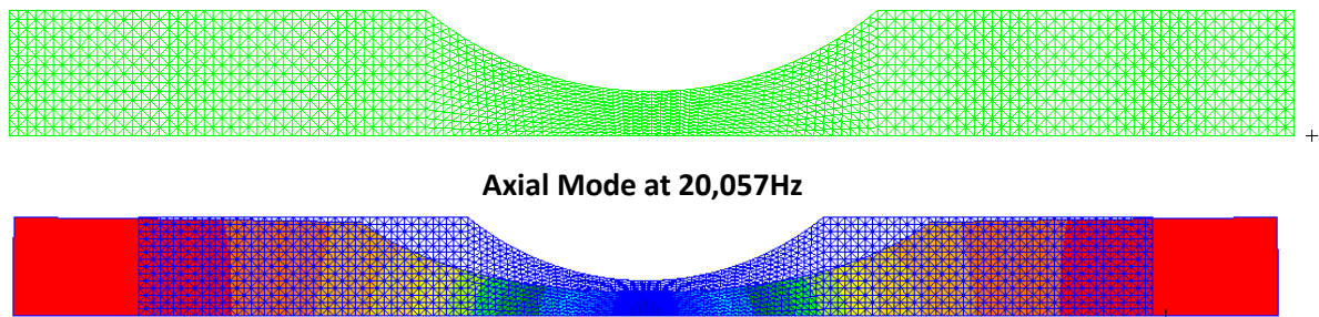
Figure 4-23: 2D Specimen model and applicable mode in 10 kHz to 30 KHz range
