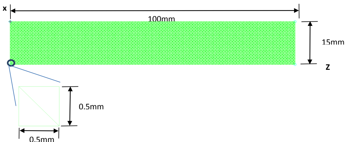
Figure 4-4: Axisymmetric Tria3 element model
