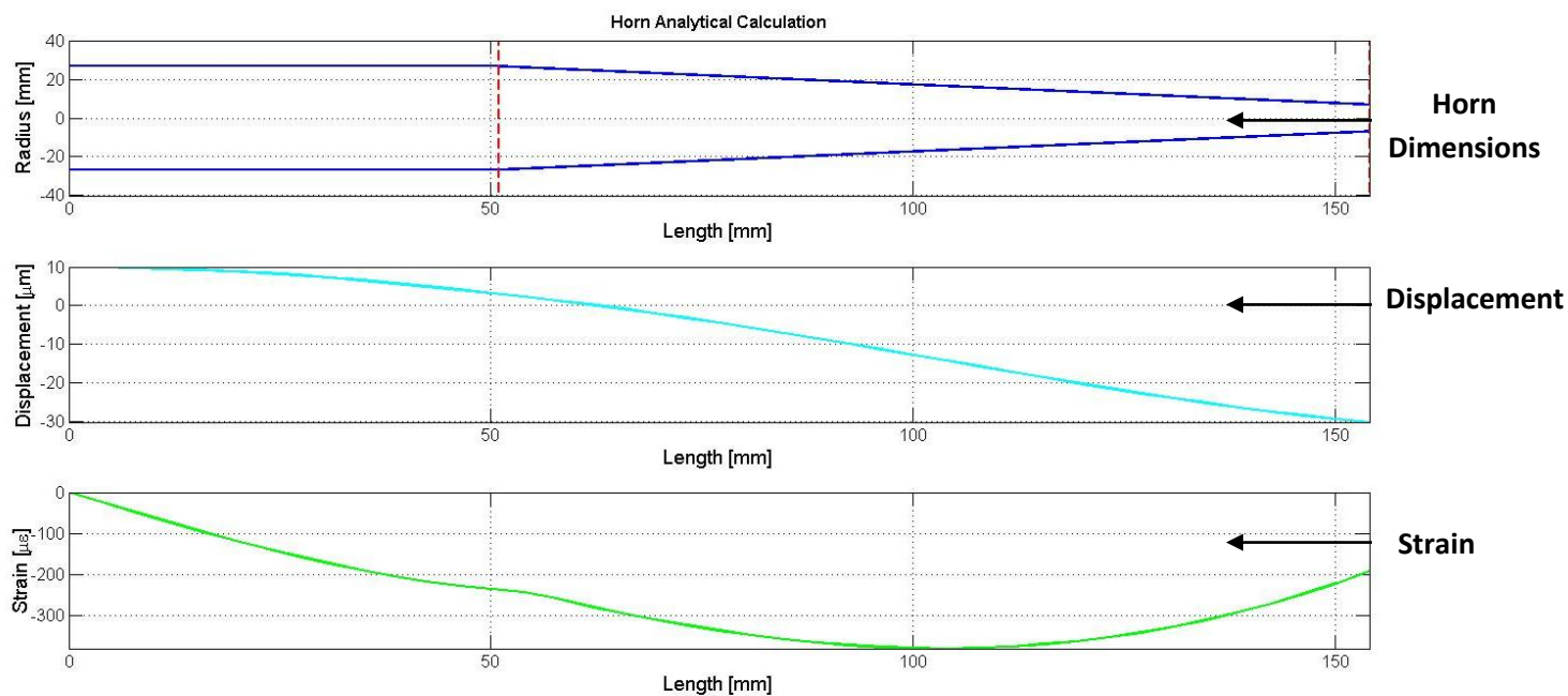
Figure 4-19: Analytical displacement and stress variation of horn length
