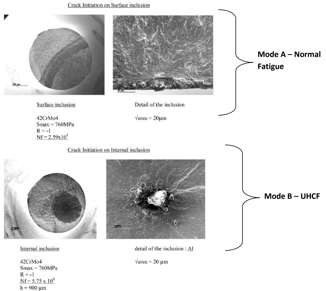
Figure 2-9: Crack initiation in surface inclusion and crack initiation in internal inclusion [9]
