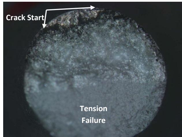
Figure 5-2: Micrographic image of AL2024 Specimen H1-S2-13
