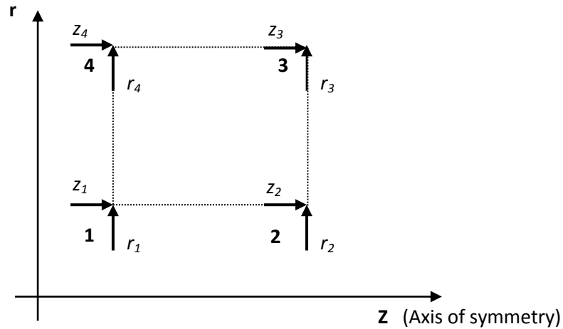
Figure C-12: Axis definition for an element
