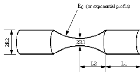
Figure 2-27: Geometry definition for specimen as defined by Bathias [4]
