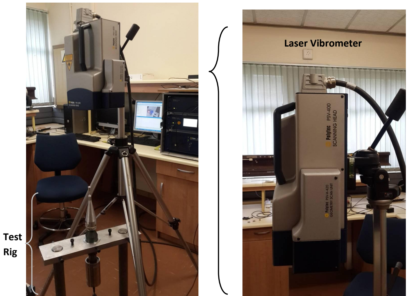
Figure 4-38: Mark 3 final setup
