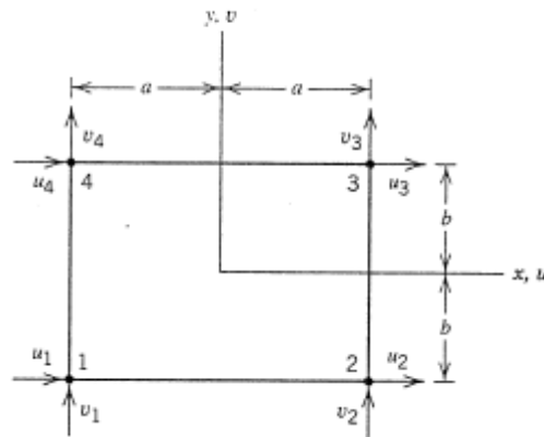
Figure C-1: Four node quadrilateral (Q4) [28]
