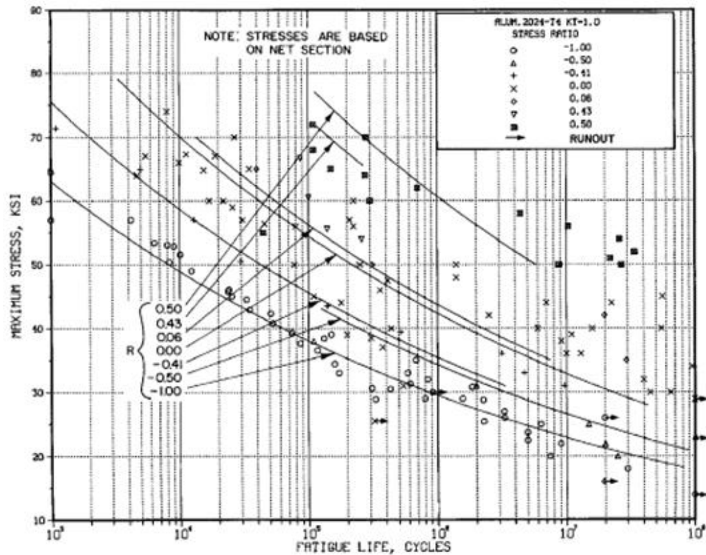
Figure 2-20: AL2024-T4 as per MMPDS [20]
