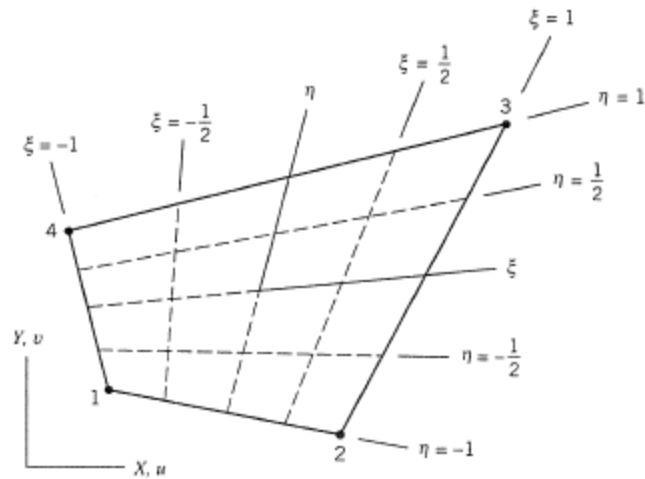
Figure C-2: Four node Isoperimetric quadrilateral (Q4) [28]
