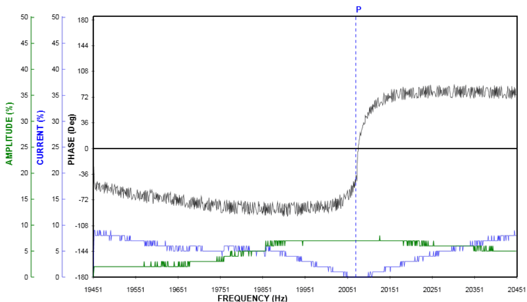
Figure 4-10: Typical horn natural frequency after gauges are applied
