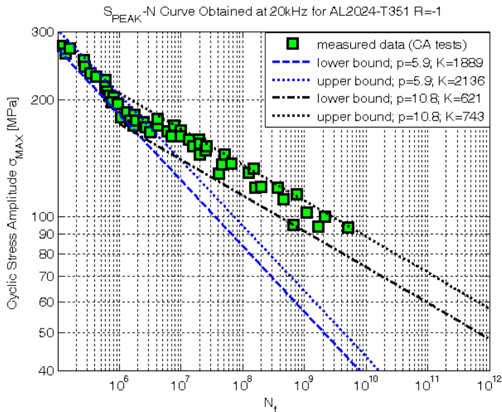
Figure 2-8: Haibach curve compared to Stanzl's UHCF data
