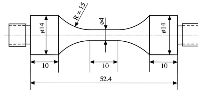
Figure 2-22: Specimen size for AL2024 data, Mayer [21]
