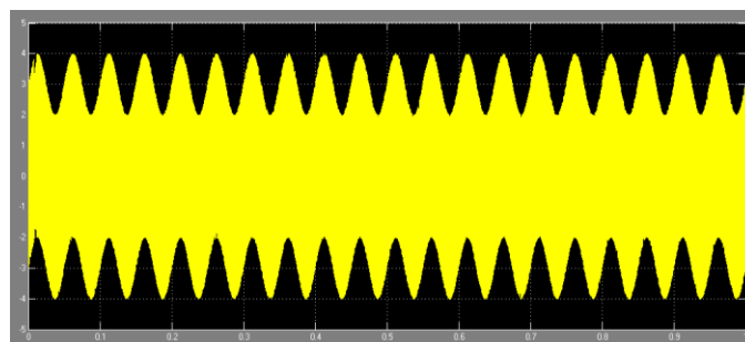
Figure D-3: Two input signals
