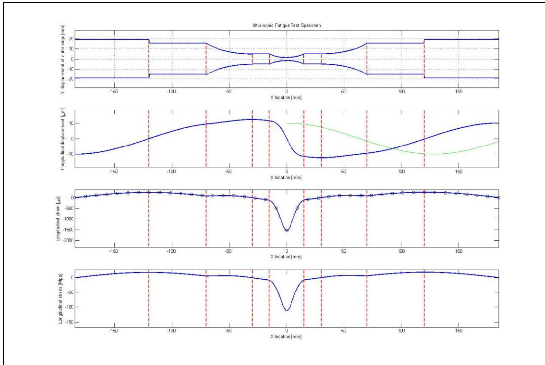
Figure A-4: Plot for 5 section specimen model variable geometry
