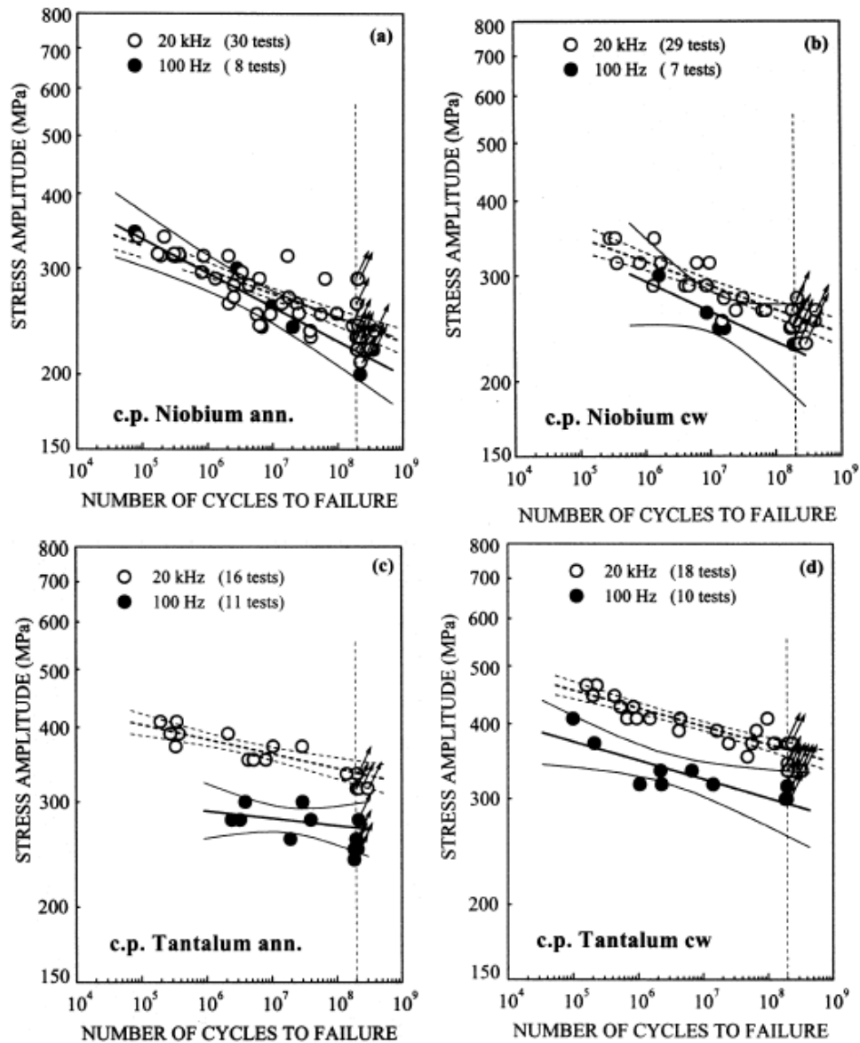
Figure 2-12: Endurance data of (a) commercially pure Niobium annealed and (b) commercially pure Niobium cold worked, (c) commercially pure Tantalum annealed and commercially pure Tantalum cold worked [15]
