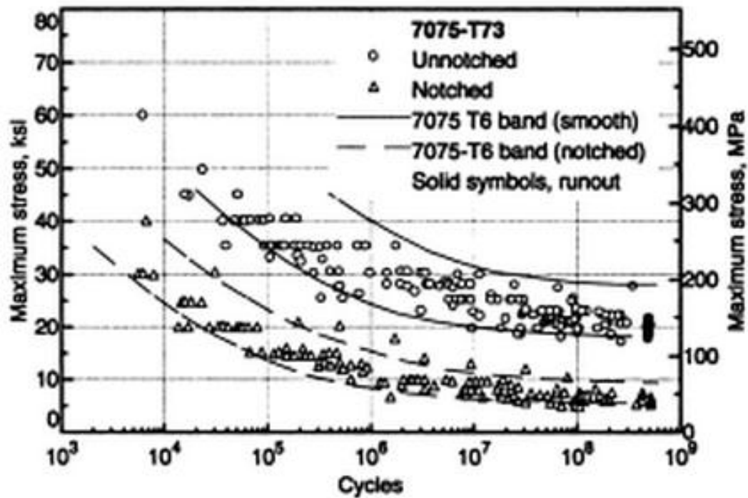
Figure 2-29: AL7075-T73 fatigue data [22]
