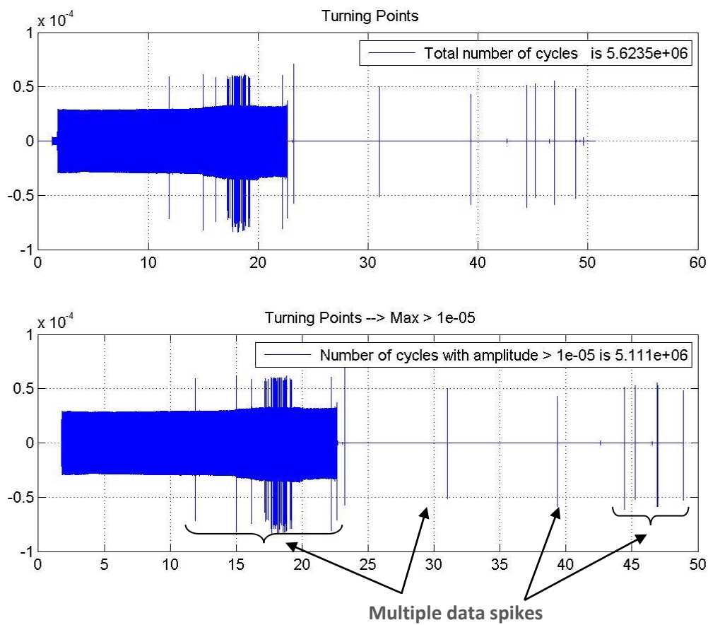
Figure 4-22: Laser vibrometer data for Al7075 horn and Al2024 test specimen 4
