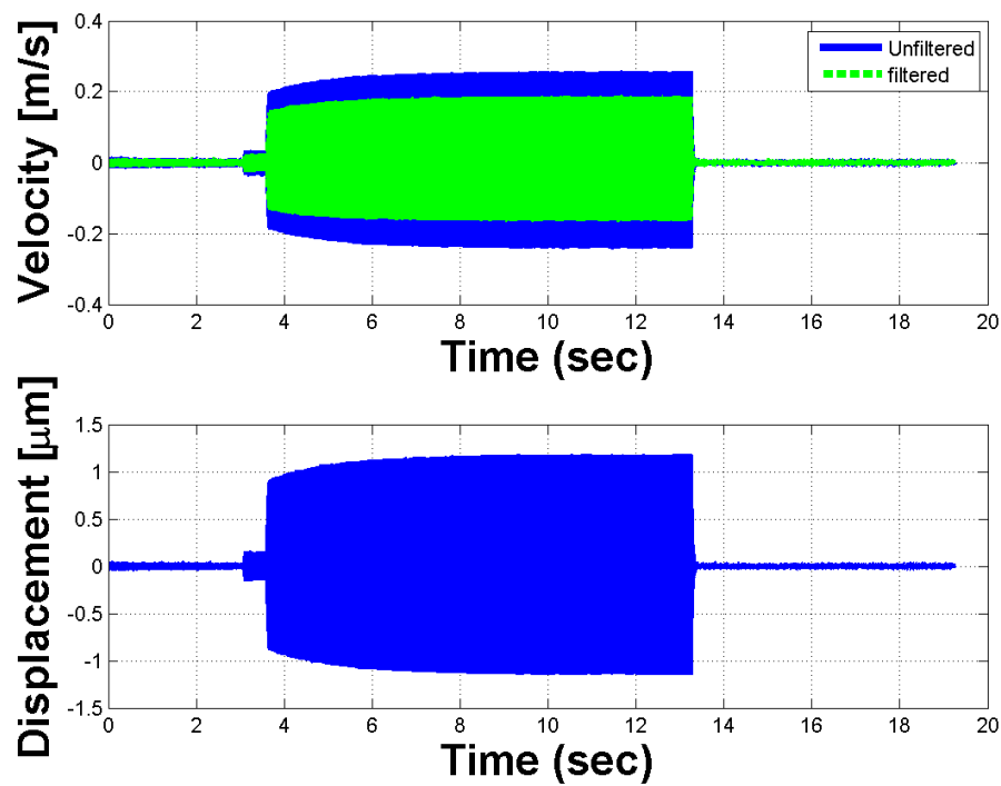
Figure 4-31: Booster coupling displacement
