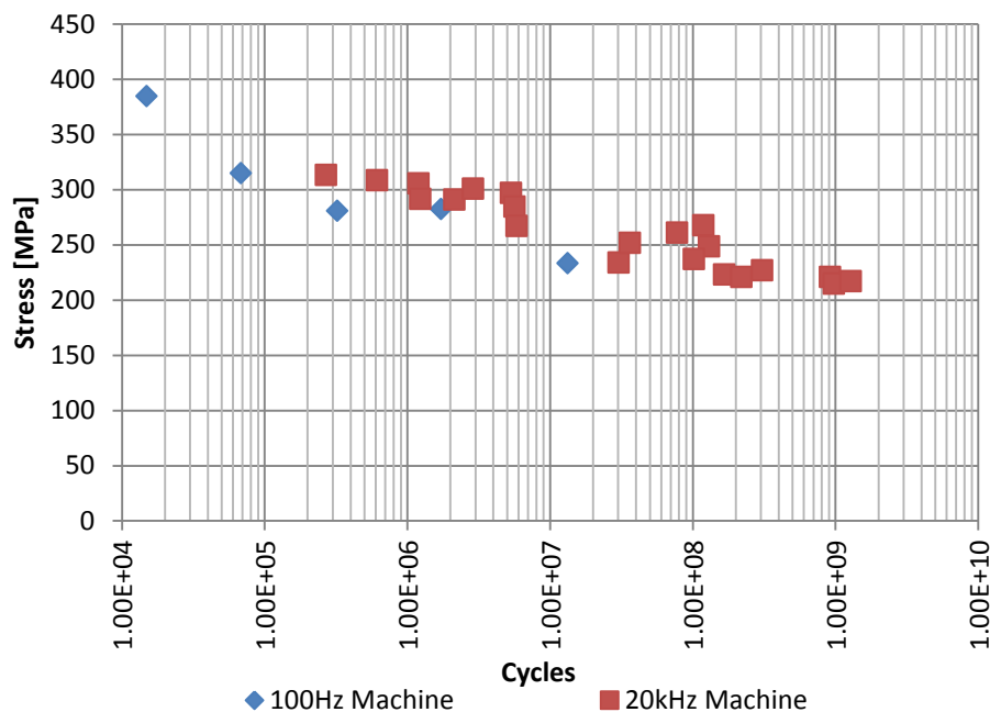
Figure 2-32: Papkyriacou data for AL7075 (AlZnMgCu1.5-T6) [16]
