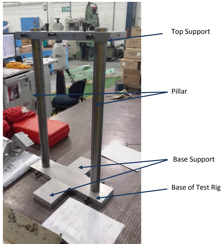
Figure 4-13: Test rig construction
