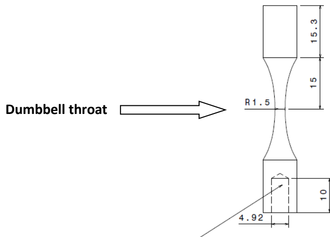
Figure 4-3: Mark 1 specimen sizing
