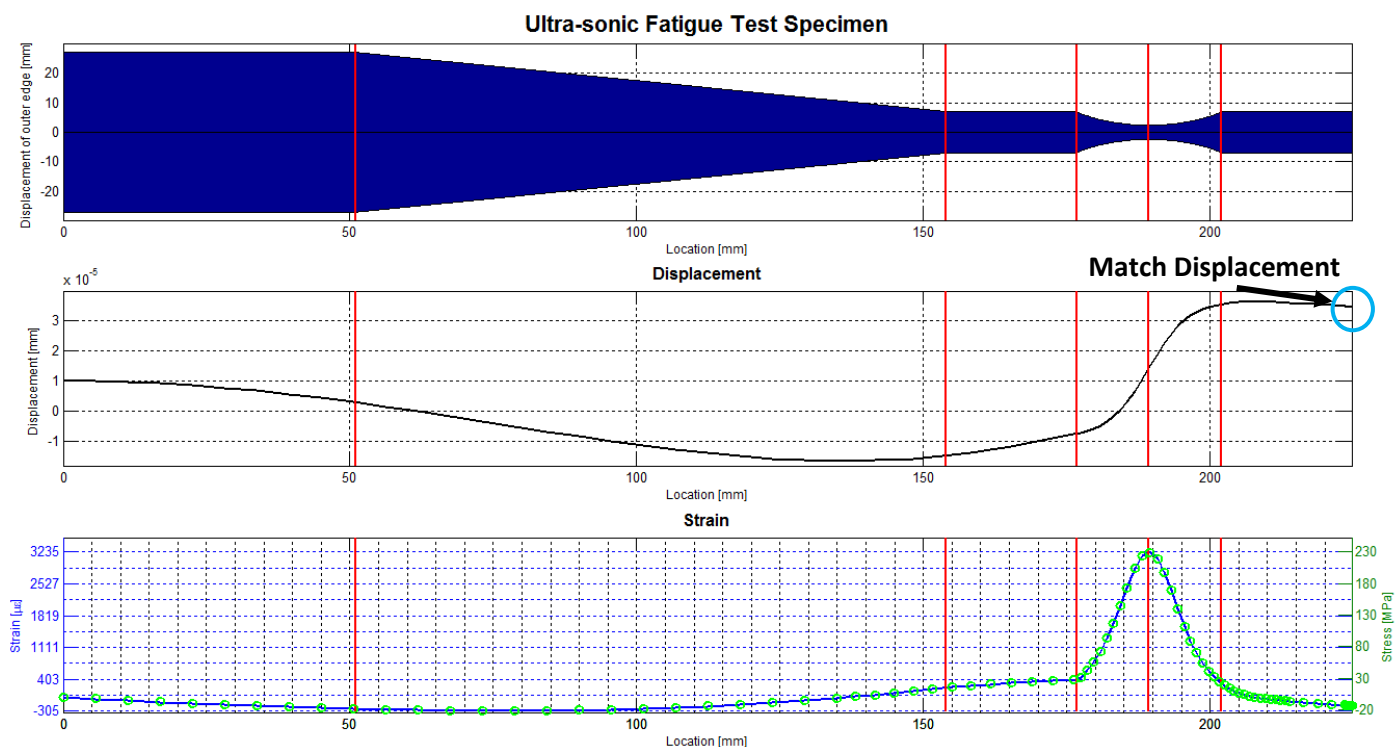
Figure 4-25: Typical displacement, strain and stress output
