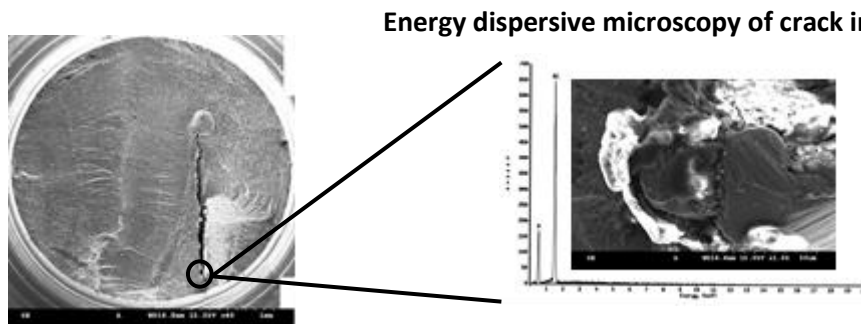
Figure 2-26: AL2024 cleavage fracture [14]
