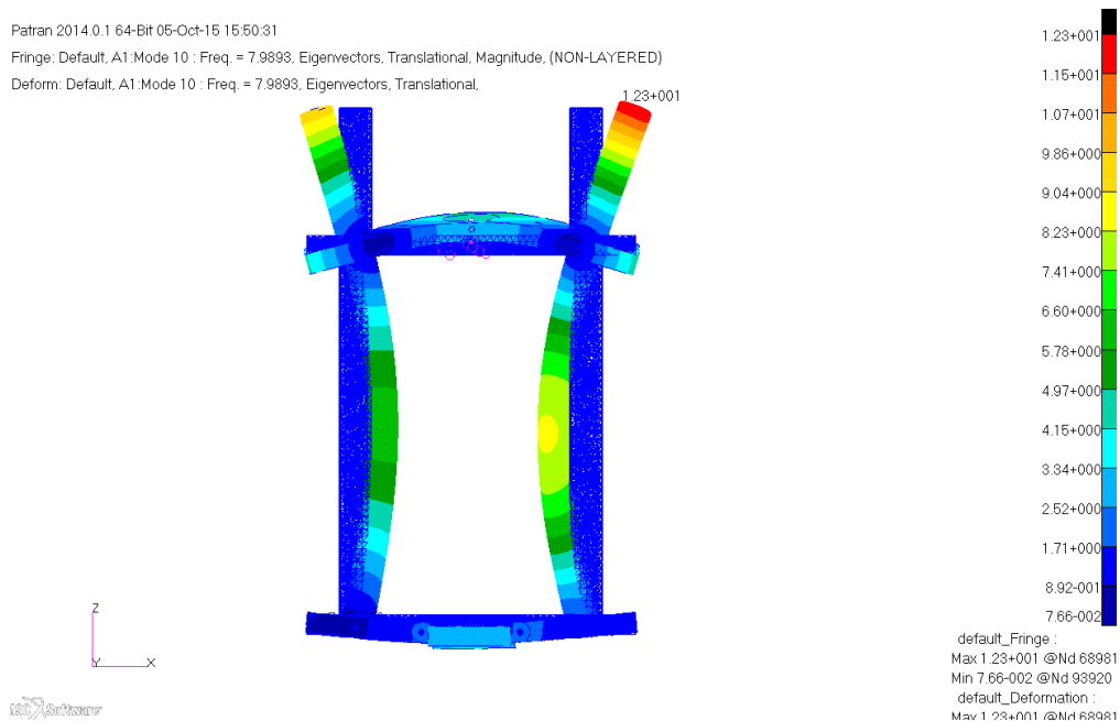
Figure 4-34: First bending mode of top support
