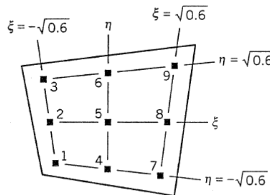
Figure C-7: Third order Gauss Quadrature node locations [28]
