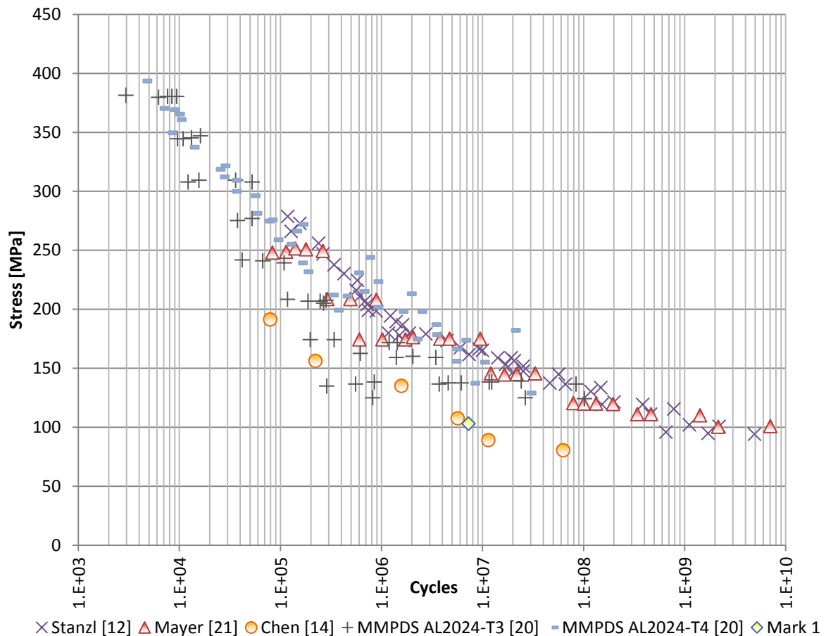
Figure 4-12: Proof of concept comparison to known data
