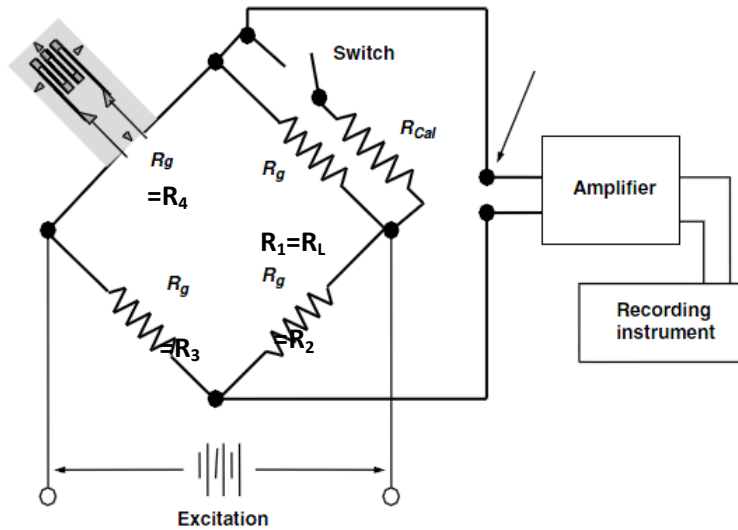
Figure B-6: Shunt resistor across R3 [27]
