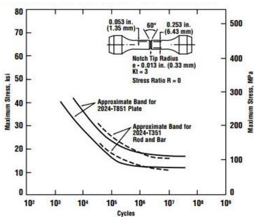
Figure 2-19: Data for AL2024 [19]
