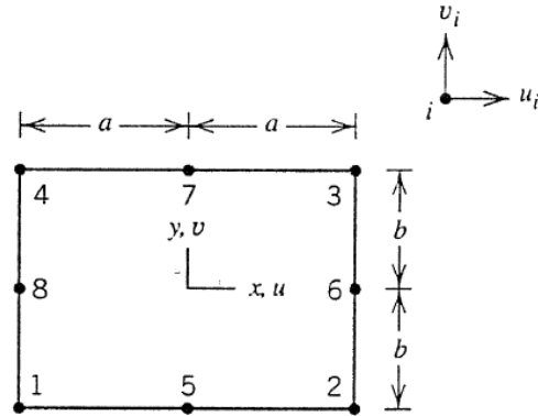
Figure C-8: General node number of quad8 element
