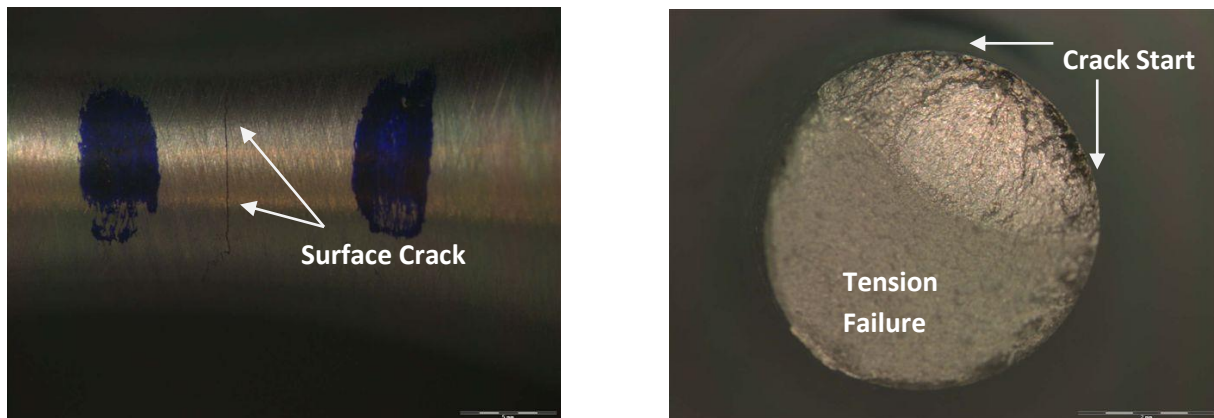
Figure 5-4: Typical failure of AL7075
