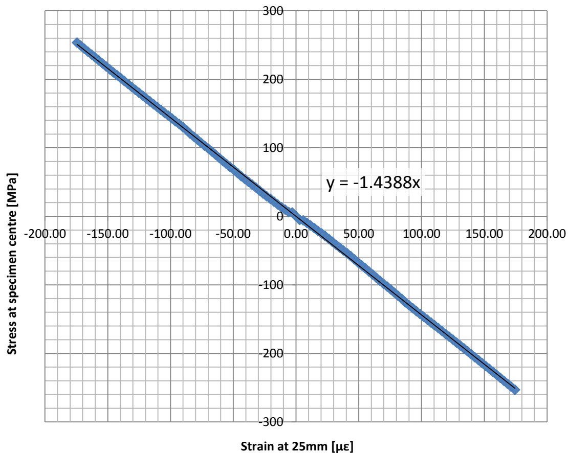
Figure 4-29: Strain gauge transfer function of AL2024
