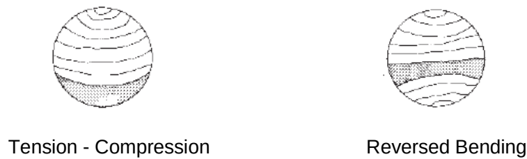
Figure 2-15: Typical failure method achieved during standard fatigue testing [18]
