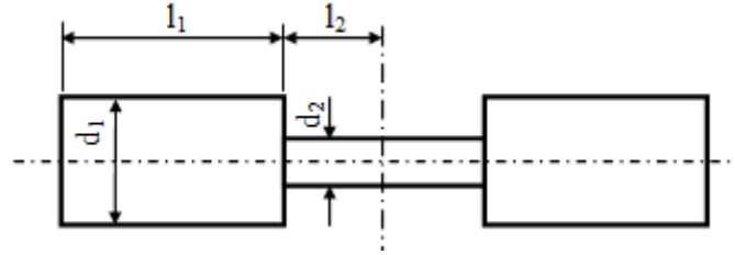
Figure 2-25: Dumbbell formula geometry definition [14]
