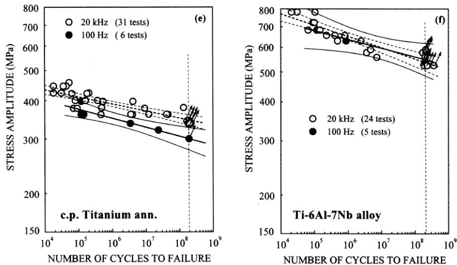
Figure 2-13: Endurance data for commercial pure anneal Titanium and Titanium [15]
