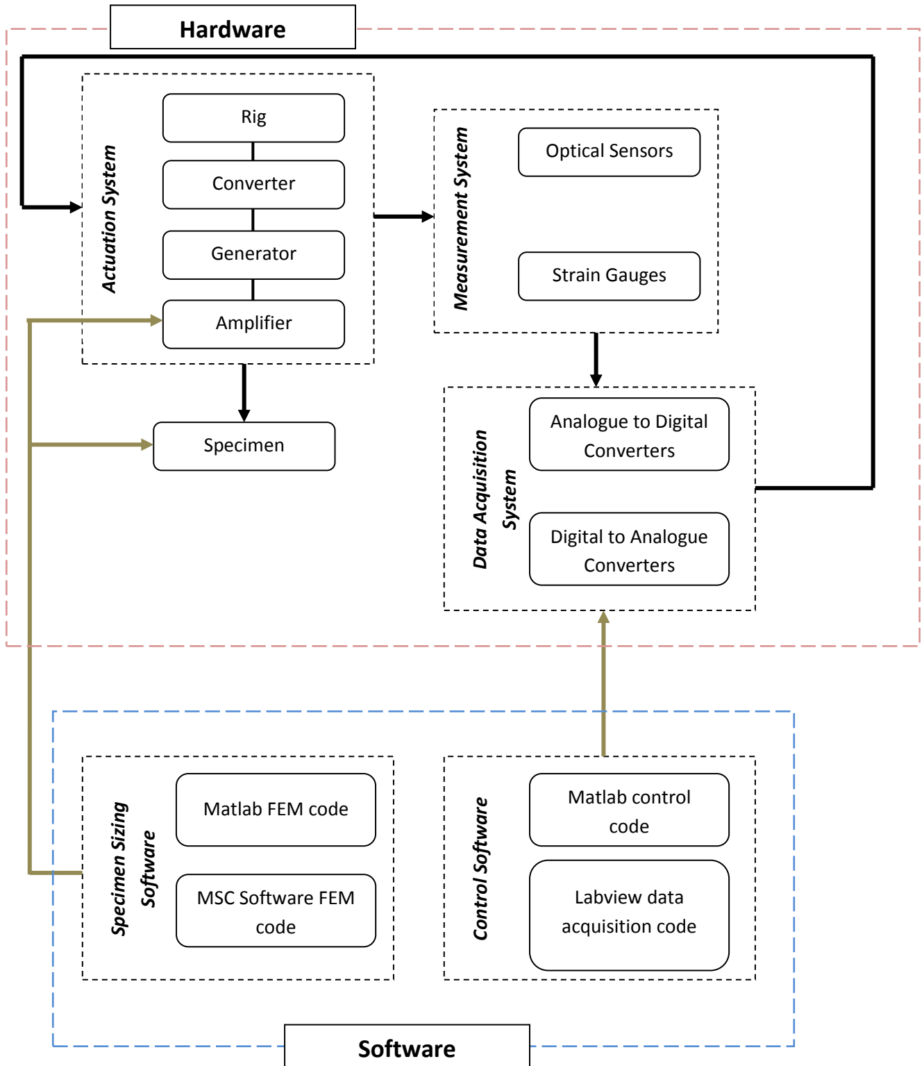
Figure 3-1: PRS for Design
