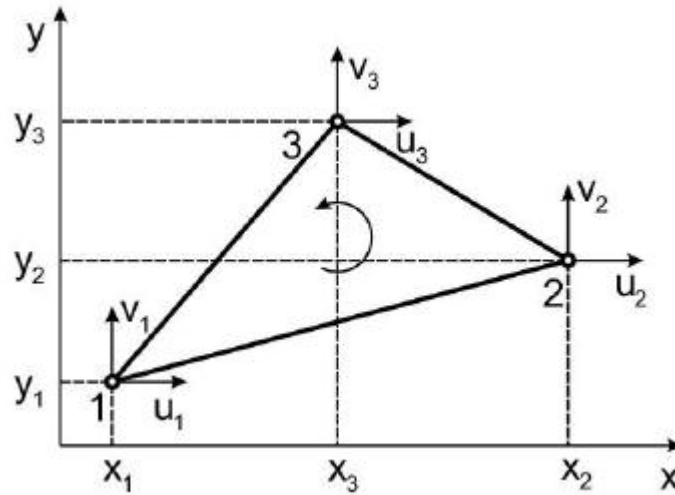
Figure C-13: linear triangle element nodal co-ordinates and displacement [30]
