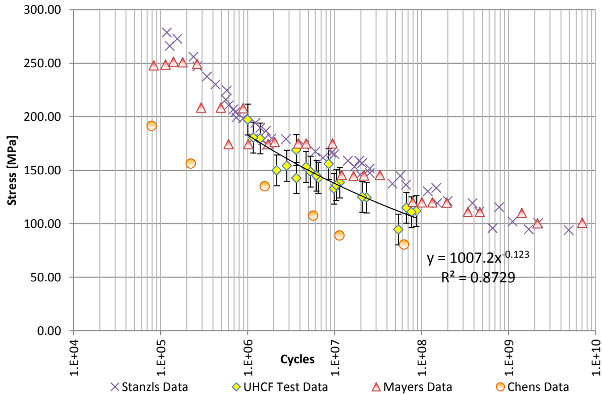
Figure 5-1: Comparison of AL2024-T351 Data
