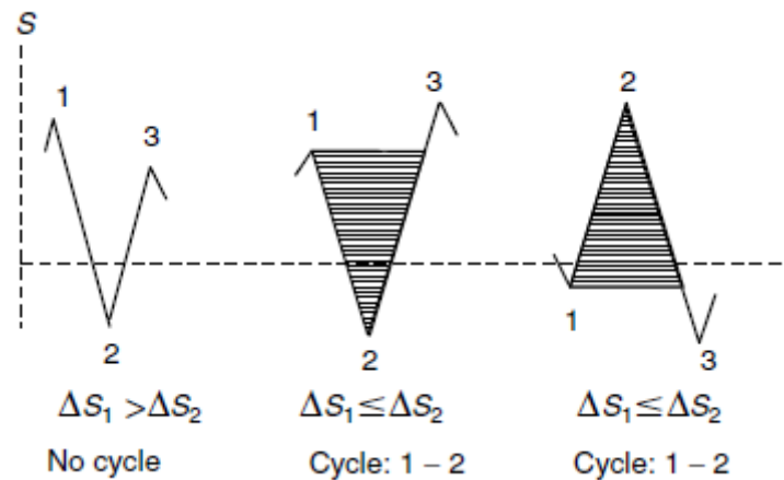
Figure 2-4: Three point Rainflow counting [5]
