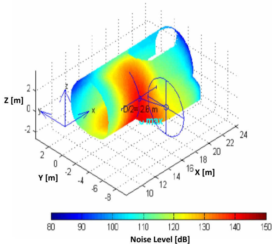
Figure 2-6: Typical pressure plot of one harmonic of the blade pass frequency
