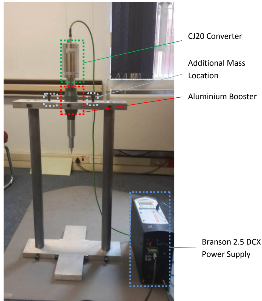
Figure 4-14: Test rig combined with the actuating system and power source
