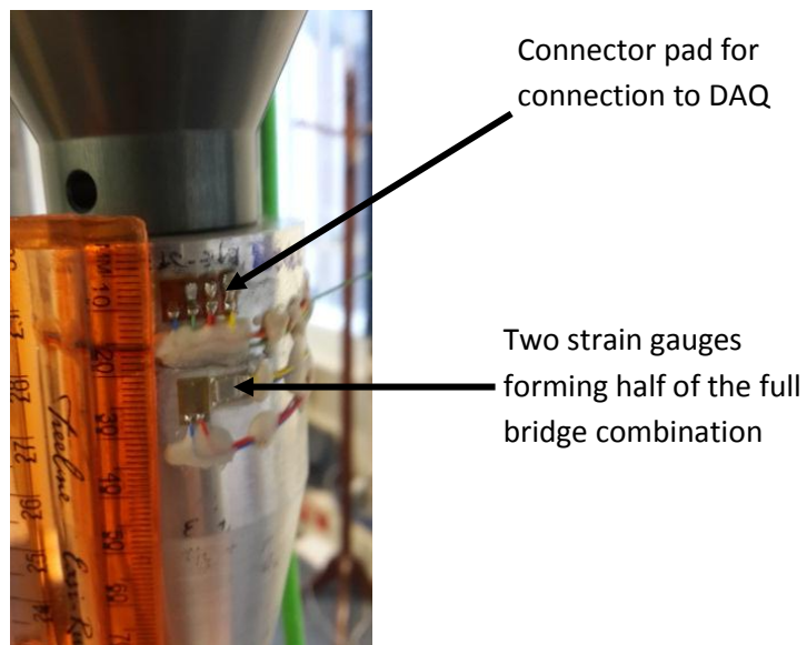
Figure 4-28: Strain gauge location on horn
