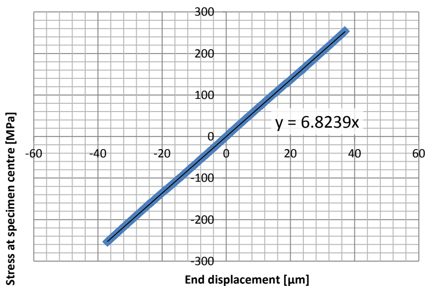
Figure 4-26: Laser vibrometer transfer function of AL2024
