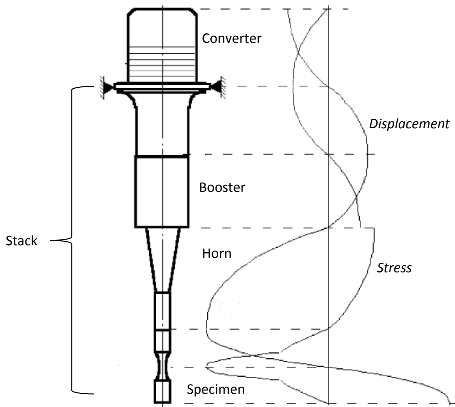
Figure 2-2: Variation of stress and displacement in a typical stack [4]
