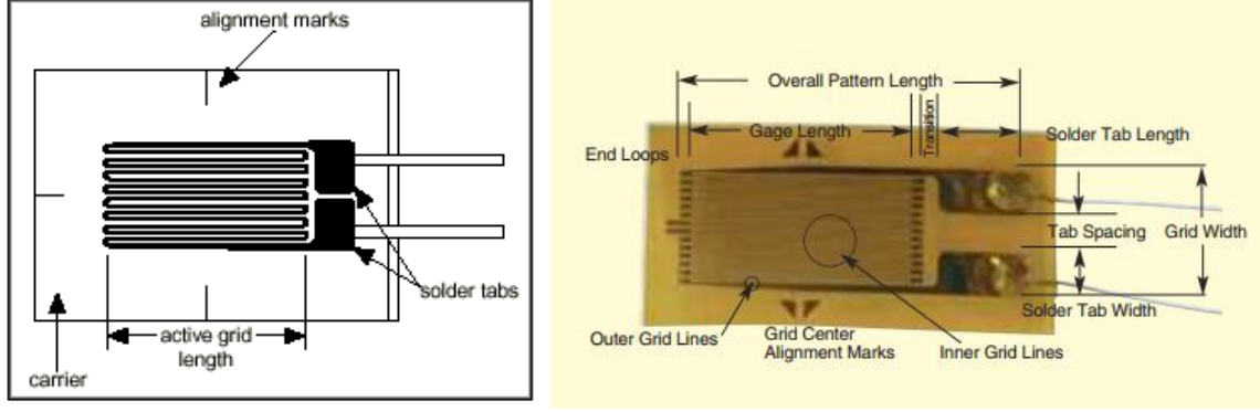
Figure B-2: Typical metallic bonded strain gauge [26] [27]
