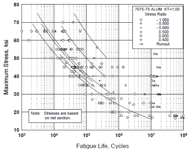
Figure 2-28: S/N curves for un-notched 7075-T6 aluminium alloy [20]
