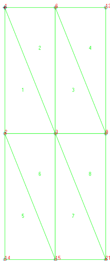
Figure C-16: Eight element verification model
