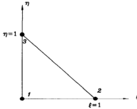
Figure C-11: Three node triangular element
