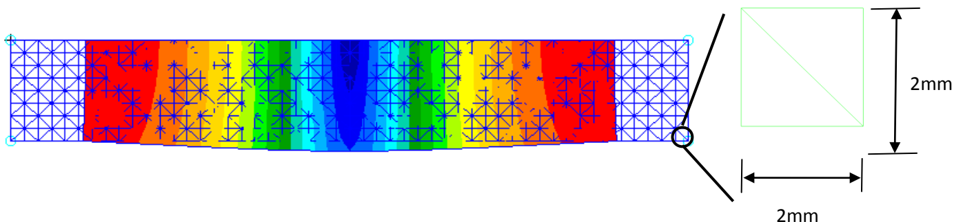
Figure 4-7: Mode shape and element size for 2mm square axisymmetric element
