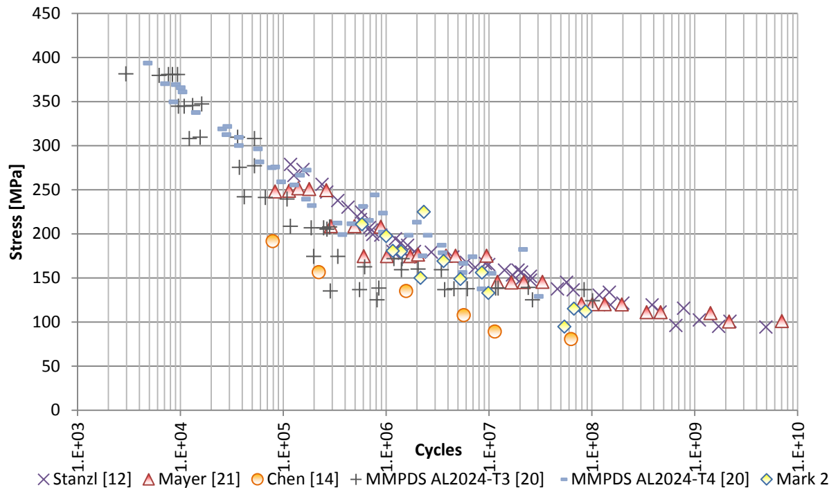
Figure 4-35: Mark 2 AL2024-T351
