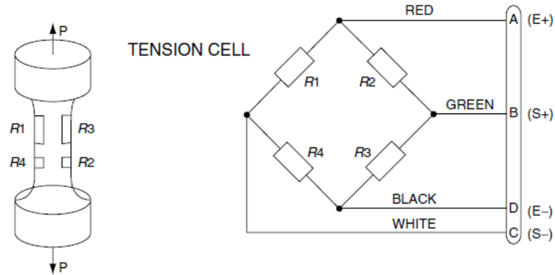
Figure B-4: Tension configuration [5]
