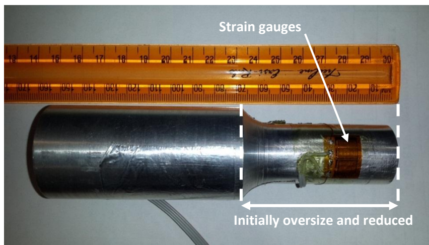
Figure 4-1: Mark 1 proof of concept horn with two gauges indicated
