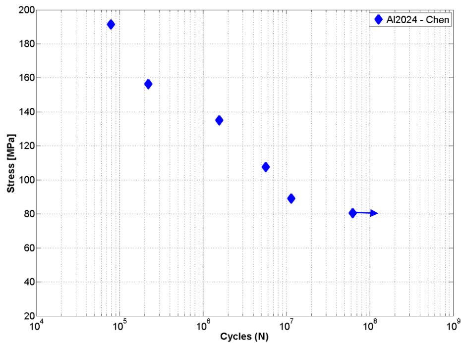
Figure 2-18: Fatigue data for aluminium 2024, Chen [14]
