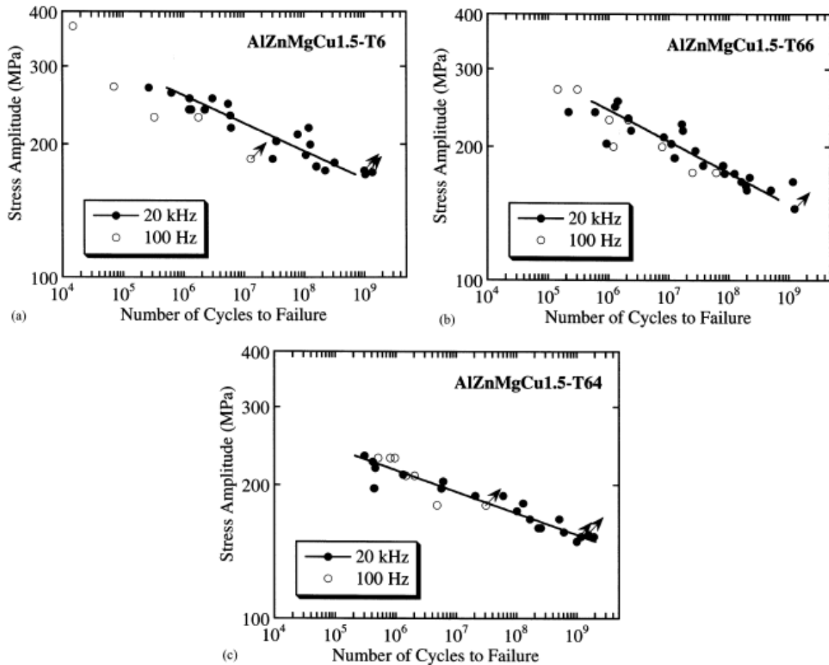
Figure 2-11: Endurance data T6 (a), T66 (b) and T64(c) at 20 kHz (dots) and 100Hz (circles) [16]
