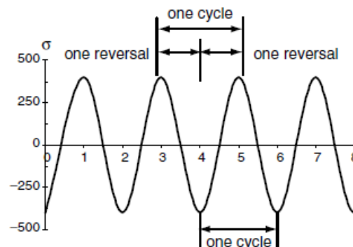
Figure 2-3: Constant cyclic loading [5]
