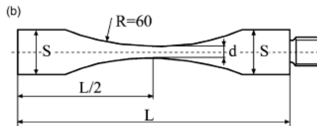
Figure 2-30: Aluminium 7075-UA typical specimen [23]
