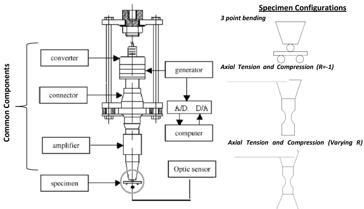
Figure 2-1: Typical ultrasonic fatigue testing system [2]
