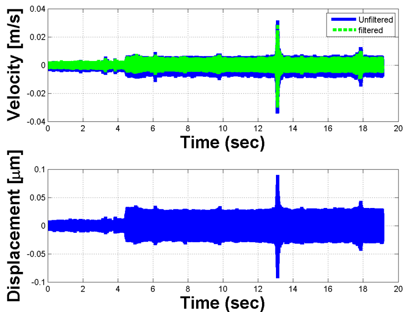
Figure 4-33: Right pillar displacement
