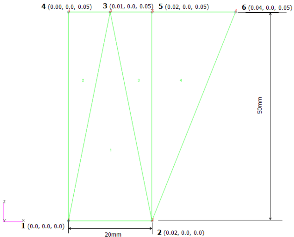
Figure C-15: Four element verification model
