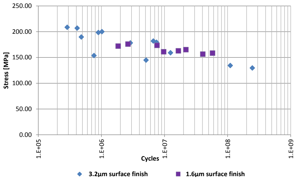
Figure 4-42: AL7075 variation due to surface finish
