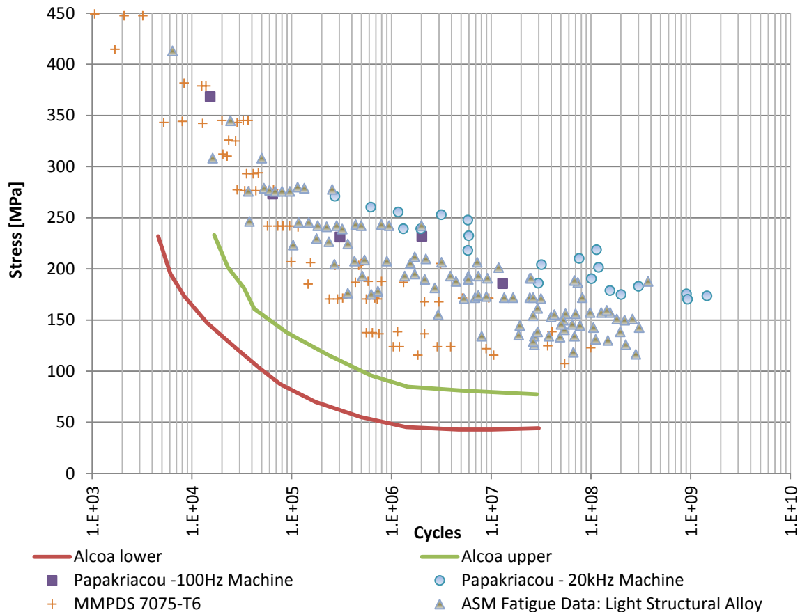
Figure 2-33: AL7075 combined data
