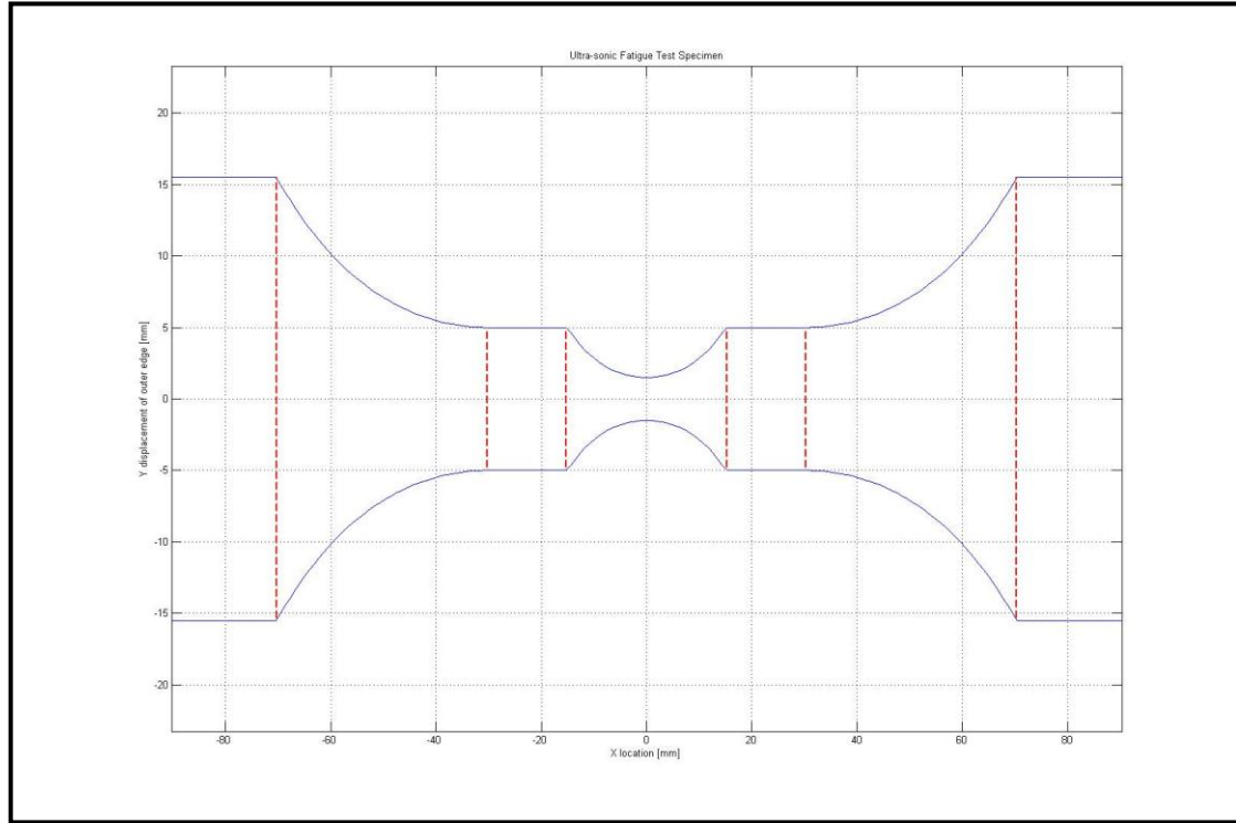
Figure A-2: Profile plot of specimen using Matlab
