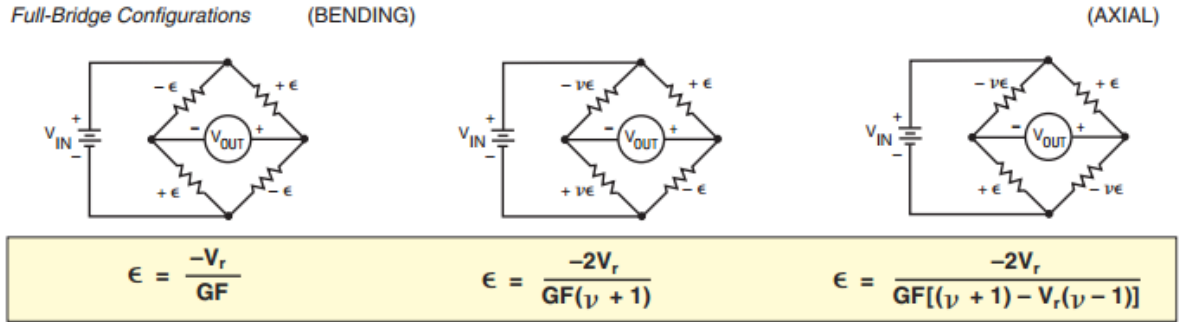
Figure B-3: Full bridge configuration [27]
