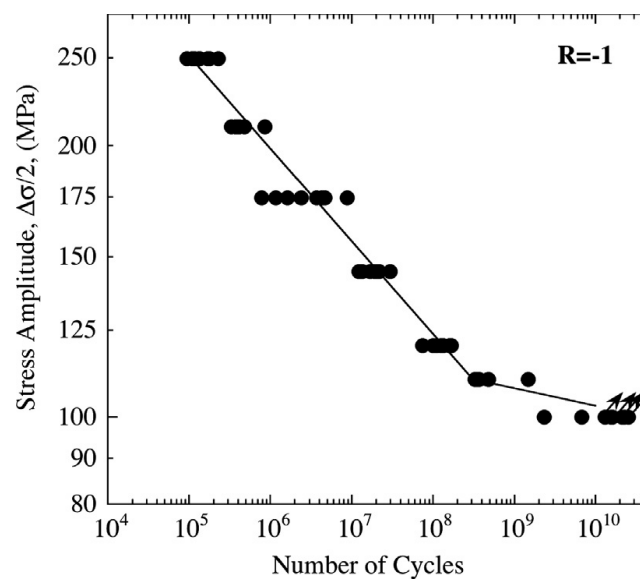
Figure 2-23 AL2024 data for load ratio of -1, Mayer [21]
