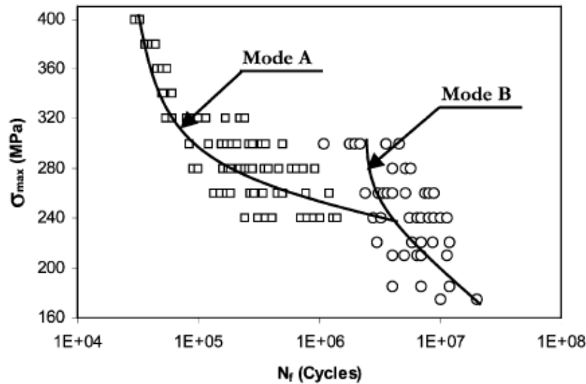
Figure 2-10: S-N curve of aluminium alloy 2024/T3; R=0.1 [1]
