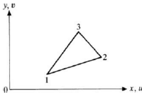
Figure C-9: Linear triangle
