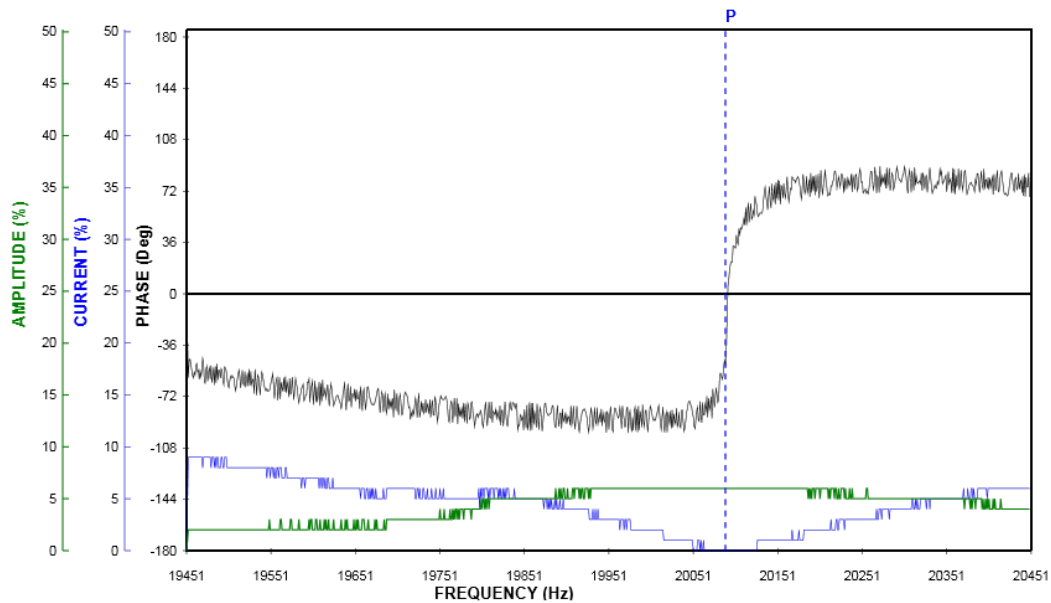
Figure 4-9: Typical horn natural frequency before gauges are applied
