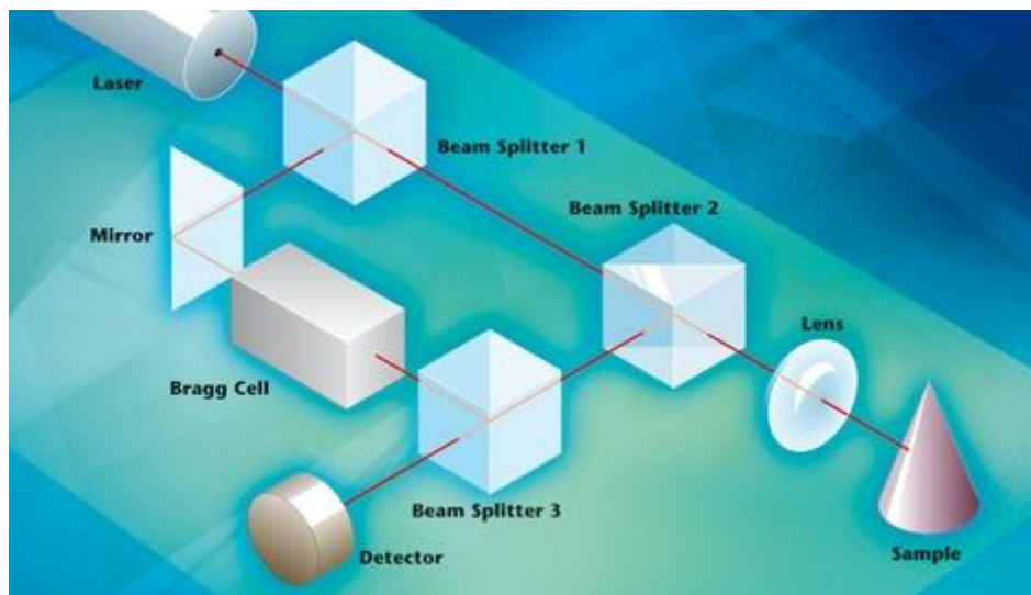
Figure B-1 : Laser vibrometer internal setup [25]
