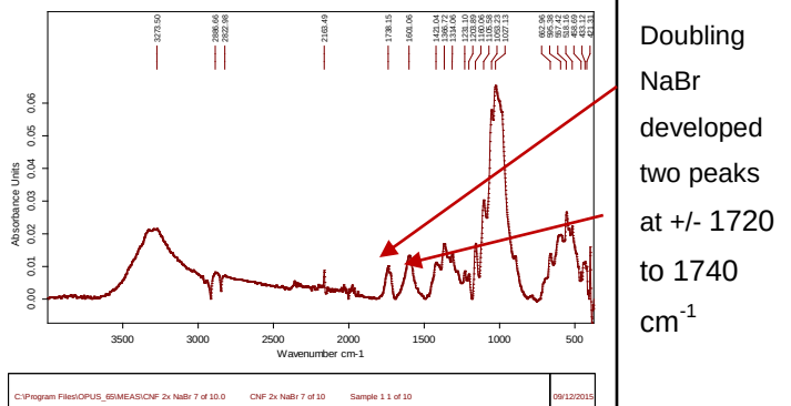
Figure 4.16: Spectrum of cellulose when the NaBr concentration was doubled
