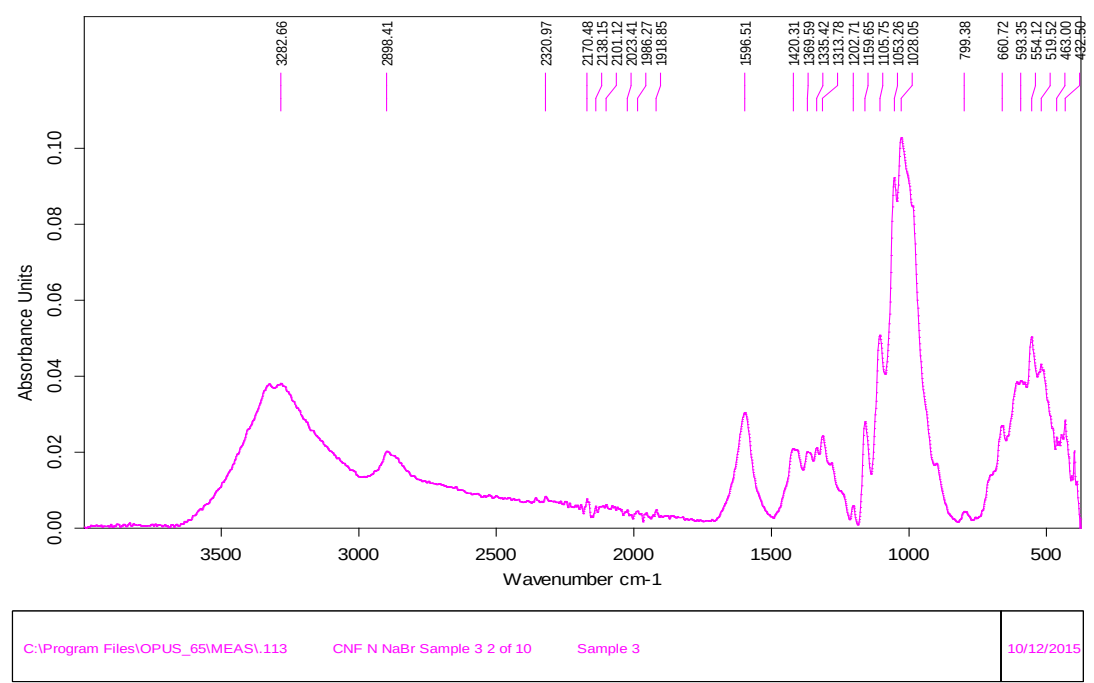
Figure B.2: FTIR Spectra of normal NaBr concentration
