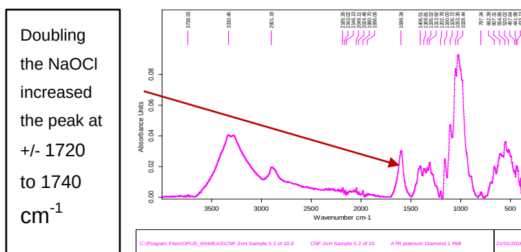
Figure 4.15 Spectrum of cellulose when the NaOCl concentration was doubled
