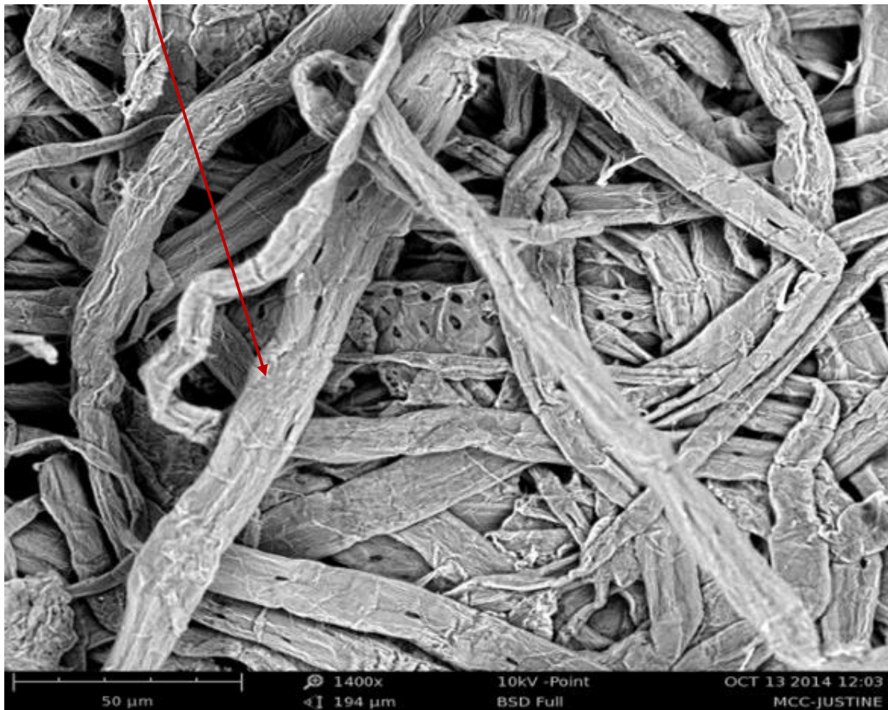
Figure 4.3: SEM image of unrefined E. grandis pulp, 1400x resolution
