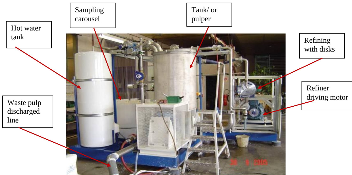
Figure 3.1: Photograph of the Pilot refiner
