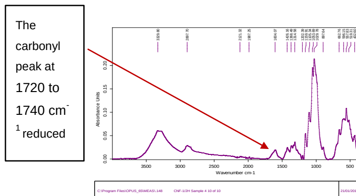
Figure 4.13: FTIR spectrum of cellulose when the NaOCl concentration was halved
