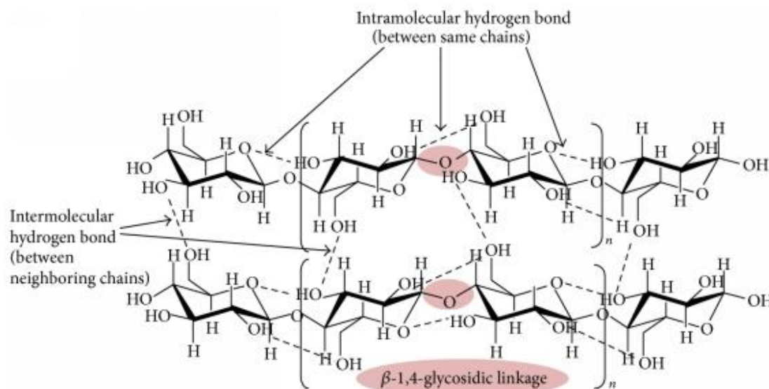
Figure 2.4: Chemical structures in cellulose chains (Lee et al., 2014).
