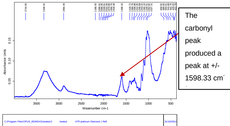
Figure 4.12: FTIR spectrum of oxidized cellulose after six hours
