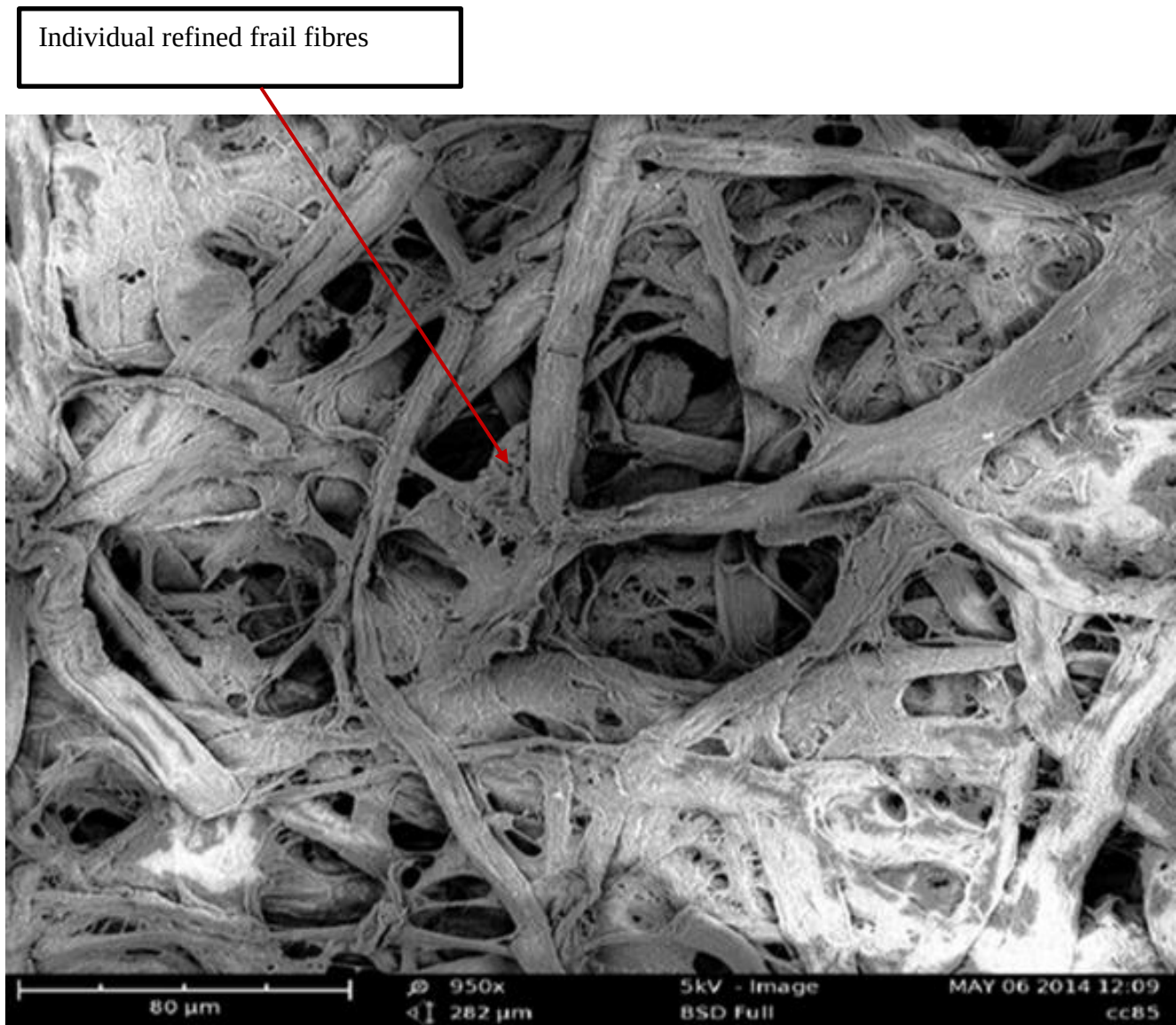
Figure 4.4: SEM image of mechanically refined E. grandis pulp, 950x resolution
