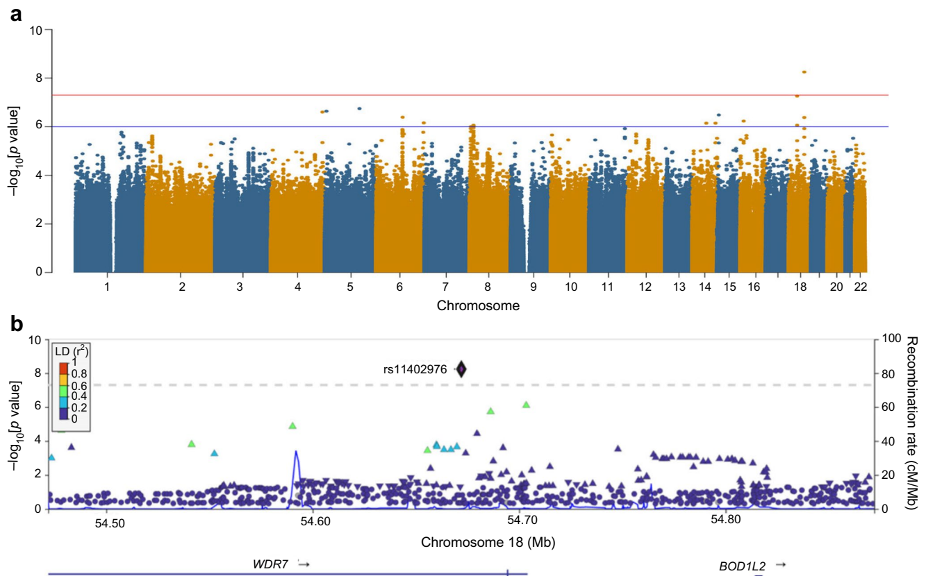
Fig. 2 (a) Manhattan plot for the FI GWAS. The red horizontal line indicates the genome-wide significance threshold ( p=5 \times 10^{-8} ); the blue horizontal line shows the suggestive significance threshold of p=1 \times 10^{-6} . (b) Regional plot of chromosome 18 ( WDR7 and BOD1L2 gene region) showing associations with FI in the African AWI-Gen cohort: the lead SNP (rs11402976) is shown as a black
