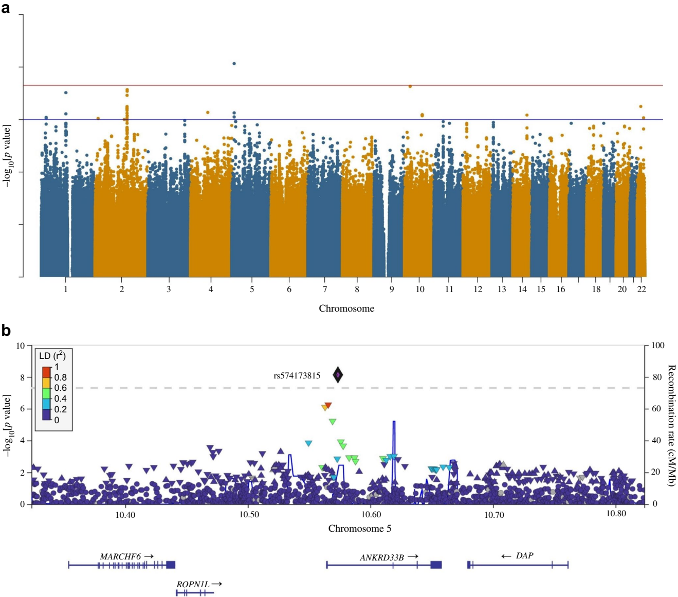
Fig. 1 (a) Manhattan plot for the FG GWAS. The red horizontal line indicates the genome-wide significance threshold ( p = 5 \times 10^{-8} ); the blue horizontal line shows the suggestive significance threshold of p = 1 \times 10^{-6} . (b) Regional plot of chromosome 5 (including the ANKRD33B gene region), showing association with FG in the African AWI-Gen cohort: the lead SNP (rs574173815) is shown as a
