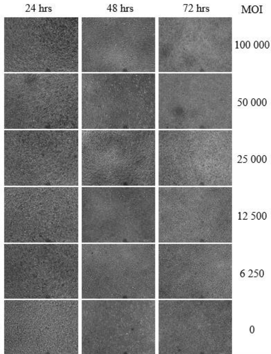
Supplementary Figure 8: Corresponding bright field images for the relative transduction efficiency of the rAAV-GFP vector in vitro . HEK293 T cells were infected in duplicate at various MOIs (range 100 000 - 0). The bright field images were taken at 24, 48, and 72 hours post-transduction (exposure time 5 ms). Magnification = 100x.
