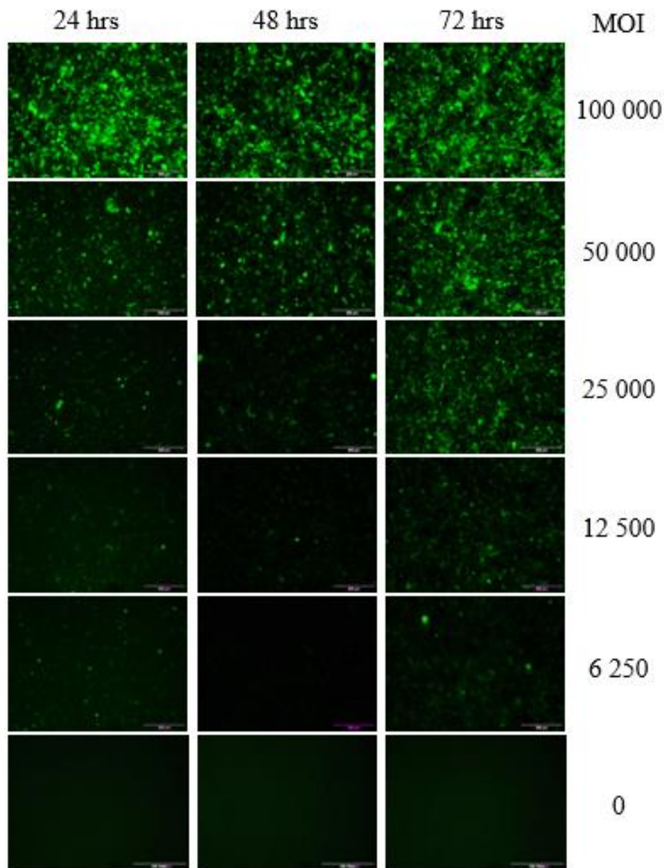
Figure 3.12: Relative transduction efficiency of the rAAV-GFP vector in vitro . HEK293 T cells were infected in duplicate at various MOIs (range 100 000 - 0). GFP expressed was monitored was fluorescent microscopy of infected HEK293 T cells: 24, 48, and 72 hours post-transduction (exposure time 2 000 ms). Magnification = 100x. Scale bar (lower right corners) = 200 \mu m.
