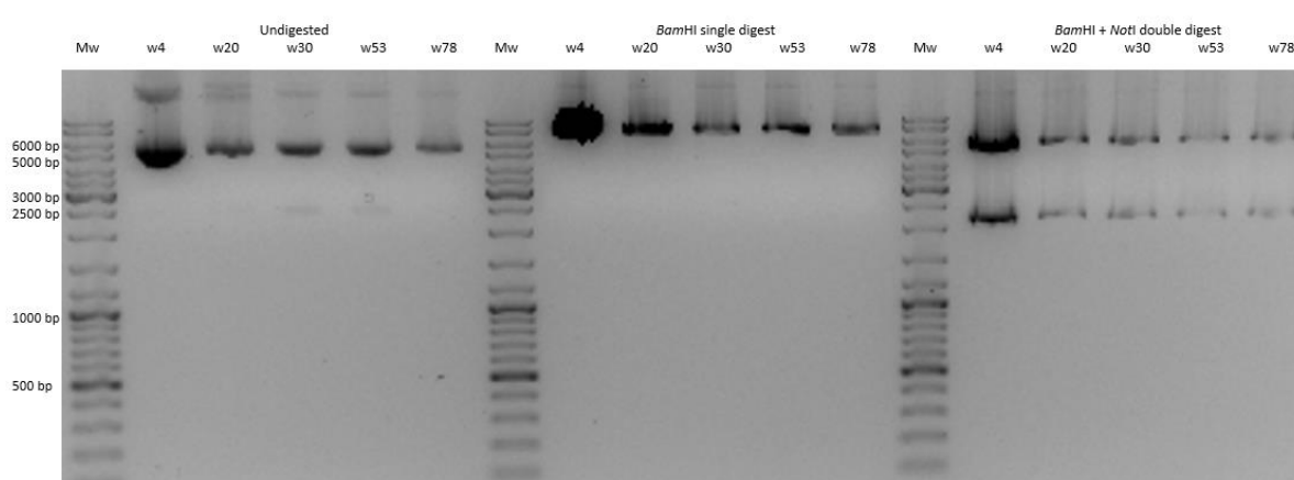
Figure 3.3: Restriction enzyme digest analysis of the pcDNA3.3wngp140 expression vectors. All DNA samples were resolved on a 1% agarose gel and visualised under UV light following ethidium bromide staining. The undigested DNA was run as a negative control. All 5 plasmids were digested with Bam HI alone (one restriction site); or Bam HI and Not I in a double digest reaction. w4-w78 corresponds to the CH505 HIV-1 Env isolate weeks post infection, described previously. The O'Gene Ruler DNA ladder (Thermo Fisher Scientific, Waltham, MA, USA) was used as a reference molecular weight marker (Mw) bands are indicated on the left of the image in base pairs (bp).
