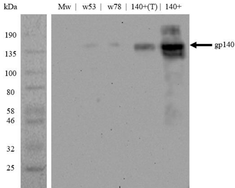
Figure 3.4: Western Blot analysis of FVgp140 and selected CH505gp140 envelope glycoproteins.
