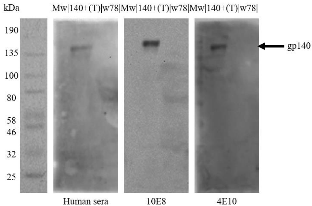
Figure 3.5: Western Blot analysis of FVgp140 and CH505gp140w78 envelope glycoproteins. Following transient transfections of HEK293 T cells, unpurified cell culture supernatants were analysed via Western blot. Protein expression was confirmed by probing for Env using 10E8, 4E10, or HIV-1 positive patient sera as a primary antibody (diluted 1: 1 000). Subsequent detection of primary antibody was done using a horse radish peroxidase (HRP)-conjugated anti-human secondary antibody (diluted 1: 2 000). Mw- prestained protein marker, broad range (New England Biolabs® Inc., MA, USA) and corresponding bands are indicated on the left in kilodaltons (kDa). Photograph of the pre-stained molecular weight standard on nitrocellulose membrane taken under white light.
