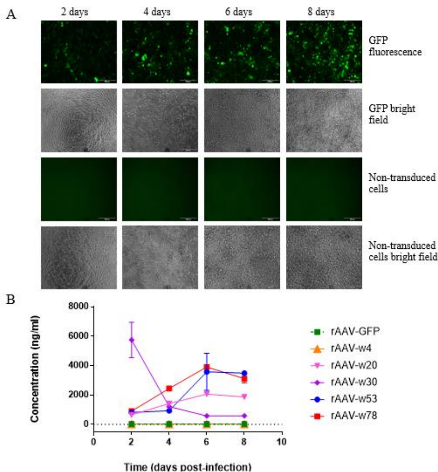
Figure 3.13: rAAV transduction and recombinant Env glycoprotein evaluation in HEK293 T cell line. HEK293 T cells were infected in duplicate at an MOI of 50 000 using the rAAV vectors. GFP expression from the rAAV-GFP vector was monitored by fluorescent microscopy at: 2, 4, 6, 8 days post-transduction (exposure time 2 000 ms). Supernatant was collected from all the assayed wells at the same time points and replaced with fresh media. Magnification = 100x. Scale bar (lower right corners) = 200 \mu m. (A) Relative transduction efficiency of the rAAV-GFP vector in vitro . GFP fluorescent and brightfield images for the cells transduced with the rAAV-GFP, and for the non-transduced (control) cells were taken at the indicated timepoints. (B) ELISA showing the relative concentrations of rAAV vectors over 8 days. The GFP and CH505-Env proteins produced from the respective rAAVs were tested for interaction with the IgG1b12 primary antibody. Each well was tested in duplicate to obtain an average absorbance and standard deviation was used to calculate error bars. The bound antibodies were detected using an HRP-conjugated, anti-human IgG antibody and established TMB/ stop solution chromogenic methods.
