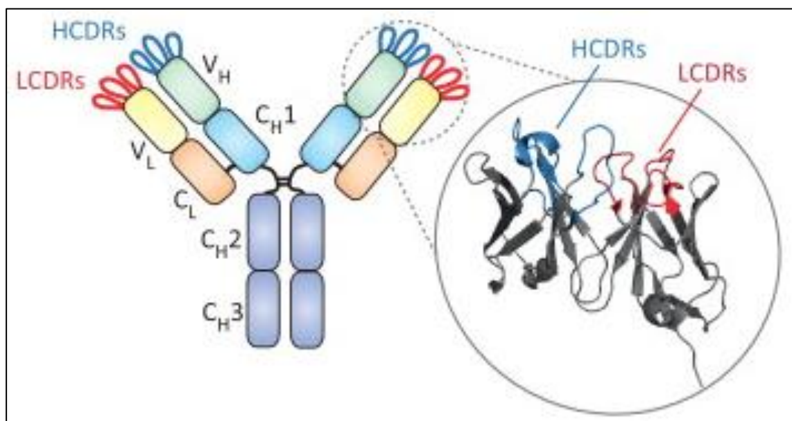
Figure 1.4: Schematic representation of a typical antibody structure. The heavy (H) and light (L) chains are indicated, along with the constant (C) and variable (V) regions. The complementarity-determining regions (CDR) are indicated for the heavy and light chains. Figure obtained from [186].
