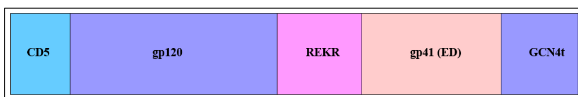
Figure 3.2: A schematic representation of the engineered trimeric Env constructs ( wngp140 ) used for this study. The gp140 constructs comprised the full gp120 sequence (gp120) and the gp41 ectodomain (ED; residues 522-693) sequence, with an intact cleavage site (REKR (+)), and a heterologous trimeric GCN4 leucine zipper sequence (GCN4t) fused to the C-terminus of the gp41 ED. The native Env leader sequence was replaced with the heterologous human CD5 antigen leader peptide (CD5) at the gp120 N-terminus.
