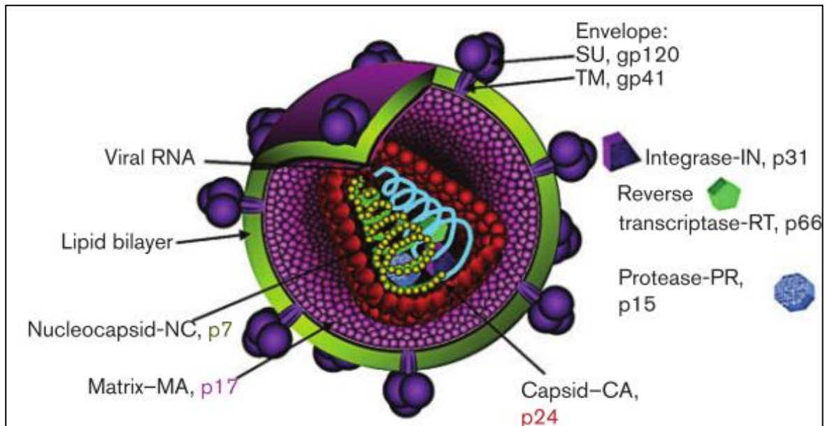
Figure 1.2: Structure of the HIV-1 virion showing the associated viral proteins. Image obtained from [22].
