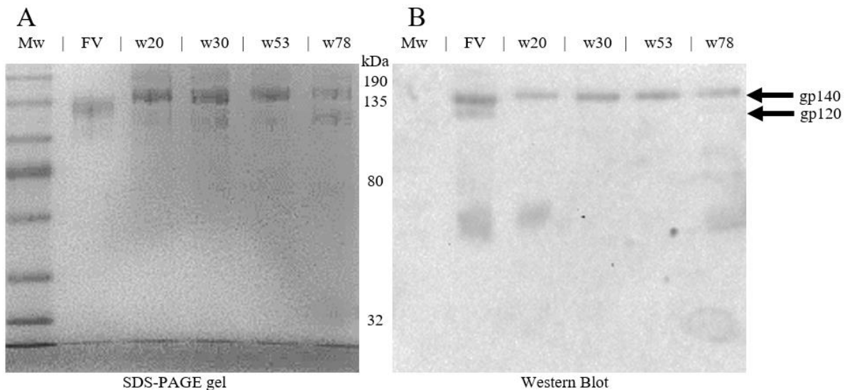
Figure 3.6: SDS-PAGE (A) and Western Blot (B) analysis of G. nivalis lectin-affinity purified FVgp140 and CH505gp140 envelope glycoproteins. Following transient transfections in HEK293 T cells, culture supernatant was clarified via centrifugation and filtered through a 0.45 \mu m filter membrane. (A) SDS-PAGE: 4 \mu g of protein loaded on an 8% SDS-PAGE gel and visualised with Coomassie staining. Mw- prestained protein marker, broad range (New England Biolabs® Inc., MA, USA) and corresponding bands are indicated on the left in kilodaltons (kDa). (B) Western blot: Protein expression was confirmed by probing for Env (2 \mu g of protein loaded) using the 10E8 primary antibody (diluted 1: 1 000). Subsequent detection with a horse radish peroxidase (HRP)-conjugated anti-human secondary antibody (diluted 1: 2 000).
