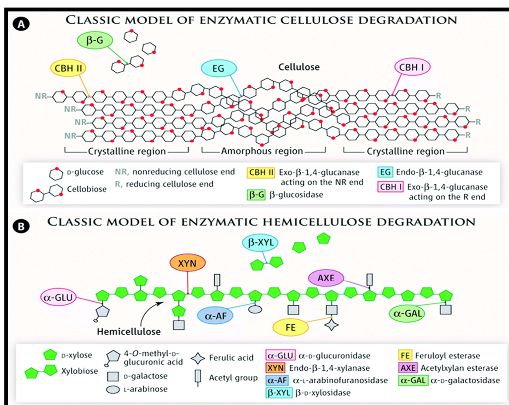
Figure 2.2: A simplified schematic of cellulose hydrolysis by a typical non-complexed cellulase system mediated by cellobiohydrolases (CBH I and CBH II) and endoglucanases (EG I to EG V) adsorption, cellobiose and cellodextrin production, and their catalysis to glucose by β-glucosidase. Also shown is one of the cellulase components with different domains (Wyman, 2013).
