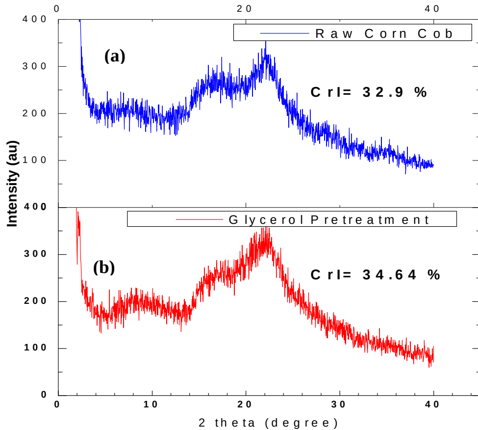
Figure 4.1: The X-ray diffractograms of the corncob before and after glycerol blending (a) raw corncob (b) Glycerol blended corncob
