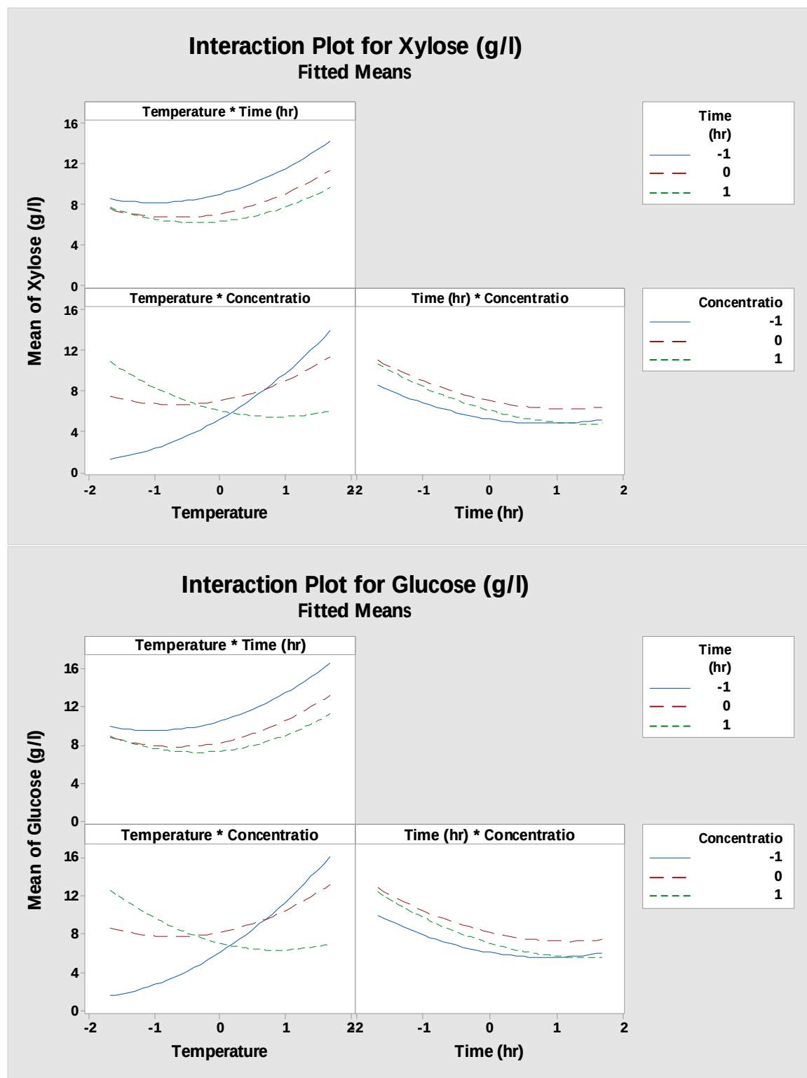
Figure 4.18: Interaction Effects of input Parameters
