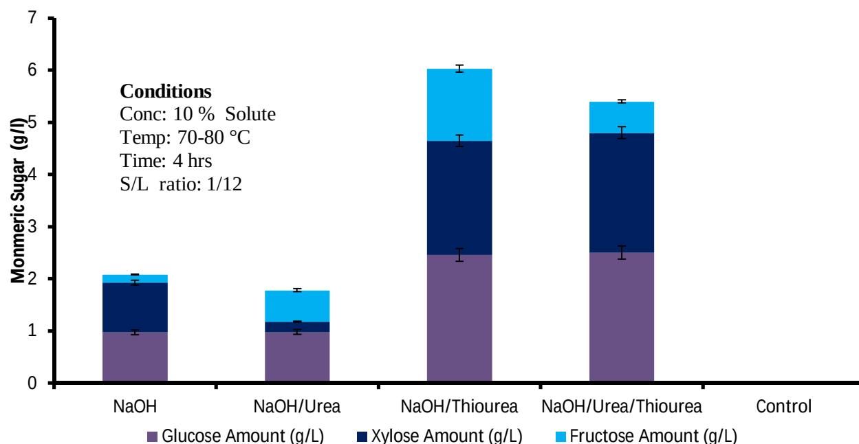
Figure 4.13: Monomeric sugar yield of corncob after dilute NaOH, urea and thiourea and combination pretreatment using 10% (w/v), temperature 70-80 °C, time 4 hrs, 10 g corncob solids and 120 ml liquid volume
