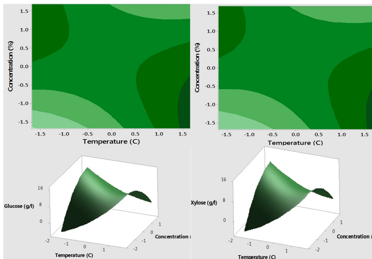
Figure 4.20: Reaction time, Response contour plots and corresponding surface plots of the glucose and xylose yield from pretreated corncob
