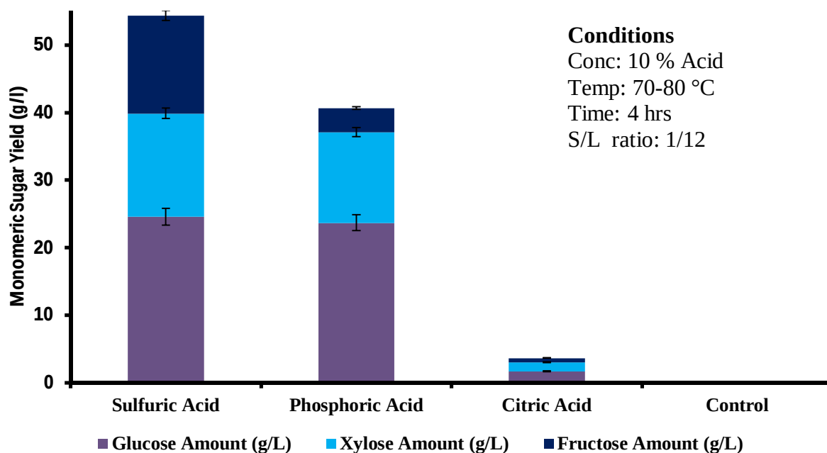
Figure 4.10: Monomeric sugar yield of corncob after diluting the sulfuric, citric and phosphoric acid pretreatment using 10% (w/w), temperature 70-80 °C, time 4 hrs, 10 g corncob solids and 120 ml liquid volume
