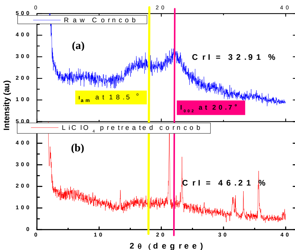
Figure 4.2: The X-ray diffractograms of the corncob before and after lithium perchlorate pretreatment (a) raw corncob (b) Lithium perchlorate pretreated corncob
