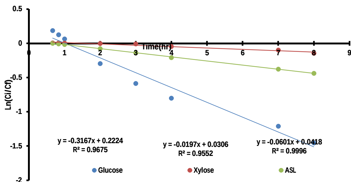
Figure 4.27: Kinetic model for glucose, xylose and SL dissolution at 180 °C: logarithm plots
