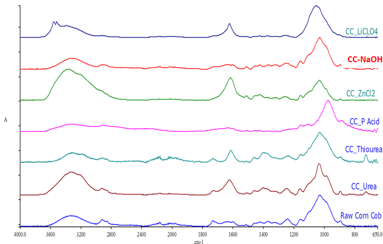
Figure 4.6: FTIR spectrum of raw corncob and aqueous pretreated corncob samples. For better visualization, the spectra were normalized.
