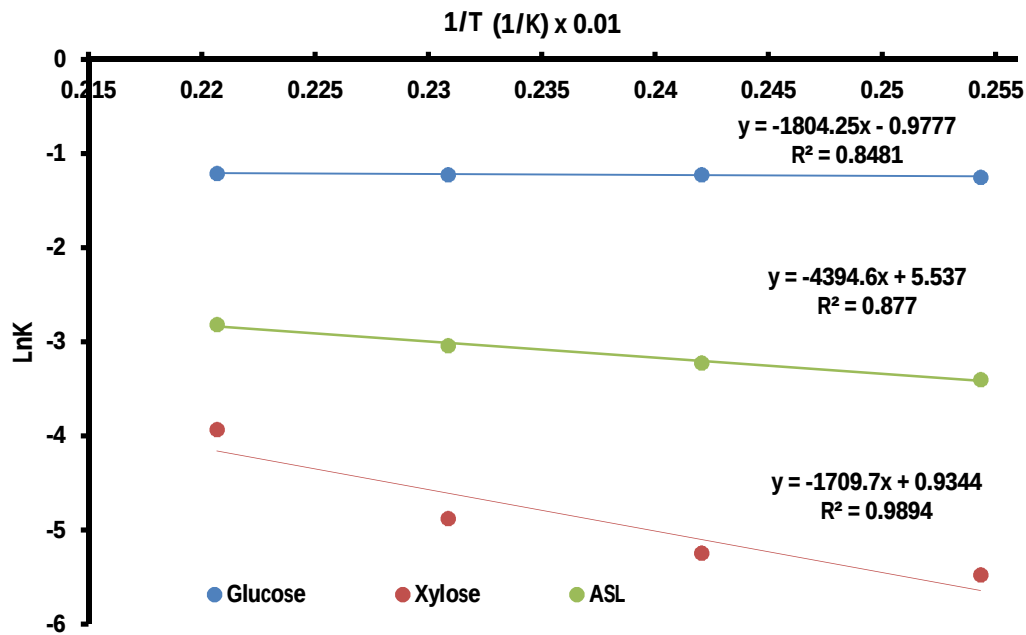
Figure 4.28: Kinetics of lignin content dissolution, glucose and xylose: Arrhenius plot for the treated biomass. Note: temperature in kelvin (K)
