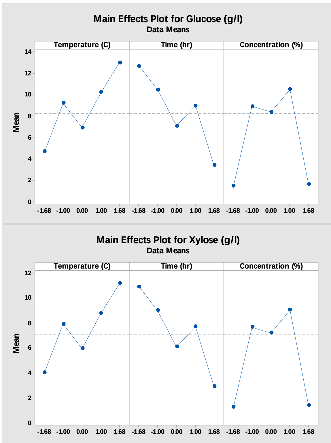
Figure 4.17 : Main Effect of Parameters, data means: (top) glucose yield (bottom) xylose yield
