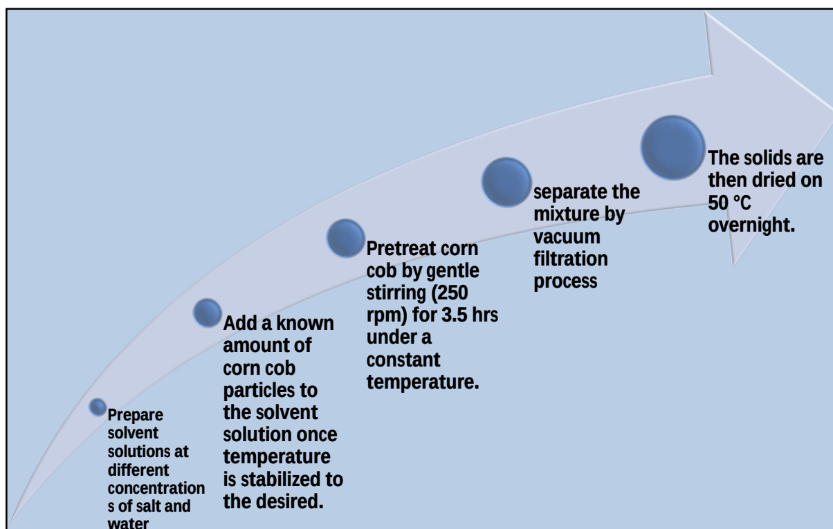
Figure 3.2: Dissolution procedure for all the different solvent systems
