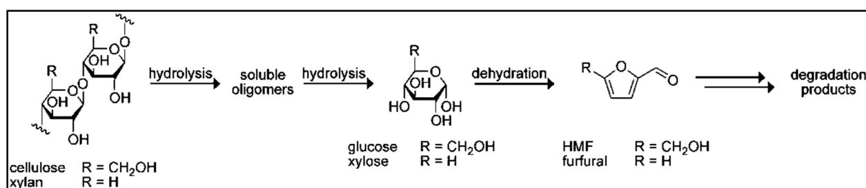
Figure 2.3: Hydrolysis reactions of cellulose and xylan. Chemical hydrolysis of cellulose and hemicellulose into monomeric sugars proceeds through oligomers and is accompanied by side reactions that form furans and other degradation products Adapted from Binder, 2010).
