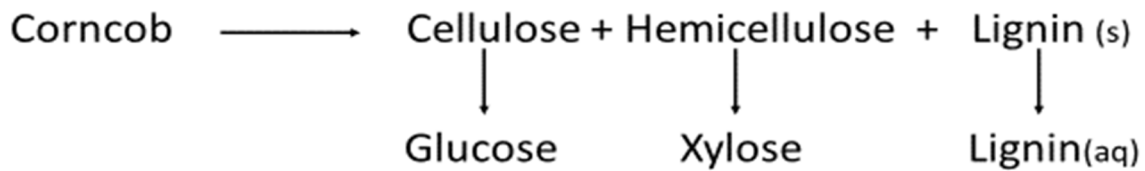
Figure 3.4: Dissolution and Hydrolysis mechanism
