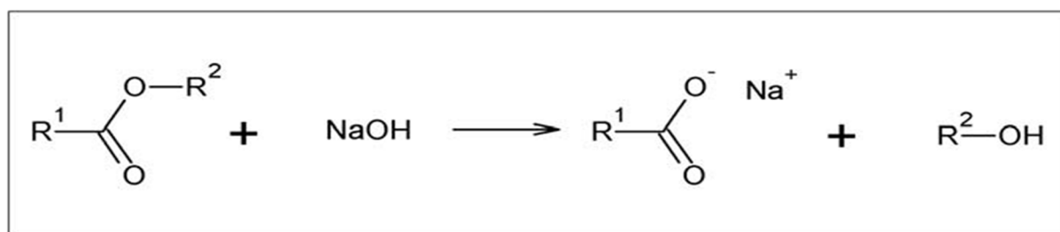
Figure 4.14: Saponification of ester bonds to yield a carboxylic salt and an alcohol Source: Pedersen & Meyer, 2010.
