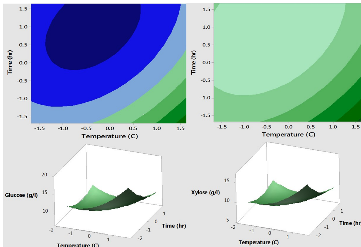
Figure 4.21: Concentration, Response contour plots and corresponding surface plots of the glucose and xylose yield from pretreated corncob
