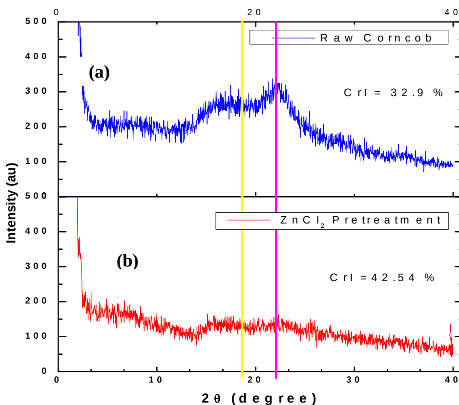
Figure 4.3: The X-ray diffractograms of the corn cob before and after zinc chloride pretreatment (a) raw corn cob (b) zinc chloride pretreated corn cob
