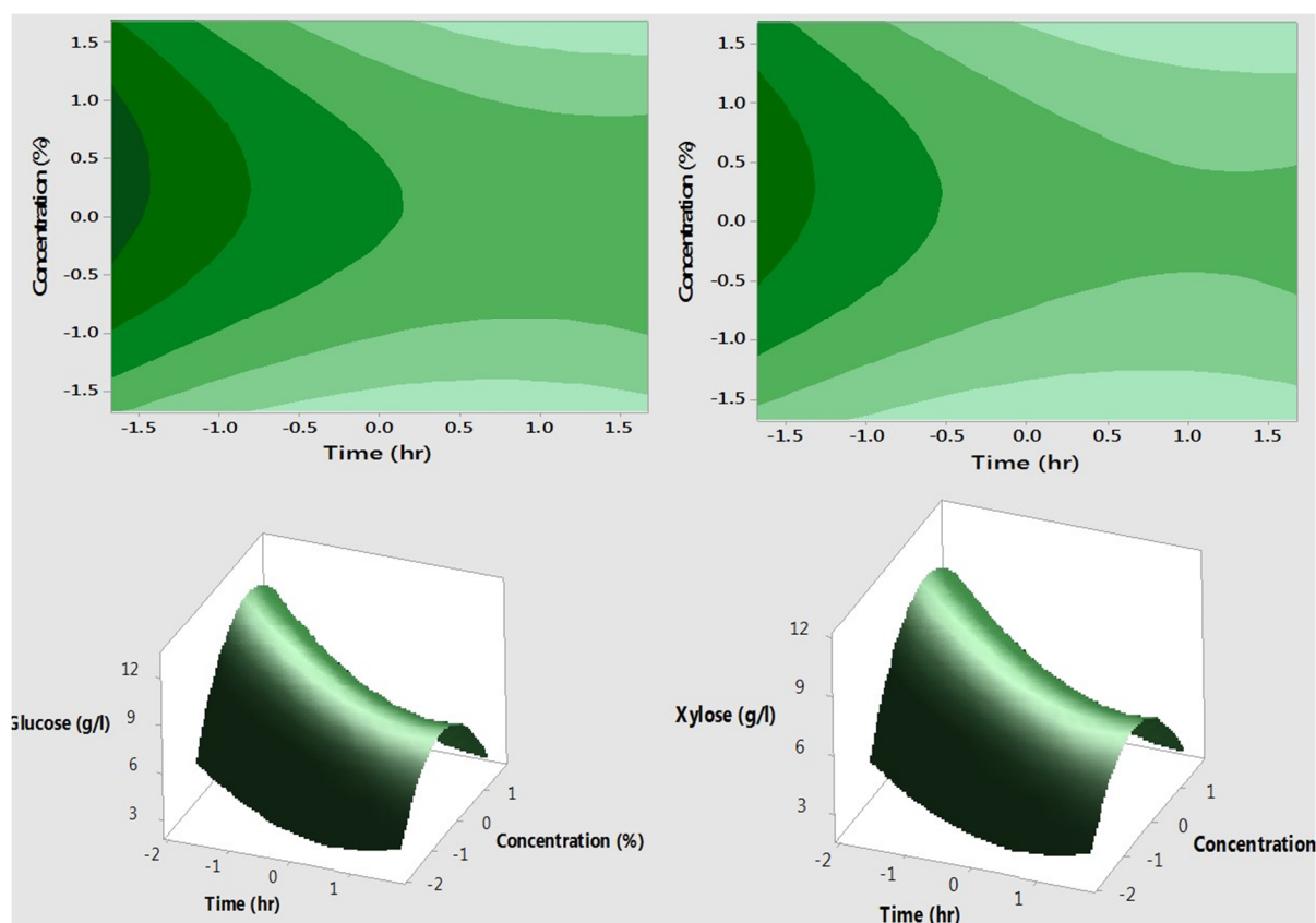
Figure 4.19: Temperature, Response contour plots and corresponding surface plots of the glucose and xylose yield from pretreated corncob
