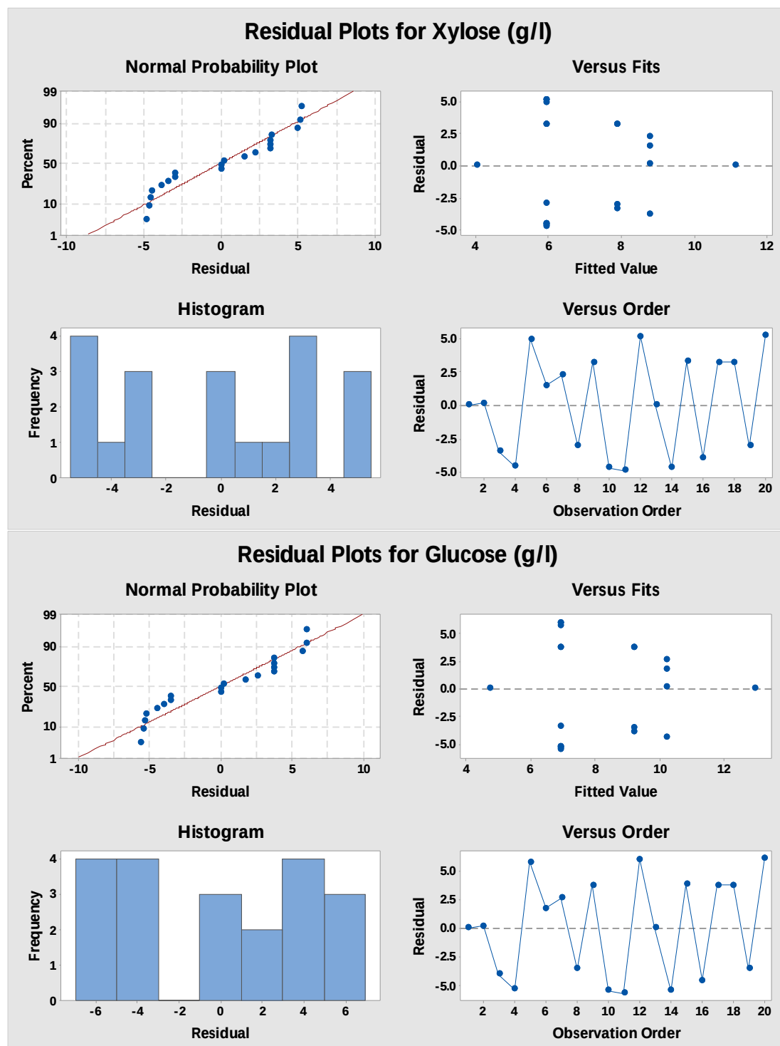
Figure 4.22: Validation of the ANOVA assumptions: normality, constant variance, and independence
