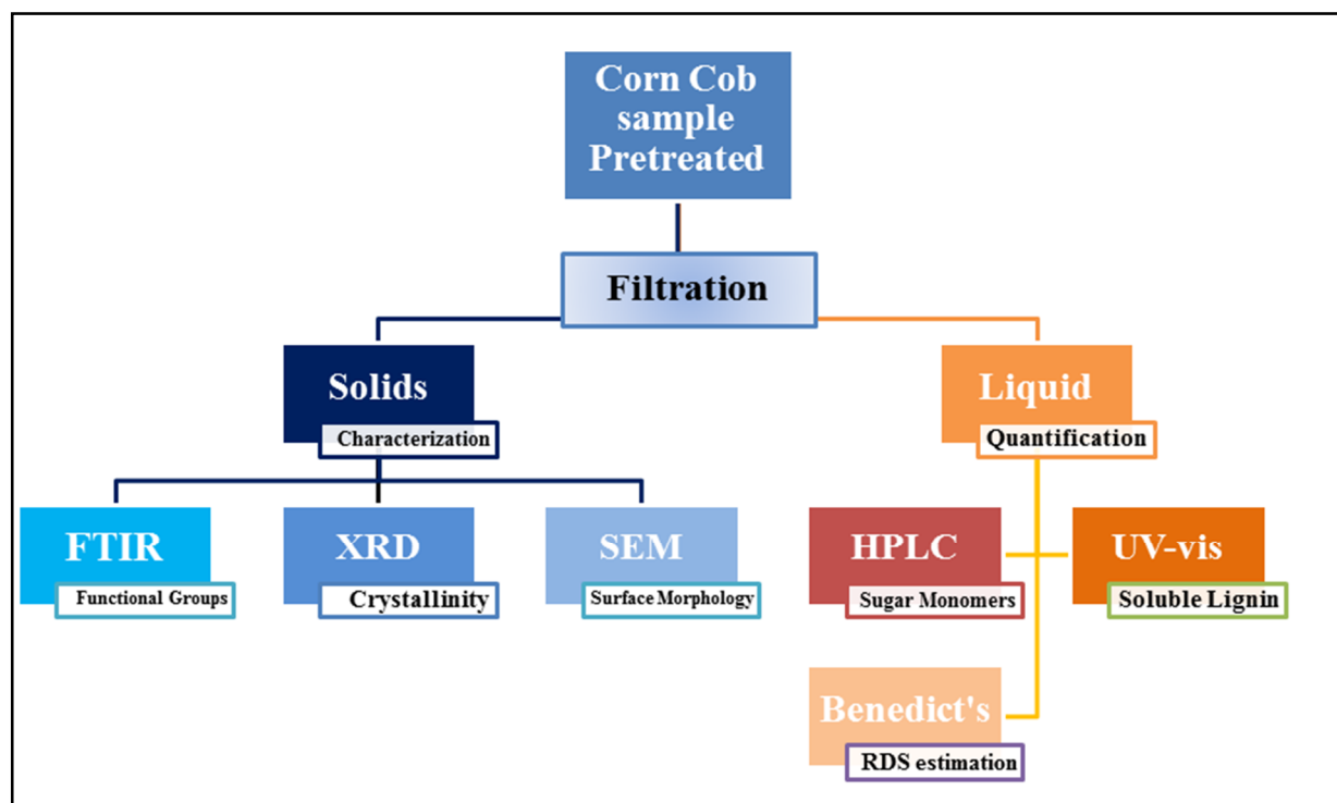
Figure 3.5: Schematic diagram for corncob methods of analysis
