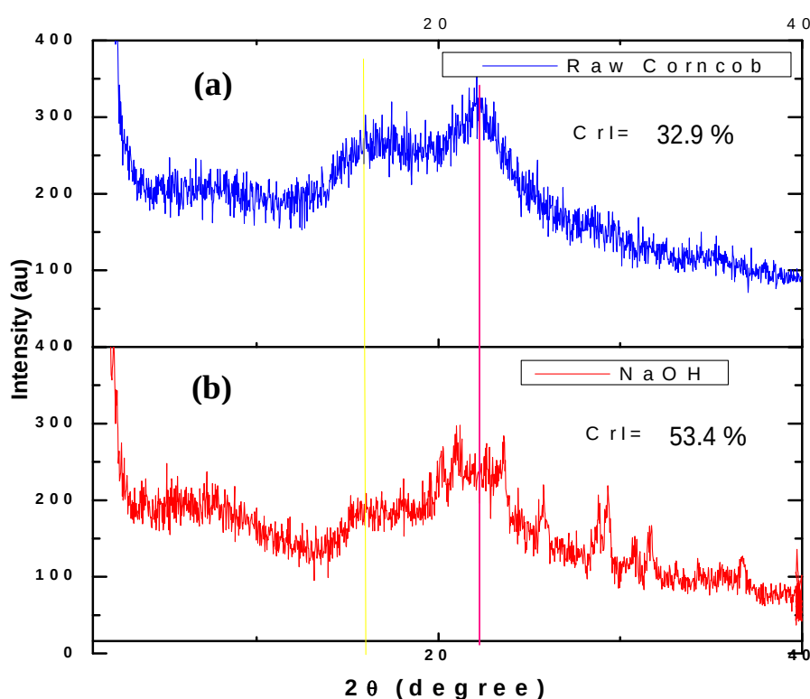
Figure 4.4: The X-ray diffractograms of the corncob before and after sodium hydroxide pretreatment (a) raw corncob (b) NaOH pretreated corn cob
