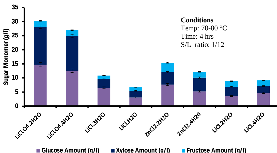
Figure 4.15: Effect of molten hydrates pretreatment process on glucose, xylose and fructose yield
