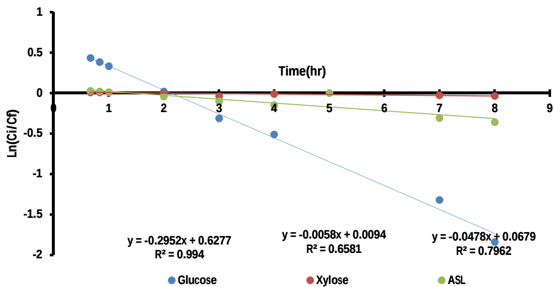
Figure 4.26: Kinetic model for glucose, xylose and SL dissolution at 160 °C: logarithm plots
