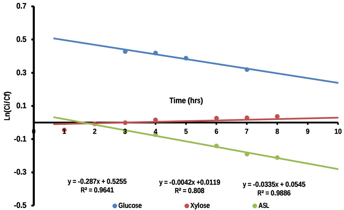
Figure 4.24: Kinetic model for glucose, xylose and SL dissolution at 120 °C: logarithm plots
