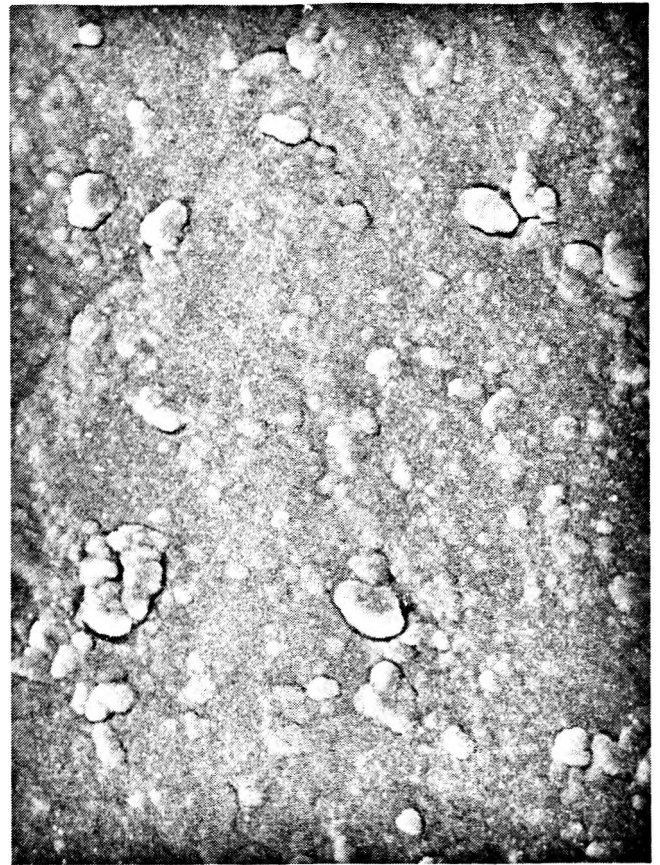
Fig. 7. Mechanical polishing for approximately 2 seconds of the hand scaled enamel surface after bond removal. SEM X 2000.
