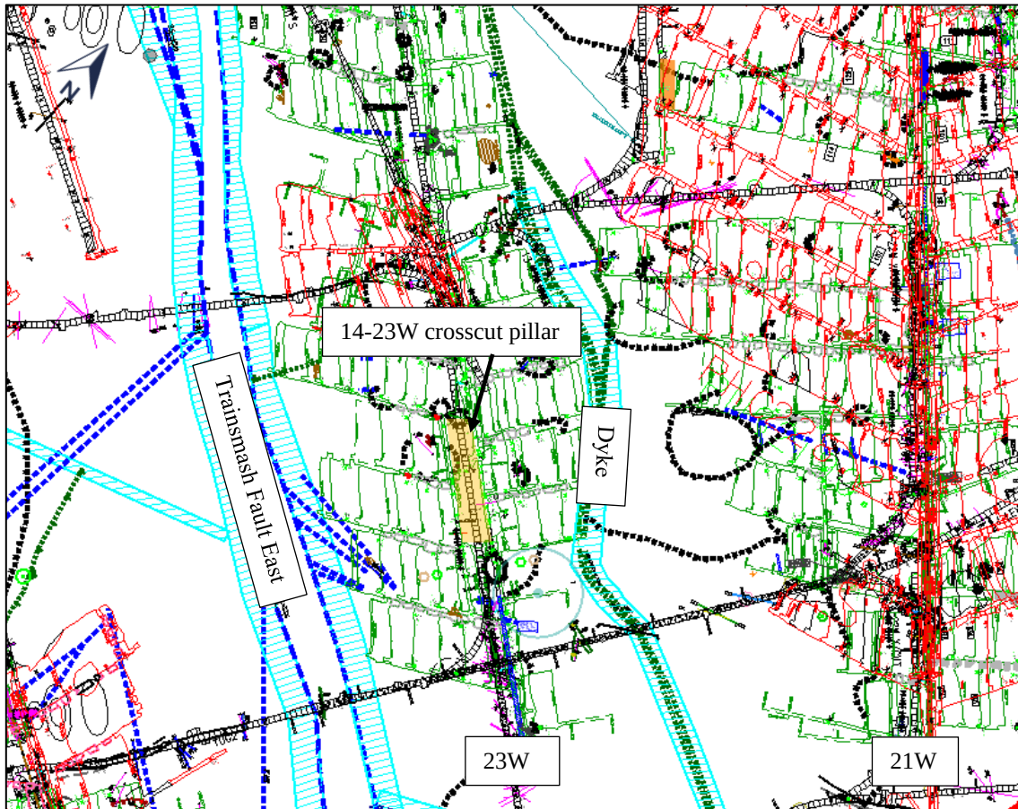
Figure 53: Plan showing the geology in the vicinity of the 14-23W UG2 crosscut. Red outlines showed the mined Merensky Reef areas and green outlines showed the UG2 Reef mined out areas
