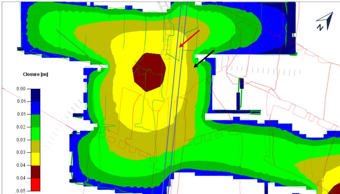
Figure 86: Expected closure at 14-20W panels (current state). The red arrow indicates the centre gully of 14-20W, and the black arrow indicates the 4E in-stope pillar which dynamically failed
