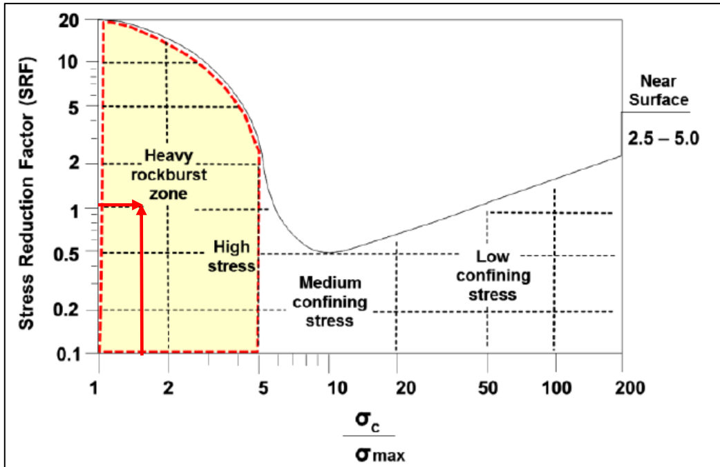
Figure 10: Graph showing the excavation behaviour as a function of compressive stress to the induced stress (Villaescusa et al , 2016). The arrows indicate the placement of the 14-23W UG2 crosscut
