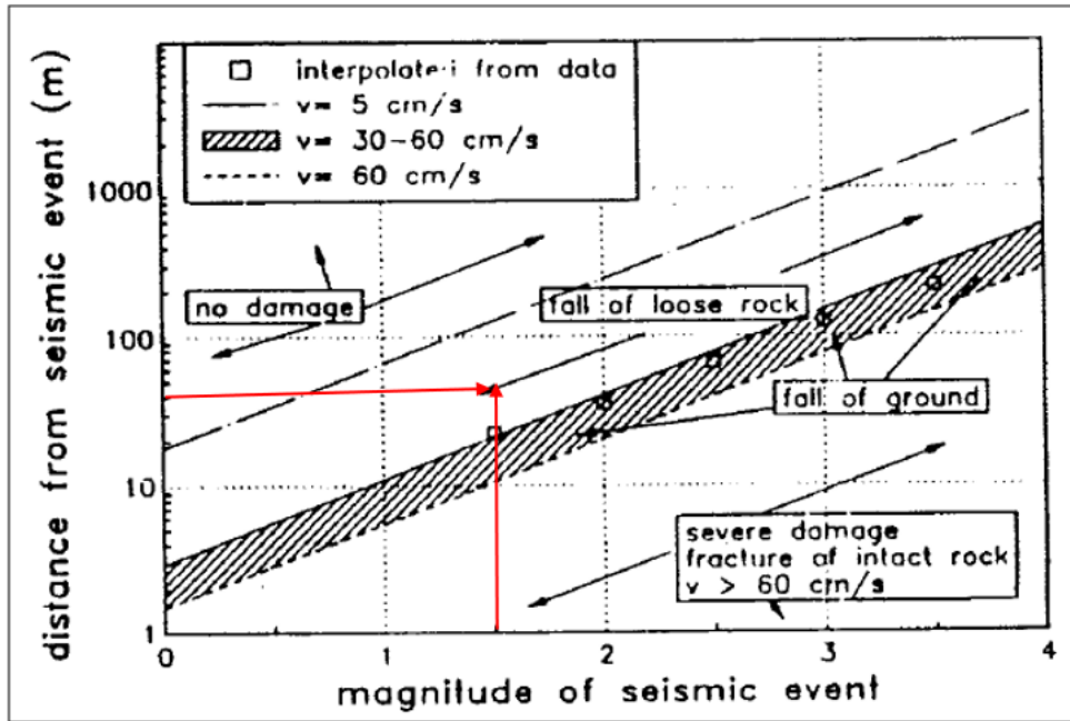
Figure 25: Damage in terms of peak ground velocity (from Lenhardt, 1988). The red arrows indicate the conditions for Tumela 1 Shaft mine for 95% of all seismic events
