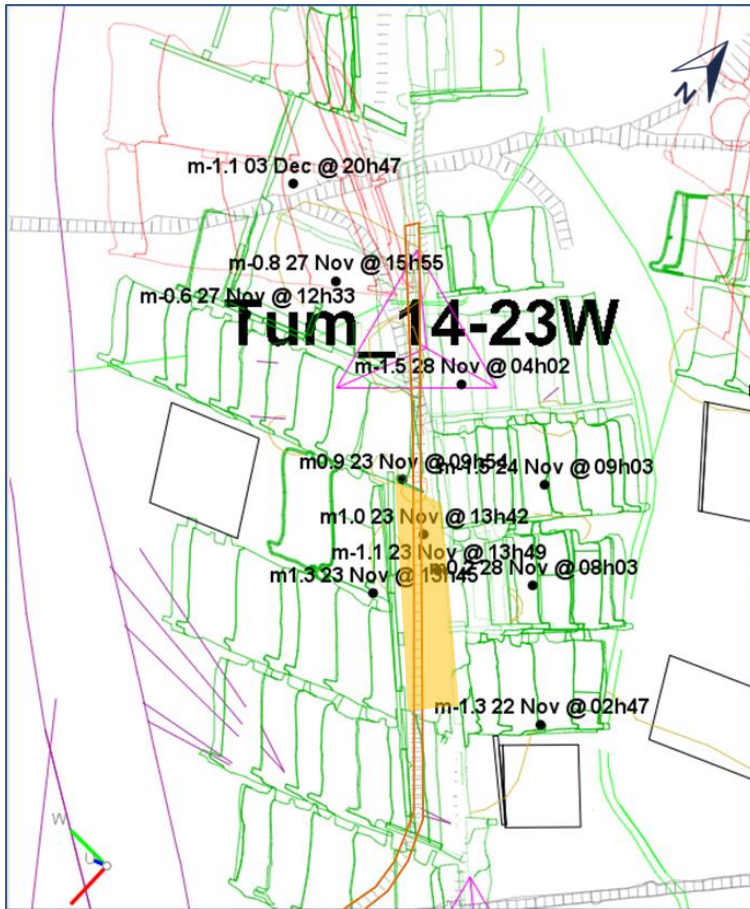
Figure 15: Plot showing all seismic events in the vicinity of 14-23W UG2 crosscut from 20 November 2018 to 31 December 2018. The orange area is the crosscut protection pillar
