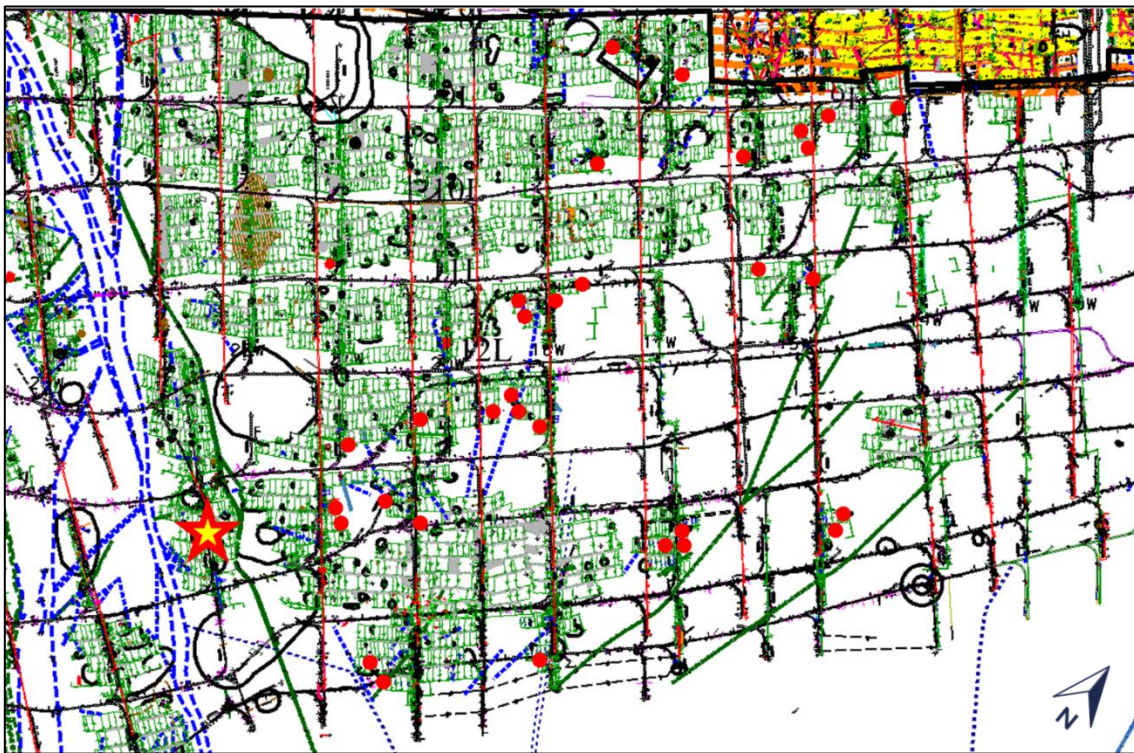
Figure 18: Plan showing 15-23W 1W panel (red star) and the mining panels at the time of the crosscut dynamic failure (red circles)
