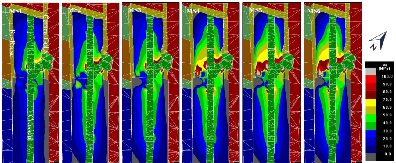
Figure 63: The stress changes (Sigma 1- in plane) made over the six mining steps as shown in MAP3D
