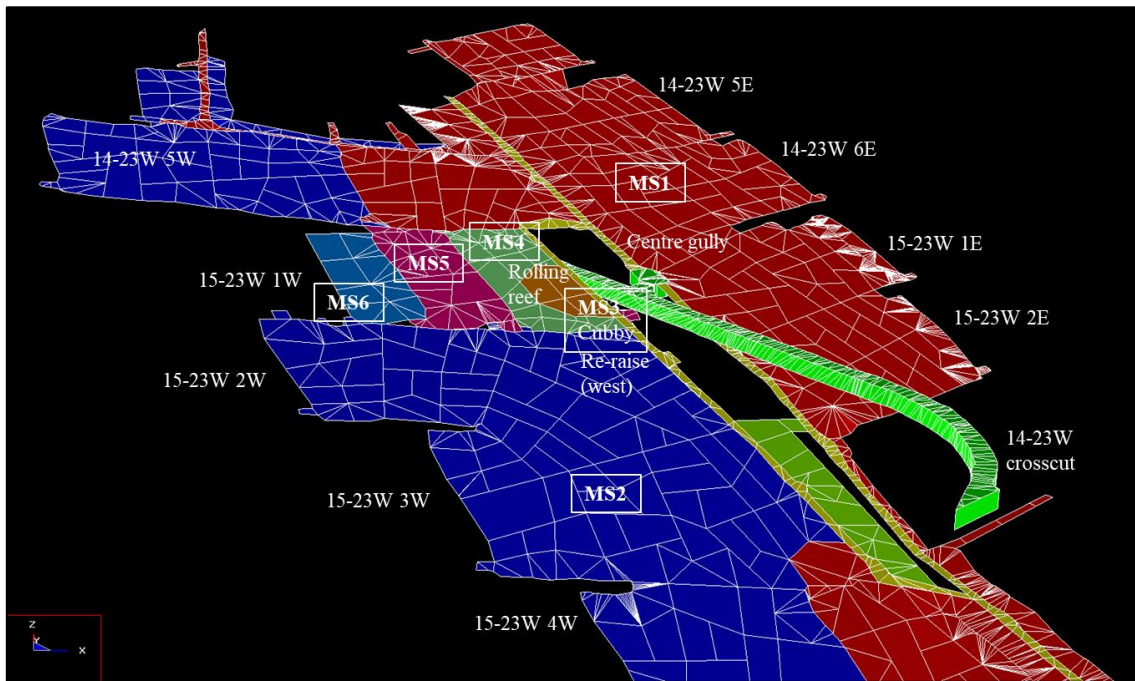
Figure 56: MAP3D model of the 14-23W UG2 crosscut indicating the mining steps used in the numerical modelling analysis (looking North)
