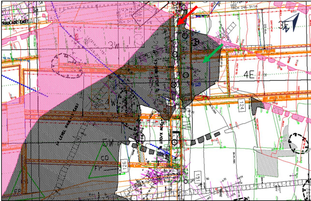
Figure 19: Plan showing the Merensky Reef remnant (black was off - reef and pink was - on reef projections) over UG2 panels. The red arrow indicates the centre gully of 14-20W, and the green arrow indicates the 4E in-stope pillar which dynamically failed
