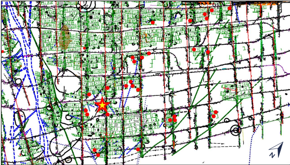
Figure 87: Plan showing the panels mined out and the position of 14-20W (red star) in relation to other mining panels
