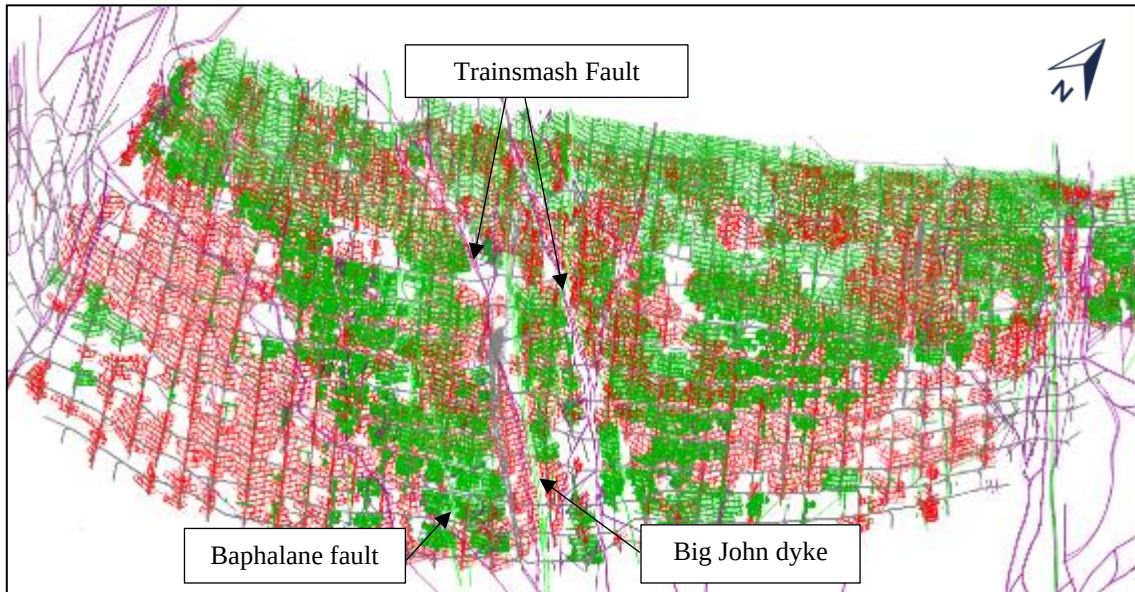
Figure 3: Plan showing the major geological features at Tumela Mine
