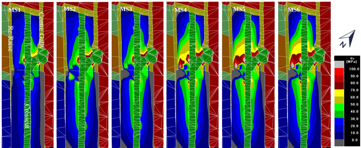
Figure 65: The stress changes (Sigma 1- in plane) made over the six mining steps as shown in MAP3D
