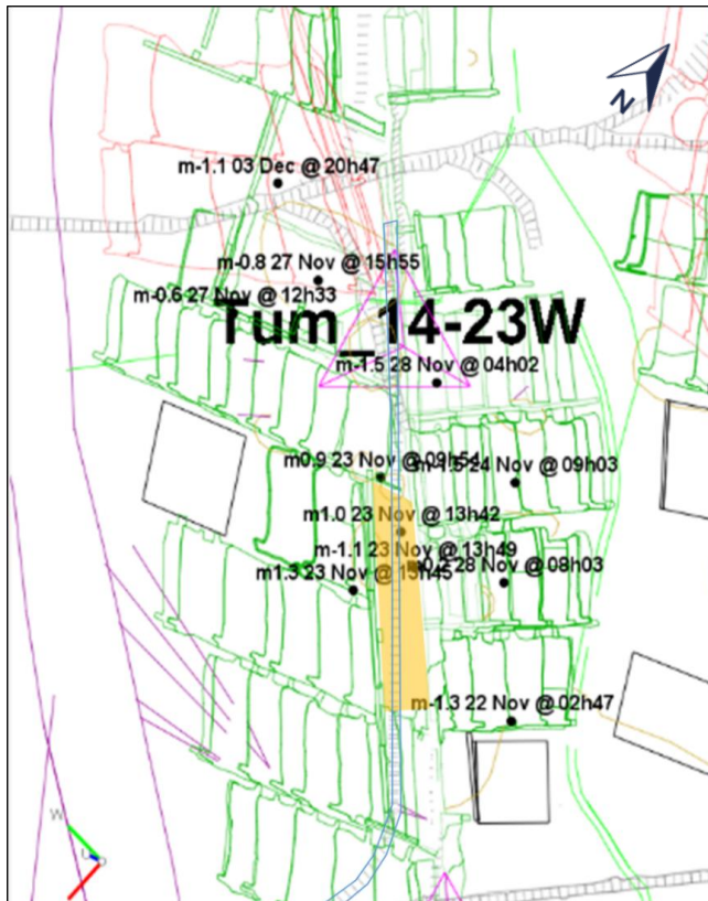
Figure 51: Plot showing all seismic events in the vicinity of 14-23W UG2 crosscut from 20 November 2018 to 31 December 2018. The orange area was the crosscut protection pillar
