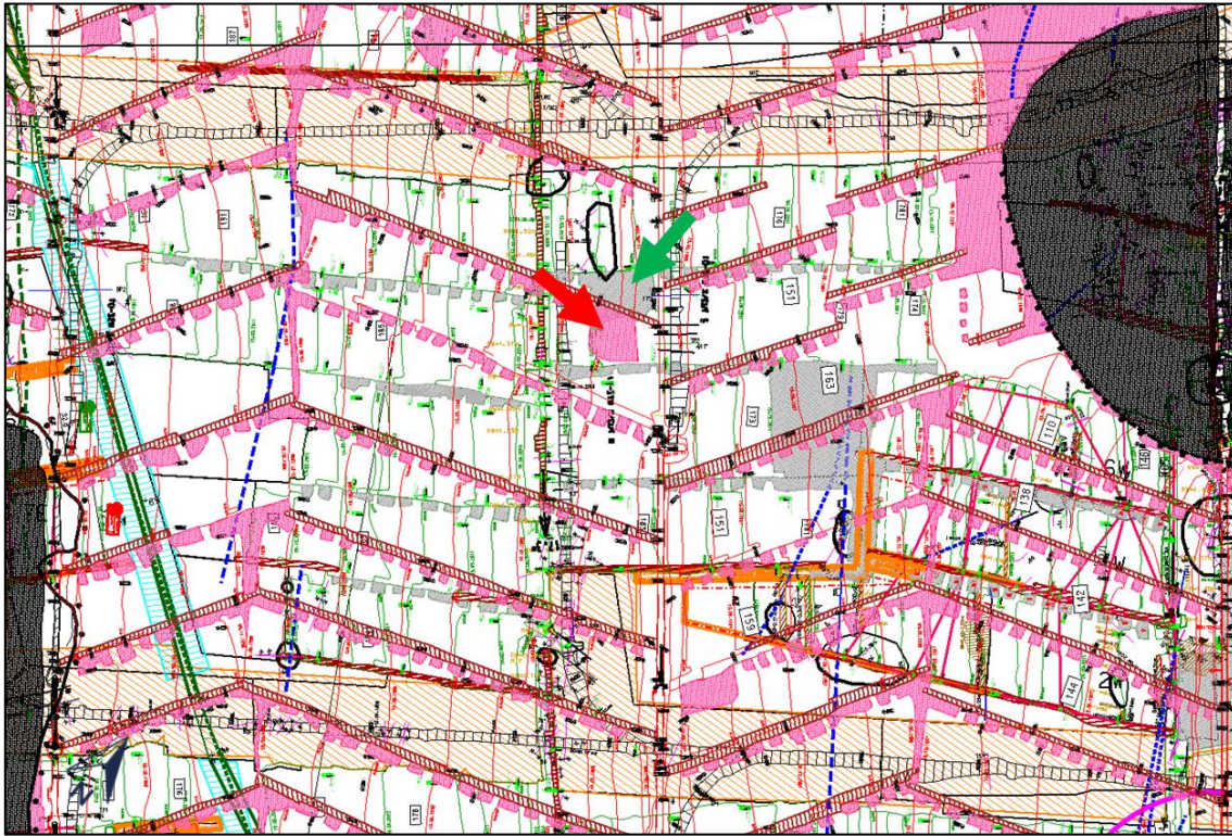
Figure 27: Plan showing the 11-32W UG2 Reef (green) and Merensky Reef stopes (red). The pink hatched areas were the Merensky Reef pillars and the grey hatched areas were the UG2 Reef pillars. The red arrow indicates the pillar which was the source of the event
