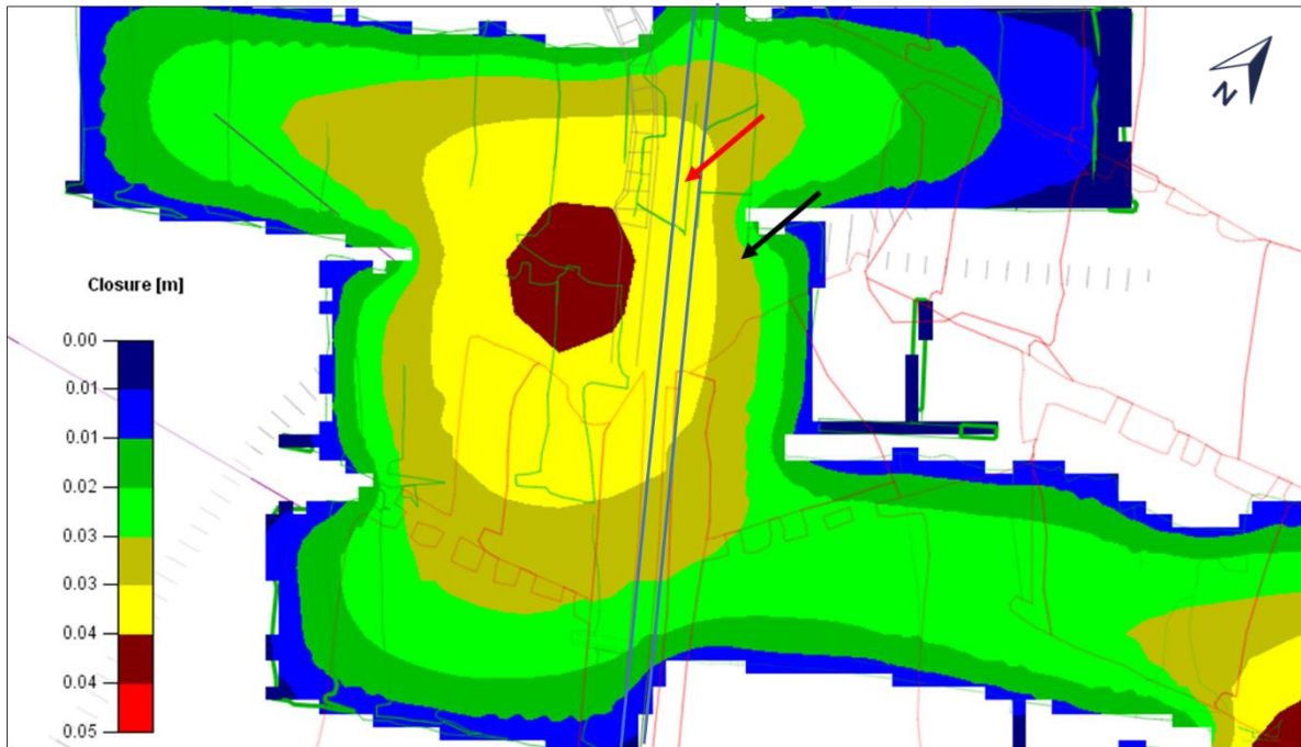
Figure 20: Expected closure at 14-20W panels (current state). The red arrow indicates the centre gully of 14-20W, and the black arrow indicates the 4E in-stope pillar which dynamically failed
