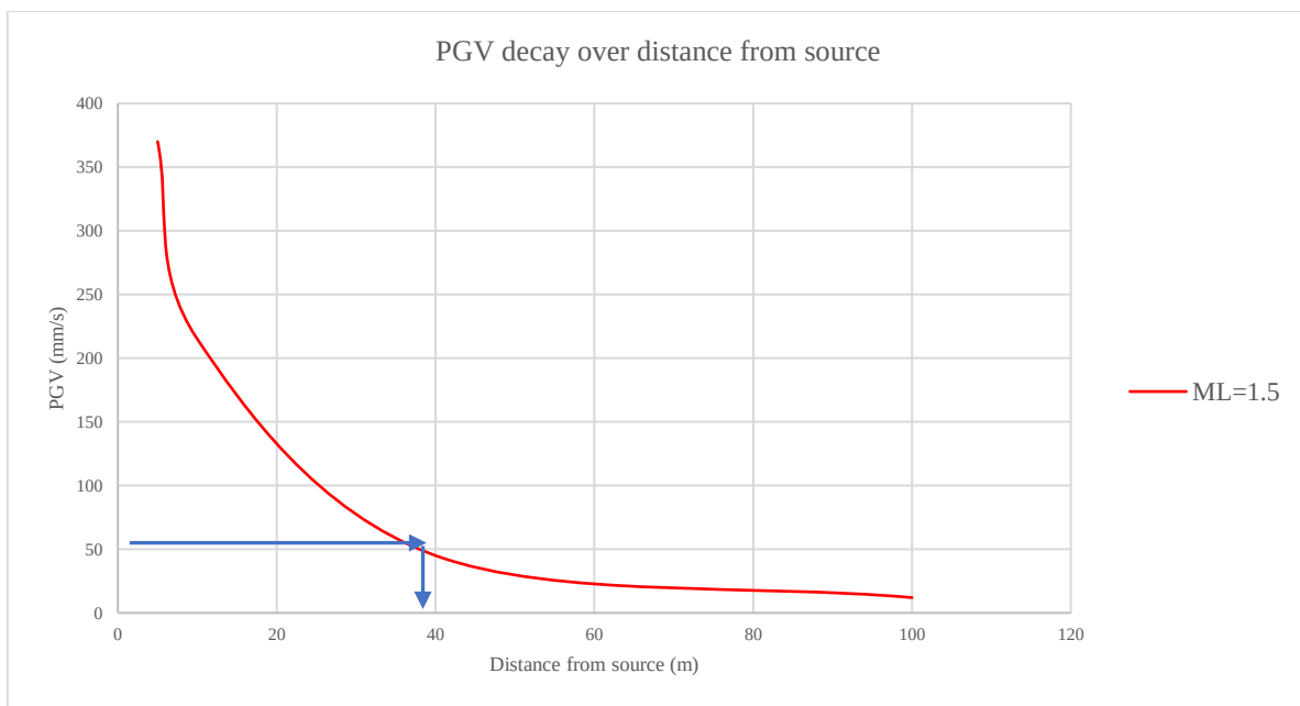
Figure 23: Graph showing the decay in PGV with distance from the source for a M1.5 event
