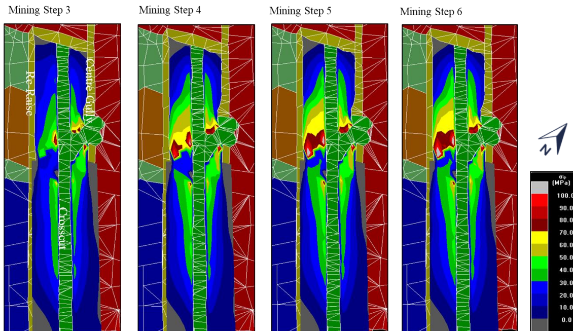
Figure 68: Scenario 2- Stress changes from the winch cubby not being blasted between mining steps 4 to 6
