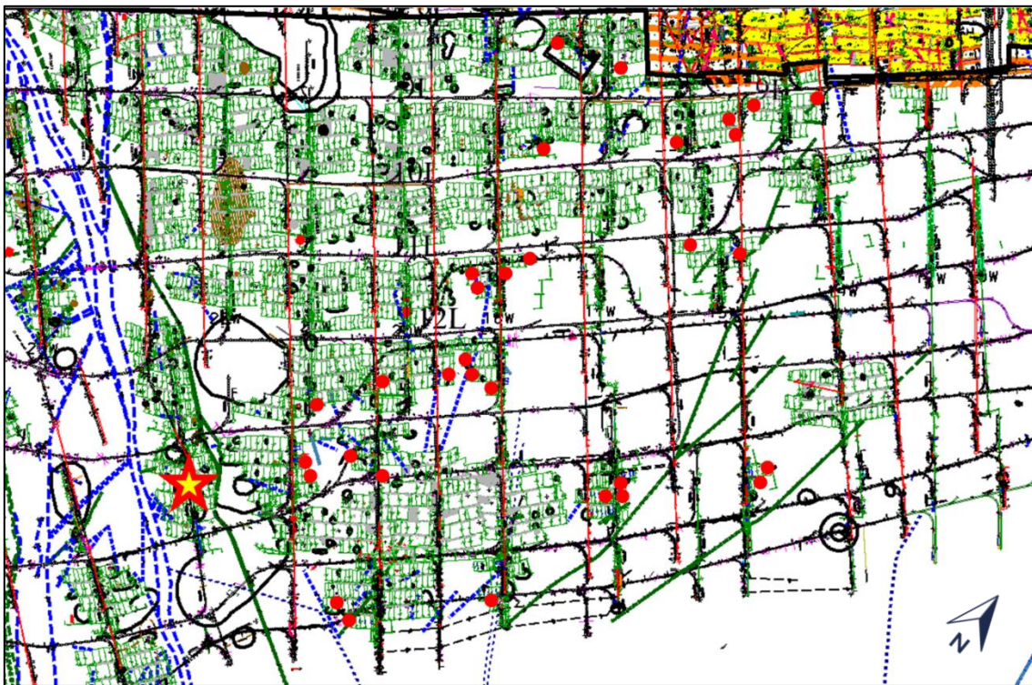
Figure 66: Plan showing 15-23W 1W panel (red star) and the mining panels at the time of the crosscut dynamic failure (red circles)
