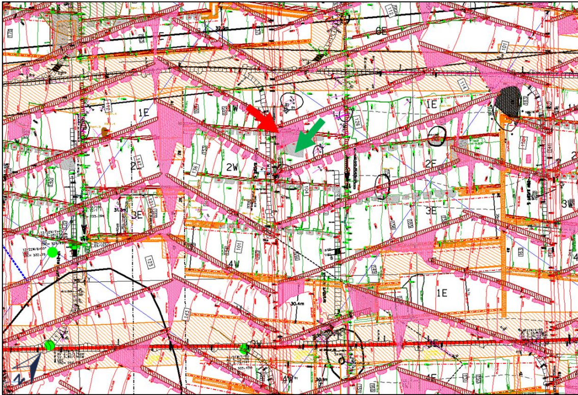
Figure 37: Plan showing the 12-21W UG2 Reef (green) and Merensky Reef stopes (red). The pink hatched areas were the Merensky Reef pillars and the grey hatched areas were the UG2 Reef pillars
