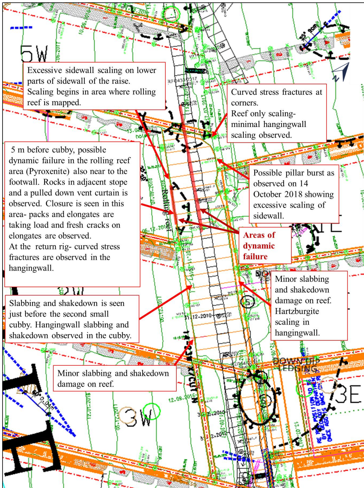
Figure 55: Underground observations on UG2 Reef elevation at the relevant locations
