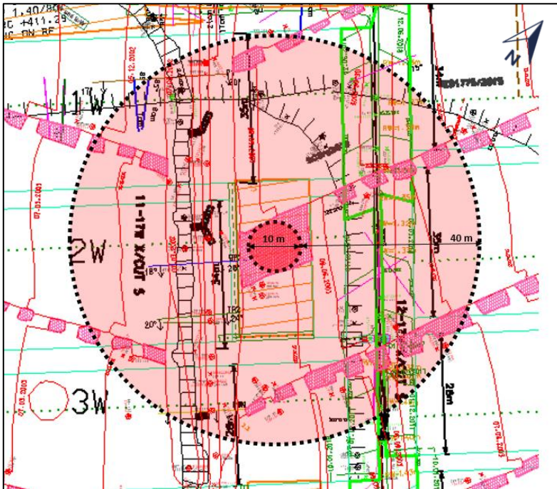
Figure 24: The Figure indicates how to measure the minimum width of a square pillar and the 40 m radial area affected by the Merensky Reef pillar
