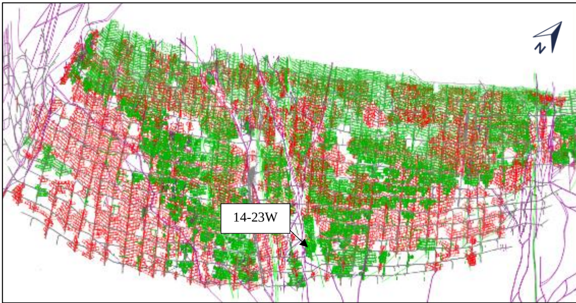
Figure 52: Location of 14-23W UG2 at Tumela Mine
