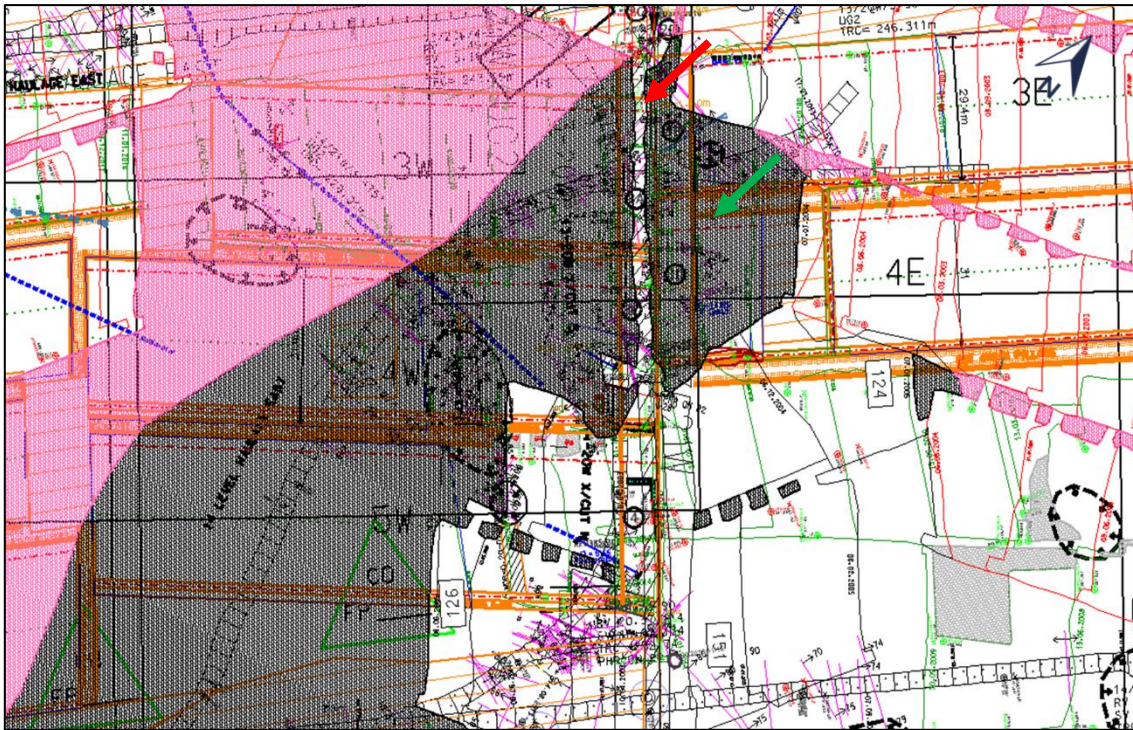
Figure 80: Plan showing the Merensky Reef remnant (black was off - reef and pink was - on reef projections) over UG2 panels. The red arrow indicates the centre gully of 14-20W, and the green arrow indicates the 4E in-stope pillar which dynamically failed
