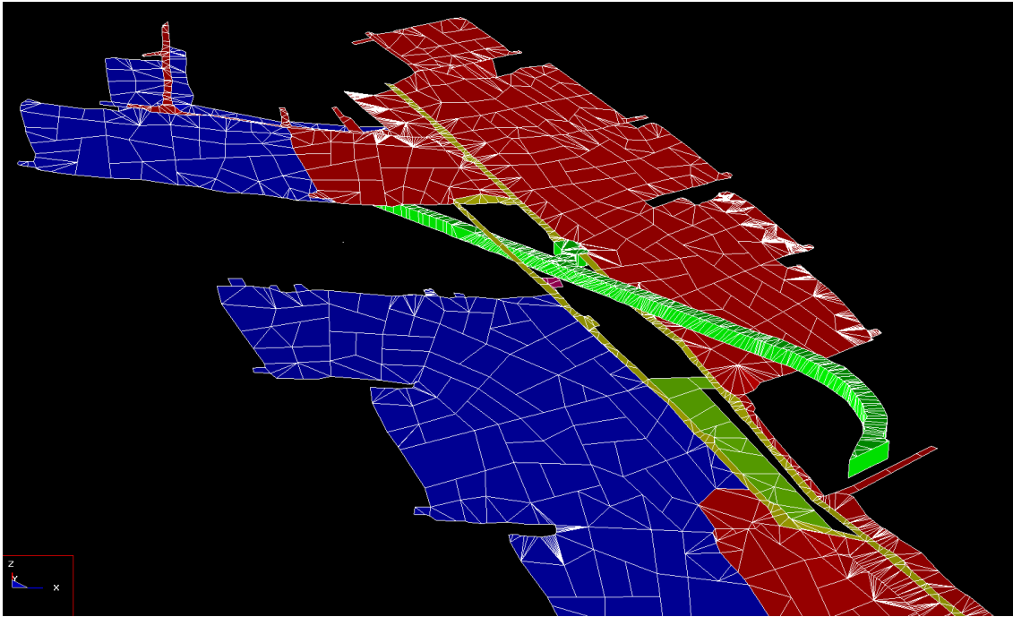
Figure 59: Mining step 3 -15-23W 1W Winch cubby is mined out - looking North
