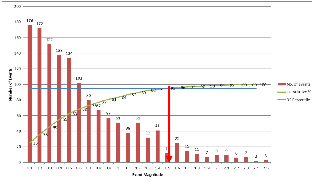
Figure 22: Cumulative assessment of seismic events. Graph shows that 95% of seismic events (2009 to 2018) are below a magnitude of approximately M1.5
