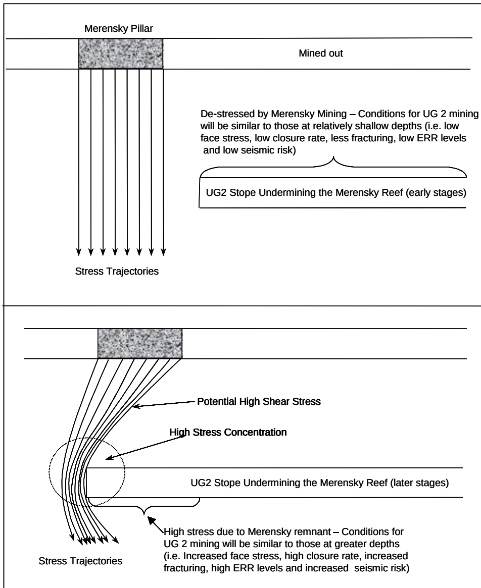
Figure 11: Diagram showing the stress distribution as UG2 Reef mines under a Merensky Reef remnant (Urcan et al , 2004)
