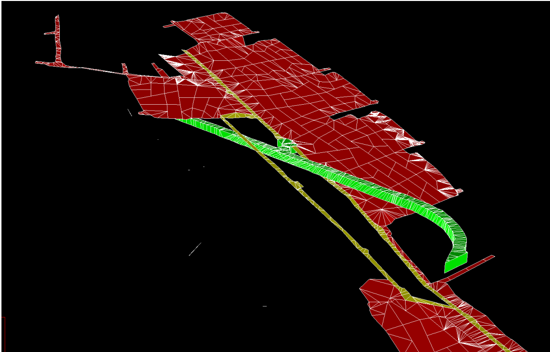
Figure 57: Mining step 1 - all areas mined out until the first scaling is observed in the crosscut (April 2017) - looking North
