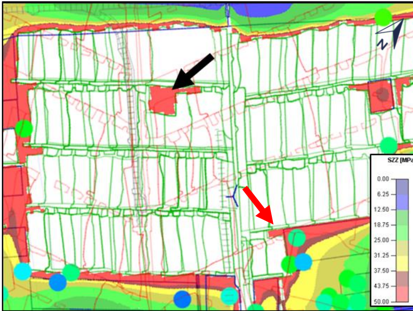
Figure 43: A Plan showing the position of the failed UG2 Reef pillar (red arrow) and the failed Merensky Pillar (black arrow)
