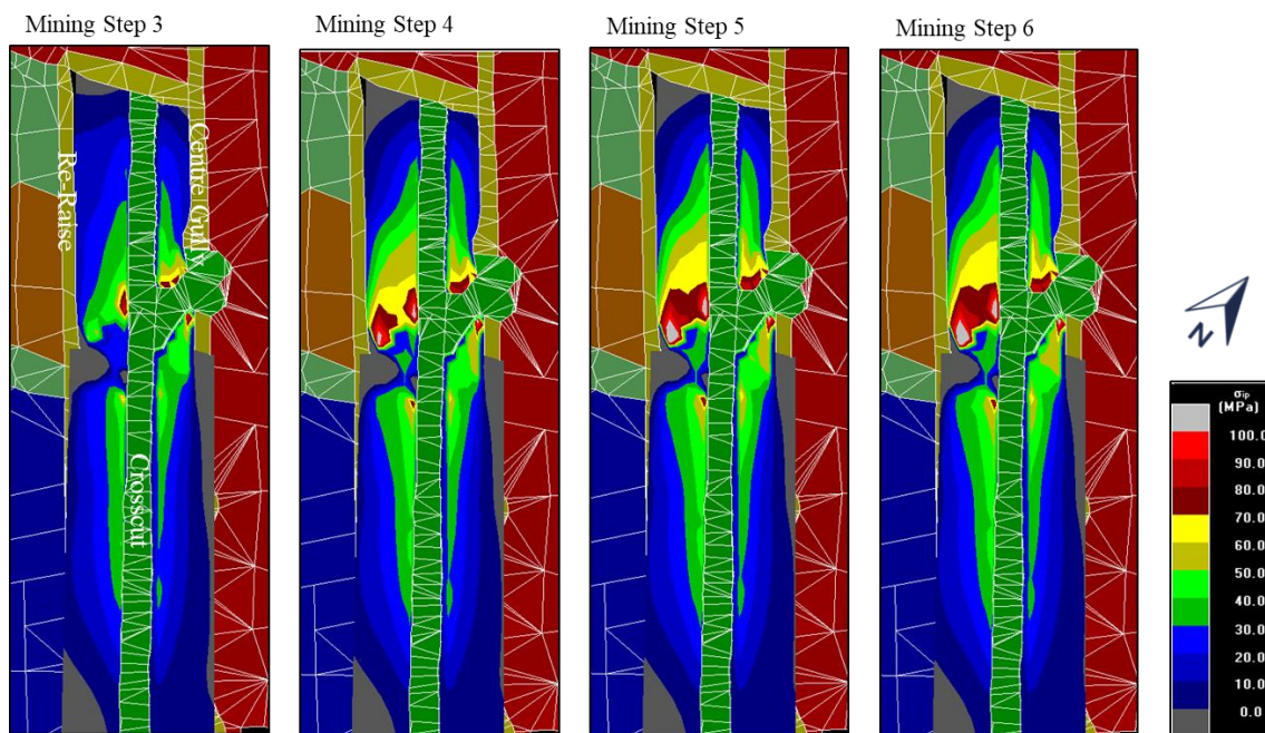
Figure 67: Scenario 1 Baseline model - Stress changes from the winch cubby being blasted between mining steps 4 to 6
