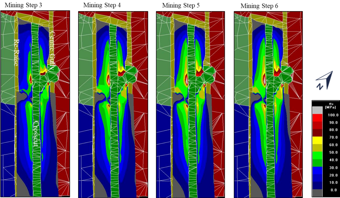
Figure 71: Scenario 4- Stress changes from no rolling reef present (no rock type change) between mining steps 4 to 6
