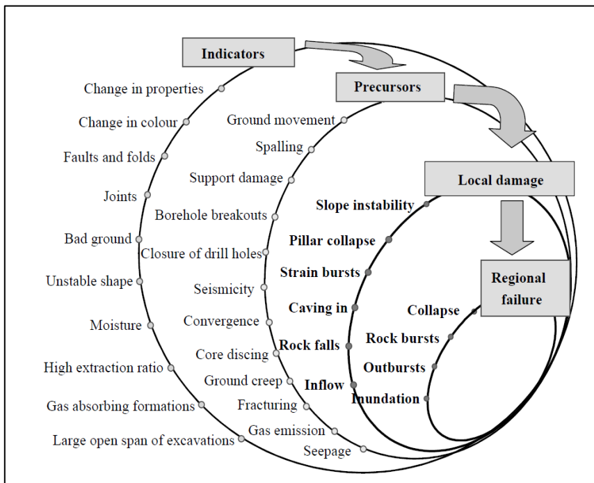
Figure 21: Progression of failure and warning signs (from Szwedzicki, 2003)
