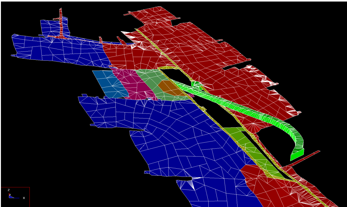
Figure 62: Mining step 6 - month 3 of 15-23W 1W (up to time of seismic event) where the face was stopped on 23 November 2018- looking North
