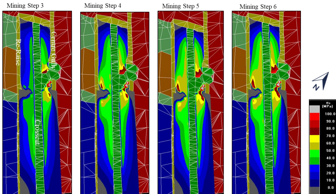
Figure 70: Scenario 3- Stress changes from no UG2 Reef/crosscut intersection (no rock type change) between mining steps 4 to 6
