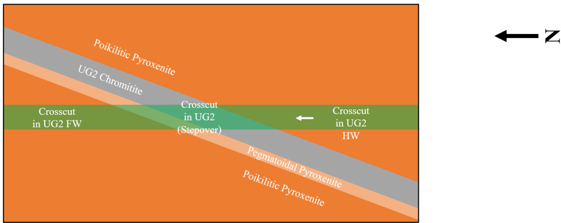
Figure 69: Diagram showing how the crosscut mines firstly through the UG2 Reef hangingwall, the UG2 Reef and then the UG2 Reef footwall
