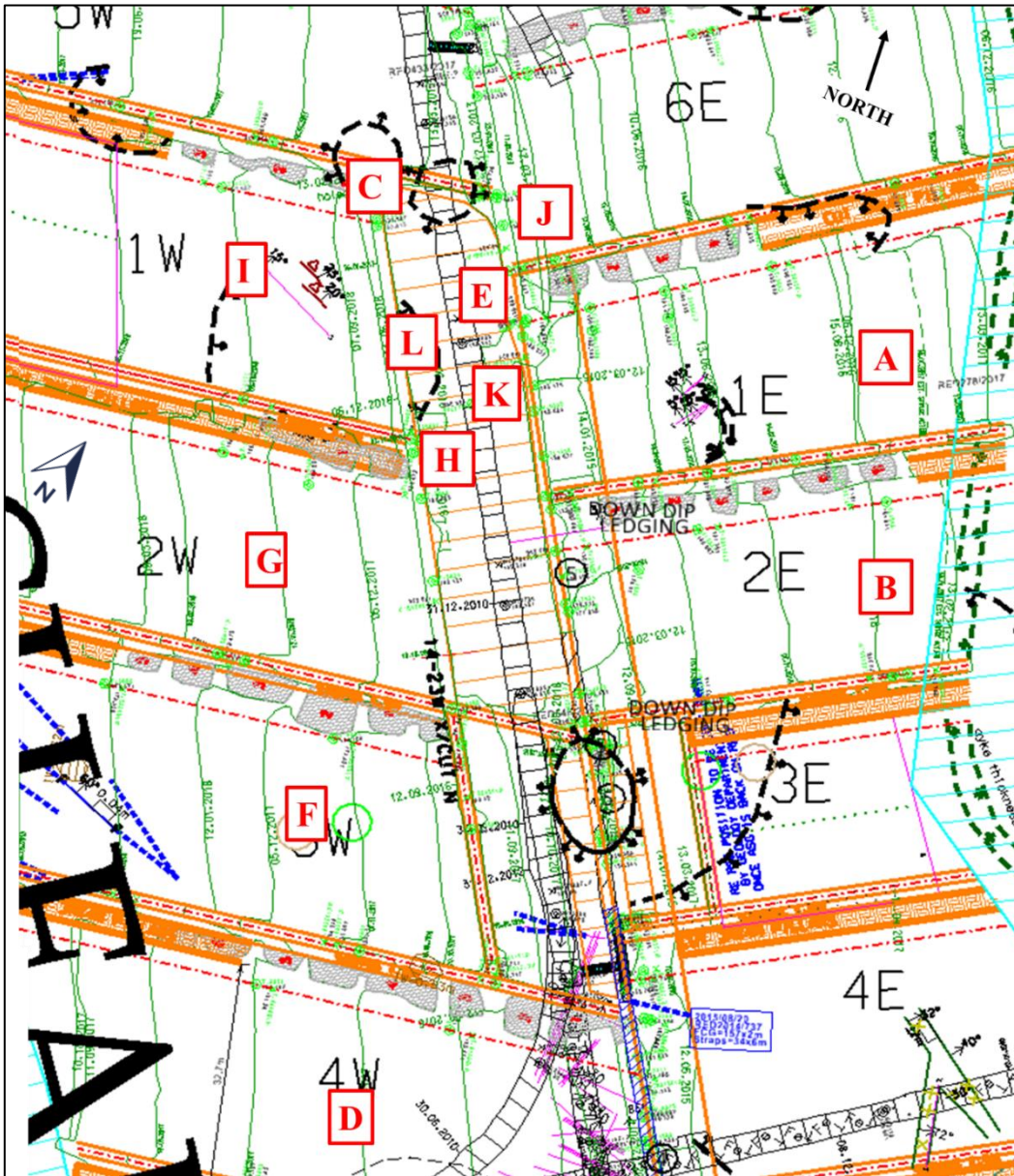
Figure 54: Plan showing the sequence of events before dynamic failure at 14-23W crosscut
