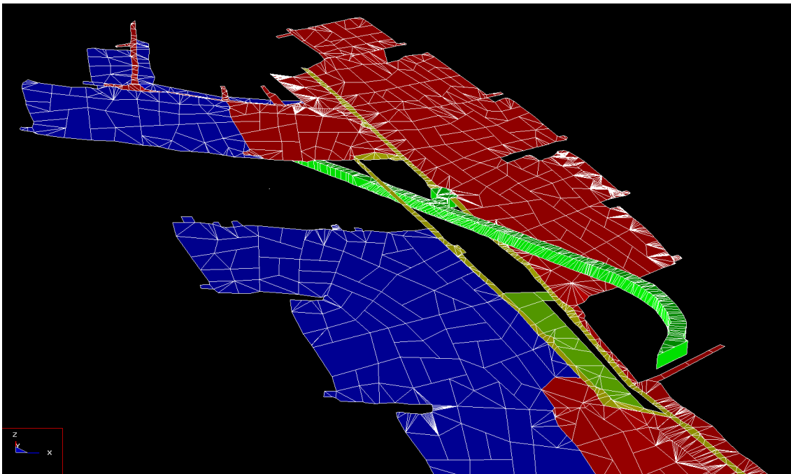
Figure 58: Mining step 2 - all panels are mined out except 15-23W 1W - looking North
