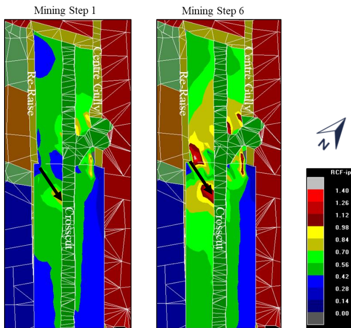
Figure 64: MAP3D plot showing the RCF at step 1 (when scaling was first noticed on the sidewall) and at step 6 (dynamic failure). The black arrows indicate the point of interest (the failure area)
