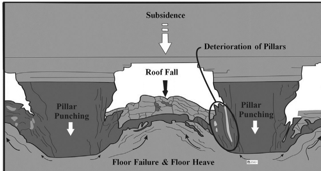
Figure 8: Diagram showing the modes of pillar failure (Richardson et al , 1999)
