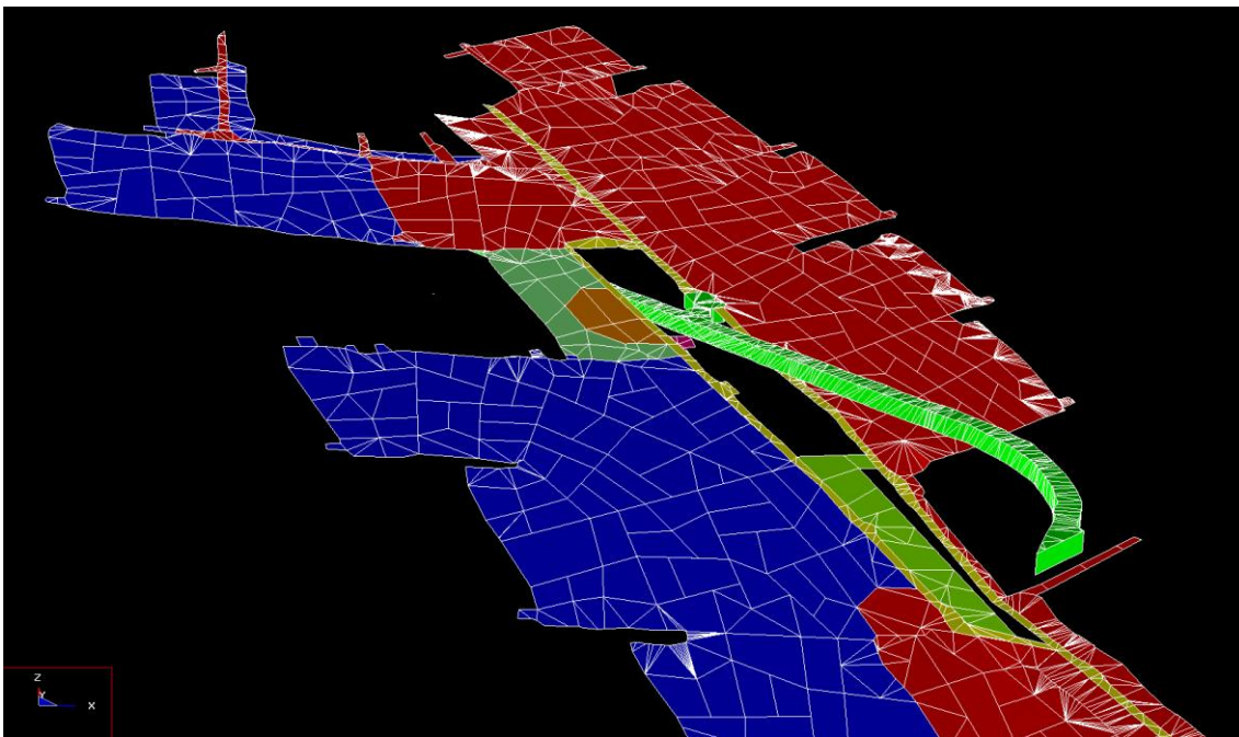
Figure 60: Mining step 4 - month 1 of 15-23W 1W - looking North
