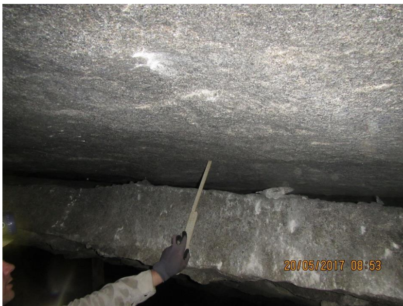
Figure 29: Hangingwall detachment in the vicinity of the failed pillar
