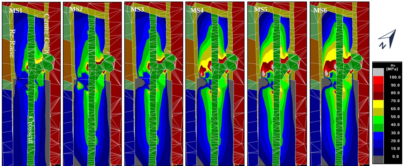
Figure 17: The stress changes (Sigma 1- in plane) made over the six mining steps as shown in MAP3D
