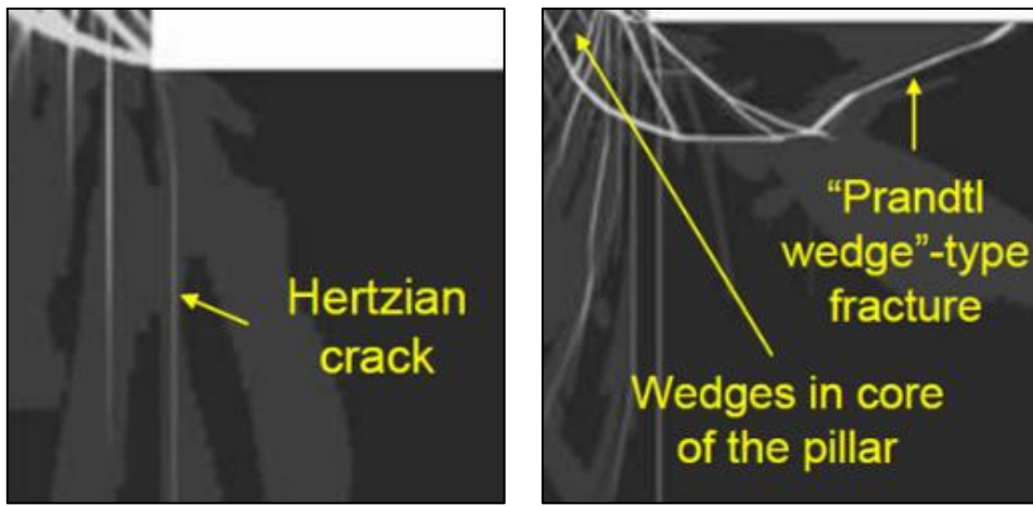
Figure 9: Types of failures in the footwall of a pillar: w:h = 2 (left) and w:h = 5 (right), (Maybee, 2000; Watson, 2008)
