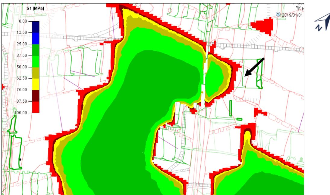
Figure 83: Stress modelled on Merensky Reef pillars i.e. stresses induced on the UG2 Reef by Merensky Reef remnant. Black Arrow indicates the dynamically failed in-stope pillar at 14-20W 4E
