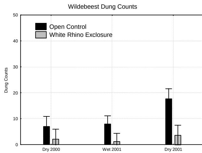
Figure 3- Seasonal dung counts in white rhino exclosures and open control areas for wildebeest, zebra and impala/nyala. Means and 95% CL's reported.
