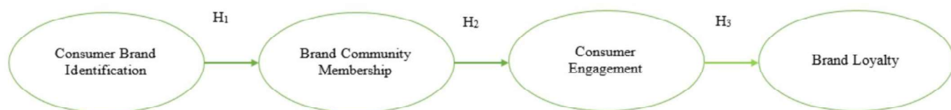
Figure 10 Theoretical Model
