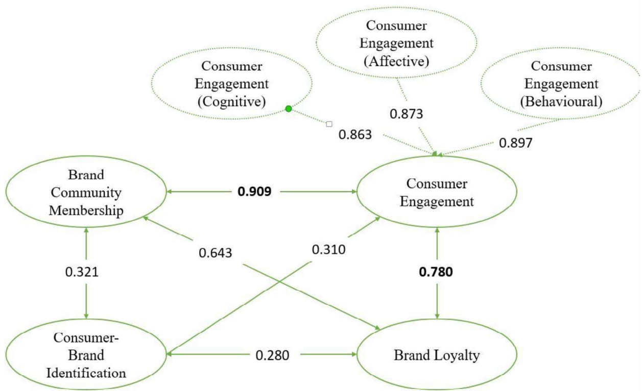
Figure 11 Summary of the Path Coefficients
