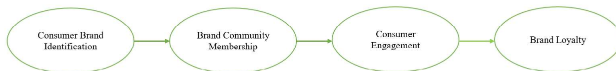
Figure 1 Theoretical Model
