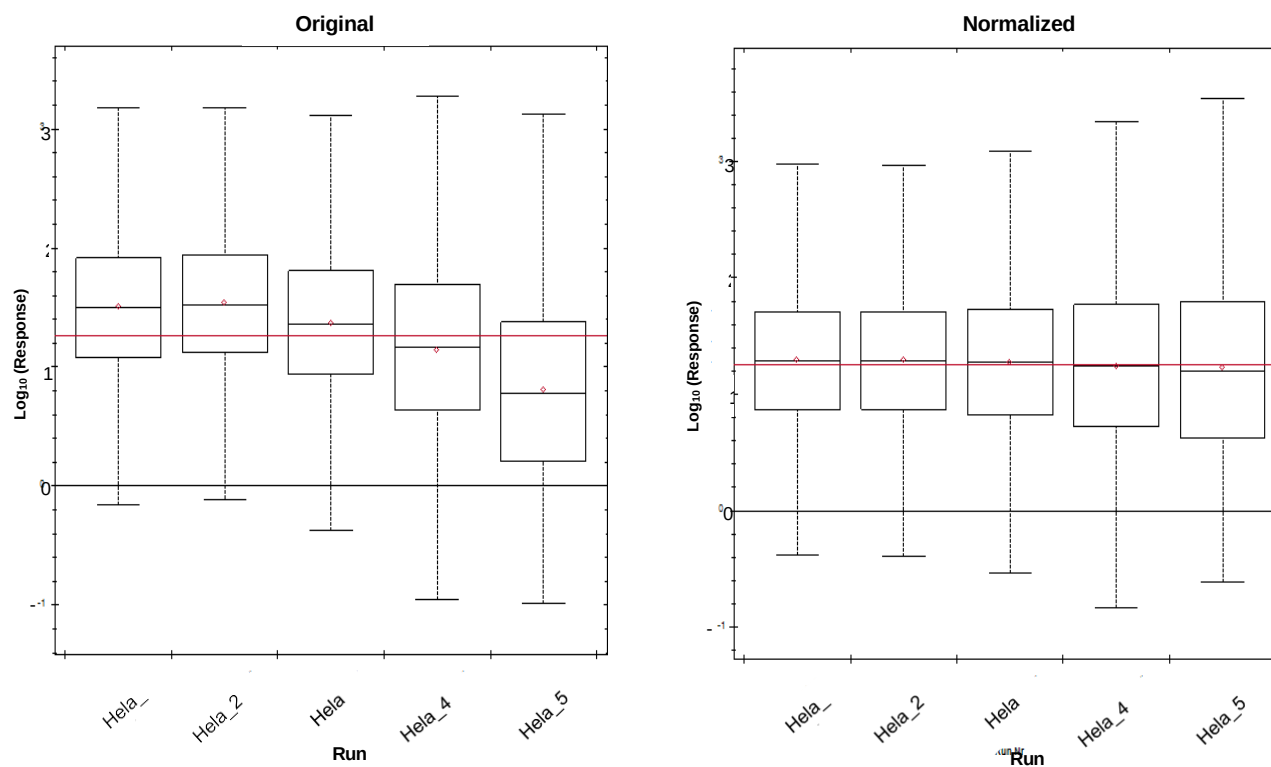
Figure 6.2: Boxplots indicating the original and normalised ( \log_{10} ) response signal for the Hela_QC replicates analysed over 5 days. The signal of the original responses of the 5 Hela_QC replicates was normalised around the median of the data.
