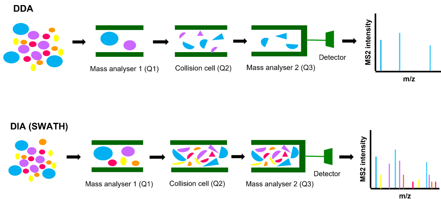
Figure 1.8: Schematic diagram of DDA and DIA (SWATH) acquisition methods during untargeted tandem mass spectrometry analysis.
