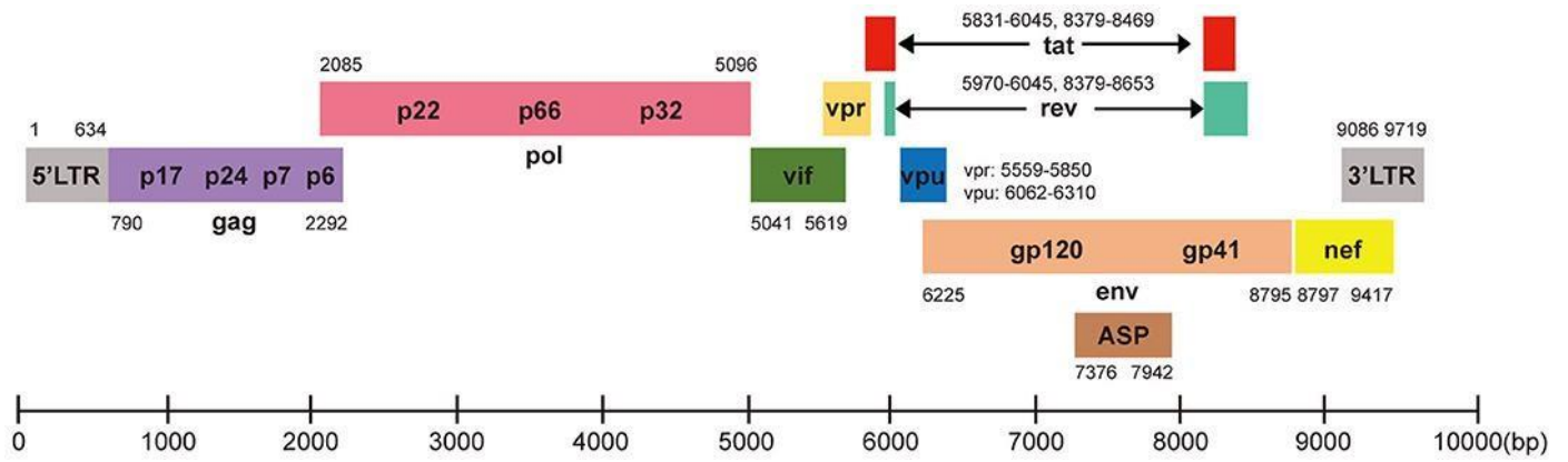
Figure 1.2: Diagram of HIV-1 RNA genome structure. Diagram shows open reading frames of structural and regulatory HIV-1 genes encoded between a 5' and 3' long term repeats. Figure taken from Xiao et al., 2019.
