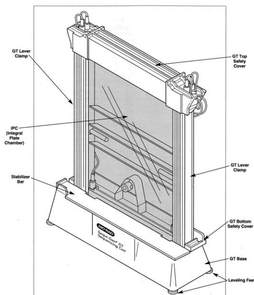
Figure 5.2 Sequi-Gen GT nucleic acid electrophoresis cell (BioRad Instruction Manual)
