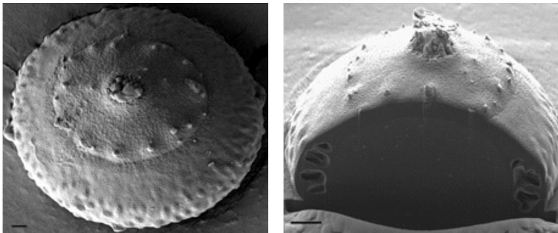
Figure 1. External view of a whole pollen grain of Isoglossa glandulosa and a cross-section of the same grain cut by FIB-SEM. Scale bars = 3 \mu\text{m} .
