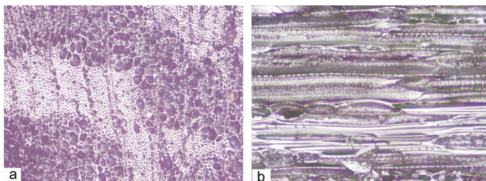
Figure 1. Photomicrographs of charcoal from Stratum 4d, sample M28-0-5cm-B, Heteromorpha arborescens . a , transverse section showing clustered vessels in a dendritic arrangement; b , tangential longitudinal section showing tracheids with spiral thickenings and uniseriate rays.
