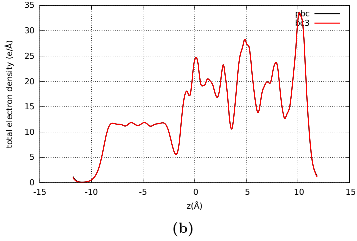
Figure 4.2: The graphs of the potential (a) and the electron density (b) for the system \text{AlH}_2\text{ONa} , when there is insufficient vacuum between the electrode and the ESM medium. ESM1 represents vacuum and ESM2 represents a metal. The red curve (labelled bc3) is for the charged system. The black curve (labelled pbc) is a reference system where the periodicity of the system is preserved. For pbc the system is not charged and for bc3 the system is charged.
