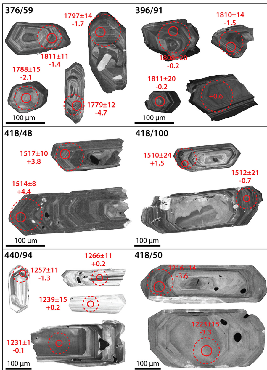
Fig. 3. Representative cathodoluminescence (CL) images of zircon grains from the studied igneous samples. Also shown are laser spot positions for U–Pb dating (solid circles) and Hf isotope analyses (dashed circles), as well as U–Pb ages (Ma) and \epsilon_{\text{Hf}(t)} values for each spot. U–Pb age errors are 1 sigma.
