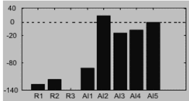
Figure 15. comparative returns over 200 hands.
