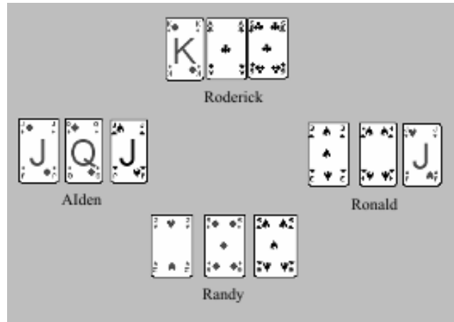
Figure 18. Agent bluffing
