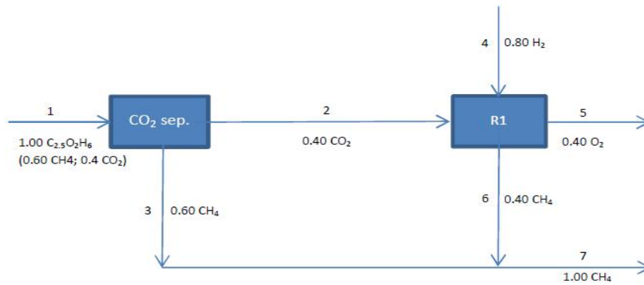
Figure 6.9: Electro-catalytic reduction of CO 2 using H 2 to produce methane
