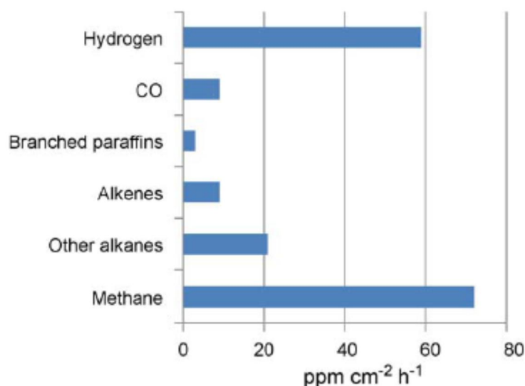
Figure 2.14: Product yield from Nitrogen-doped nanotubes (Centi and Perathoner, 2009)
