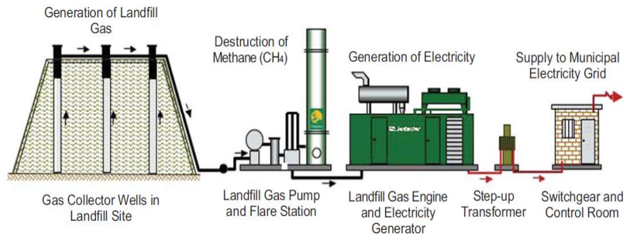
Figure 1.1: Schematic layout of Landfill gas to Electricity Project (Interwaste Environmental Solutions, 2010)
