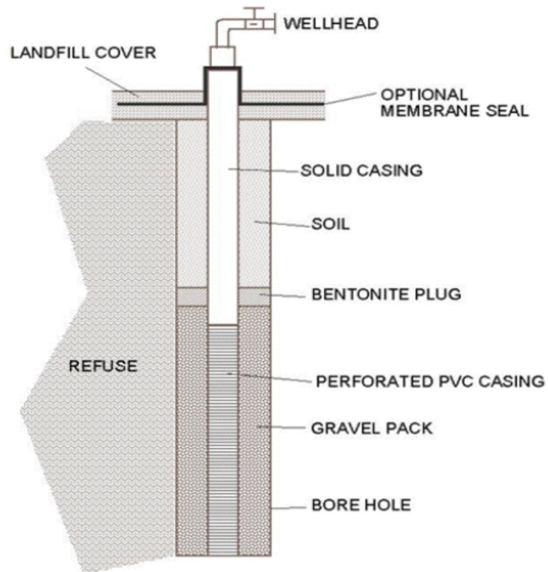
Figure 2.3: Vertical LFG extraction wells (U.S. EPA LMOP, n.d)
