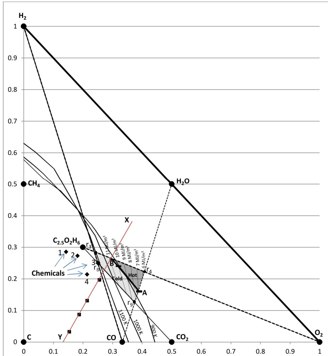
Figure 6.28: CHO diagram for Feed 1 – representing locus of chemicals
