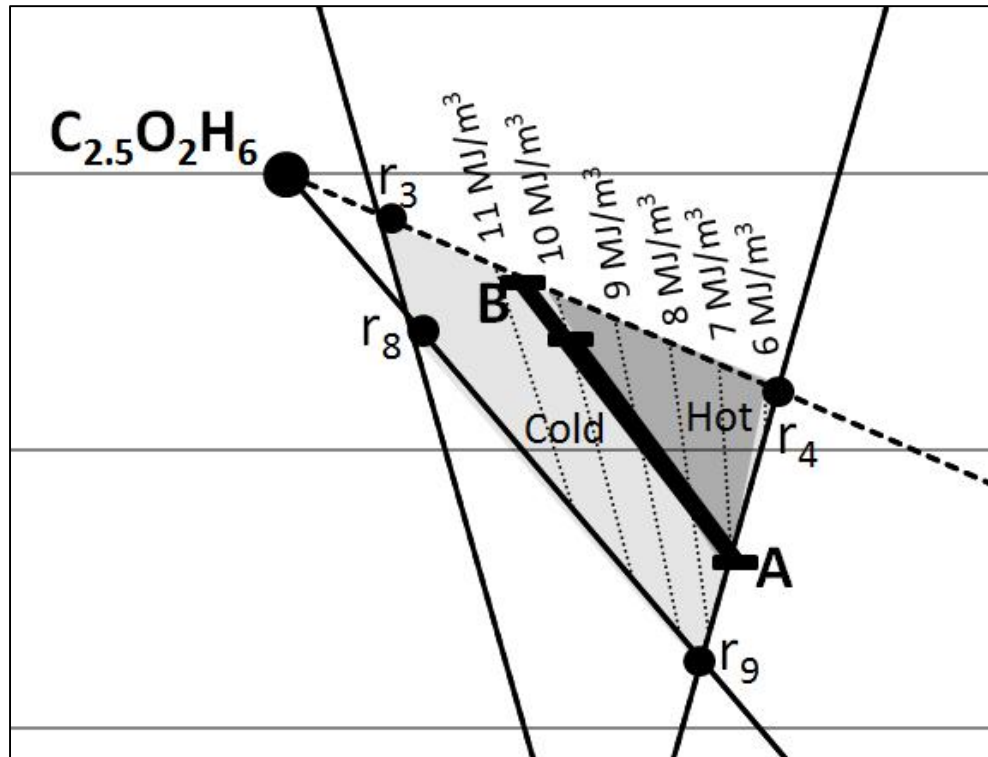
Figure 5.3: Close up Representation of HHV – Feed 1
