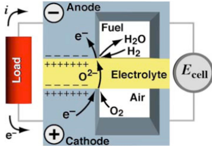
Figure 2.12: Practical SOFC with three phase boundary to facilitate charge transfer (Kee et al., 2004)
