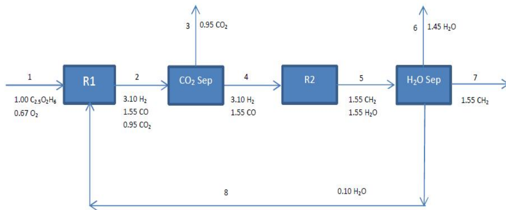
Figure 6.14: CH 2 production using Feed 2 with a H 2 O recycle stream
