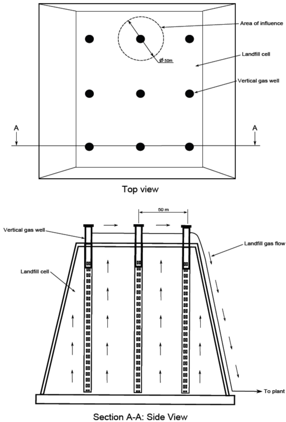
Figure 2.5: The area of influence and spacing of vertical gas wells (Swanepoel, 2009)
