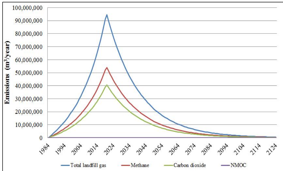
Figure 1.2: Emissions Evolution Curve for Coastal Park (Theeboom and Nontangane, 2010)
