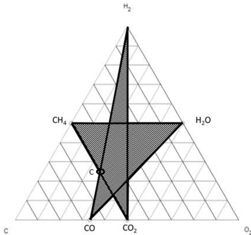
Figure 4.2: The Star of Gasification
