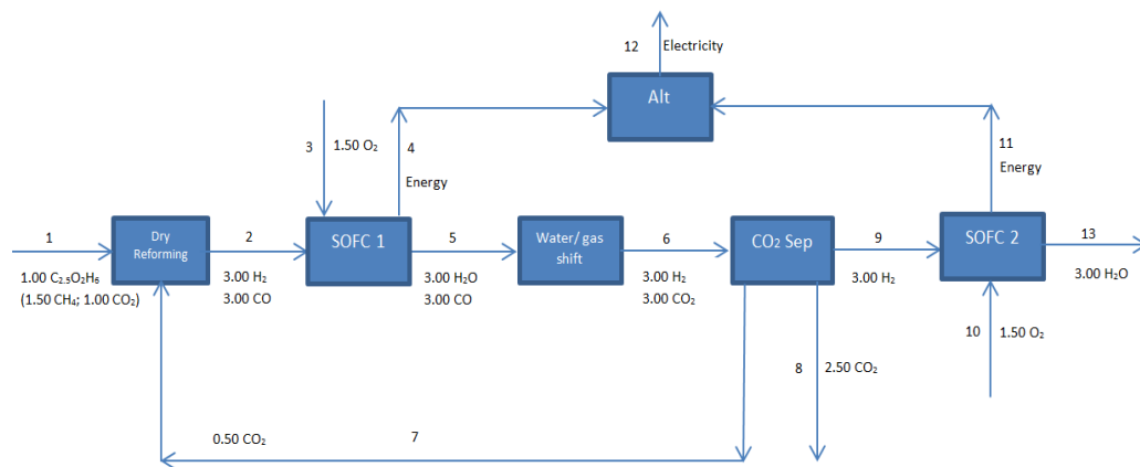
Figure 6.4: Electricity generations using SOFC's and dry reforming – Feed 1
