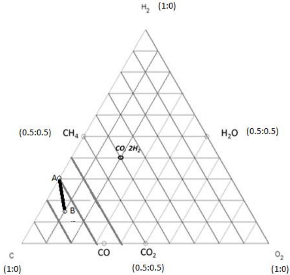
Figure A1: CHO Diagram
