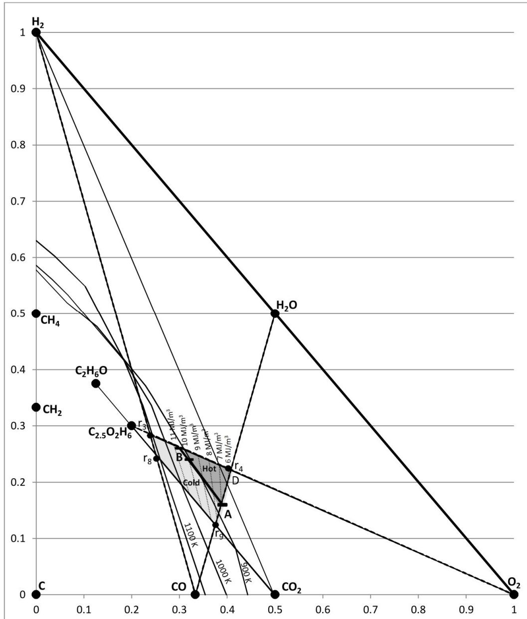
Figure 6.22: DME production using Feed 1 with a CO 2 recycle stream
