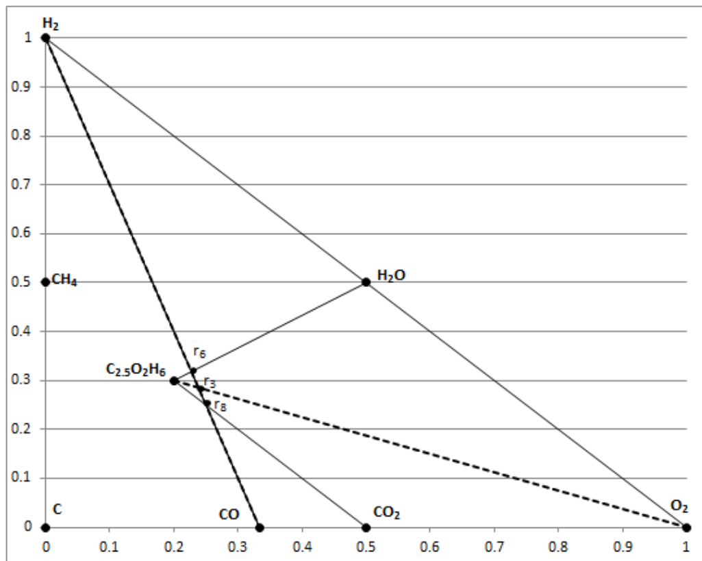
Figure 4.5: Graphical representation of LFG reactions using Feed 3
