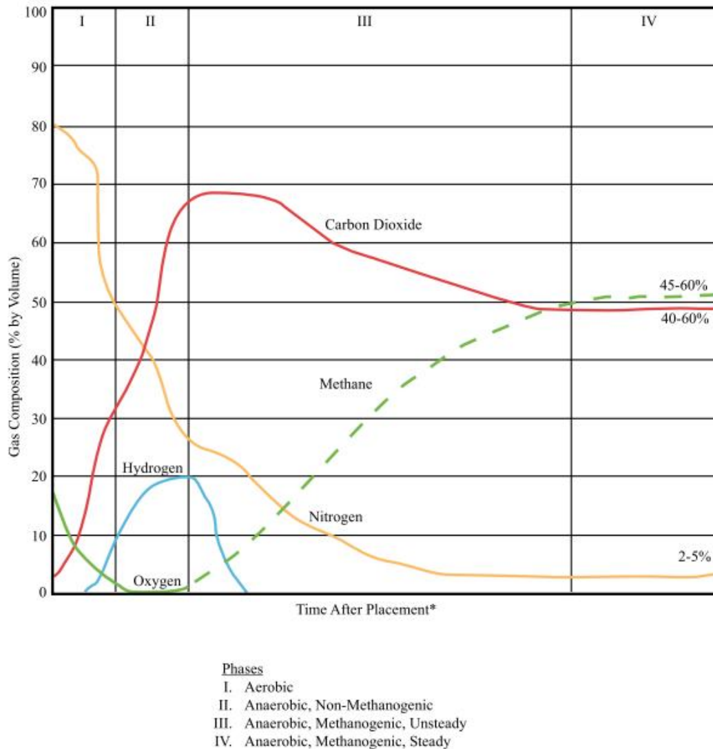
Figure 2.2: Changes in Typical LFG composition after Waste disposal (Berger and Mann, 2001)
