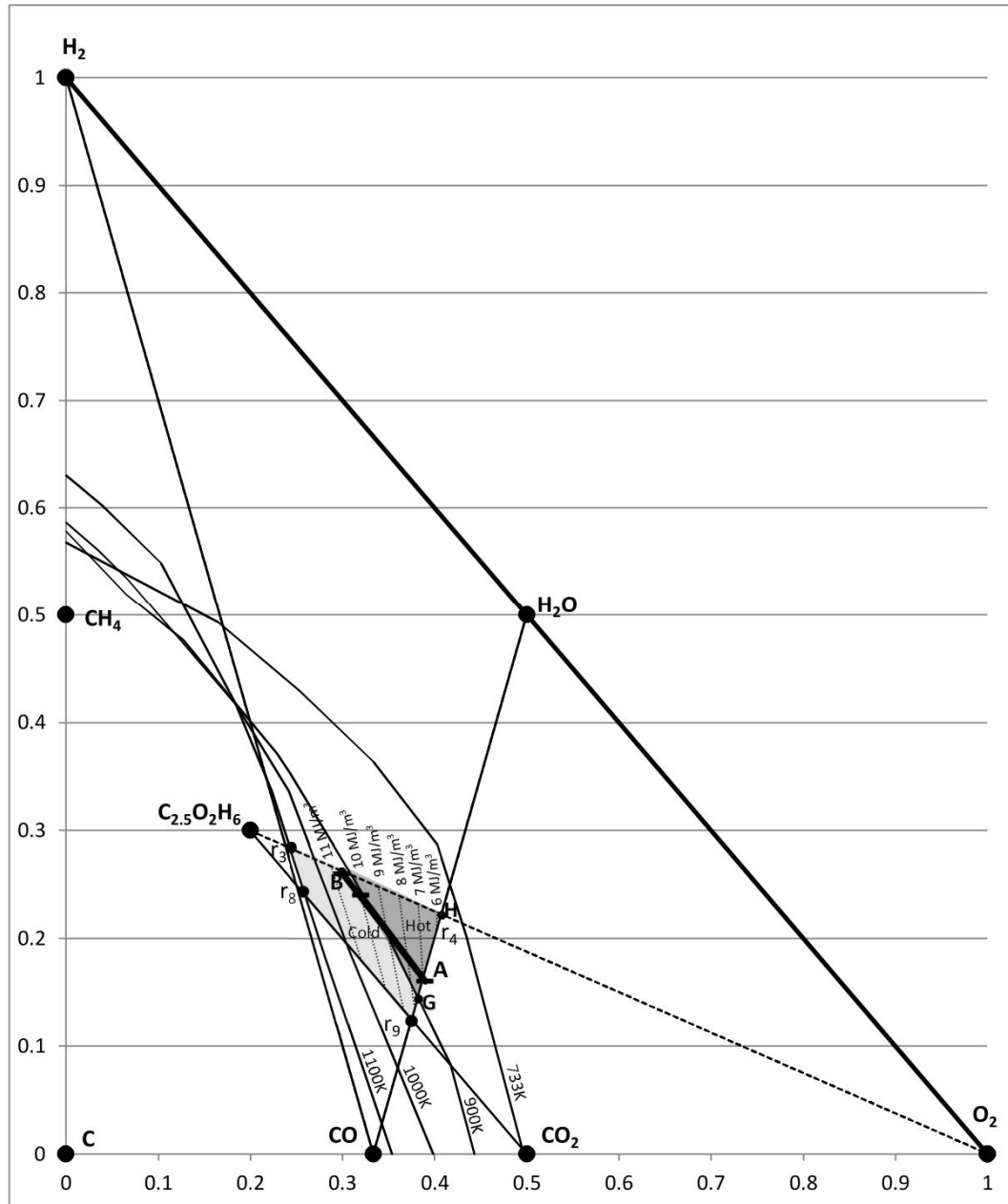
Figure 5.5: Thermally balanced line, carbon boundaries and calorific value contours for Feed 1
