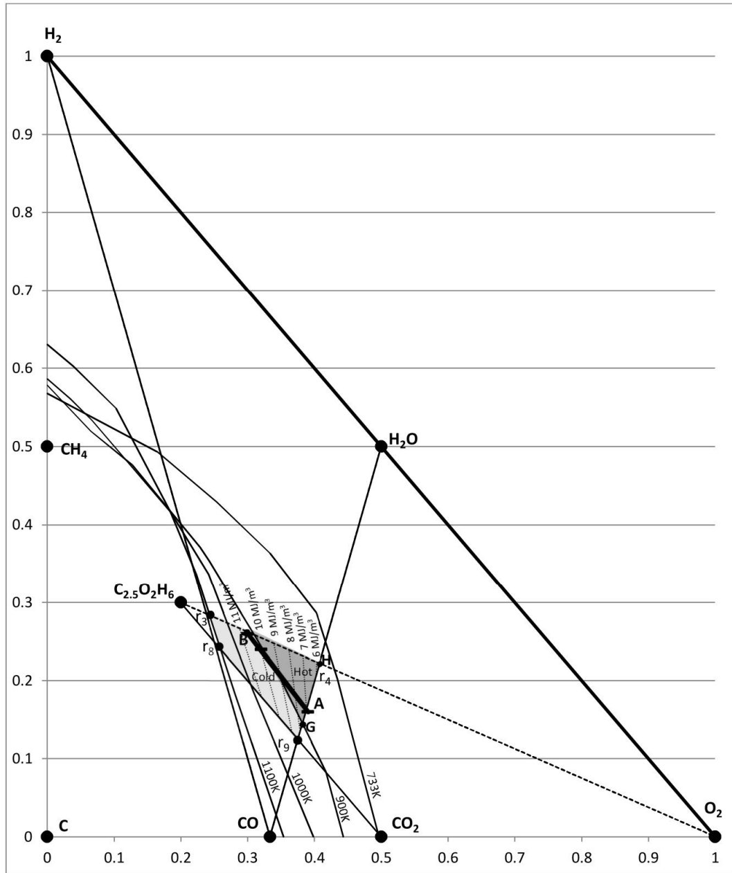
Figure C1: Representing Calorific Value Contours on the CHO Diagram for Feed 1.
