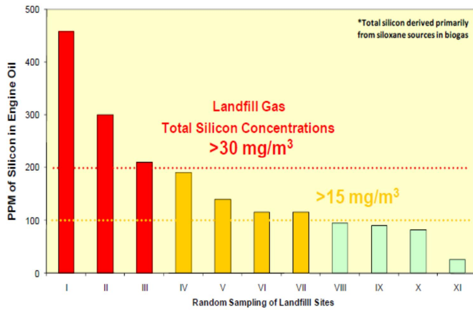
Figure 2.9: One third of all landfill sites have a severe siloxane problem (Xebec Adsorption Inc., 2007)
