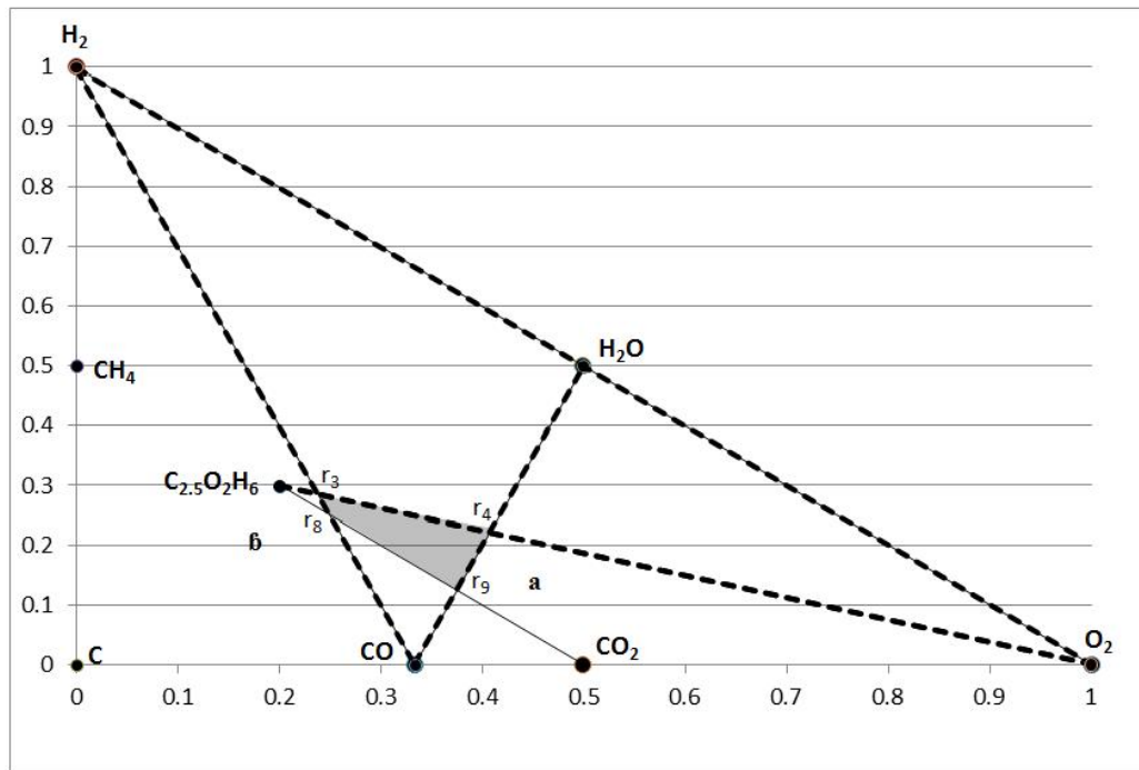
Figure 4.3: Graphical representation of LFG reactions using Feed 1
