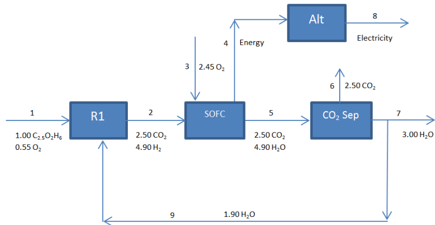
Figure 6.5: Electricity generations using SOFC's and Feed 2
