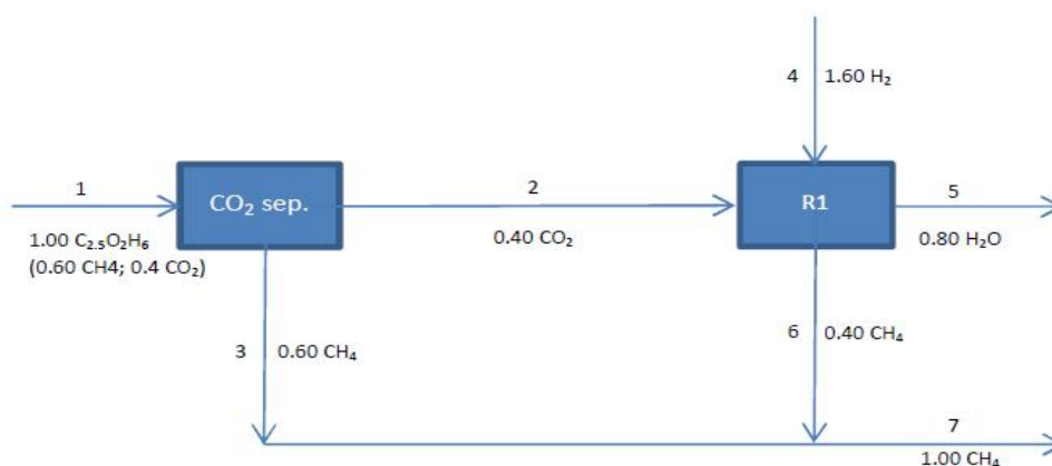
Figure 6.10: Production of methane using the Sabatier reaction
