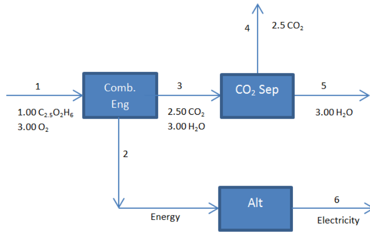
Figure 6.1: Electricity generation using an Internal Combustion Engine.
