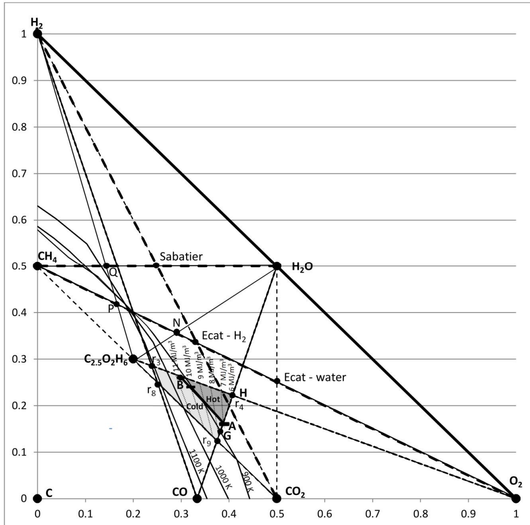
Figure 6.11: Methane generation using Feed 1
