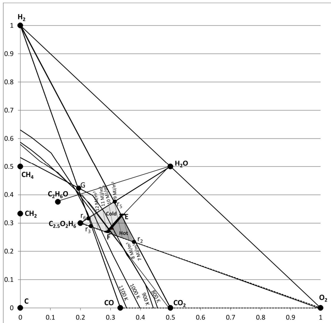
Figure 6.24: DME production using Feed 2
