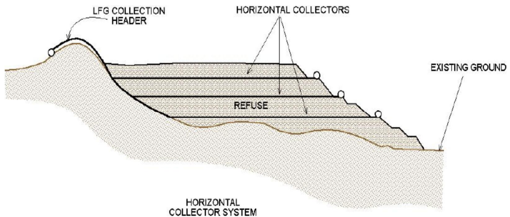
Figure 2.4: LFG Collection system with horizontal Trenches (U.S. EPA LMOP, n.d)
