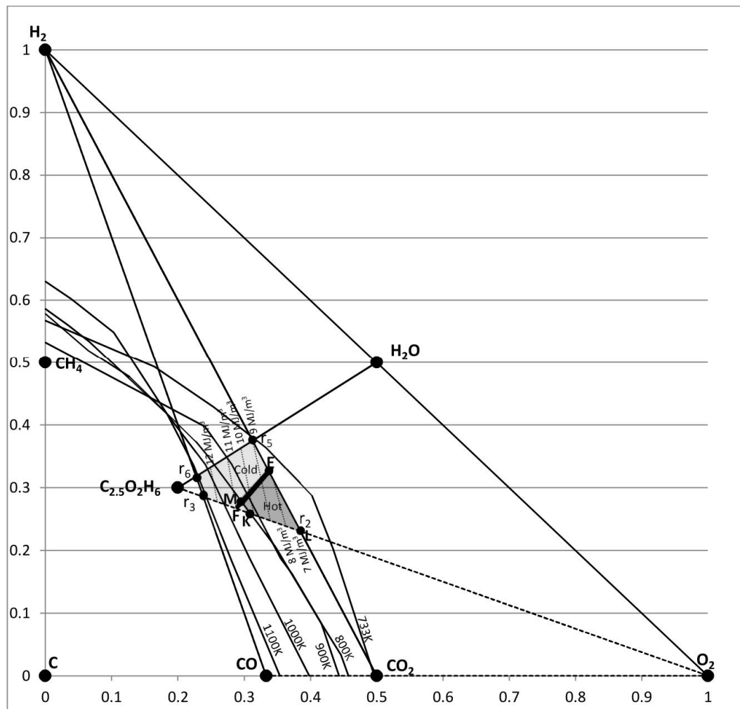
Figure C2: Representing Calorific Value Contours on the CHO Diagram for Feed 2.
