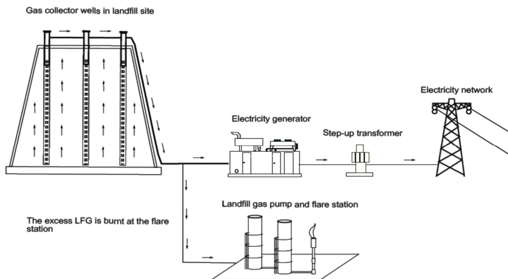
Figure 2.11: The flow of LFG from extraction to electricity generation (Swanepoel, 2009)
