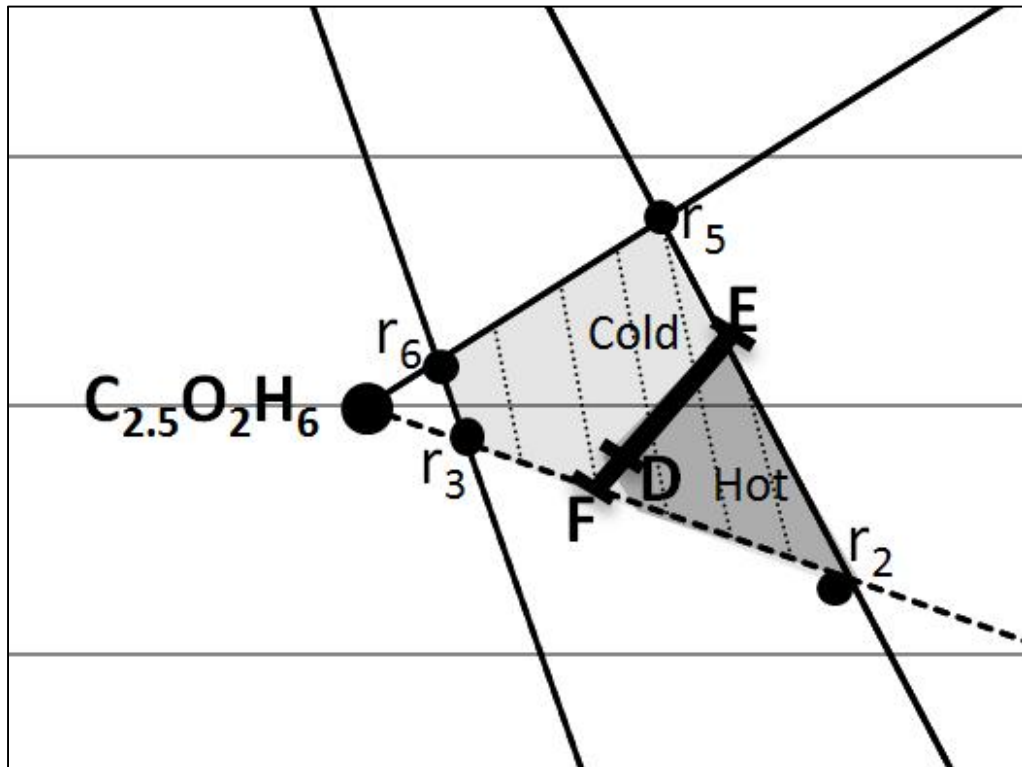
Figure 5.2: Indicating the TBL - Feed 2
