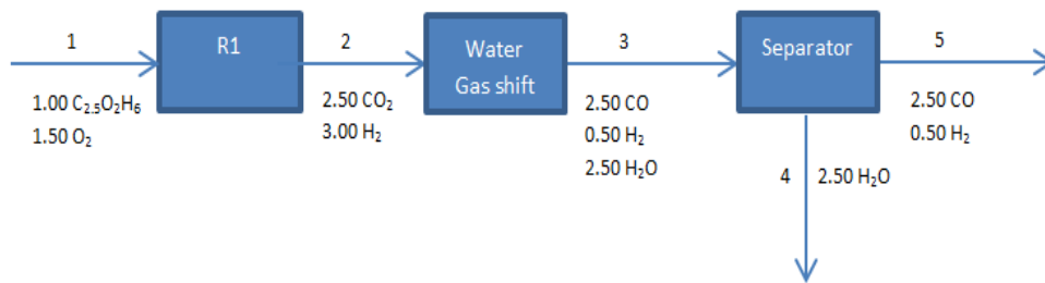
Figure 6.27: Production of syngases with zero emissions – Feed 2 ( r_2 )
