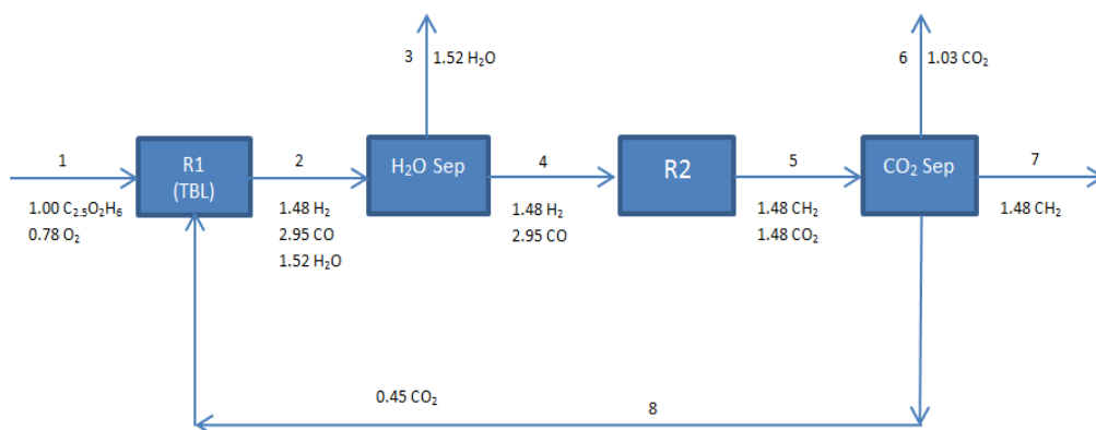
Figure 6.13: CH 2 production using Feed 1
