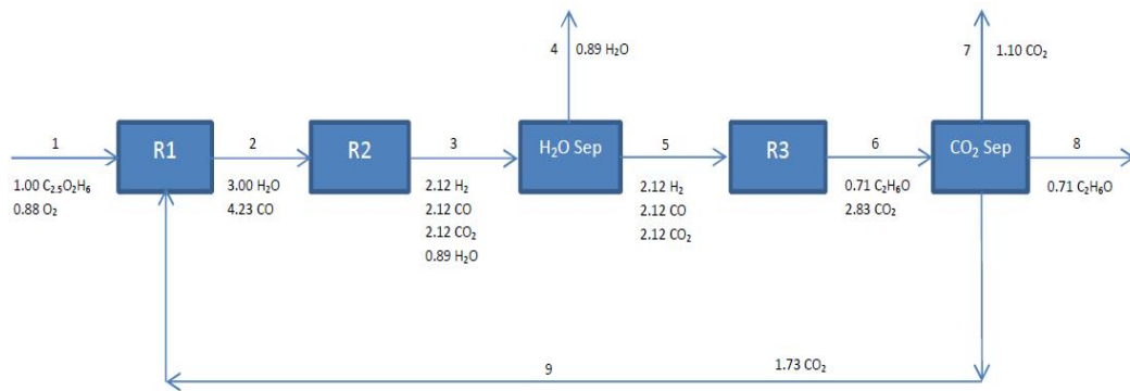
Figure 6.19: DME production using Feed 1 with a CO 2 recycle stream
