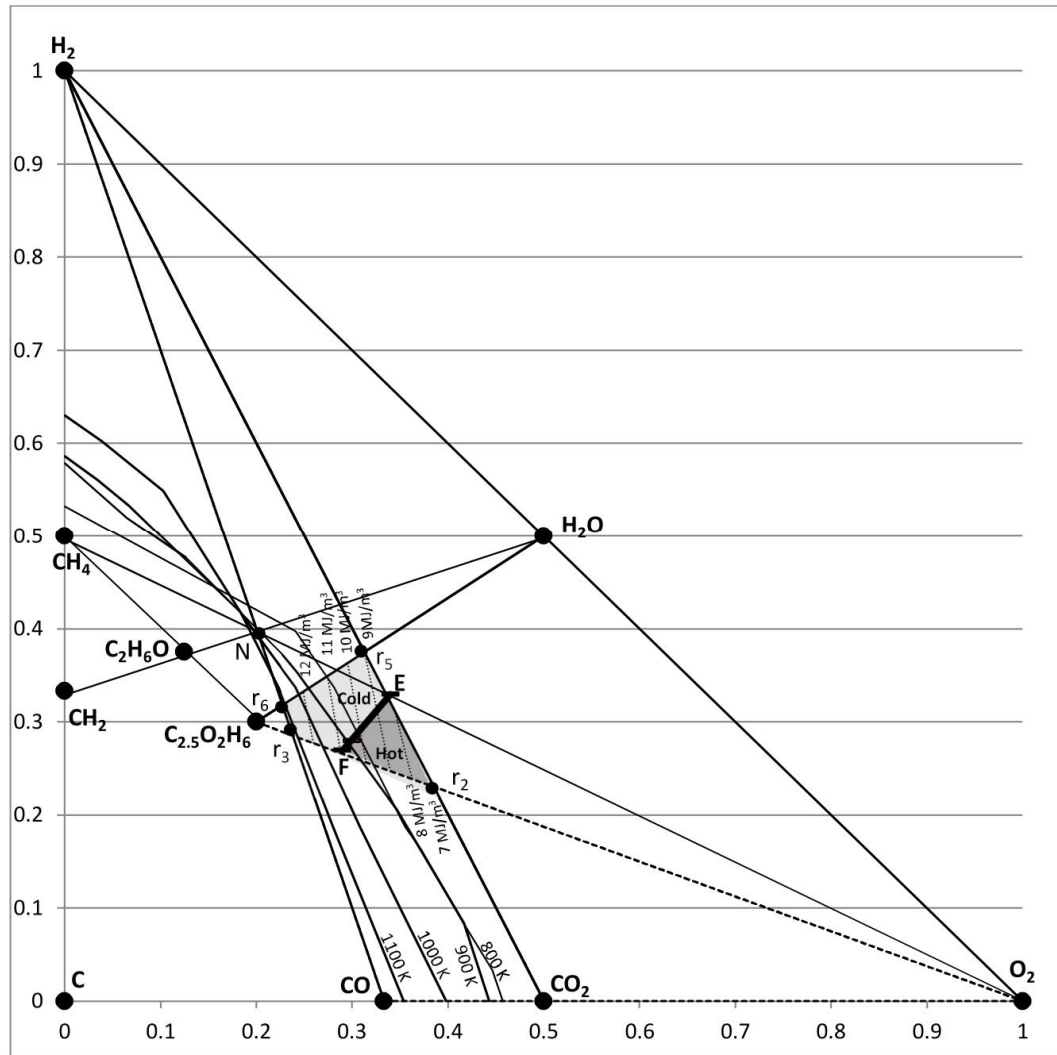
Figure 6.18: CH 2 production using Feed 2 – CO 2 elimination
