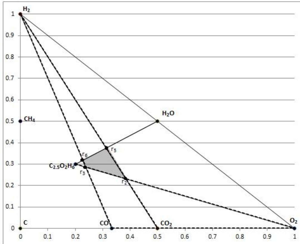
Figure 4.4: Graphical representation of LFG reactions using Feed 2
