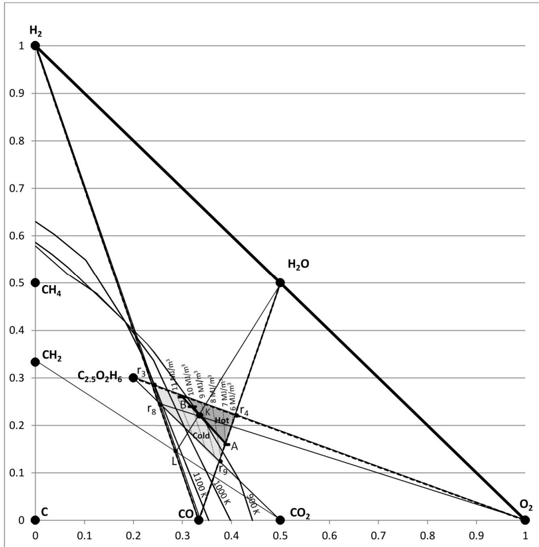
Figure 6.16: CH 2 production using Feed 1
