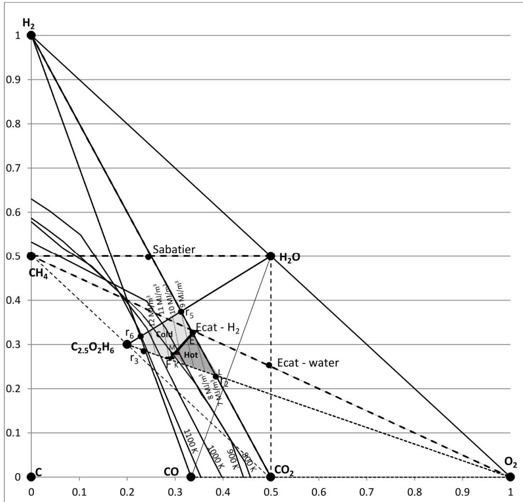
Figure 6.12: Methane generation using Feed 2
