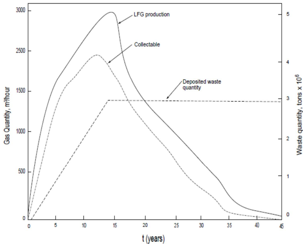
Figure 2.1: Landfill gas production over the course of time (Koch, 2001)
