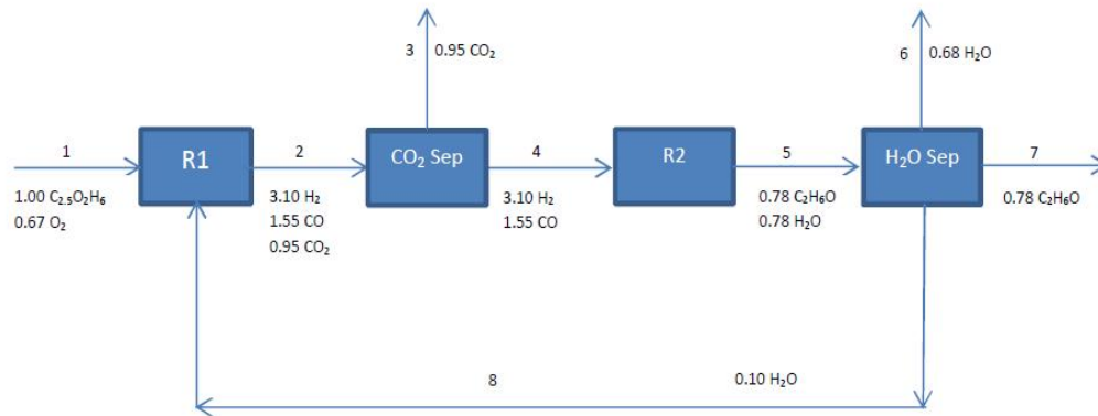
Figure 6.21: DME production using Feed 2
