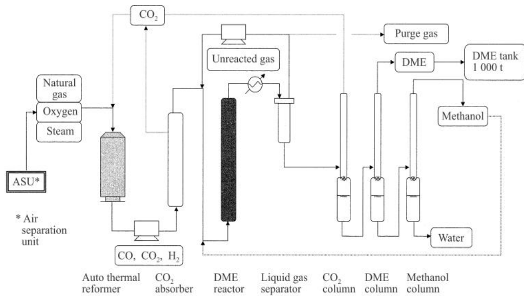
Figure 2.15: Process flow diagram of 100 t/day DME synthesis plant (Yotaro et al., 2006)
