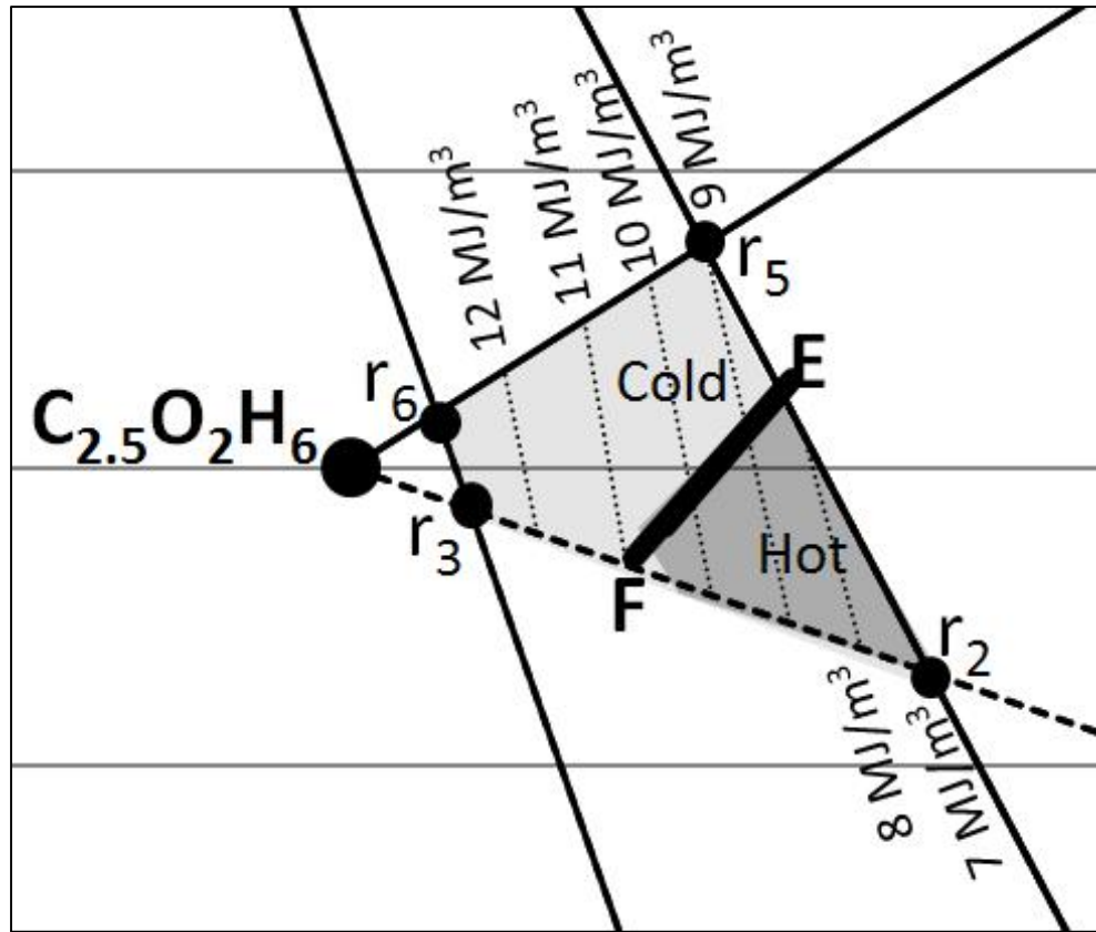
Figure 5.4: Close up Representation of HHV – Feed 2
