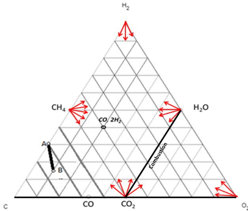
Figure 4.1: CHO Diagram
