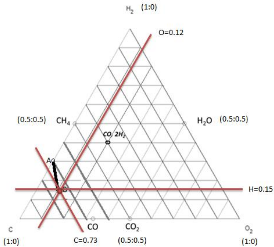
Figure A2: Representing mixtures
