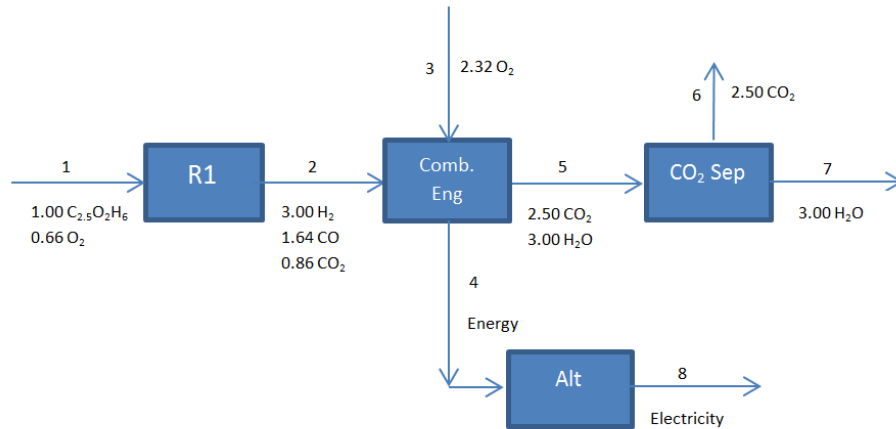
Figure 6.3: Electricity generation using an Internal Combustion Engine represented on the TBL – Feed 2
