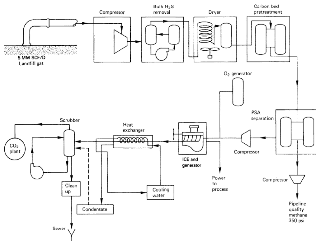
Figure 2.8: Removal of H 2 S for CO 2 , methane and electricity production (Malik et al., 1987)
