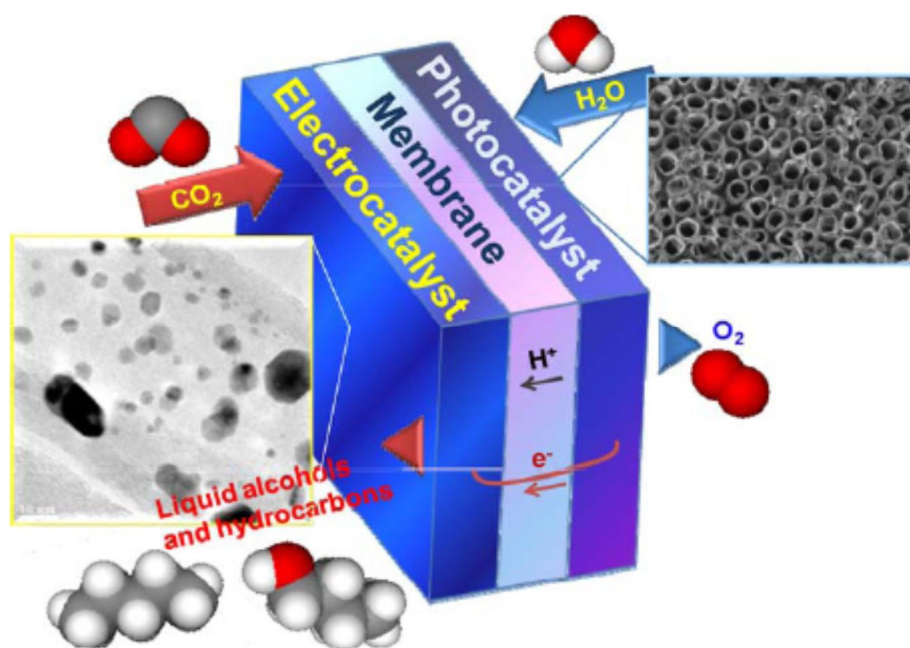
Figure 2.13: Simplified scheme of a photo-electro-catalytic device for \text{CO}_2 reduction to fuels using solar energy (Centi and Perathoner, 2009)
