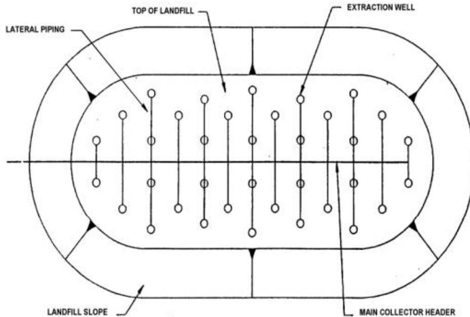
Figure 2.7: LFG Extraction site plan (U.S. EPA LMOP, n.d)
