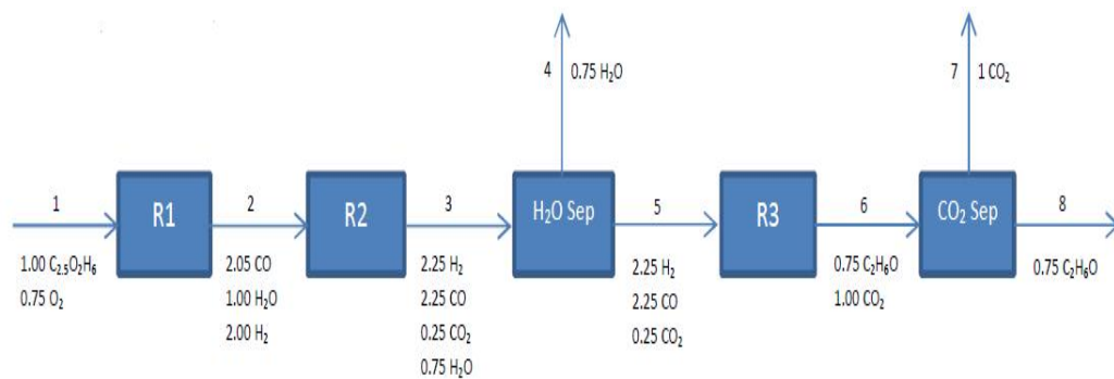
Figure 6.20: DME production using Feed 1 without a CO 2 recycle stream
