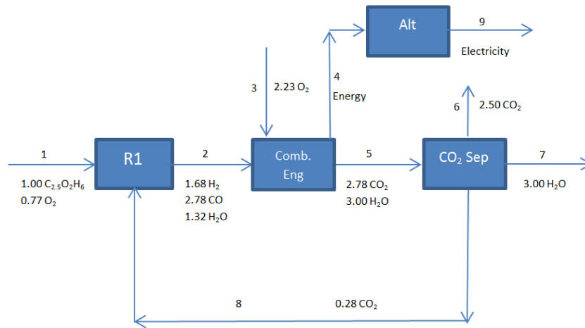
Figure 6.2: Electricity generation using an Internal Combustion Engine represented on the TBL – Feed 1.
