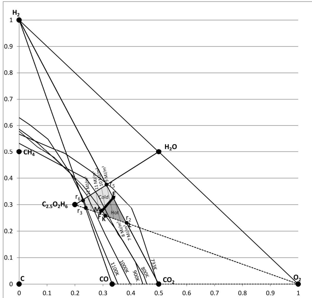
Figure 5.6: Thermally balanced line, carbon boundaries and calorific value contours for Feed 2
