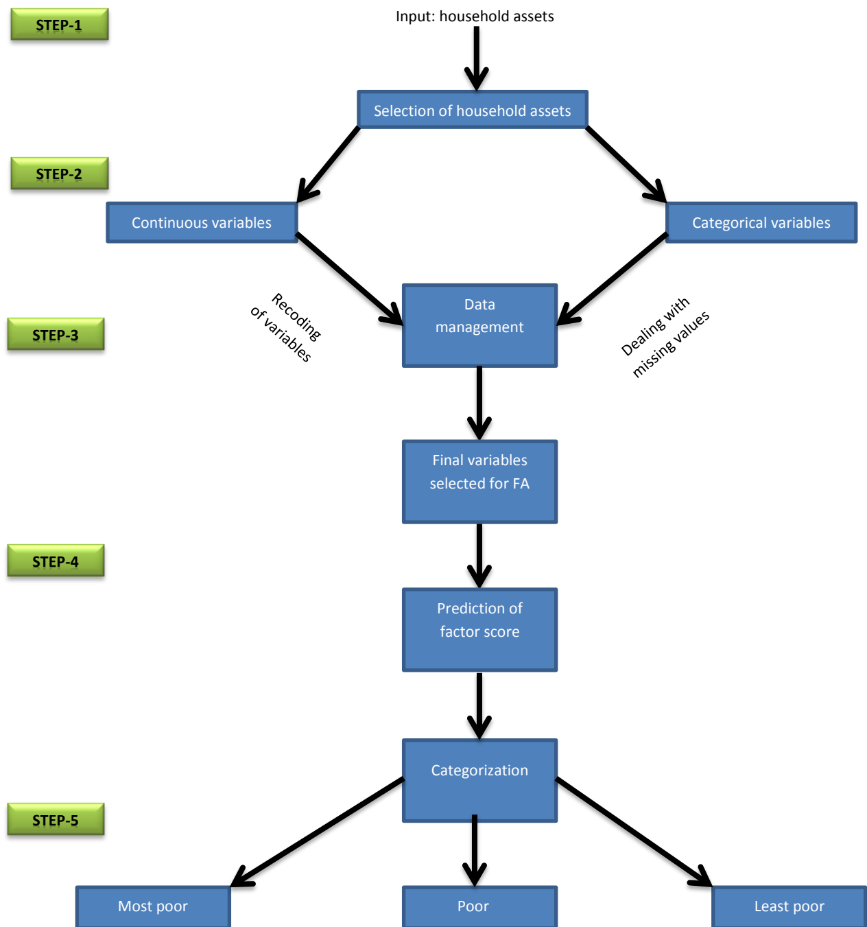
Figure 5: Flowchart to determine SES using factor analysis technique
