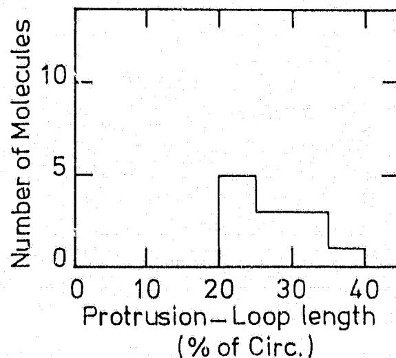
Fig. 11(b). Distribution of Protrusion-Loop distances. The distance between the single strand loop and the nearest protrusion was measured. Note that the minimum distance observed is 20-25 percent of the total molecule length. Also note, that the distribution decreases towards increasing percentages. This implies that the relative insertion has occurred 20-25 percent from that end of the molecule, distal to the pac site. A location of 20-25 percent from the pac site would have led to a distribution exhibiting a maximum at the insertion/deletion site (as observed) but a decrease towards the axes origin.
