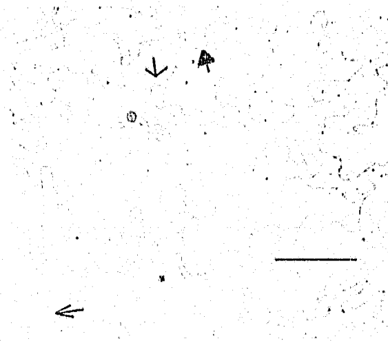
Fig. 5. Electron micrograph of an \alpha 3 genome and ColE1 plasmids. Phage \alpha 3 genome lengths were measured with respect of ColE1 present in the same field. Bar indicates 1 \mu\text{m} . Phage \alpha 3 \leftarrow ; plasmid ColE1 \leftarrow .
