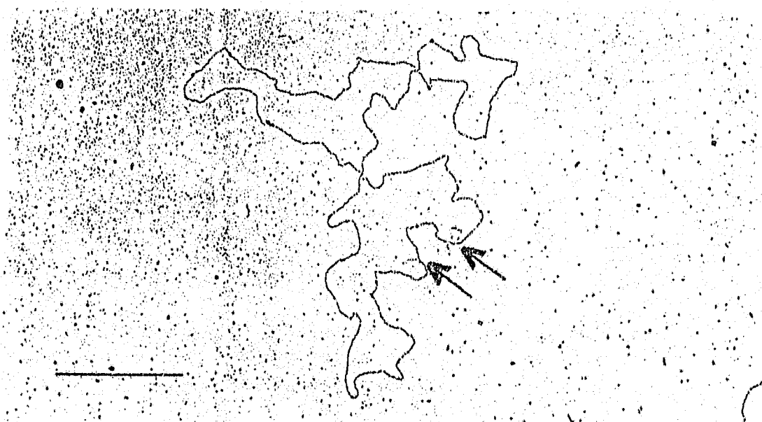
FIG 10(a). Homoduplex of \alpha 3 . Denaturation-renaturation of \alpha 3 DNA was found to result in circularisation. Two single strand protrusions are observed (arrows), which are due to terminal redundancy in permuted molecules. Single strand protrusions were found to be 2.4 \pm 0.8 percent of the phage genome, as determined from 40 molecules. Bar represents 1 \mu\text{m} .
