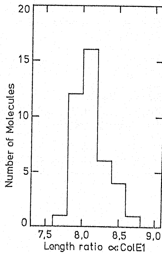
Fig. 6. Distribution of \alpha 3 genome lengths with respect to the length of plasmid ColE1. The length of the \alpha 3 genome was found to be 8,2 \pm 0,2 times the length of plasmid ColE1. This was converted to kilobases ( 51,98 \pm 1,29 kb) and subsequently to molecular weight ( 34,66 \pm 1,95 Md).
