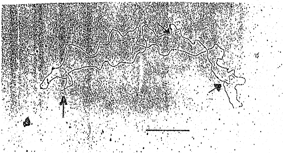
Fig. 10(b). Heteroduplex of \alpha 3 . A second class of circular molecules was observed from the DNA of the \alpha 3 stock lysate. These possessed, in addition to the two single strand protrusions, a single strand loop (arrow). This suggests a dual phage population, namely one with an insertion or deletion in its genome with respect to the other. The single strand loop was observed and measured on 12 molecules as 2.0 percent of the genome length. Single strand protrusions \leftarrow .
