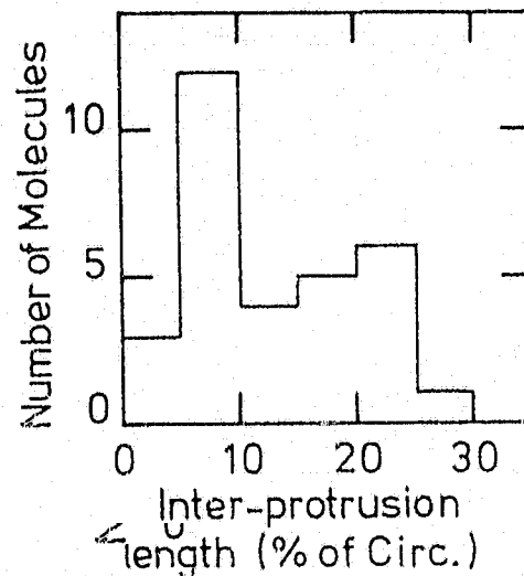
Fig. 11(a). Distribution of inter-protrusion distances. These were measured in 40 molecules and plotted. Such a distribution should mimic that of the end point distribution of Fig. 9b (Pretorius and Coetzee, 1979), having a cut off point at 27 percent. However, an upward trend is observed at 20-25 percent, and this is explained in terms of the erroneous inclusion of ill-resolved heteroduplexes.
