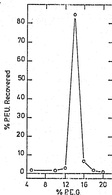
Fig. 3. Precipitation of phage by polyethylene glycol 6000 (PEG). One hundred ml. aliquots of \alpha 3 lysate ( 10^9 p.f.u./ml) were made 0,5M with NaCl and PEG was added at varying concentrations. After the PEG was dissolved, the lysate was stored at 4^\circ\text{C} overnight. Precipitated phage was pelleted at 10 000 r.p.m. for 5 minutes in a Sorval SS-4 bench centrifuge rotor S-34 and resuspended overnight in 1,0 ml saline. After a clarifying spin, this was titred and percent phage at each PEG concentration was calculated.
