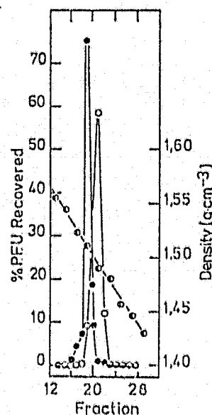
Fig. 4. Percent plaque forming units recovered and density vs. fraction number. Phages \alpha 3 and 5006M were centrifuged in CsCl to form a gradient. Fractions were titrated and results are presented as percent phage recovered from relevant fractions. The buoyant density was calculated from the refractive index of each fraction. o-o phage \alpha 3 , o-o phage 5006M and o-o density.
