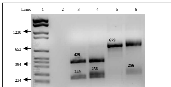
Figure E 15: Sac II screening of full length moaX with either 242G→C or 245G→C point mutations incorporated. Lane 1: Marker \lambda VI, Lane 2: Empty, Lane 3: Sac II digest of moaX carrying mutation 242G>C amplified with primer set moaX -F+ moaX -R, Lane 4: Sac II digest of moaX carrying mutation 242G>C amplified with primer set moaX ga1F+ moaX -R, Lane 5: Sac II digest of moaX carrying mutation 245G>C amplified with primer set moaX -F+ moaX -R, Lane 6: Sac II digest of moaX carrying mutation 245G>C amplified with primer set moaX ga2F+ moaX -R
