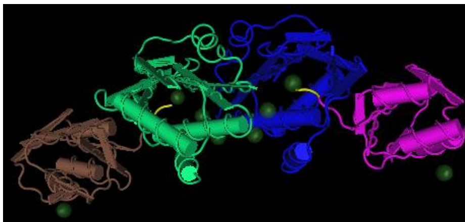
Figure 4.1: Crystal structure of E. coli MPT synthase enzyme. MoaD subunits are shown in brown and magenta while MoaE subunits are depicted in cyan and blue. Glycine residues involved in catalysis are shown in yellow.
