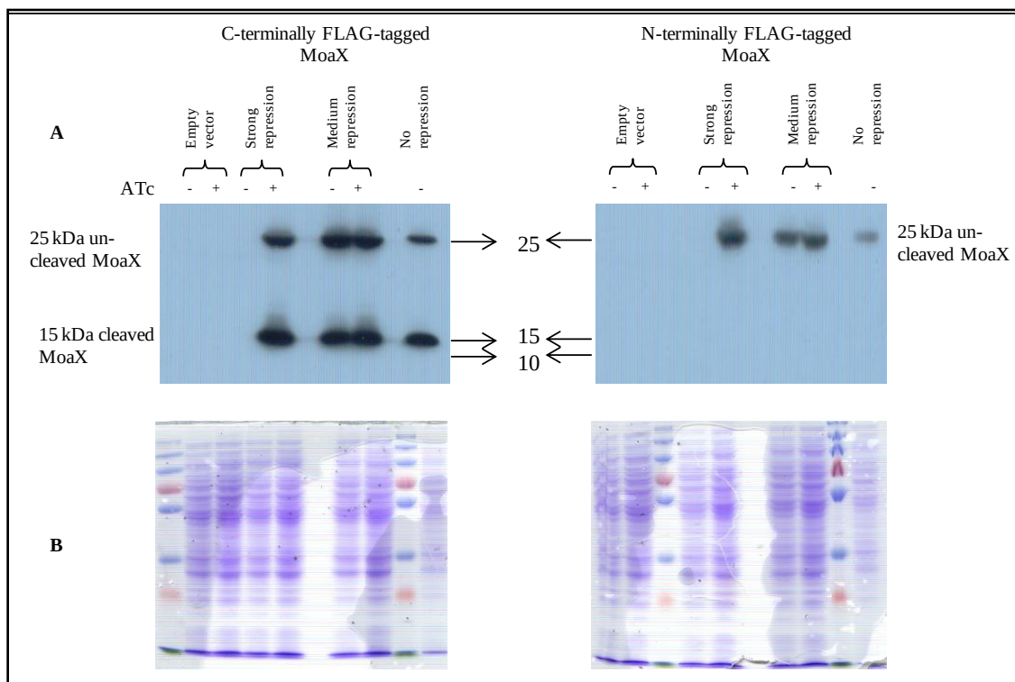
Figure 3.18: Western blot showing the post-translational cleavage of MoaX. (A) Western blots of N- and C-terminally FLAG tagged MoaX from strains grown in 7H9 and the presence or absence ATc (50 ng/ml). (B) Coomassie blue stained gels corresponding to the blots above them. These are images of one of three independent experiments.
