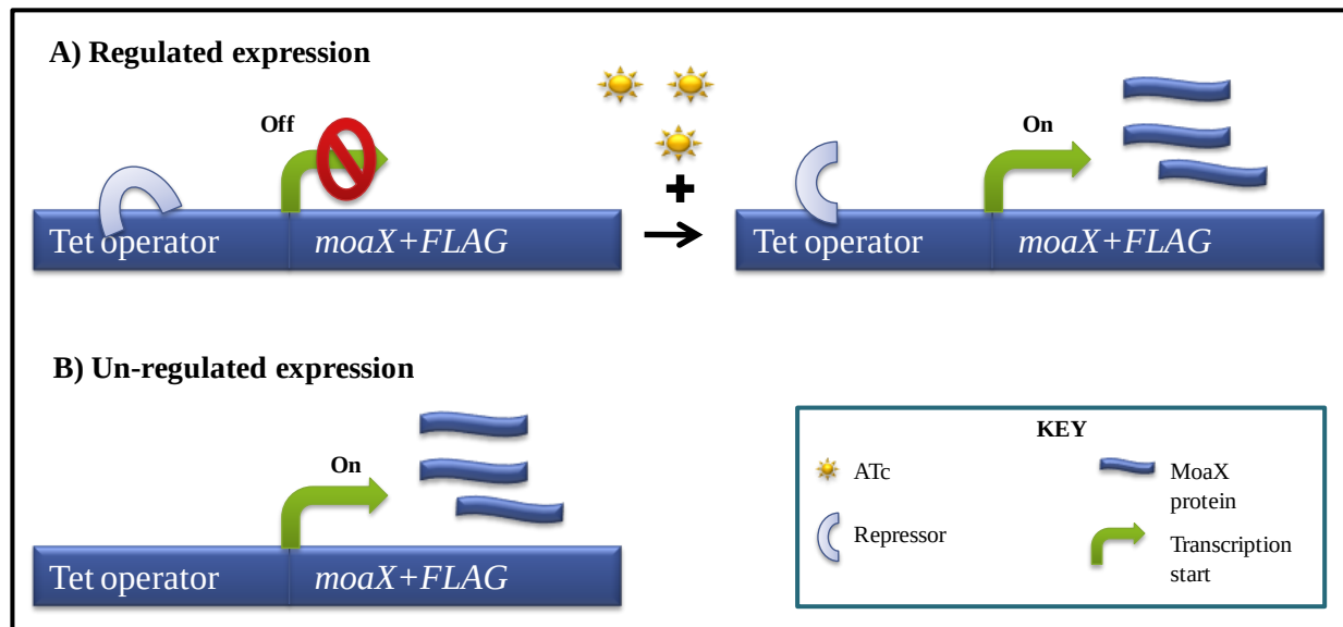
Figure 2.1: Schematic representation of the induction of moaX in the Tet system. (A) Regulated expression of moaX in the Tet system requires the addition of ATc which causes a conformational change in the repressor allowing transcription to proceed. (B) The unregulated expression of moaX takes place when no repressor is being expressed in the cell resulting in the constitutive expression of the gene of interest.
