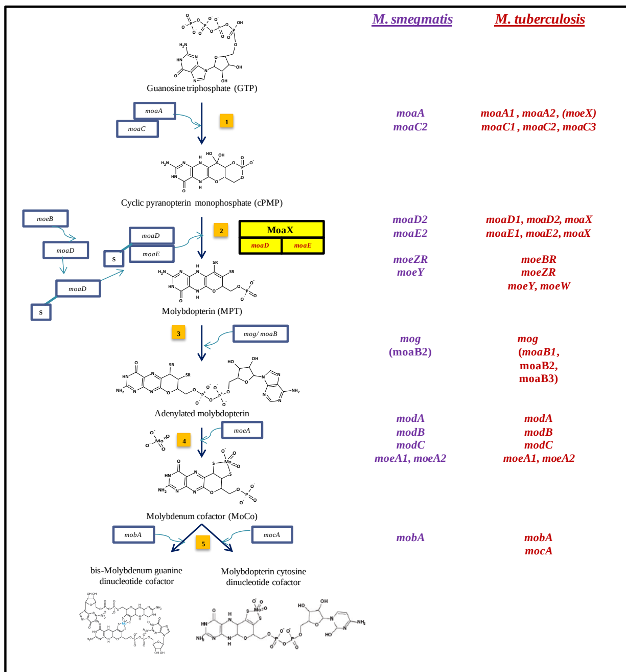
Figure 1.3: The highly conserved multi-step MoCo biosynthetic pathway in bacteria. Steps 1-5 are labeled in yellow boxes and the structures and names of each substrate and product are shown. The pathway is labeled according to the E. coli nomenclature for each of the genes involved (boxed in blue) while the M. smegmatis and Mtb homologues are listed in purple and red respectively. The black-bordered yellow box highlights Mtb MoaX which has been identified as a fused MPT synthase with homology to MoaD and MoaE (Williams et al. , 2011).
