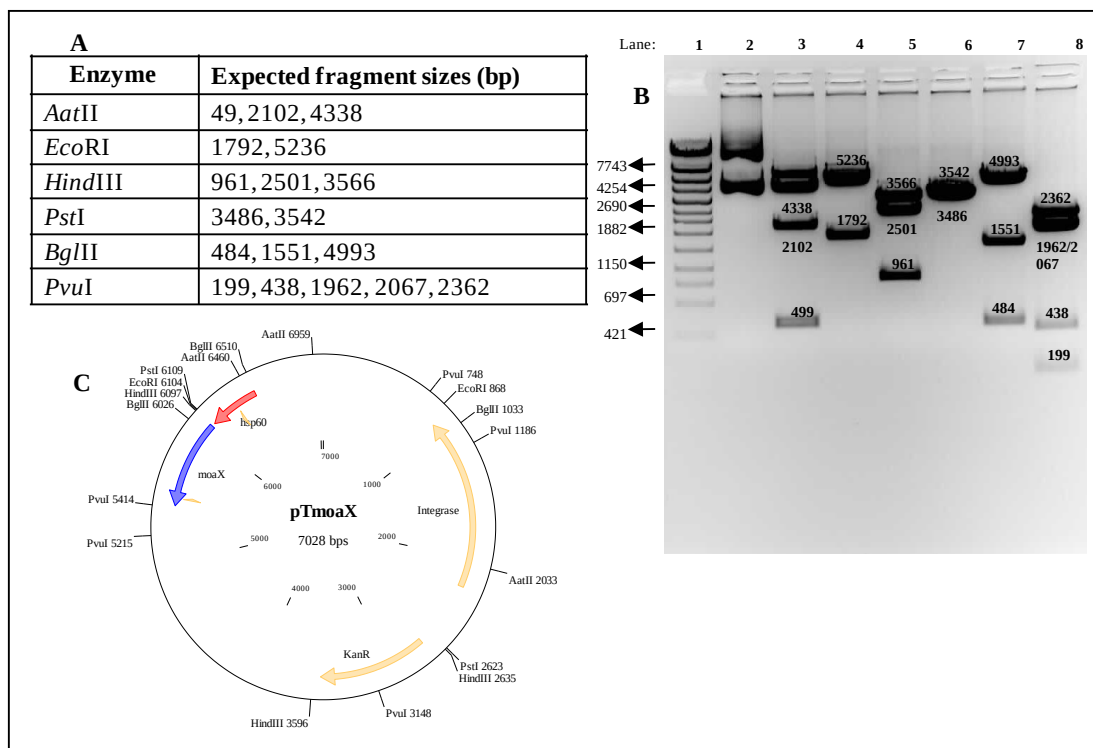
Figure E 5: Restriction analysis of integrating vector, pTmoaX carrying a single copy of moaX driven off the constitutive hsp60 promoter (A) Expected fragment sizes for restriction digests (B) Restriction digests of pTmoaX with several enzymes Lane 1: Marker \lambda IV, Lane 2: Uncut pTX, Lane 3: AatII digest, Lane 4: EcoRI digest, Lane 5: HindIII digest Lane 6: PstI digest, Lane 7: BglII digest, Lane 8: PvuI digest. (C) pTmoaX vector map showing cloned moaX in blue and the hsp60 promoter in red. The integrase and kan R genes are shown in yellow.
