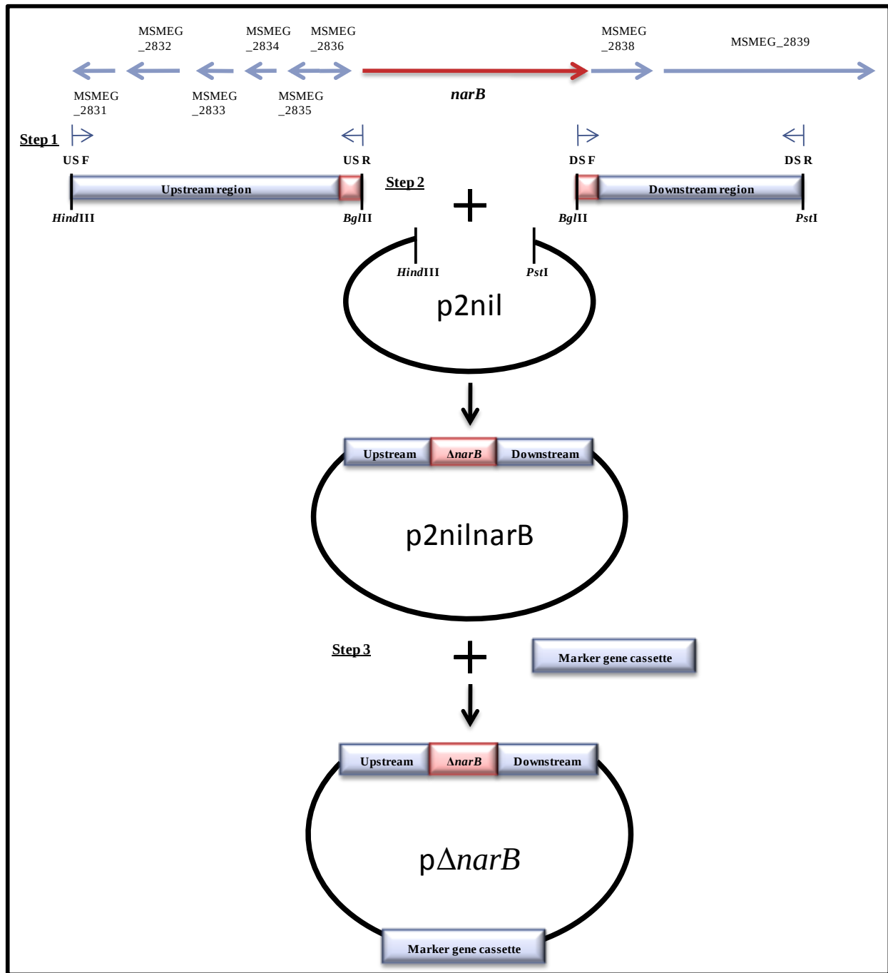
Figure 2.4: Schematic representation of the generation the suicide vector p \Delta narB. Step 1: Amplification of upstream and downstream regions by PCR with a high fidelity Taq polymerase. Step 2: Restriction digestion and ligation of the upstream and downstream regions to p2nil to generate the intermediate vector p2nilnarB. Step 3: Ligation of p2nilnarB with the selectable-counterselectable marker cassette to generate the suicide vector p \Delta narB.
