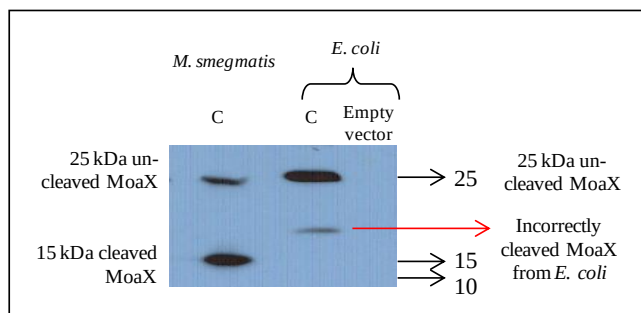
Figure 3.22: Western blot analysis of FLAG-tagged MoaX protein samples extracted from E. coli and M. smegmatis . C-terminally tagged MoaX from M. smegmatis serves as a positive control for cleavage. The blot shown is one of three independent experiments.
