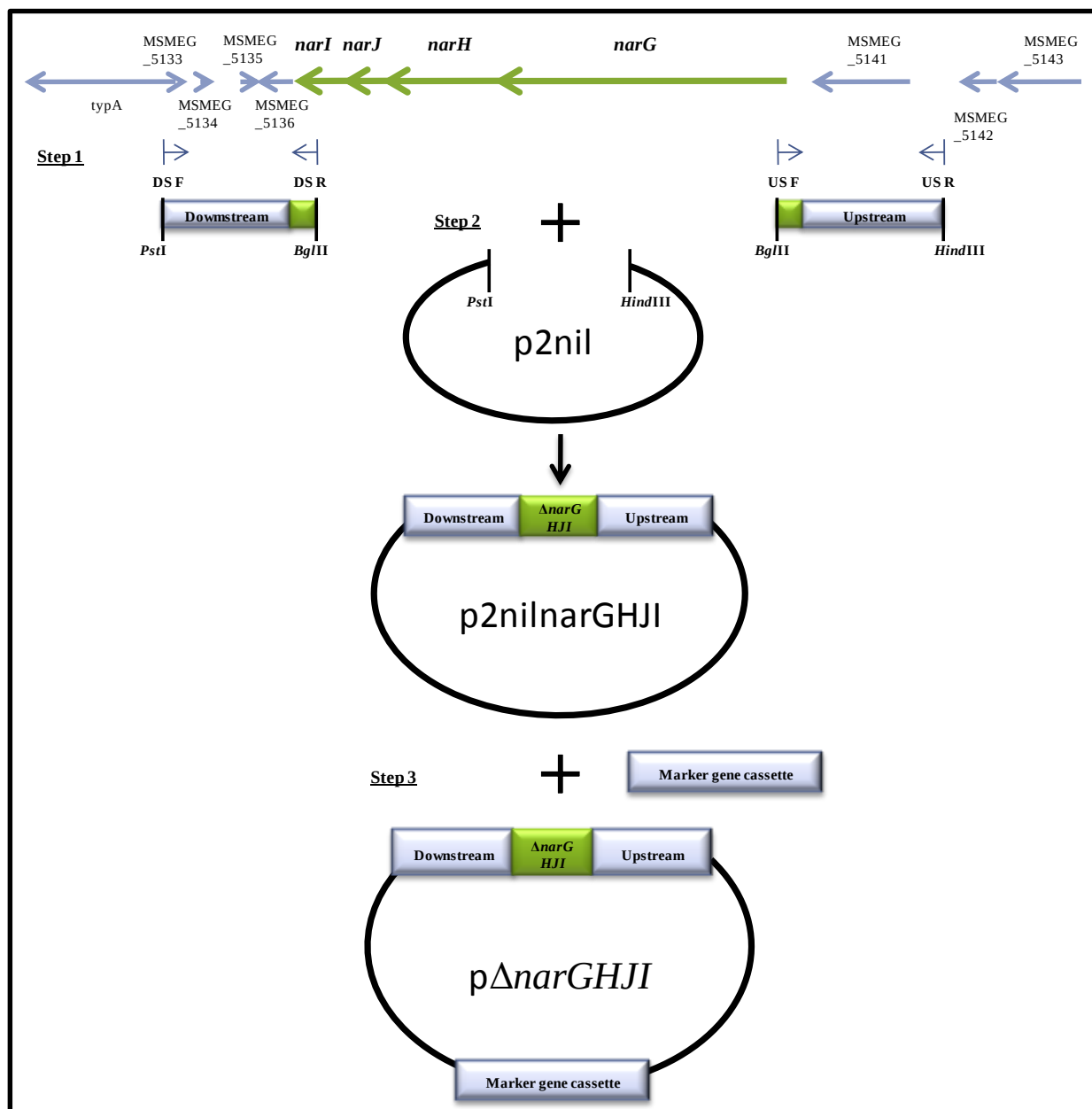
Figure 2.5: Schematic representation of the generation the suicide vector p\Delta narGHJI . Step 1: Amplification of upstream and downstream regions by PCR with a high fidelity Taq polymerase. Step 2: Restriction digestion and ligation of the upstream and downstream regions to p2NIL to generate the intermediate vector p2nilnarGHJI . Step 3: Ligation of p2nilnarGHJI with the selectable-counter-selectable marker cassette to generate the suicide vector p\Delta narGHJI .
