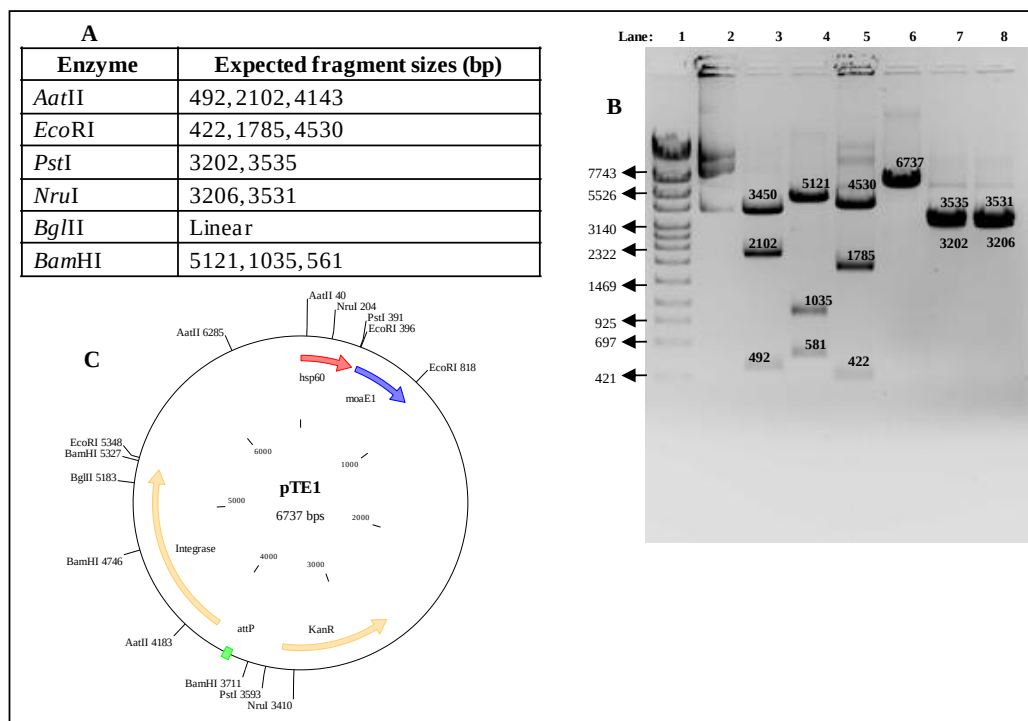
Figure E 3: Restriction analysis of integrating vector, pTE1 carrying Mtb moaE1 driven off the constitutive hsp60 promoter. (A) Expected fragment sizes for restriction digest. (B) Restriction digests of pTE1 with several enzymes. Lane 1: Marker \lambda IV, Lane 2: Uncut pTE1, Lane 3: AatII digest, Lane 4: BamHI digest, Lane 5: EcoRI digest, Lane 6: BglII digest, Lane 7: PstI digest, Lane 8: NruI digest. (C) pTE1 vector map showing cloned moaE1 in blue and the hsp60 promoter in red. The integrase and kan R genes are shown in yellow and the attP site in green.
