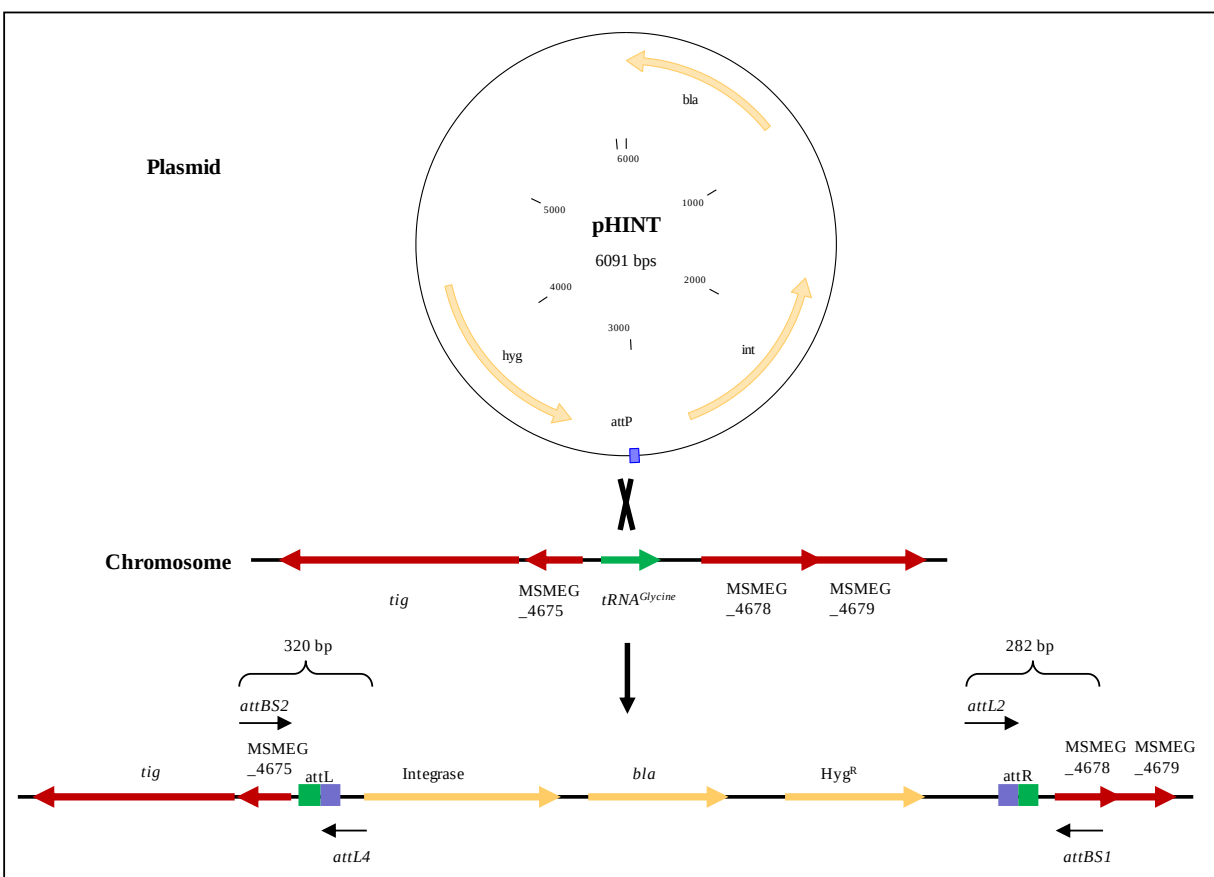
Figure 3.2: Schematic representation of integration of pHINT into the chromosome of M. smegmatis . pHINT has an L5 based integration system and the attachment site on the plasmid (blue attP block) integrates at the tRNA Gly site on the M. smegmatis chromosome (green arrow). Integration of the plasmid results in the reconstitution of the tRNA Gly site on either side of the integrated plasmid, attL and attR . The primers used to confirm the site specific integration of pHINT and expected amplicons are shown. attBS2 and attL4 produce a 320 bp amplicon confirming integration on the left. attL2 and attBS1 produce a 282 bp amplicon confirming integration on the right.
