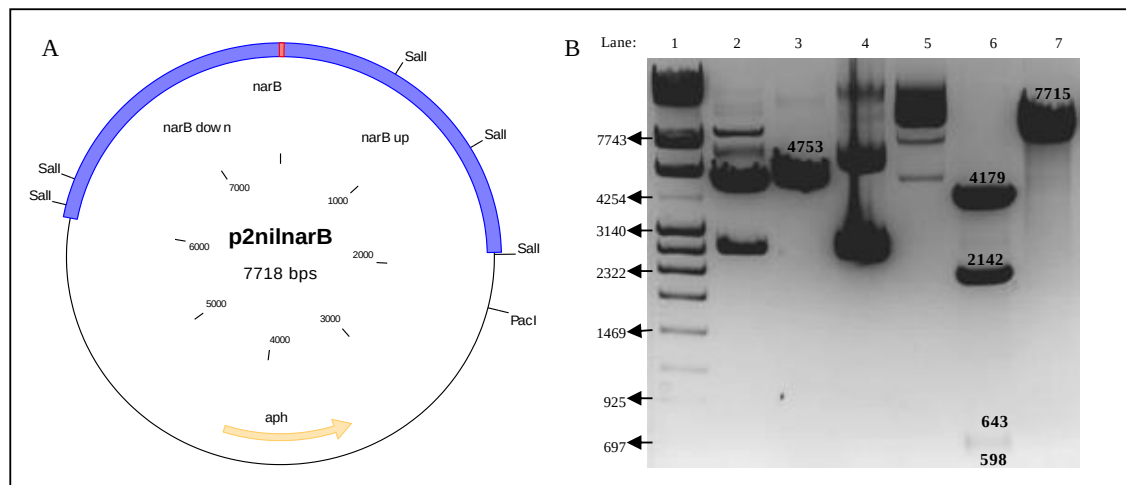
Figure E 20: Confirmation of p2nilnarB clone by restriction digestion. (A) p2nilnarB vector map showing restriction site positions. The upstream and downstream regions are shown in blue, deleted narB region in red and kanamycin resistance gene in yellow. (B) Restriction digests of p2nil and p2nilnarB. Lane 1: Marker λIV, Lane 2: p2nil uncut, Lane 3: p2nil PacI digest, Lane 4: p2nil SalI digest, Lane 5: p2nilnarB uncut, Lane 6: p2nilnarB SalI digest, Lane 7: p2nilnarB PacI digest.
