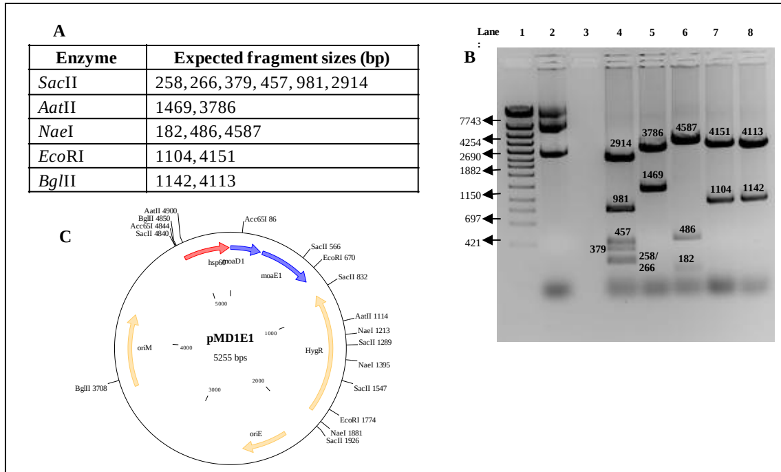
Figure E 6: Restriction analysis of episomal vector carrying Mtb moaD1 and moaE1 genes driven off the constitutive hsp60 promoter as an operon. (A) Expected fragment sizes for restriction digests (B) Restriction digests of pMD1E1 with several enzymes Lane 1: Marker \lambda IV, Lane 2: Uncut pMD1E1, Lane 3: Empty, Lane 4: SacII digest, Lane 5: AatII digest Lane 6: NaeI digest, Lane 7: EcoRI digest, Lane 8: BglII digest. (C) pMD1E1 vector map showing cloned moaD1 and moaE1 in blue and the hsp60 promoter in red. The hyg R gene, mycobacterial origin of replication ( oriM ) and E. coli origin of replication ( oriE ) are shown in yellow.
