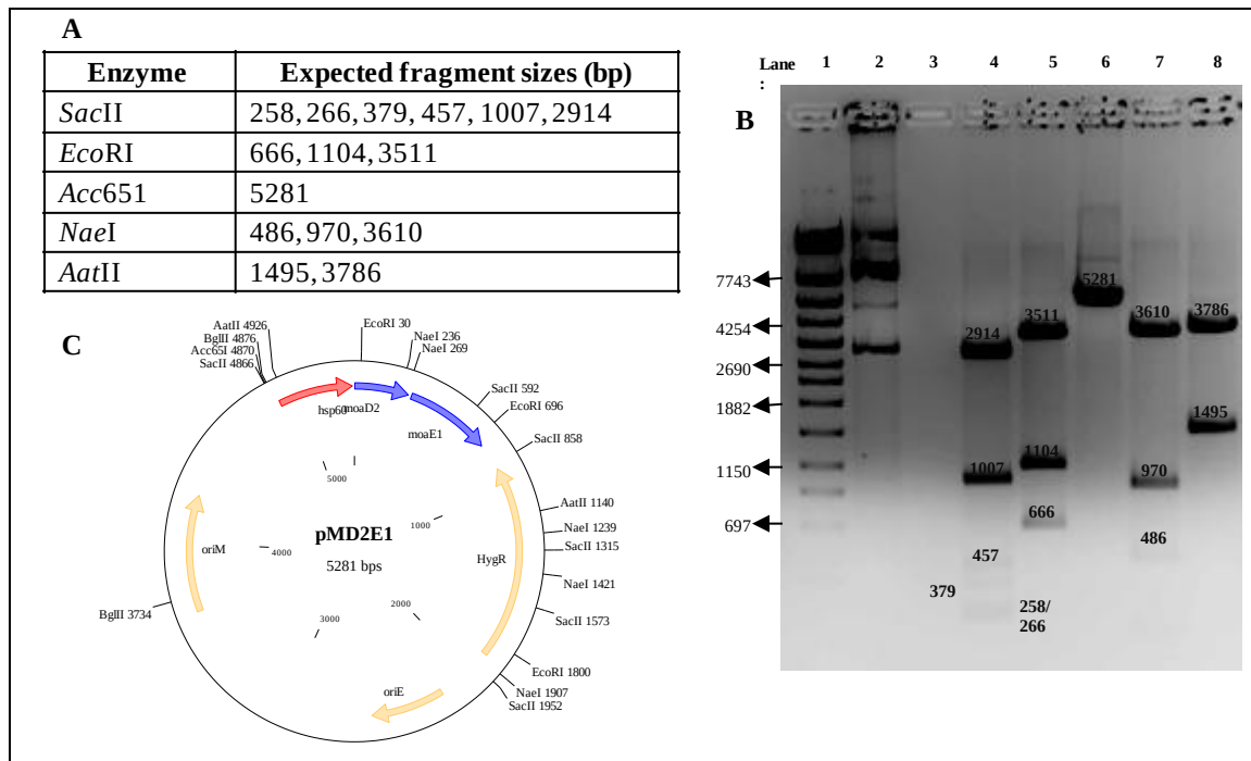
Figure E 9: Restriction analysis of episomal vector carrying Mtb moaD2 and moaE1 genes driven off the constitutive hsp60 promoter as an operon. (A) Expected fragment sizes for restriction digests (B) Restriction digests of pMD2E1 with several enzymes Lane 1: Marker \lambda IV, Lane 2: Uncut pMD2E1, Lane 3: Empty, Lane 4: Sac II digest, Lane 5: Eco RI digest Lane 6: Acc 651 digest, Lane 7: Nae I digest, Lane 8: Aat II digest. (C) pMD2E1 vector map showing cloned moaD2 and moaE1 in blue and the hsp60 promoter in red. The hyg R gene, mycobacterial origin of replication ( ori M) and E. coli origin of replication ( ori E) are shown in yellow.
