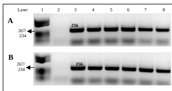
Figure E 12: Generation of megaprimers carrying point mutations to be incorporated into moaX . (A) Megaprimer carrying mutation 242G→C. (B) Megaprimer carrying mutation 245G→C. Lane 1: Marker \lambda V, Lane 2: No DNA control, Lane 3: to Lane 8: Megaprimer amplicons
