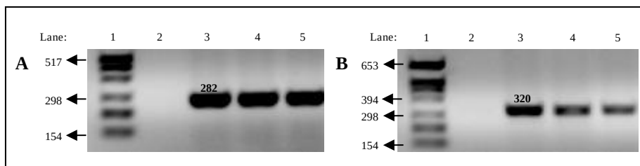
Figure 3.15: PCR confirmation of the site-specific integration of pMC1s (A) PCR amplicons from reaction using the primers attL2 and attBS1 . (B) PCR amplicons from reactions using the primer set attL4 and attBS2 . Both gels were loaded in the same order Lane 1: Marker \lambda VI, Lane 2: No DNA control, Lane 3: Positive control, Lane 4: Amplicon from transformant carrying N-terminally FLAG-tagged MoaX, Lane 5: Amplicon from transformant carrying C-terminally FLAG-tagged MoaX.
