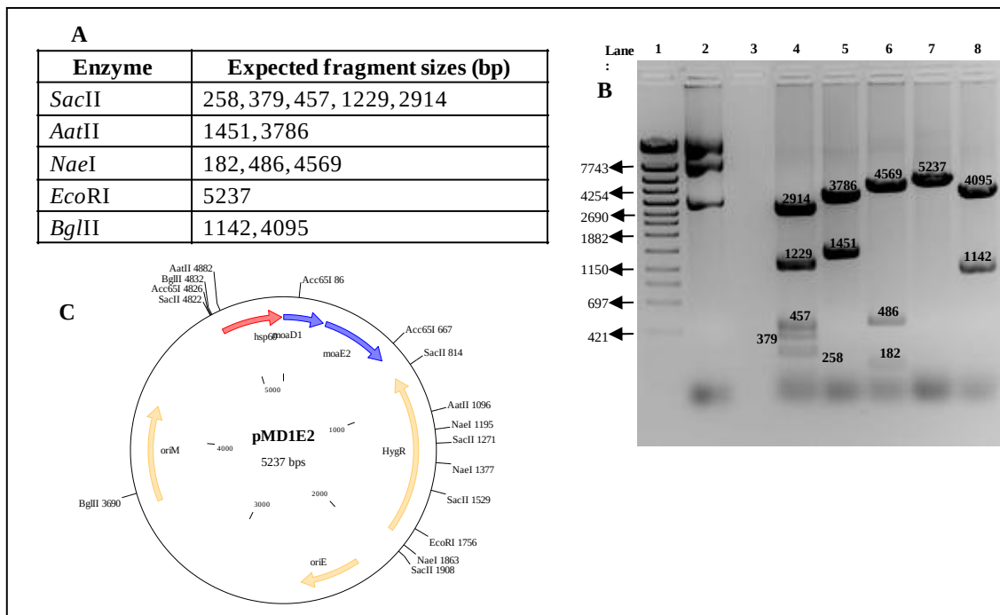
Figure E 7: Restriction analysis of episomal vector carrying Mtb moaD1 and moaE2 genes driven off the constitutive hsp60 promoter as an operon. (A) Expected fragment sizes for restriction digests (B) Restriction digests of pMD1E2 with several enzymes Lane 1: Marker \lambda IV, Lane 2: Uncut pMD1E2, Lane 3: Empty, Lane 4: SacII digest, Lane 5: AatII digest Lane 6: NaeI digest, Lane 7: EcoRI digest, Lane 8: BglII digest. (C) pMD1E2 vector map showing cloned moaD1 and moaE2 in blue and the hsp60 promoter in red. The hyg R gene, mycobacterial origin of replication ( oriM ) and E. coli origin of replication ( oriE ) are shown in yellow.
