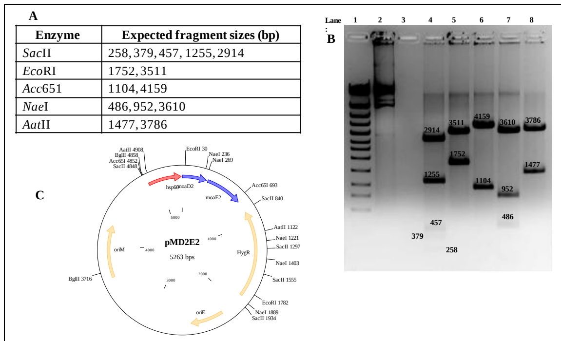
Figure E 8: Restriction analysis of episomal vector carrying Mtb moaD2 and moaE2 genes driven off the constitutive hsp60 promoter as an operon. (A) Expected fragment sizes for restriction digests (B) Restriction digests of pMD2E2 with several enzymes Lane 1: Marker \lambda IV, Lane 2: Uncut pMD2E2, Lane 3: Empty, Lane 4: Sac II digest, Lane 5: Eco RI digest Lane 6: Acc 651 digest, Lane 7: Nae I digest, Lane 8: Aat II digest. (C) pMD2E2 vector map showing cloned moaD2 and moaE2 in blue and the hsp60 promoter in red. The hyg R gene, mycobacterial origin of replication ( ori M) and E. coli origin of replication ( ori E) are shown in yellow.
