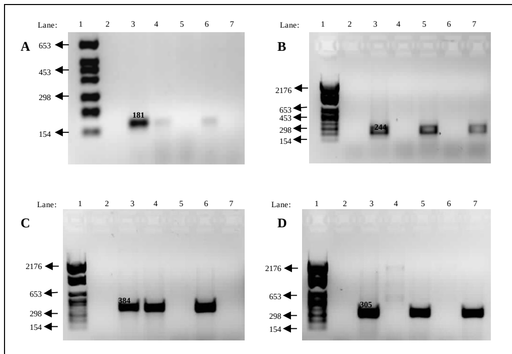
Figure 3.6: PCR confirmation of M. smegmatis single mutant strains complemented with Mtb genes on integrating or episomal vectors (A) Amplification with primers TBD1F+TBD1R. (B) Amplification with primers moaD2F+moaD2R. The gels in A and B were loaded in the same order- Lane 1: Marker \lambda VI, Lane 2: No DNA control, Lane 3: Positive control, Lane 4: \Delta moaD2 (pMD1), Lane 5: \Delta moaD2 (pMD2), Lane 6: \Delta moaD2::pHD1 , Lane 7: \Delta moaD2::pHD2 (C) Amplification with primers TBE1F+TBE1R (D) Amplification with primers TBE2F+TBE2R. The gels in C and D were loaded in the same order- Lane 1: Marker \lambda VI, Lane 2: No DNA control, Lane 3: Positive control, Lane 4: \Delta moaE2 (pME1), Lane 5: \Delta moaE2 (pME2), Lane 6: \Delta moaE2::pTE1 , Lane 7: \Delta moaE2::pTE2
