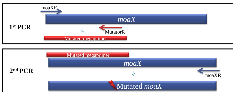
Figure 2.2: Diagram depicting the Megaprimer method of generating site-directed mutations in moaX . The first PCR reaction generates a mutated megaprimer using the wild type forward primer and a reverse primer carrying the point mutation. This megaprimer is then used in a second PCR reaction as a forward primer along with the wild type reverse primer generating the full length gene carrying the mutation.
