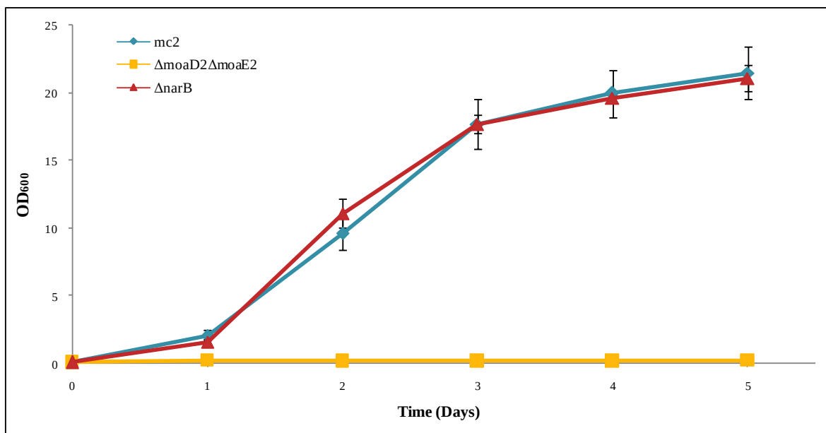
Figure 3.24: Growth curve analysis of \Delta narB in nitrate minimal media shows that it is dispensable for growth. Averages of at least three independent experiments were plotted for each strain with standard errors included.
