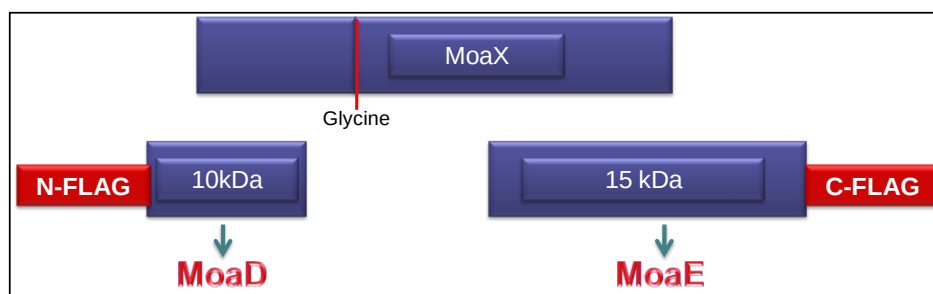
Figure 3.14: Schematic representation of the cleavage of MoaX showing the predicted site of cleavage and the expected sizes of each subunit once MoaX is processed at this site.
