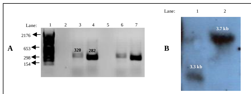
Figure 3.7: Confirmation of site specific integration of pHINT carrying Mtb moaD1 or moaD2 and pTT1b carrying moaE1 or moaE2 into the chromosome of the M. smegmatis single mutants. (A) PCR confirmation of pHINT integration. Lane 1: Marker \lambda VI, Lane 2: No DNA control, Lane 3: Amplification of \Delta moaD2::pHD1 with primers attBS2 and attL4, Lane 4: Amplification of \Delta moaD2::pHD1 with primers attL2 and attBS1, Lane 5: Empty, Lane 6: Amplification of \Delta moaD2::pHD2 with primers attBS2 and attL4, Lane 7: Amplification of \Delta moaD2::pHD2 with primers attL2 and attBS1. (B) Southern blot confirmation of pTT1b integration using the right probe. Lane 1: Sac II digested genomic DNA from \Delta moaE2::pTE1 , Lane 2: Sac II digested genomic DNA from \Delta moaE2::pTE2
