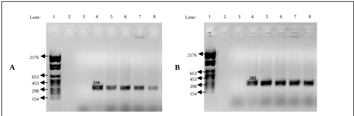
Figure 3.3: PCR confirmation of site-specific integration of pHINT carrying Mtb moaD1 and moaD2 into the M. smegmatis chromosome at the attB site, tRNA Glycine . (A) Amplicons for primer set attBS2+attL4 (B) Amplicons for primer set attL2+attBS1. Lane 1: Marker \lambda VI, Lane 2: Empty, Lane 3: No DNA control, Lane 4: Positive control, Lane 5: DE::IntD1E1, Lane 6: DE::IntD1E2, Lane 7: DE::IntD2E1, Lane 8: DE::IntD2E2
