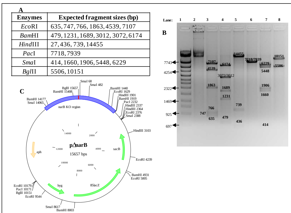
Figure E 21: Restriction digest confirmation of p \Delta narB. (A) Expected fragment sizes for restriction digest. (B) Restriction digests of p \Delta narB with several enzymes. Lane 1: Marker \lambda IV, Lane 2: Uncut p \Delta narB, Lane 3: EcoRI digest, Lane 4: BamHI digest, Lane 5: HindIII digest, Lane 6: PacI digest, Lane 7: SmaI digest, Lane 8: BglII digest (C) p \Delta narB vector map showing upstream and downstream regions in blue and the deleted narB allele in red. The selectable marker genes are shown in green and kan R gene is shown in yellow.
