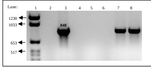
Figure 3.9: PCR confirmation of \Delta moaD2 \Delta moaE2:: pTX Lane 1: Marker \lambda VI, Lane 2: Empty, Lane 3: Positive control, Lane 4: Empty, Lane 5: No DNA control, Lane 6: Empty, Lane 7: Amplification of DE::pTX, Lane 8: Amplification of DE (pMX)
