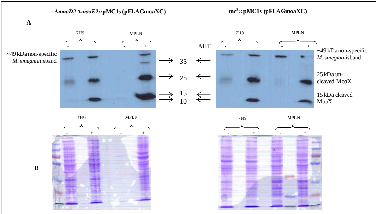
Figure 3.19: MoaX is cleavage is not altered by media composition. (A) Western blot of protein samples extracted from \Delta moaD2 \Delta moaE2::pMC1s (pFLAGmoaXC) and mc^2::pMC1s (pFLAGmoaXC) grown in modified M. phlei . (B) Gel images of the corresponding blots above.
