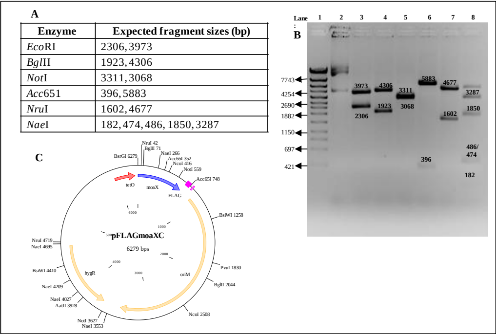
Figure E 10: Restriction analysis of pFLAG vector carrying C-terminally FLAG-tagged Mtb moaX under the control of the tet operator. (A) Expected fragment sizes for restriction digests (B) Restriction digests of pFLAGmoaXC with several enzymes Lane 1: Marker λIV, Lane 2: Uncut pMD2E2, Lane 3: EcoRI digest, Lane 4: BglII digest, Lane 5: NotI digest Lane 6: Acc651 digest, Lane 7: NruI digest, Lane 8: NaeI digest. Incomplete cleavage products are unlabeled (C) pFLAGmoaXC vector map showing cloned moaX in blue and the tet operator in red. The hyg R gene and mycobacterial origin of replication ( oriM ) are shown in yellow
