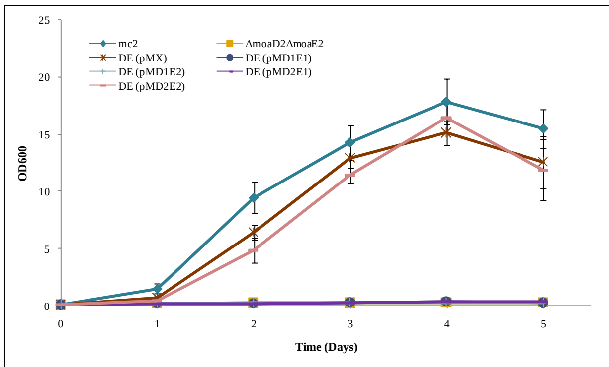
Figure 3.12: Growth curve of strains complemented with episomal vectors carrying different combinations of Mtb moaD1 , moaD2 , moaE1 and moaE2 genes. Cultures were grown in nitrate minimal media for 5 days with OD readings taken daily. The plotted data points are an average of at least three independent experiments and the standard error for each point is included.
