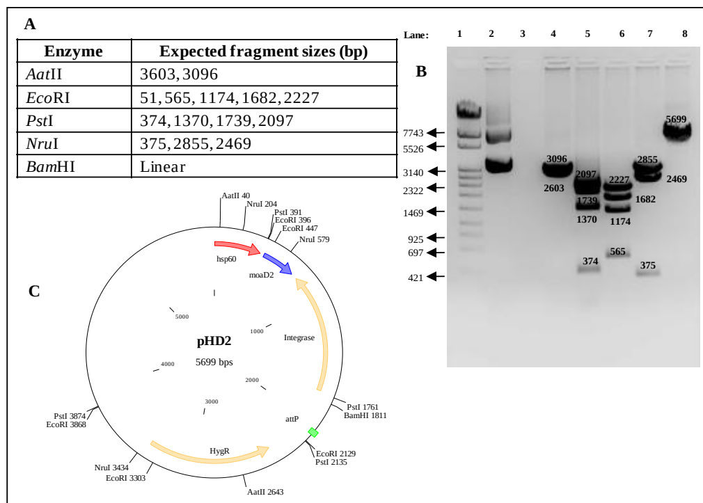
Figure E 2: Restriction analysis of integrating vector, pHD2 carrying Mtb moaD2 driven off the constitutive hsp60 promoter. (A) Expected fragment sizes for restriction digest. (B) Restriction digests of pHD2 with several enzymes. Lane 1: Marker \lambda IV, Lane 2: Uncut pHD2, Lane 3: Empty, Lane 4: AatII digest, Lane 5: EcoRI digest, Lane 6: PstI digest, Lane 7: NruI digest, Lane 8: BamHI digest. (C) pHD2 vector map showing cloned moaD2 in blue and the hsp60 promoter in red. The integrase and hyg R genes are shown in yellow and the attP site in green.
