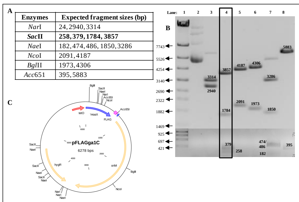
Figure E 17: Restriction mapping of pFLAGga1C carrying a C-terminally FLAG-tagged derivative of moaX with point mutation 242G>C. (A) Expected fragment sizes for restriction digests. (B) Restriction digests of pFLAGga1C with several enzymes Lane 1: Marker \lambda IV, Lane 2: uncut vector, Lane 3: NarI digest, Lane 4: SacII digest, Lane 5: NcoI digest, Lane 6: BglII digest, Lane 7: NaeI digest, Lane 8: Acc651 digest. Incomplete cleavage products are unlabeled (C) pFLAGga1C vector map showing cloned moaX in blue, the tet operator in red and the FLAG tag in pink. The hyg R gene and mycobacterial origin of replication ( oriM ) are shown in yellow.
