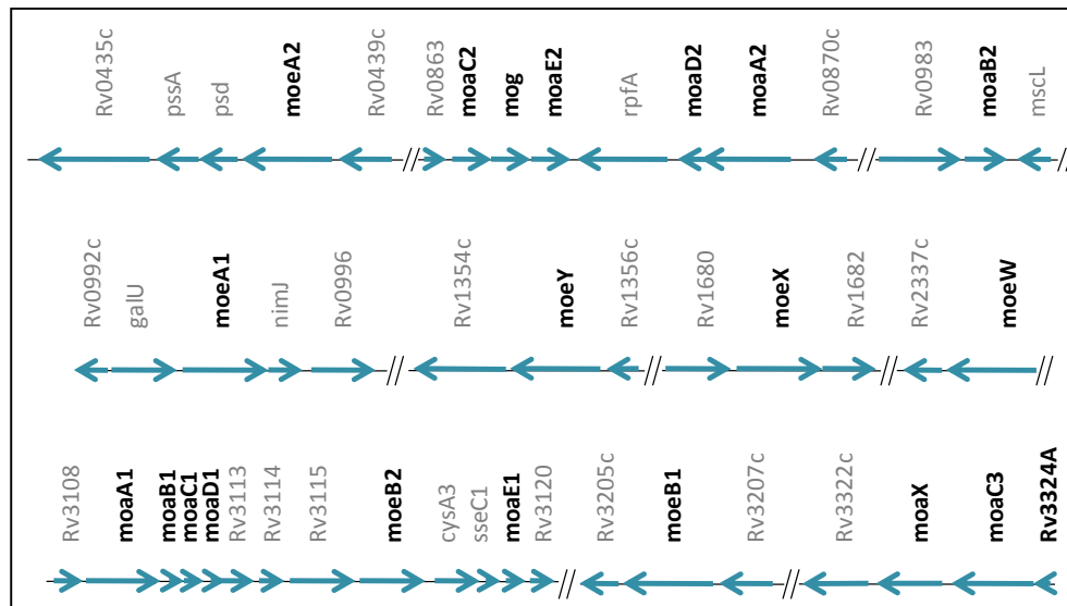
Figure 1.4: Chromosomal distribution of Mtb genes involved in MoCo biosynthesis. Genes shown in bold are predicted by homology to be involved in MoCo biosynthesis.
