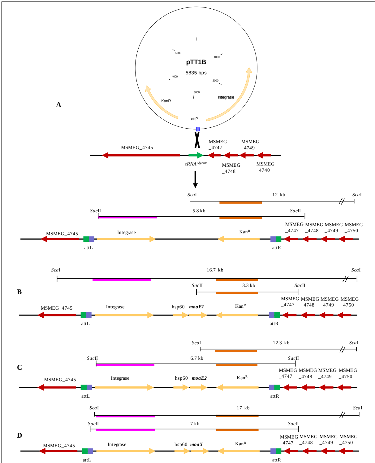
Figure 3.4: Schematic representation of the integration of pTT1b into the chromosome of M. smegmatis . The restriction enzymes used for southern blot confirmation are shown as well as the fragment sizes expected with each probe and construct. (A) Genomic map of the integration of pTT1b into the M. smegmatis chromosome and the expected fragment sizes for southern blot analysis. (B) Genomic map of the integration of pTE1 into the M. smegmatis chromosome and the expected fragment sizes for southern blot analysis. (C) Genomic map of the integration of pTE2 into the chromosome of M. smegmatis and the expected fragment sizes for Southern blot analysis. (D) Genomic map of the integration of pTX into the M. smegmatis chromosome and the expected fragment sizes for southern blot analysis. The right probe used for Southern blotting is shown in orange and the left probe in pink.
