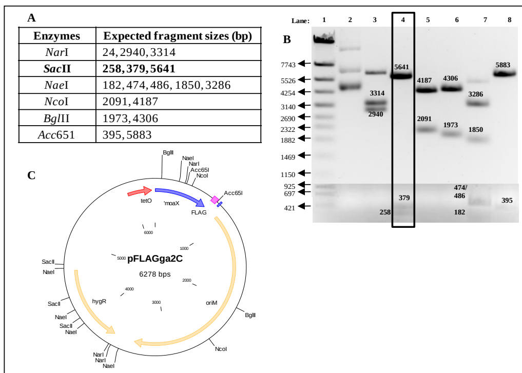
Figure E 18: Restriction mapping of pFLAGga2C carrying a C-terminally FLAG-tagged derivative of moaX with point mutation 245G>C. (A) Expected fragment sizes for restriction digests. (B) Restriction digests of pFLAGga2C with several enzymes Lane 1: Marker \lambda IV, Lane 2: uncut vector, Lane 3: NarI digest, Lane 4: SacII digest, Lane 5: NcoI digest, Lane 6: BglII digest, Lane 7: NaeI digest, Lane 8: Acc651 digest. Incomplete cleavage products are unlabeled (C) pFLAGga2C vector map showing cloned moaX in blue, the tet operator in red and the FLAG tag in pink. The hyg R gene and mycobacterial origin of replication ( oriM ) are shown in yellow.
