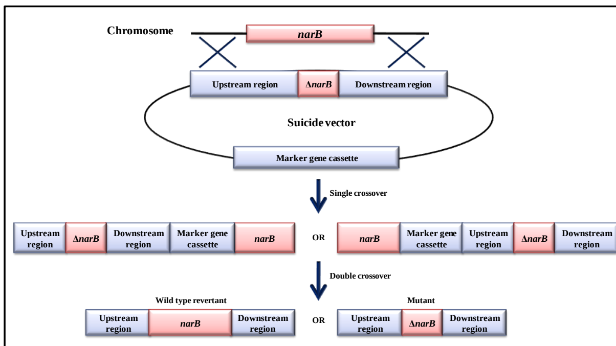
Figure 2.3: Schematic depiction of two-step allelic exchange mutagenesis using narB as the example gene.
