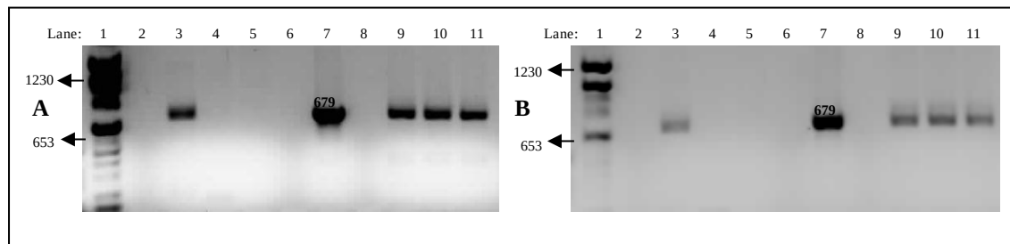
Figure E 13: Generation of full length moaX with point mutations (A) 242G→C and (B) 245G→C incorporated. Lane 1: Marker \lambda VI, Lane 2: Empty, Lane 3: No DNA control, Lane 4: Forward primer only, Lane 5: Reverse primer only, Lane 6: Empty, Lane 7: Positive control, Lane 8: Empty, Lane 9 to Lane 11: Full length moaX amplicons with point mutations incorporated.
