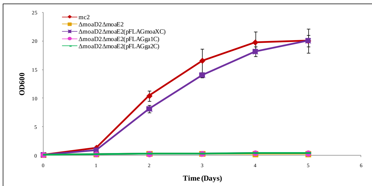
Figure 3.20: Growth curve analysis of strains carrying FLAG-tagged derivatives of moaX with either a 242G>C or 245G>C mutation. C-terminally FLAG-tagged MoaX and mc 2 were included as positive controls for growth. Growth curves were performed in MPLN with optical density readings taken daily for five days.
