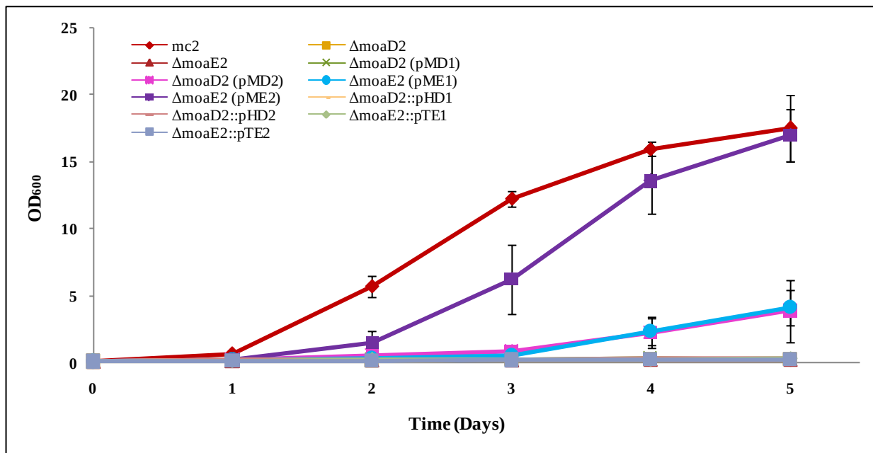
Figure 3.8: Growth curve of M. smegmatis single mutants, \Delta moaD2 and \Delta moaE2 complemented with either Mtb moaD1 , moaD2 , moaE1 or moaE2 carried on integrating and episomal vectors. Growth curves were carried out in MPLN media with optical density readings taken daily for 5 days. The plotted data points are an average of at least three independent experiments and the standard error for each point is included.
