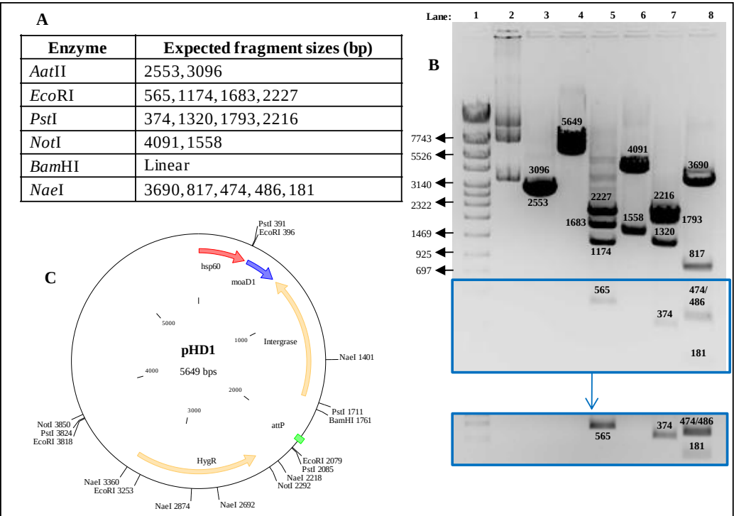
Figure E 1: Restriction analysis of integrating vector, pHD1 carrying Mtb moaD1 driven off the constitutive hsp60 promoter. (A) Expected fragment sizes for restriction digest. (B) Restriction digests of pHD1 with several enzymes. Lane 1: Marker \lambda IV, Lane 2: Uncut pHD1, Lane 3: AatII digest, Lane 4: BamHI digest, Lane 5: EcoRI digest, Lane 6: NotI digest, Lane 7: PstI digest, Lane 8: NaeI digest (C) pHD1 vector map showing cloned moaD1 in blue and the hsp60 promoter in red. The integrase and hyg R genes are shown in yellow and the attP site in green.
