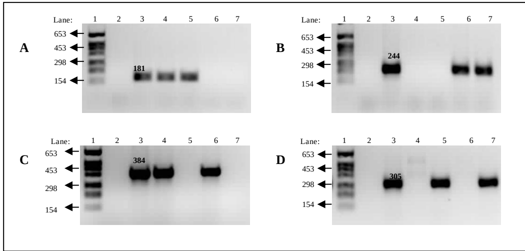
Figure 3.1: PCR confirmation of M. smegmatis double mutant strains complemented with different combinations of Mtb moaD1 , moaD2 , moaE1 and moaE2 genes carried on integrating vectors. (A) Amplification with primers TBD1F+TBD1R (B) Amplification with primers moaD2F+moaD2R (C) Amplification with primers TBE1F+TBE1R (D) Amplification with primers TBE2F+TBE2R. Lane 1: Marker \lambda VI, Lane 2: No DNA control, Lane 3: Positive control, Lane 4: DE::IntD1E1, Lane 5: DE::IntD1E2, Lane 6: DE::IntD2E1, Lane 7: DE::IntD2E2
