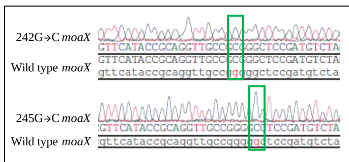
Figure E 19: Image of chromatogram showing the incorporation of the point mutations 242G→C and 245G→C into moaX . The wild type base pair is shown in red and the wild type together with the corresponding mutated base pair are boxed in green.
