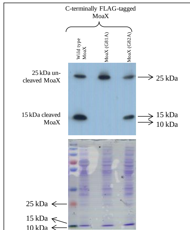
Figure 3.21: Western blot analysis of protein extracts from strains carrying mutated copies of moaX . Wild type MoaX serves as a positive control for cleavage. Mutation G81A of C-terminally FLAG-tagged MoaX abolished cleavage, whereas mutation G82A did not interfere with processing.
