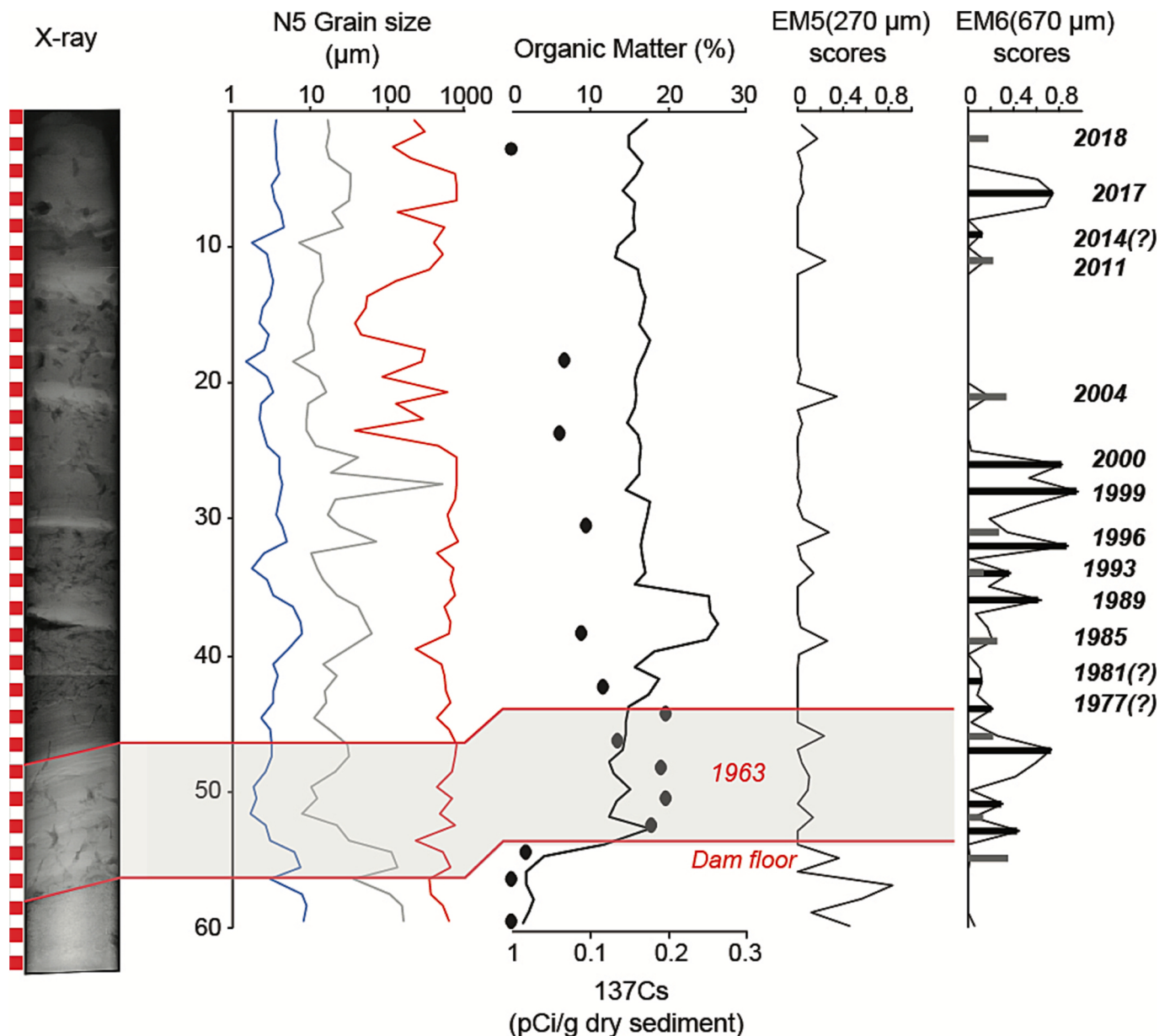
Fig. 2. Sediments core from the Nwanedi Dam (from left to right): x-ray image of the core N5; grain size distribution Dx10 (blue), Dx50 (grey) Dx90 (red); Organic matter content and ^{137}\text{Cs} activity (solid black circles); End Member scores for EM5 (270 \mu\text{m} ) and EM6 (670 \mu\text{m} ). EM5 is in grey in the last column on the right while EM6 values are in black.
