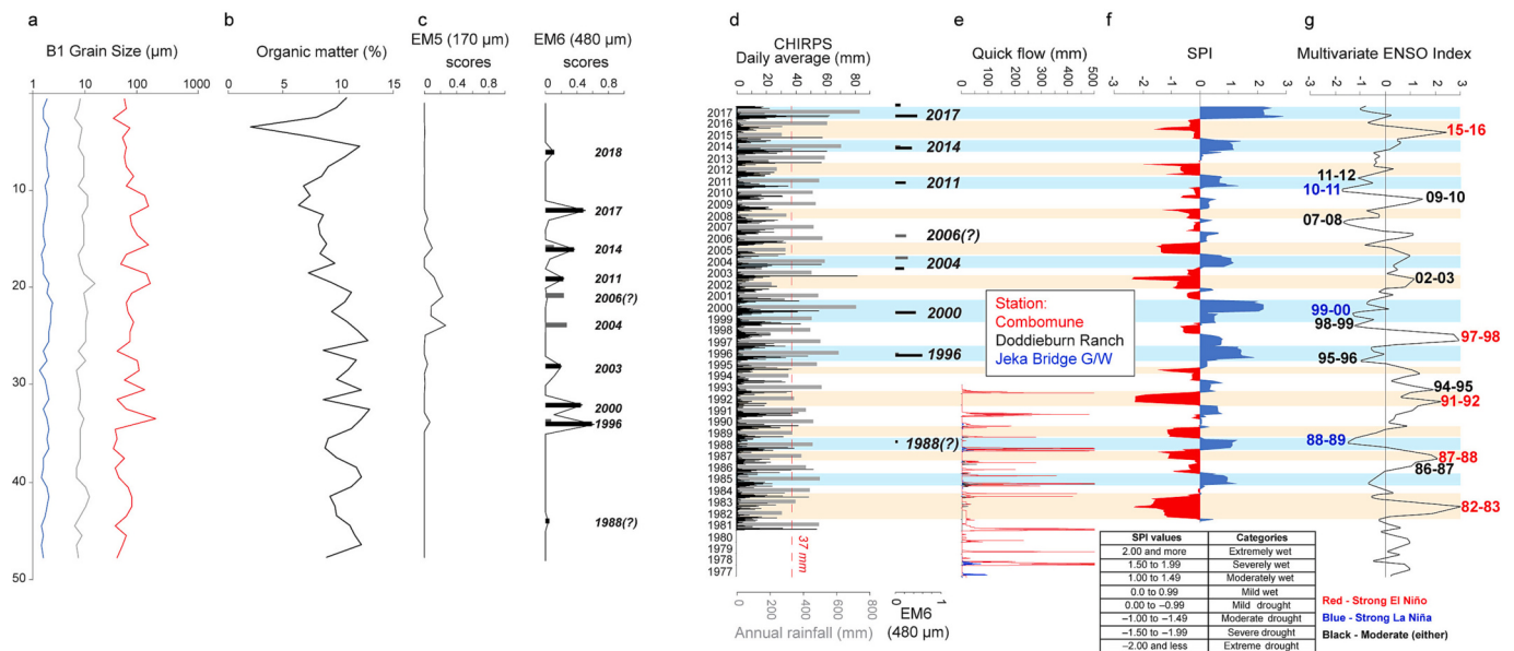
Fig. 4. Sedimentological and hydrological data from Ripple Creek Dam catchment a) grain size distribution D x10 (blue), D x50 (grey) D x90 (red) of sediments core B1 from the Ripple Creek Dam; b) Organic matter content of core B1; c) End Member scores for EM5 (170 \mu\text{m} ) and EM6 (480 \mu\text{m} ); d) CHIRPS rainfall data across the Ripple Creek Dam catchment and EMMAgeo results for EM6 (in black); e) quick flow measurements for 3 GRDC stations (see Fig. 1 for locations): Jeka Bridge G/W (1496360) = Mwenezi River; Doddieburn Ranch (1496321) = Mzingwane River; Combomune (1896502) = Limpopo River; f) Standardized Precipitation Index (SPI) at the timescales of 12 months for Massingir Dam, red areas represent droughts, and blue areas represents wetter periods; g) multivariate ENSO indexes from Baddoo et al. (2015).
