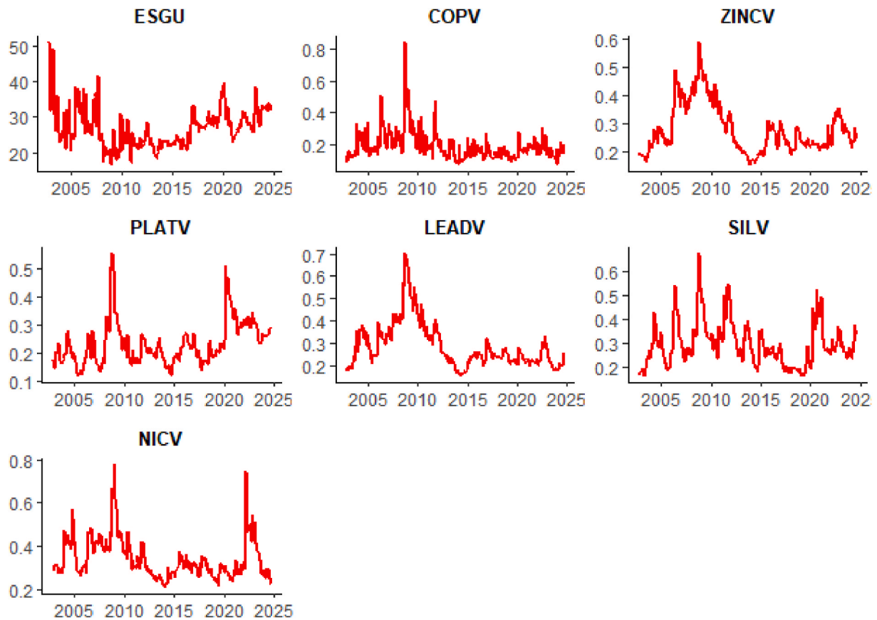
Fig. 1. Monthly ESGU index and critical minerals volatility from November 2002 to September 2024.
