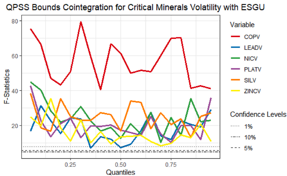
Fig. 4. QPSS bounds test.
