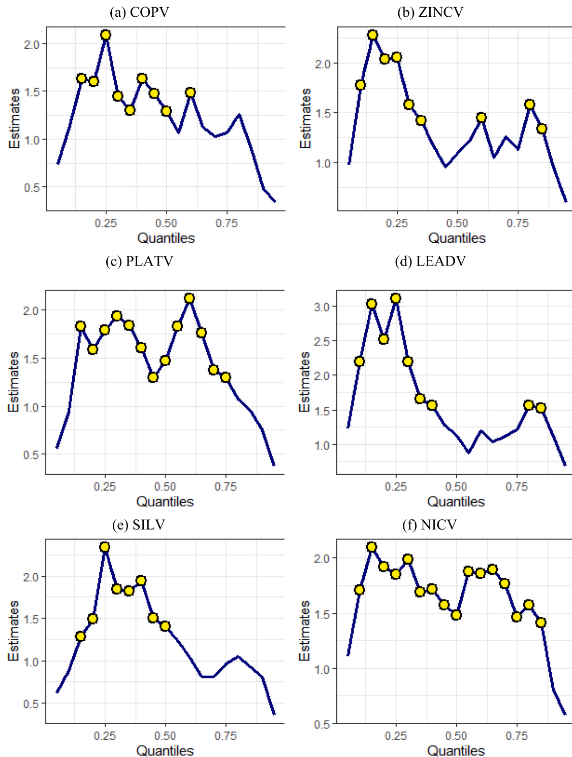
Fig. 5. QC results. Note: ● denotes (Pr) \leq 0.1 .
