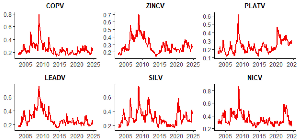
Fig. A1. Monthly critical minerals GAS-GARCH Student T volatility from November 2002 to September 2024
