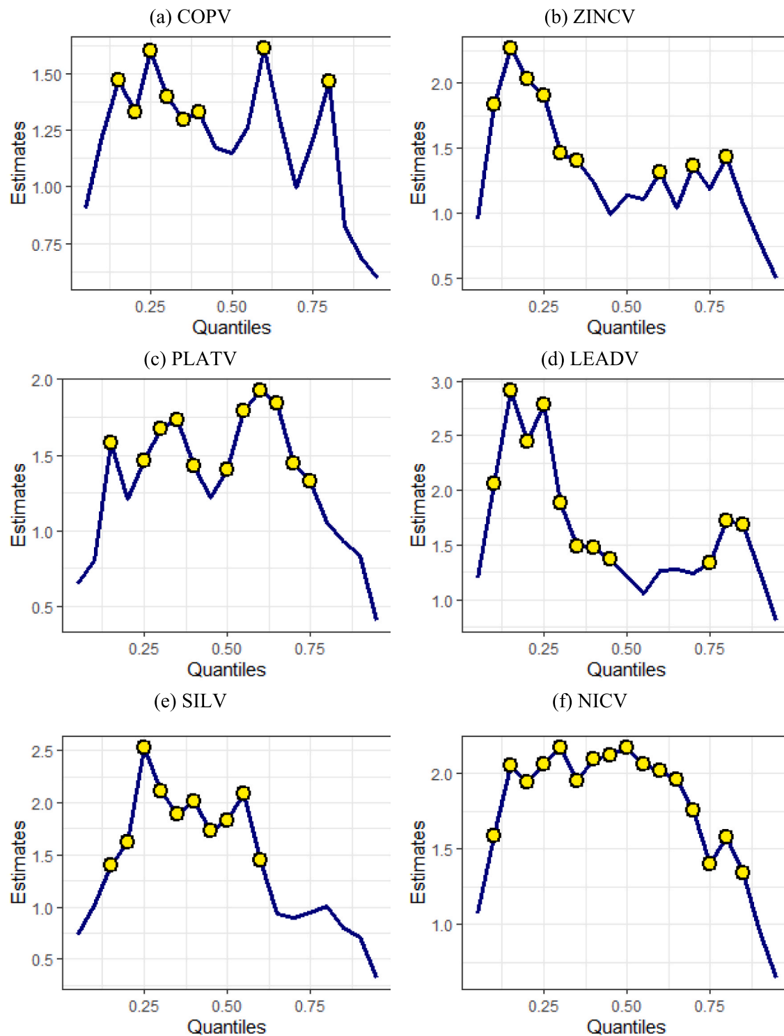
Fig. 8. QC results. Note: ● denotes (Pr) \leq 0.1 .
