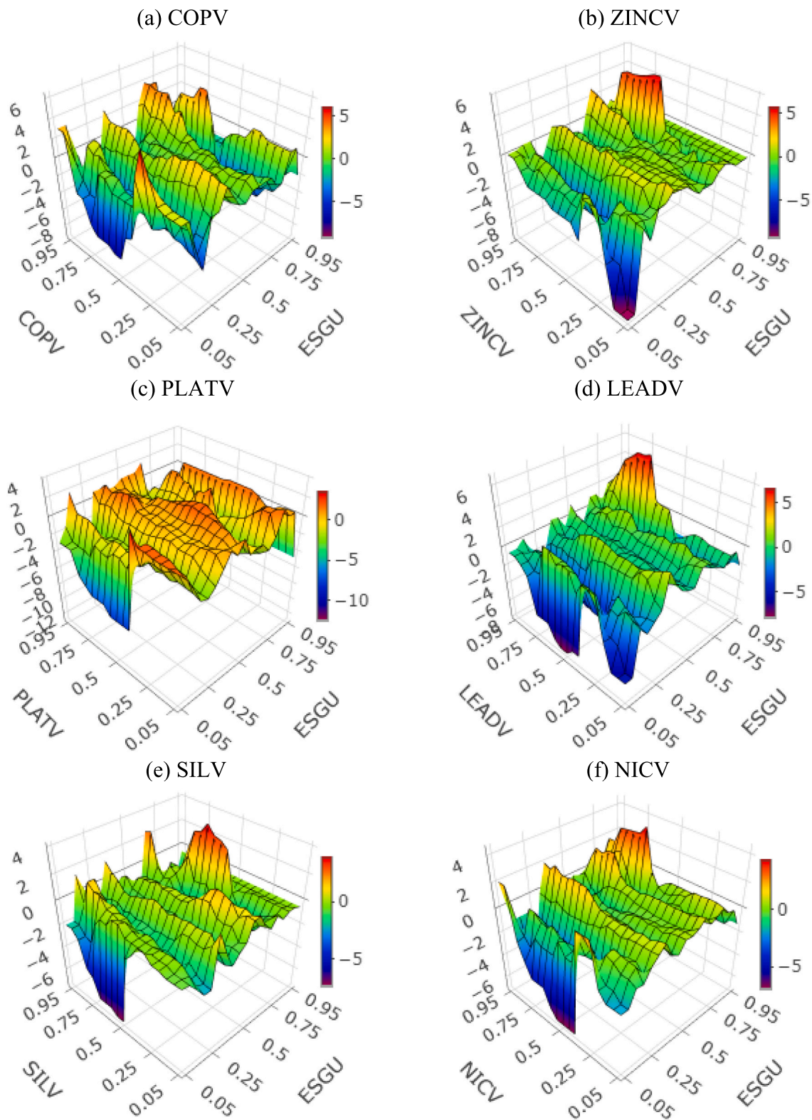
Fig. 6. QQR results.
