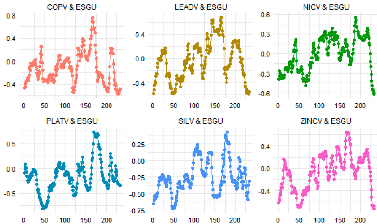
Fig. A3. Rolling window correlations between ESGU and critical minerals GAS-GARCH Student T volatility
