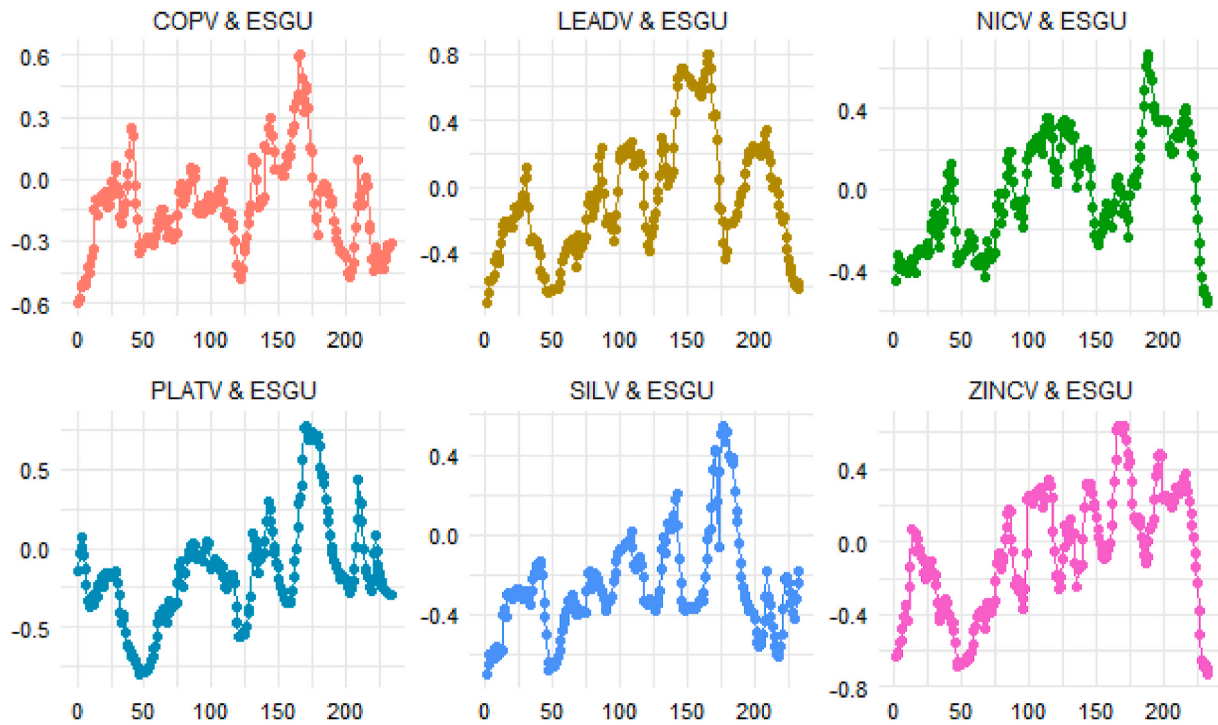
Fig. 3. Rolling window correlations between ESGU and critical minerals volatility.
