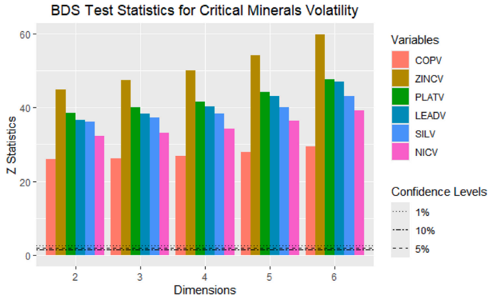
Fig. A2. BDS test for critical minerals GAS-GARCH Student T volatility
