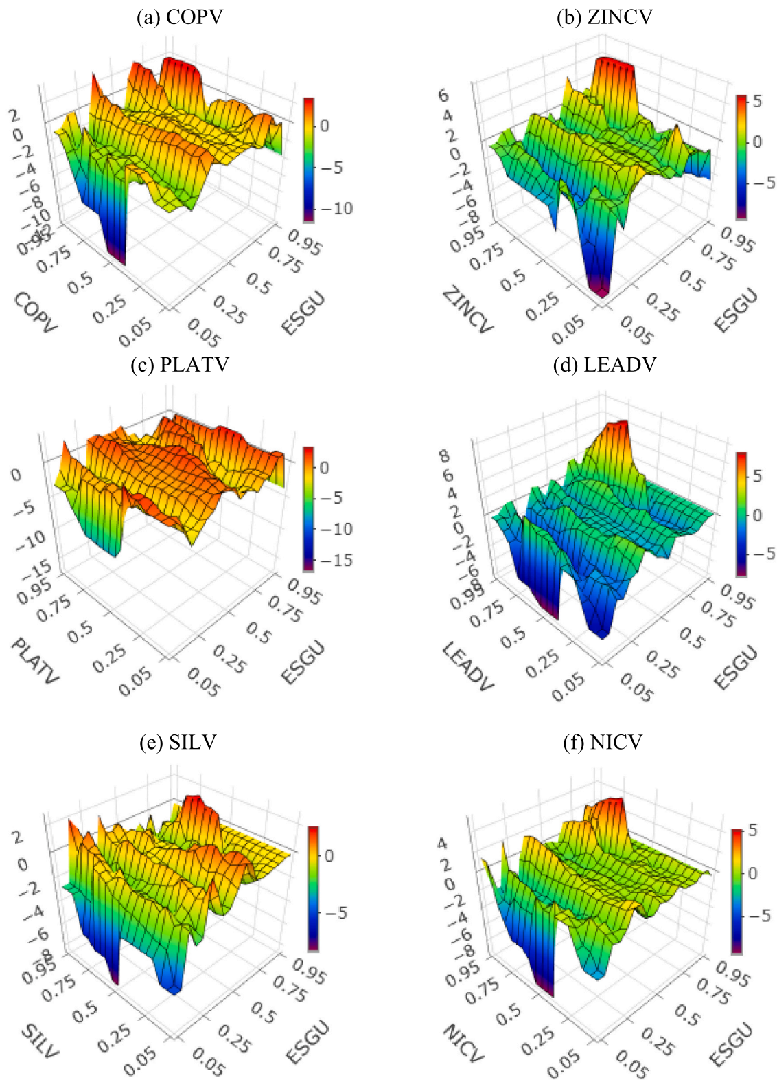
Fig. 9. QQR results.
