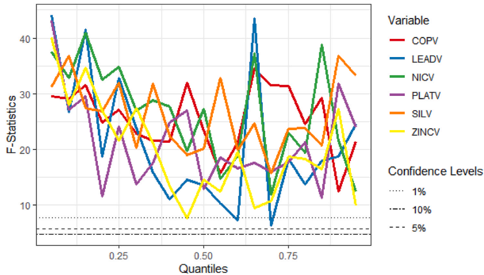
Fig. 7. QPSS bounds test.
