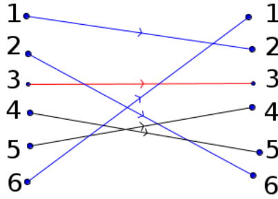
Figure 2.1: A graphical illustration of a permutation.
