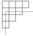
Figure 2.3: The hook length of a box in a Young diagram. For the box shown h = 5 .
