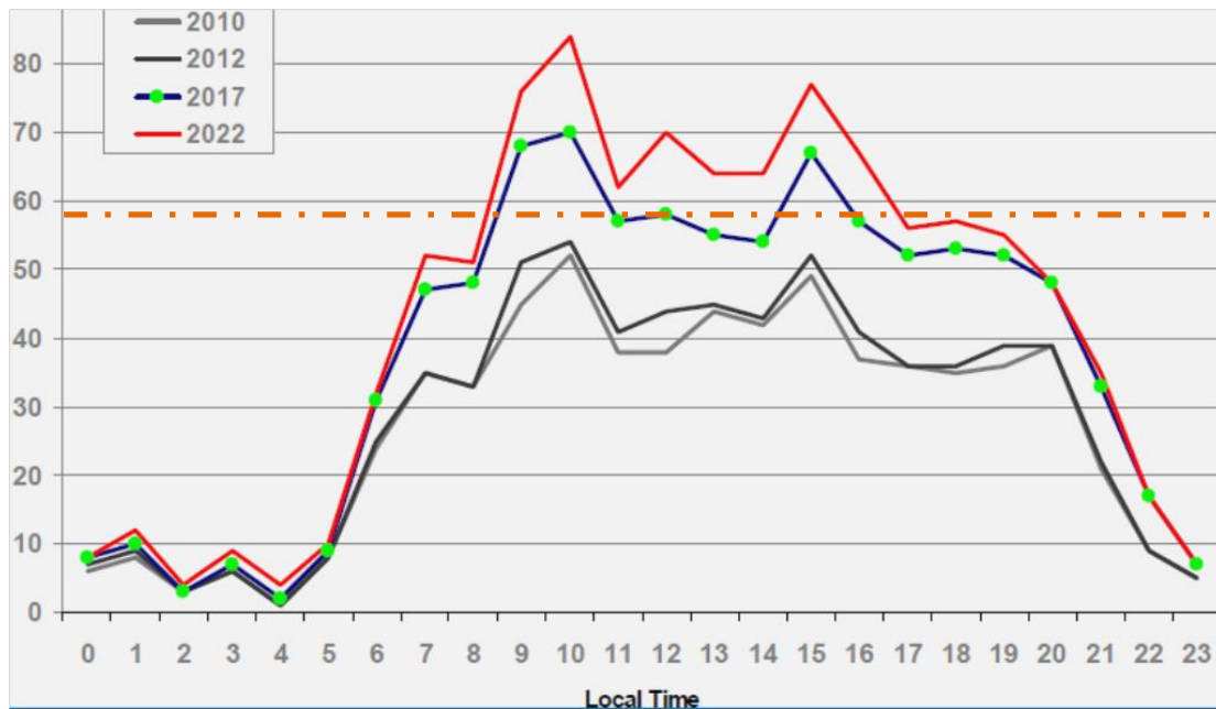
Figure 3-6: Busy day hourly distribution of aircraft movements. ACI (2011:28)
