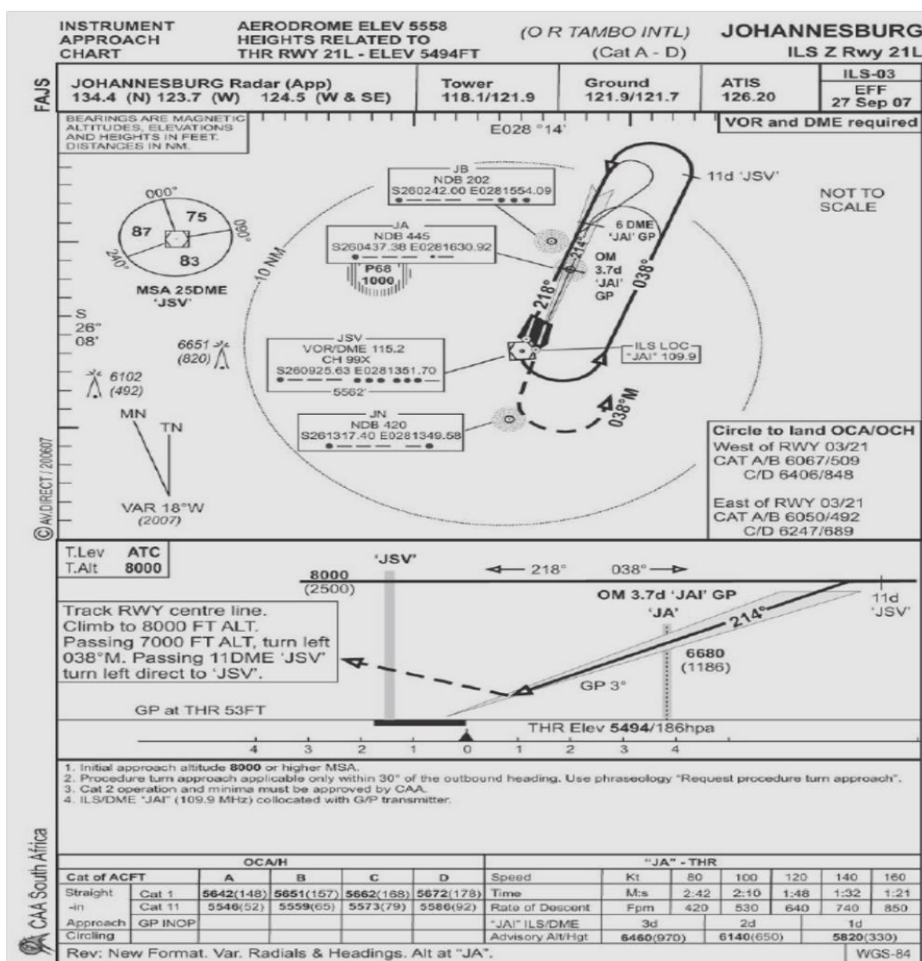
Figure 6-6: ORTIA Southbound ILS Approach. SACAA (2007)
