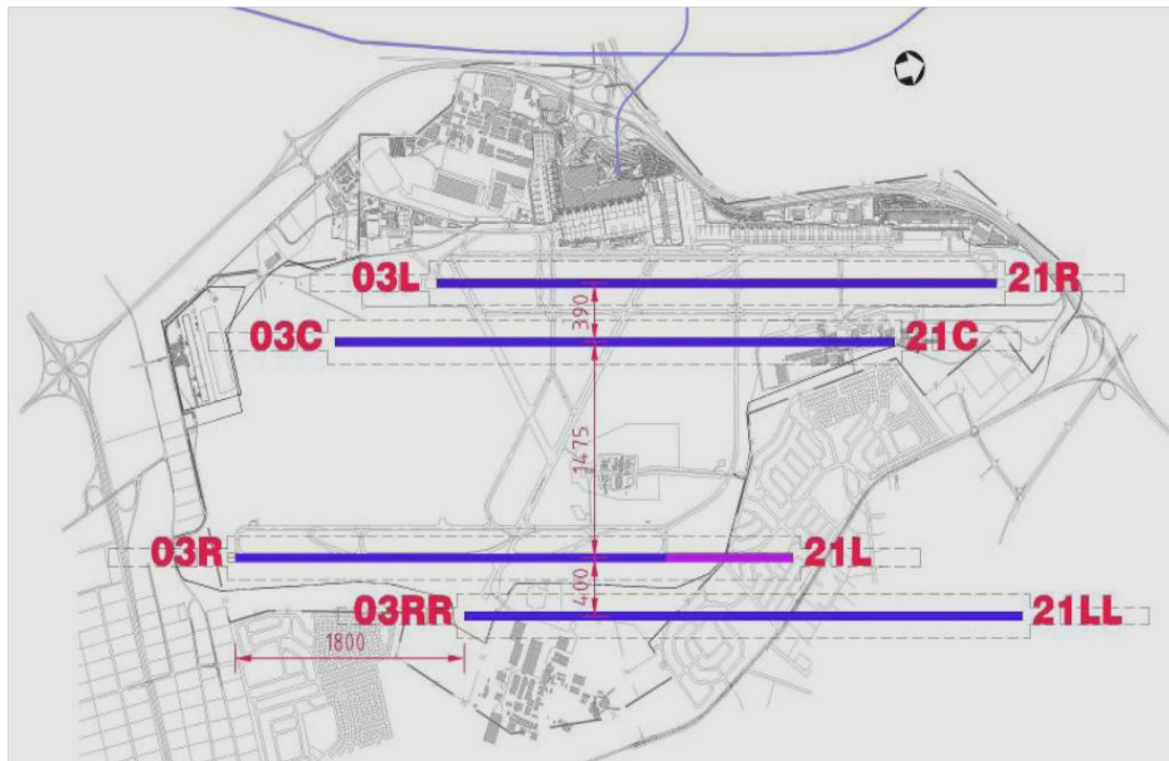
Figure 6-7: Proposed runway designations at ORTIA. ACSA (2007)
