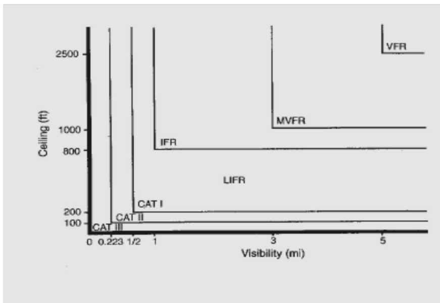
Figure 2-5: A typical classification of weather conditions at an airport in the United States. De Neufville and Odoni (2003:388)
