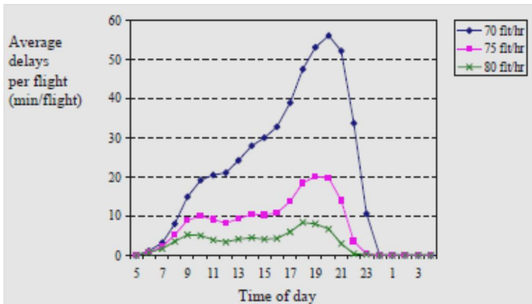
Figure 2-20: Average flight delays at LGA under different capacities. Fan and Odoni (2001:7)
