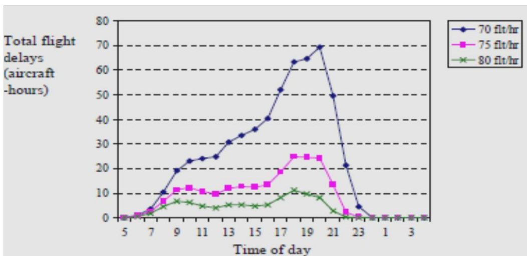
Figure 2-21: Total flight delays at LGA under different capacities. Fan and Odoni (2001:7)
