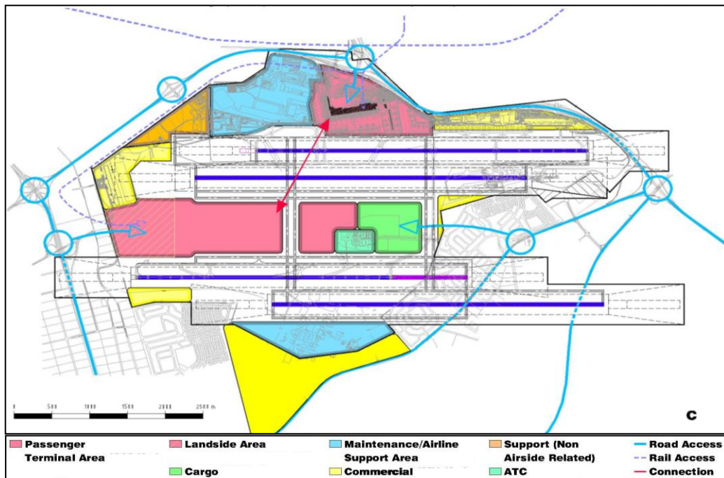
Figure 6-8: ORTIA Ultimate Master Plan layout. ACSA (2007)
