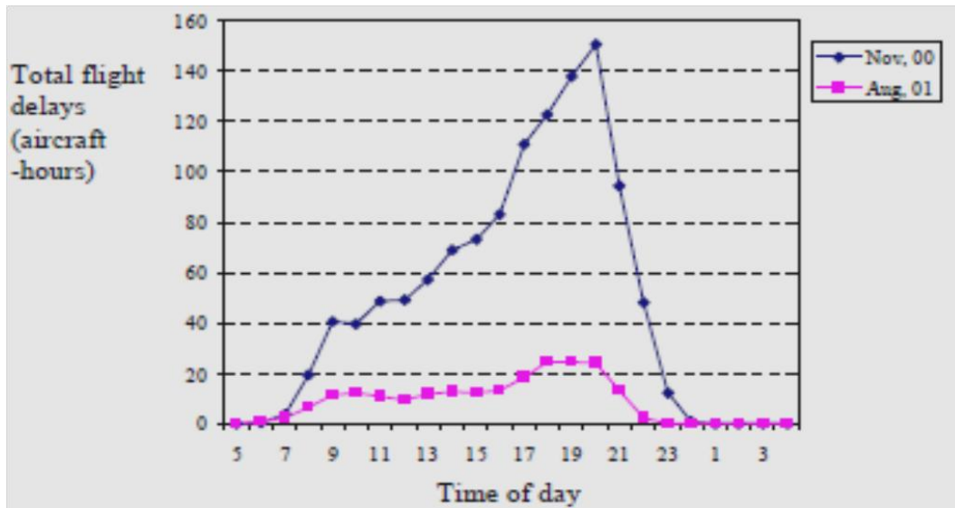
Figure 2-19: Total flight delays at LGA before and after lottery. Fan and Odoni (2001:6)
