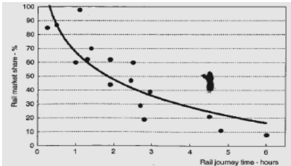
Figure 2-15: Market share of HSR competing with APT on journey time in selected European corridors-market. Air and rail competitions and complementarity (2000)
