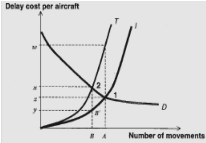
Figure 2-16: The effect of charging for external delay costs. De Neufville and Odoni (2003:479)
