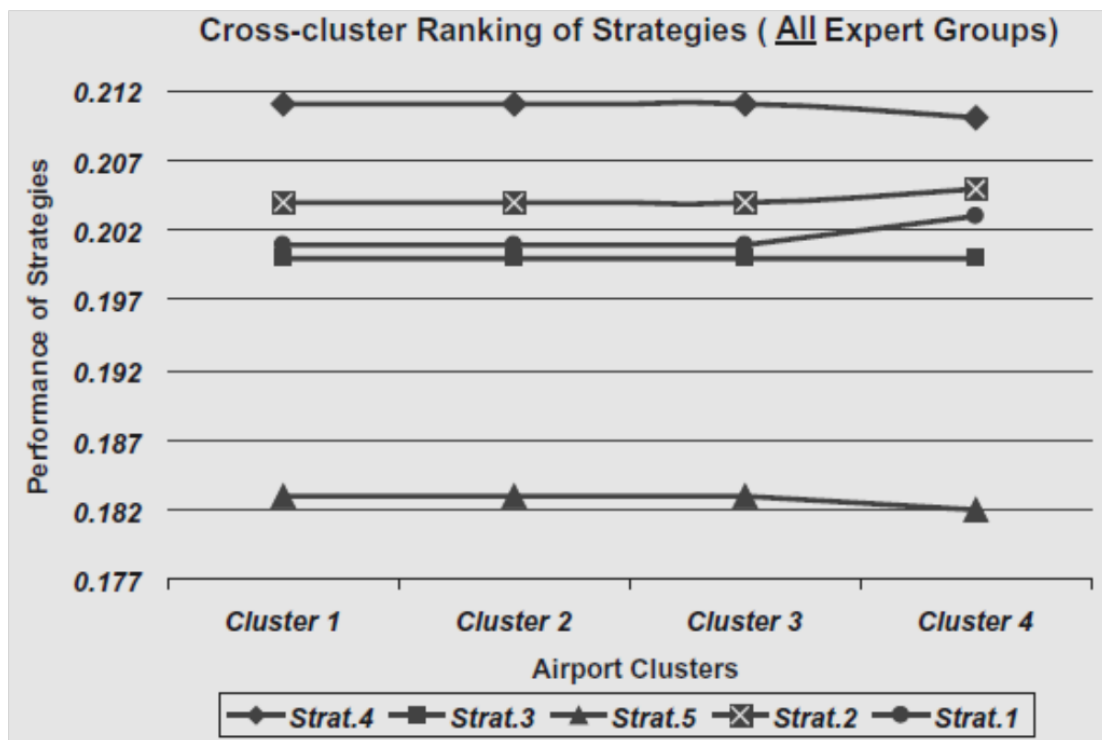
Figure 4-3: Performance and ranking of strategies per airport cluster. Madas and Zografos (2006:220)
