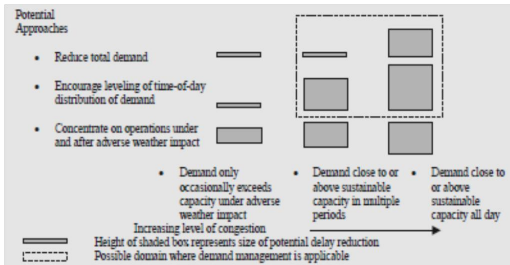
Figure 2-26: Notional illustration of delay reduction for different airports. Fan and Odoni (2001:10)
