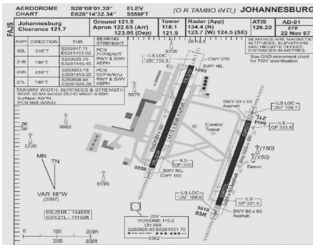
Figure 6-3: ORTIA aerodrome chart. SACAA (2007)
