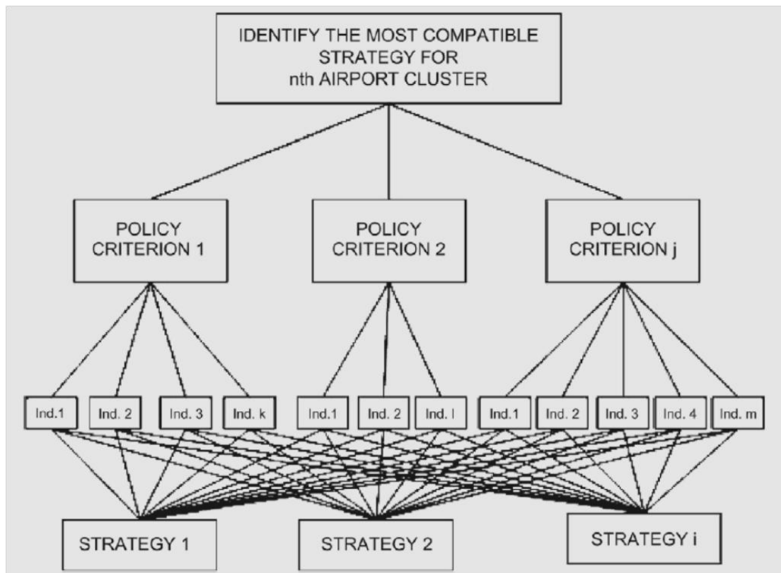
Figure 4-1: Hierarchical decomposition of the policy compatibility assessment problem. Madas and Zografos (2006:216)
