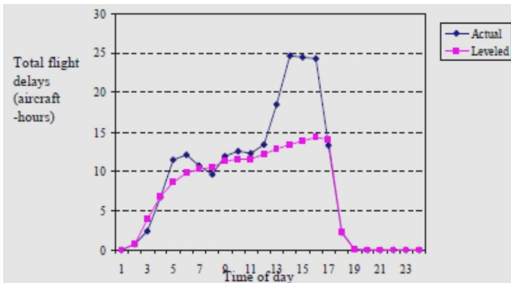
Figure 2-24: Total flight delays for leveled distribution of flight from August flight schedule. Fan and Odoni (2001:9)
