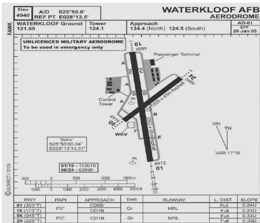
Figure 6-5: Waterkloof Aerodrome Chart. SACAA (2005)
