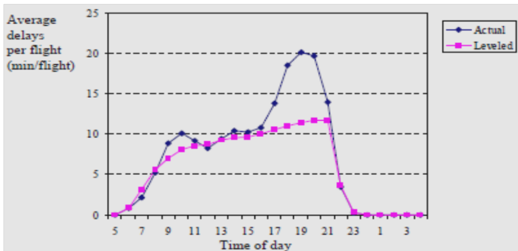
Figure 2-23: Average flight delays for leveled distribution of flight from August Schedule. Fan and Odoni (2001:9)
