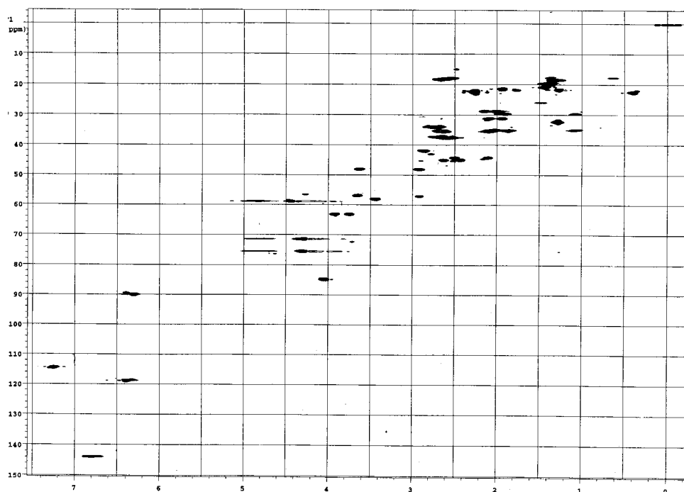
Figure A1.6 HMQC spectrum of aqua-10-nitrosocobalamin.
