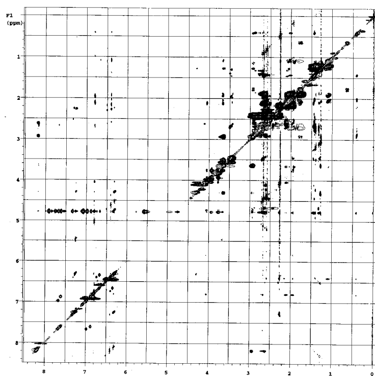
Figure A1.3 ROESY spectrum of aqua-10-nitrosocobalamin.
