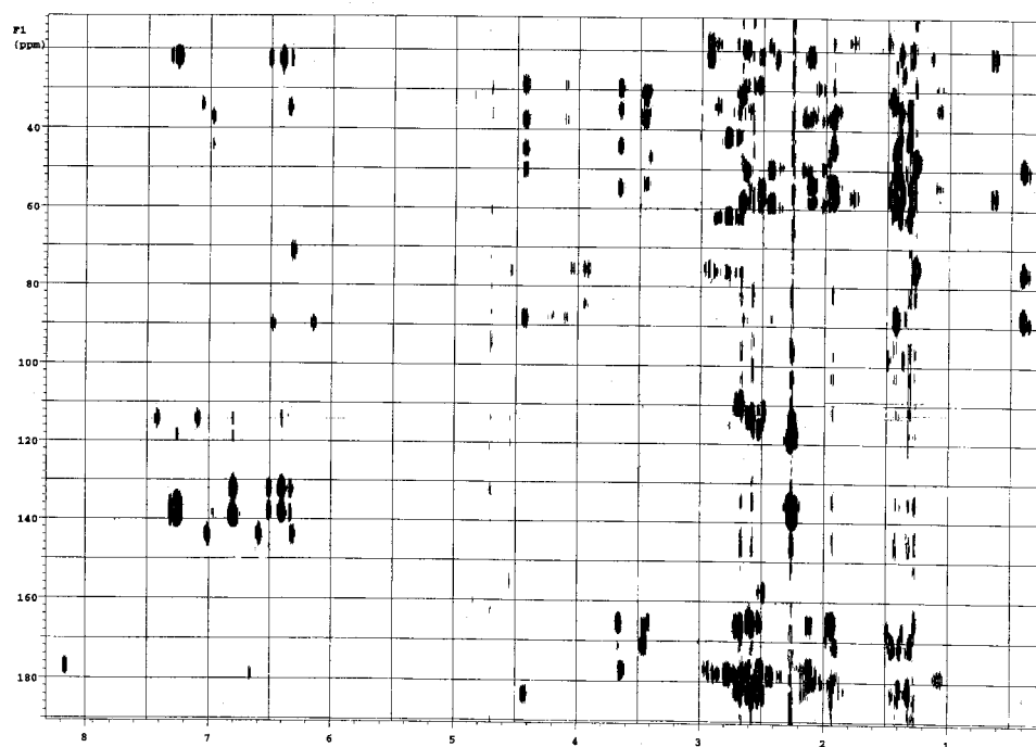
Figure A1.5 HMBC spectrum of aqua-10-nitrosocobalamin.
