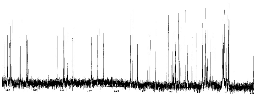
Figure A1.2 ^{13}\text{C} NMR spectrum of aqua-10-nitrosocobalamin.
