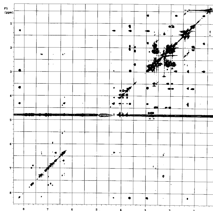
Figure A1.4 TOCSY spectrum of aqua-10-nitrosocobalamin.
