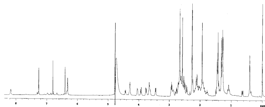
Figure A1.1 ^1\text{H} NMR spectrum of aqua-10-nitrosocobalamin.
