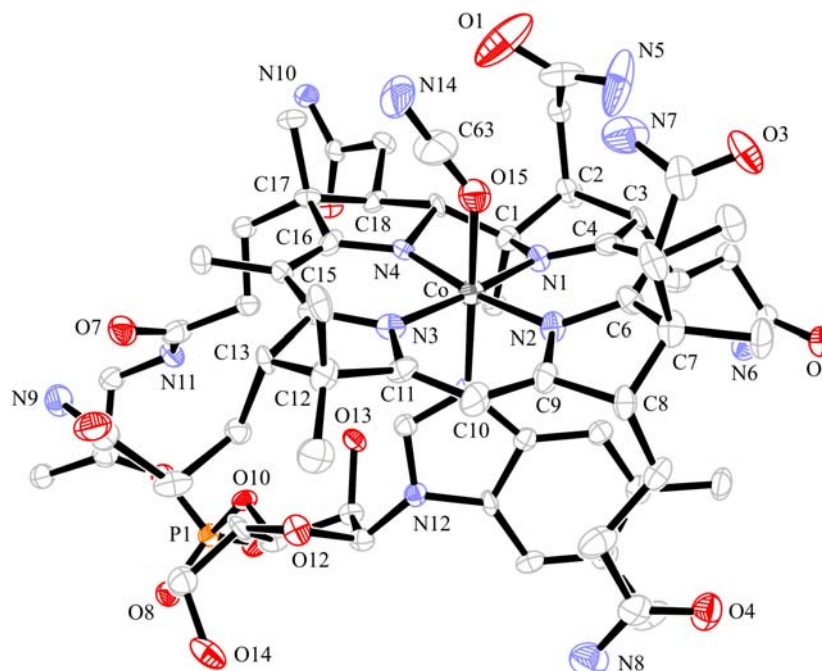
Figure A8.1 ORTEP diagram of NCOcobalamin (ellipsoids drawn at the 30% probability level). Hydrogen atoms and water molecules have been removed for clarity. The binding shown through oxygen is just a representation as the data was not good enough to determine through which atom the \text{OCN}^- binds.
