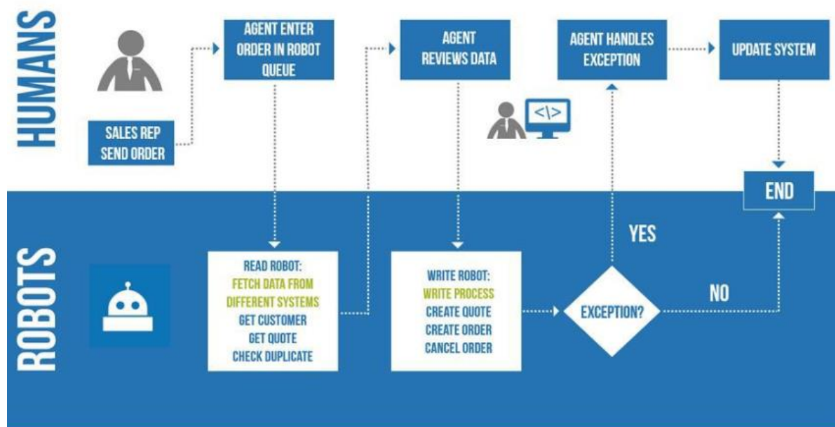
Figure 2.4: RPA in customer ordering architecture
