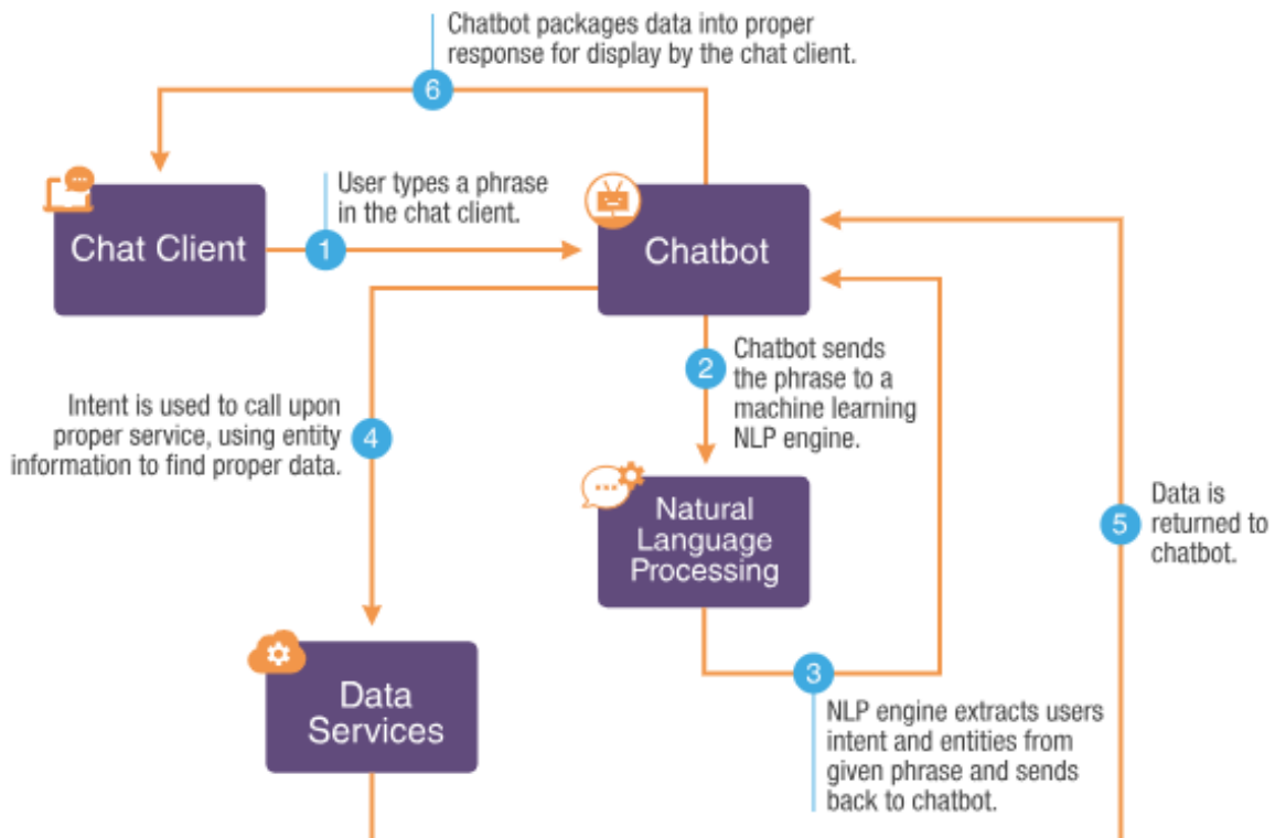
Figure 2.6: Chatbot architecture
