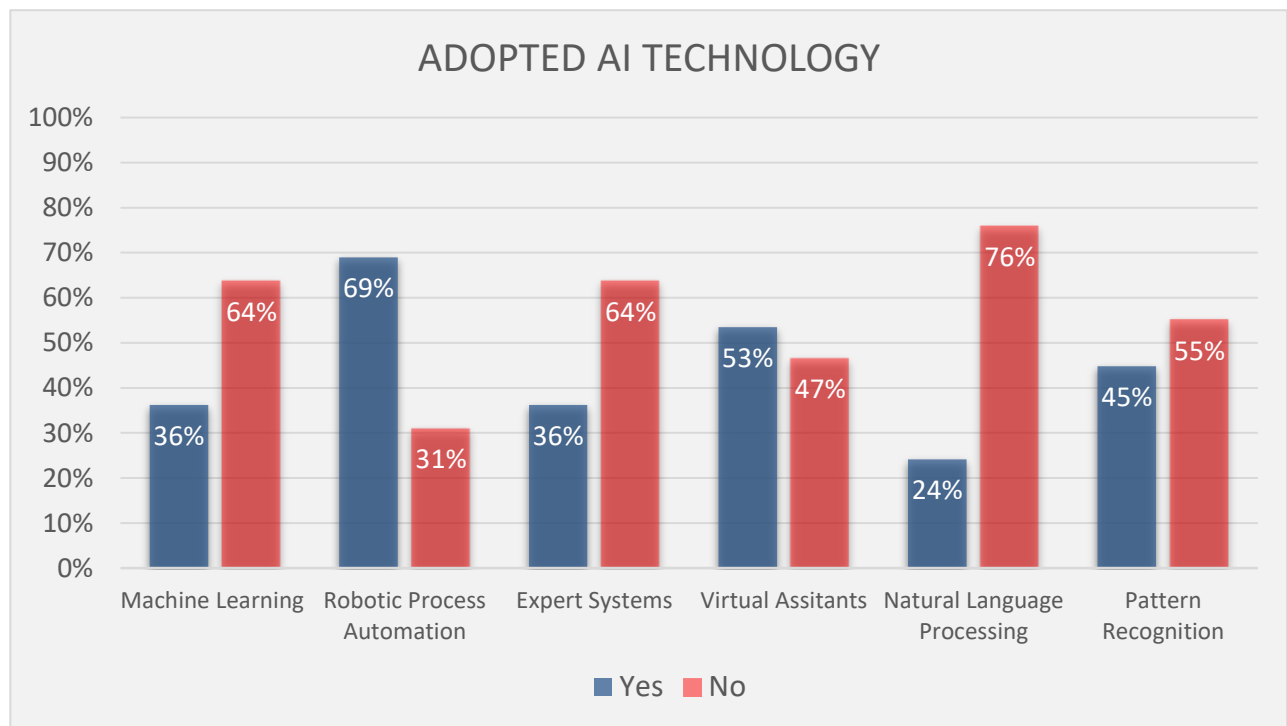
Figure 5.2: Adoption status of AI technologies (n=58)
