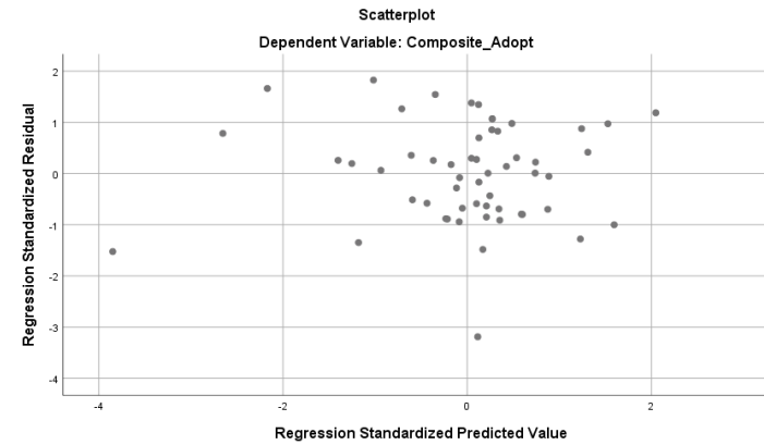
Figure A7: Organisational homoscedasticity plot
