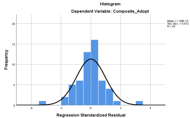
Figure A3: Technological residual histogram
