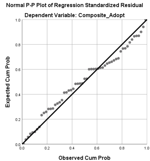
Figure A2: Technological residual p-p plot
