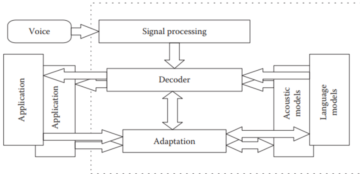
Figure 2.7: Speech recognition system architecture
