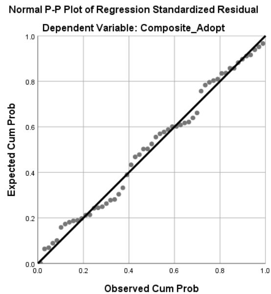
Figure A8: Environmental residual p-p plot
