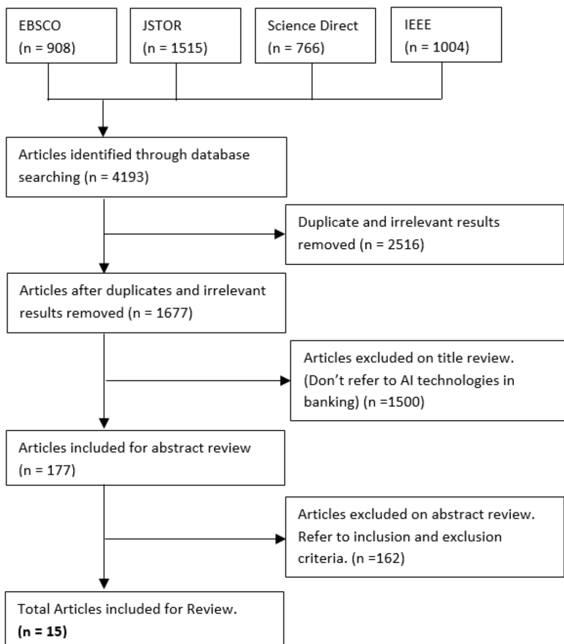
Figure 2.9: Systematic literature review results for TOE organisational studies
