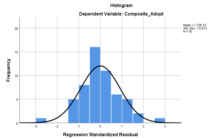
Figure A12: Stepwise residual histogram
