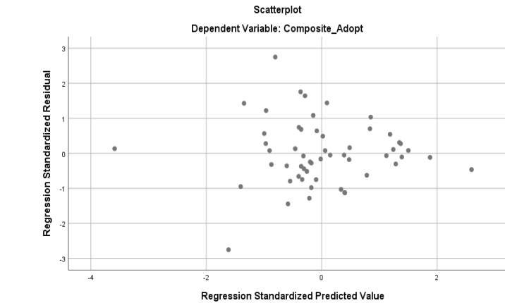
Figure A10: Stepwise homoscedasticity plot
