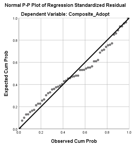
Figure A11: Stepwise residual p-p plot
