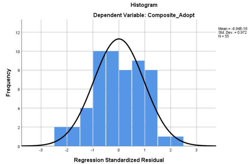
Figure A6: Organisational residual histogram
