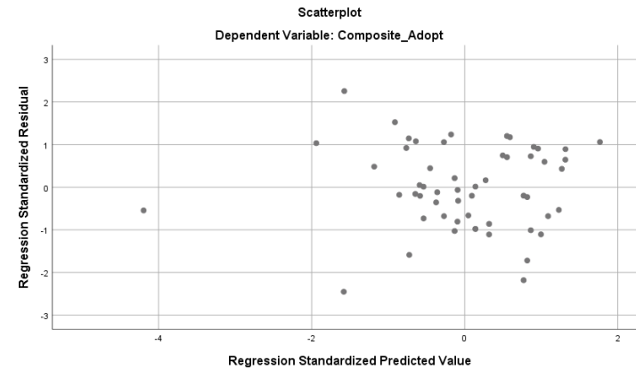
Figure A4: Organisational homoscedasticity plot
