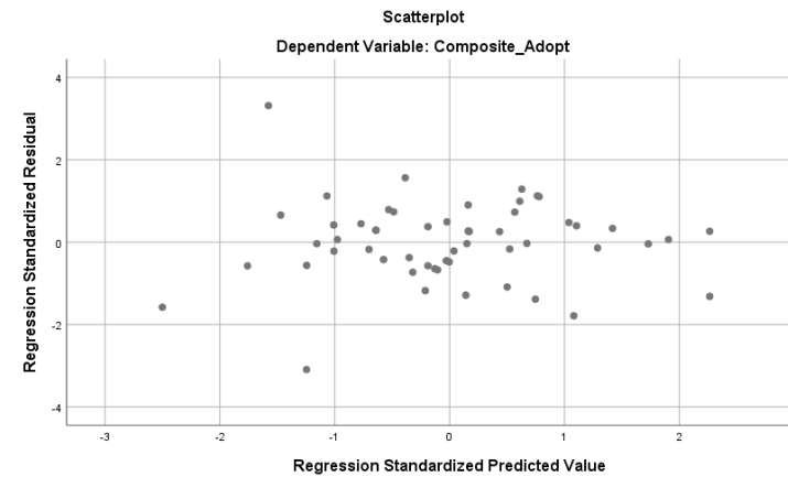
Figure A1: Technological homoscedasticity plot
