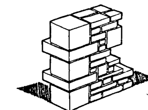
• STONE QUOIN WORK IN RUBBLE WALL
