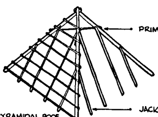
• PYRAMIDAL ROOF JACK RAFTERS.
