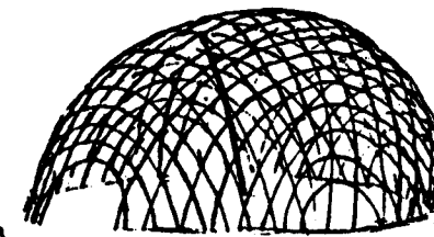
3. Structure of the beehive. 1. Entrance 2. Inner wall 3. Outer wall 4. Cone and beehive 5. Small hole for entrance 6. Entrance for cattle 7. Entrance for cattle
