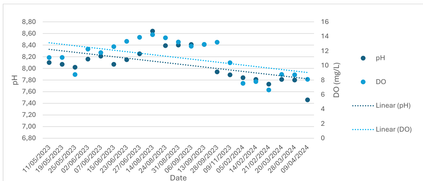
Figure 14: pH and DO analysis from the Montgomery Spruit.
