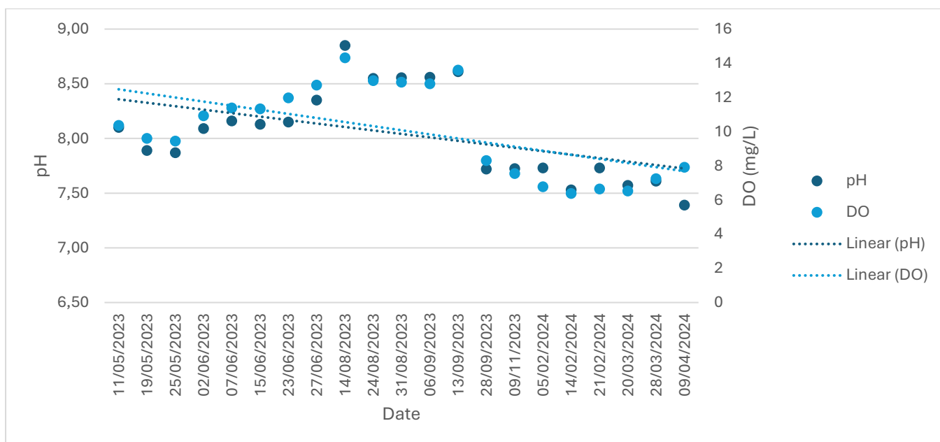
Figure 32: The pH and DO results from The Braamfontein Spruit at Delta Park
