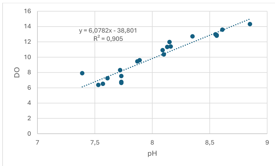
Figure 61: A graph showing the correlation between pH and DO in the Braamfontein Spruit at Delta Park
