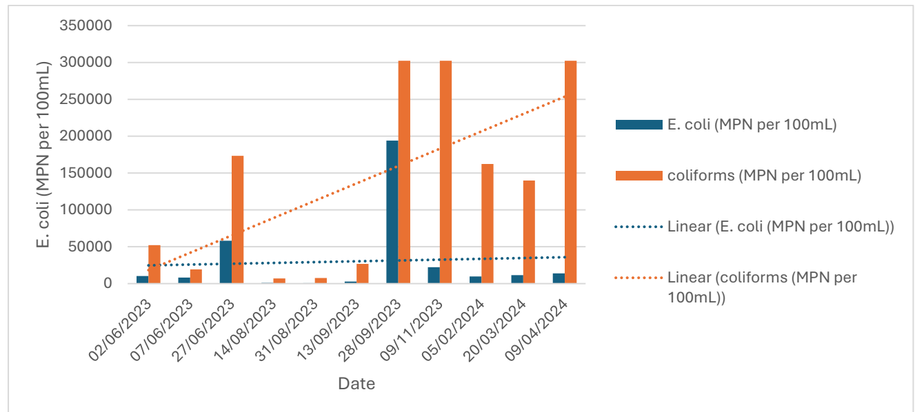
Figure 35: The E. coli and coliform results from The Braamfontein Spruit at Delta Park
