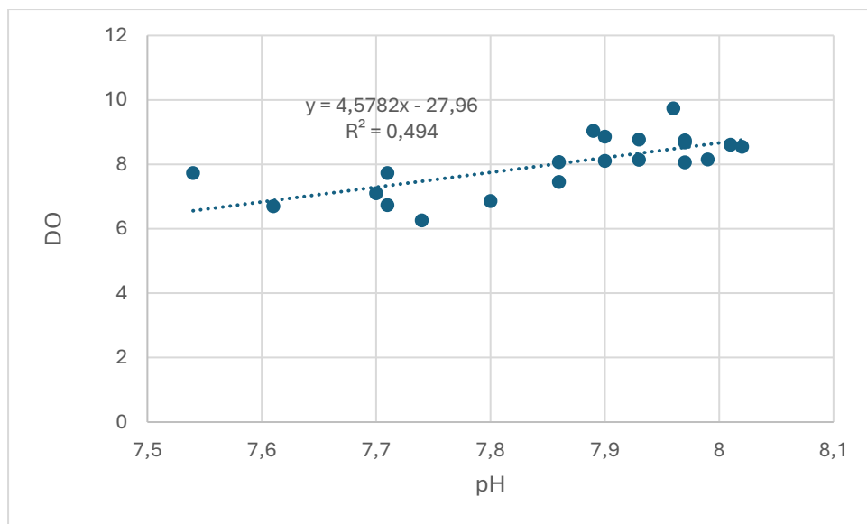
Figure 58: A graph showing the correlation between pH and DO in the Braamfontein Spruit at Parkview Golf Course
