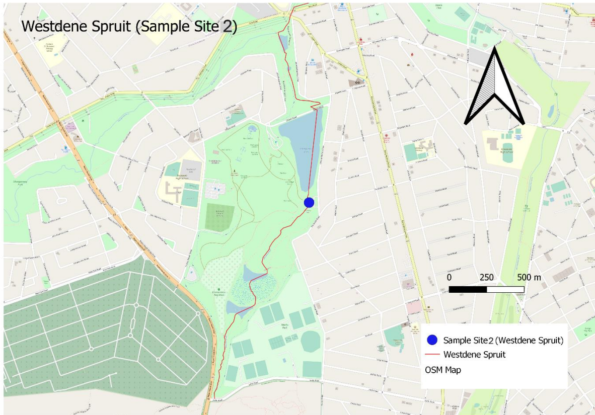
Figure 4: Site 2, The Westdene Spruit at Emmarentia Botanical Gardens
