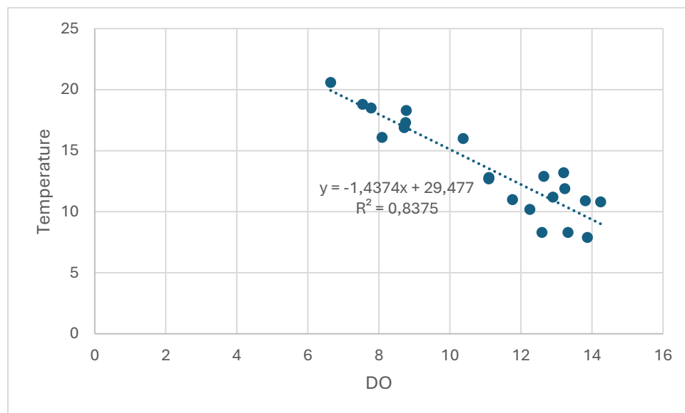
Figure 52: A graph showing the correlation between temperature and DO in the Montgomery Spruit
