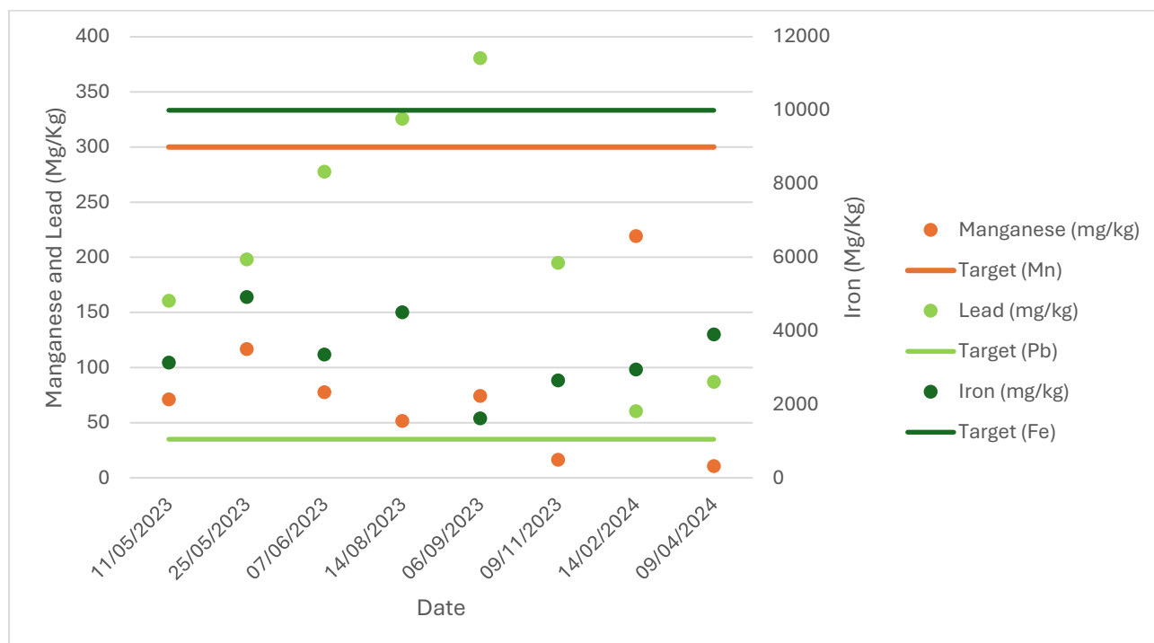
Figure 30: The manganese, iron and lead concentrations from the sediment samples taken from the Braamfontein Spruit at Parkview Golf Course
