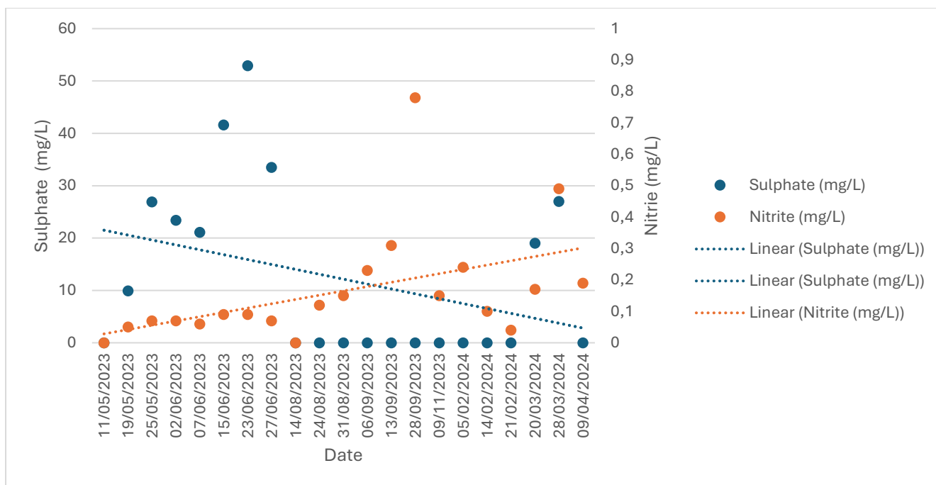
Figure 40: The Sulphate and Nitrite results from the Braamfontein Spruit at Sandton Riverclub Golf Course
