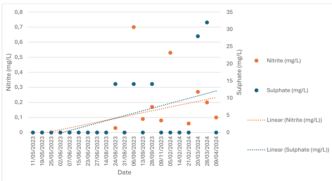
Figure 22: The nitrite and sulphate results from The Westdene Spruit at the Emmarentia Botanical Gardens
