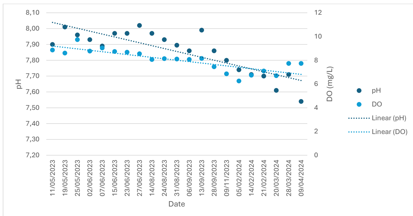
Figure 26: The pH and DO from The Braamfontein Spruit at the Parkview Golf Course
