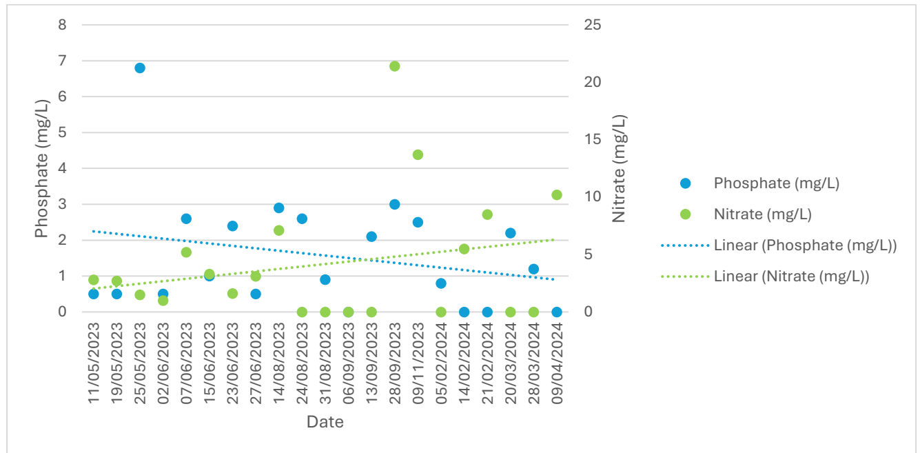
Figure 27: The Phosphate and Nitrate results from The Braamfontein Spruit at the Parkview Golf Course
