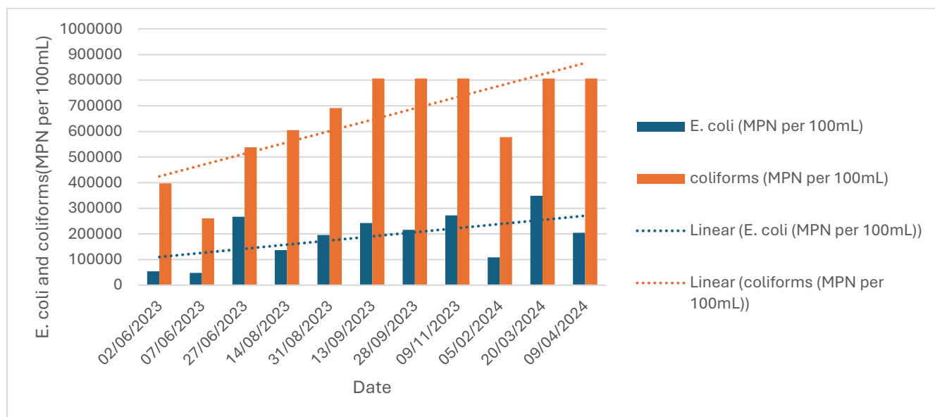
Figure 29: The E. coli and coliform results from The Braamfontein Spruit at the Parkview Golf Course
