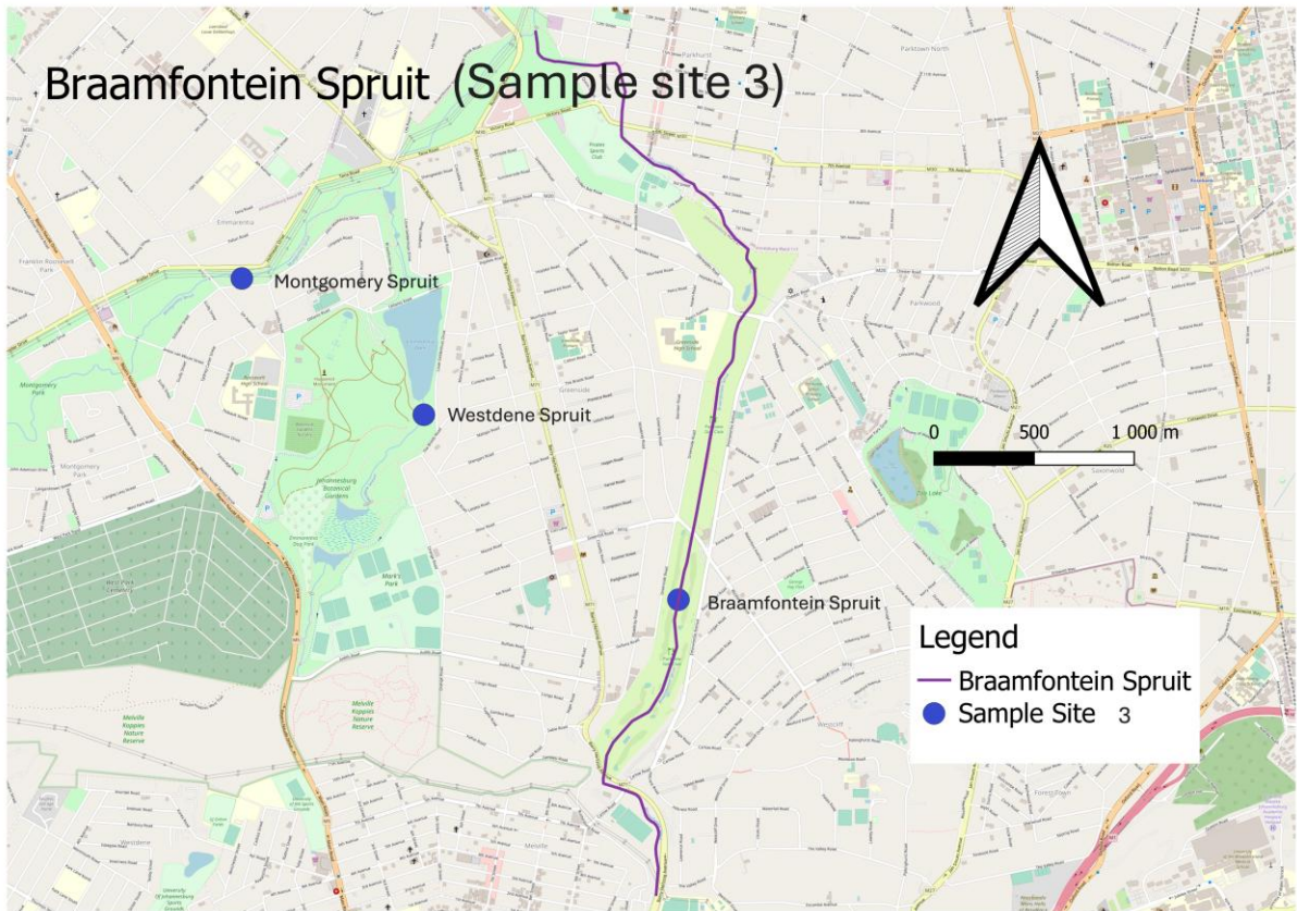
Figure 5: Site 3, The Braamfontein Spruit at Parkview Golf course (Site 1 and 2 included as reference)
