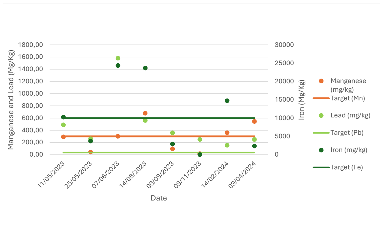
Figure 42: The manganese, iron and lead concentrations from the sediment samples taken from the Braamfontein Spruit at Sandton River Club
