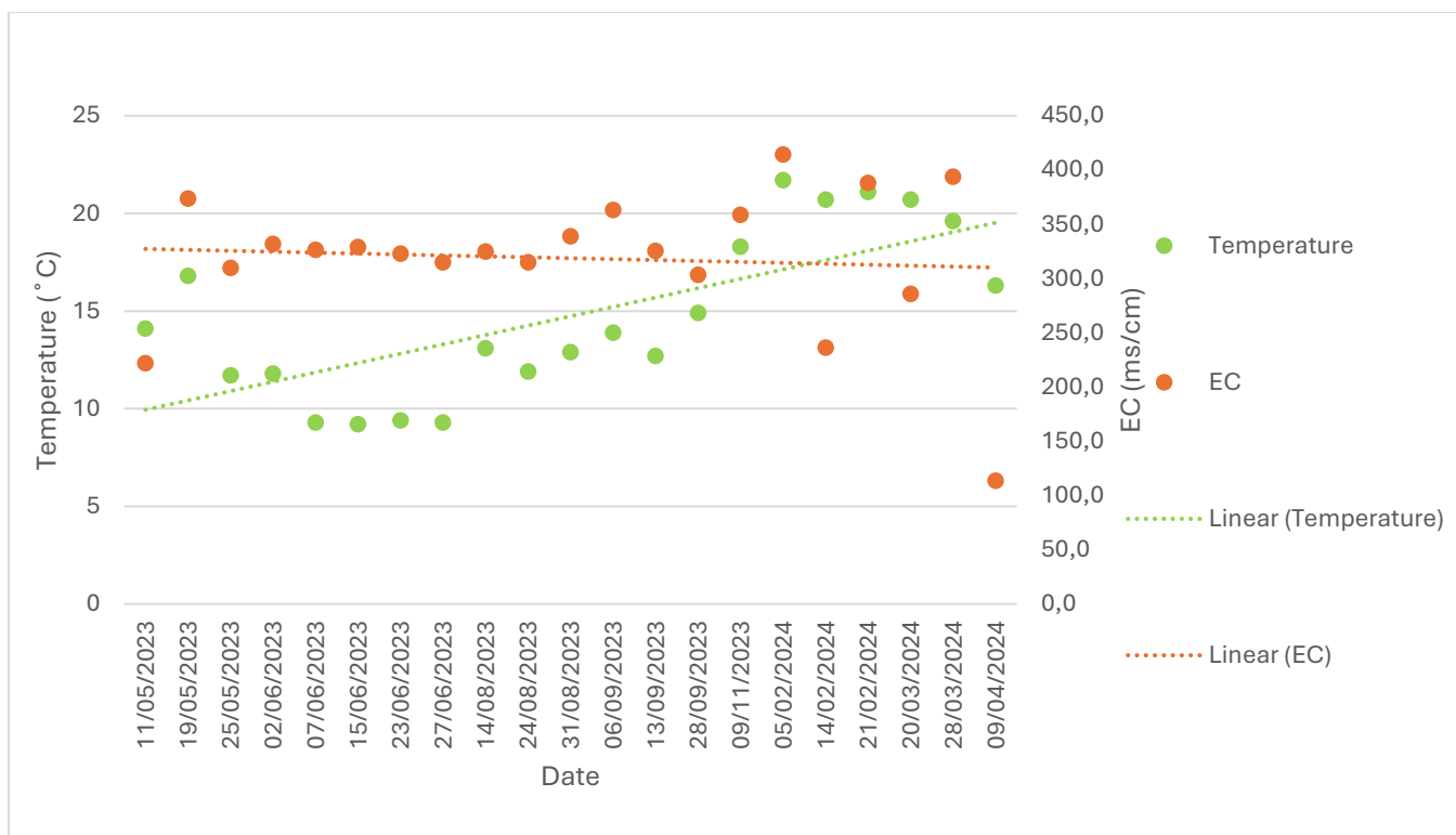
Figure 37: The Temperature and EC results from the Braamfontein Spruit at Sandton Riverclub Golf Course
