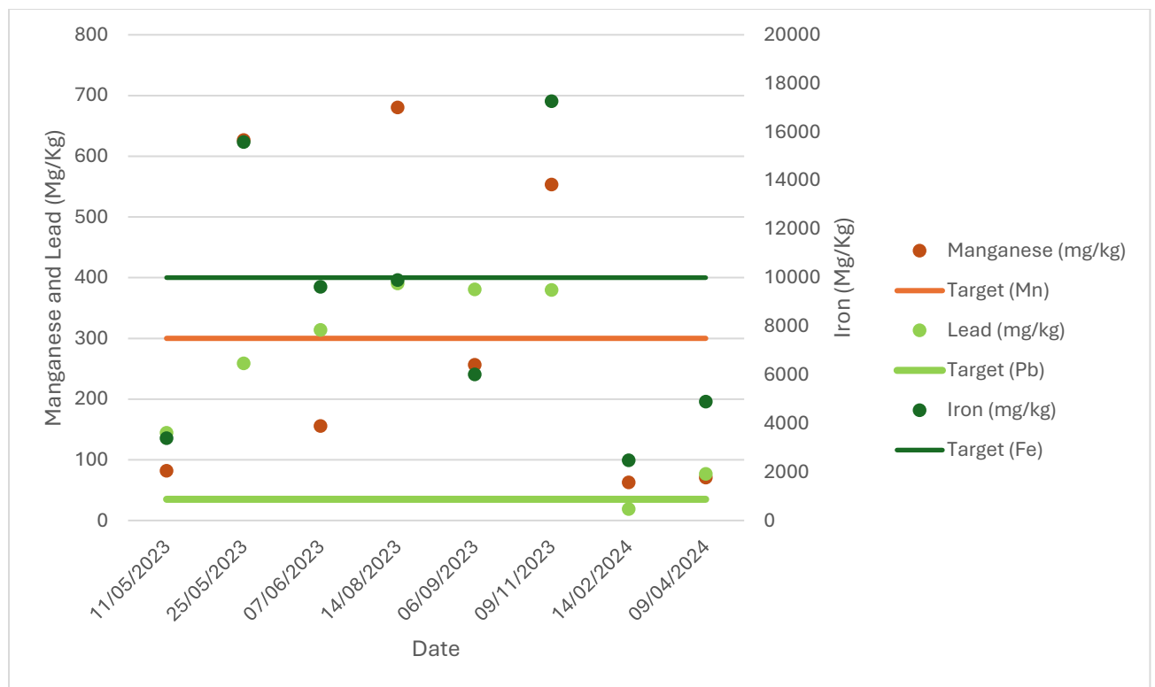
Figure 24: The manganese, iron and lead concentrations from the sediment samples taken from the Westdene Spruit
