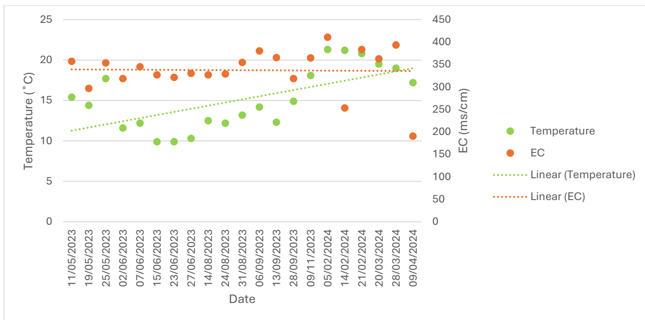
Figure 31: the Temperature and EC results from The Braamfontein Spruit at Delta Park
