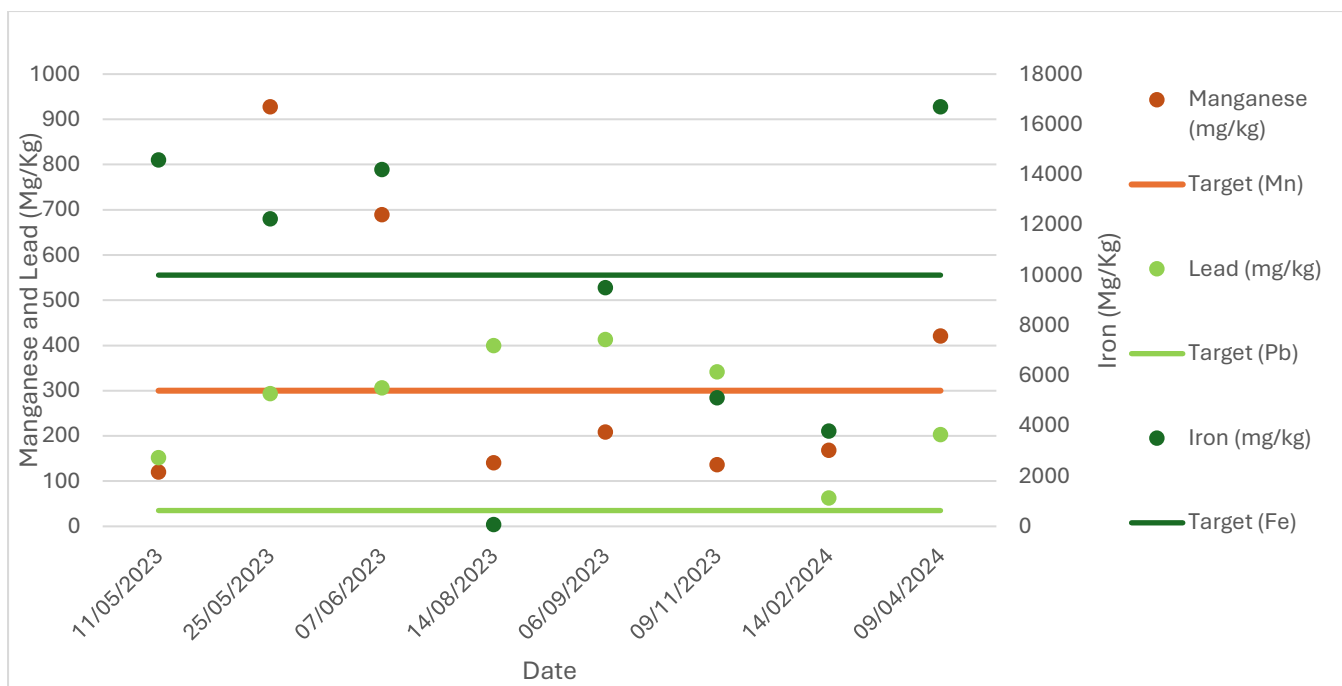
Figure 18: The manganese, iron and lead concentrations from the sediment samples taken from Montgomery Spruit
