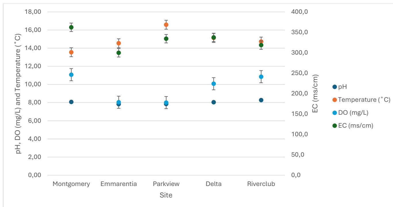
Figure 43: The average values recorded at each site for pH, DO, EC and temperature at each site
