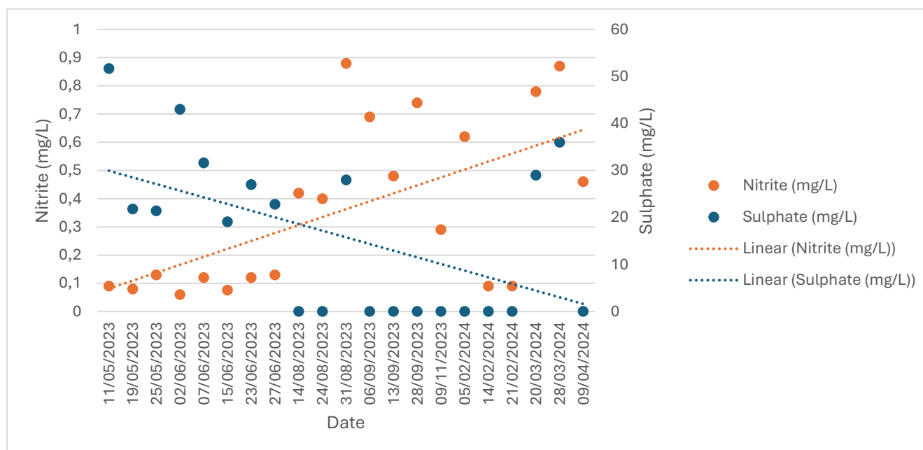
Figure 34: The Nitrite and Sulphate results from The Braamfontein Spruit at Delta Park
