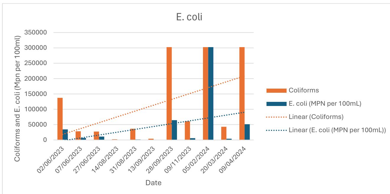
Figure 41: The E. coli and total coliforms results from the Braamfontein Spruit at the Sandton Riverclub Golf Course
