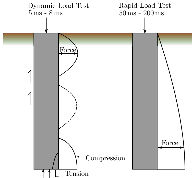
Figure 1.3: Comparison of the force profile developed along the pile [4].
