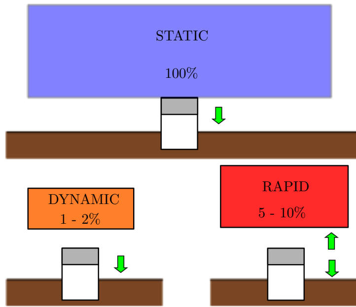
Figure 1.2: Load comparison of the various testing methods, adapted from [5].
