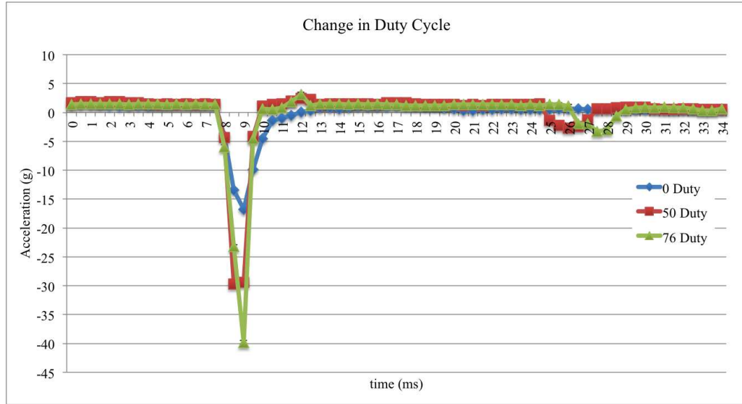
Figure 7.6: Comparison of all the different duty cycle schemes.
