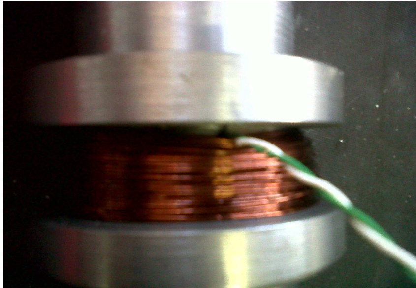
Figure 5.10: Placement of the thermocouple cable through the piston.
