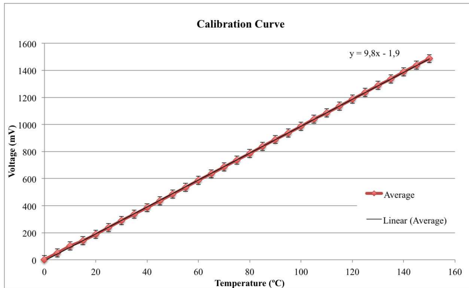
Figure 5.14: The calibration curve for the thermocouple amplifier.
