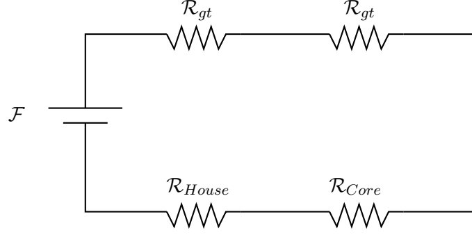
Figure 3.7: Equivalent magnetic circuit model.
