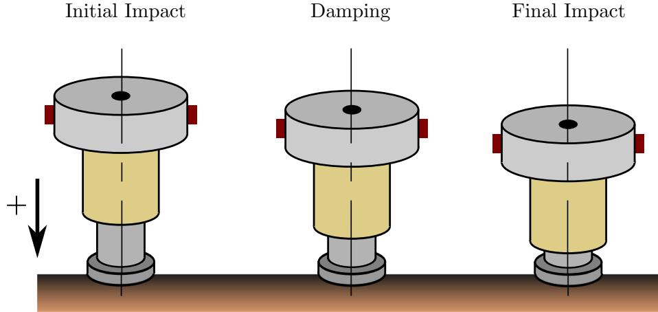
Figure 3.5: Operation of the damper as it impacts with the test pile.
