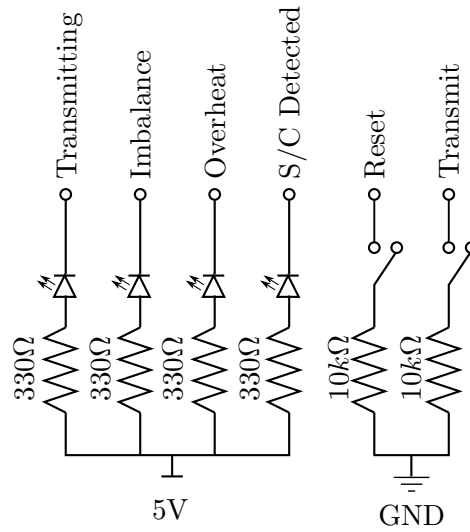
Figure 4.5: Pull-up LED indicator circuit.
