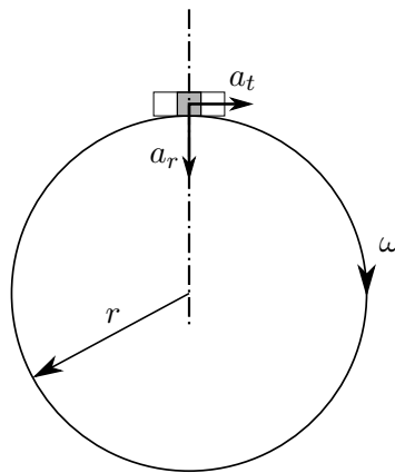
Figure 5.4: The accelerometer as placed on a rotating trajectory, adapted from [53].
