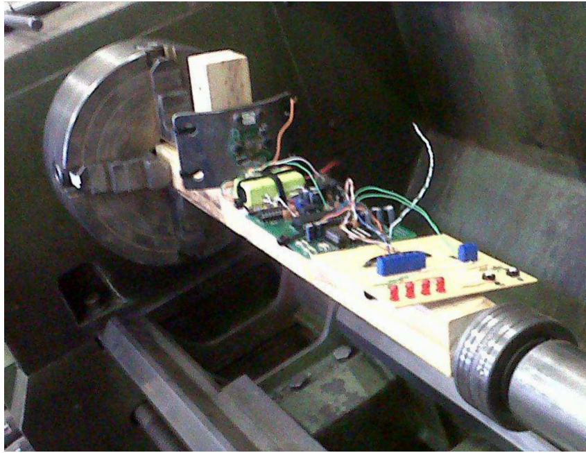
Figure 5.6: The mounted accelerometer and circuit in the lathe.
