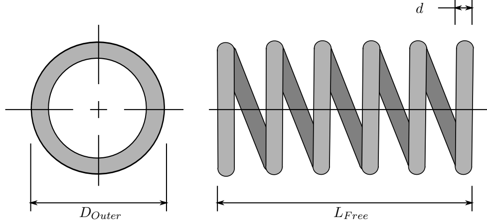
Figure 3.3: Annotated diagram of the spring.
