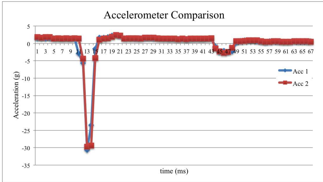
Figure 7.1: Comparison of the two accelerometers.
