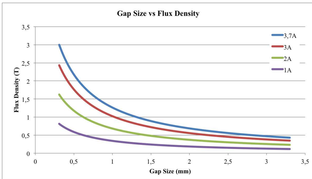
Figure 3.9: The relationship between the gap and current for the installed coil.
