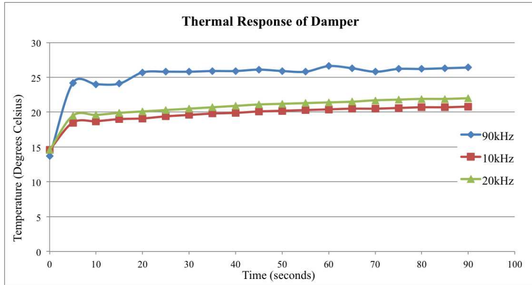
Figure 7.3: Thermal response of the three operating frequencies.
