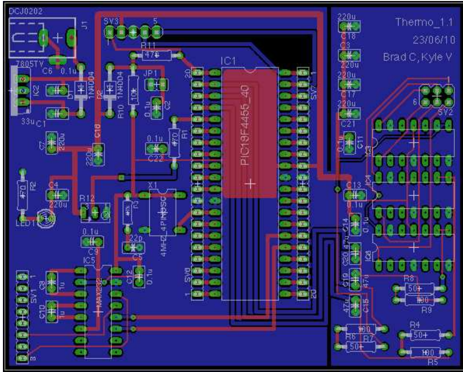
Figure 4.7: Top and bottom layers of the controller PCB.
