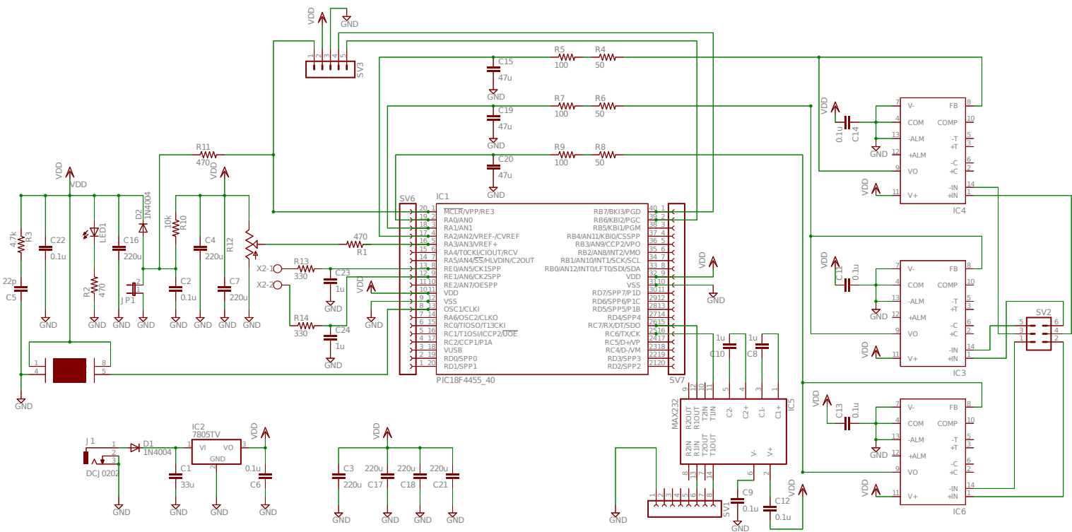
Figure A.1: Circuit diagram of the controller.
