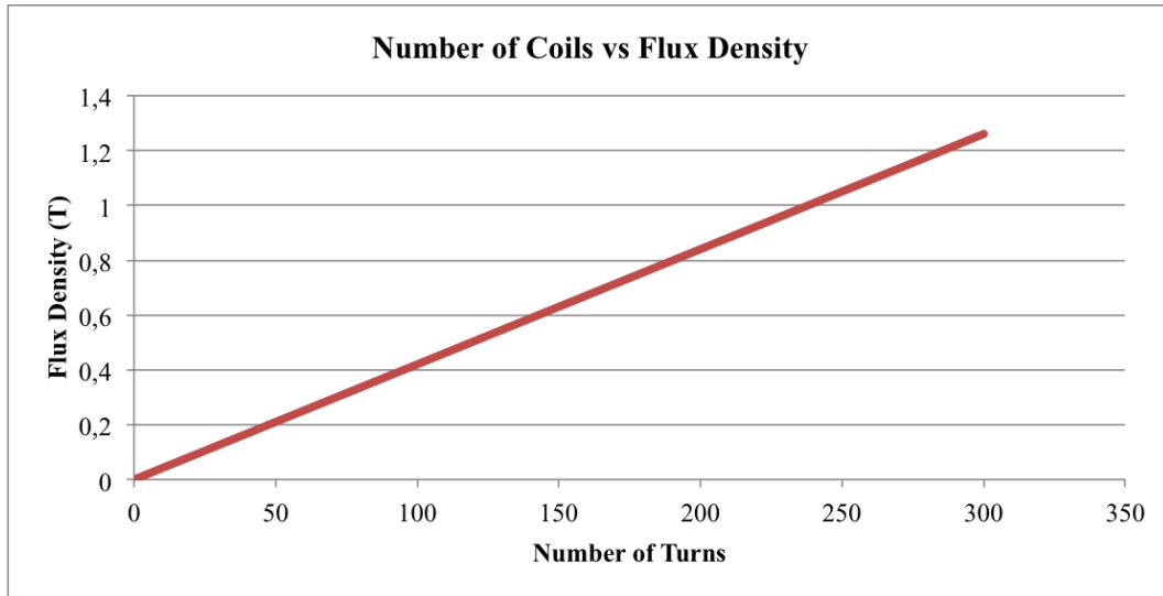
Figure 3.8: Number of turns versus the flux density in the gap.
