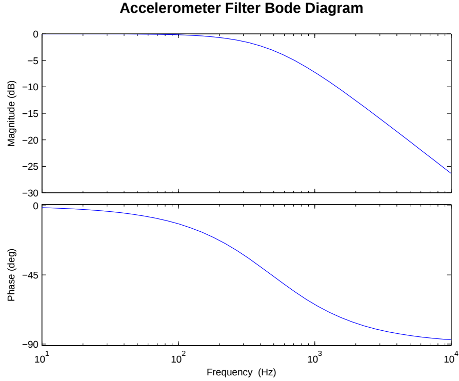
Figure 4.4: Bode diagram of the accelerometer filters.
