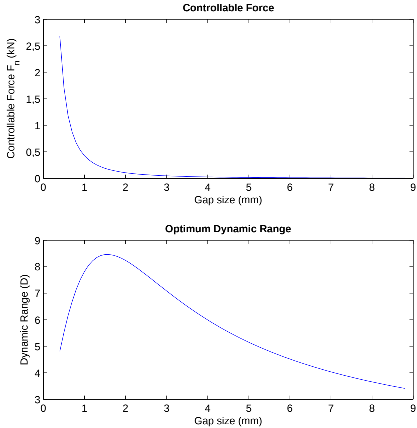
Figure 3.14: Modelled response of shock absorber for a change in gap size.
