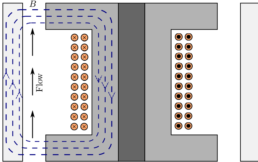
Figure 3.6: Cross-section of the magnetic circuit region.
