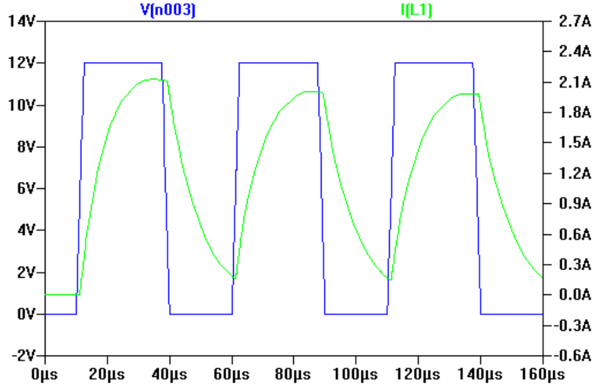
Figure 4.10: Simulation of the current through the coil versus the gate voltage.
