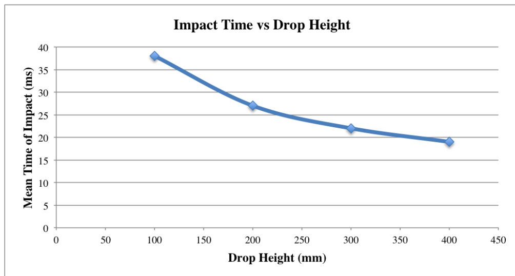
Figure 2.4: The results from the damper in its second revision.
