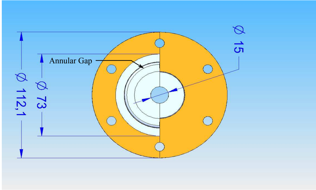
Figure 3.4: Half cross-section of the damper viewed from the top plane.
