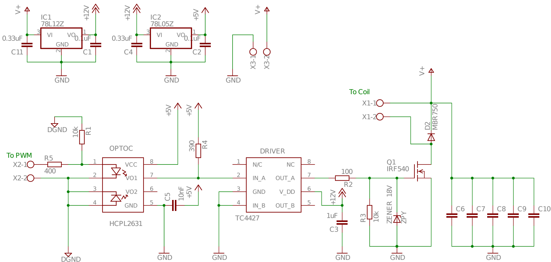
Figure B.1: Circuit diagram of the MOSFET driving circuit.
