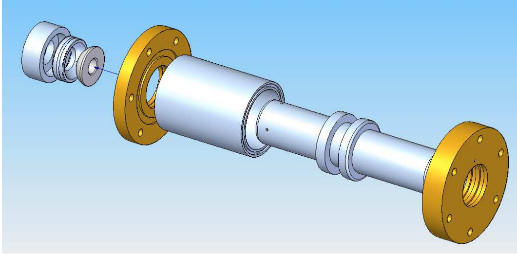
Figure 3.2: An exploded view of the damper.
