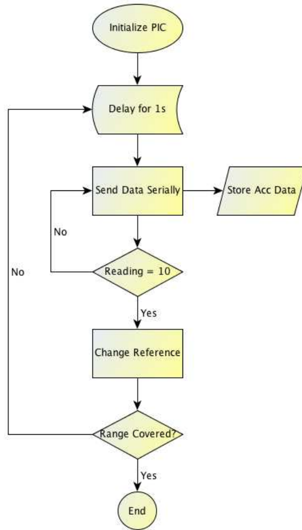
Figure 5.11: Flow diagram of the thermocouple calibration process.
