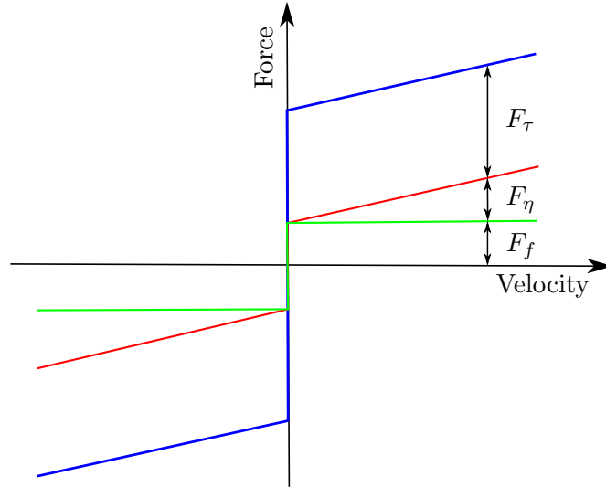
Figure 3.13: Decomposition of forces in an MR fluid, adapted from [7].
