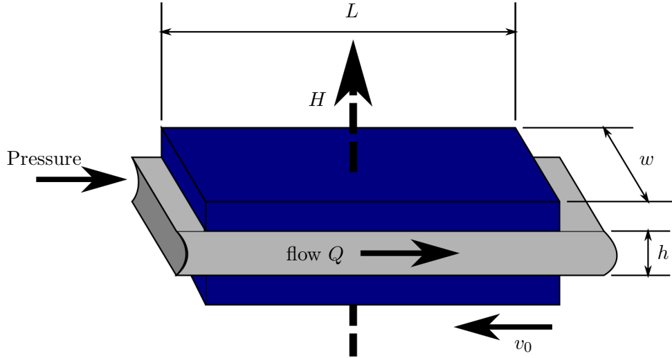
Figure 3.12: Behaviour of MR fluid through a parallel duct, adapted from [7].
