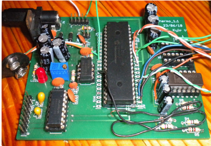
Figure 4.1: Photograph of the controller unit, showing the populated PCB.
