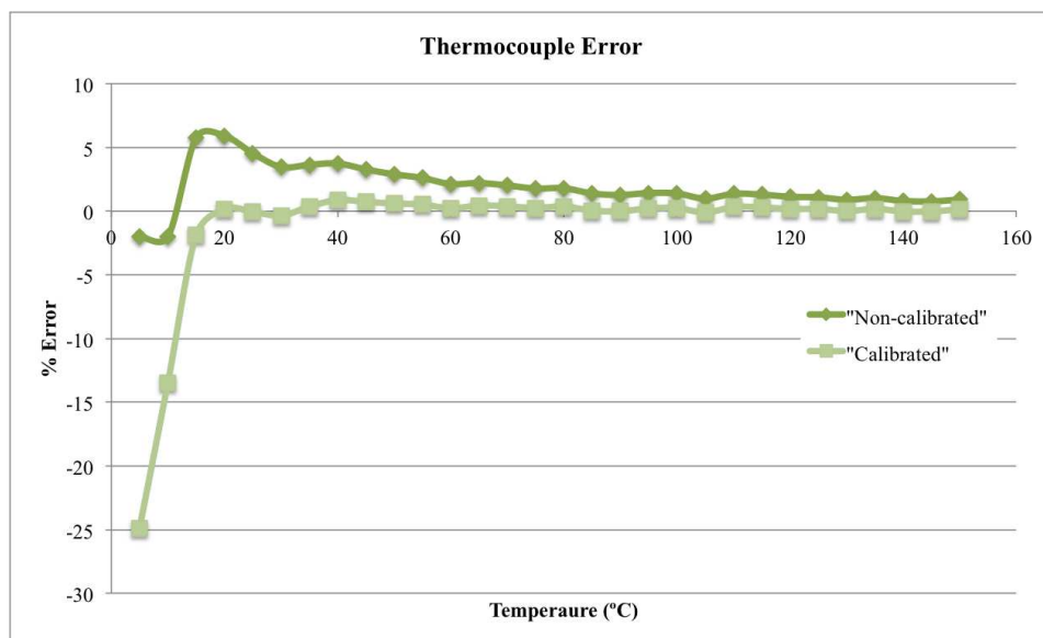
Figure 5.15: Comparison between calibrated and non-calibrated error.
