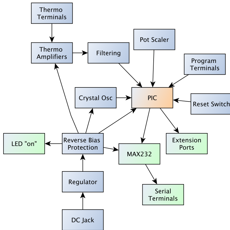
Figure 4.6: Block diagram representation of the controller functions.
