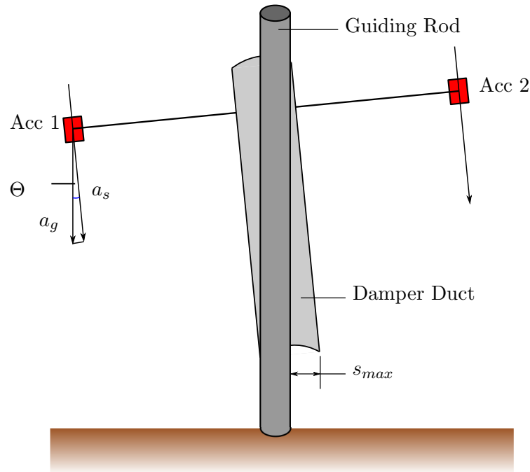
Figure 6.2: Misalignment affect on the experiment.
