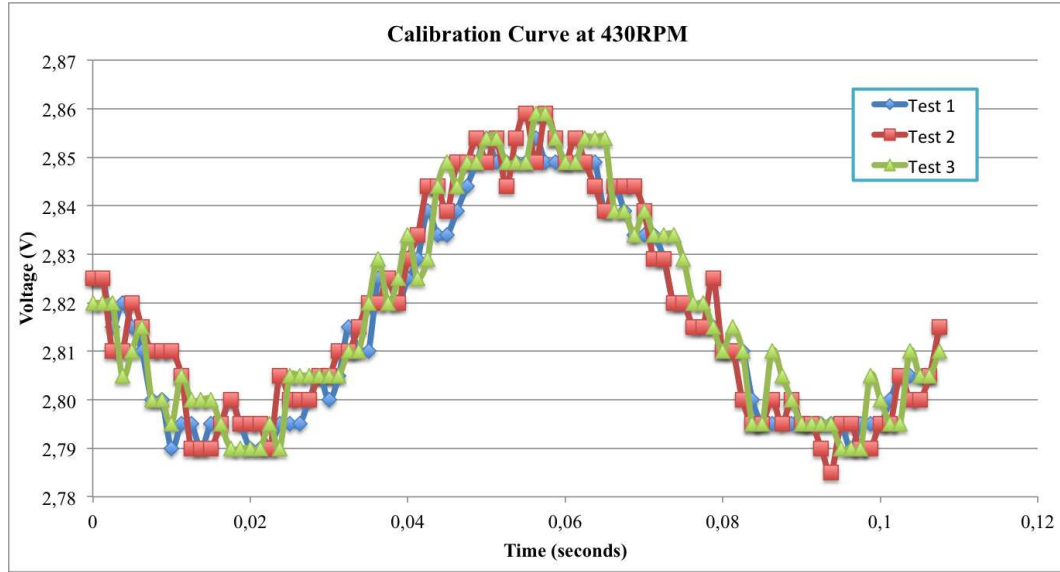
Figure 5.7: Results obtained from three experiments at 430 RPM using Acc 1.
