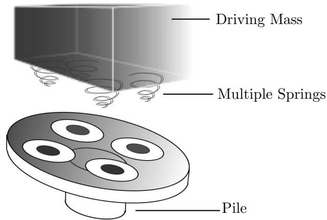
Figure 2.3: Concept behind the Fundex Pile Test [3].
