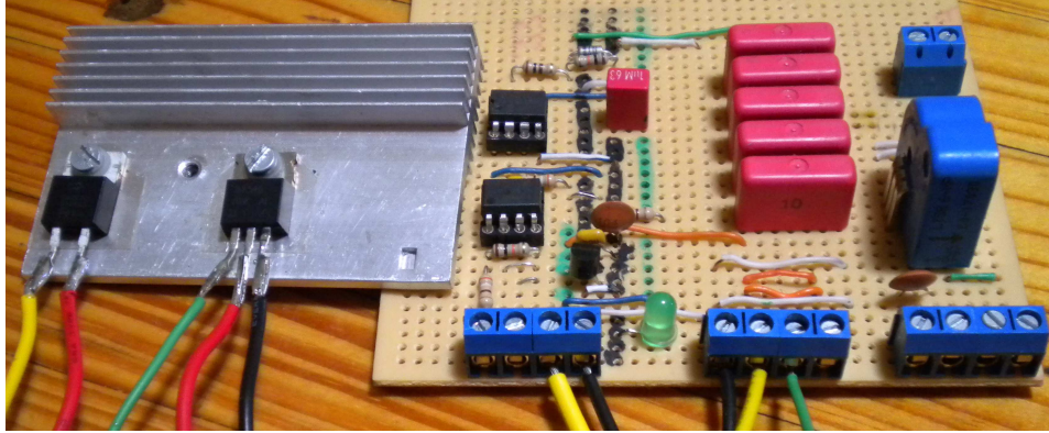
Figure 4.9: Photograph of the driver circuit on veroboard.
