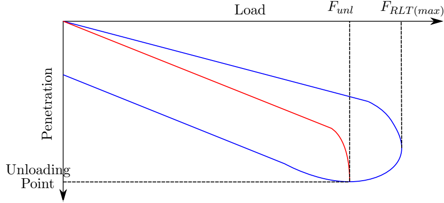
Figure 2.1: The RLT using the Unloading Point Method, adapted from [4, 24]
