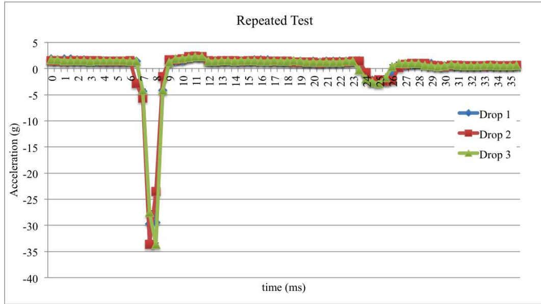
Figure 7.5: Acceleration data from three tests under identical conditions.
