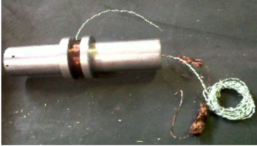
Figure 3.10: Photograph of piston with wound coil and thermocouple cable.
