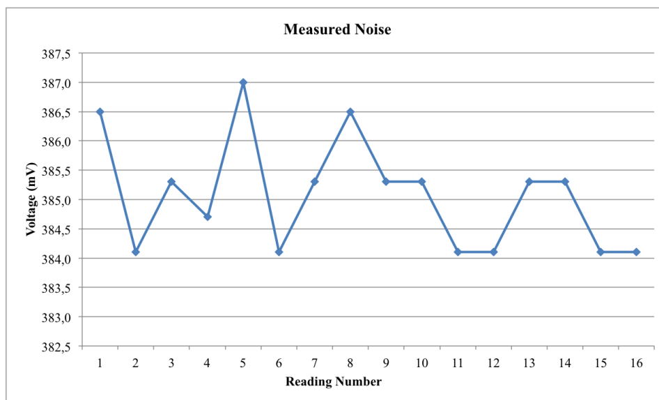
Figure 5.13: Typical noise on thermocouple circuit at 38,5°C.
