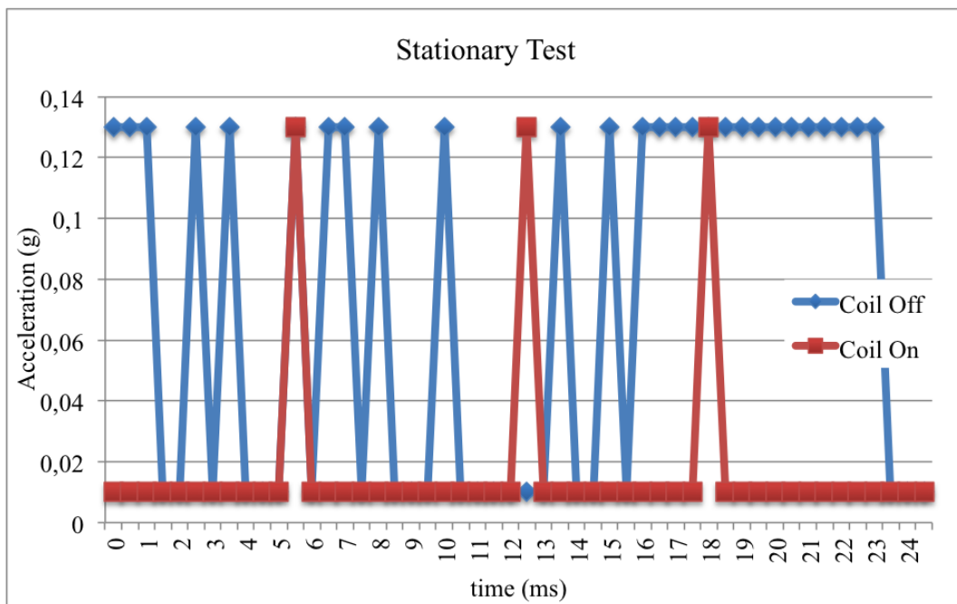
Figure 7.2: Accelerometer output while stationary.
