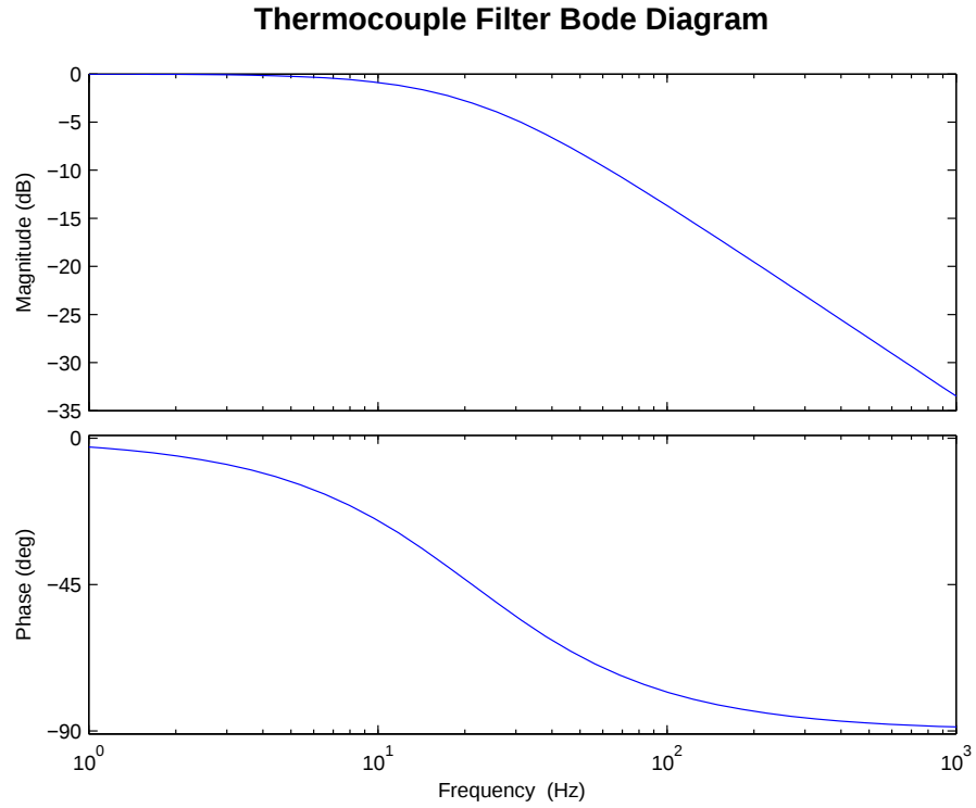
Figure 4.3: Bode diagram of the thermocouple filters.
