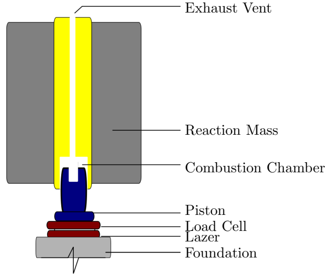
Figure 2.2: The typical Statnamic test apparatus, adapted from [5].
