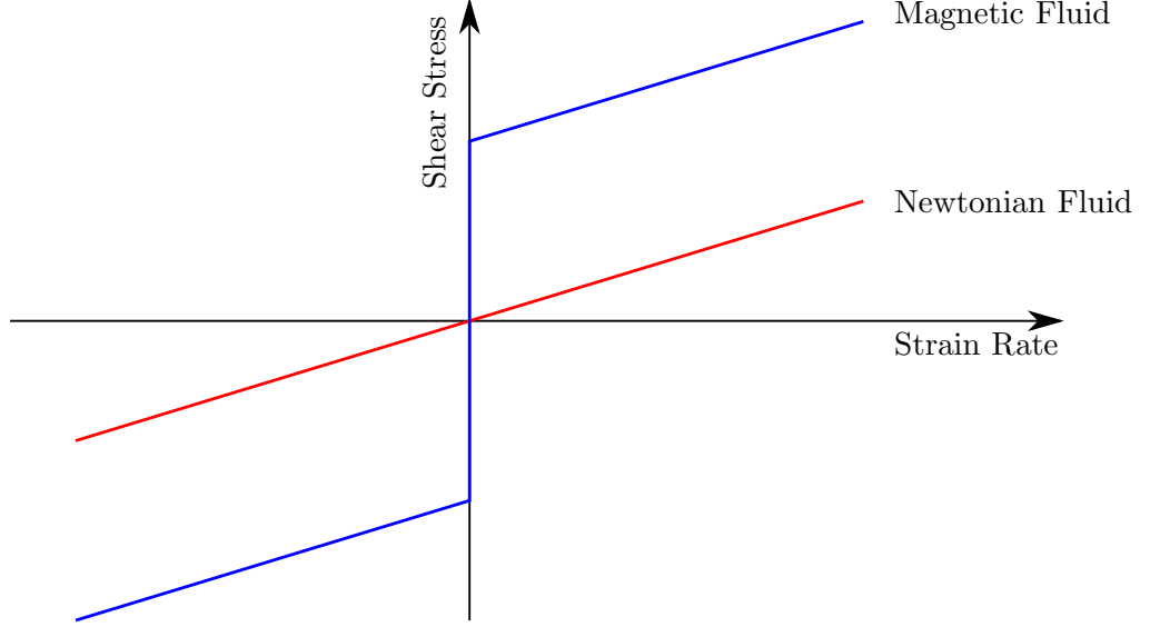
Figure 1.5: Newton model of fluid [7].
