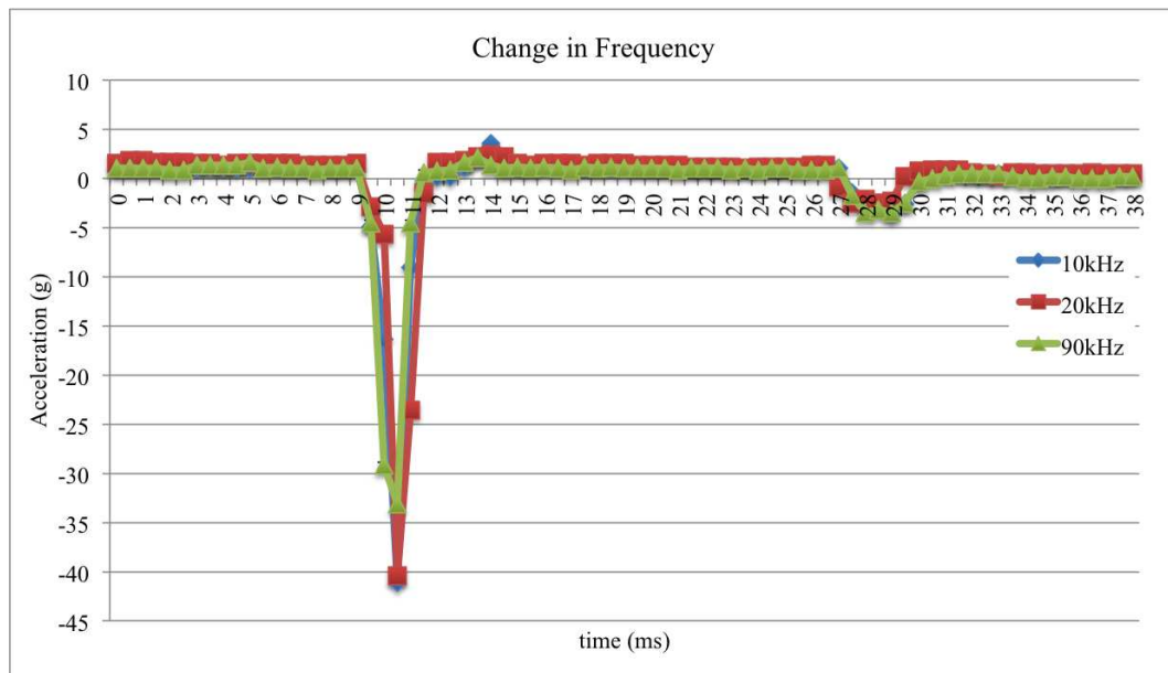
Figure 7.4: Comparison of all the different frequency schemes.
