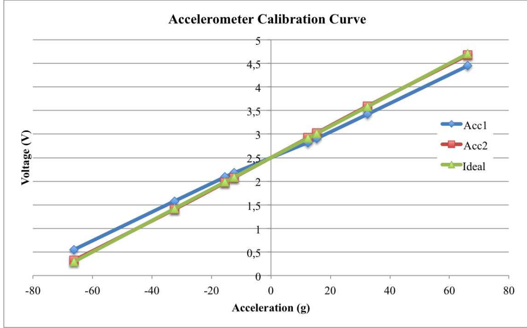
Figure 5.8: Calibration curves for the accelerometers.
