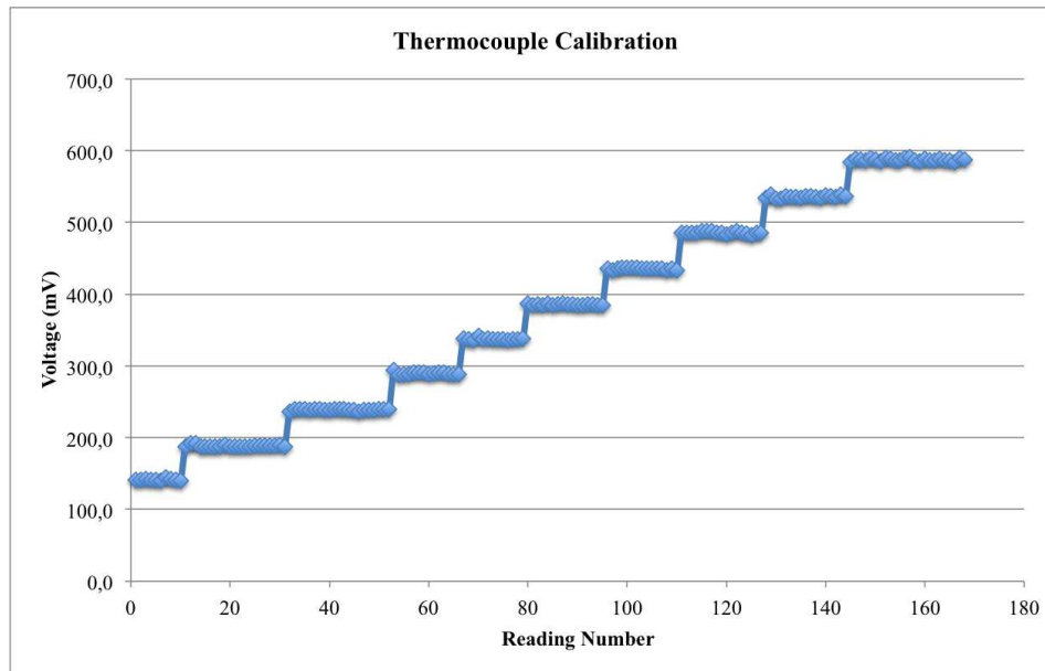
Figure 5.12: Results obtained directly from the calibration process.
