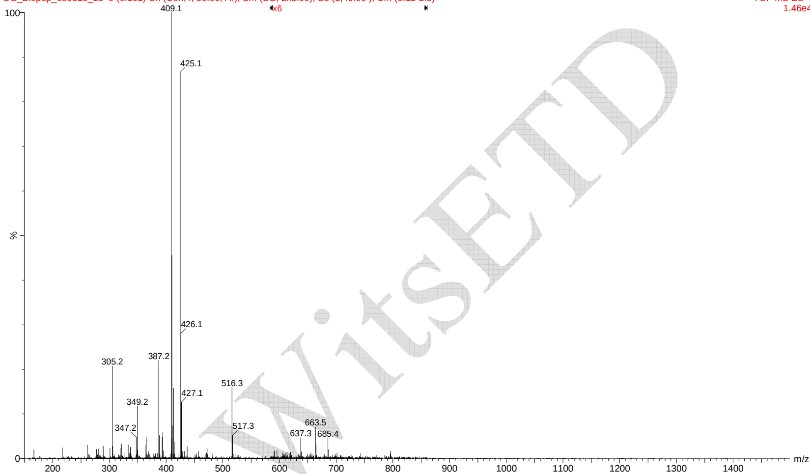
Figure 38: ESI-MS spectra of fractionated crude extract sample Fraction 4 for sample A.
