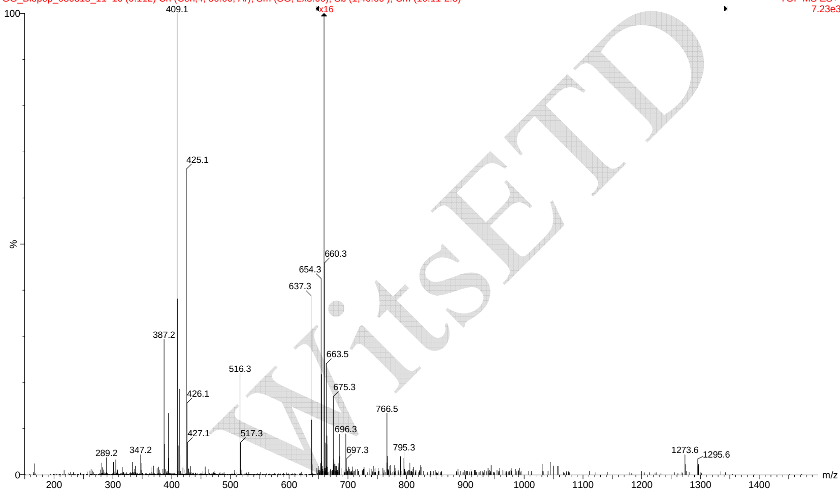
Figure 36: ESI-MS spectra of fractionated crude extract sample diluted Fraction 5 for sample A.
