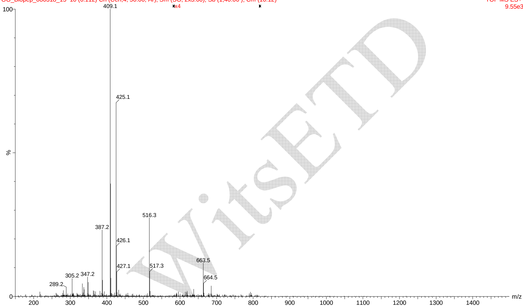
Figure 40: ESI-MS spectra of sample blank for fractionated crude extract samples.
