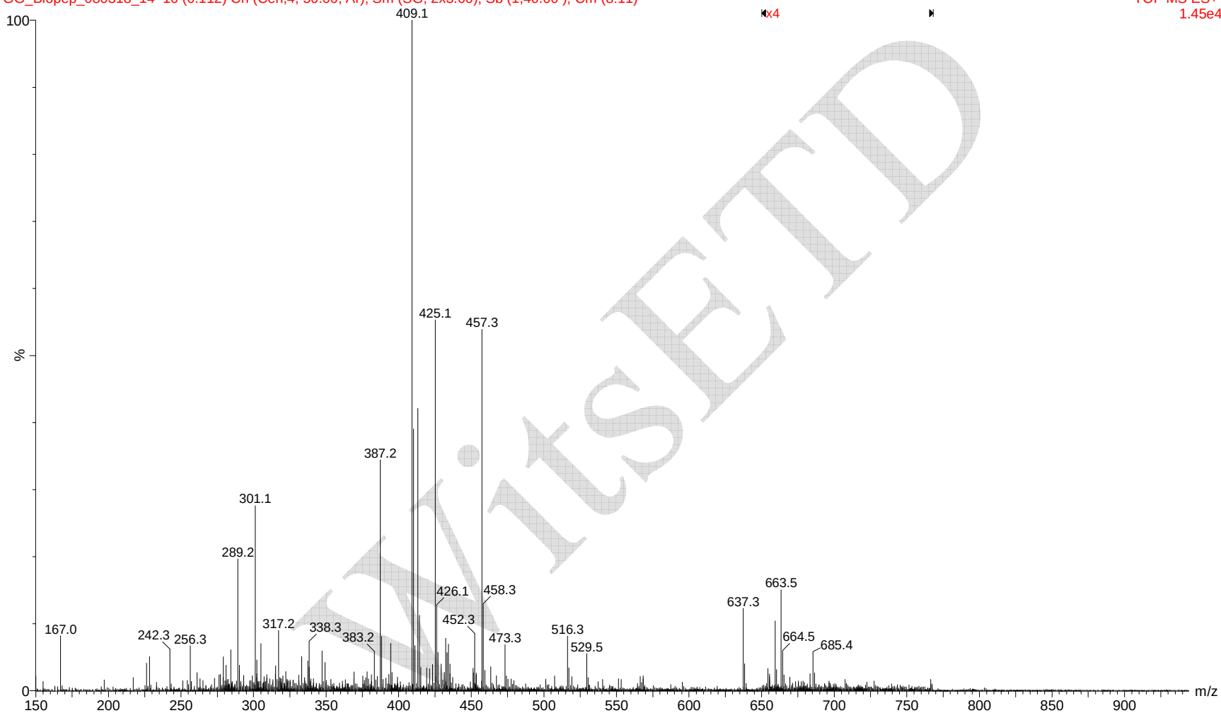
Figure 39: ESI-MS spectra of fractionated crude extract sample Fraction 5 for sample A.
