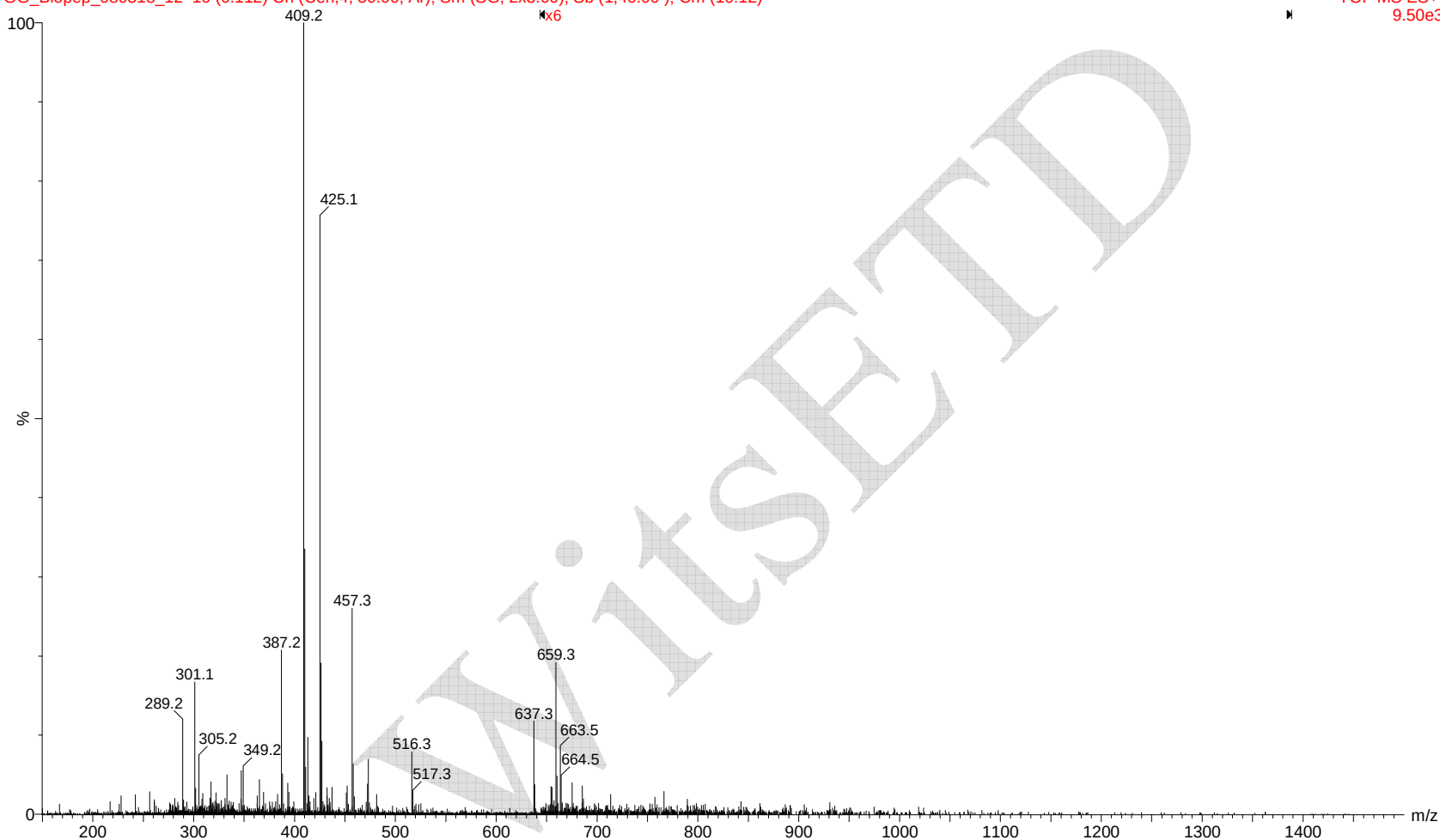
Figure 37: ESI-MS spectra of fractionated crude extract sample diluted Fraction 6 for sample A.
