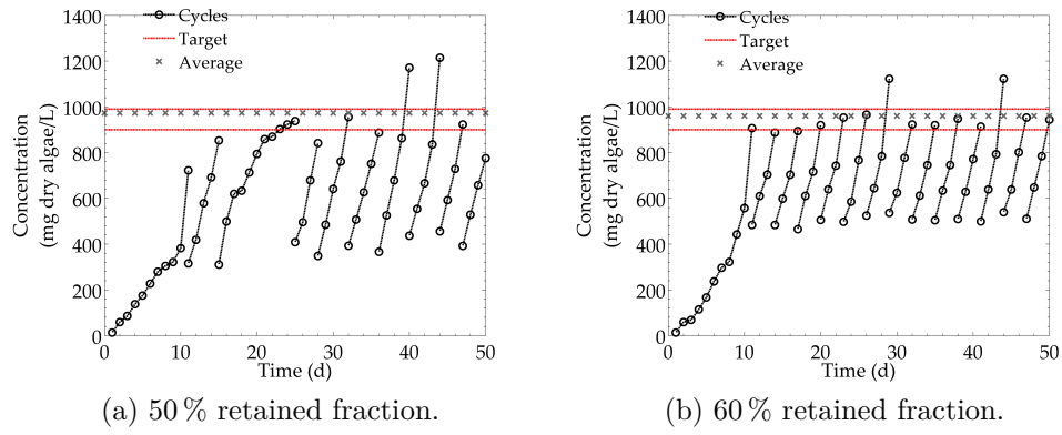
Figure G.1.12: Growth profile 50–60% \Phi at 900–1000 mg/L range.
