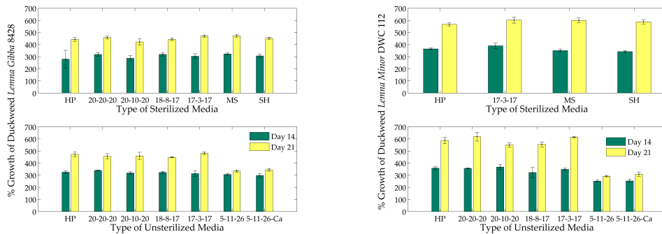
Figure G.2.3: % Growth rate comparison for Lemna in sterilized and unsterilized media. For each species, at day 21, there was no difference ( p > 0.05 ) when grown in unsterilized media with: 1) sterilized media 2) SH and MS control.
