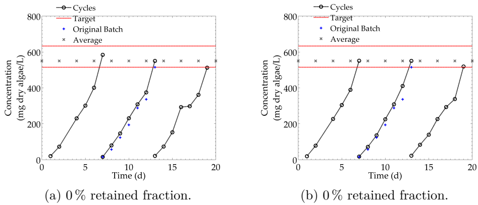
Figure G.1.14: Growth profile 0% \Phi at 500–600 mg/L range.
