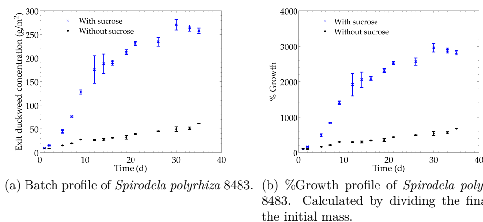
Figure 6.3.1: Batch and growth percentage for sucrose and no sucrose.
