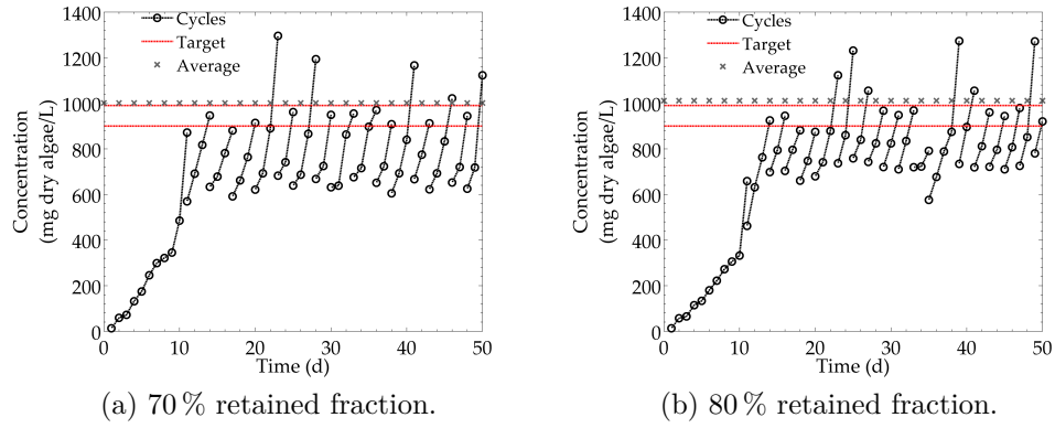
Figure G.1.13: Growth profile 70–80% \Phi at 900–1000 mg/L range.
