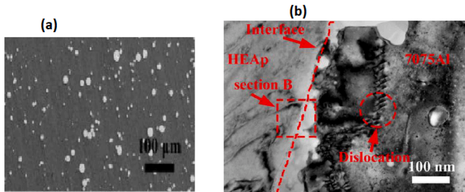
Fig. 3. Composite's microstructure showing (a) the morphologies and distribution of the high entropy alloy particle reinforcements (5 vol%) in the 7075 Al matrix and (b) transmission electron micrograph revealing the interfacial interaction between the high entropy alloy particles and the 7075 Al matrix. [68] culled with permission from Elsevier.
