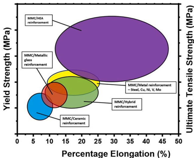
Fig. 19. Material selection chart for metal matrix composites (MMCs) with different reinforcement materials (ceramics, metals, metallic glass, hybrid and high entropy alloys (HEAs)).
