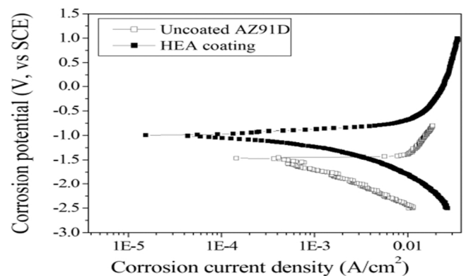
Fig. 18. Several specimens' potentiodynamic polarisation curves in 3.5 wt% sodium chloride solution (HEA – high entropy alloy). [121] culled with permission from Elsevier.
