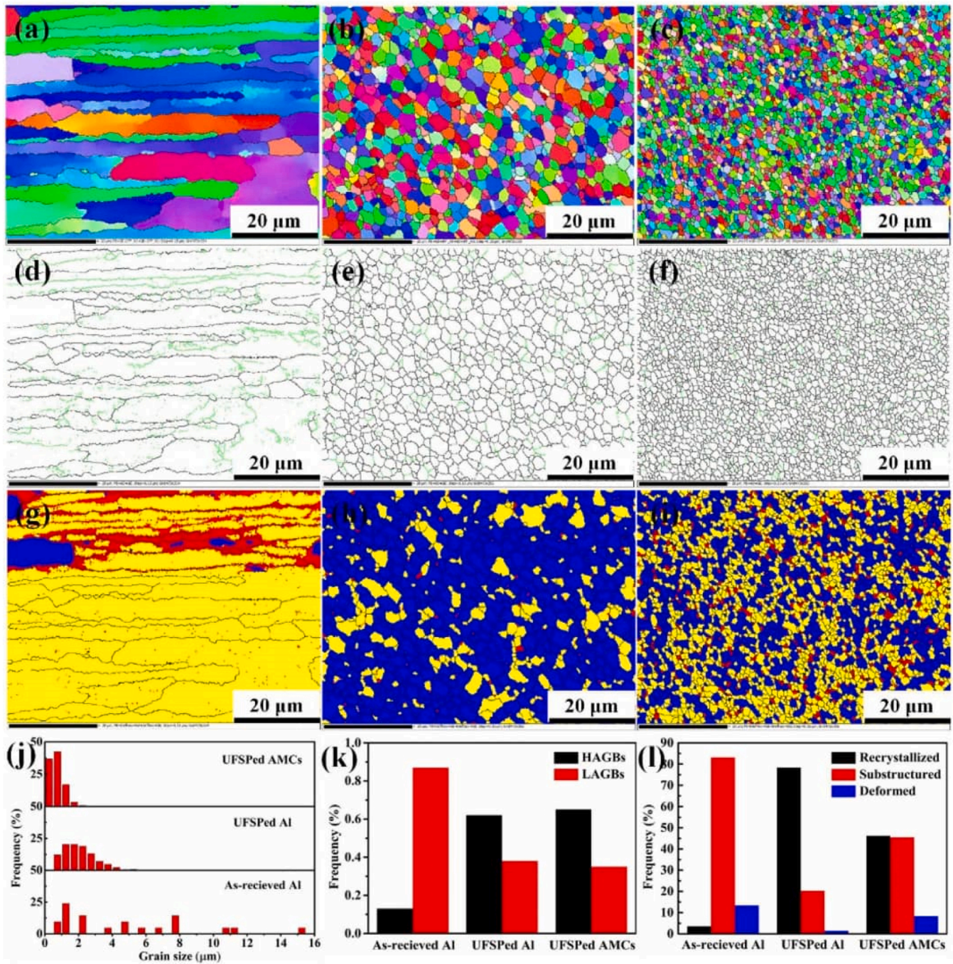
Fig. 8. Electron backscatter diffraction results of the as-received Al, underwater friction stir processed (UFSPed) Al, and UFSPed Al matrix composites (AMCs) showing (a, b, c) the inverse pole figures, (d, e, f) microstructures, (g, h, i) recrystallisation maps, respectively, (j) grain size distribution, (k) summarised results of high-angle grain boundaries (HAGBs) and low-angle grain boundaries (LAGBs), (l) summarised results of recrystallised, substructured and deformed region. [76] culled with permission from Elsevier.
