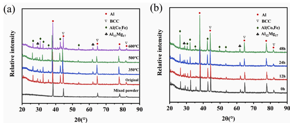
Fig. 10. X-ray diffraction patterns of composites under different heat treatment conditions show (a) heat treatment at different temperatures at 24 h; (b) heat treatment at 500°C at different times.
