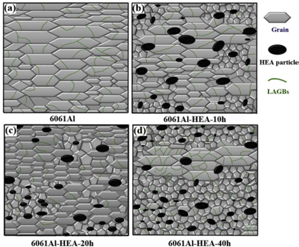
Fig. 7. Schematic diagram of grain characteristics in 6061 Al, 6061 Al-HEAp-10 h composite, 6061 Al-HEAp-20 h composite and 6061 Al-HEAp-40 h composite (HEA – high entropy alloy; LAGBs – low-angle grain boundaries). [101] culled with permission from Elsevier.
