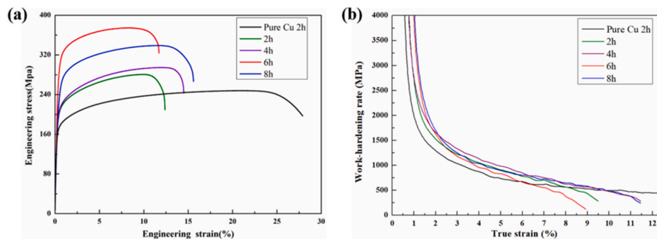
Fig. 12. Mechanical properties of 10 vol% high entropy alloy particle/Cu composites as-extruded under various heating times (a) tensile strain-stress curves and (b) work-hardening-strains.
