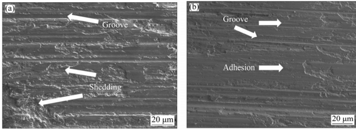
Fig. 17. Scanning electron micrographs of the damaged surfaces of (a) high entropy alloy particle/Cu (B) high entropy alloy particle/transition layer/Cu. [37] culled with permission from Elsevier.
