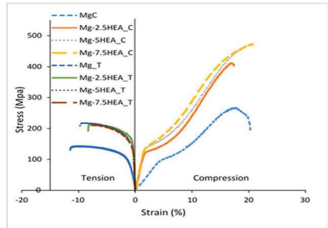
Fig. 13. Stress-strain graphs of Mg and Mg-HEAp composites under tensile and compression strain.
