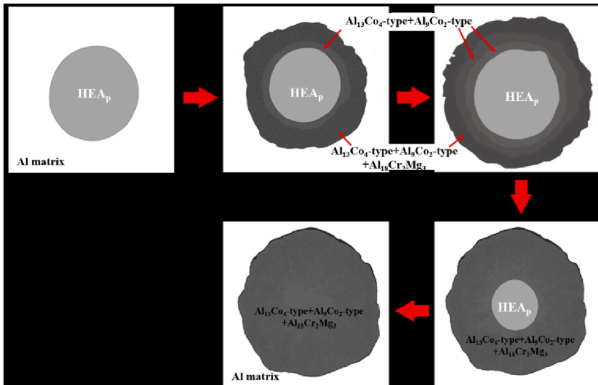
Fig. 4. Effect of annealing conditions on the composition and pattern of the interface diffusion layer region in Al/high entropy alloy particle (HEAp) composites [53] culled with permission from Elsevier.
