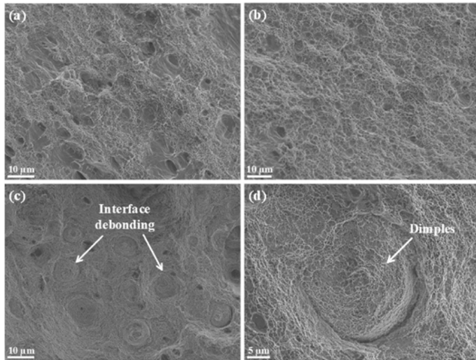
Fig. 9. Fracture surfaces of (a) Al-based matrix, (b) submerged friction stir processed 5083 Al, (c) and (d) submerged friction stir processed HEAp/5083 Al composites.
