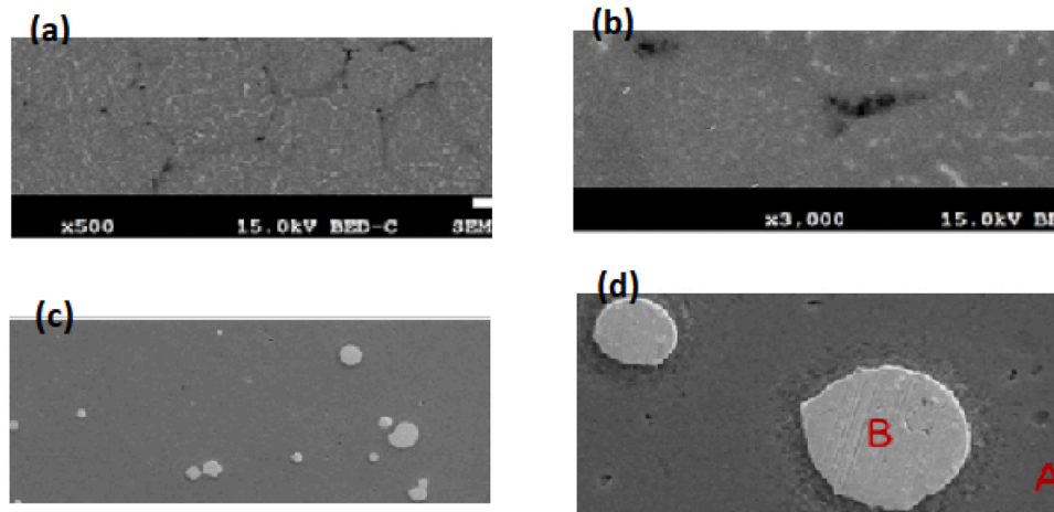
Fig. 2. Scanning electron micrographs showing (a) particle boundaries in the AZ91 metal matrix, (b) Mg precipitates in the AZ91 matrix, (c) the distribution of high entropy alloy particles in the AZ91-HEAp composites, and (d) the boundary of high entropy alloy particles in the AZ91 matrix [67] culled with permission from Elsevier.
