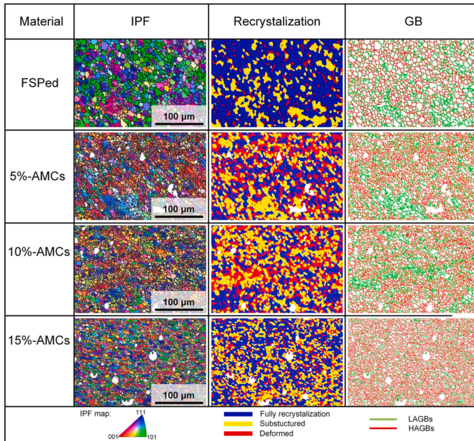
Fig. 11. Electron backscatter diffraction results of composites with different volume fractions (FSPed – underwater friction stir processed; GB – grain boundaries; HAGBs – high-angle grain boundaries; IPF – xxx; LAGBs – low-angle grain boundaries). [105] culled with permission from Elsevier.
