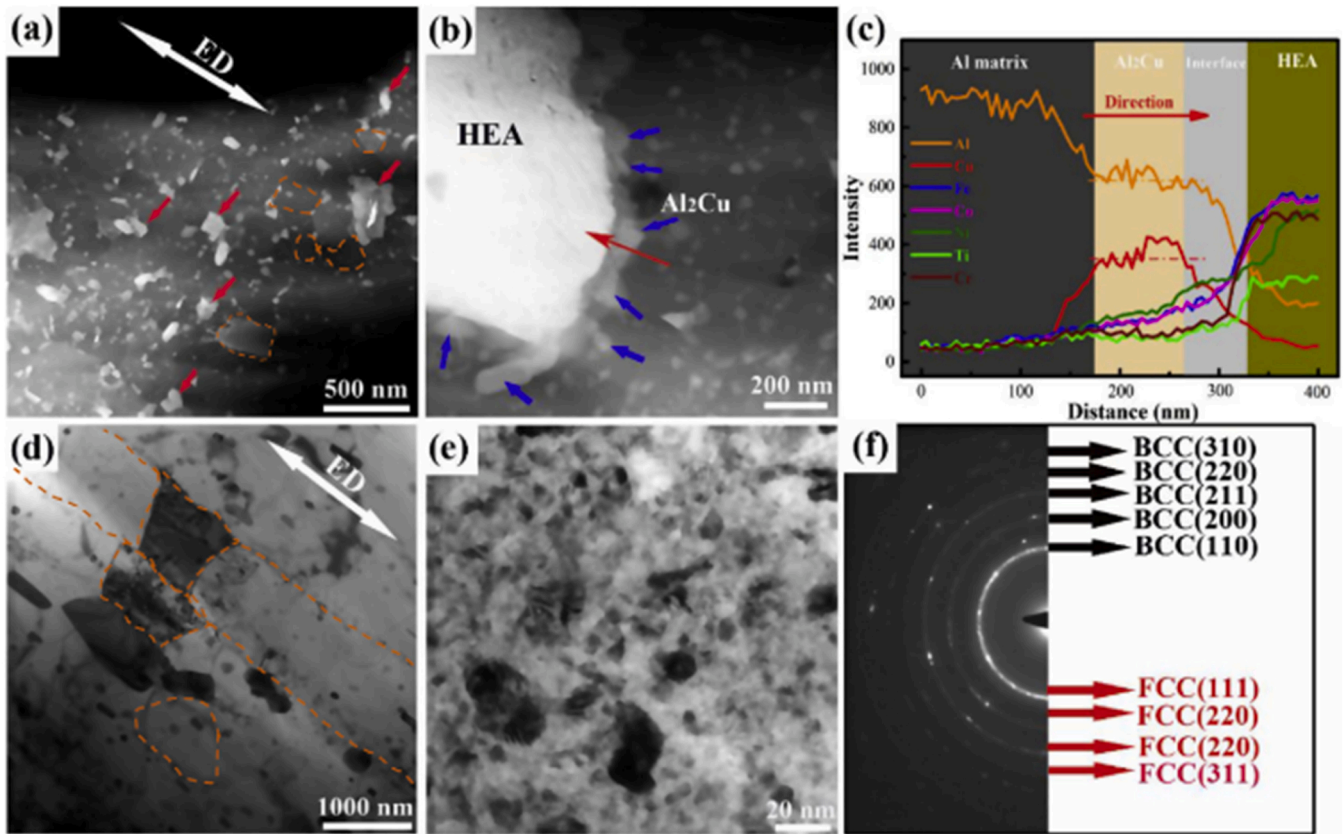
Fig. 6. (a) Dark-field transmission electron microscopy (TEM) image of the 7.5HEA-2024 Al sample, (b) the high entropy alloy particle (HEA)/2024 Al interface in the 7.5HEA-2024 Al sample, (c) linear scanning of HEA/2024 Al interface in (b), (d) the bright-field TEM image of the 2024 Al sample, (e) the grains of nano-crystalline-HEAs in the composite, (f) the selected area diffraction pattern corresponding to (e).
