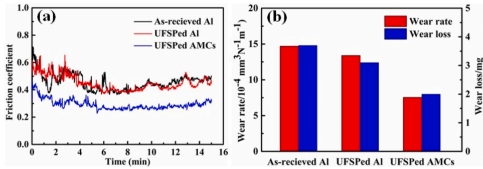
Fig. 15. Comparison of (a) the friction coefficient and (b) the wear rate and wear weight loss of as-received Al, underwater friction stir processed (UFSPed) Al and UFSPed Al matrix composites (AMCs).
