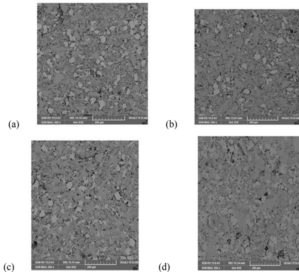
Fig. 14. Scanning electron micrographs of metal matrix composite (sample 5) heat treated at (a) 600 °C, (b) 700 °C, (c) 800 °C and (d) 900 °C. [64] culled with permission from Elsevier.
