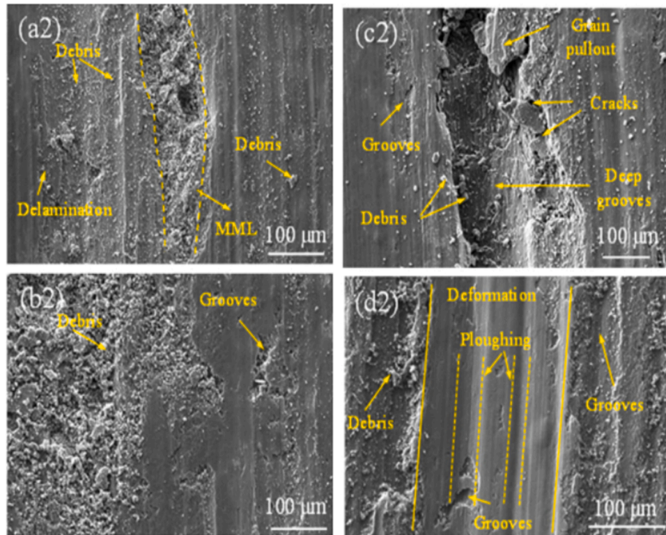
Fig. 16. Wear track topography for the different HEAs at a fixed applied load of 30 kN and sliding velocity of 70 mm/s for (a2) AA2219, (b2) 1.5 wt%, (c2) 3.0 wt% and (d2) 5.0 wt% high entropy alloy particle/Al matrix composites (MML – mechanically mixed layer).
