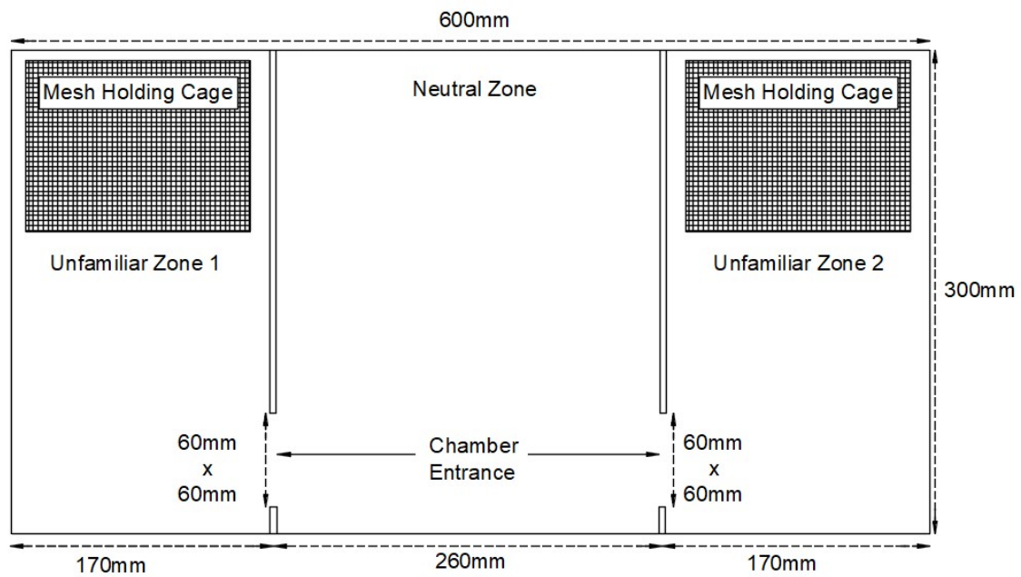
Figure 5.1. The three-chambered test apparatus as viewed from above, with dimensions. The unfamiliar zones are the test area/chambers that contained the stimulus mice within mesh holding cages. White tiles above holding cages are omitted from this image. Zones were divided by 3mm thick clear flexiglass barriers with breathing holes.
