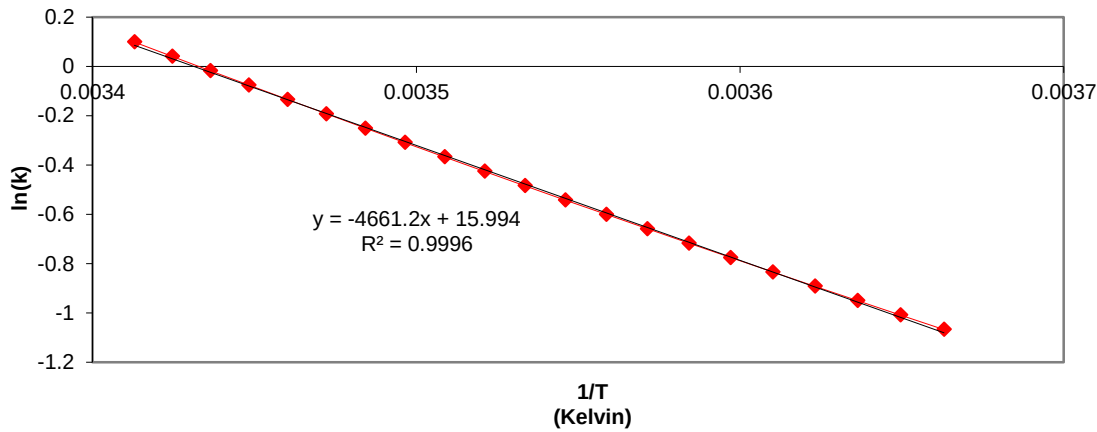
Figure 3.1. A graph of the MAF to find the parameters for the Arrhenius Equation with regressed line shown
