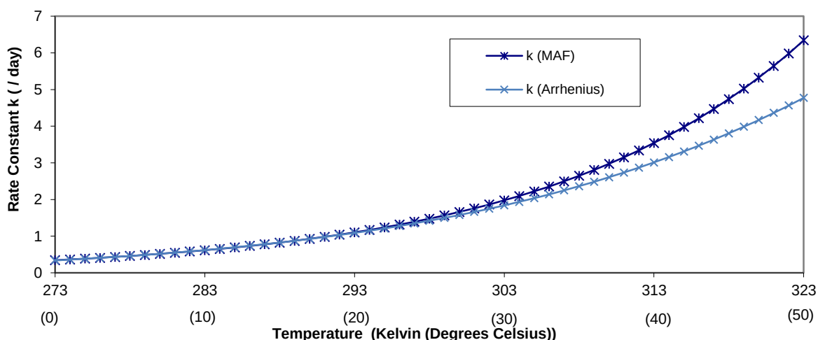
Figure 3.2. A comparison of the rate constants as calculated by the MAF and the Arrhenius equation showing differences at higher temperatures
