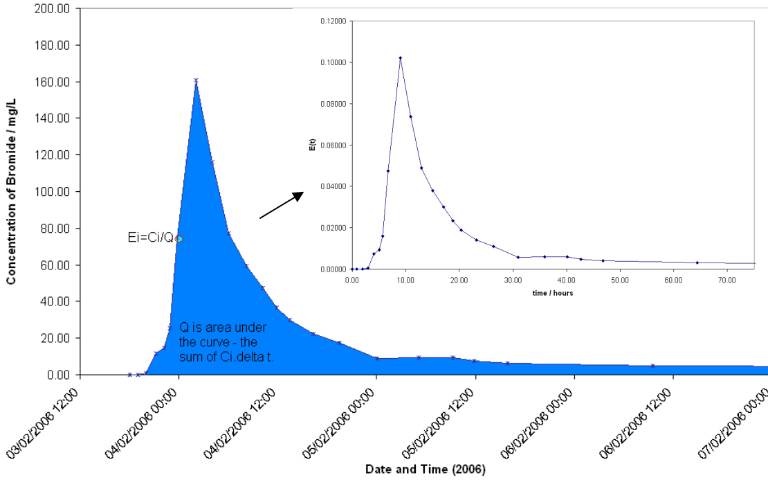
Figure 2.4. An example of a concentration vs. time plot [C(t) curve] and its age distribution [E(t) curve (inset)]
