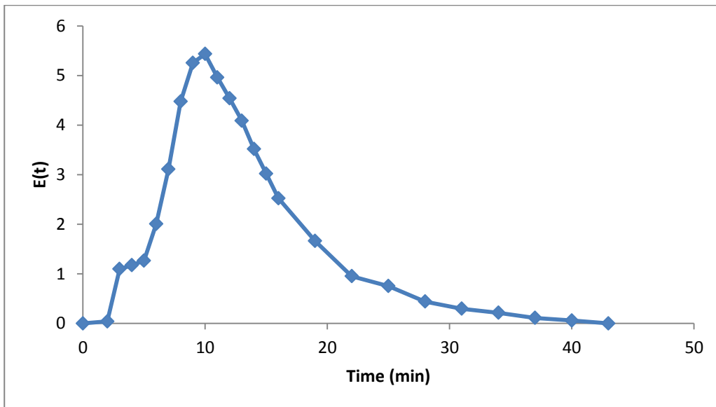
Figure 5.11. RTD for the impulse-response laboratory experiment with a well distributed feed and outlet.
