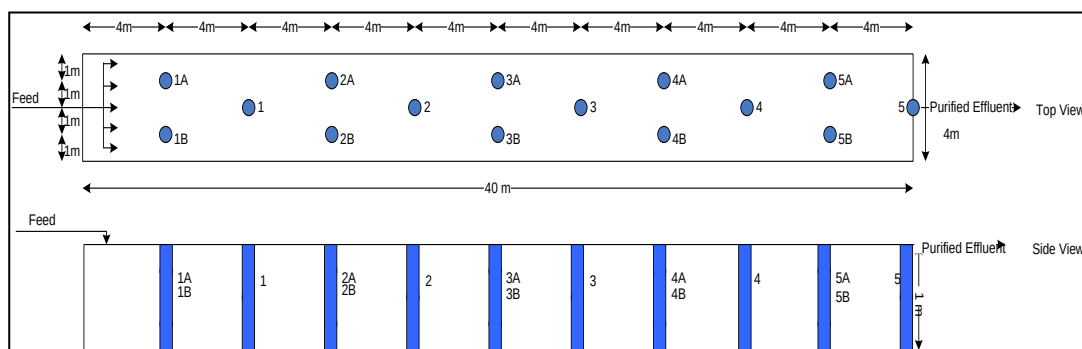
Figure 7.5. Schematic diagram of the VSR showing a side and a top view
