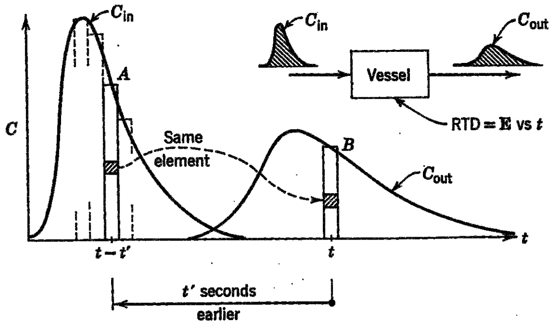
Figure 2.8. A graphical depiction of the movement of tracer through a reactor taken from Levenspiel
