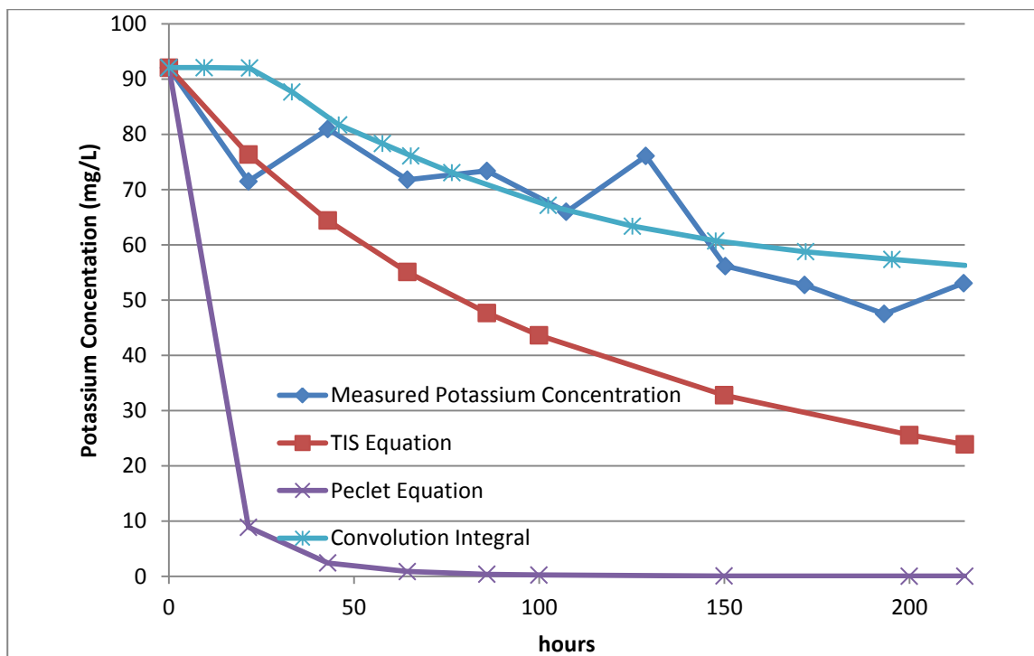
Figure 7.16. Base case for comparison of the three different rate constant calculations (Pe equation rate constant k=0.22/\text{hr} , TIS equation rate constant = 0.0049/\text{hr} and convolution integral k=0.037/\text{hr} )
