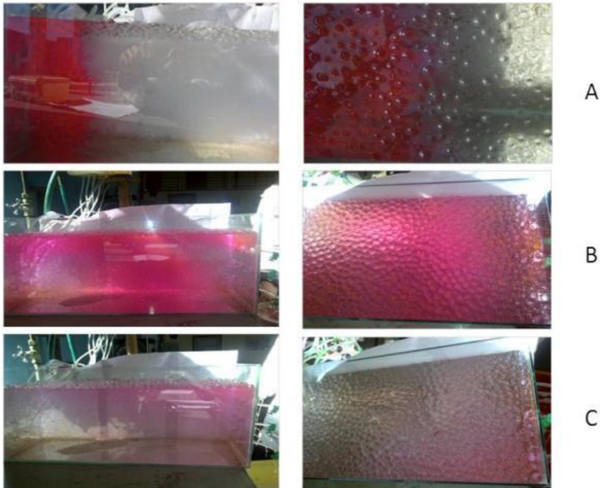
Figure 5.12. Photographs showing the flow patterns of tracer through the laboratory apparatus.
