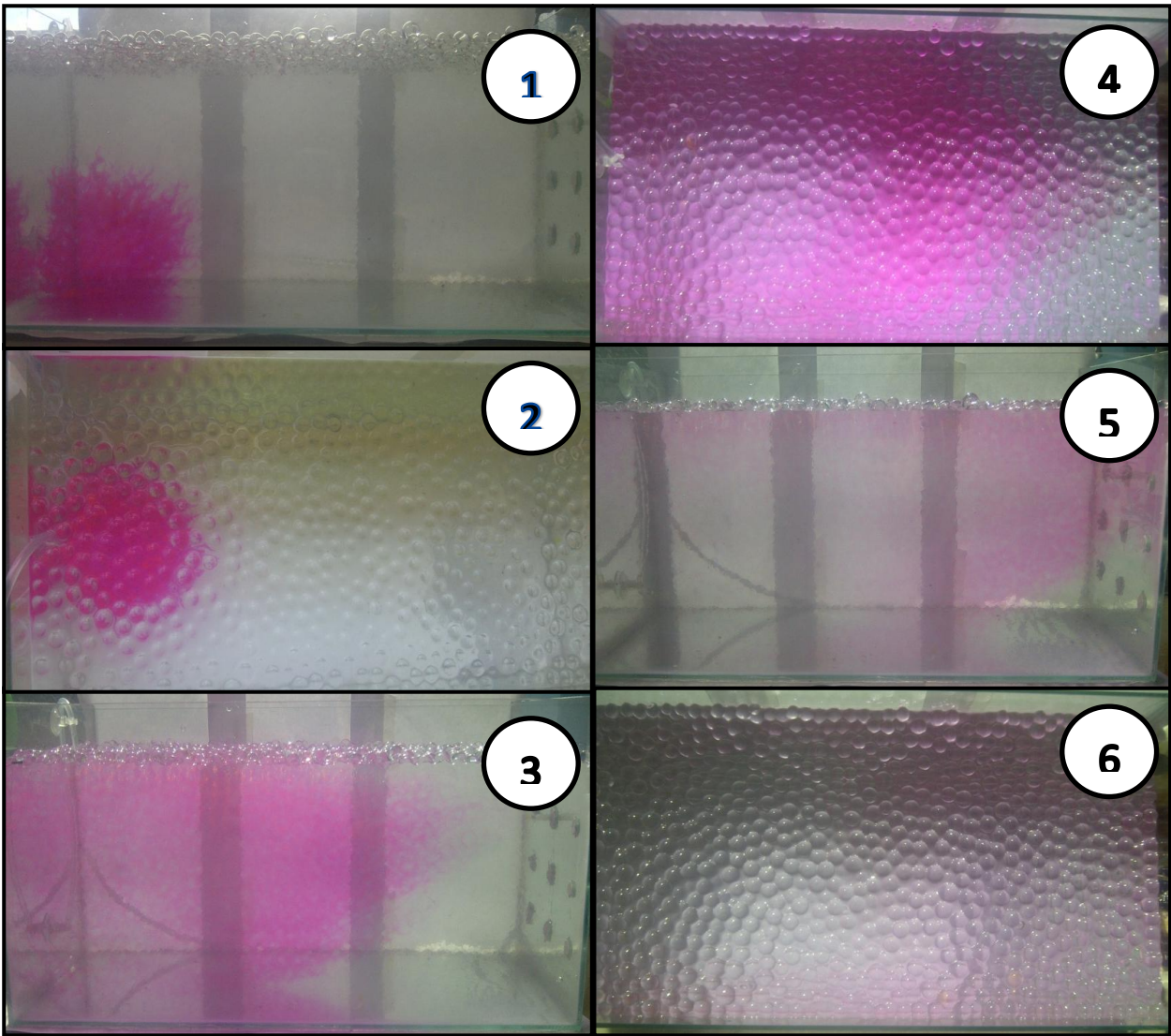
Figure 6.3. Experiment 2 - Connecting the inlet to the lowest central port and the outlet to the highest central port
