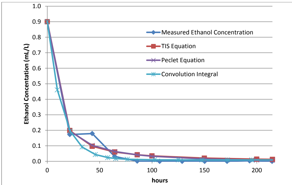
Figure 7.14. Optimised case for comparison of the three different rate constant calculations with Pe and N solved for minimum sum of squared errors (Pe equation rate constant k=7.85/\text{hr} , TIS equation rate constant = 0.088/\text{hr} and convolution integral k=0.804/\text{hr} ).
