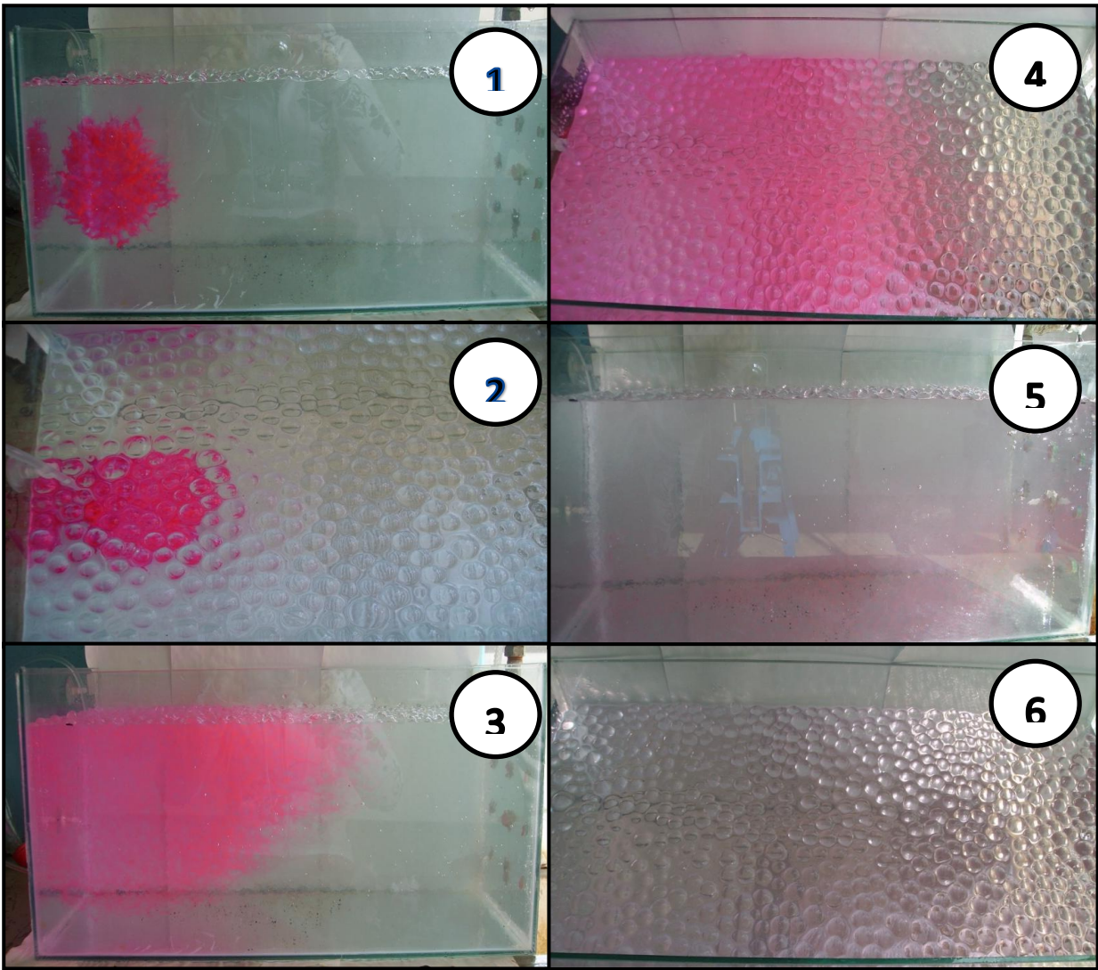
Figure 6.2. Experiment 1 - Connecting the inlet to the central inlet port and the outlet to the central outlet port
