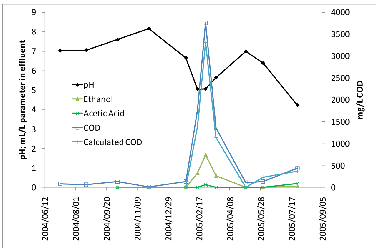
Figure 4.1. Organic components (ethanol and acetic acid) overlaid on pH and COD at Cellar 1
