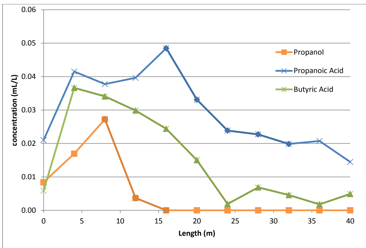
Figure 7.7. Average concentration of propanol, propanoic acid and butyric acid for the entire harvest with increasing duration of flow along the length of the CW
