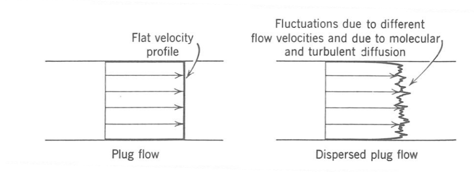
Figure 2.2. An example of increasing dispersion with increasing time/length in a reactor taken from Levenspiel (Levenspiel 1972)
