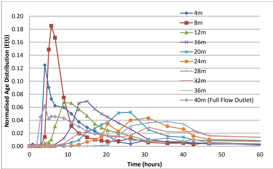
Figure 5.4. Normalised age distributions showing the progression and dispersion of the pulse as it moves through the VSR (with lateral variation averaged).
