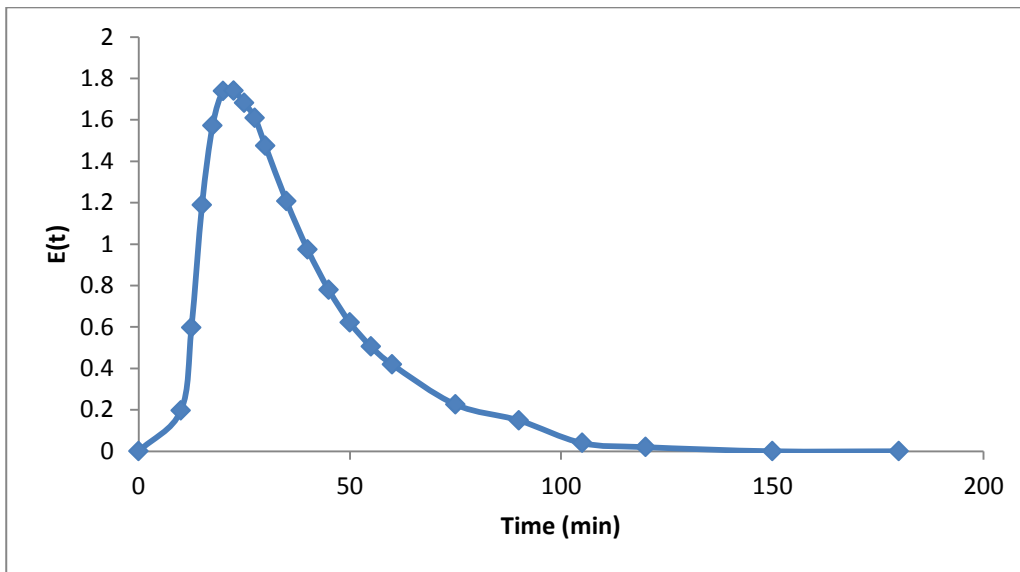
Figure 5.9. RTD for the impulse-response laboratory experiment.
