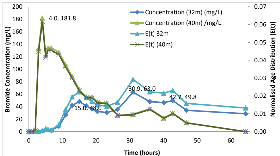
Figure 5.5. Residence time distributions for sample ports at 32m and 40m with multimodal distributions
