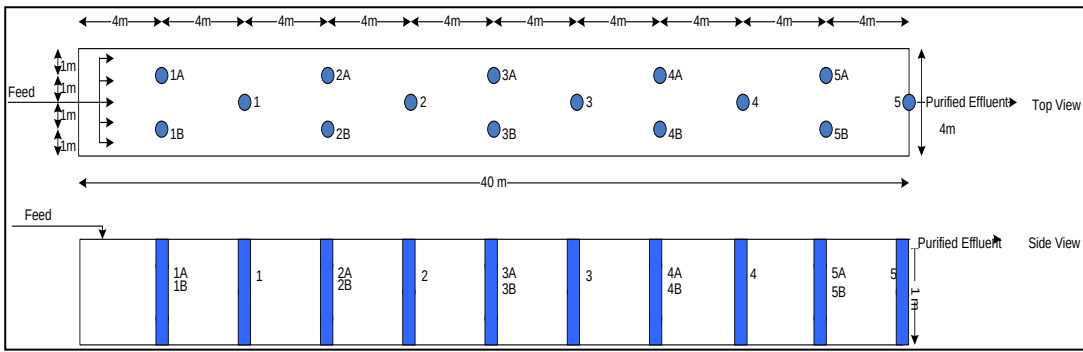
Figure 5.2. Schematic diagram of the VSR showing a side and a top view
