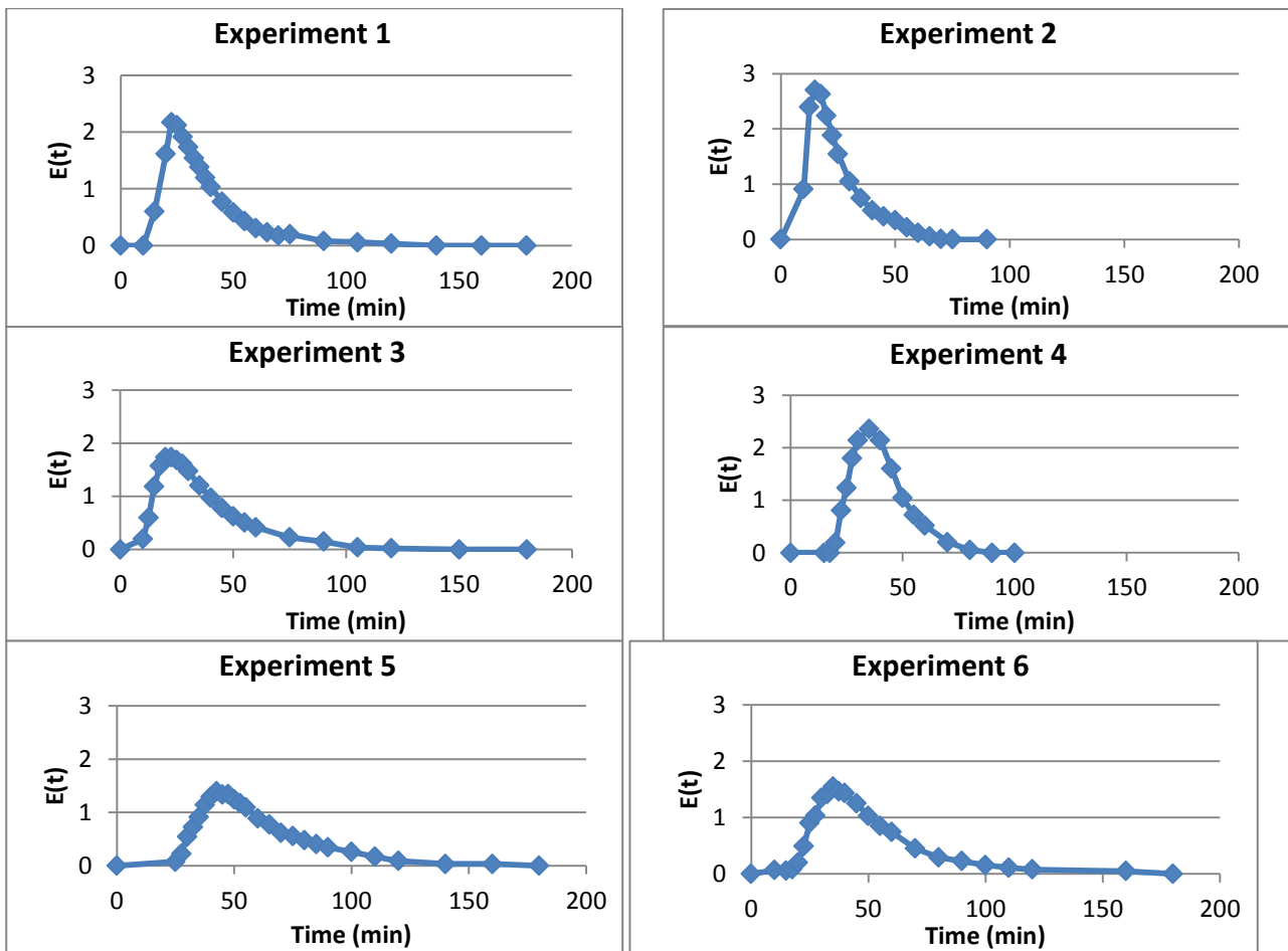
Figure 6.1. The residence time distributions of the six experiments. 1. Connecting the inlet to the central inlet port and the outlet to the central outlet port; 2. Connecting the inlet to the lowest central port and the outlet to the highest central port; 3. Connecting the inlet and outlet to the central highest ports; 4. Connecting the inlet to the central lowest port and the outlet to all three highest outlet ports; 5. Connecting the inlet to the right lowest port and the outlet to the right highest port; and 6. Inserting a wedge in the location of the dead zone identified.
