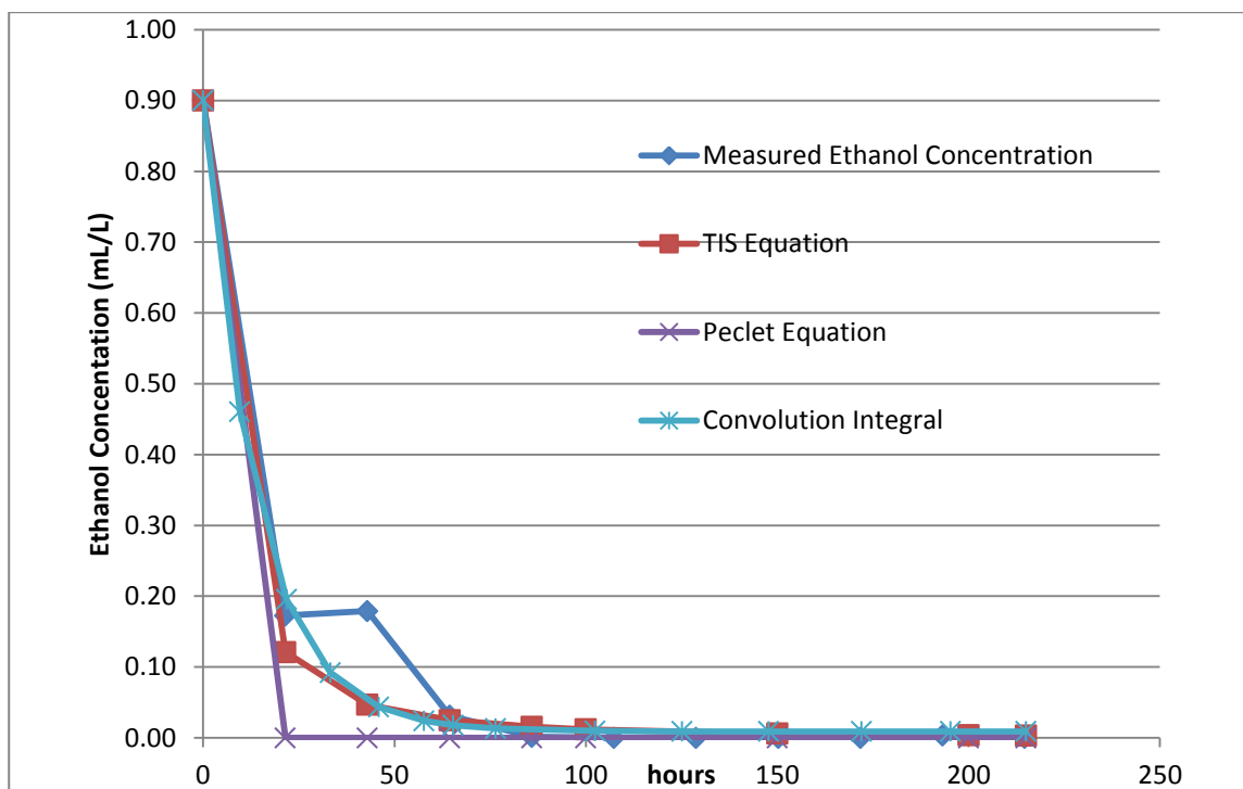
Figure 7.13. Base case for comparison of the three different rate constant calculations (Peclet equation rate constant k=7.85/\text{hr} , TIS equation rate constant = 0.088/\text{hr} and convolution integral k=0.804/\text{hr} )
