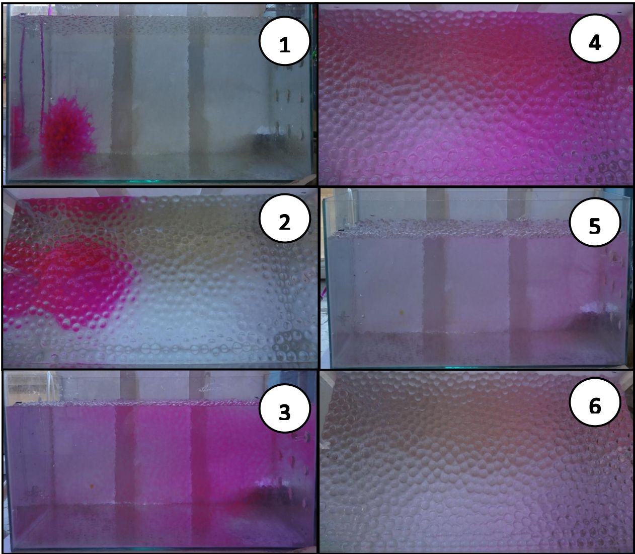
Figure 6.5. Experiment 4 - Connecting the inlet to the central lowest port and the outlet to all three highest outlet ports
