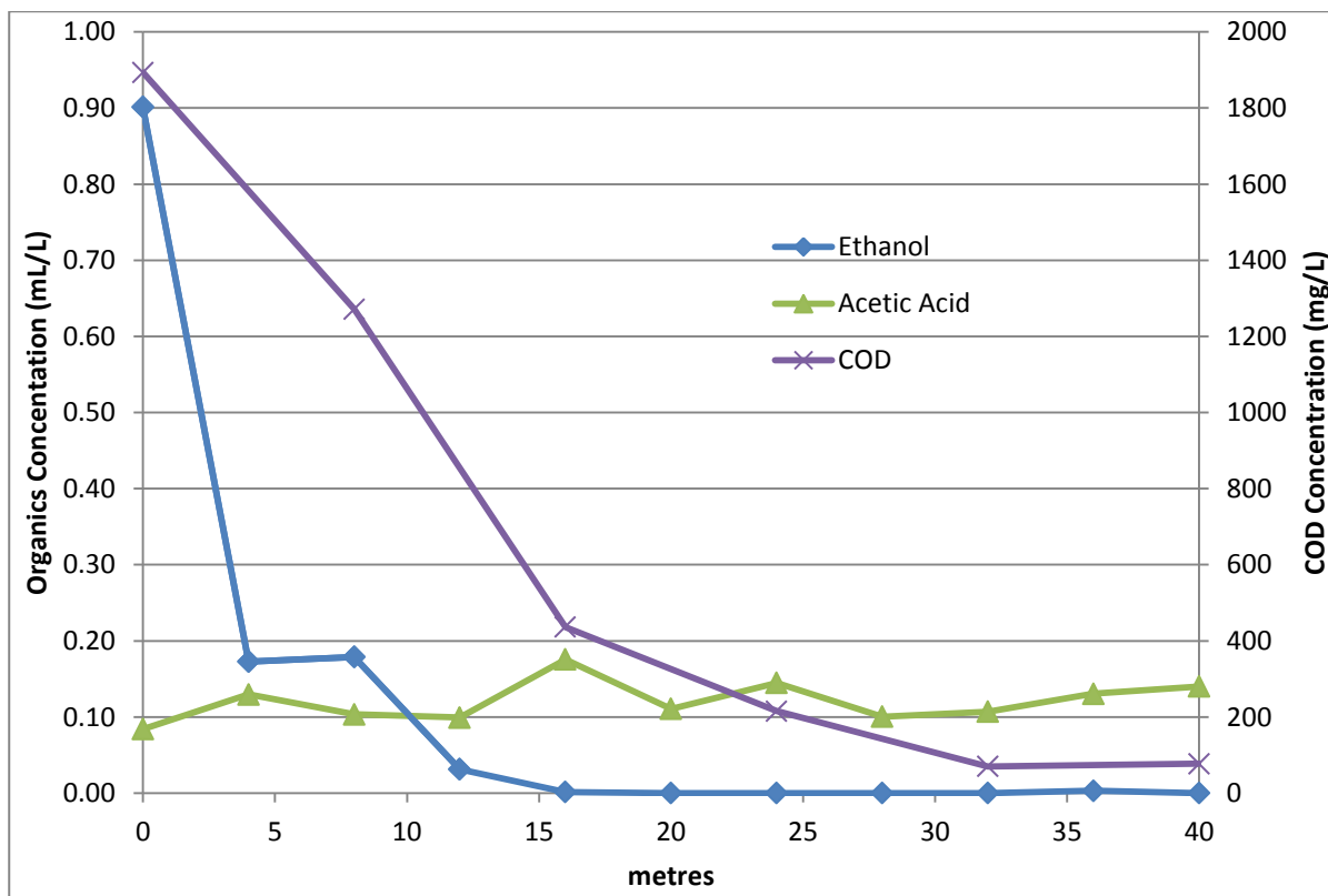
Figure 7.8. Average major organic components and COD concentration for the entire harvest at various locations along the length of the CW
