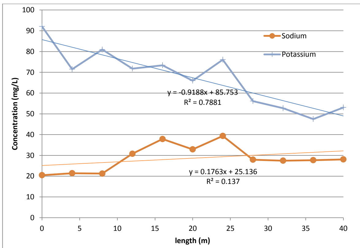
Figure 7.9. Average changes in concentration of sodium and potassium for the entire harvest as it travels along the CW
