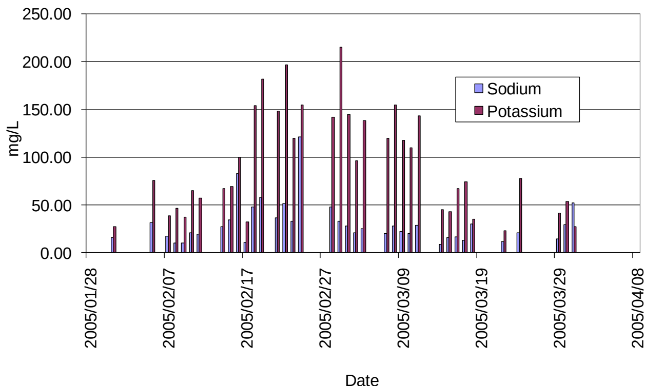
Figure 4.4. Cationic components in winery effluent measured over a harvest season at Cellar 2
