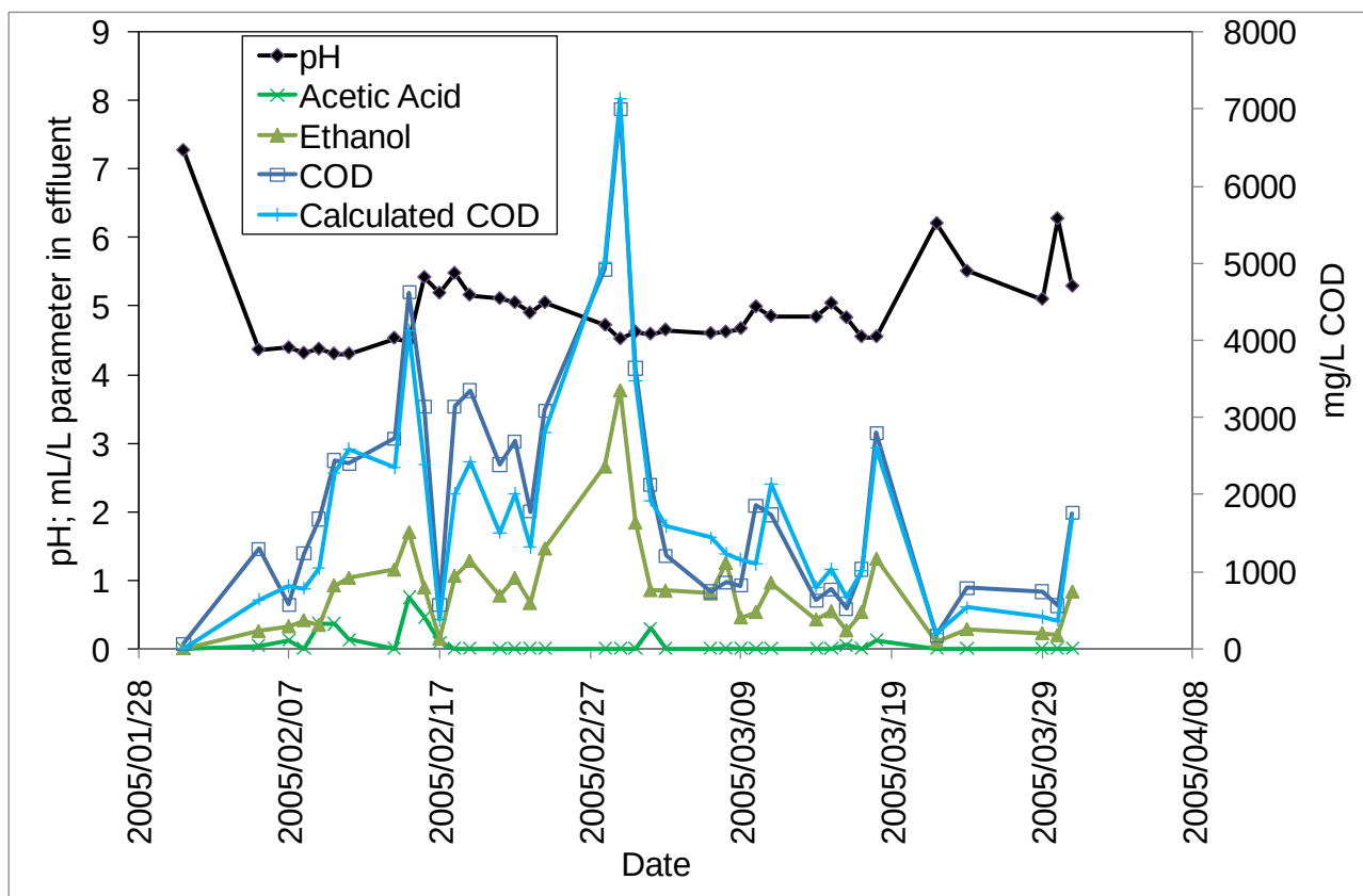
Figure 4.3. Organic components (ethanol and acetic acid) overlaid on pH and COD at Cellar 2
