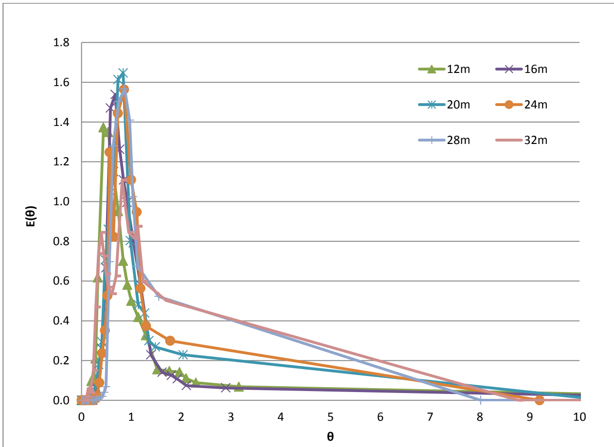
Figure 7.11. Normalised age distributions for the middle sections of the CW
