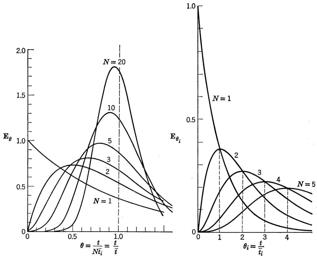
Figure 2.5. Residence time distributions for N CSTR reactors in series taken from Levenspiel
