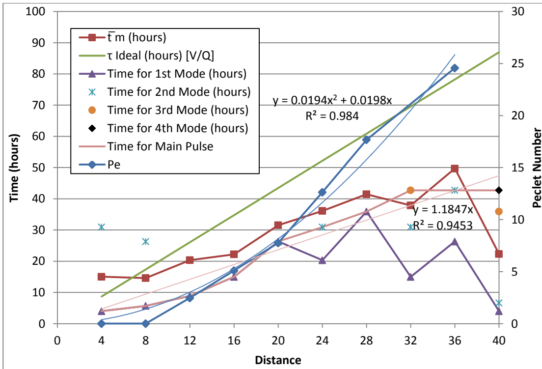
Figure 5.6. An analysis of the modes of distribution for the VSR
