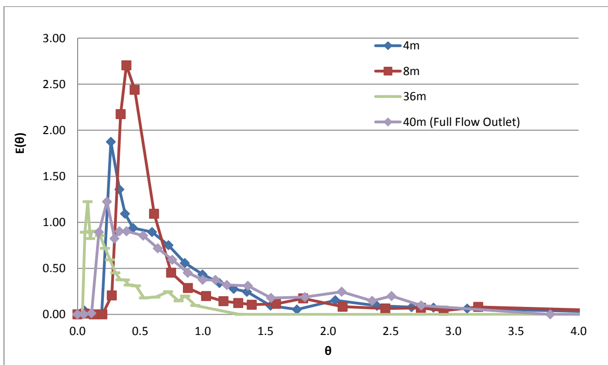
Figure 7.12. Normalised age distributions for the initial and final sections of the CW
