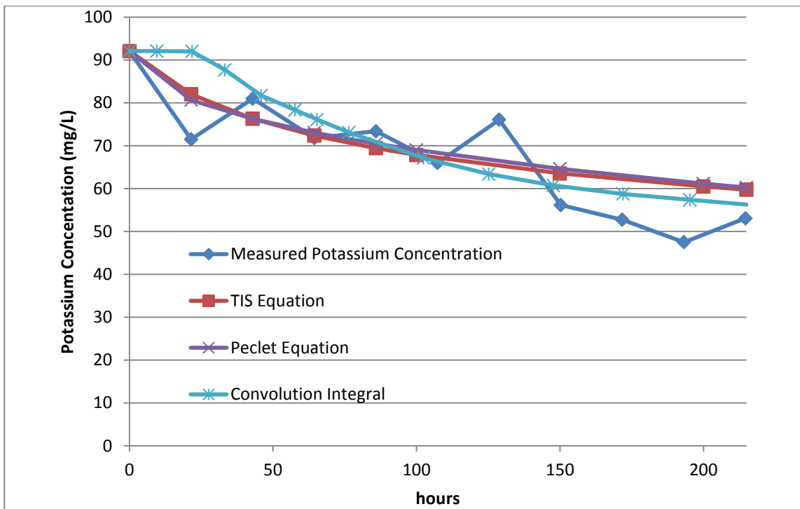
Figure 7.18. Second optimised case for comparison of the three different rate constant calculations with Pe and N solved for minimum sum of squared errors, using the rate constant found with the convolution integral method ( k=0.0374/\text{hr} ).
