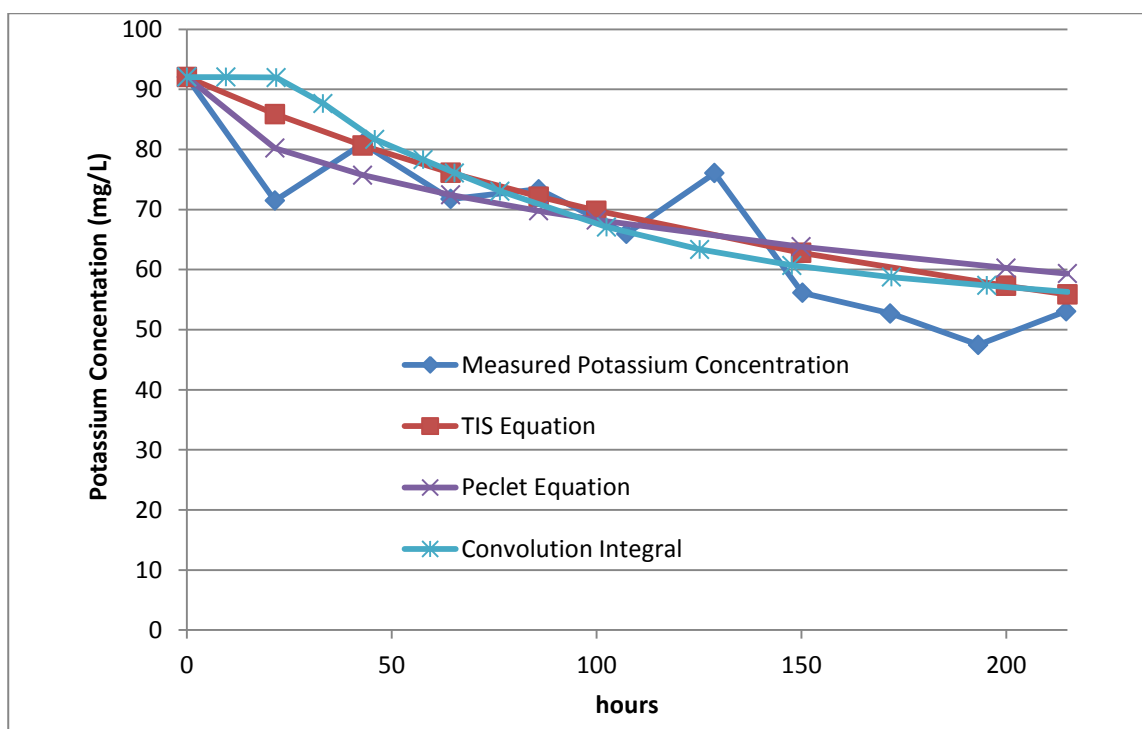
Figure 7.17. Optimised case for comparison of the three different rate constant calculations with Pe and N solved for minimum sum of squared errors (Pe equation rate constant k=0.22/\text{hr} , TIS equation rate constant = 0.0049/\text{hr} and convolution integral k=0.037/\text{hr} ).
