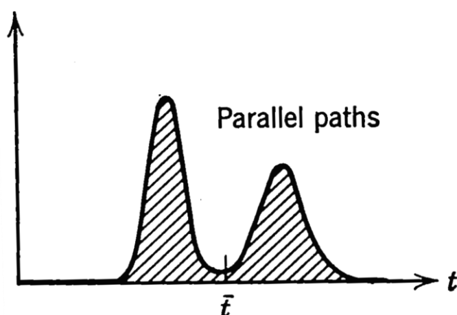
Figure 2.3. An example taken from Levenspiel indicating that tracer may follow two parallel (independent) paths within a reactor.
