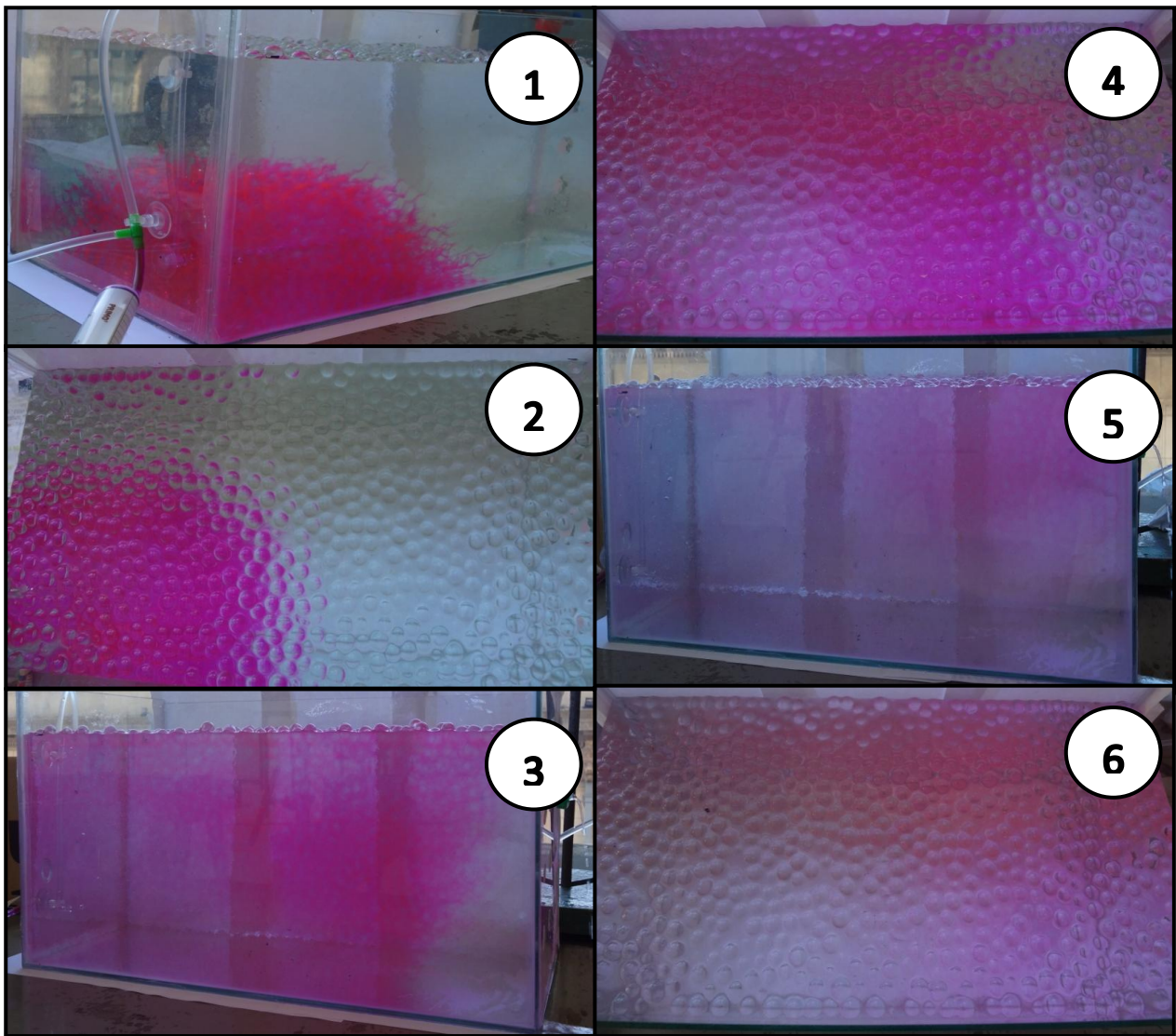
Figure 6.6. Experiment 5 - Connecting the inlet to the right lowest port and the outlet to the left highest port
