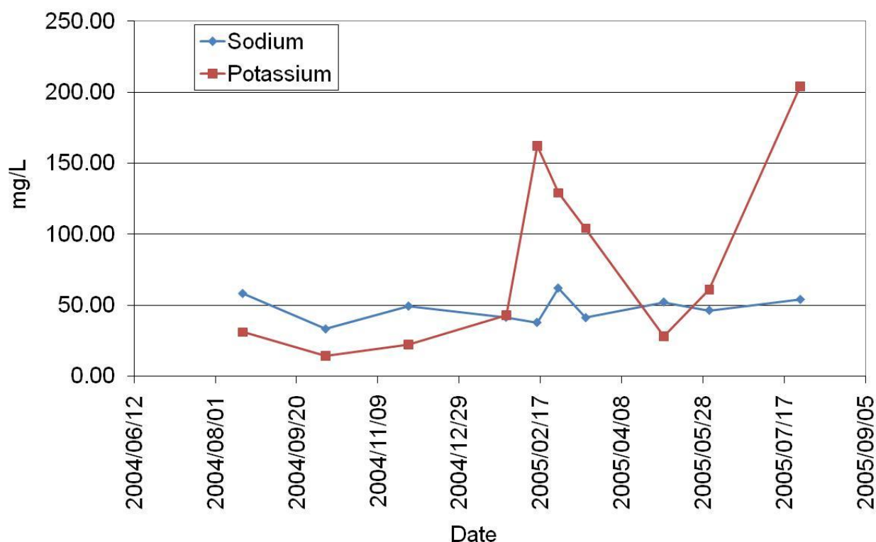
Figure 4.2. Cationic components in winery effluent measured over a year at Cellar 1
