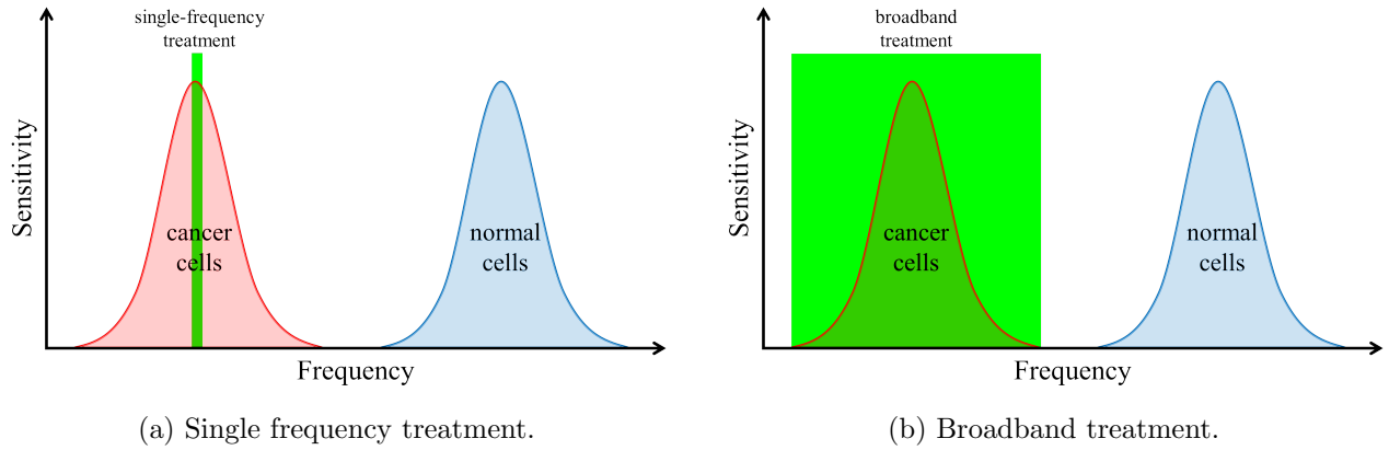
Figure 1.2.2: Treatment of the cancerous cell population.
