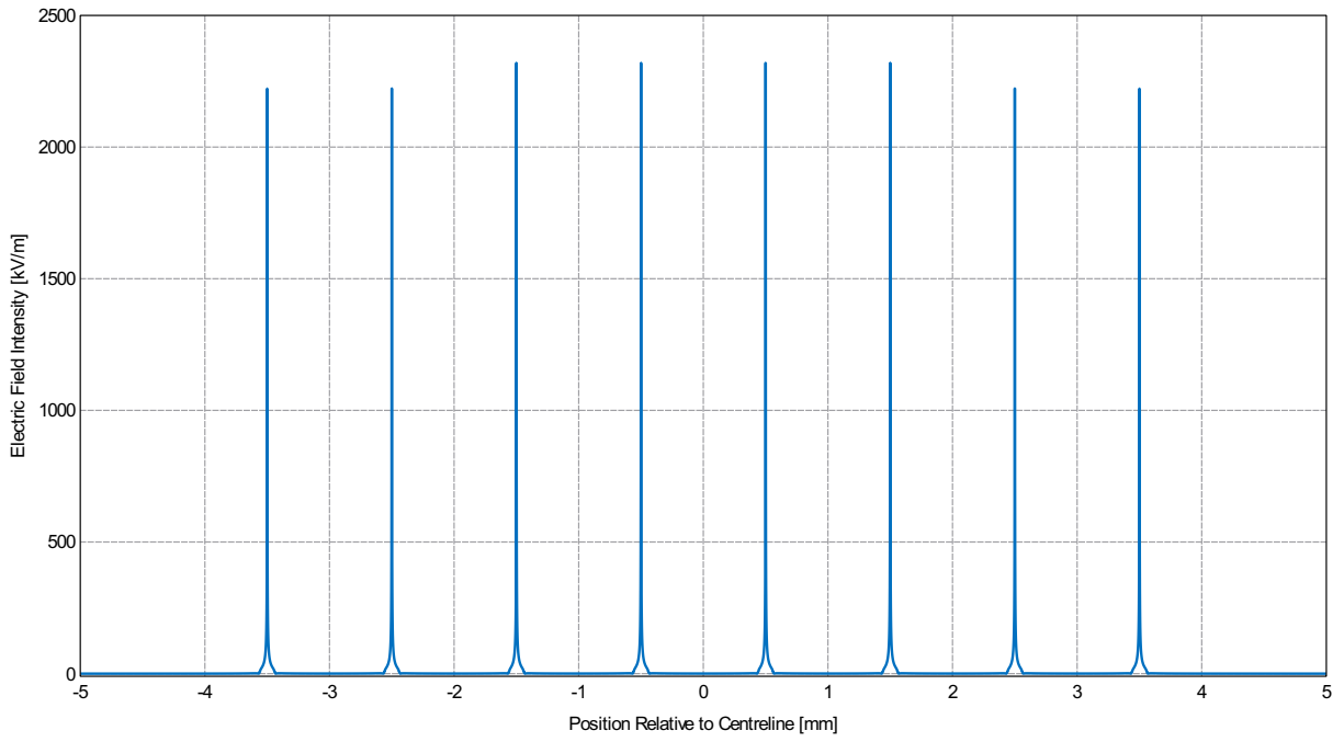
Figure 5.2.4: Simulation results for four pairs of insulated wires in culture medium.
