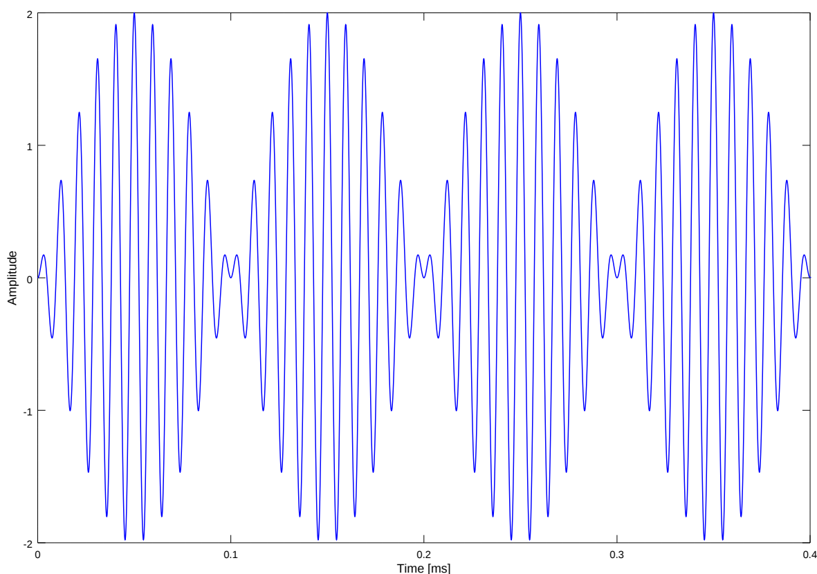
Figure 2.2.2: Superposition of two closely-spaced sinusoids (initially out-of-phase).
