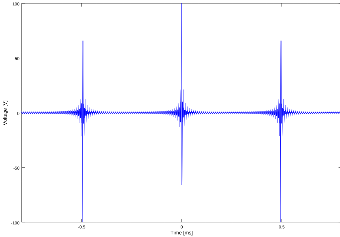
Figure 2.2.3: Summation of 100 sinusoids (all in-phase at t = 0 ).
