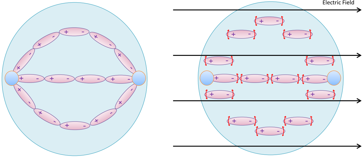
Figure 2.1.2: Alignment of tubulin subunits in an electric field.
