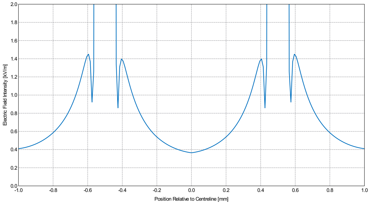
Figure 5.2.6: Simulation results for four pairs of insulated wires in culture medium (axes further adapted).
