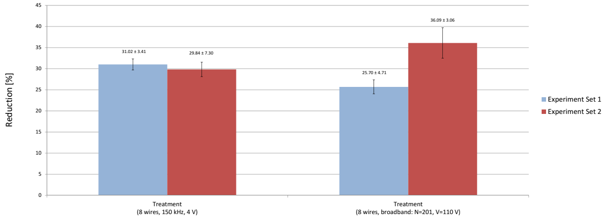
Figure 7.2.5: Reduction of the dye in the test comparing the efficacies of single-frequency treatment and broadband treatment. The experiment sets display opposite trends with Experiment Set 2 showing an increase in reduction for the broadband treatment.
