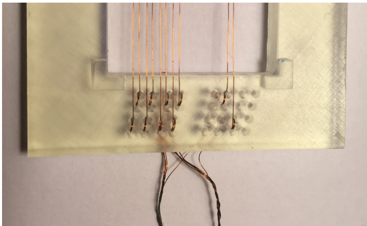
Figure 6.1.3: Threaded wires for a 8-wire set-up (left) and a 2-wire set-up (right).
