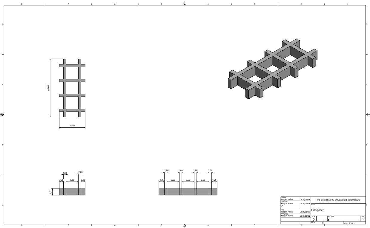
Figure 4.2.4: Lid Spacer.
