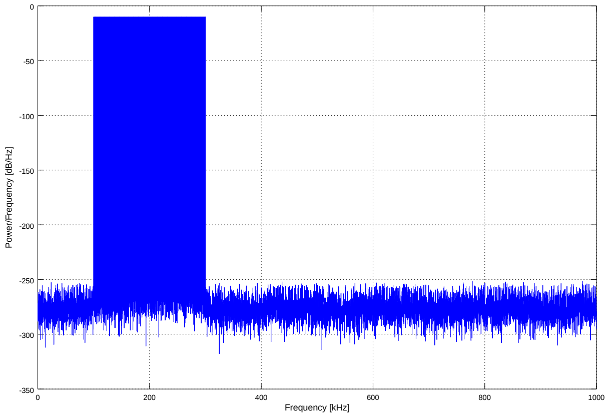
Figure 6.1.8: Power spectral density of the broadband signal.
