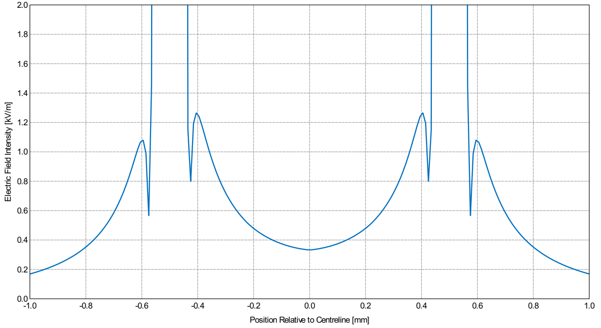
Figure 5.2.3: Simulation results for a single pair of insulated wires in culture medium (axes further adapted).
