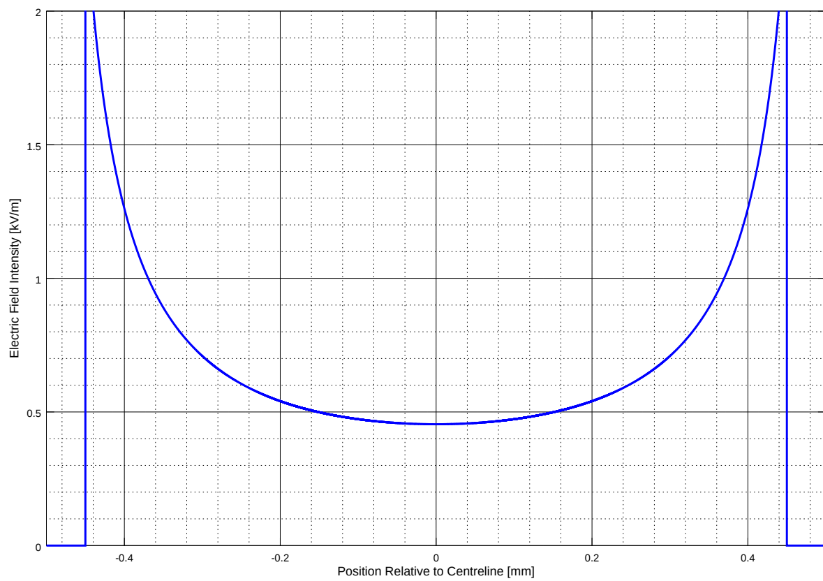
Figure 5.3.2: Analytical predictions for the electric field intensity (axes adapted).
