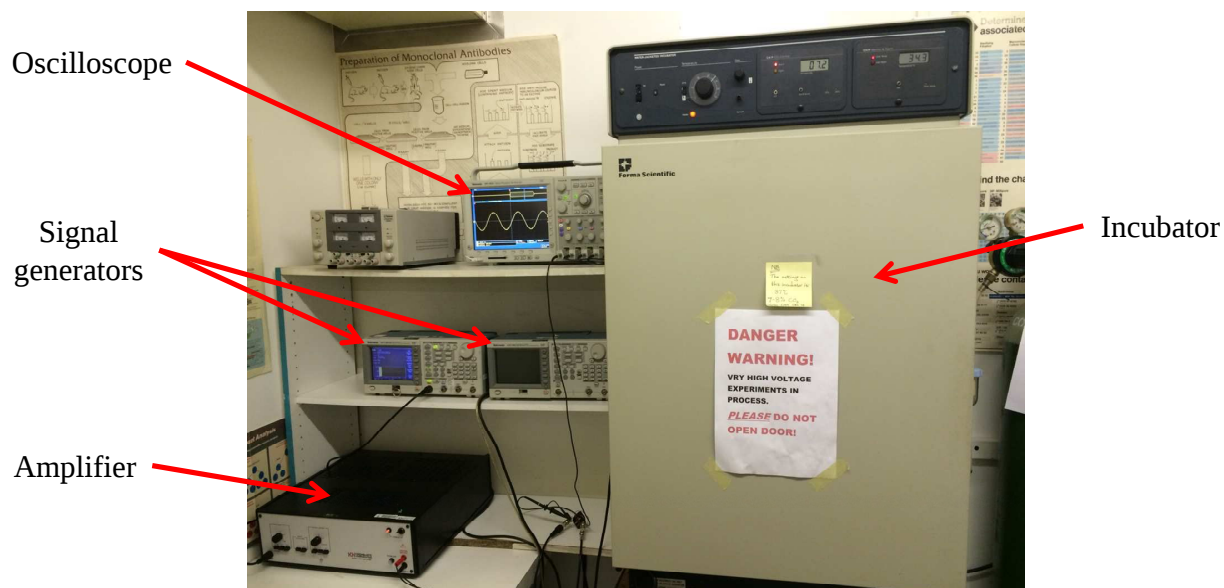
Figure 6.2.1: Laboratory set-up.
