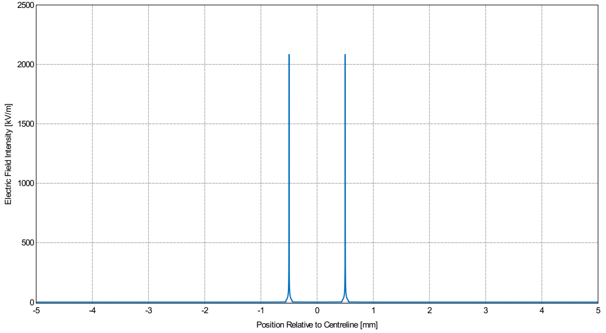
Figure 5.2.1: Simulation results for a single pair of insulated wires in culture medium.
