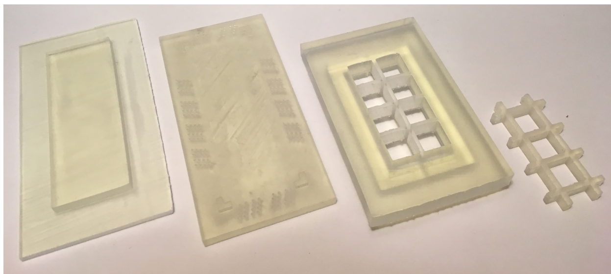
Figure 6.1.1: 3D-printed parts. From left to right: Slide Platform, Wire Guider, Clamp Brace and Lid Spacer.
