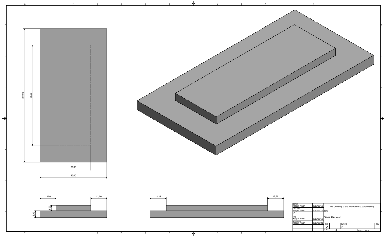
Figure 4.2.2: Slide Platform.
