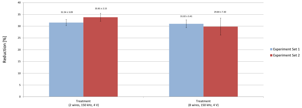
Figure 7.2.3: Reduction of the dye in the test comparing the efficacies of treatment using 2 wires and 8 wires, where Experiment Set 1 shows very similar reductions but Experiment Set 2 shows a lowered reduction for the 8-wire treatment.
