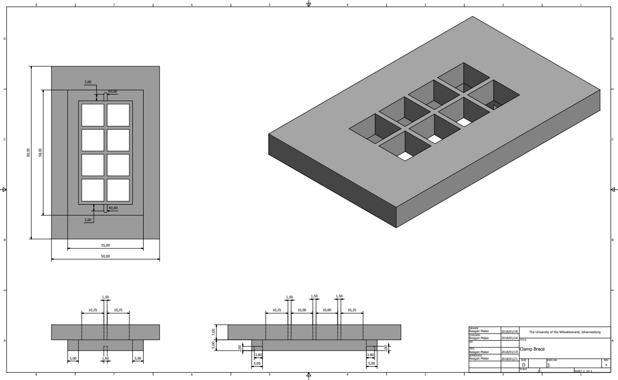
Figure 4.2.3: Clamp Brace.
