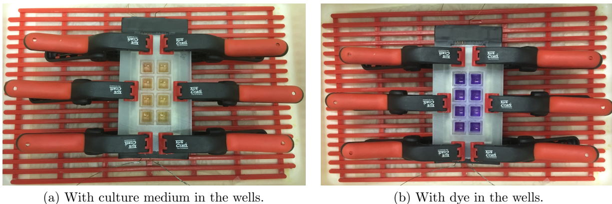
Figure 6.3.1: Sealed assembly.
