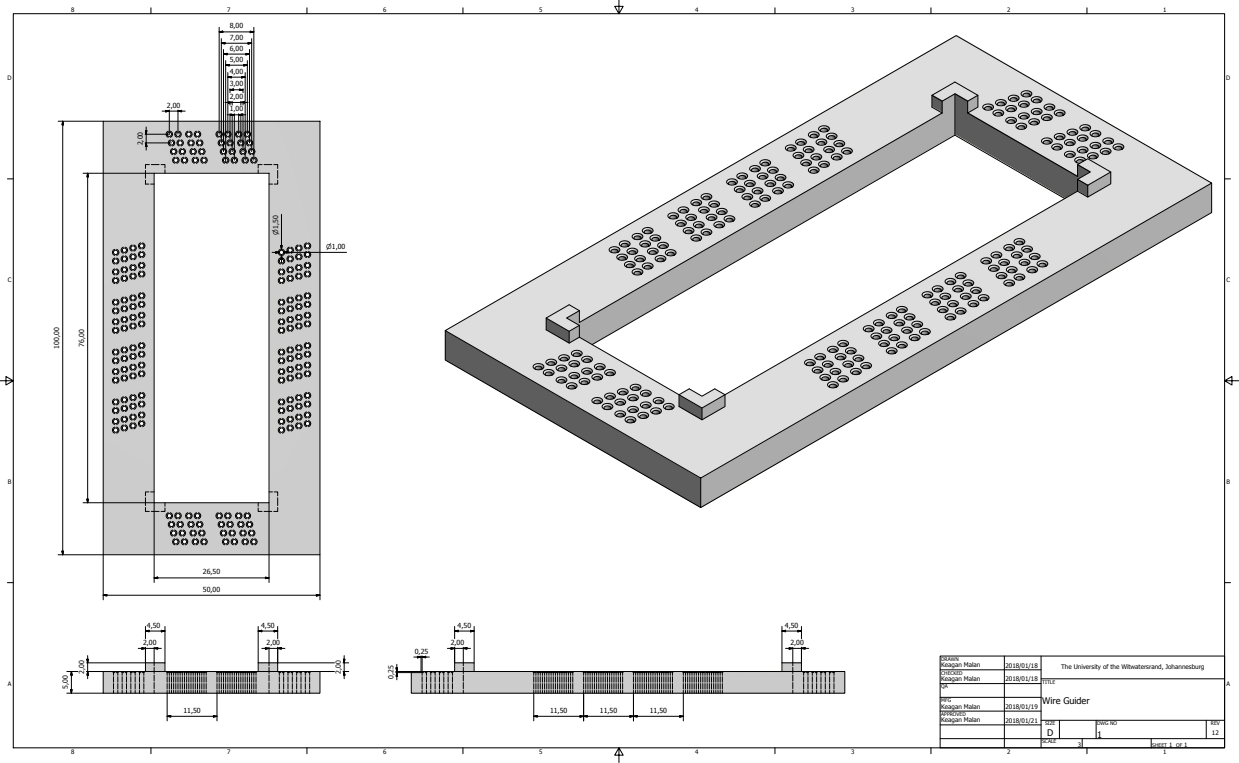
Figure 4.2.1: Wire Guider.
