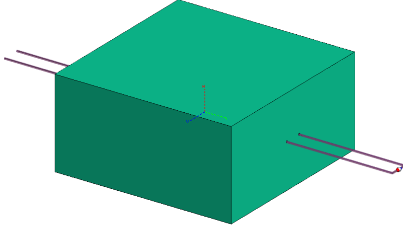
Figure 5.1.1: Geometry used for the 2-wire simulations.
