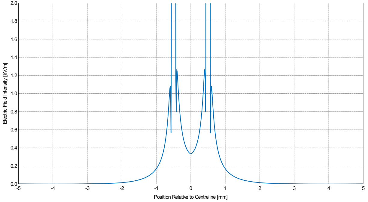
Figure 5.2.2: Simulation results for a single pair of insulated wires in culture medium (axes adapted).
