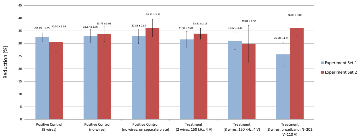
Figure 7.3.1: Percent reduction data showing large uncertainties in both experiment sets.
