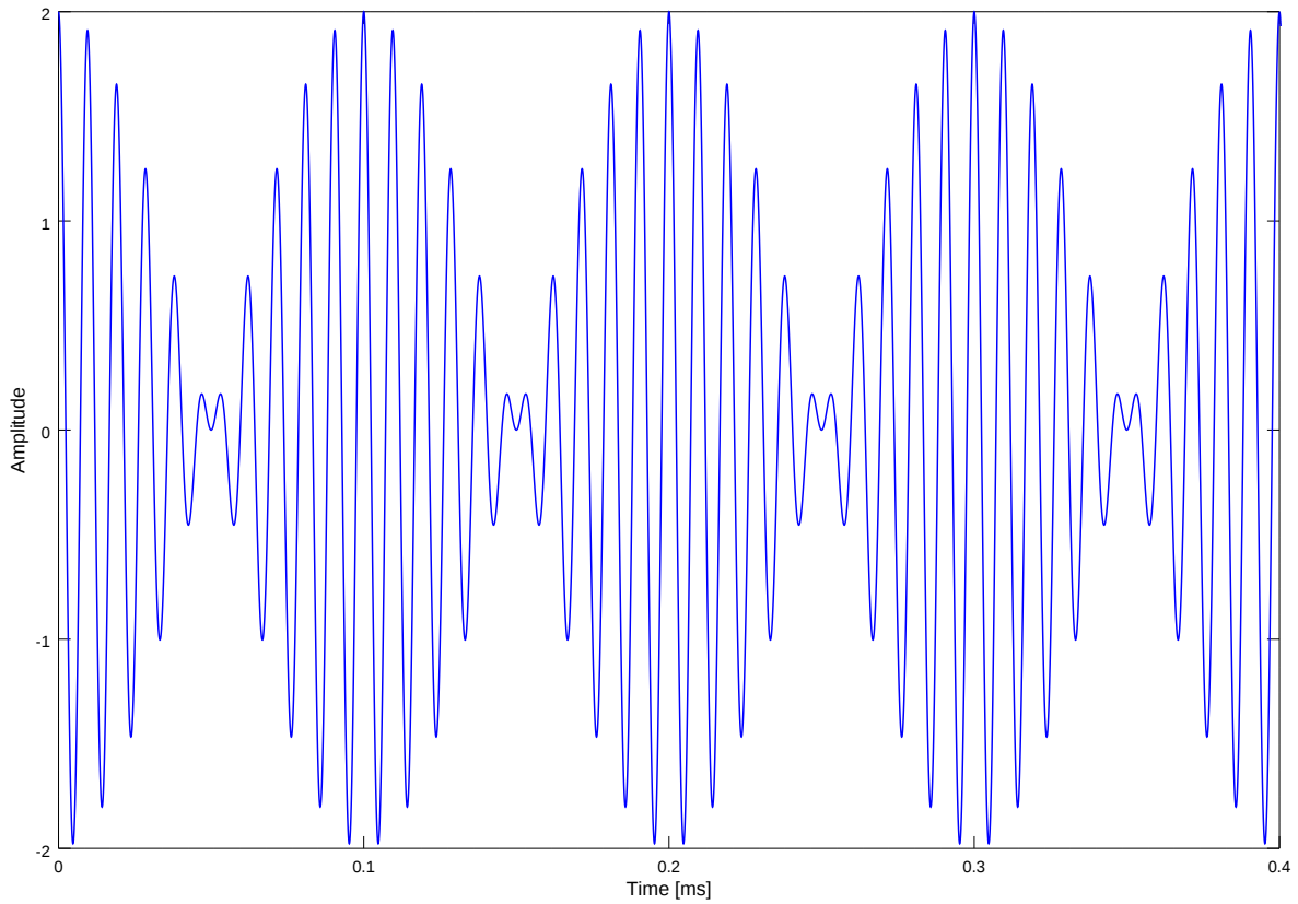
Figure 2.2.1: Superposition of two closely-spaced sinusoids (initially in-phase).
