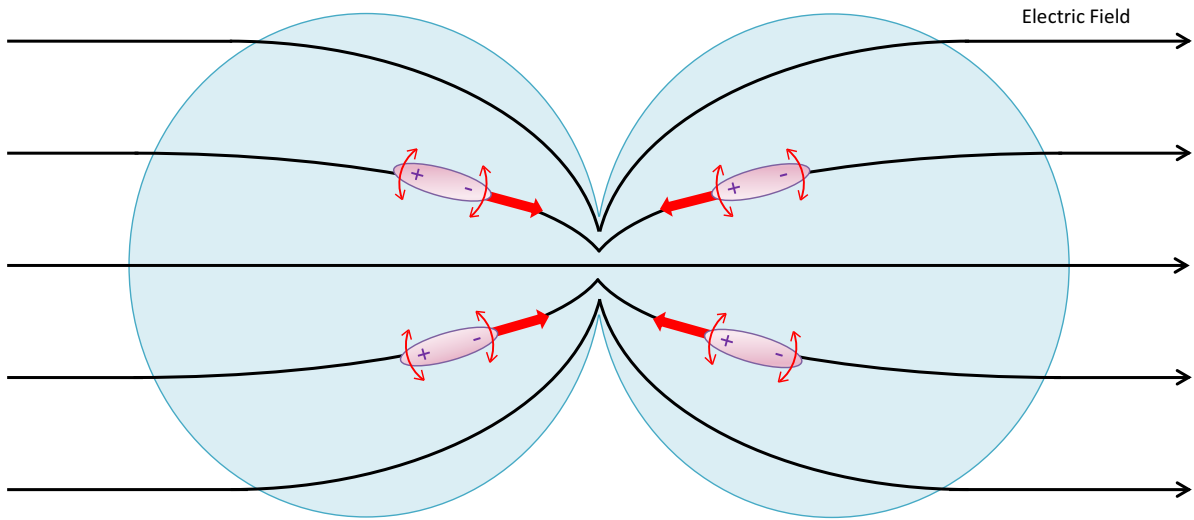
Figure 2.1.3: Converging of tubulin subunits towards a higher electric field density.
