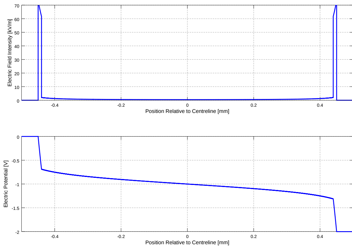
Figure 5.3.1: Analytical predictions for electric field intensity and electric potential.
