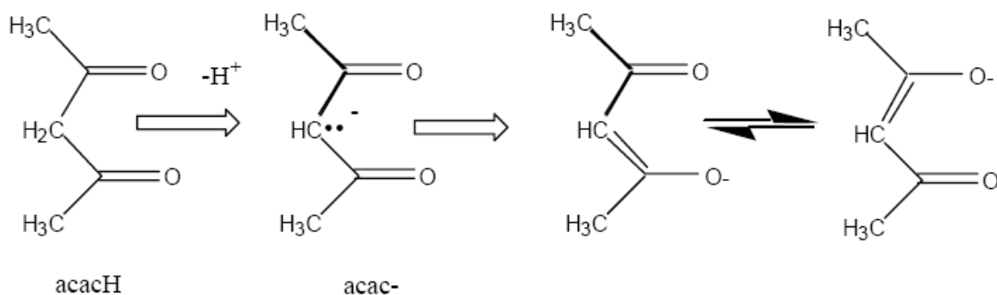
Figure 2-2 The inter-conversion between the keto and enolic form of the acac anion
