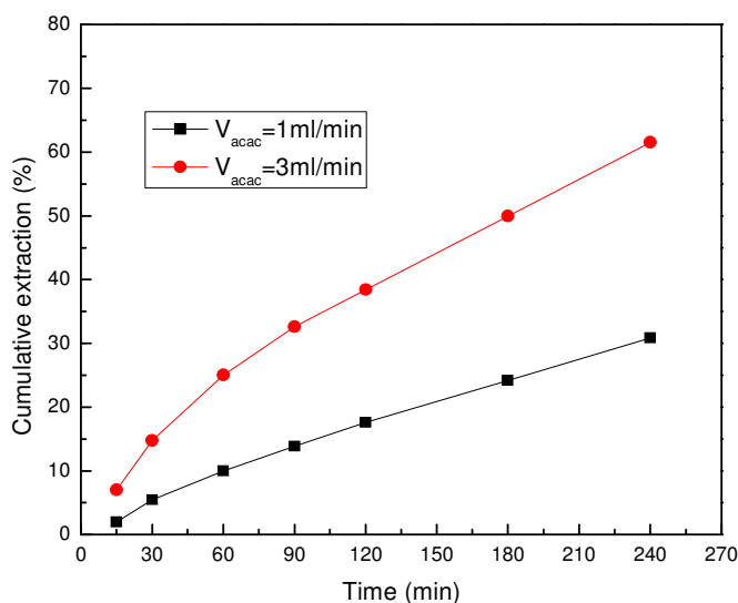
Figure 4-5 Effect of ligand flow rate on extraction for a 10wt% mixture at 250°C
