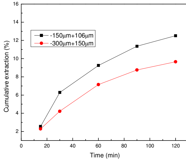
Figure 4-9 Effect of particle size on extraction at 3ml/min on a 3wt% mixture at 210°C
