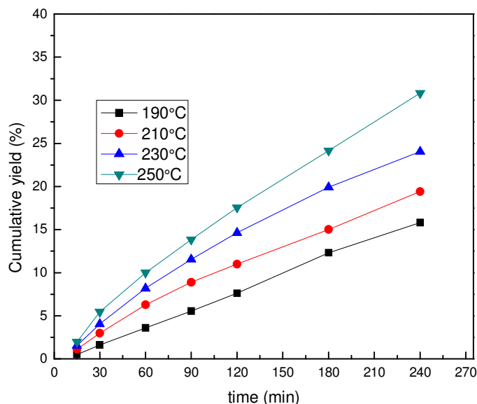
Figure 4-3 Effect of temperature on extraction for a 10wt% \text{Fe}_2\text{O}_3 mixture
