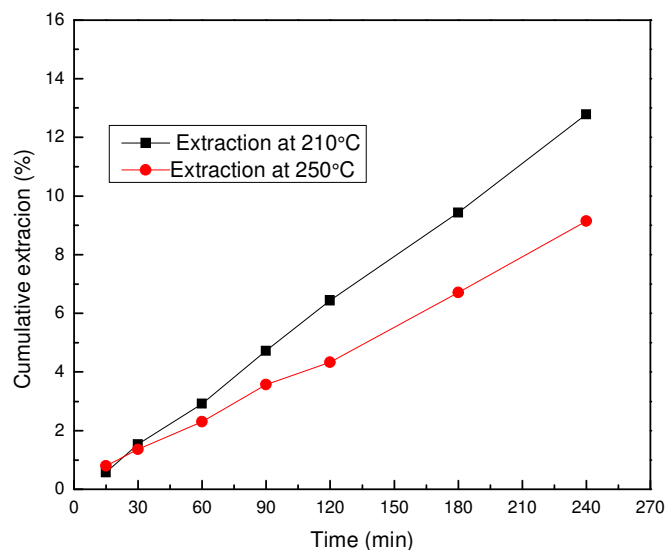
Figure 4-10 Extraction from a mixture containing 3wt% \text{Cr}_2\text{O}_3 at 3ml/min
