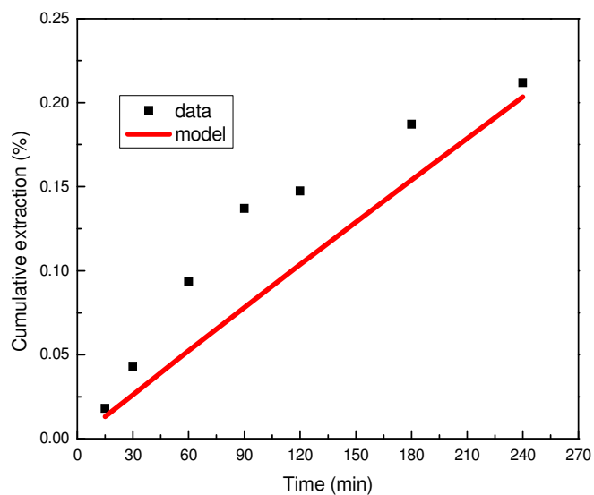
Figure 5-6 Comparison of conversion predicted by gas film diffusion control model with actual data obtained at 190°C
