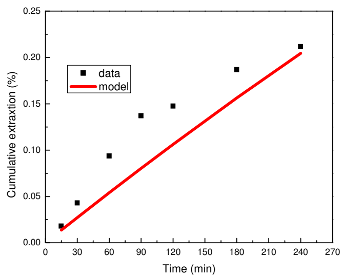
Figure 5-1 Comparison of conversion predicted by chemical reaction control model with actual data obtained at 190°C
