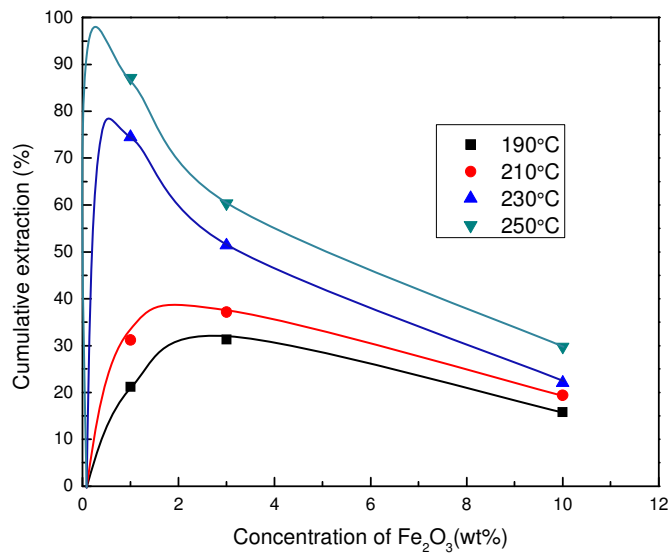
Figure 4-7 Effect of metal oxide concentration on extraction at 1ml/min flow rate after 4hrs
