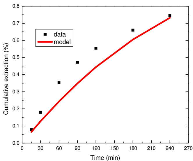
Figure 5-3 Comparison of conversion predicted by chemical reaction control model with actual data obtained at 230°C
