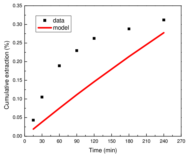
Figure 5-2 Comparison of conversion predicted by chemical reaction control model with actual data obtained at 210°C
