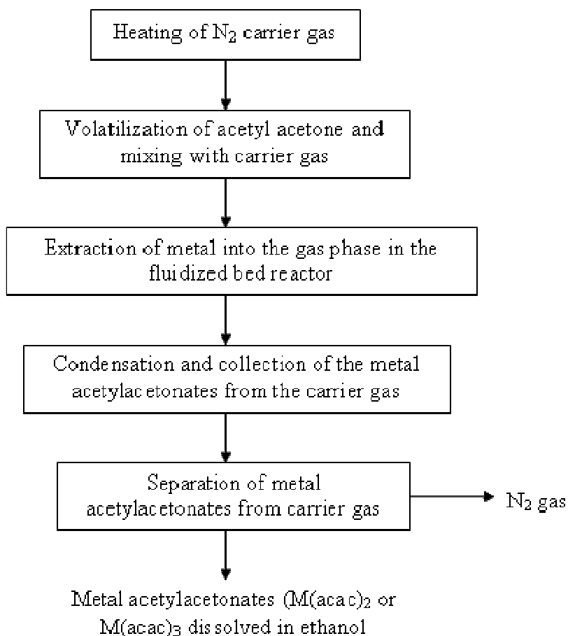
Figure 3-1 Process flow sheet for metal extraction in a fluidized bed reactor
