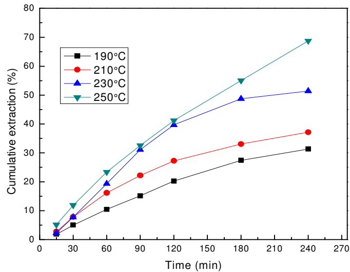
Figure 4-2 Effect of temperature on extraction for a 3wt% \text{Fe}_3\text{O}_2 mixture
