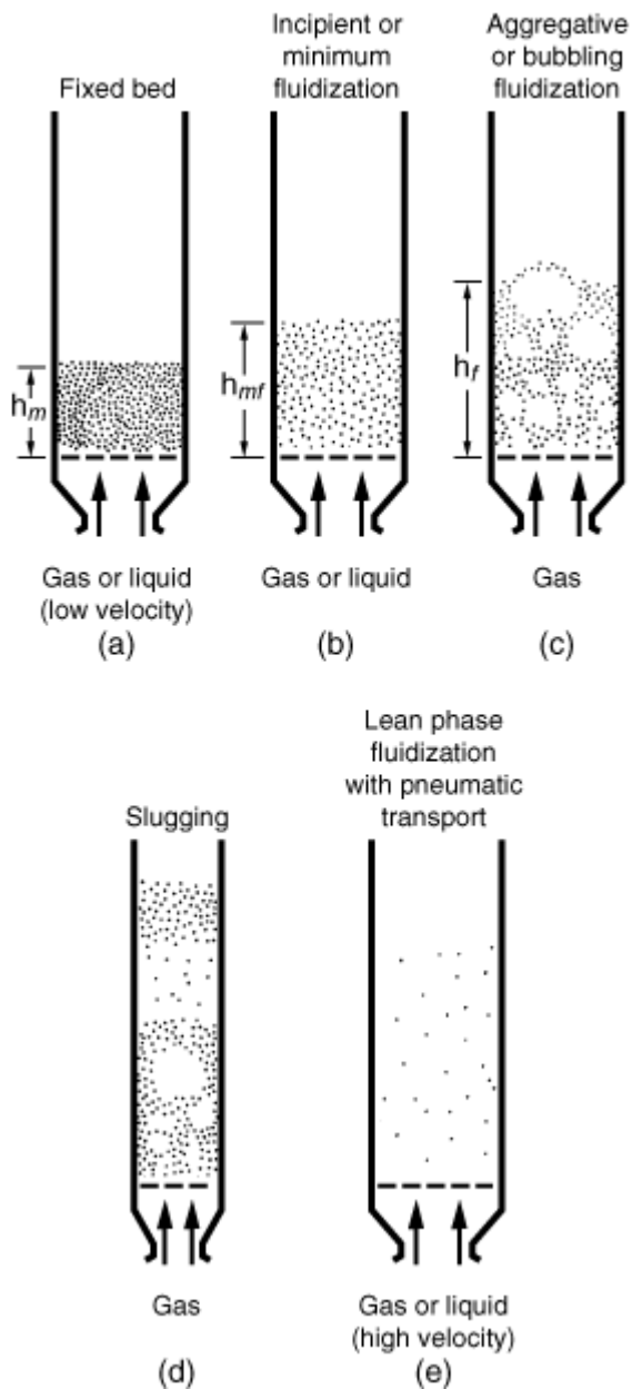
Figure 2-5 Behaviour of particles at various stages of fluidization
