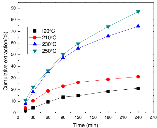
Figure 4-1 Effect of temperature on extraction for a 1wt% \text{Fe}_2\text{O}_3 mixture
