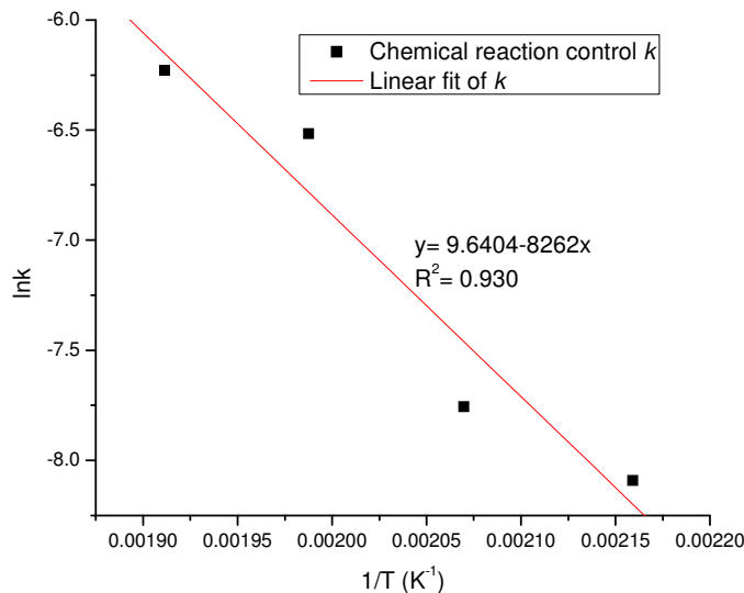
Figure 5-5 Arrhenius plot for chemical reaction control model at 1wt%Fe 2 O 3 and 1ml/min ligand flow rate
