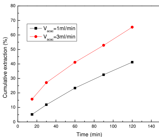
Figure 4-4 Effect of ligand flow rate on the extraction for a 3wt% mixture at 250°C
