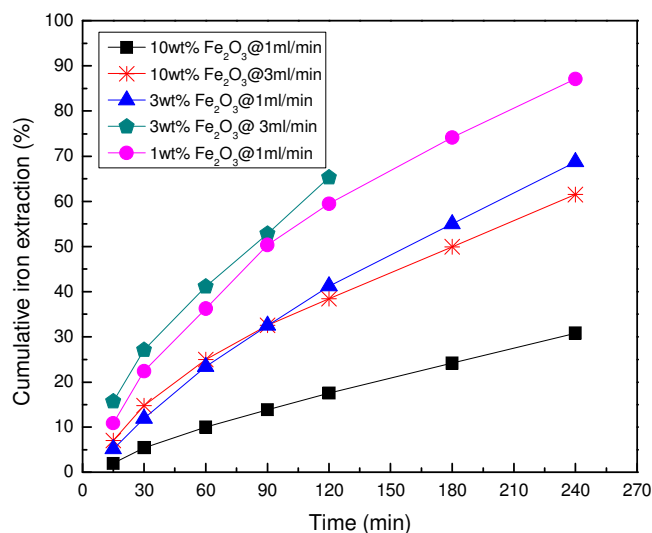
Figure 4-6 Effect of ligand concentration on extraction at 1wt%, 3wt% and 10wt% at 250°C
