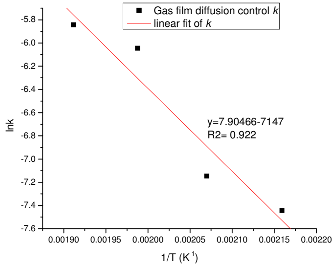
Figure 5-10 Arrhenius plot for gas film diffusion control model at 1wt%Fe 2 O 3 and 1ml/min ligand flow rate
