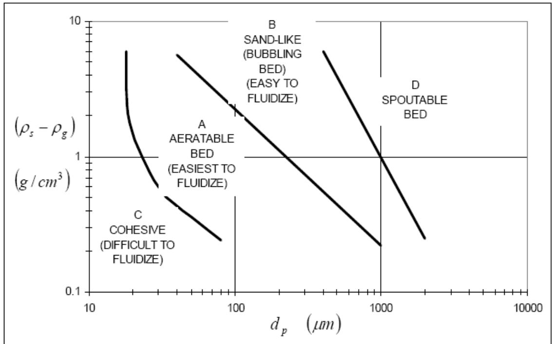
Figure 2-6 Geldart's fluidization classification of powders (Geldart, 1986)
