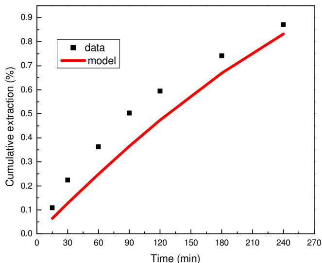
Figure 5-9 Comparison of conversion predicted by gas film diffusion control model with actual data obtained at 250°C
