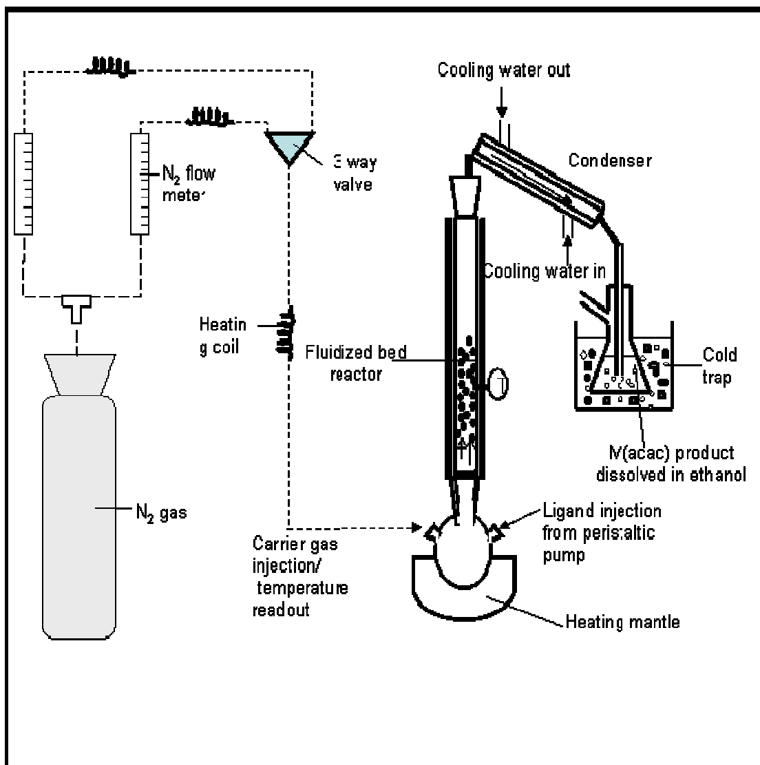
Figure 3-2 Schematic diagram of gas phase extraction
