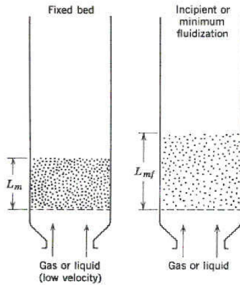
Figure 2-4 Behaviour of a packed bed before and at minimum fluidization velocity
