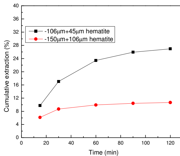
Figure 4-8 Effect of particle size on extraction at 3ml/min on a 3wt% mixture at 230°C
