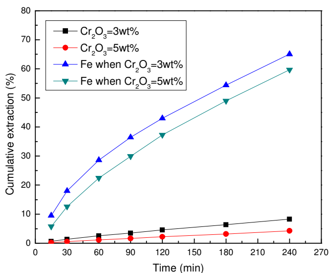
Figure 4-12 Extraction of Fe and Cr from mixtures containing Cr 2 O 3 & 5wt% Fe 2 O 3 at 3ml/min & 210°C
