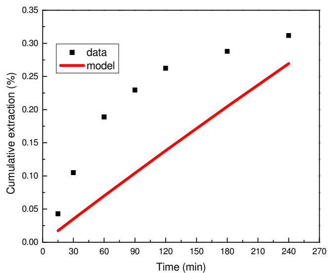
Figure 5-7 Comparison of conversion predicted by gas film diffusion control model with actual data obtained at 210°C
