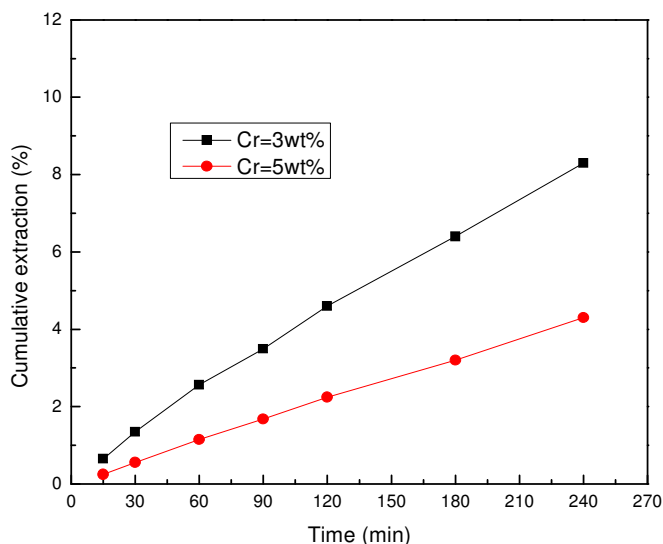
Figure 4-11 Extraction of Cr from a mixture containing \text{Cr}_2\text{O}_3 and 5wt% \text{Fe}_2\text{O}_3 at 3ml/min & 210°C
