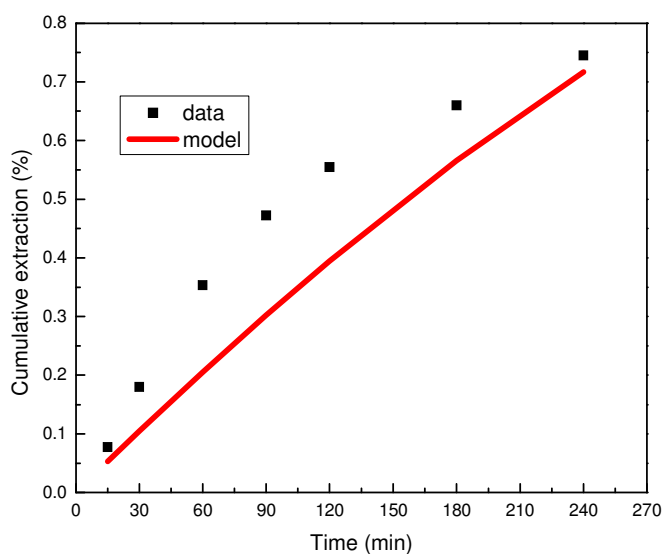
Figure 5-8 Comparison of conversion predicted by gas film diffusion control model with actual data obtained at 230°C
