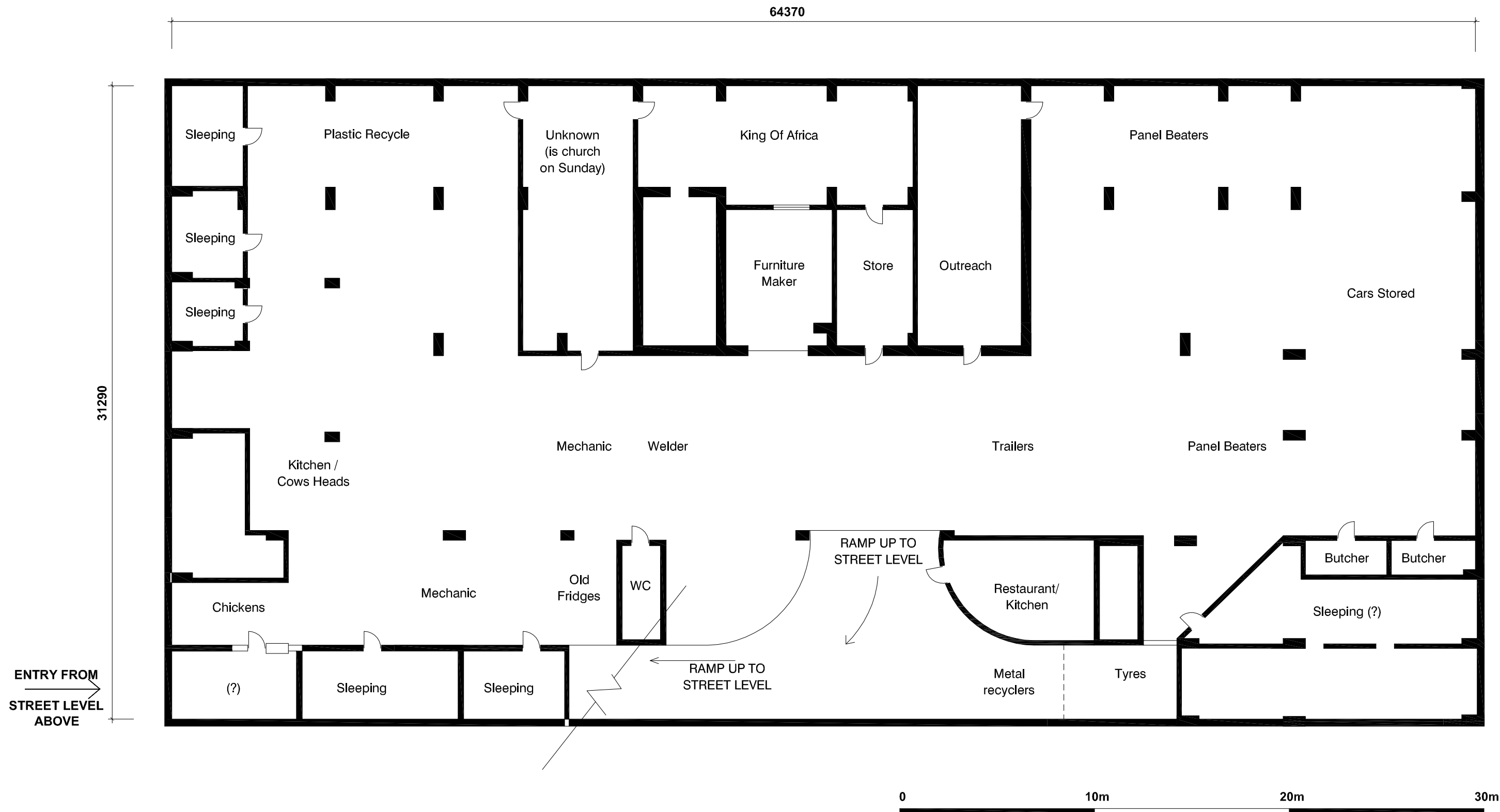
FIGURE 15: Plan of Basement. Approximately 64 x 31 metres, approximately 2,000 square metres area
