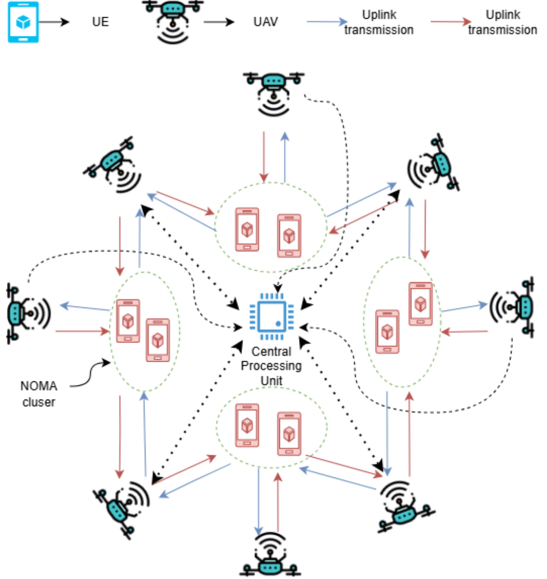
FIGURE 3.1: System model of CF-mMIMO with NOMA clusters.
