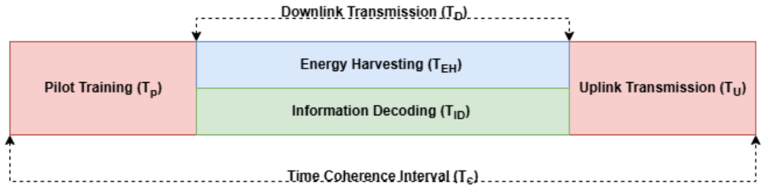
FIGURE 2.8: Frame structure for the PS-SWIPT protocol.
