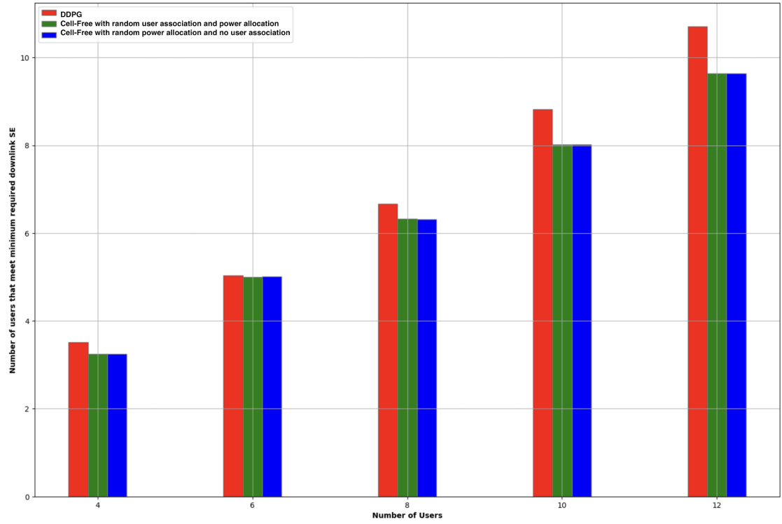
FIGURE 3.22: Achievable number of UE that meet the minimum required UL SE.
