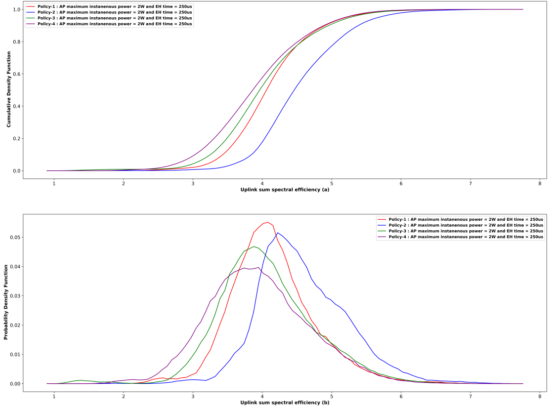
FIGURE 3.15: CDF and PDF UL SSE.
