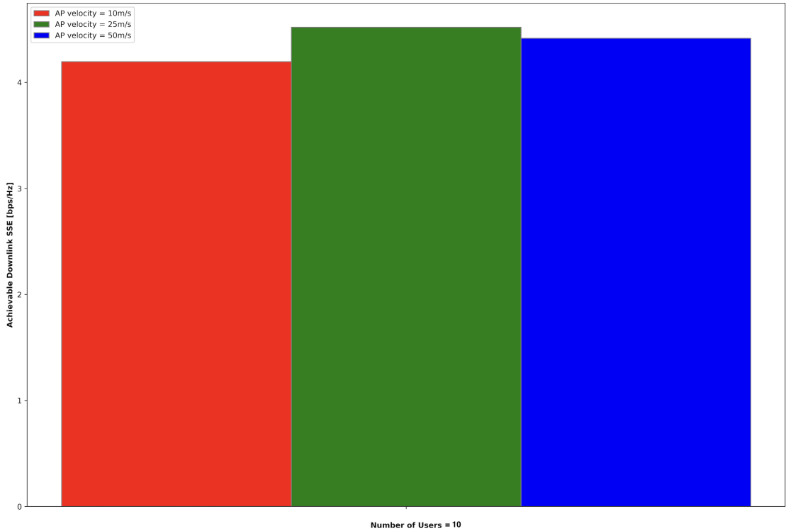
FIGURE 3.19: The impact of UAV operating velocity on trained DDPG model performance.
