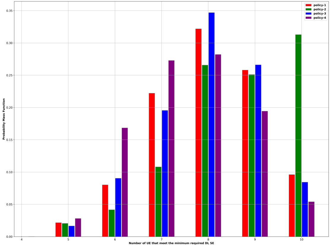
FIGURE 3.16: PMF of the number UE that meet minimum required DL SE.
