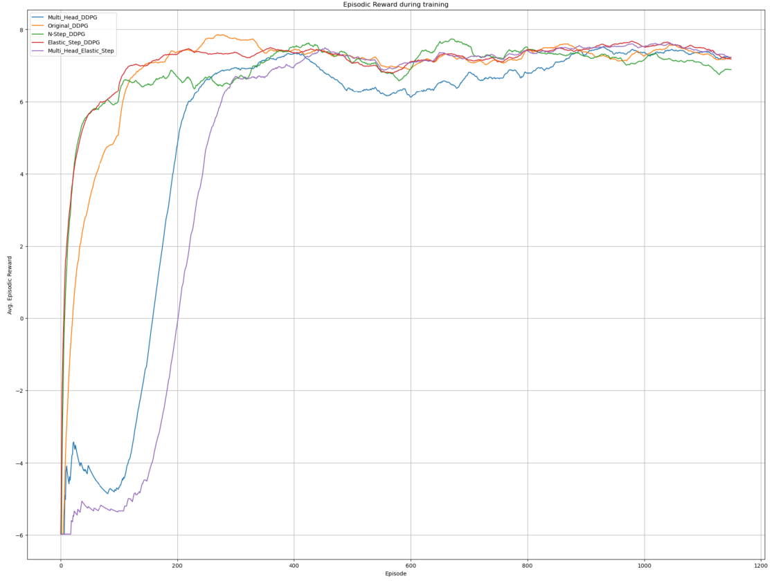
FIGURE 4.1: DDPG variants training performance.
