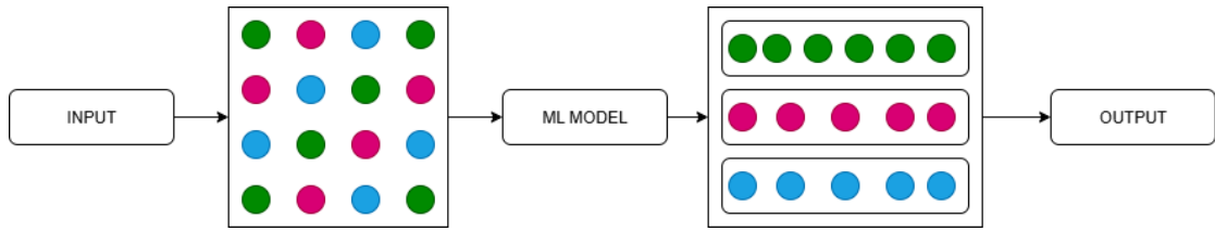
FIGURE 2.10: Unsupervised learning architecture.
