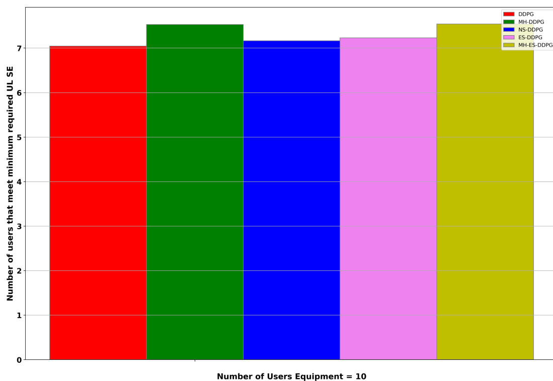
FIGURE 4.5: Comparison of the achievable number of UE that meet the minimum required UL SE.
