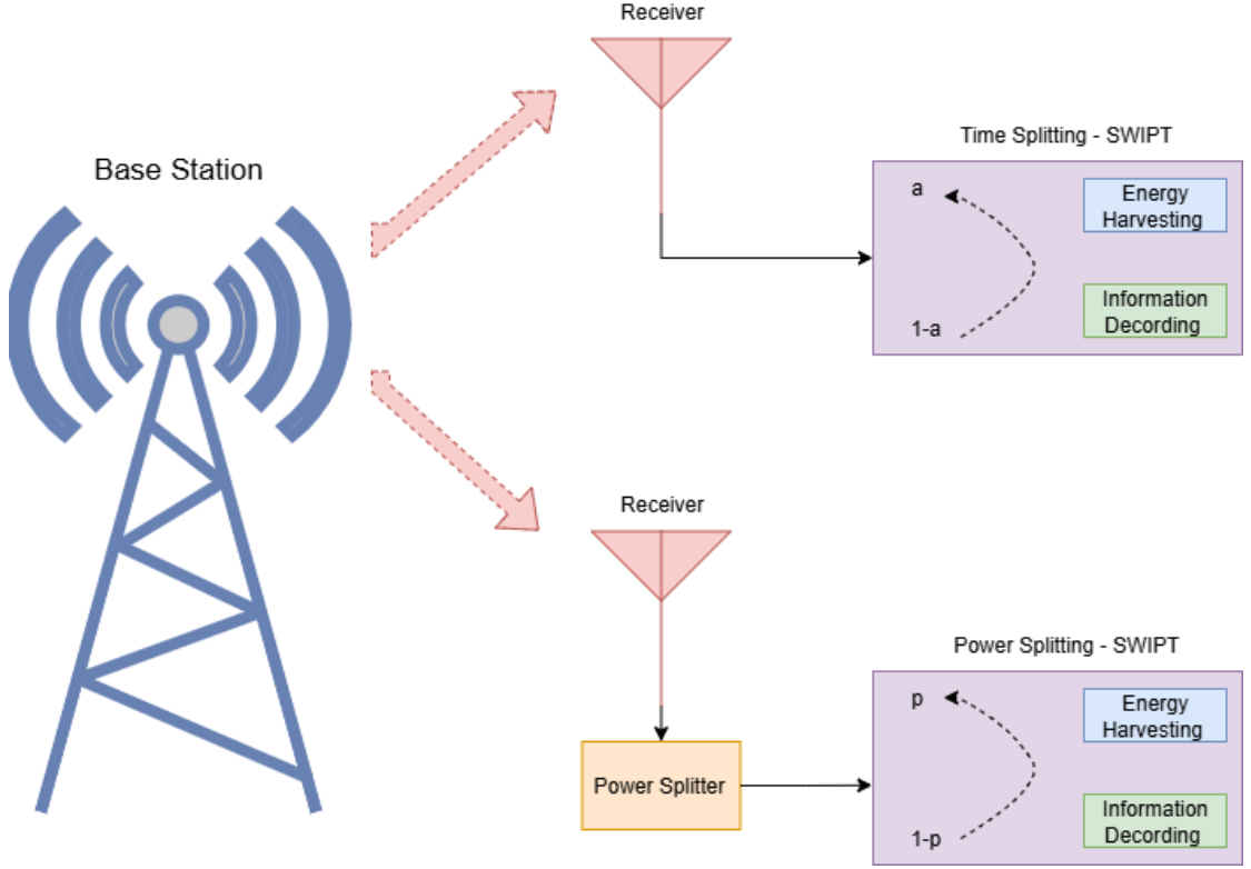
FIGURE 2.6: Two architectures for SWIPT.
