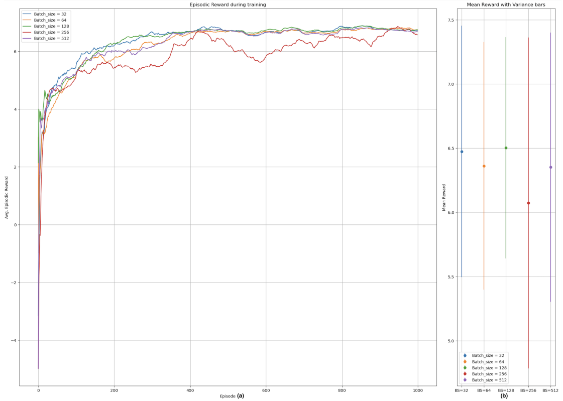
FIGURE 3.8: DDPG training performance after hyper-parameter tuning.
