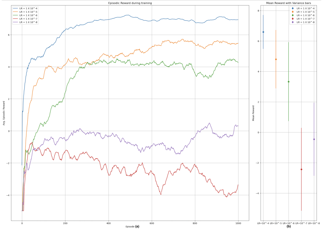
FIGURE 3.5: The effect of learning rate on DDPG training performance.
