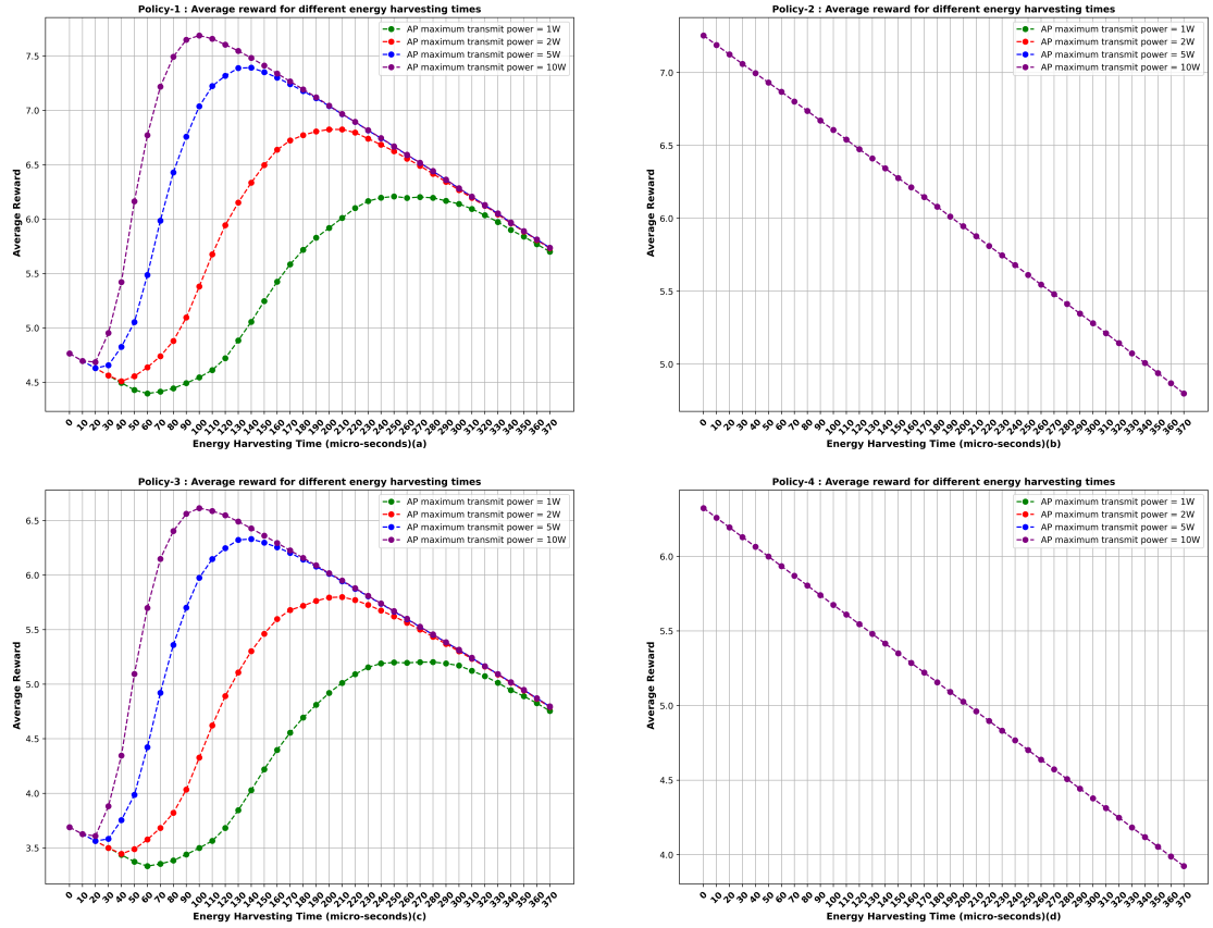
FIGURE 3.10: Impact for energy harvesting time on policy performance.
