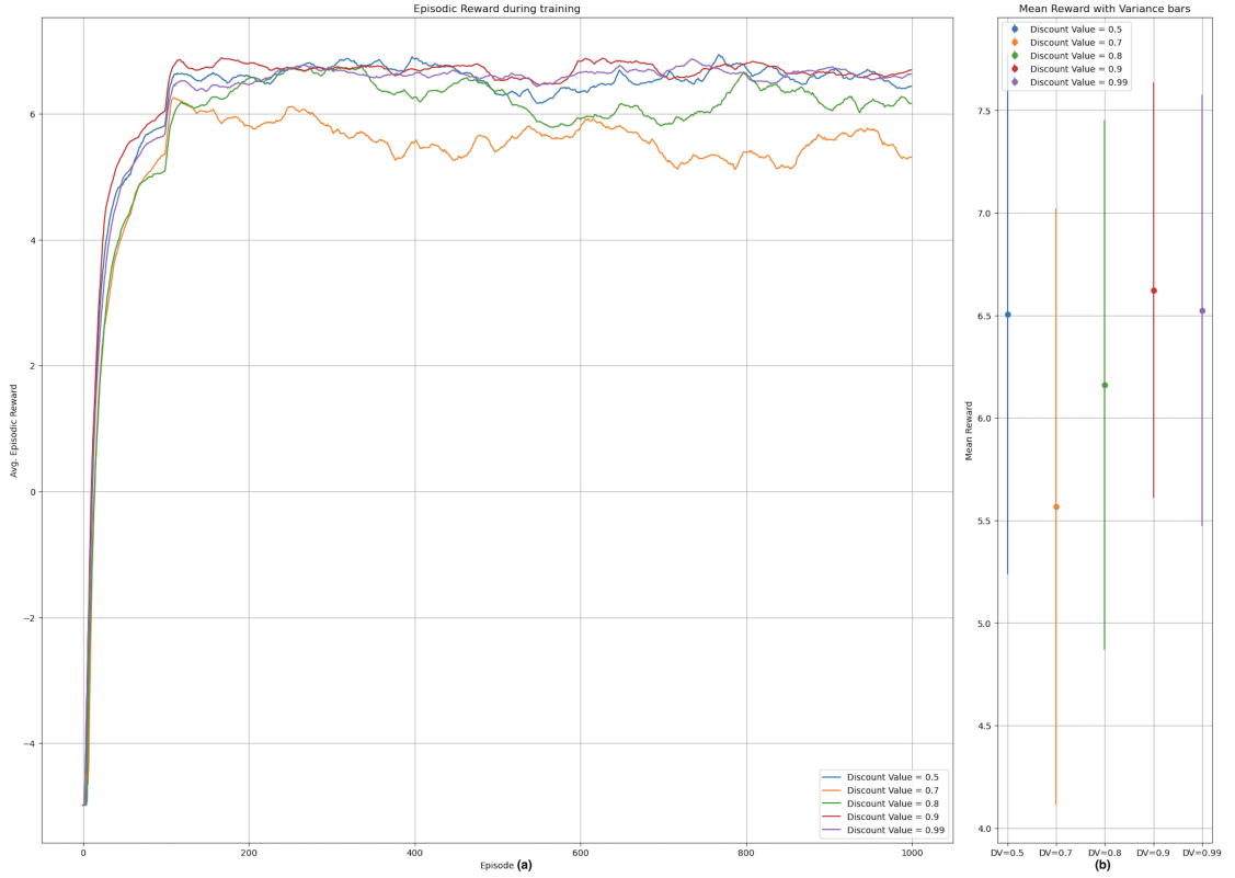
FIGURE 3.7: The effect of discount value on training performance
