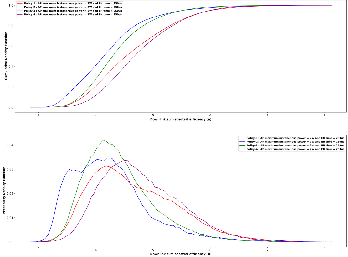
FIGURE 3.14: CDF and PDF of DL SSE.
