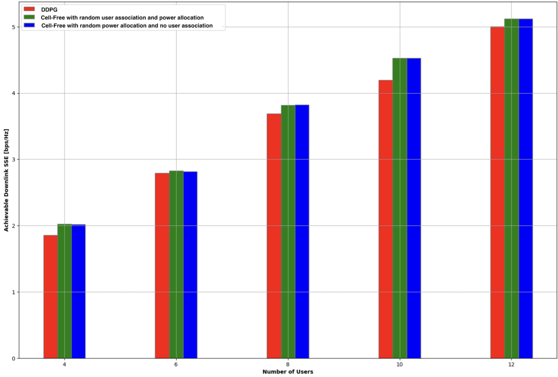
FIGURE 3.20: Achievable DL SSE performance of DDPG model.
