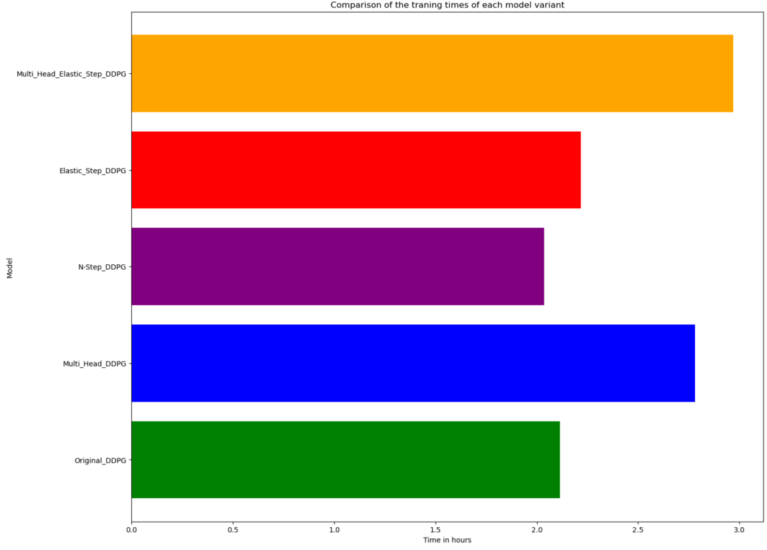
FIGURE 4.2: Comparison of DDPG variants training times.
