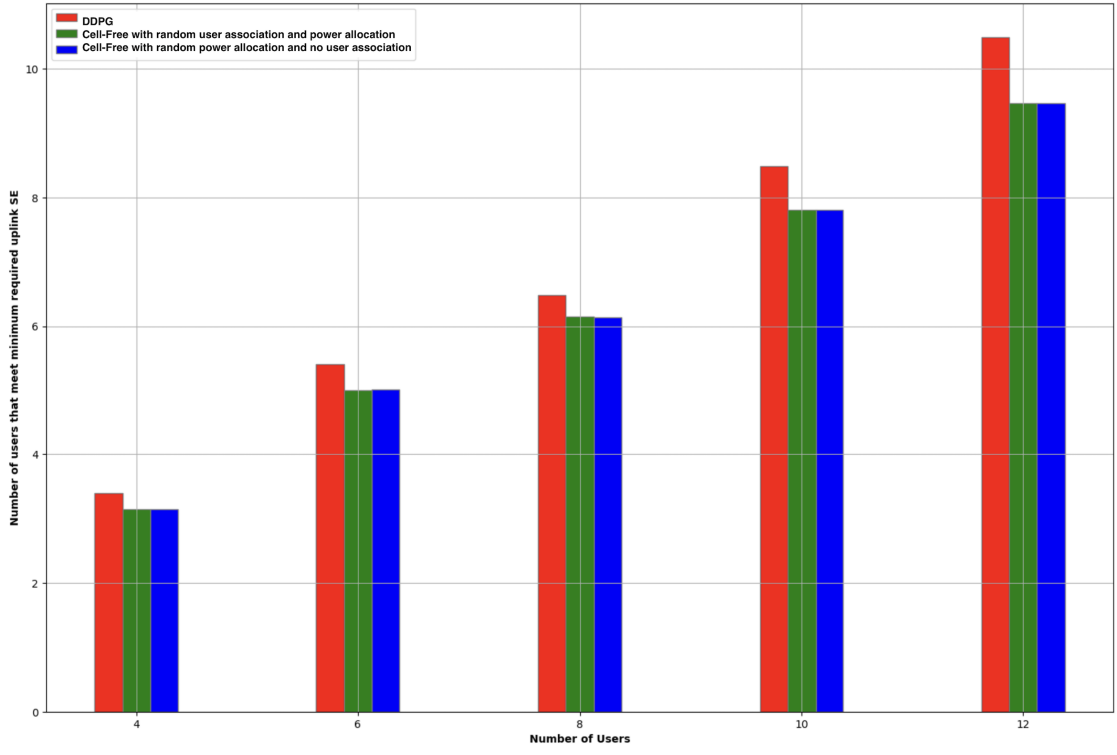
FIGURE 3.21: Achievable number of UE that meet the minimum required DL SE.
