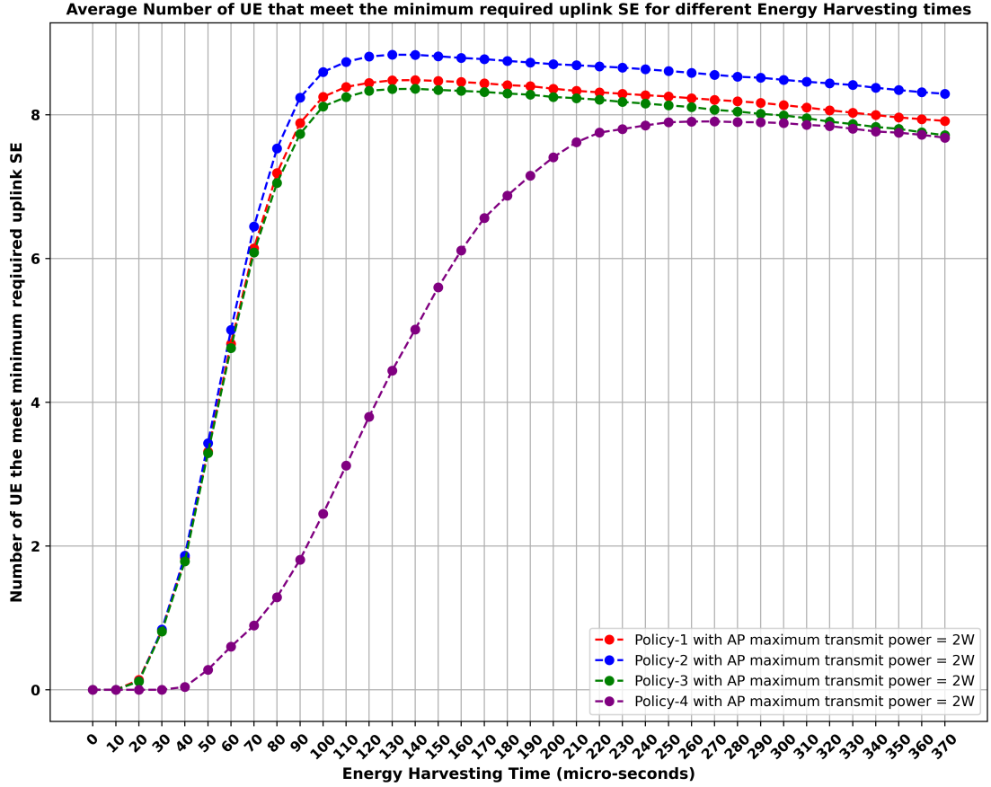
FIGURE 3.12: Policy performance for the number of UE that meet minimum required UL SE.
