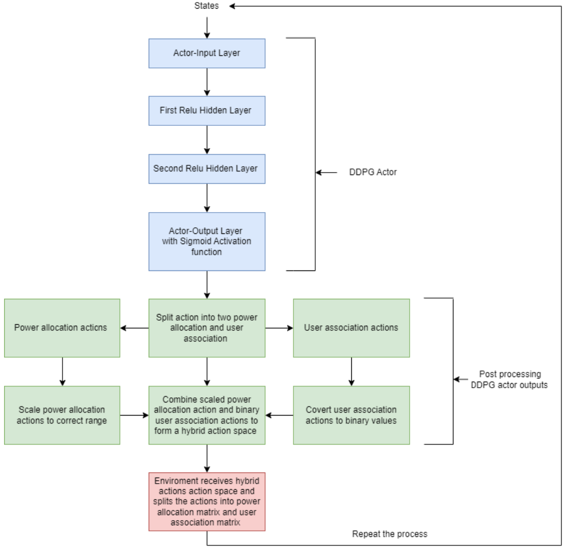
FIGURE 3.3: Post processing actions from the actor network.
