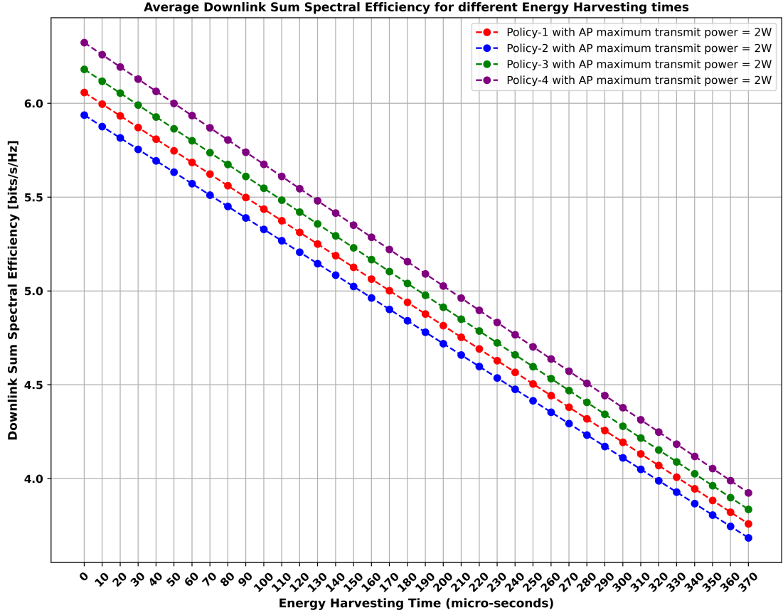
FIGURE 3.13: DL SSE performance for different policies.
