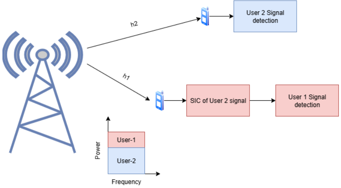
FIGURE 2.4: Downlink NOMA transmission.
