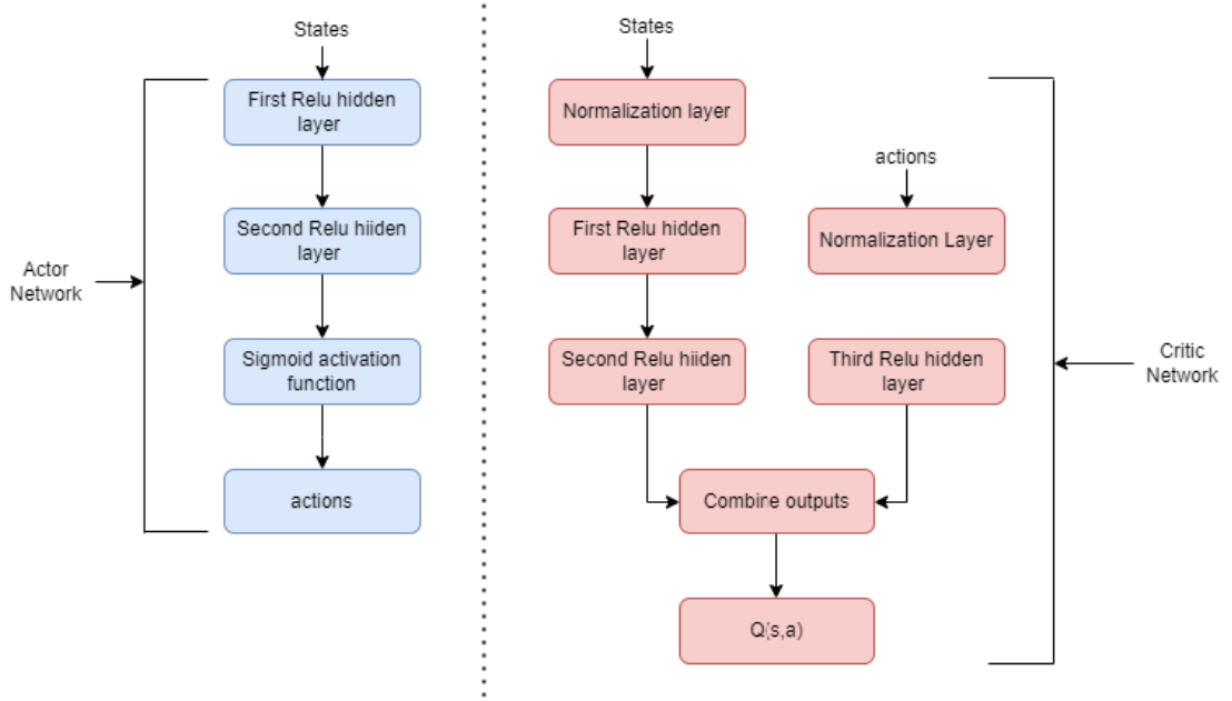
FIGURE 3.4: Actor and critic network structure.
