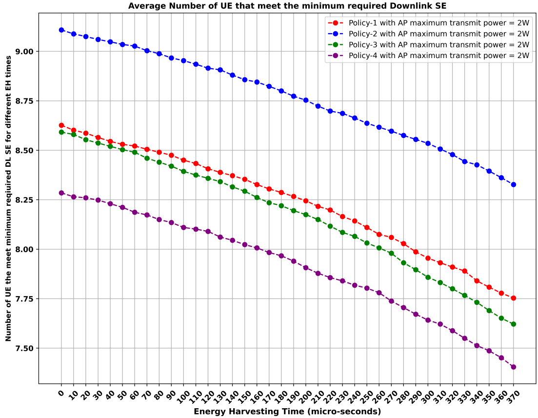
FIGURE 3.11: Policy performance for the number of UE that meet minimum required DL SE.
