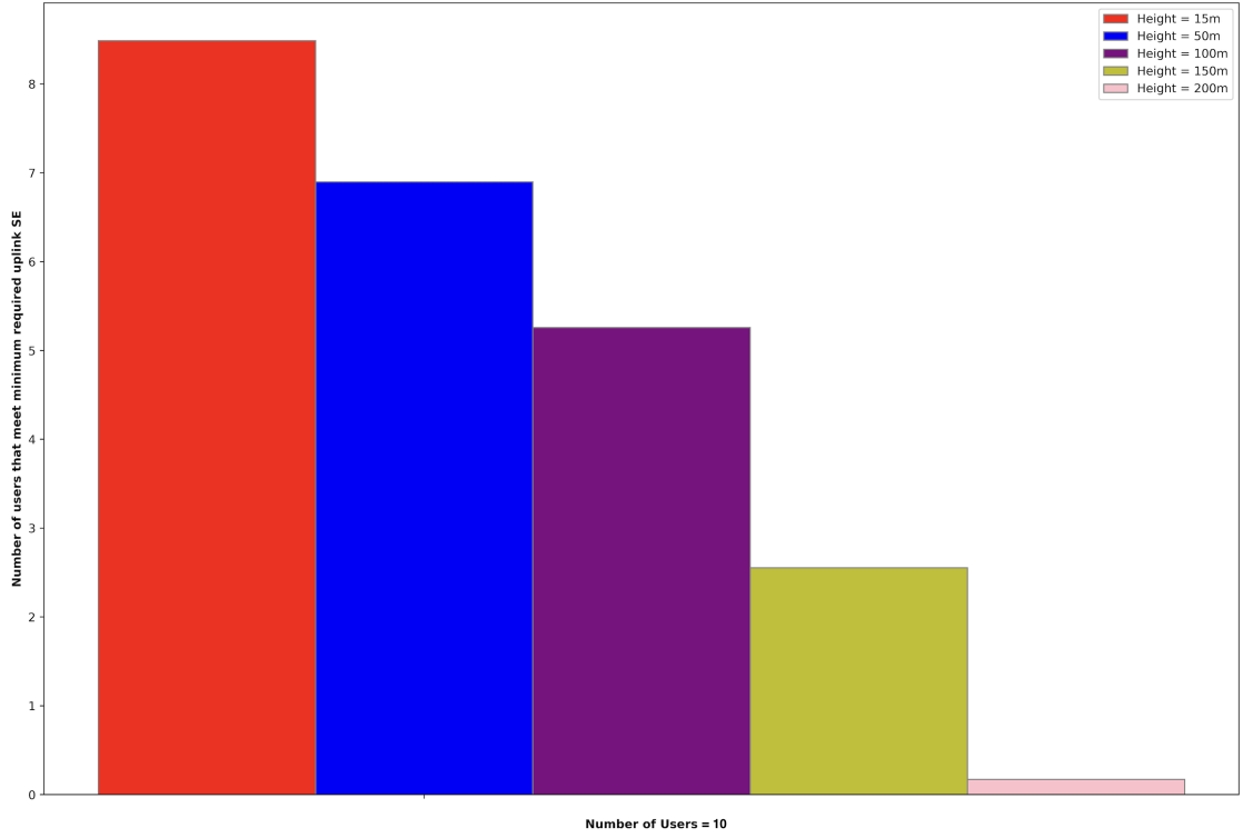
FIGURE 3.18: The impact of UAV operating height on trained DDPG model performance.
