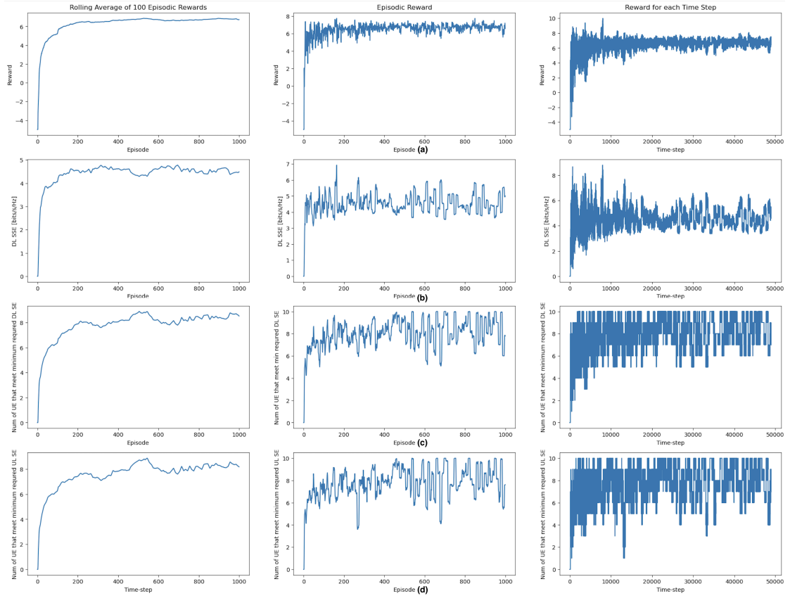
FIGURE 3.9: DDPG training performance after hyper-parameter tuning.
