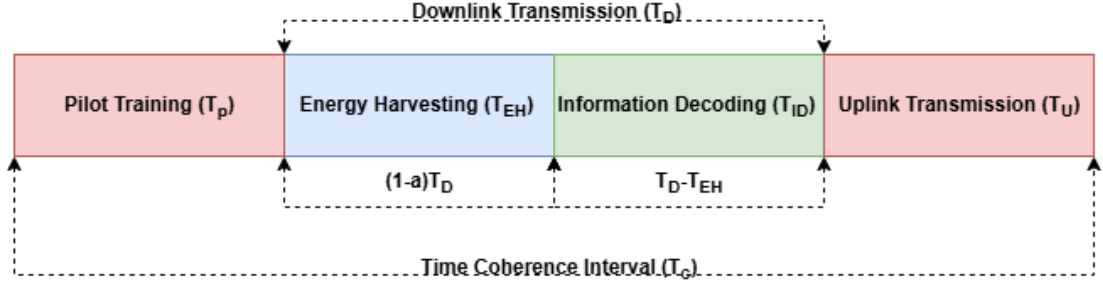
FIGURE 2.7: Frame structure for the TS-SWIPT protocol.
