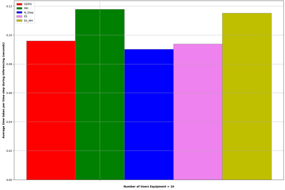
FIGURE 4.7: Comparison of DDPG variants' inferencing speeds.
