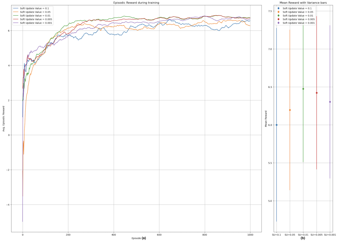
FIGURE 3.6: The effect of soft update size on training performance.
