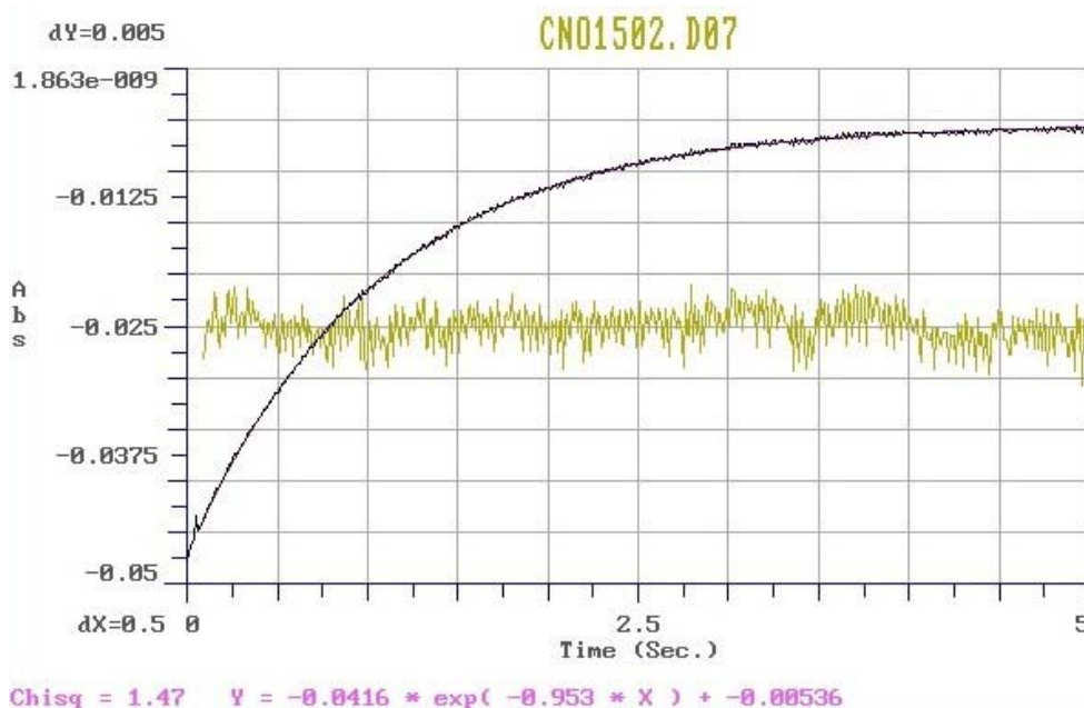
Figure 2.2 An example of a trace recorded for the \text{OCN}^- ligand with the fit obtained using a non-linear least-squares programme that employs a Newton–Raphson procedure. The yellow trace represents a plot of the residuals.
