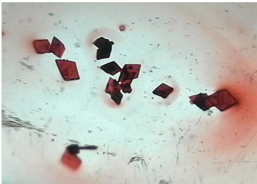
Figure 2.4 Crystals of aqua-10-nitrosocobalamin grown from a 50% acetonitrile/water solution and obtained by slow evaporation of the solution.
