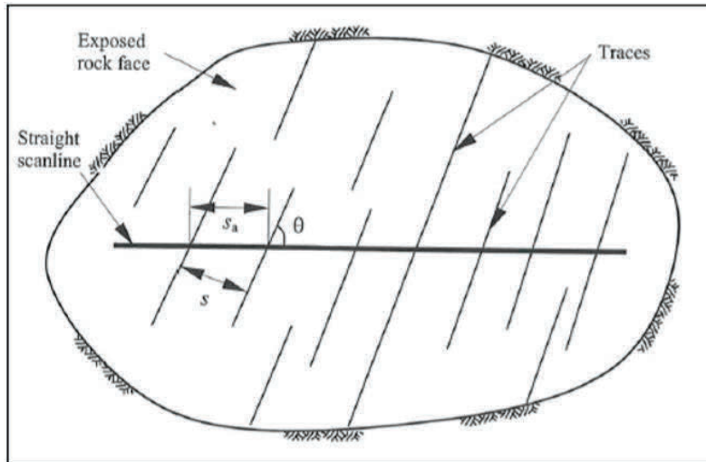
Figure 5.6: Scanline mapping (Zhang , 2004)
