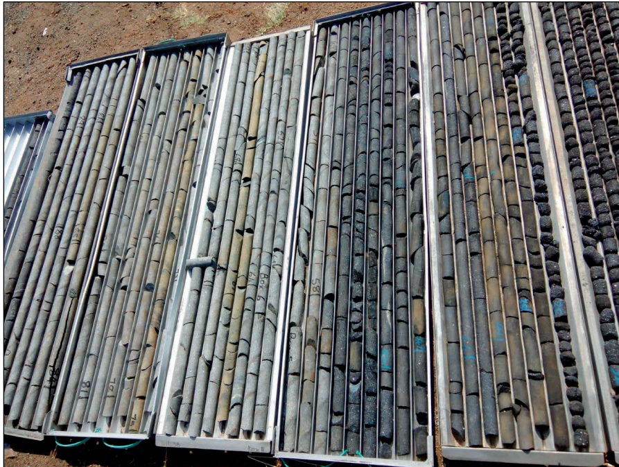
Figure 5.5: Orientated core from diamond drilling
