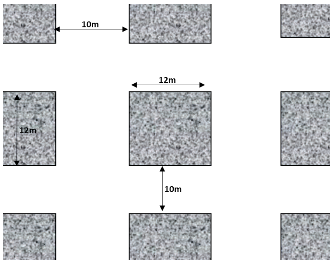
Figure 6.6: Mine working layout
