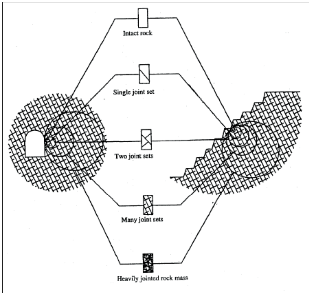
Figure 5.2: Difference between intact rock and rock mass (Hoek et al., 1998)
