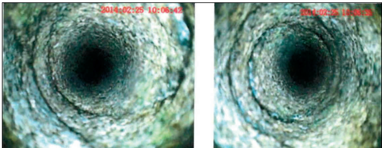
Figure 3.6: Two continuous sub-horizontal weakness planes with visible infilling material ( Internal Mine Document (a) , 2014)
