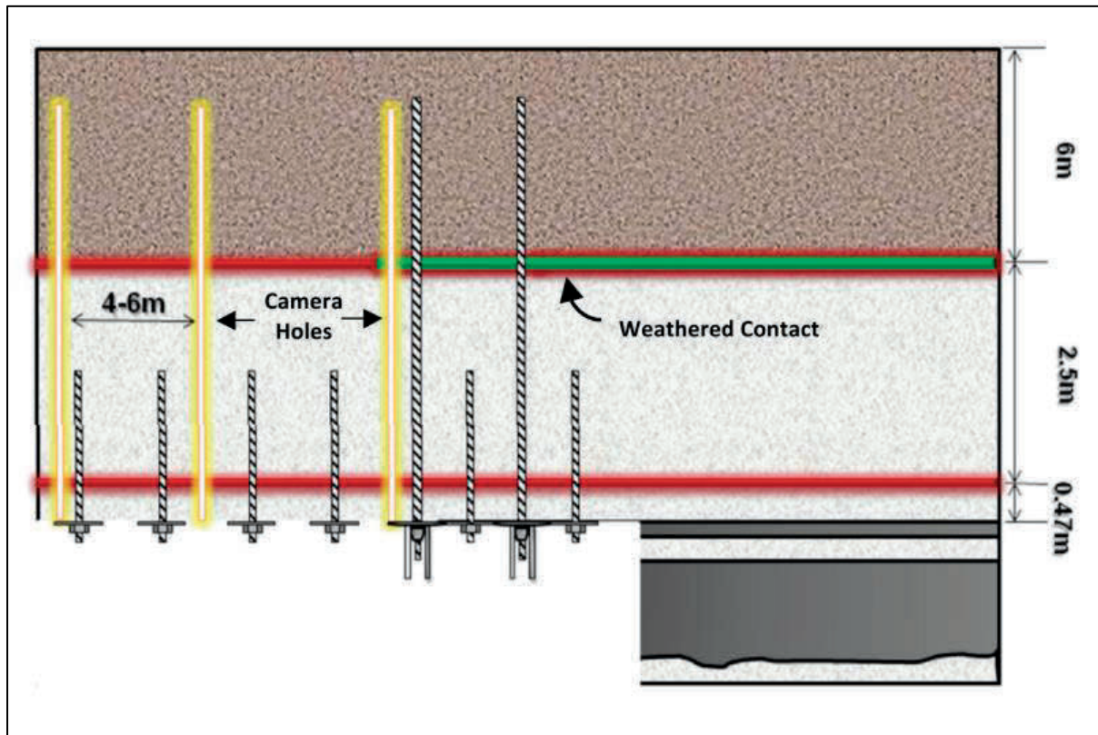
Figure 8.4: Adjusted support strategy based on local ground conditions (Esterhuizen, 2014)
