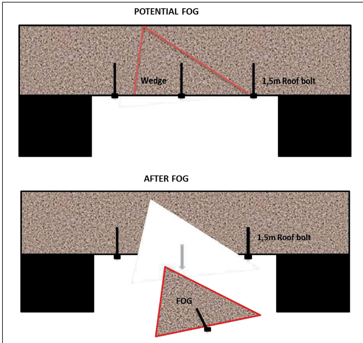
Figure 4.4: Schematic diagram of wedge failure mechanism
