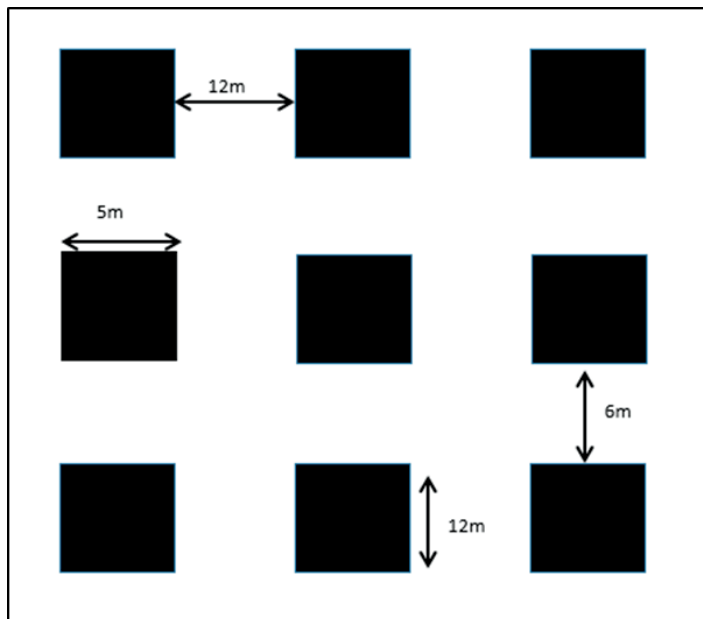
Figure 2.11: Schematic diagram of a regular pillar layout
