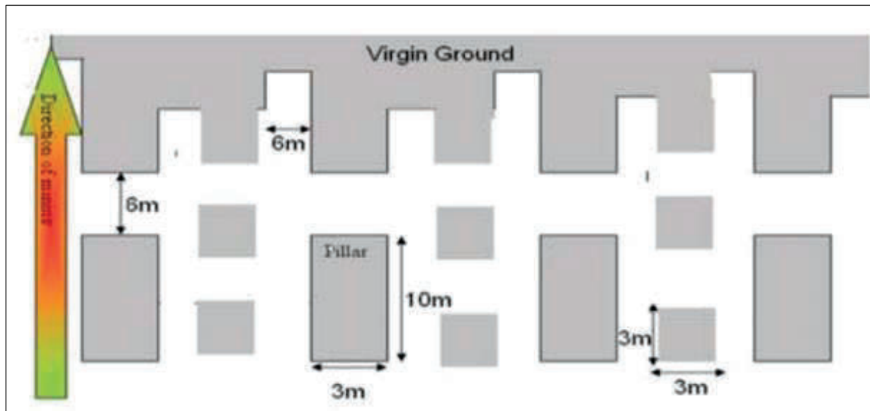
Figure 2.12: Mining layout in poor ground conditions at a Zimbabwean platinum room and pillar mine (Chikande & Zvarivadza, 2016)
