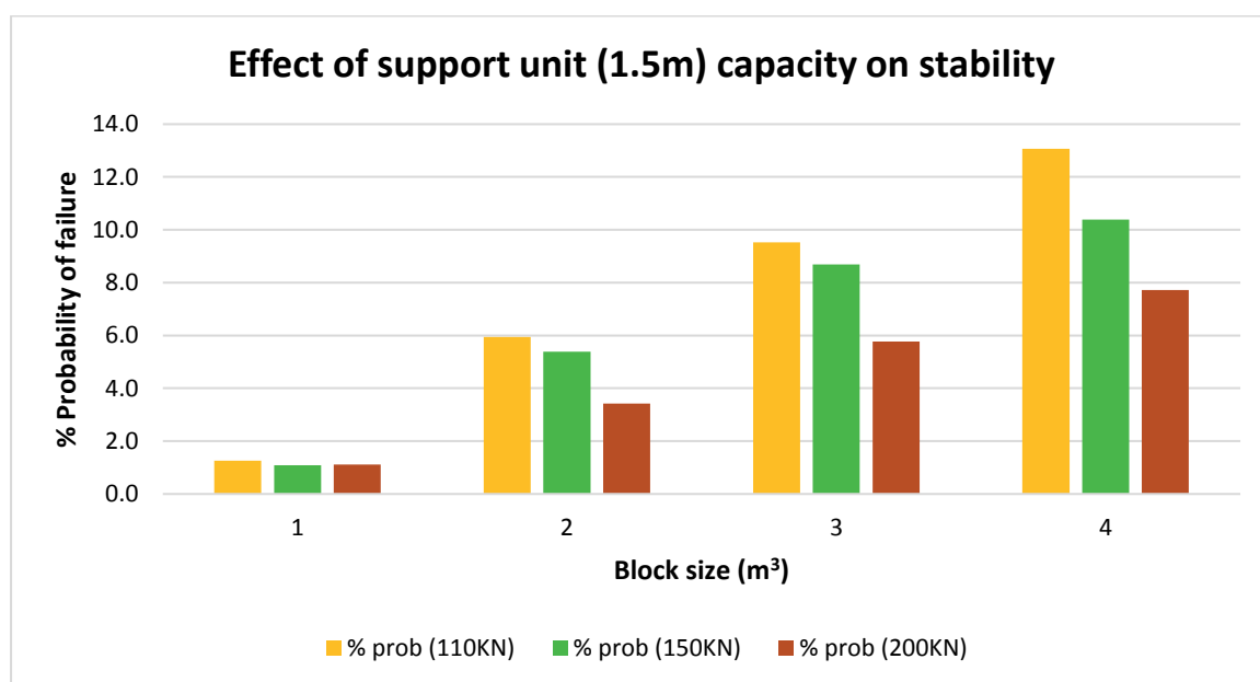
Figure 7.11: Effect of support unit capacity on stability
