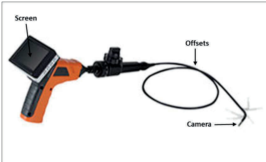
Figure 3.4: Borehole camera ( Anon, nd )
