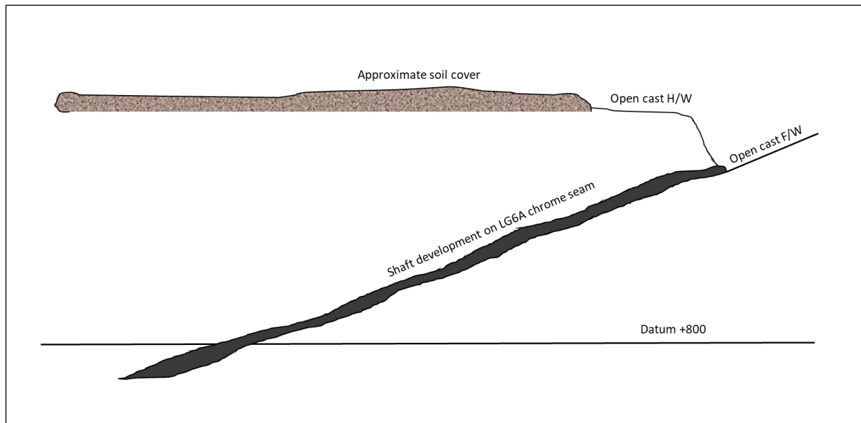
Figure 2.10: Flat dipping ore body at shallow depth ( Internal Mine Document, 2013 )
