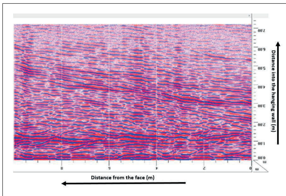
Figure 8.1: GPR scan image showing distance scanned and penetration depth
