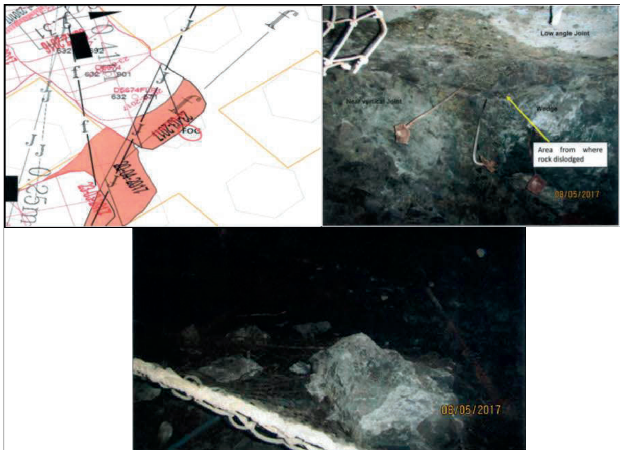
Figure 4.6: FOG following intersection of geological structures (Internal Mine Document (a), 2017)
