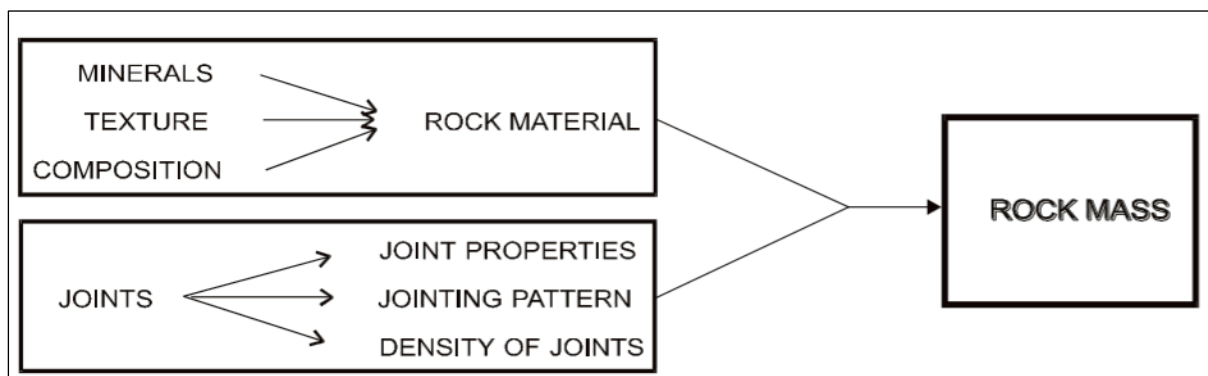
Figure 5.1: Building blocks of a rock mass (Palmström, 2001)
