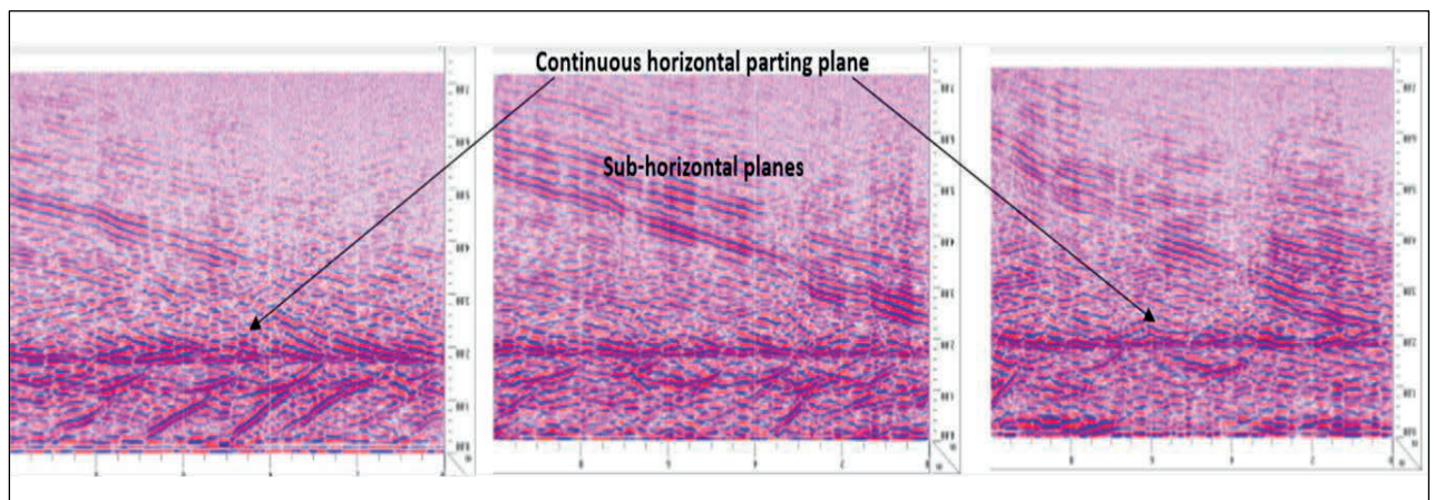
Figure 3.2: Processed GPR scan image
