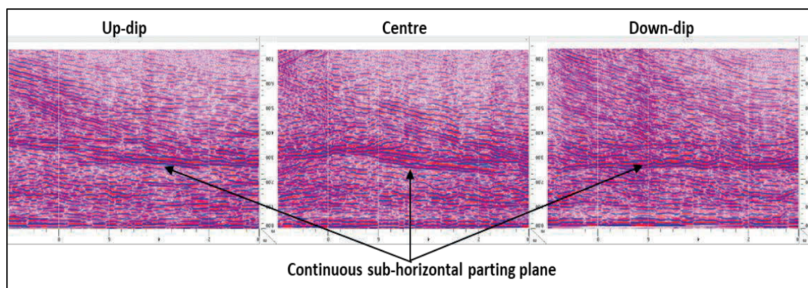
Figure 6.10: GPR scan at Panel 74S back area
