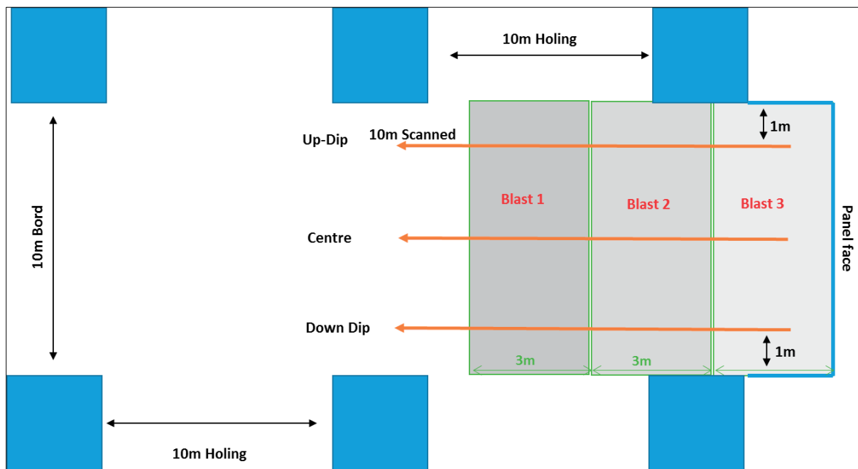
Figure 8.2: GPR scanning plan for a panel after three blasts
