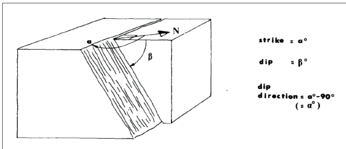
Figure 5.3: Relationship between dip, dip direction and strike (ISRM, 1978).
