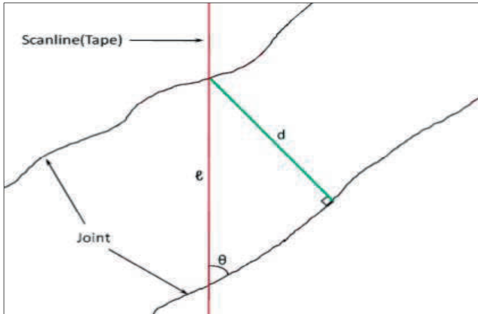
Figure 5.4: Correct measurement of joint spacing (Nezomba, 2012)
