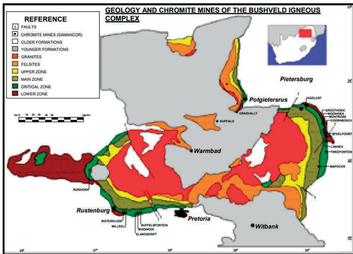
Figure 1.1: Geology and Chrome mines in the Bushveld Complex ( Internal Mine Document, 2013 )
