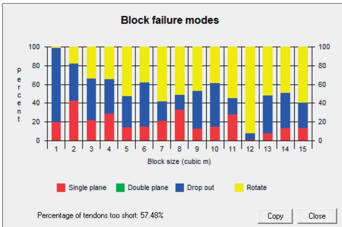
Figure 7.8: South section block failure modes
