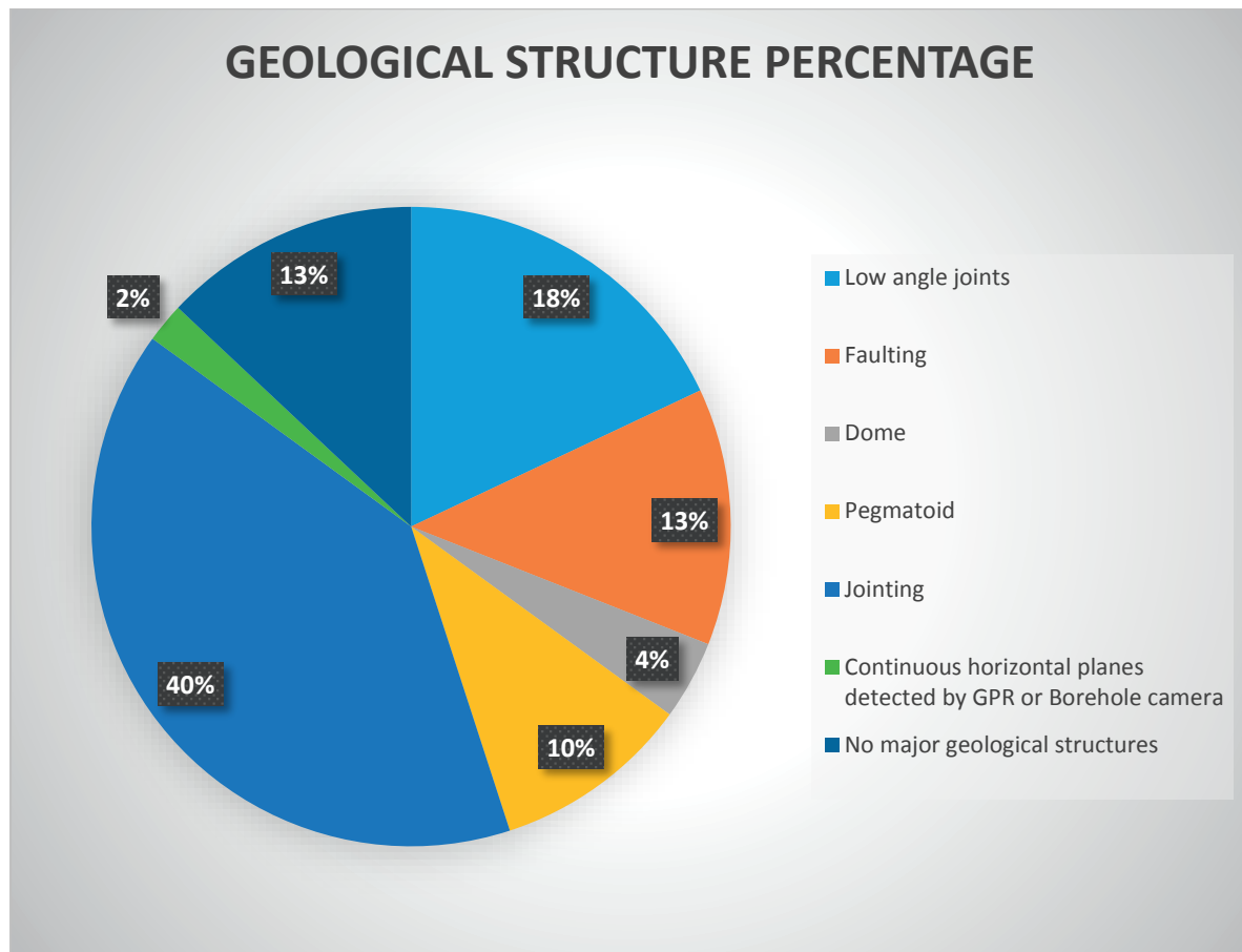
Figure 2.5: Percentages of geological structure occurrences in February 2018
