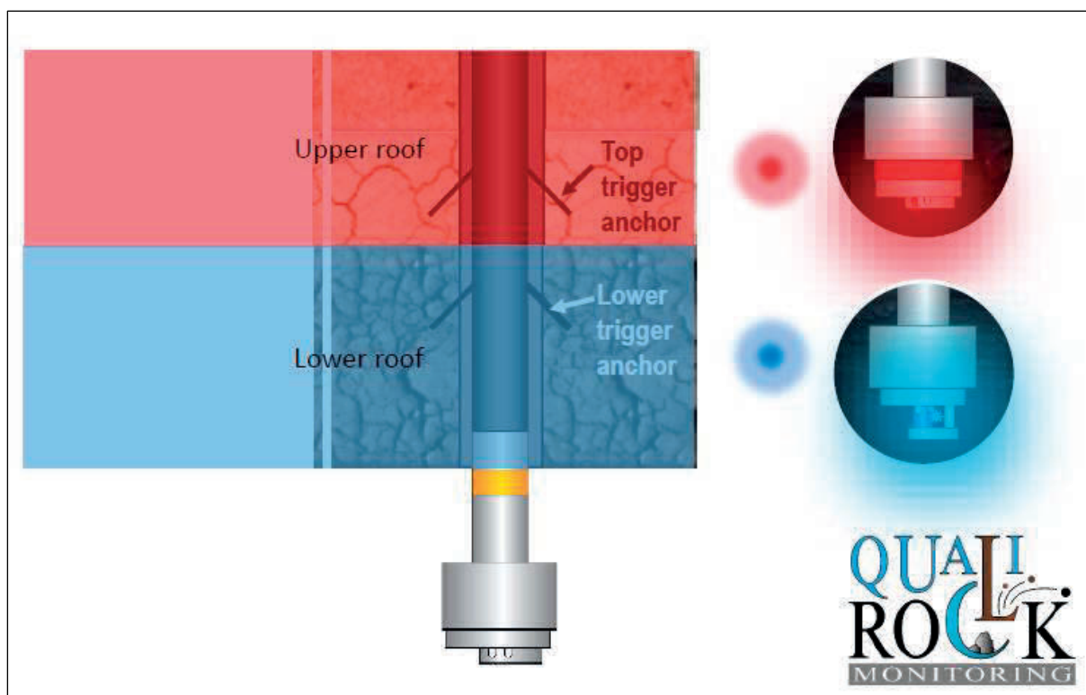
Figure 8.5: Rocktale installed in the hanging wall (QUALIROCK (b), 2016)
