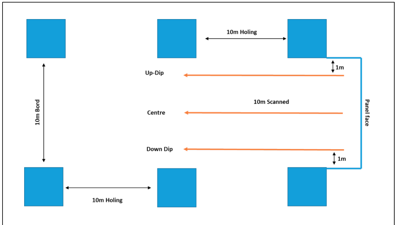
Figure 3.1: Schematic diagram of a panel to be scanned using GPR
