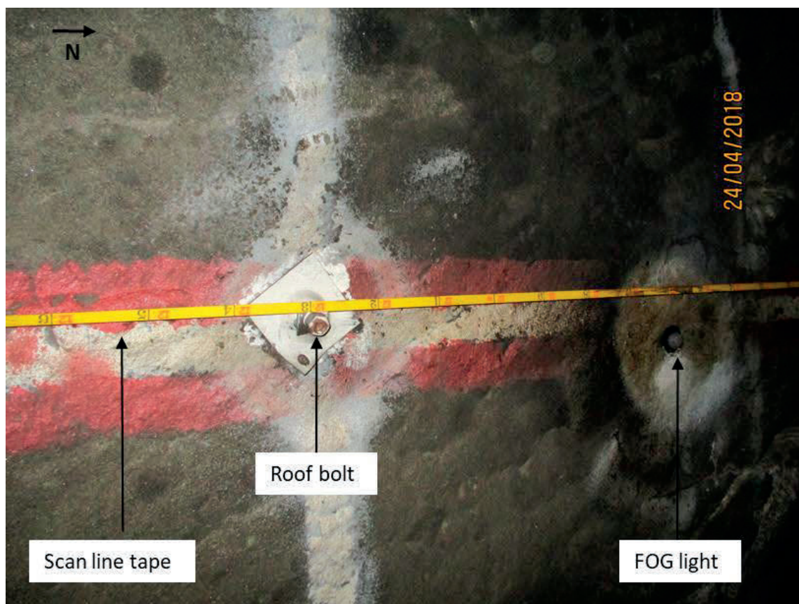
Figure 6.5: Scan line tape aligned to the centreline of the panel
