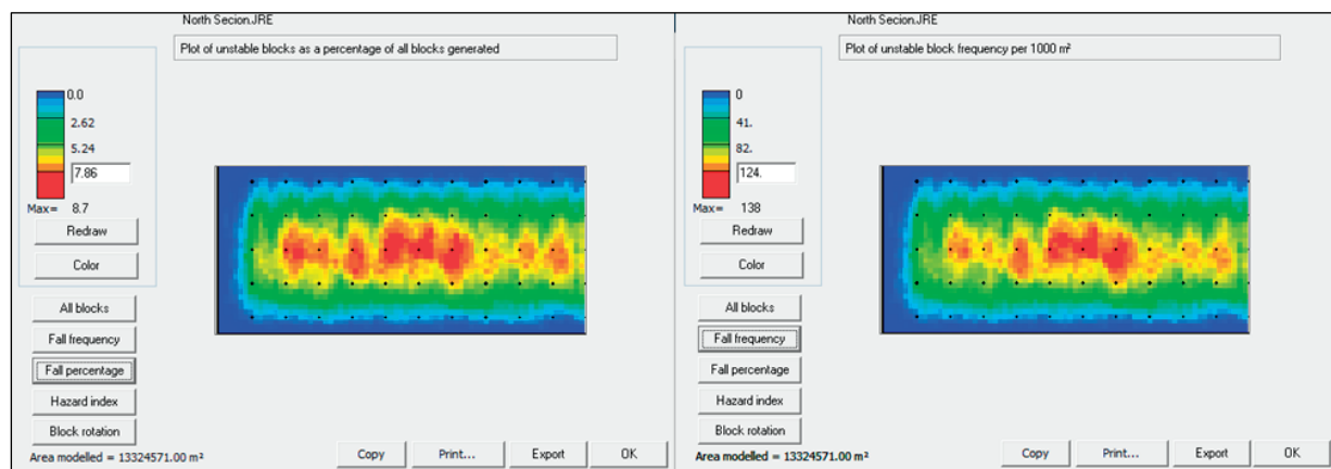
Figure 7.5: North section area modelled
