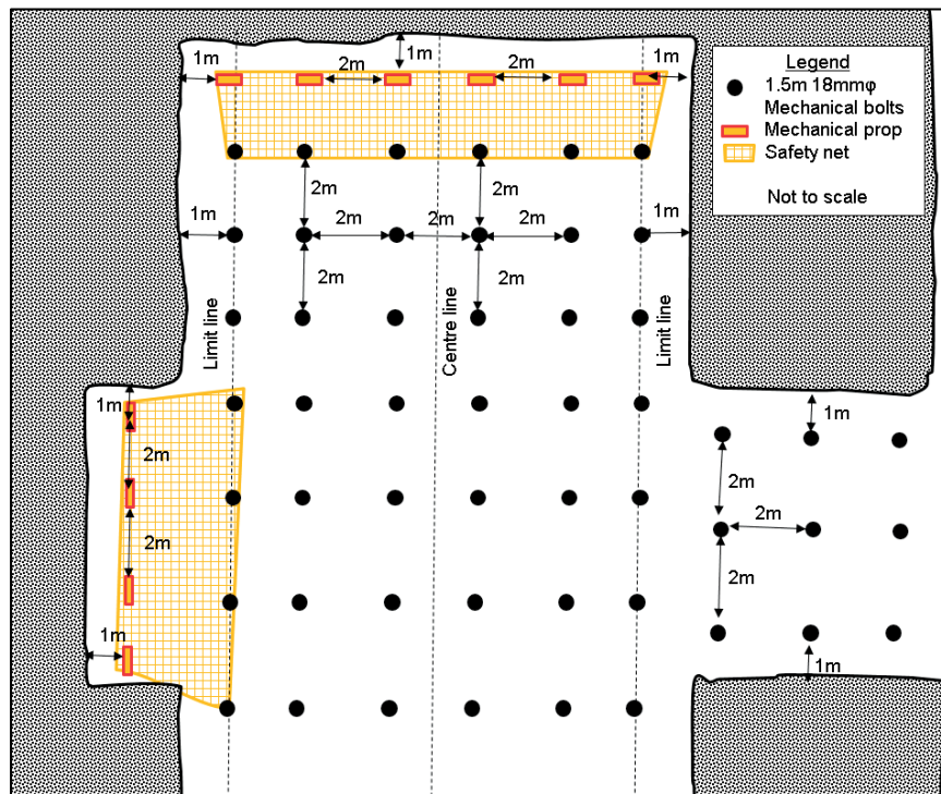
Figure 2.13: Local support layout ( Internal Mine Document (b), 2017 )
