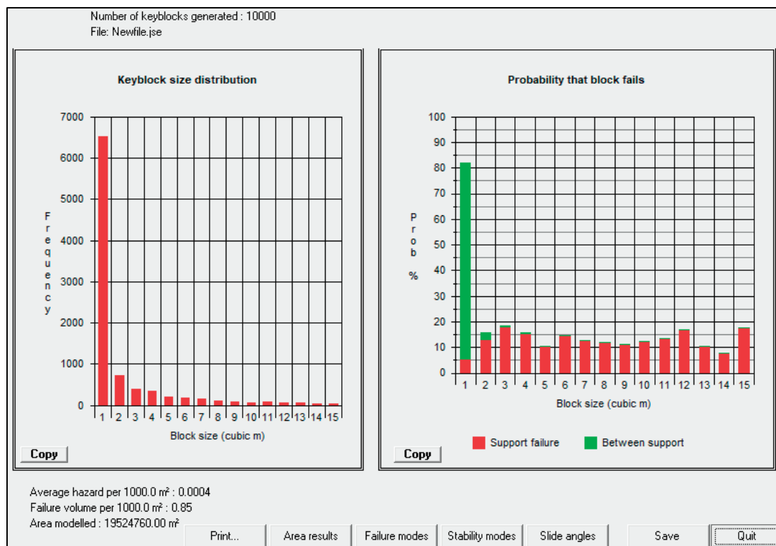
Figure 7.4: South section key block size distribution
