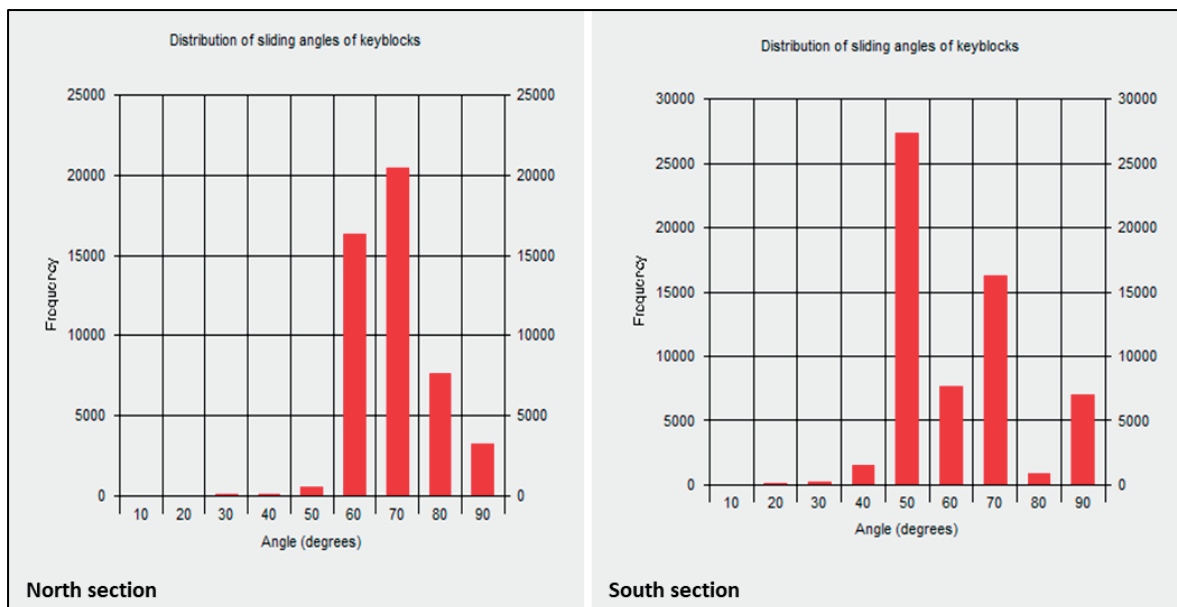
Figure 7.9: Distribution of sliding angles of key blocks
