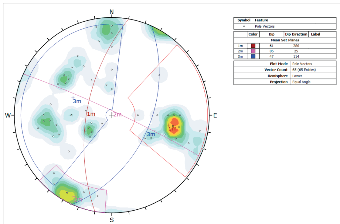
Figure 6.8: Overall joint orientation in the South Section
