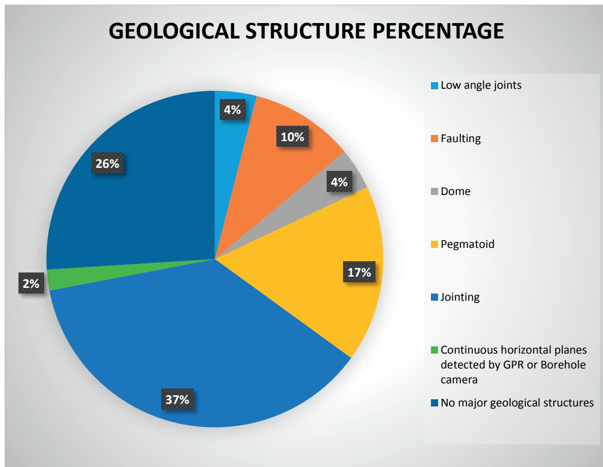
Figure 2.6: Percentages of geological structure occurrences in April 2018
