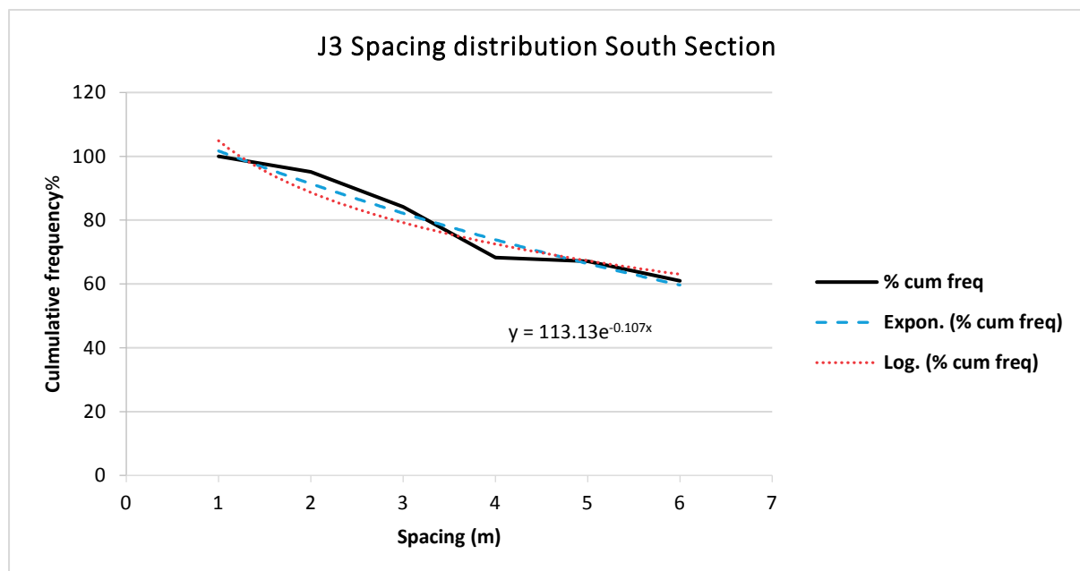
Figure 6.14: South Section J3 spacing showing negative exponential distribution
