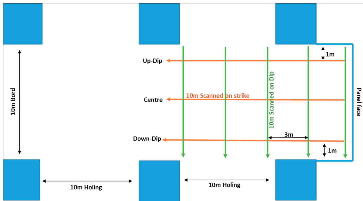
Figure 8.3: GPR scan layout for both dip and strike direction
