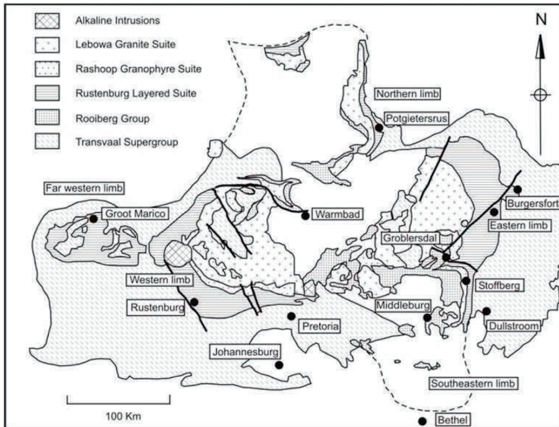
Figure 2.2: Geological distribution of the Bushveld Complex (Kinnaird, 2005)
