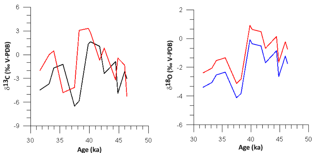
Fig. 5.21b \delta^{13}C and \delta^{18}O isotope age curve for the BL1 stalagmite for the post-hiatus section. Corrected values for carbon and oxygen are shown in red. For carbon values were corrected using the calcite-aragonite fractionation factor of 1.7 (Romanek et al. 1992). For oxygen corrections were applied using the acid fractionation factor of 1.0 (Kim et al. 2007).
