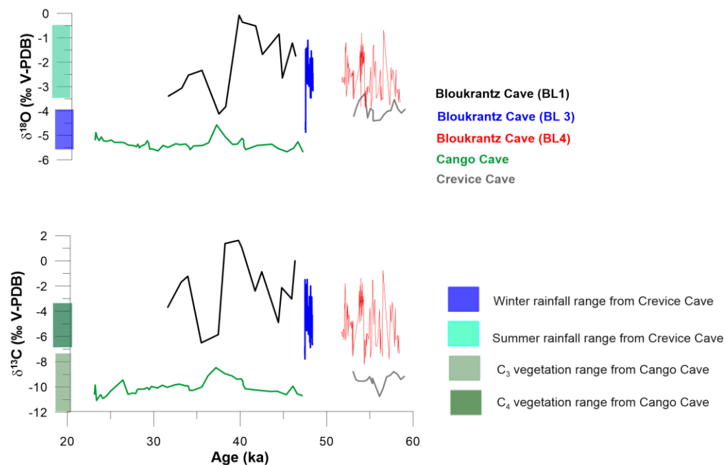
Fig. 6.4 Comparison of the \delta^{13}\text{C} and the \delta^{18}\text{O} data from the De Hoop stalagmites (BL1, BL3 & BL4) and Klipdrift Shelter (KDS) with published speleothem records from the southern Cape (Crevice Cave & Cango Cave) corresponding to MIS 3 (early & late). The raw \delta^{13}\text{C} data are shown. For the BL1 data the raw aragonite corrected \delta^{13}\text{C} data are plotted. Here the data from Pinnacle Point (PP29), Herold's Bay and Sandkraal Cave and Little Karoo data are not included as the author did not have access to the raw data generated for the composite records from these sites. The theoretical range of \delta^{13}\text{C} values for \text{C}_3/\text{CAM} and \text{C}_4 vegetation adopted from Talma and Vogel's (1992) estimates for Cango Cave are highlighted along the bottom y-axis and the theoretical range of \delta^{18}\text{O} values for summer and winter rainfall adopted from Bar-Matthews et al. 's (2010) estimates for Crevice Cave are highlighted along the top y-axis
