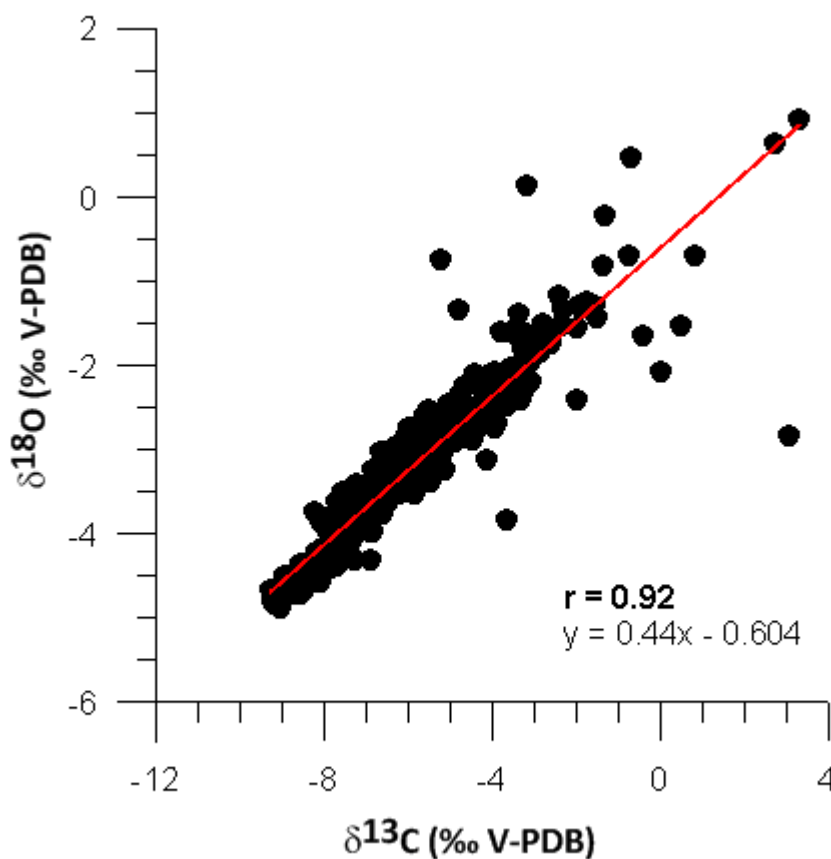
Fig. 6.5 Correlation analysis for \delta^{13}\text{C} and the \delta^{18}\text{O} values obtained from all the De Hoop (BL1, BL3, BL 4) and Klipdrift Shelter (KDS) stalagmites dating to the Late Pleistocene.
