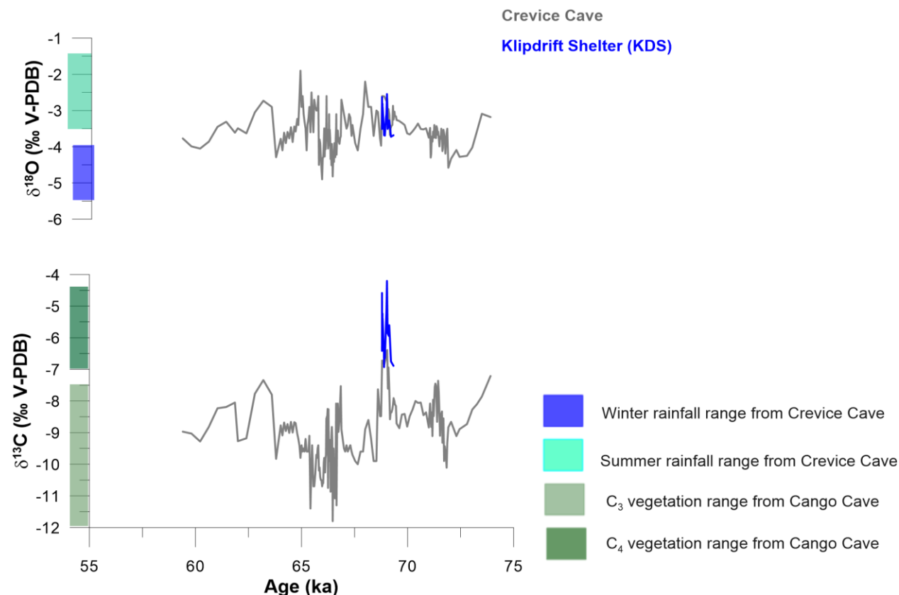
Fig. 6.3 Comparison of the \delta^{13}\text{C} and the \delta^{18}\text{O} data from the Klipdrift Shelter (KDS) stalagmite with published speleothem records from the southern Cape (Crevice Cave) corresponding to MIS 4 (early & late). The raw \delta^{13}\text{C} data are shown. For the BL1 data the raw aragonite corrected \delta^{13}\text{C} data are plotted. Here the data from Pinnacle Point (PP29), Herold's Bay and Sandkraal Cave and Little Karoo data are not included as the author did not have access to the raw data generated for the composite records from these sites. The theoretical range of \delta^{13}\text{C} values for \text{C}_3/\text{CAM} and \text{C}_4 vegetation adopted from Talma and Vogel's (1992) estimates for Cango Cave are highlighted along the bottom y-axis and the theoretical range of \delta^{18}\text{O} values for summer and winter rainfall adopted from Bar-Matthews et al. 's (2010) estimates for Crevice Cave are highlighted along the top y-axis
