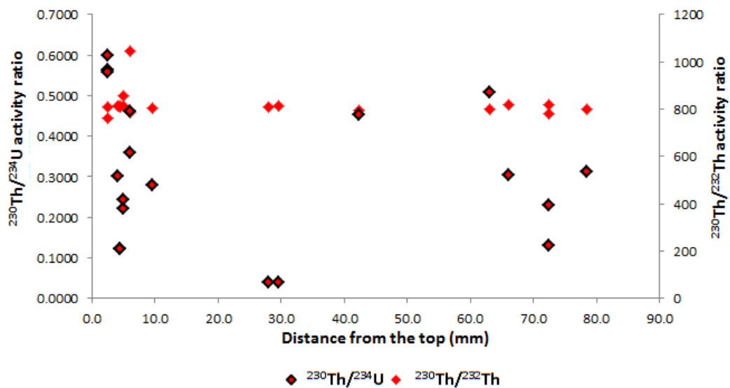
Fig. 5.14 Changes in the ^{230}\text{Th}/^{234}\text{U} and ^{230}\text{Th}/^{232}\text{Th} activity ratios along the length of the KDS stalagmite
