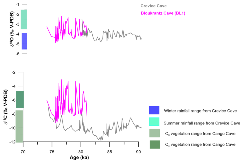
Fig. 6.2 Comparison of the \delta^{13}\text{C} and the \delta^{18}\text{O} data from the De Hoop (BL1) stalagmite with published speleothem records from the southern Cape (Crevice Cave) corresponding to MIS 5a (early & late). The raw \delta^{13}\text{C} data are shown. For the BL1 data the raw aragonite corrected \delta^{13}\text{C} data are plotted. Here the data from Pinnacle Point (PP29), Herold's Bay and Sandkraal Cave and Little Karoo data are not included as the author did not have access to the raw data generated for the composite records from these sites. The theoretical range of \delta^{13}\text{C} values for \text{C}_3/\text{CAM} and \text{C}_4 vegetation adopted from Talma and Vogel's (1992) estimates for Congo Cave are highlighted along the bottom y-axis and the theoretical range of \delta^{18}\text{O} values for summer and winter rainfall adopted from Bar-Matthews et al. 's (2010) estimates for Crevice Cave are highlighted along the top y-axis
