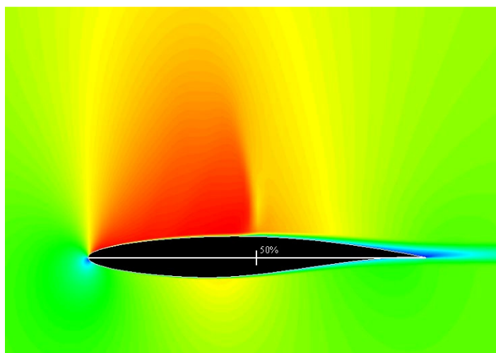
Figure 7.5 Mach 0.73 and 2.79° angle of attack
