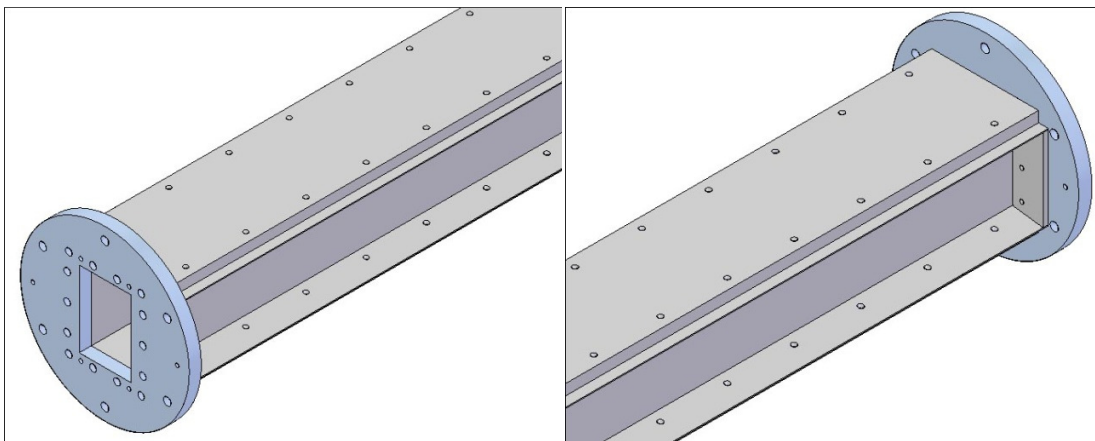
Figure 4.12 Cleanup section with channel sides and plate top and bottom
