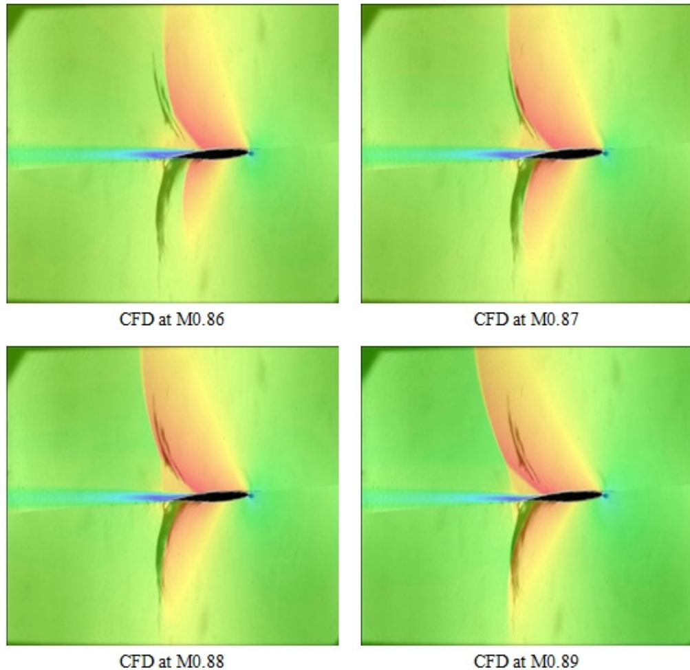
Figure 7.20 Overlay of different CFD Mach numbers onto Mach 0.83 experiment at 2.79° angle of attack
