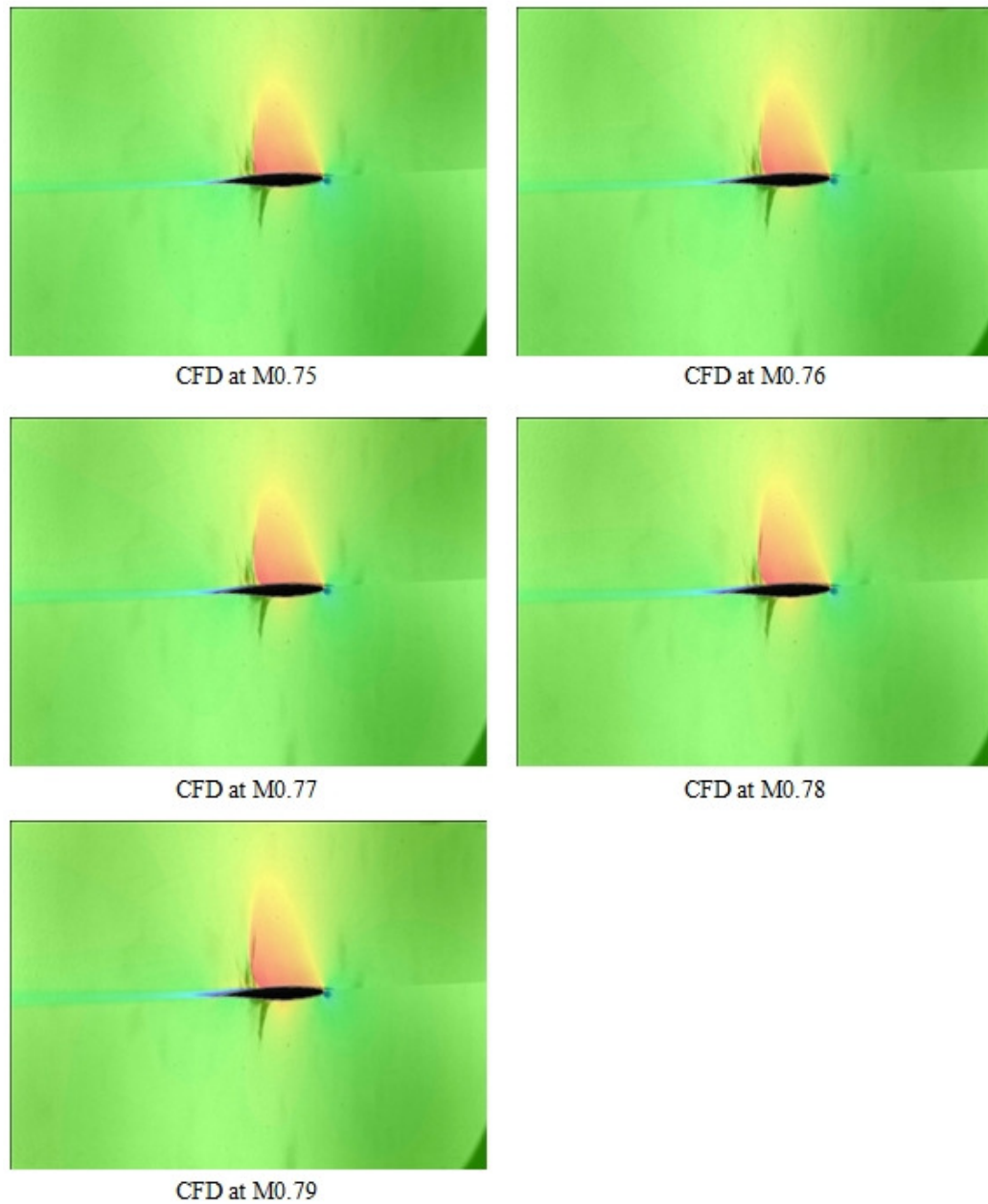
Figure 7.32 Overlay of different CFD Mach numbers onto Mach 0.73 experiment at 2.79^\circ angle of attack
