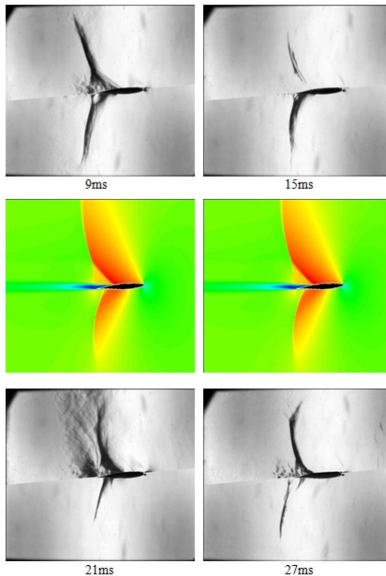
Figure 7.21 CFD at Mach 0.88 compared to experiment at 5° angle of attack
