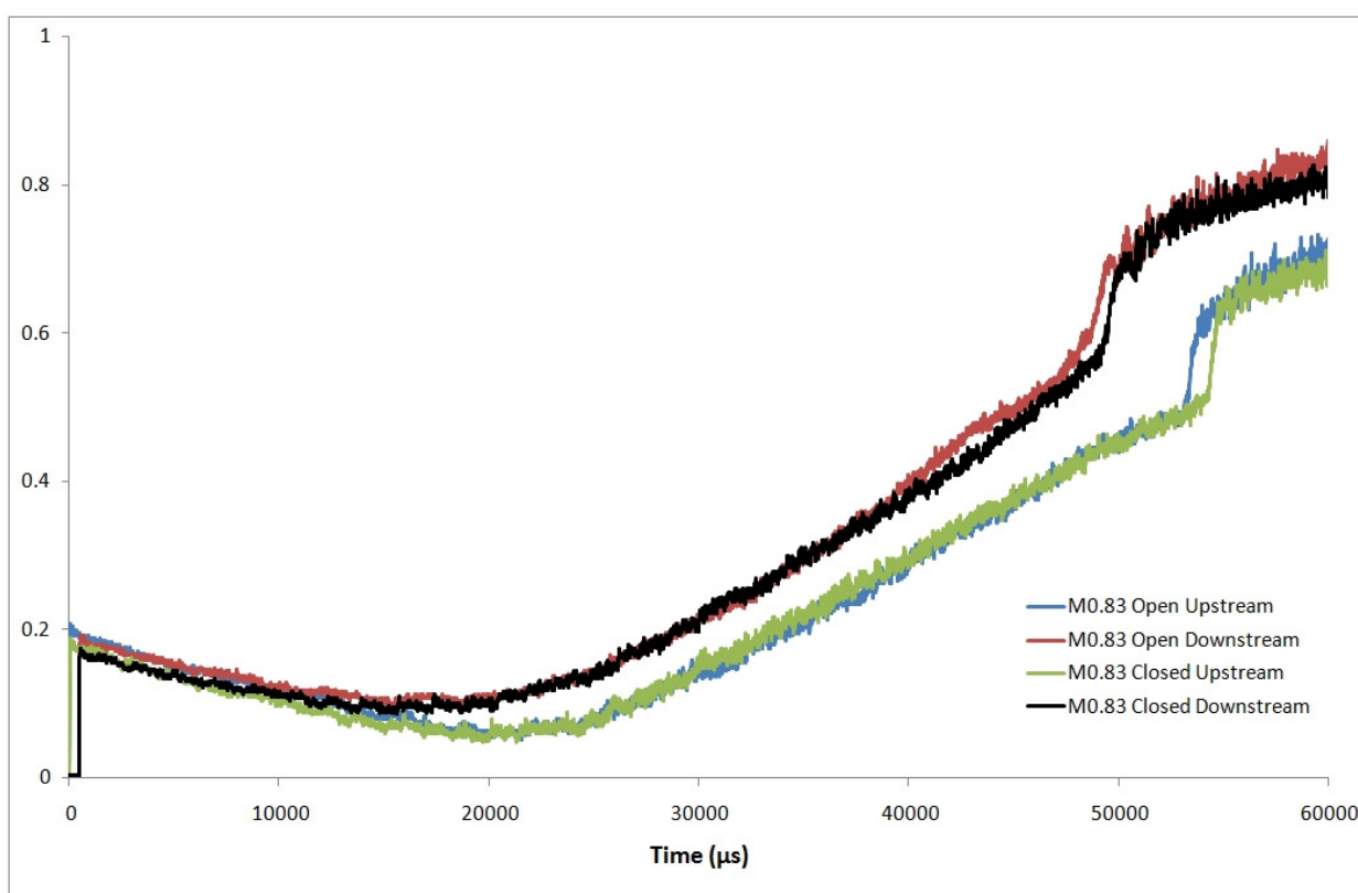
Figure 7.24 Pressure trace at Mach 0.83 and 5° aoa for open and closed walls
