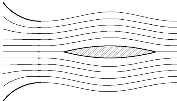
Figure 1.3 Aerofoil in an open-jet wind tunnel
