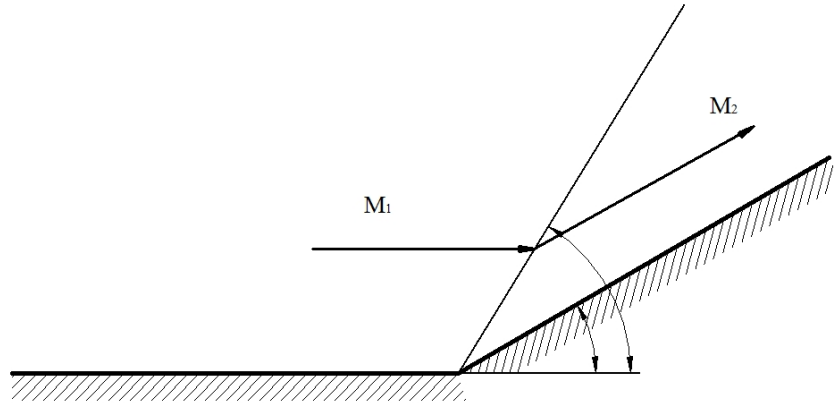
Figure 2.2 Oblique shock wave
