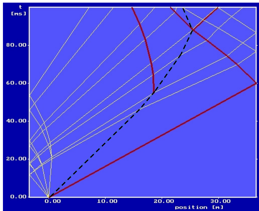
Figure 4.22 3.4 meter driver at a flow Mach number of 0.83
