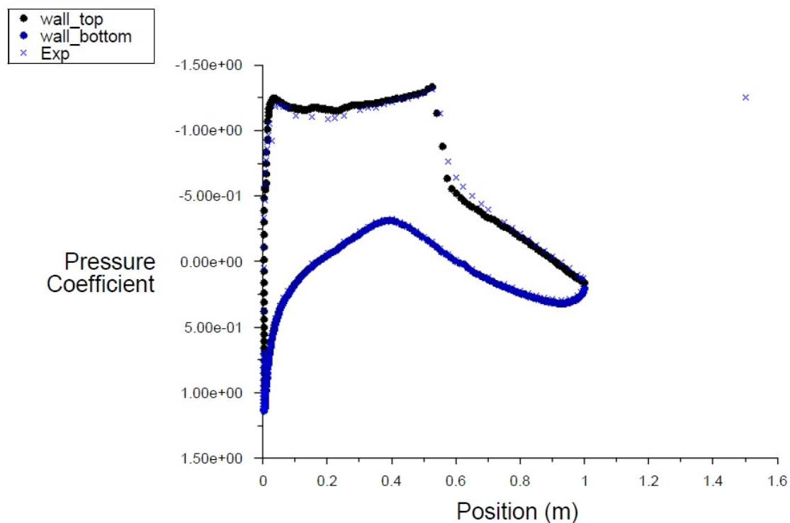
Figure 7.4 Comparison of numerical and experimental pressure coefficient by Fluent (Fluent Inc., 2006)
