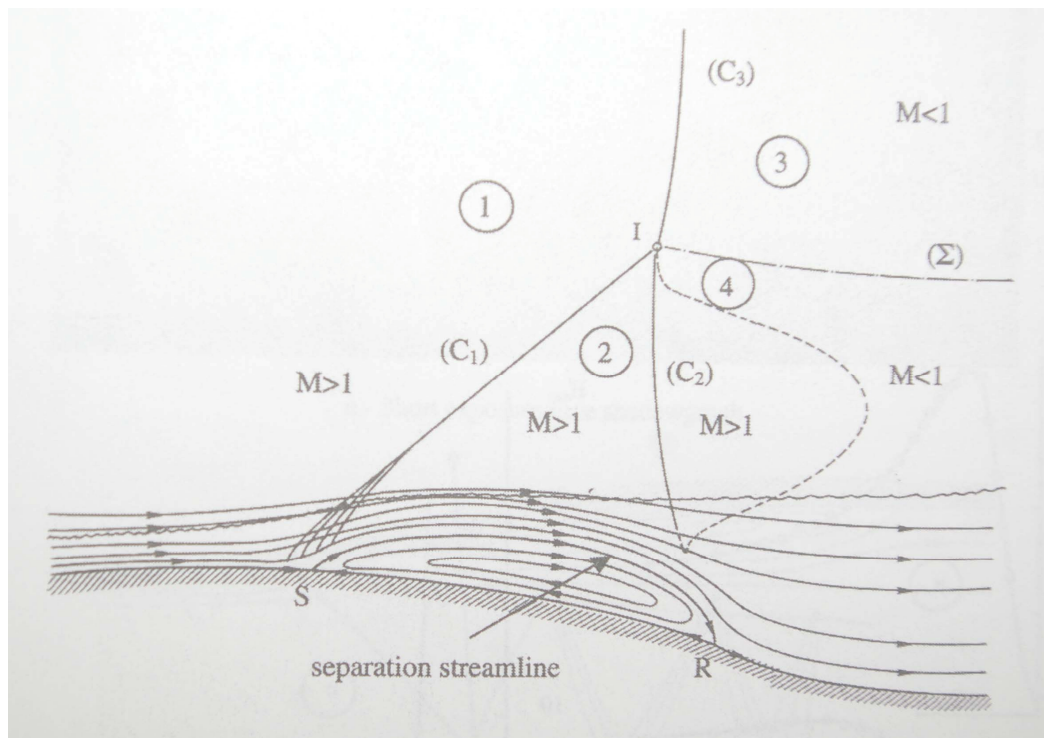
Figure 2.4 Normal shock wave with boundary layer separation (Ben-Dor, Igra, & Elperin, 2001)
