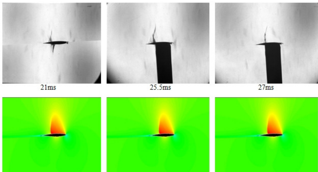
Figure 7.33 CFD at Mach 0.75 compared to experiment at 2.79° angle of attack
