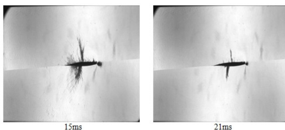
Figure 7.22 Mach 0.83 at 5° angle of attack with closed walls
