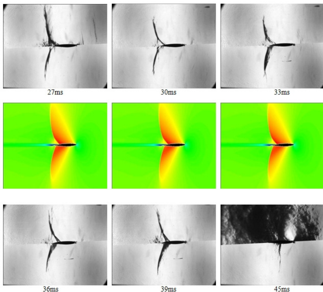
Figure 7.14 CFD at Mach 0.88 compared to experiment at 2.79^\circ angle of attack (27-45ms)
