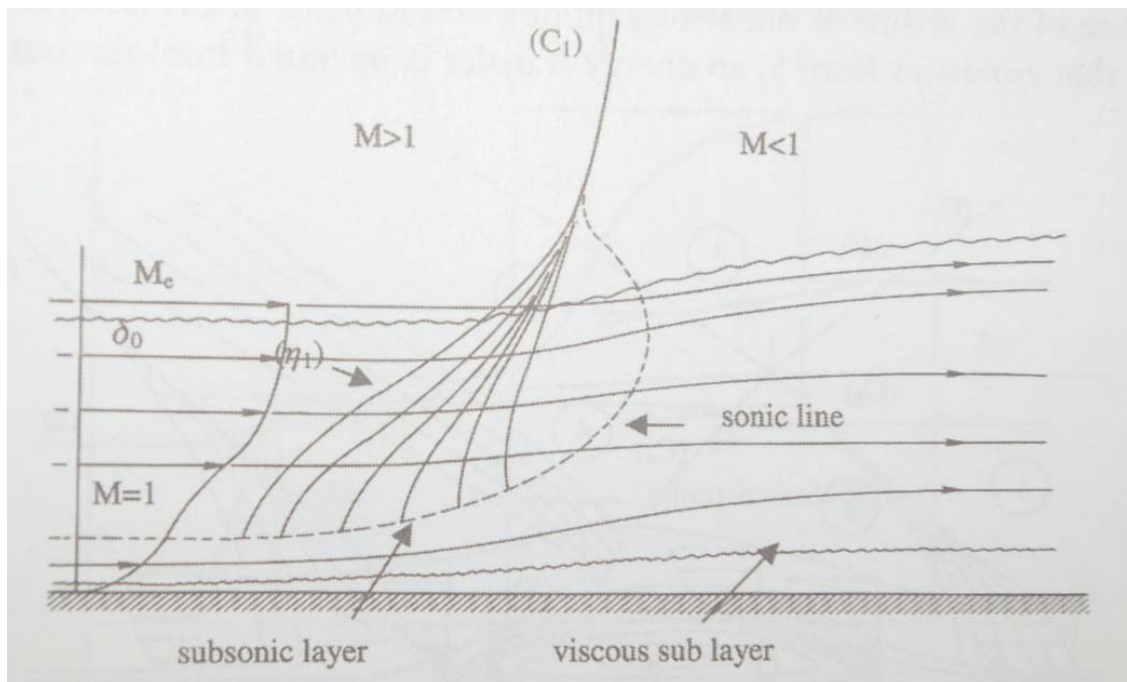
Figure 2.3 Normal shock wave without boundary layer separation (Ben-Dor, Igra, & Elperin, 2001)
