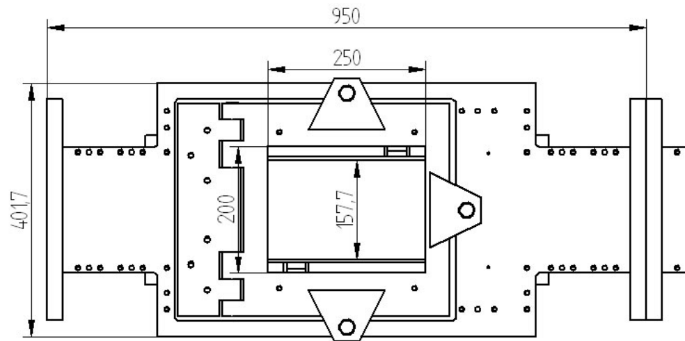
Figure 4.14 Basic dimensions of the final test section
