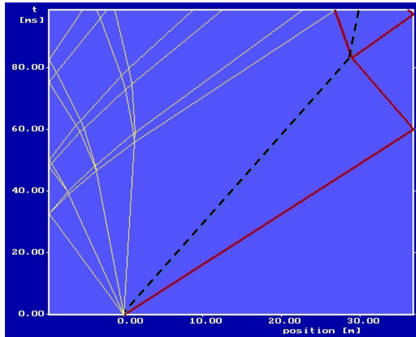
Figure 4.23 9.4 meter driver at a flow Mach number of 0.83
