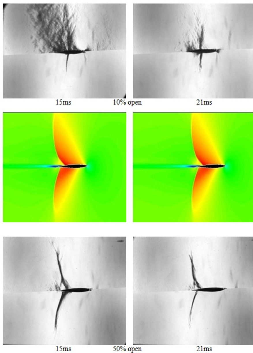
Figure 7.16 Comparison of Mach 0.88 CFD to results at 10% and 50% open wall (5° angle of attack)
