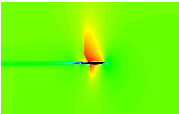
Figure 7.10 CFD at Mach 0.83 and 2.79° angle of attack
