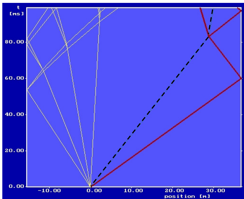
Figure 4.24 15.4 meter driver at a flow Mach number of 0.83
