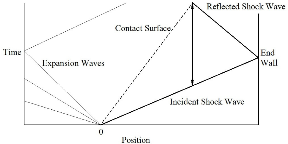
Figure 1.4 Schematic of a typical shock tube wave diagram
