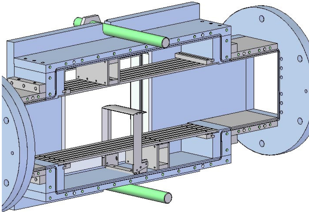
Figure 4.21 Test piece mounted into the test section with 50% open walls
