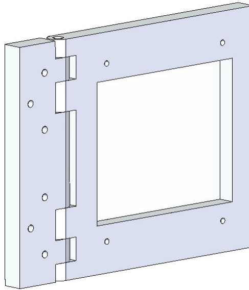
Figure 4.9 Outside view of door frame with hinge system
