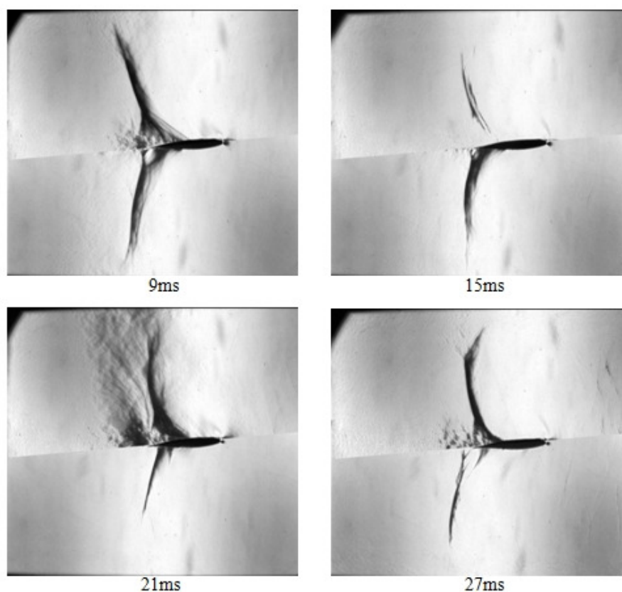
Figure 7.18 Mach 0.83 at 5° angle of attack with open walls
