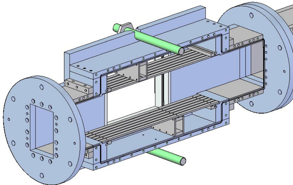
Figure 4.13 Final test section with wall removed for clarity
