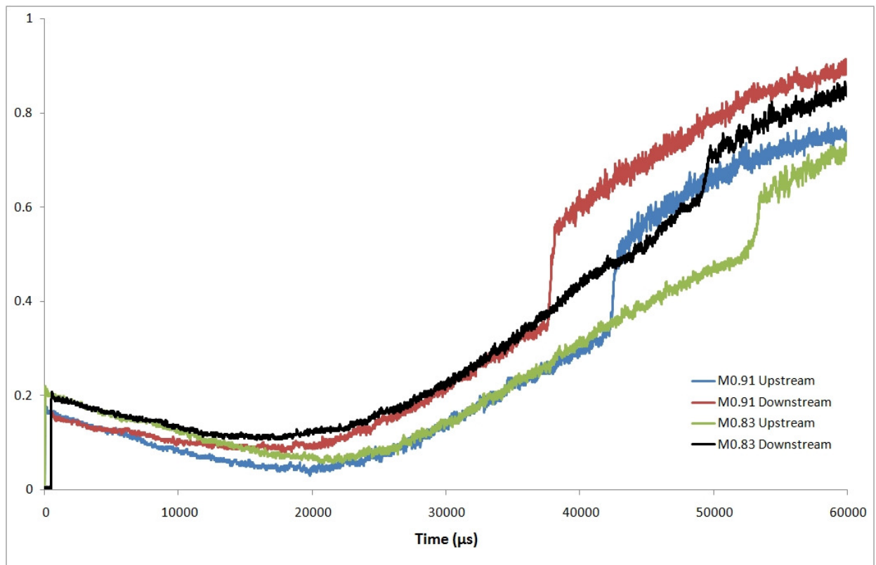
Figure 7.35 Pressure trace overlay for testing at M0.91 and M0.83
