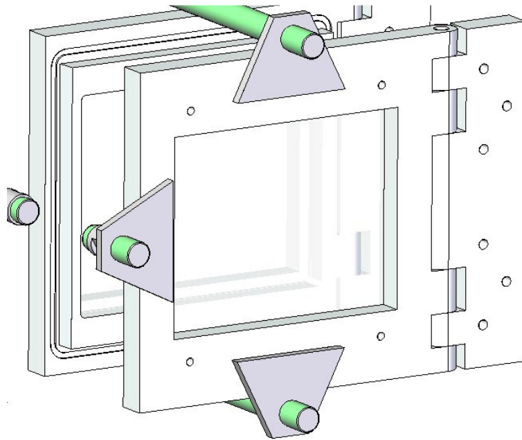
Figure 4.7 Door clamping system
