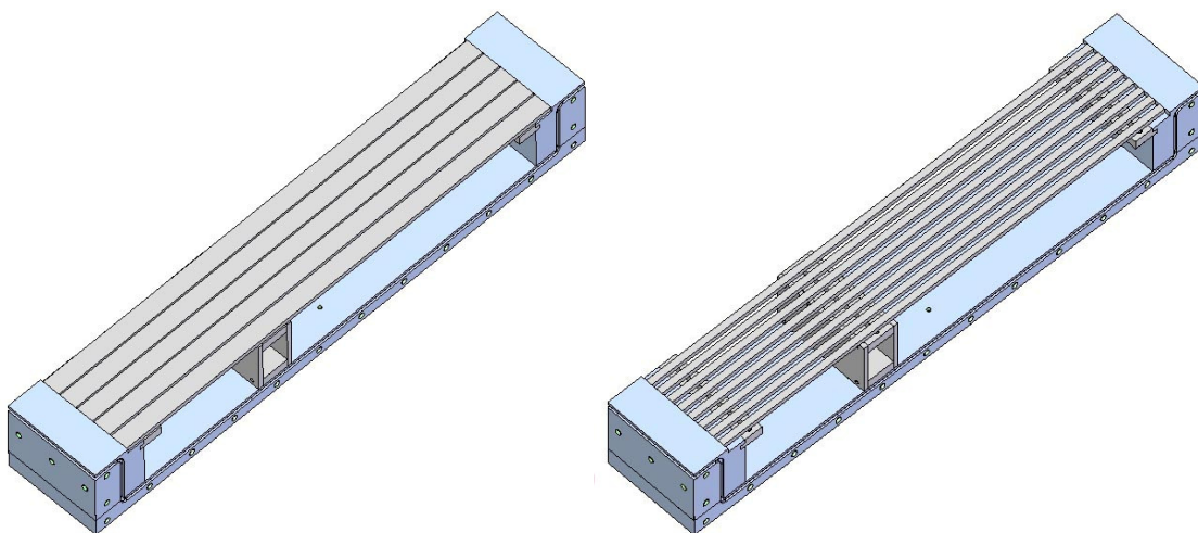
Figure 4.3 Plenum chamber with 10% open and 50% open wall slots
