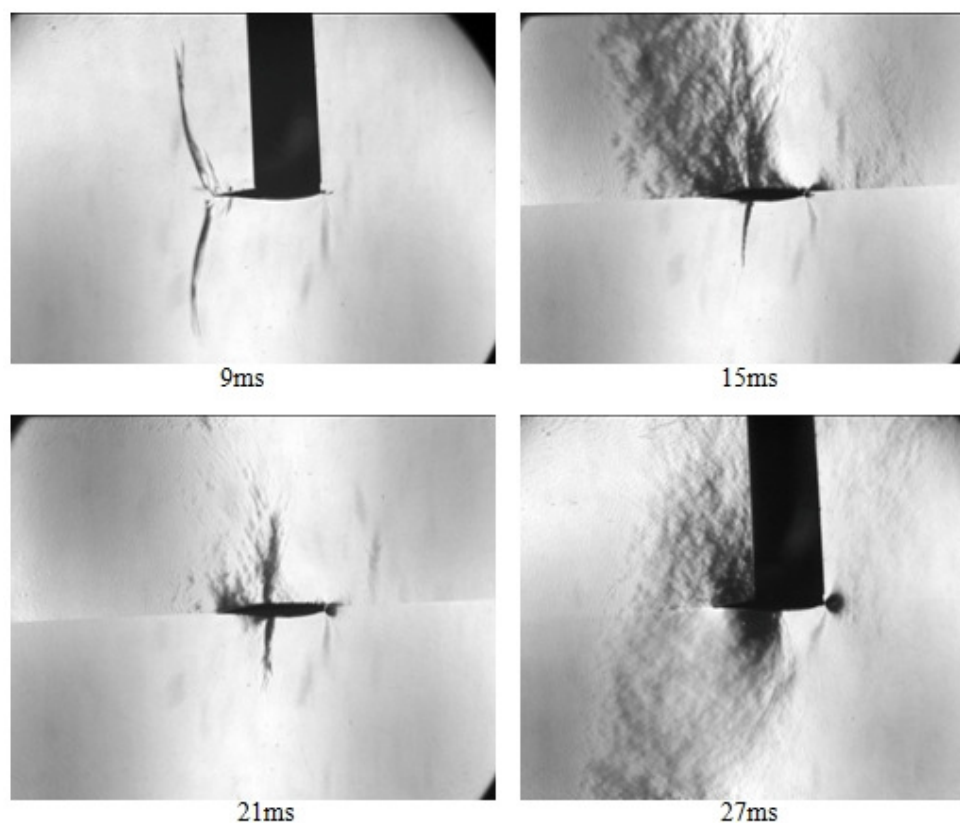
Figure 7.15 Mach 0.83 at 2.79° angle of attack with closed walls
