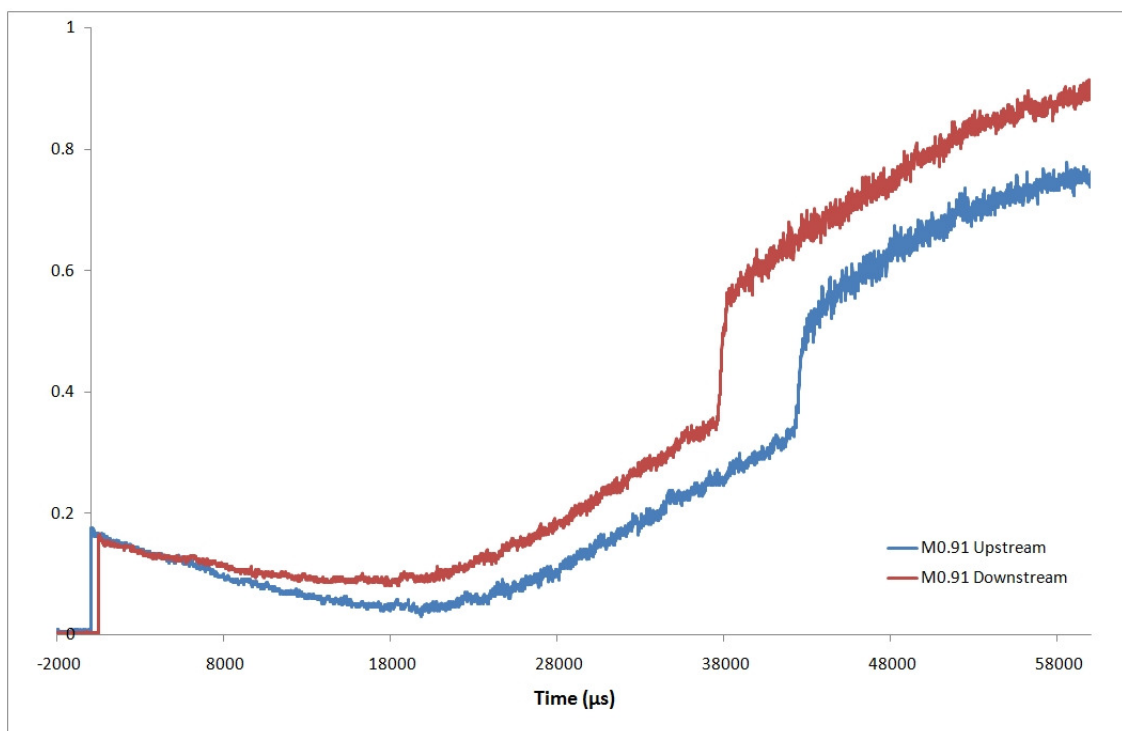
Figure 7.7 Pressure trace produced during testing at Mach 0.91
