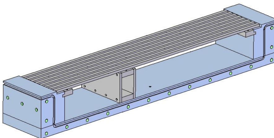
Figure 4.4 Plenum chamber with 50% open walls showing supports
