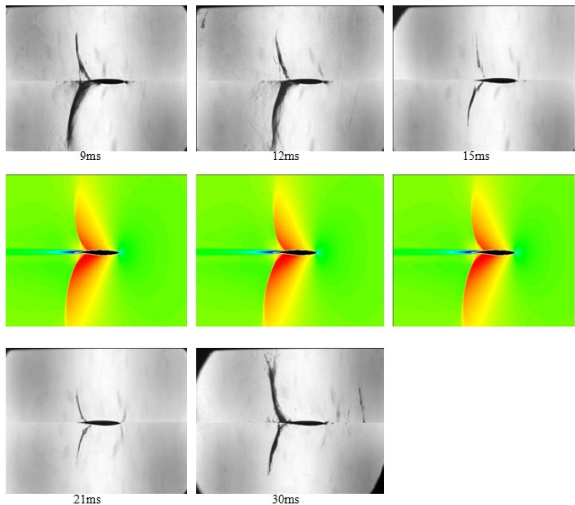
Figure 7.29 CFD at Mach 0.88 compared with experiment at 0^\circ angle of attack
