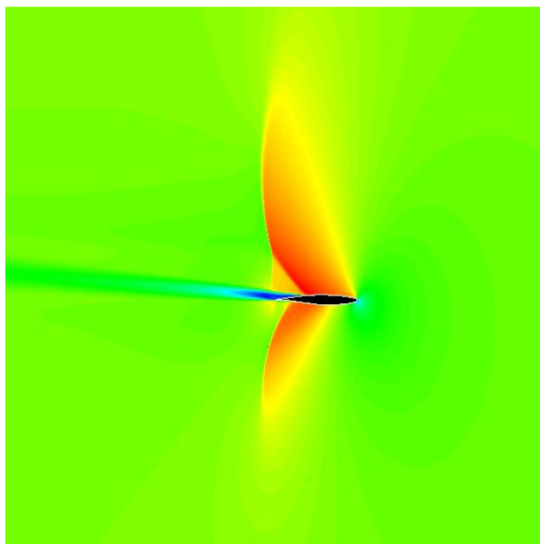
Figure 7.19 CFD at Mach 0.88 and 5° angle of attack
