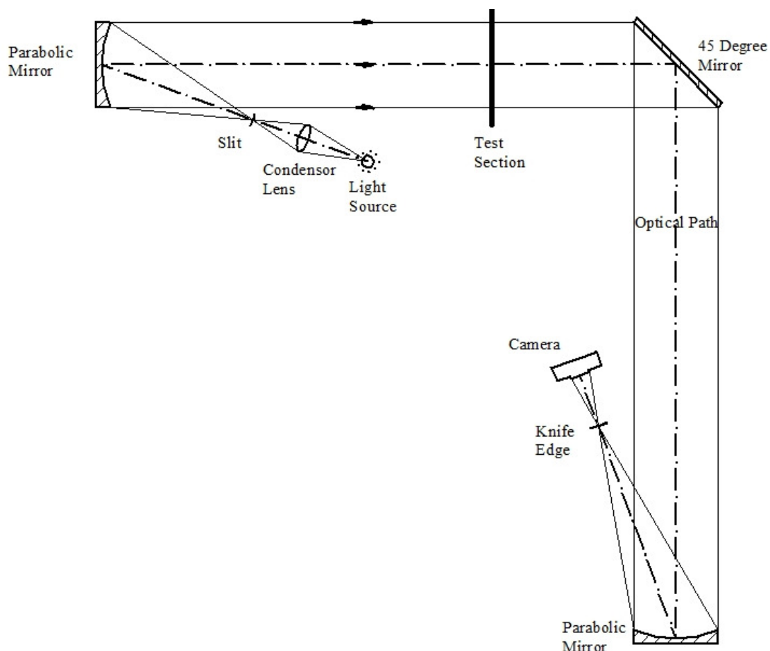
Figure 2.6 Typical Z-shape schlieren system layout bent through 90°
