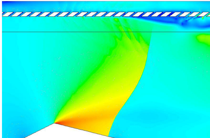
Figure 4.1 CFD of perforated wall concept at Mach 0.83 over half of a diamond shaped aerofoil
