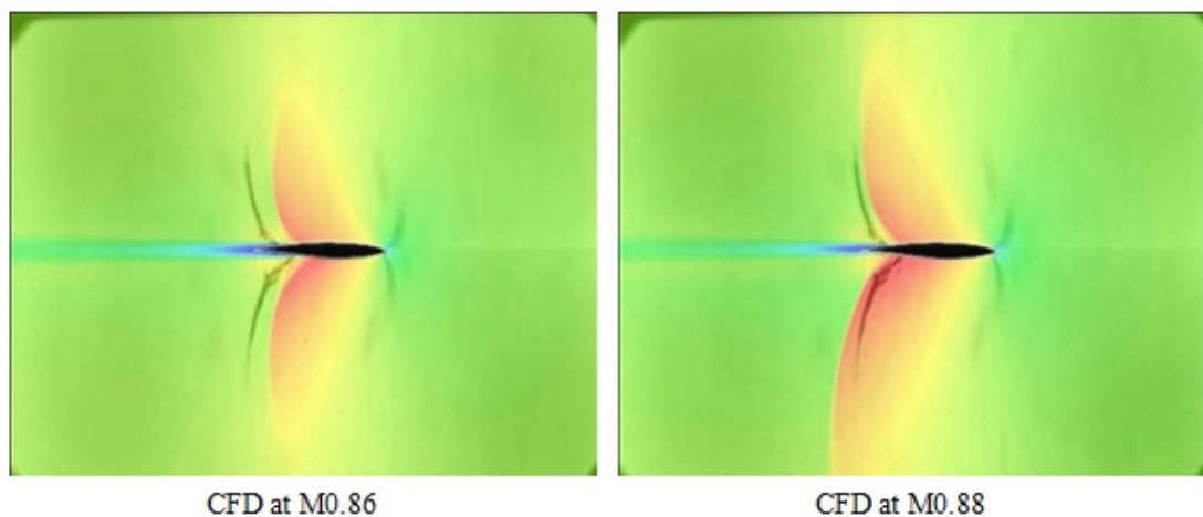
Figure 7.28 Overlay of different CFD Mach numbers onto Mach 0.83 experiment at 0° angle of attack
