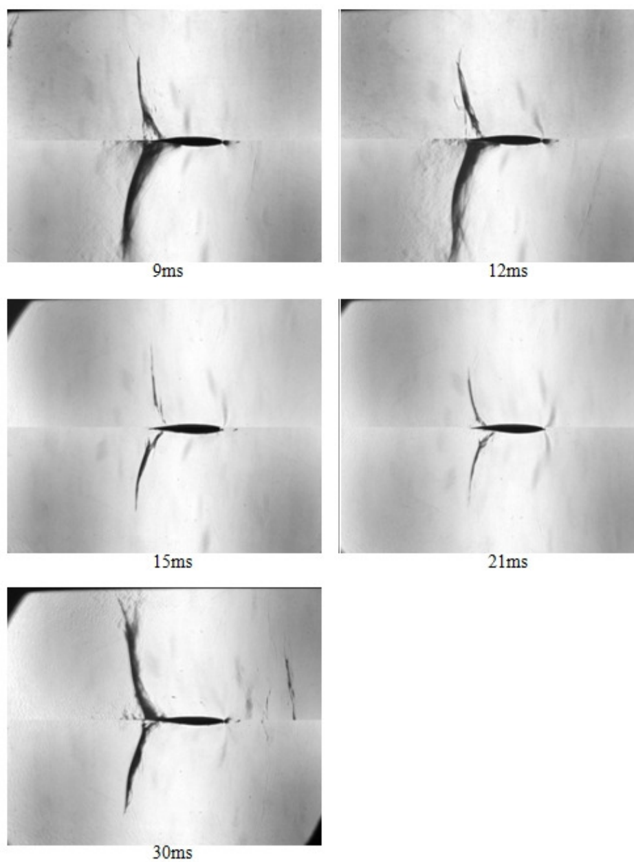
Figure 7.25 Mach 0.83 at 0° angle of attack with open walls
