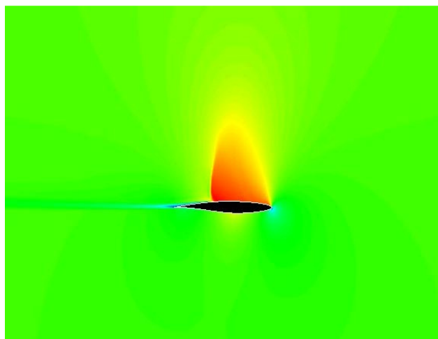
Figure 7.31 CFD at Mach 0.75 and 2.79° angle of attack
