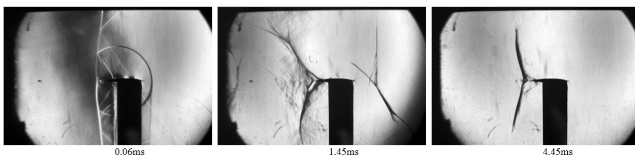
Figure 7.6 Shock tube start-up process
