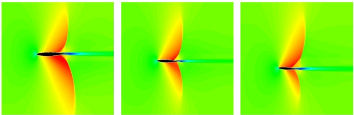
Figure 7.2 CFD at Mach 0.88 at 0^\circ , 2.79^\circ and 5^\circ angle of attack
