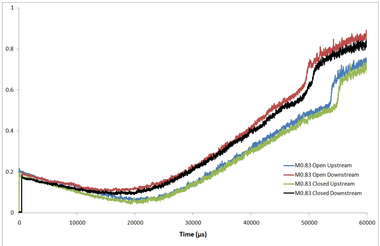
Figure 7.17 Pressure trace at Mach 0.83 and 2.79° angle of attack with open and closed walls
