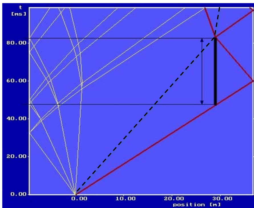
Figure 4.25 Theoretical testing time
