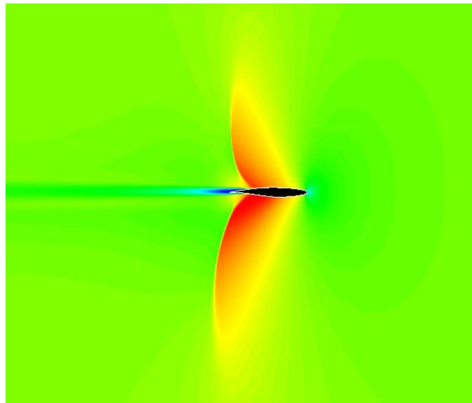
Figure 7.27 CFD at Mach 0.88 and 0° angle of attack
