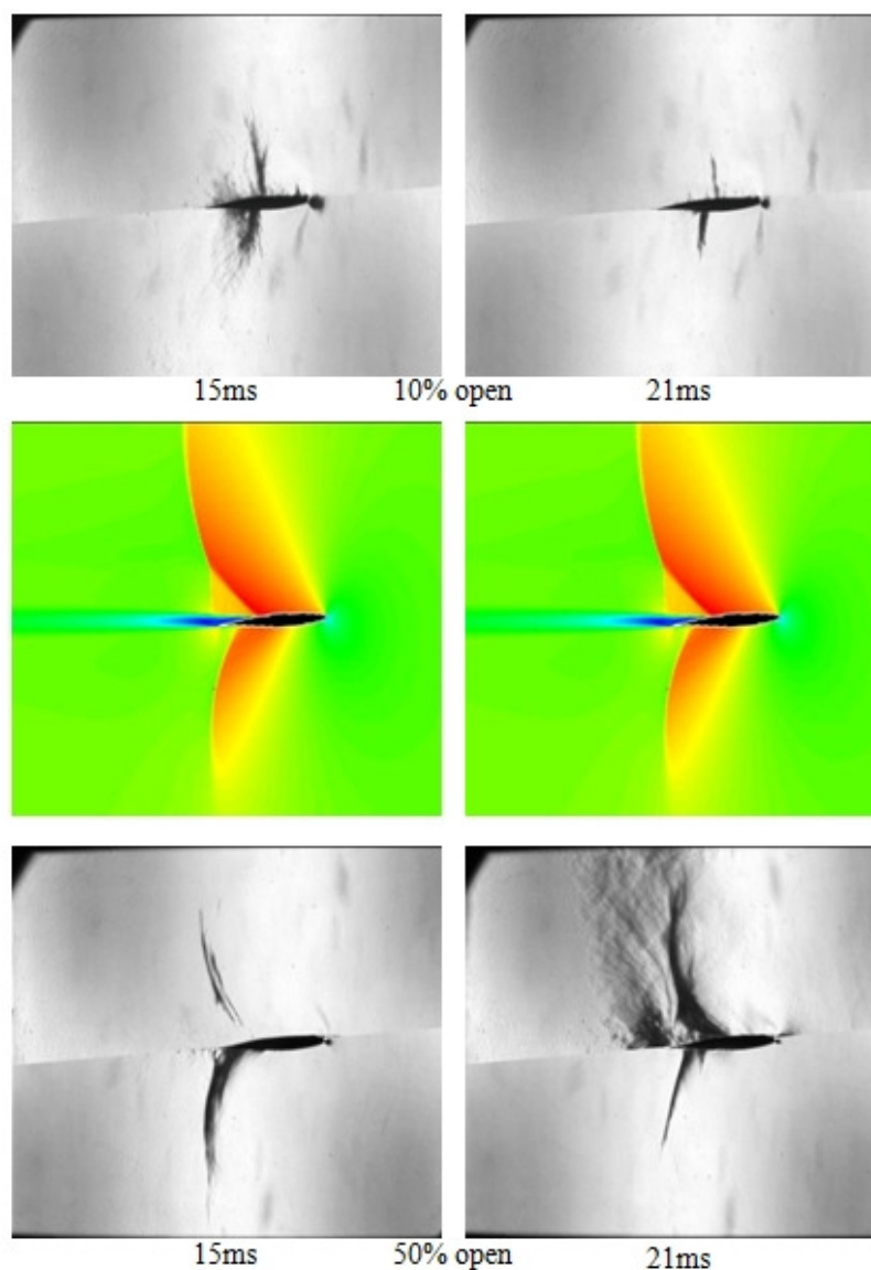
Figure 7.23 Comparison of Mach 0.88 CFD with results at 10% and 50% open wall (5° angle of attack)
