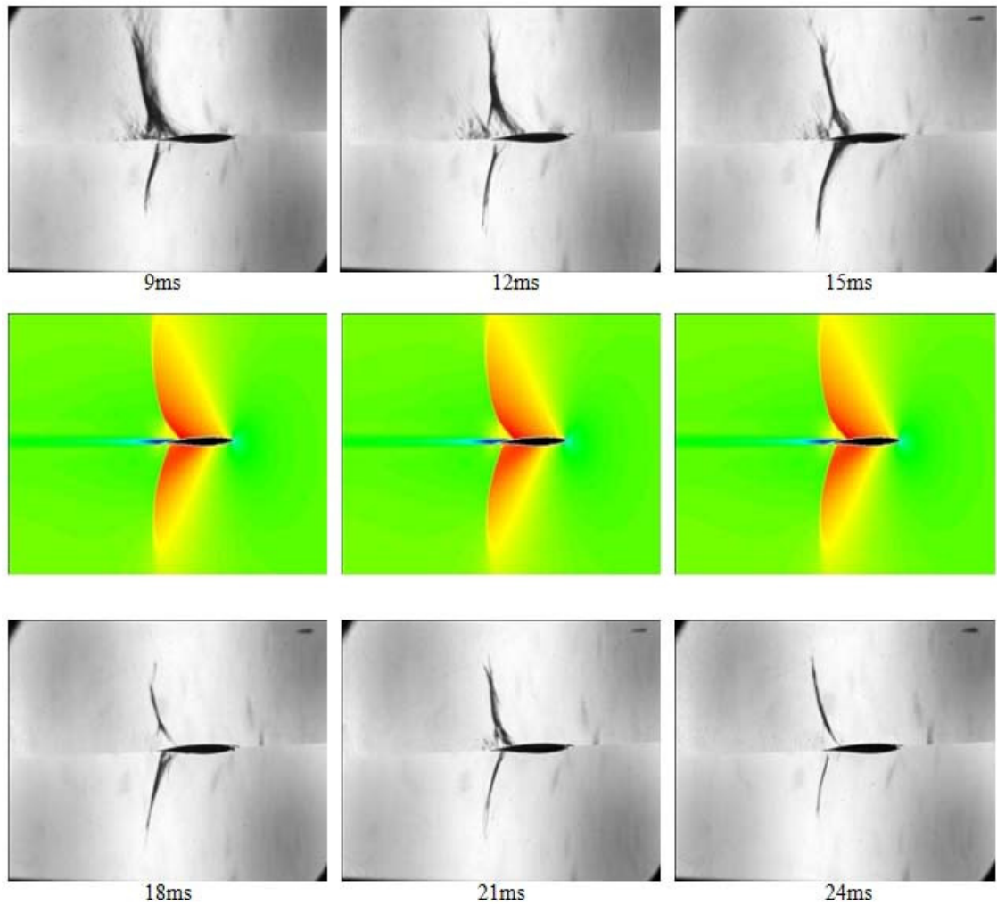
Figure 7.13 CFD at Mach 0.88 compared to experiment at 2.79° angle of attack (9-24ms)
