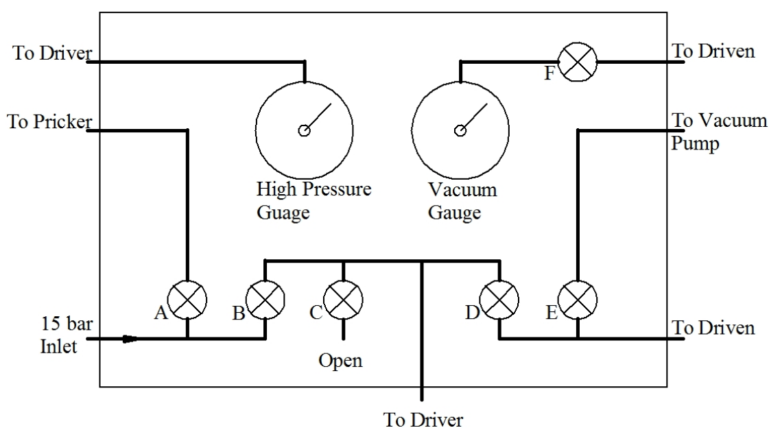
Figure 6.1 Schematic layout of the control board
