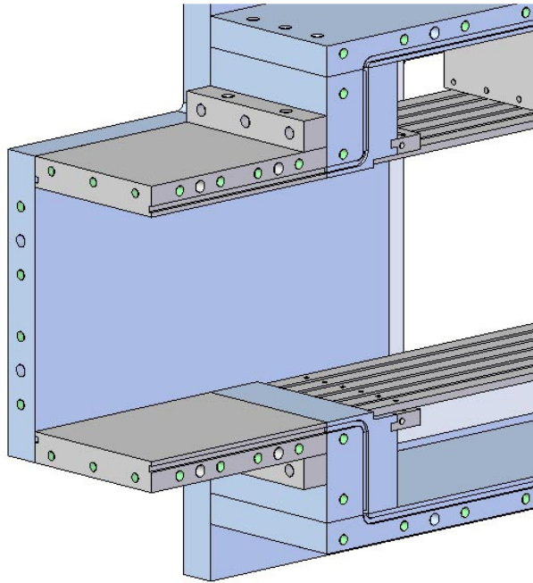
Figure 4.11 O-ring grooves, dowel and bolt holes for alignment and sealing
