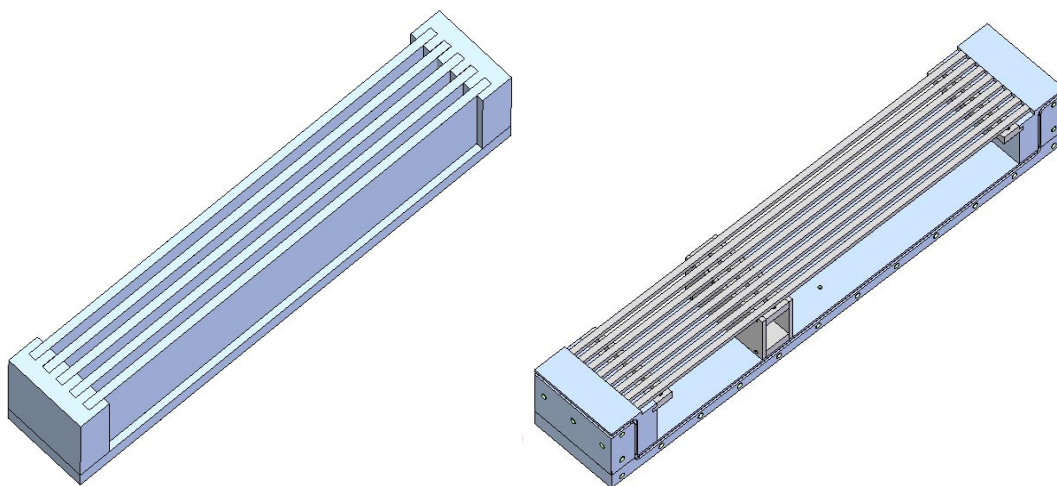
Figure 4.2 Plenum chamber concepts, with solid and bar slots
