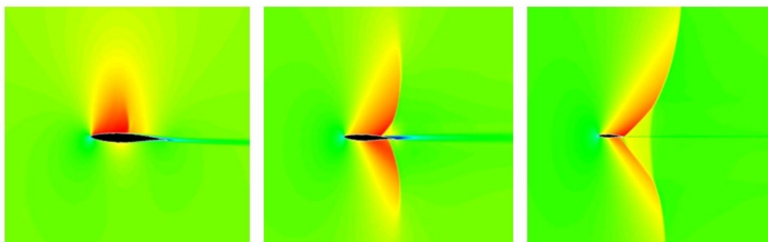
Figure 7.3 CFD at 2.79^\circ at Mach 0.73, 0.83 and 0.93
