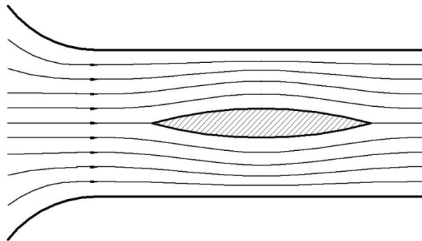
Figure 1.2 Aerofoil in a closed wall wind tunnel
