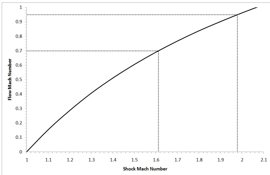
Figure 1.5 Graph of shock Mach number versus flow Mach number
