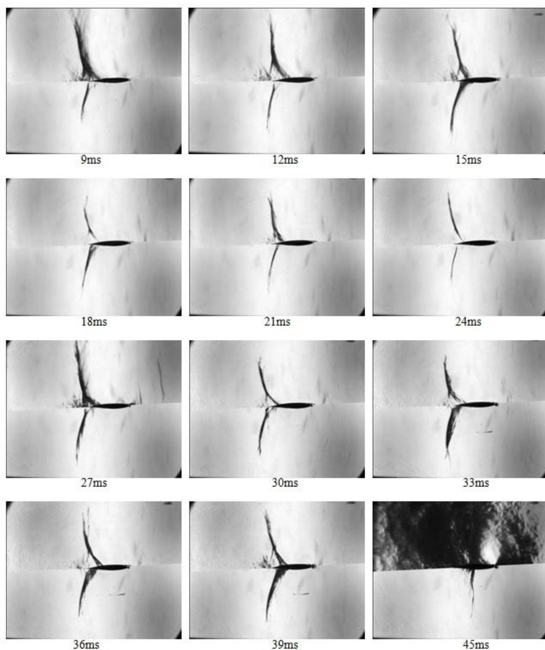
Figure 7.9 Mach 0.83 at 2.79^\circ with open walls
