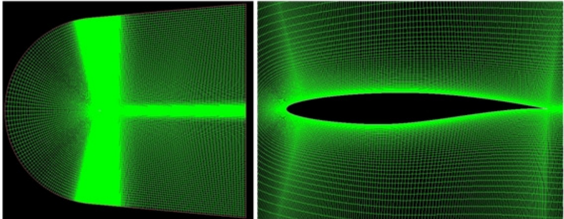
Figure 7.1 Layout of mesh
