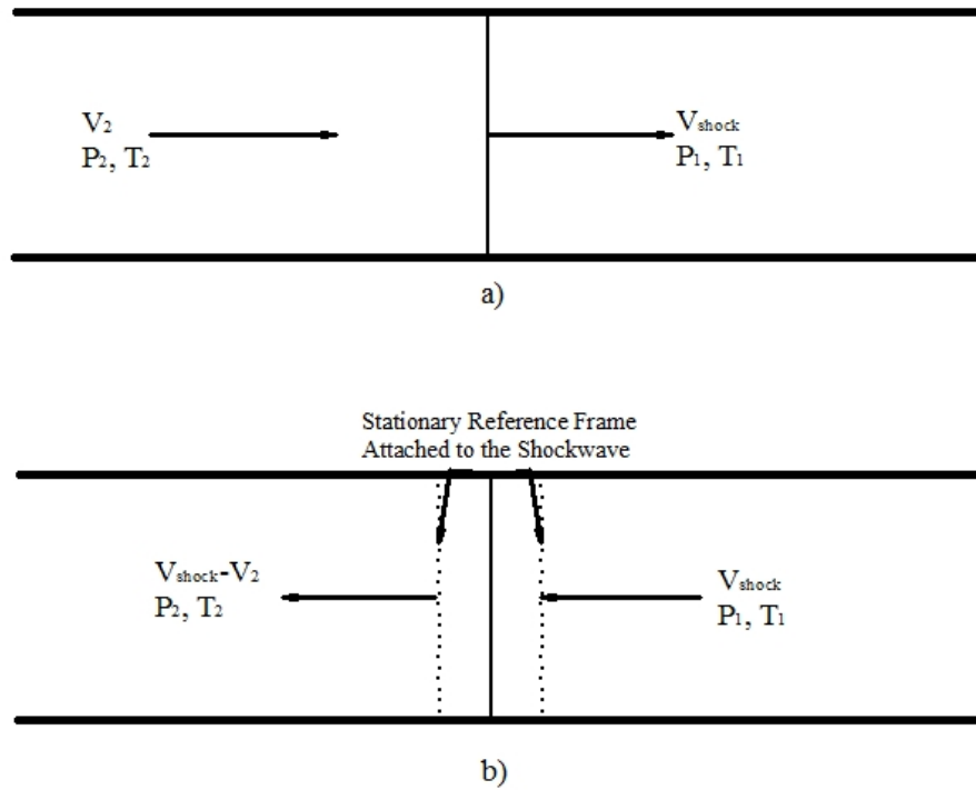
Figure 2.1 Normal shock wave with different reference frames
