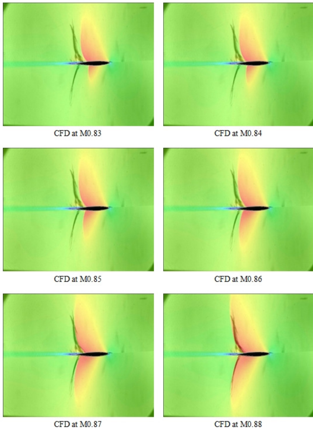
Figure 7.12 Overlay of different CFD Mach numbers onto Mach 0.83 experiment at 2.79^\circ angle of attack
