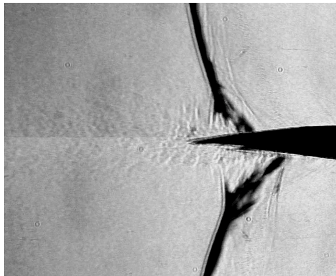
Figure 7.26 High contrast image showing wake region and lambda shock systems
