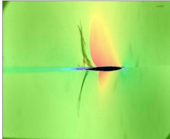
Figure 7.11 CFD Mach 0.83 overlaid onto experimental Mach 0.83
