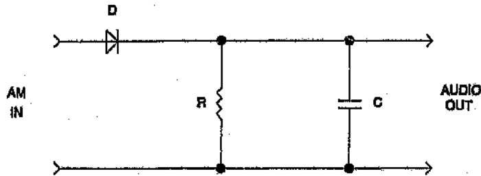
FIGURE 2.1 : ENVELOPE DETECTOR
