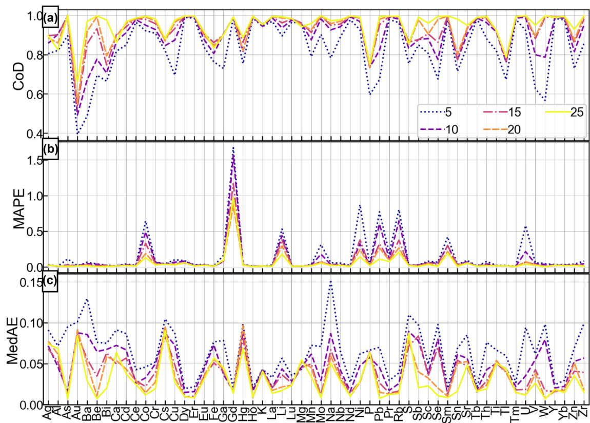
Figure 13. Image domain metric scores for the 2016 re-analyzed dataset in Labrador, for each element as a function of the coding layer size (from 5 to 25 in intervals of 5 as assessed using the (a) CoD, (b) MAPE, and (c) MedAE metrics.
