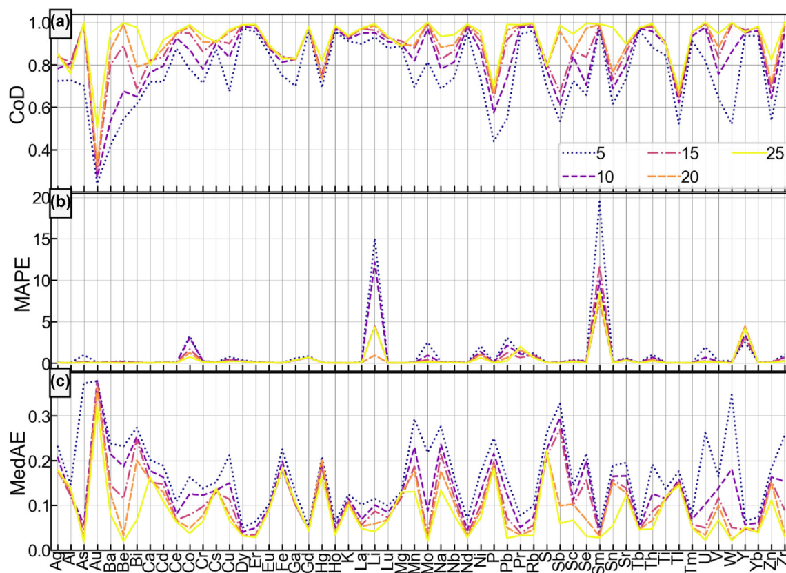
Figure 5. Autoencoder performance for coding layer sizes from 5 to 25 in intervals of 5, as assessed using the (a) CoD, (b) MAPE, and (c) MedAE metrics.
