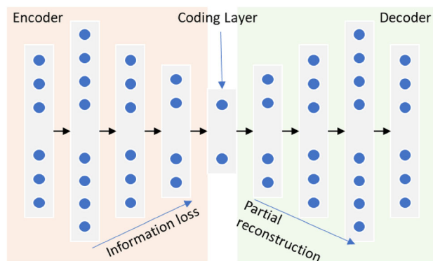
Figure 4. Network architecture of an autoencoder, featuring the encoder, coding layer and decoder sections. Through progressive lossy encoding, information is lost and only the most salient information is reconstructed.
