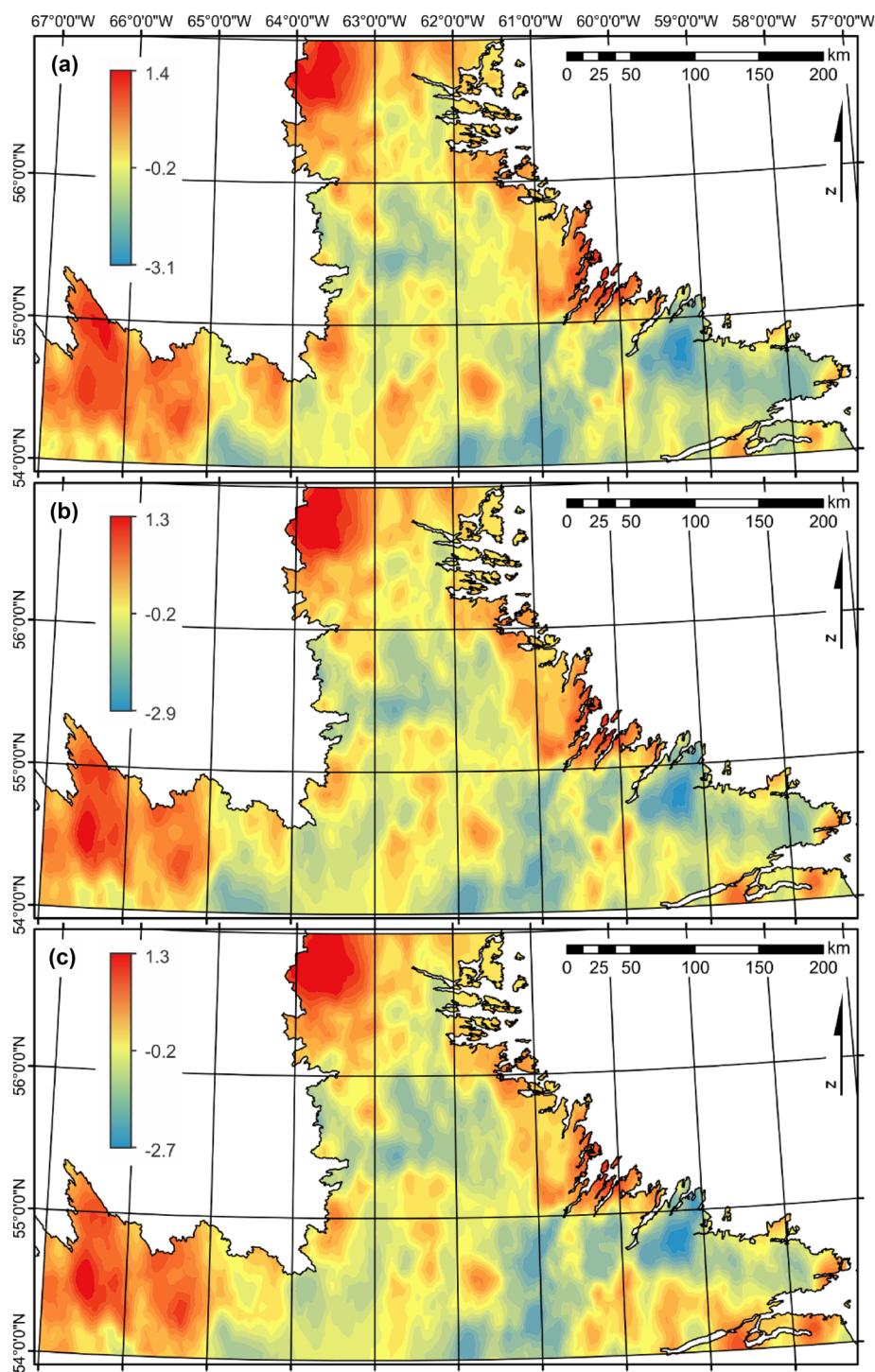
Figure 11. Spatial interpolation maps of lithium using the original Labrador dataset (Fig. 2c) in (a). Average of predicted (or reconstructed) data using hidden layer sizes of 13 in (b) and 5 in (c). The interpolation method used here was simple kriging. Hyperparameters for (a) were nugget = 0.64, sill = 0.25, range = 0.97 km, using the stable model (similar for b and c). Values correspond to CLR-transformed ppm.
