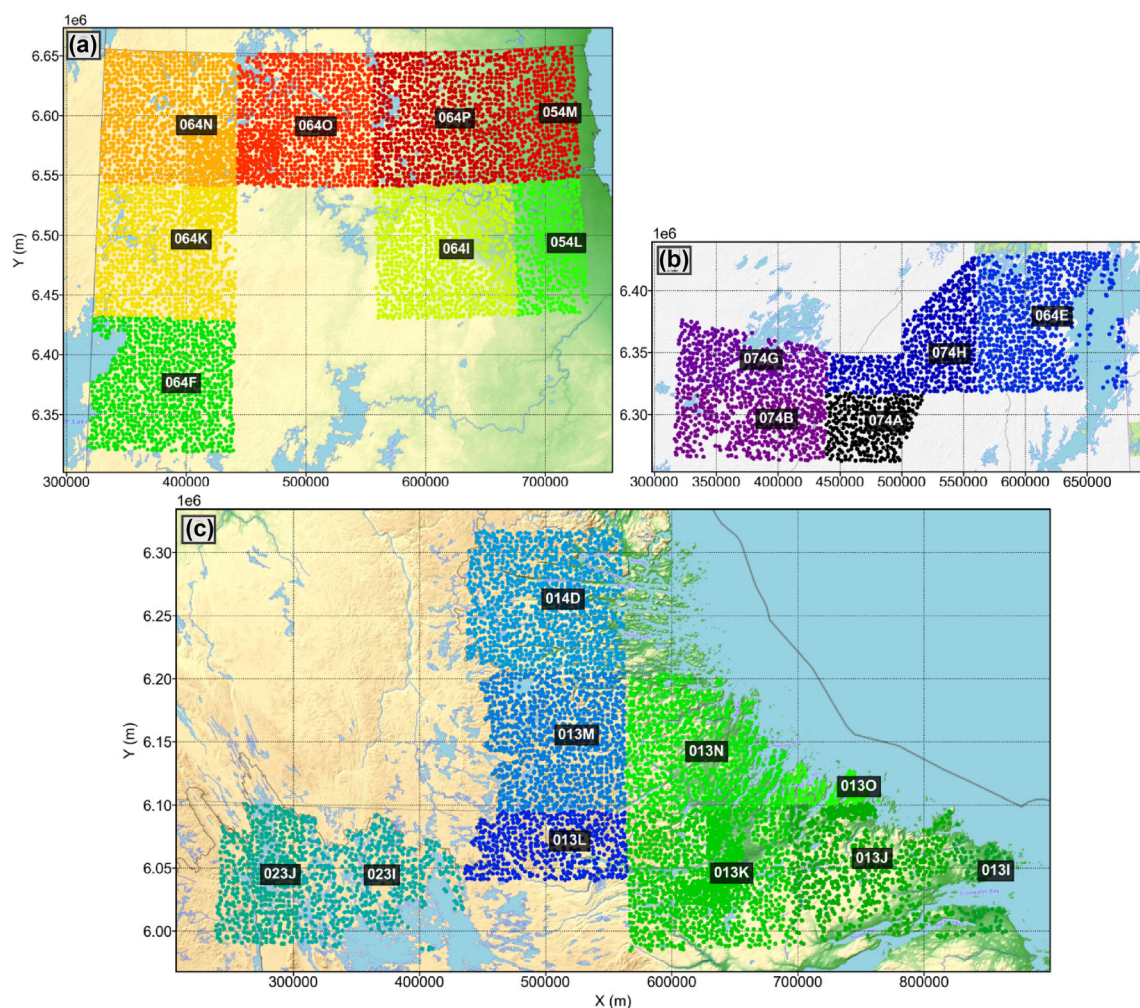
Figure 2. Detailed sample locations in (a) Manitoba, (b) Saskatchewan and (c) Labrador. The positions of the samples within Canada are presented in Figure 1.
