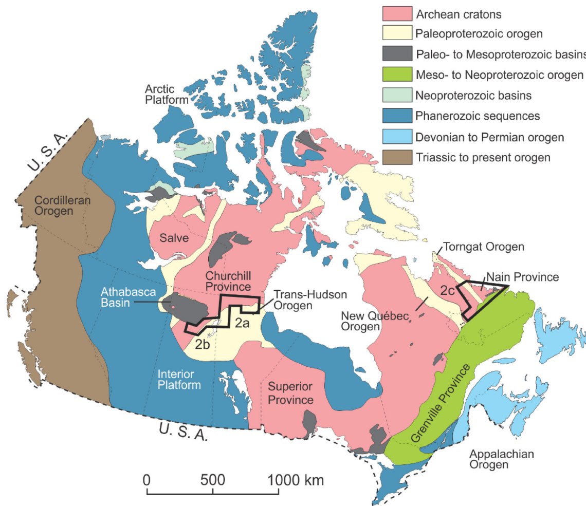
Figure 1. Simplified geological map of Canada with the location of the datasets in Manitoba, Labrador and Saskatchewan (black polygons). Detailed sample distributions, here labeled 2a, b and c, are presented in Figures 2a, b and c, respectively. Image taken and modified from Zhang et al. (2022).
