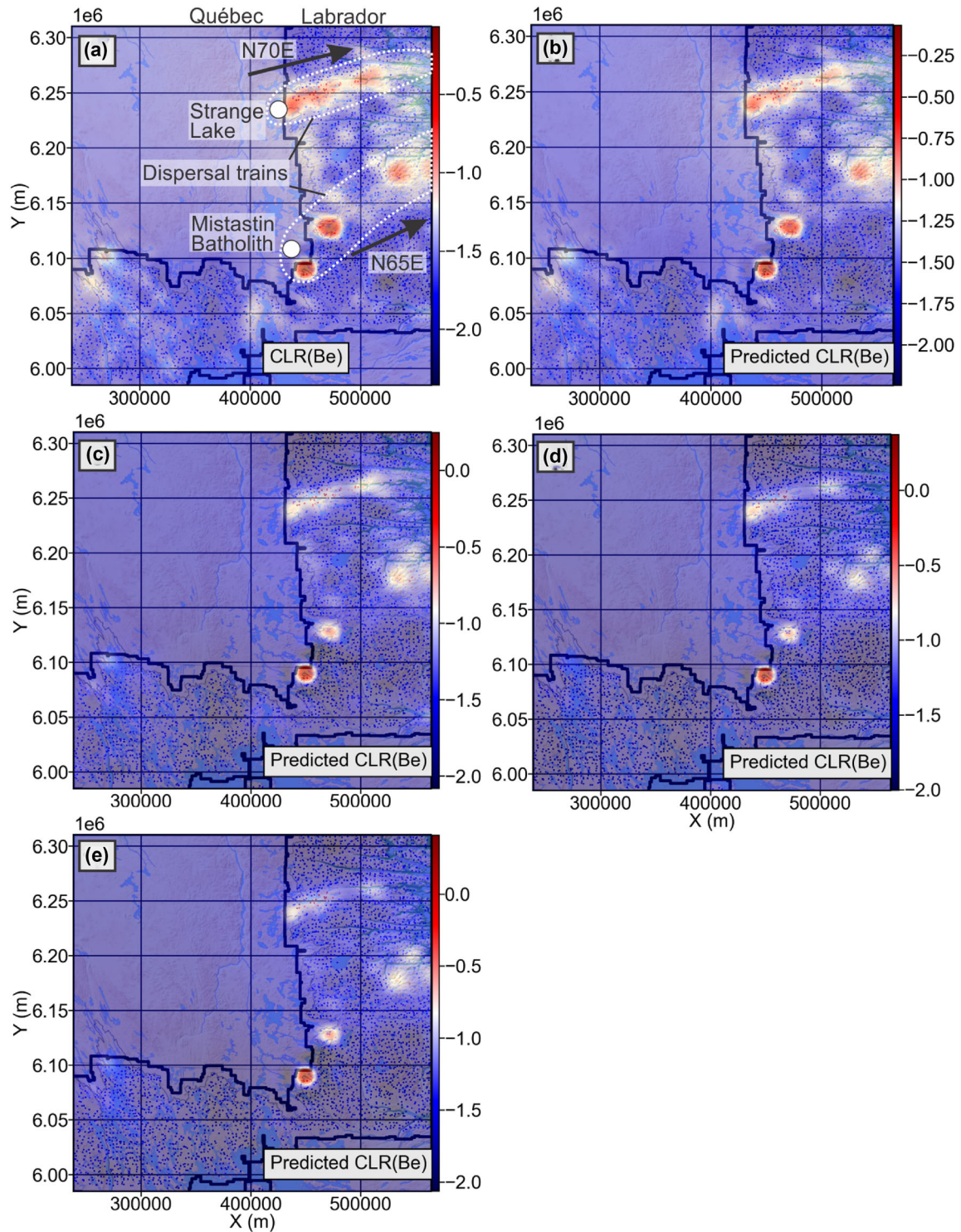
Figure 9. Maps of the original data for Be in the 2016 re-analyzed dataset in Labrador (Fig. 2a) in (a), average of predicted (or reconstructed) data using hidden layer sizes of 16 in (b), 13 in (c), 9 in (d) and 5 in (e). The black arrow in (a) corresponds to the direction of glacial dispersal trains or eskers.
