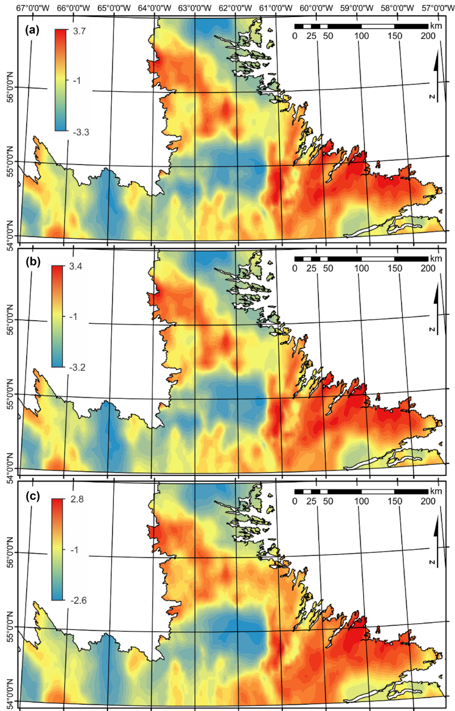
Figure 12. Spatial interpolation maps of uranium using the original Labrador dataset (Fig. 2c) in (a). Average of predicted (or reconstructed) data using hidden layer sizes of 13 in (b) and 5 in (c). The interpolation method used here was simple kriging. Hyperparameters for (a) were nugget = 0.35, sill = 0.66, range = 1.40 km, using the stable model (similar for (b) and (c)). Values correspond to CLR-transformed ppm.
