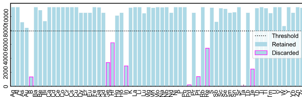
Figure 3. Abundance of non-empty records per element in the dataset (65 elements total). Data for elements that do not meet the threshold (30% missing values) were discarded.
