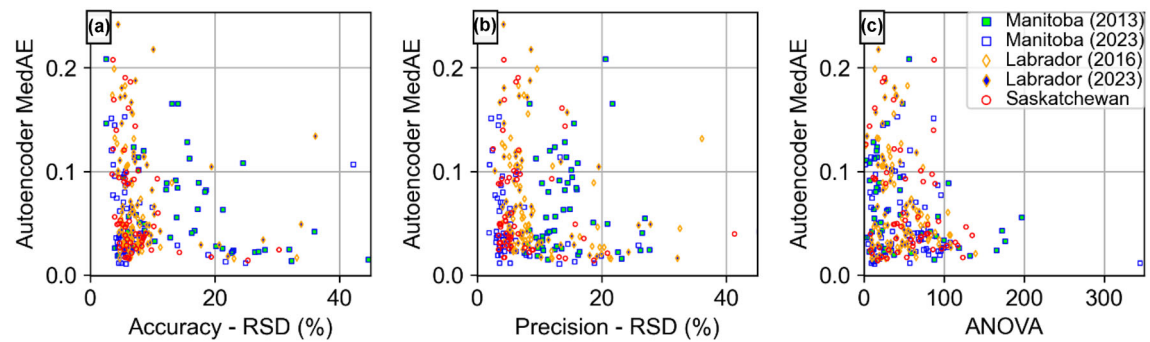
Figure 14. Performance of the autoencoder as measured using the MedAE metric versus (a) the accuracy of the input data, (b) precision of the input data, and the (c) F-statistic of the ANOVA of the input data. The label Manitoba 2013 also includes the dataset from 2010.
