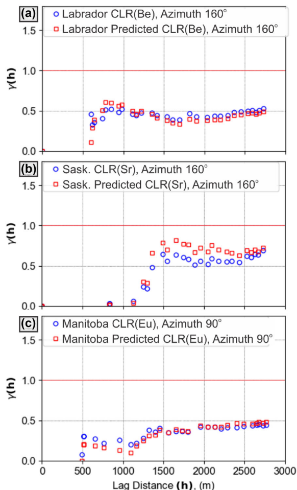
Figure 6. Variograms of (a) Be in Labrador, (b) Sr in Saskatchewan (Sask), and (c) Eu in Manitoba.
