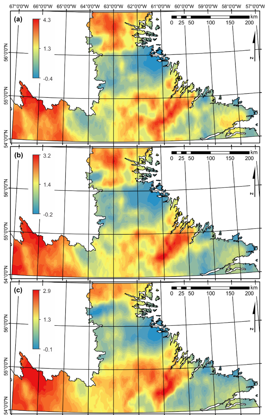
Figure 10. Spatial interpolation maps of copper using the original Labrador dataset (Fig. 2c) in (a). Average of predicted (or reconstructed) data using hidden layer sizes of 13 in (b) and 5 in (c). The interpolation method used here was simple kriging. Hyperparameters for (a) were nugget = 0.59, sill = 0.45, range = 1.48 km, using the stable model (similar for (b) and (c)). Values correspond to CLR-transformed ppm.
