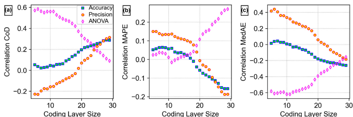
Figure 15. Spearman rank correlation coefficient between the autoencoder performance as assessed using the (a) CoD, (b) MAPE and (c) MedAE metrics, and data quality metrics versus the coding layer size.
