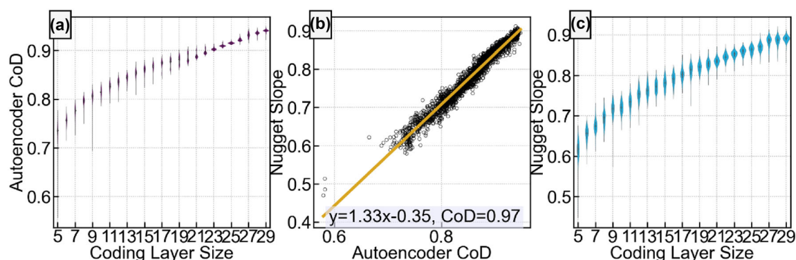
Figure 8. Effect of (a) the coding layer size on the autoencoder's performance as measured by the CoD metric, (b) the relationship between the nugget slope and the autoencoder's performance, and (c) the relationship between the nugget slope and the coding layer size.
