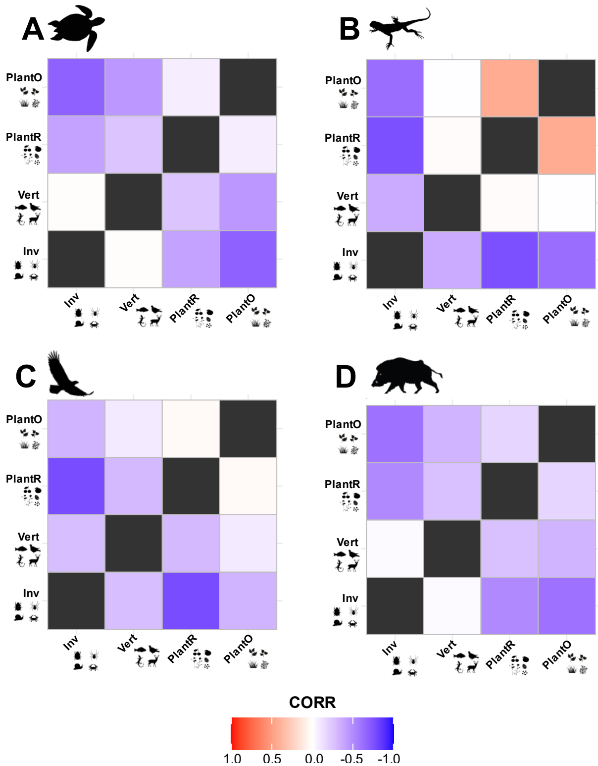
Figure 9: Correlation matrices between the second-order subdivisions in the dietary data (Inv, Vert, PlantR, PlantO) for turtles (A), lizards (B), birds (C), and mammals (D). Corr - correlation scale between two variables ranging from perfect correlation (1.0) to perfect negative correlation (-1.0).
