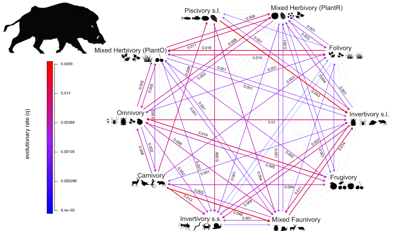
Figure 29: Rates of evolutionary between dietary guilds (k-means cluster analysis) in mammals (node-dating backbone topology) recovered by the Mk marginal maximum likelihood analysis ("all rates different" model - ARD). Only transition rates > 0.001 are shown. Direction of arrows indicates "from state - to state". Abbreviations: PlantO, vegetative plant structures; PlantR, reproductive plant structures.
