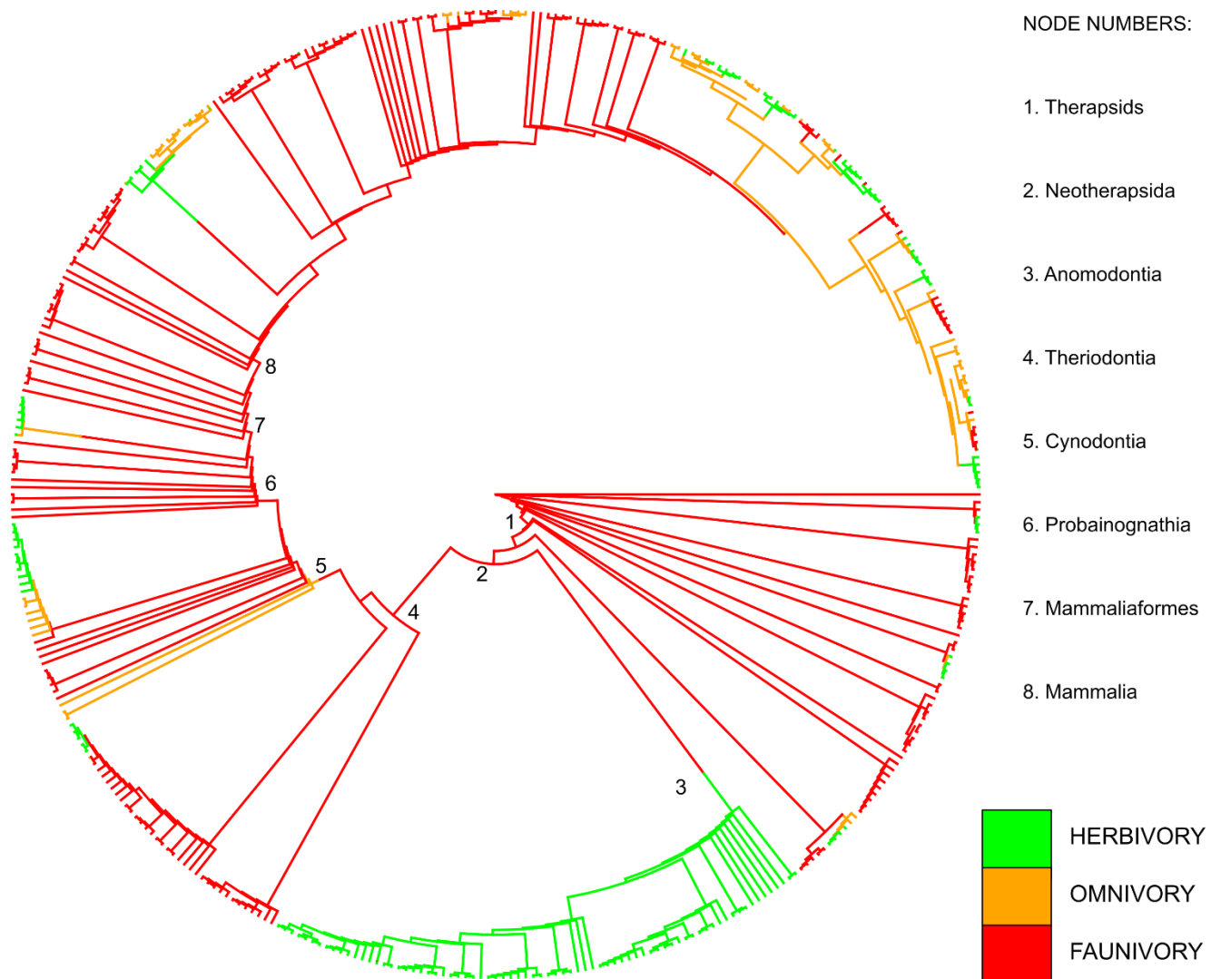
Figure 47: Synapsid phylogeny (Hellert et al. 2022) with branches coloured by the classical dietary guild with the highest probability of representing the ancestral condition at each node, taken from a single random simulation of the stochastic character mapping analysis ("all rates different" model - ARD).
