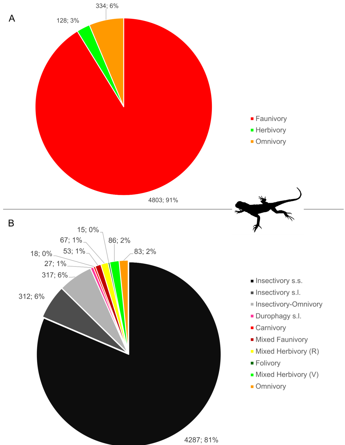
Figure 17: Numbers and percentages of all species of lizards in each (A) classical dietary guild, and (B) dietary guild recovered in the k-means cluster analysis. Abbreviations: Insectivory s.s., "strict" insectivory; Insectivory s.l., predominantly insectivorous mixed invertivory; Durophagy s.l., predominantly
