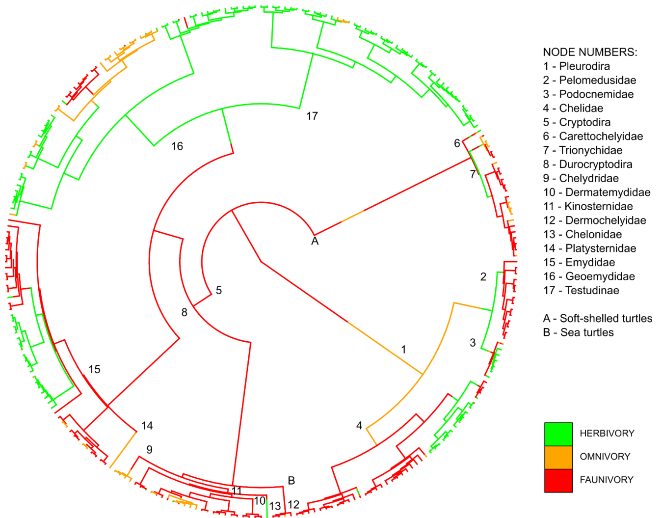
Figure 43: Turtle phylogeny (Thomson et al. 2021) with branches coloured by the classical dietary guild with the highest probability of representing the ancestral condition at each node, taken from a single random simulation of the stochastic character mapping analysis ("symmetrical" model - SYM).
