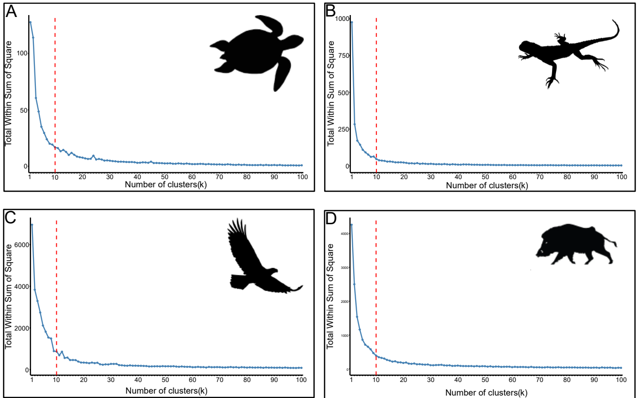
Figure 15: Elbow graphs plotting number of clusters (k-value) against within sum of squares (WSS) values per cluster for (A) turtles, (B) lizards, (C) birds, and (D) mammals.
