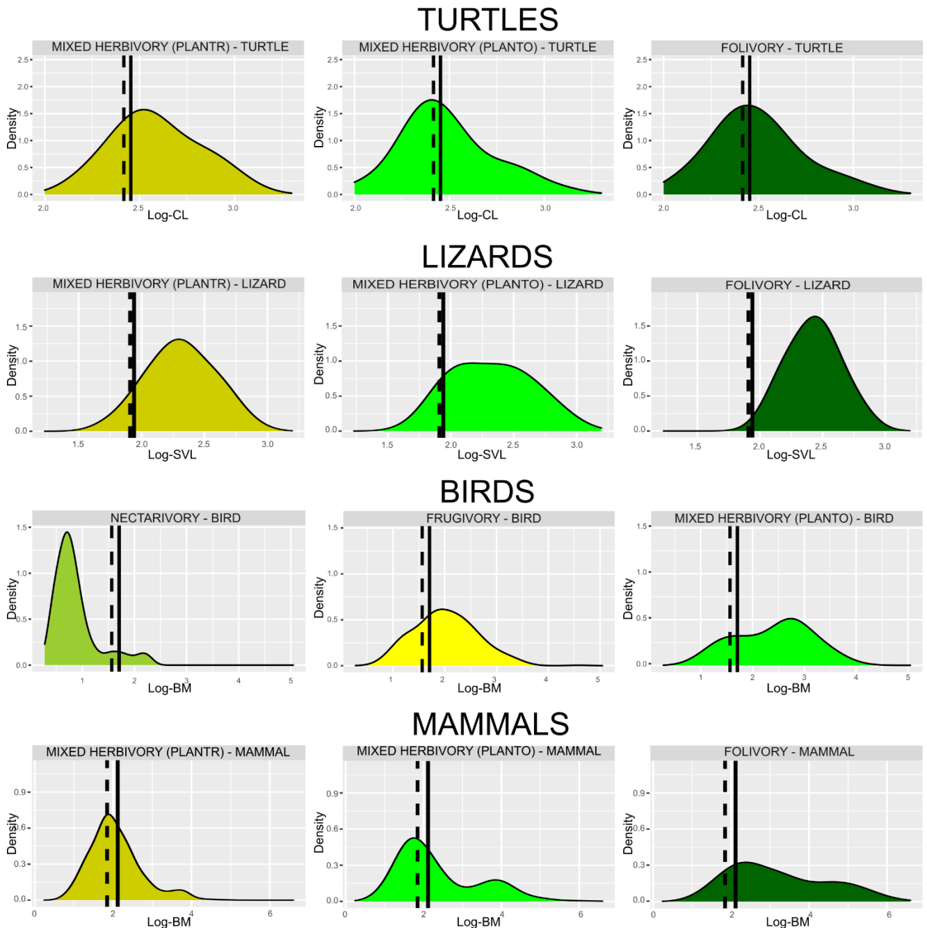
Figure 69: Comparison between density plots of log-transformed body mass (or proxy thereof) values in selected herbivorous guilds. The primary purpose of this figure is to illustrate the differences between herbivorous guilds composed of reproductive versus vegetative plant structures. The solid line represents the mean body mass value in each respective clade. The dotted line represents the median body mass value in each respective clade. For turtles, lizards, and mammal; mixed herbivory with a predominance of reproductive plant structures (dark yellow), mixed
