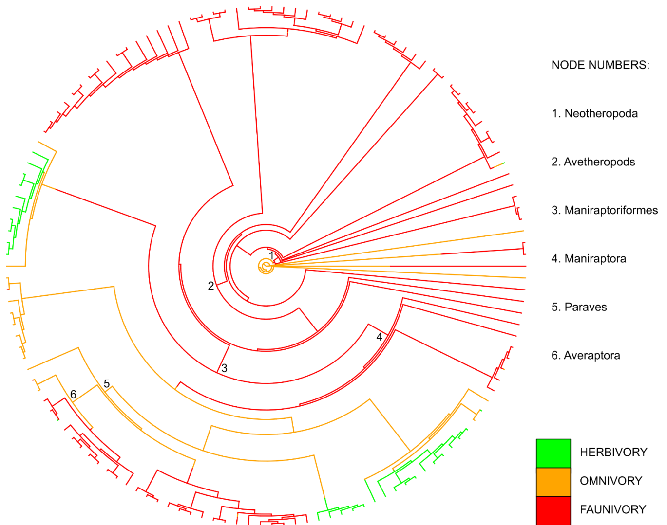
Figure 48: Theropod phylogeny (Benson et al. 2018) with branches coloured by the classical dietary guild with the highest probability of representing the ancestral condition at each node, taken from a single random simulation of the stochastic character mapping analysis ("all rates different" model - ARD).
