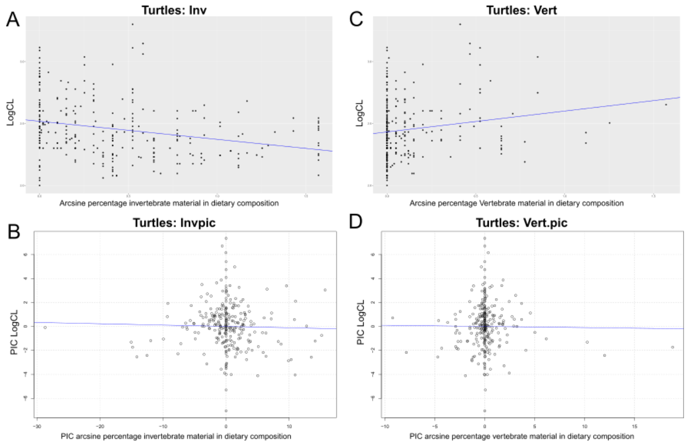
Figure 51: Ordinary, and phylogenetic linear models between log-carapace length (logCL), and arcsine-percentage of total invertebrate (A, B), and total vertebrate (C, D) material in the dietary compositions of turtle taxa. Abbreviations: Inv , percentage of total invertebrate material in the diet; Vert , percentage of total vertebrate material in the diet; PIC , phylogenetic independent contrasts.
