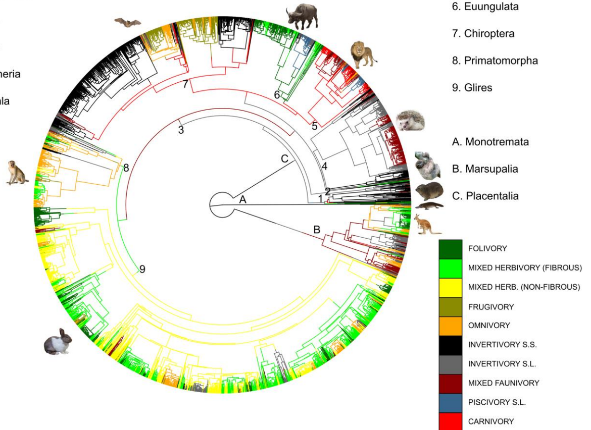
Figure 42: Mammal phylogeny (node-dating backbone topology; Upham et al. 2019) with branches coloured by the dietary guild (recovered in the k-means cluster analysis) with the highest probability of representing the ancestral condition at each node, taken from a single random simulation of stochastic character mapping analysis conducted for the purposes of visualization ("all rates different" model - ARD).
