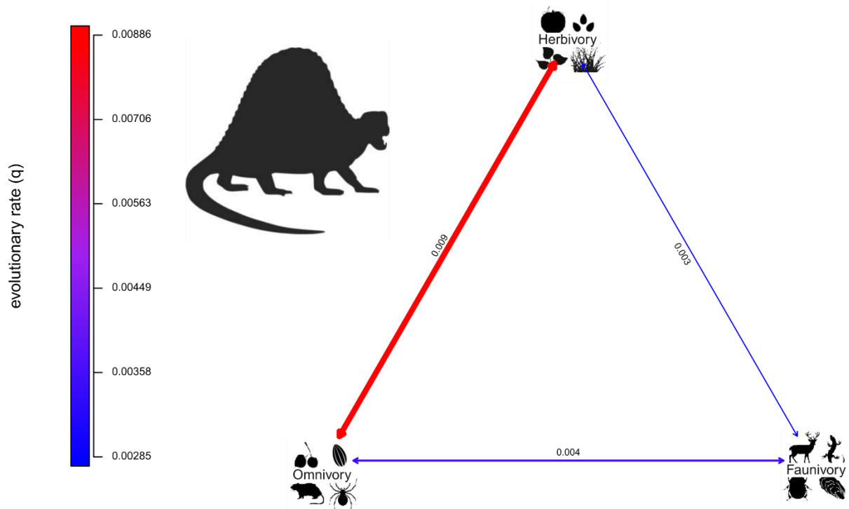
Figure 37: Evolutionary rates of transition between the classical dietary guilds in non-mammalian synapsids as per the results of the Mk analysis ("fitMk" function), "all rates different" (ARD) model. Direction of arrows indicates "from state - to state".
