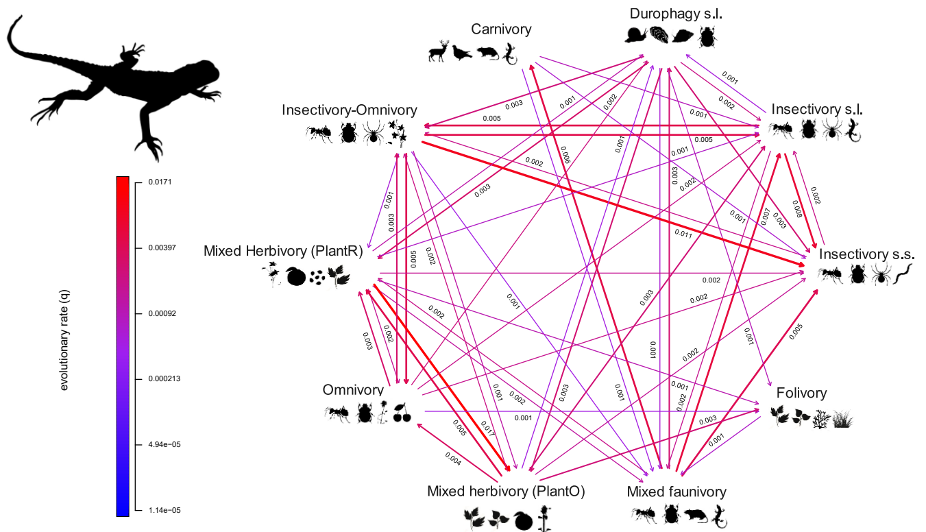
Figure 25: Rates of evolutionary transition between dietary guilds (k-means cluster analysis) in lizards (topology of Pyron et al. 2014) recovered by the Mk marginal maximum likelihood analysis ("all rates different" model - ARD). Direction of arrows indicates "from state - to state". Abbreviations: PlantO, vegetative plant structures; PlantR, reproductive plant structures.
