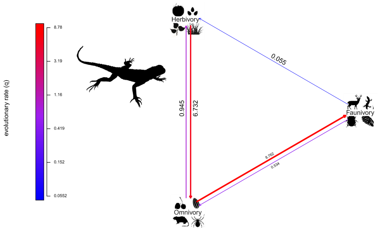
Figure 32: Evolutionary transition rates between the classical dietary guilds in lizards (topology of Pyron et al. 2013) as per the results of the Mk analysis ("fitMk" function), "all rates different" (ARD) model. Direction of arrows indicates "from state - to state".
