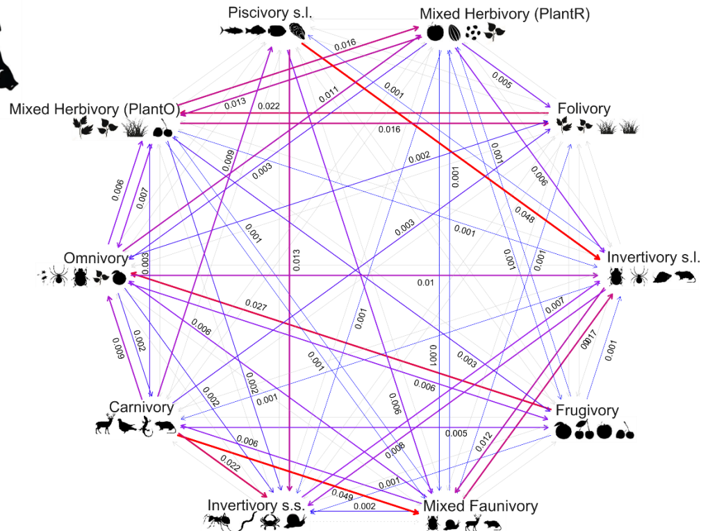
Figure 28: Rates of evolutionary transition between dietary guilds (k-means cluster analysis) in mammals (tip-dating backbone topology) recovered by the Mk marginal maximum likelihood analysis ("all rates different" model - ARD). Only transition rates >0.001 are shown. Direction of arrows indicates "from state - to state". Abbreviations: PlantO, vegetative plant structures; PlantR, reproductive plant structures.
