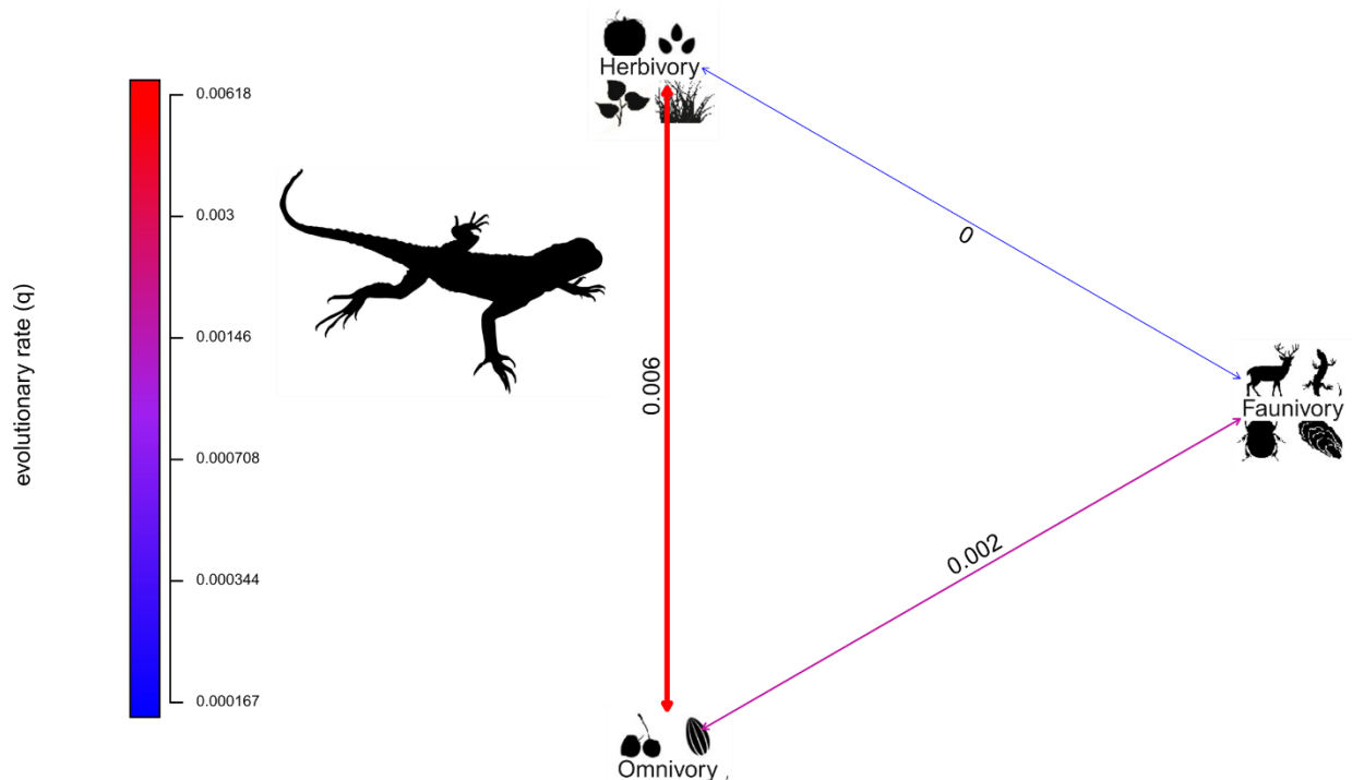
Figure 31: Evolutionary transition rates between the classical dietary guilds in lizards (topology of Tonini et al. 2016) as per the results of the Mk analysis ("fitMk" function), "symmetrical" (SYM) model. Direction of arrows indicates "from state - to state".
