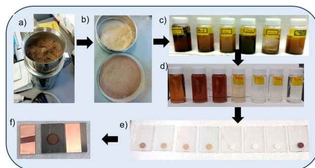
Fig. 3 A flow diagram showing the experimental processes (from top left): (a) milling/pulverizing, (b) sieving, (c) soaking/extraction, (d) after centrifuging, (e) dyeing of TiO_2 coatings into photoanodes, including N719 dye (first from right), and (f) an assembled DSSC.
