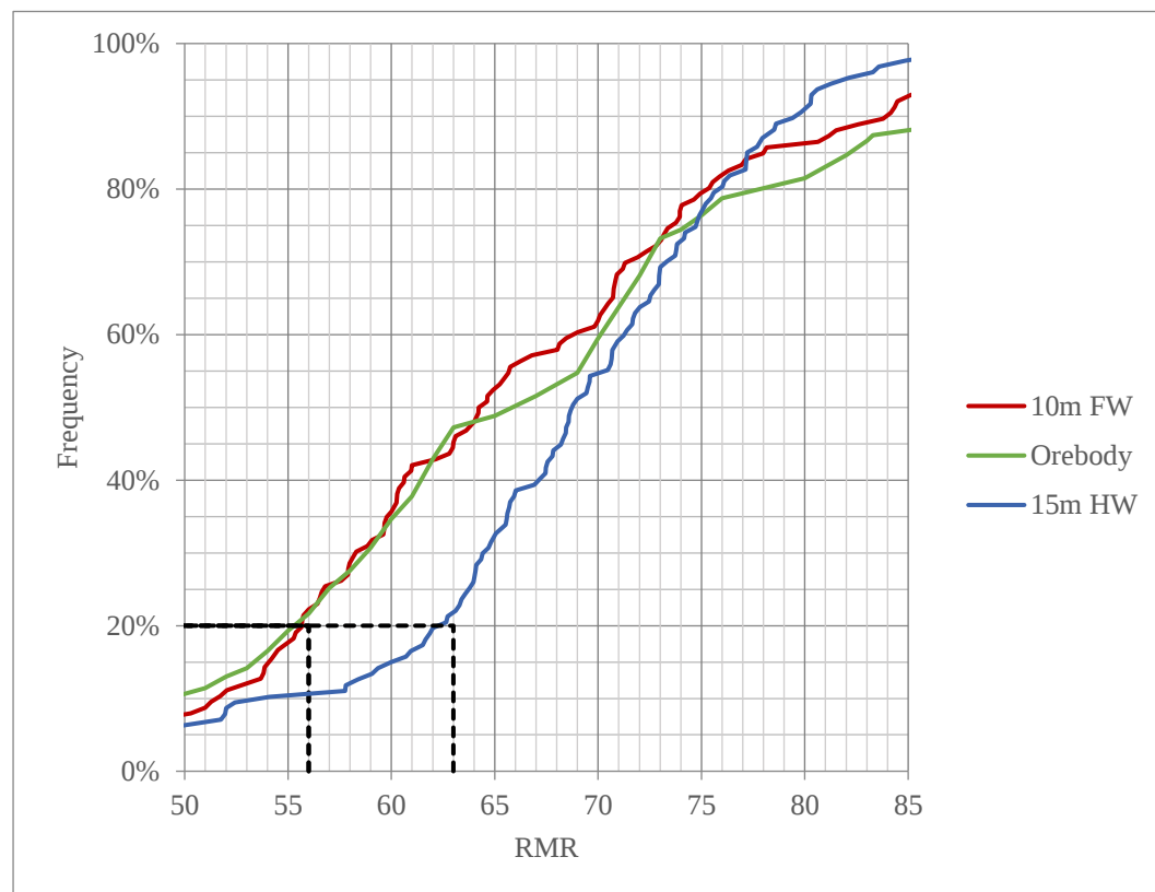
Figure 10: Cumulative frequency curve for RMR values
