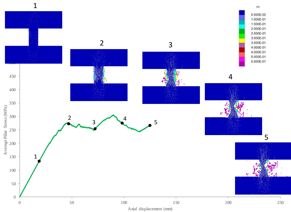
Figure 32: Average pillar stress versus axial displacement curve and displacement contours for the intact 2 m pillar
