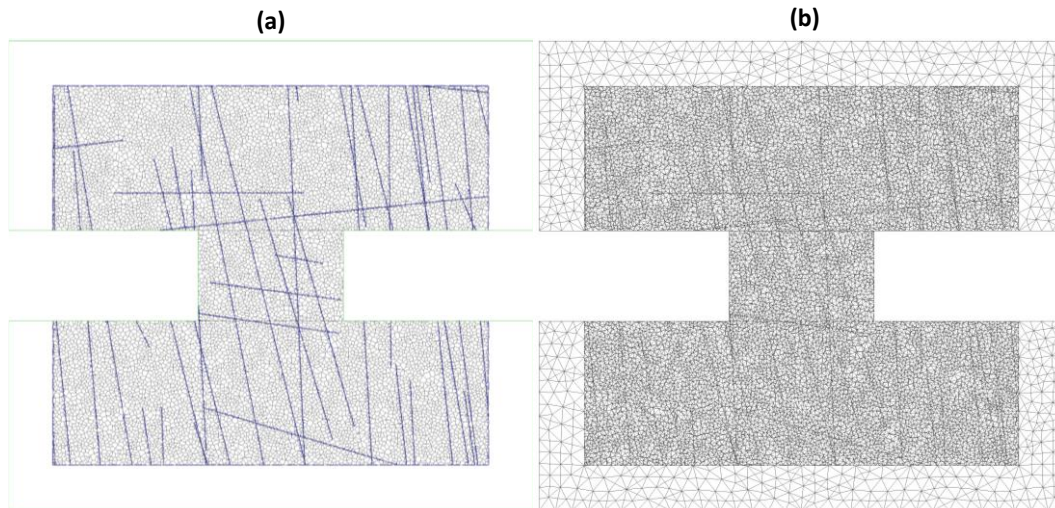
Figure 23: UDEC model of Mine X jointed pillar. (a) Pre-existing fractures and voronoi tessellation, (b) Typical mesh/grid
