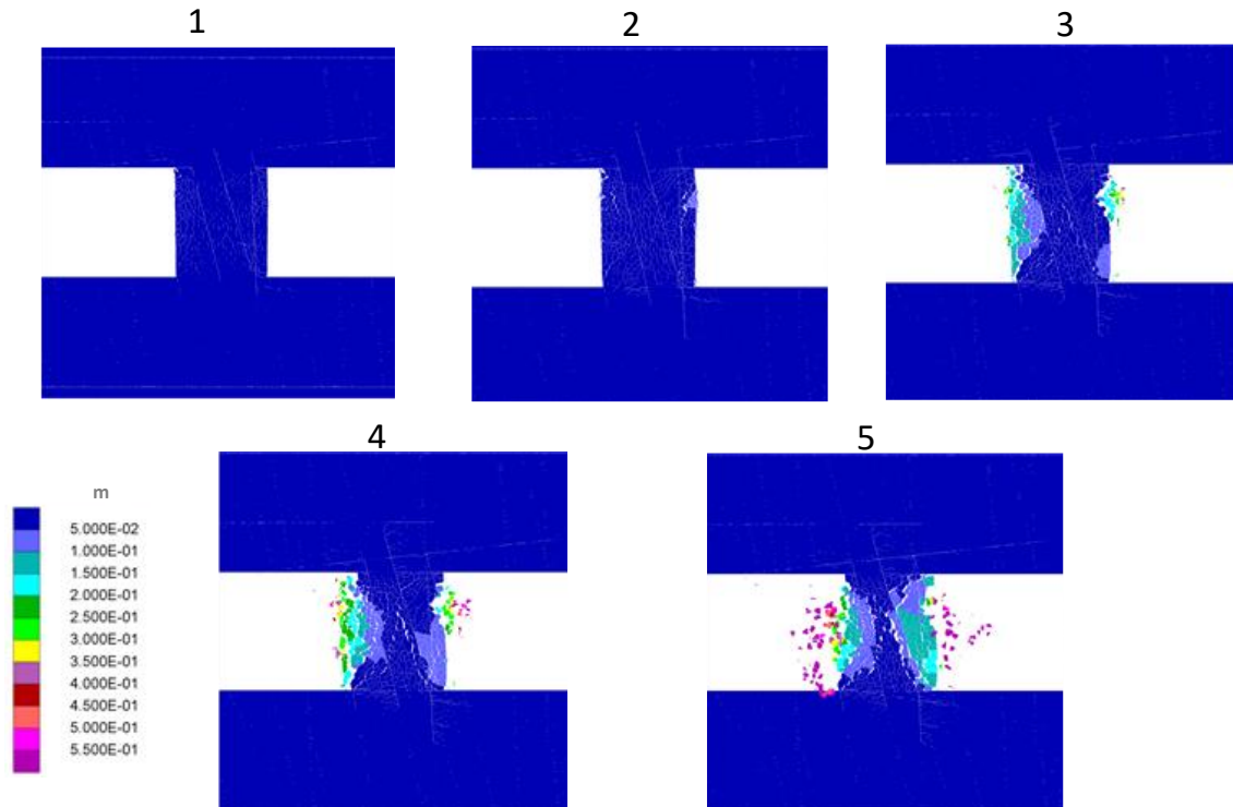
Figure 40: Progression of total displacement for 2m wide jointed pillar model for DFN 1
