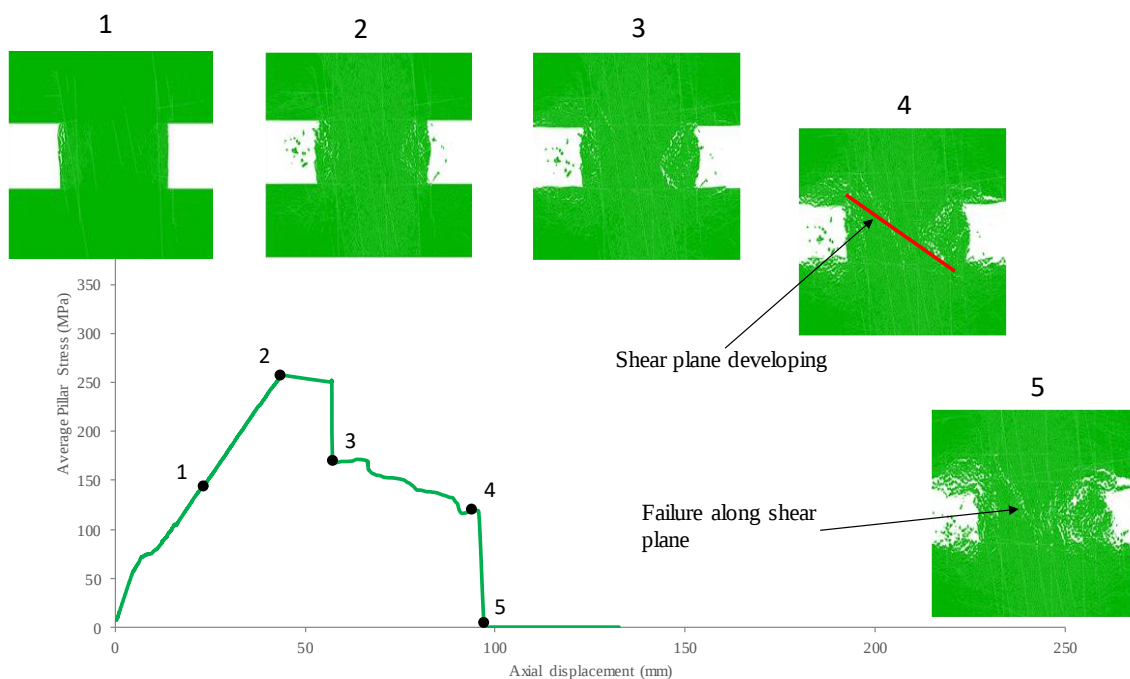
Figure 44: Average pillar stress versus axial displacement curve and associated failure mechanism for 6 m pillar for DFN 1
