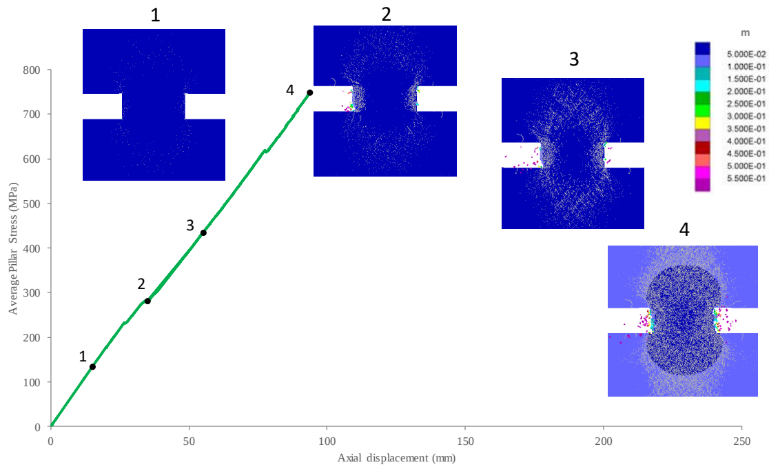
Figure 36: Average pillar stress versus axial displacement curve and displacement contours for the intact 6 m pillar
