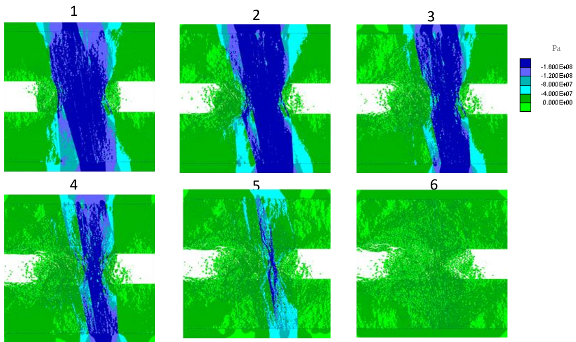
Figure 54: Progression of stresses for 6 m wide jointed pillar model for DFN 2
