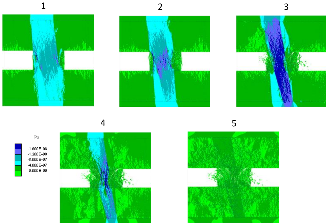
Figure 51: Progression of stresses for 4 m wide jointed pillar model for DFN 2
