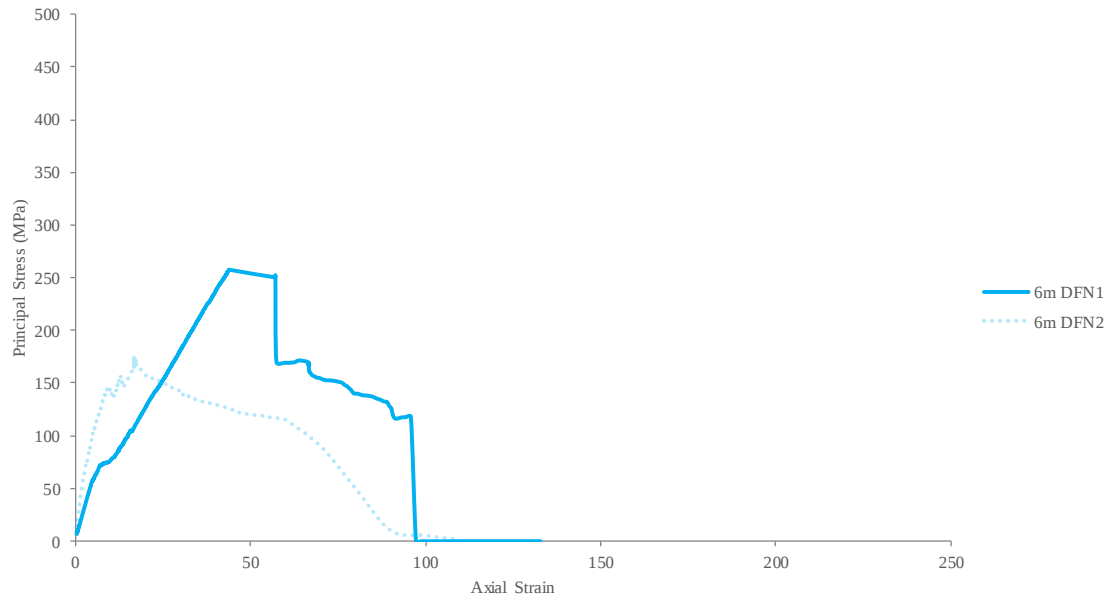
Figure 60: Pillar stress vs. axial displacement graphs of 6 m pillar model for DFN 1 with DFN 2 results in the background
