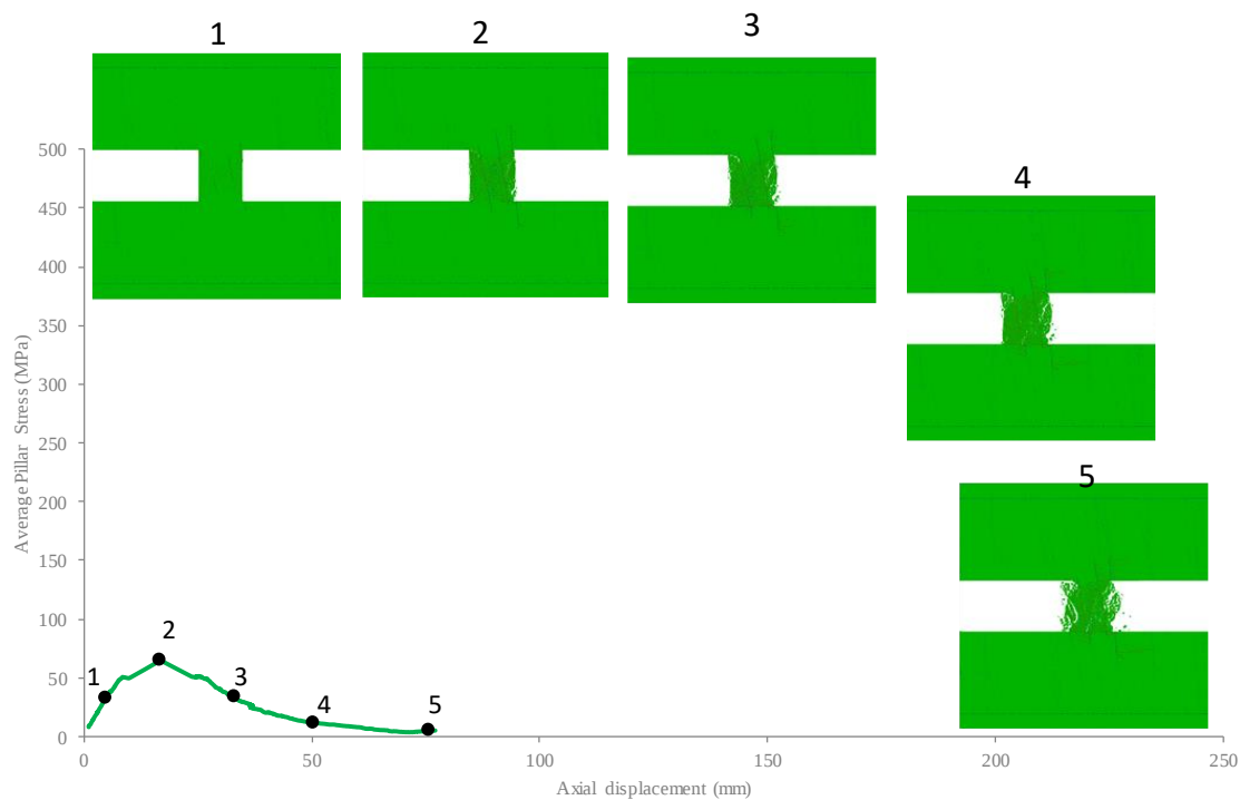
Figure 47: Average pillar stress versus axial displacement curve and associated failure mechanism for 2 m pillar for DFN 2
