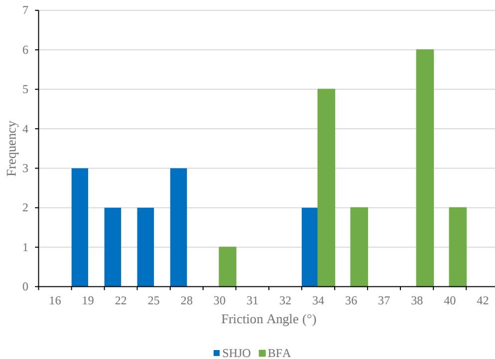
Figure 12: Distribution of peak friction angle in BFA and SHJO tests
