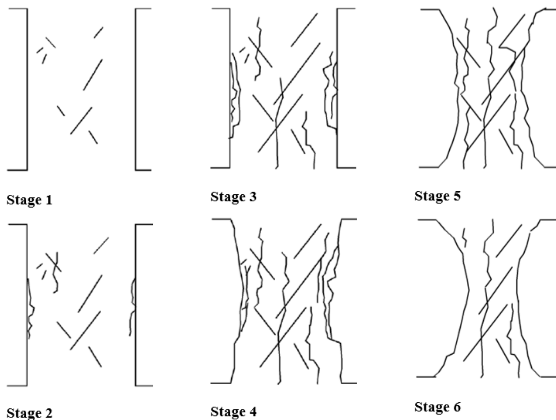
Figure 5: Pillar rating system (Roberts, et al., 1998)
