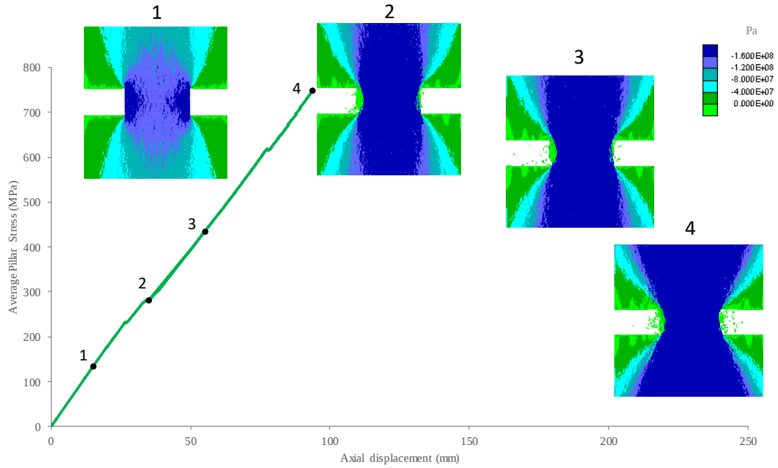
Figure 37: Average pillar stress versus axial displacement curve and displacement contours for the intact 6 m pillar
