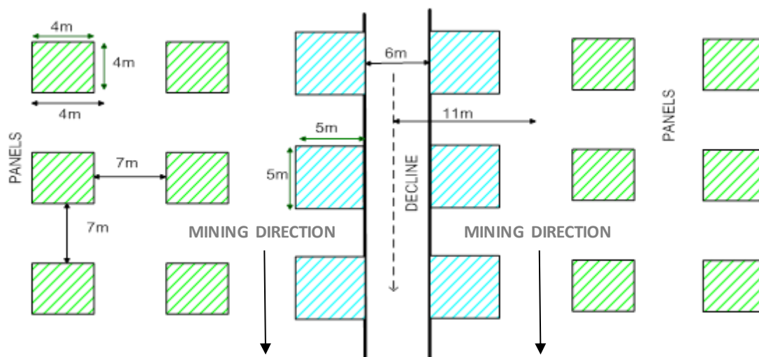
Figure 1: Schematic diagram showing room and pillar mining at Mine X
