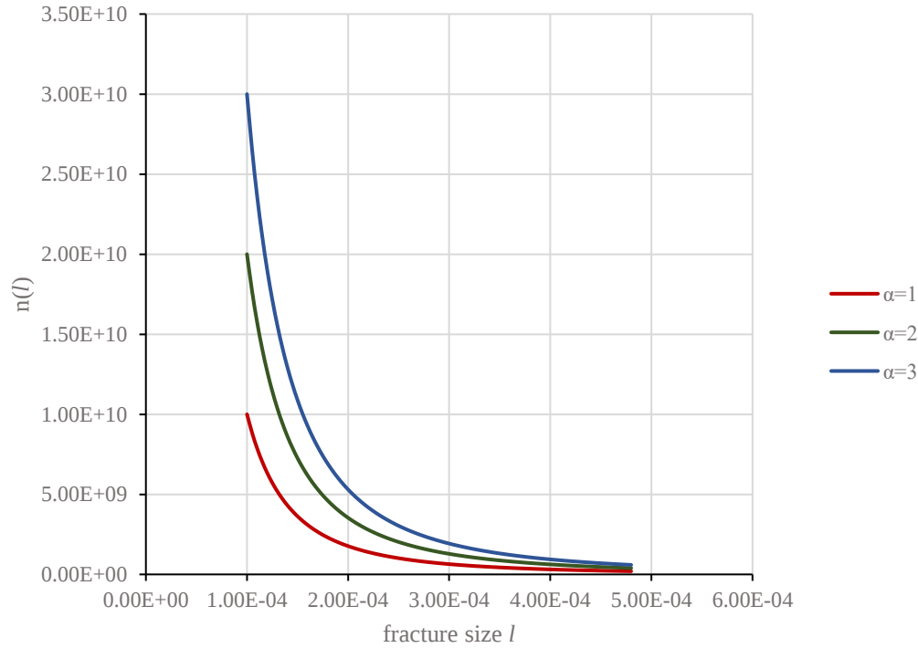
Figure 19: Effect of \alpha on fracture size distribution for a=2.5
