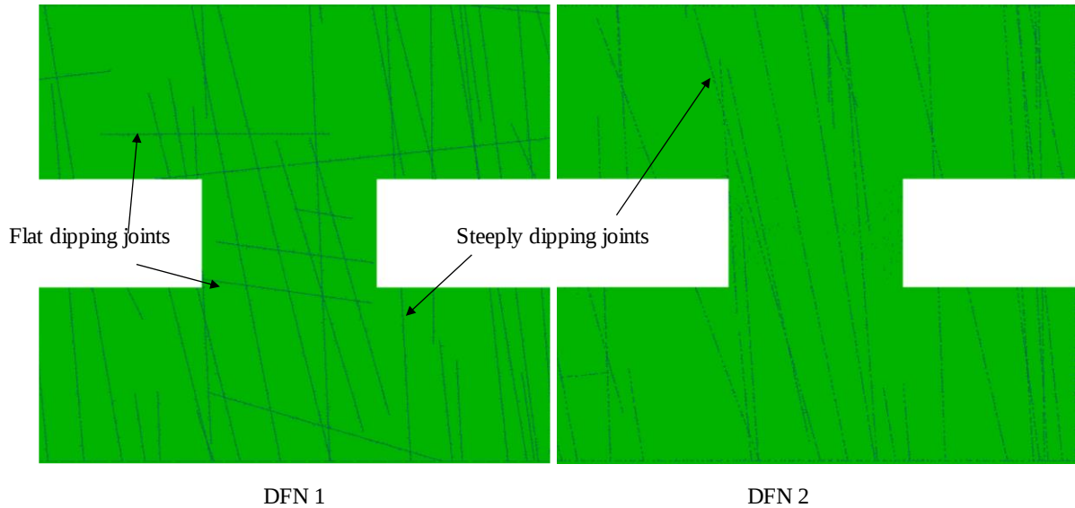
Figure 18: DFN 1 and DFN 2 models
