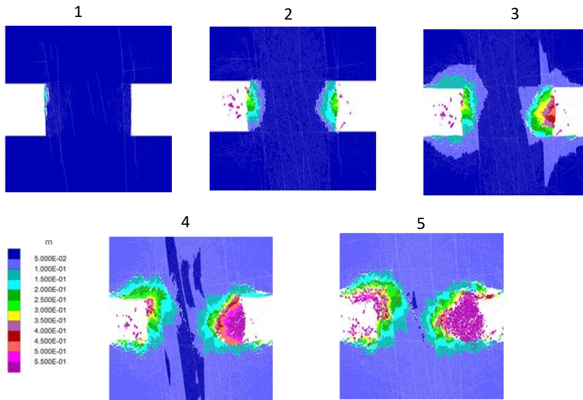
Figure 46: Progression of total displacement for 6 m wide jointed pillar model for DFN 1
