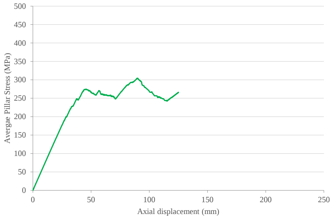
Figure 30: Average pillar stress versus axial displacement curve for the intact 2 m pillar
