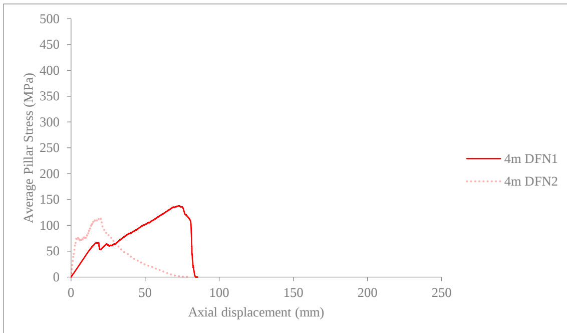
Figure 59: Pillar stress vs. axial displacement graphs of 4 m pillar models for DFN 1 with DFN 2 results in the background
