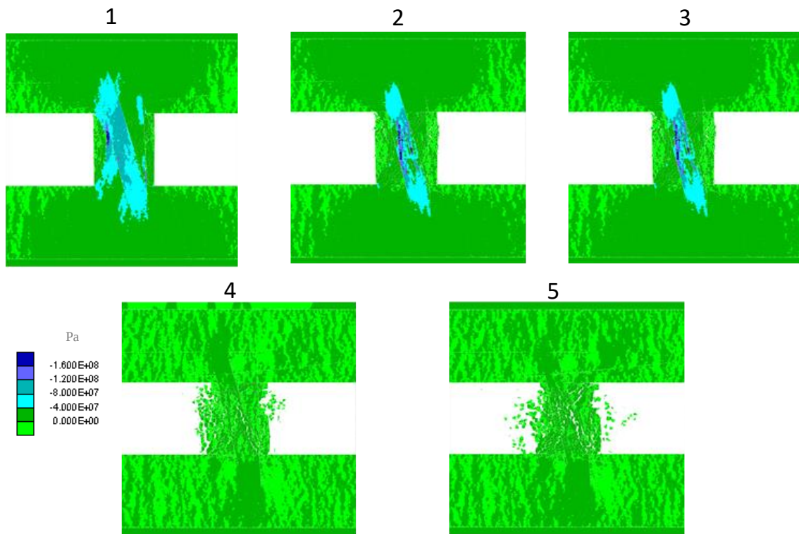
Figure 39: Progression of stress for 2m wide jointed pillar model for DFN 1
