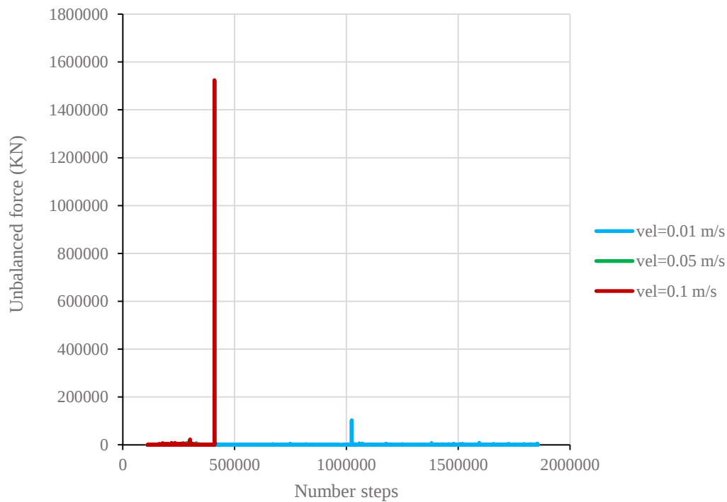
Figure 25: Loading velocity sensitivity: Unbalanced force
