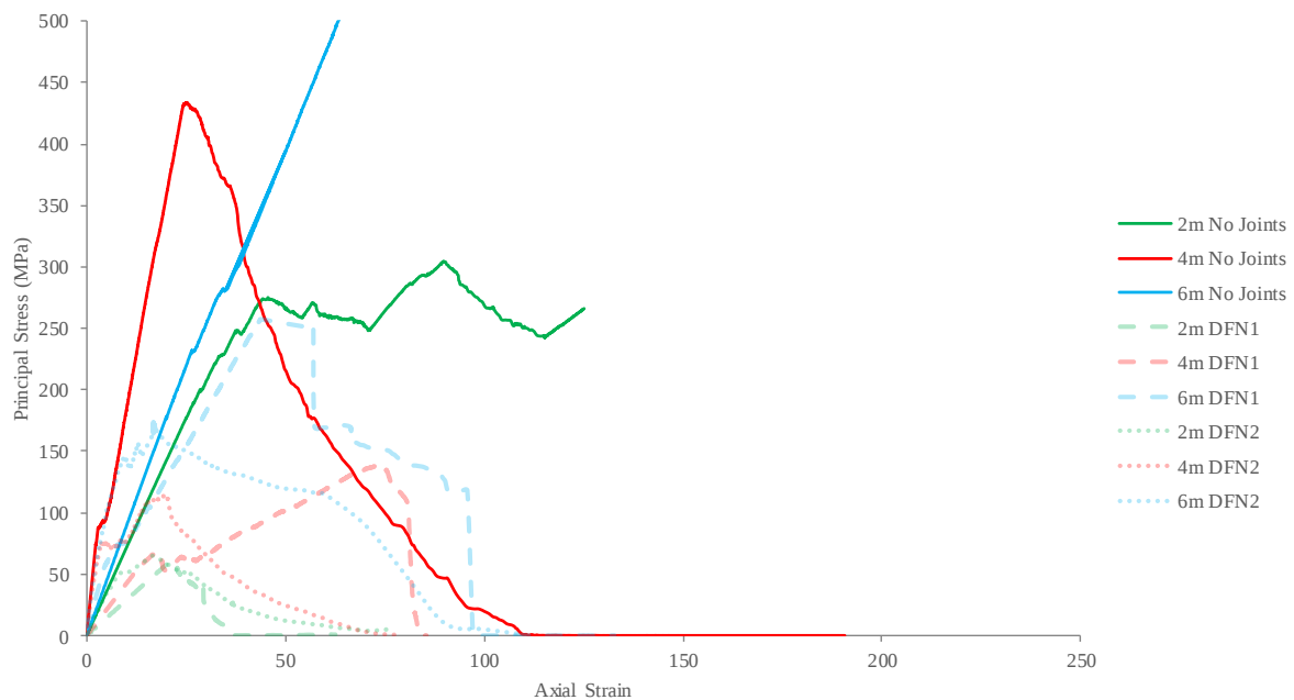
Figure 56: Average pillar stress versus axial displacement curve for intact pillars and jointed pillars results in the background
