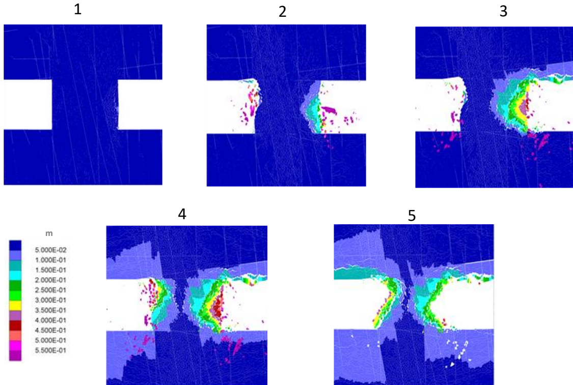
Figure 43: Progression of total displacement for 4 m wide jointed pillar model for DFN 1
