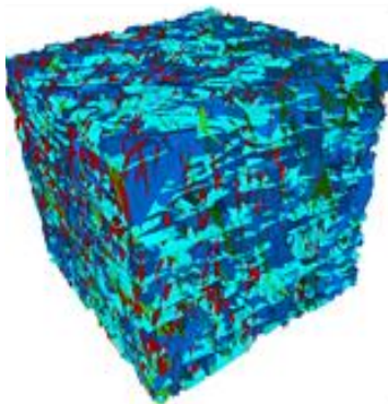
Figure 20: the 3D DFN model in 3DEC
