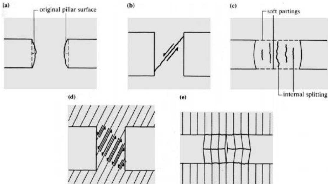
Figure 3: Principal modes of deformation behaviour of mine pillars (Brady and Brown 2004).
