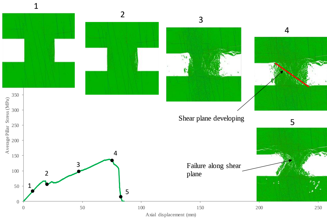
Figure 41: Average pillar stress versus axial displacement curve and associated failure mechanism for 4 m pillar for DFN 1
