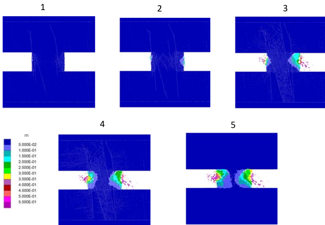
Figure 52: Progression of total displacement for 4 m wide jointed pillar model for DFN 2
