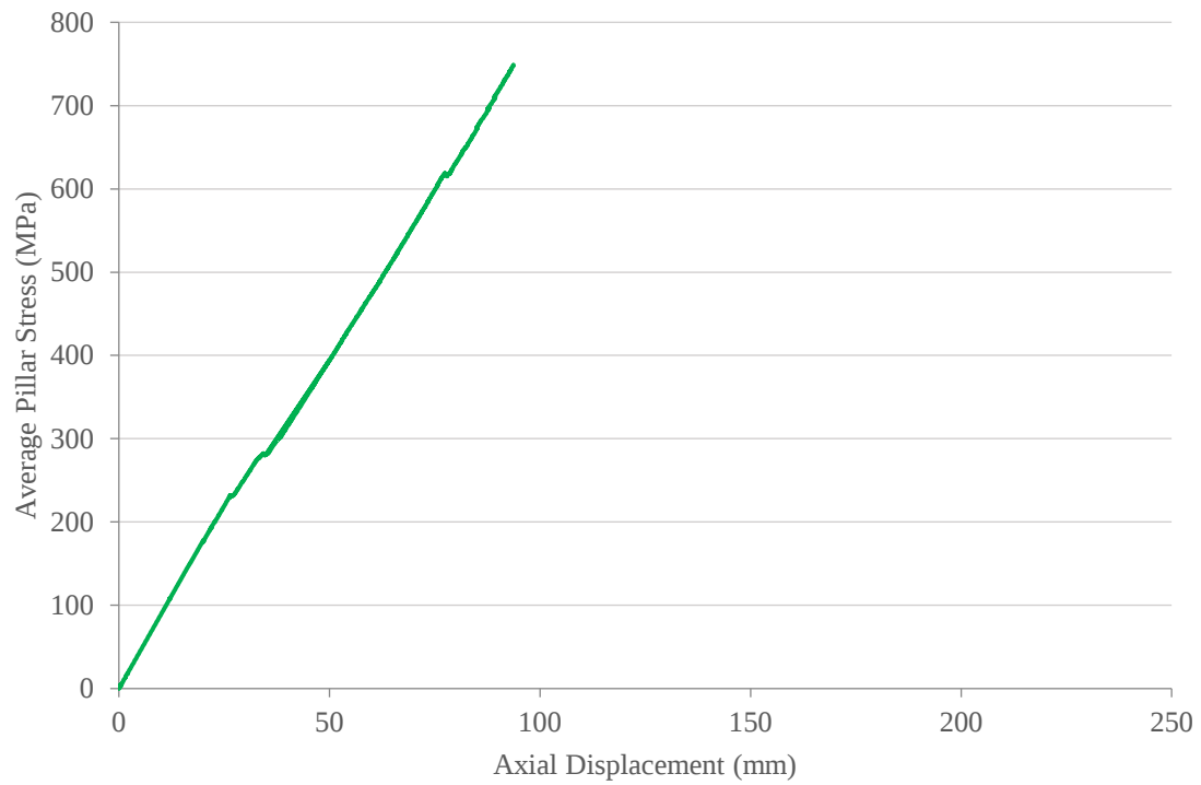
Figure 34: Average pillar stress versus axial displacement curve for the intact 6 m pillar
