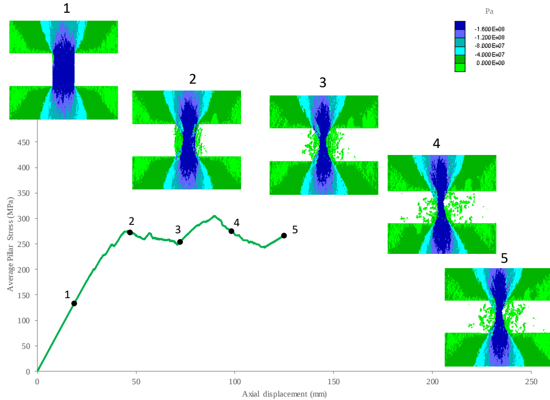
Figure 33: Average pillar stress versus axial displacement curve progression of stress for the intact 2 m pillar
