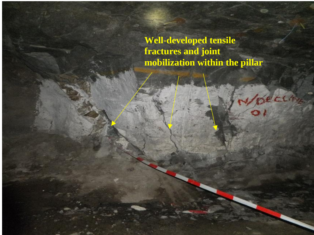
Figure 16: Pillar sidewall conditions with stress induced tensile fractures and joint mobilization with the pillar
