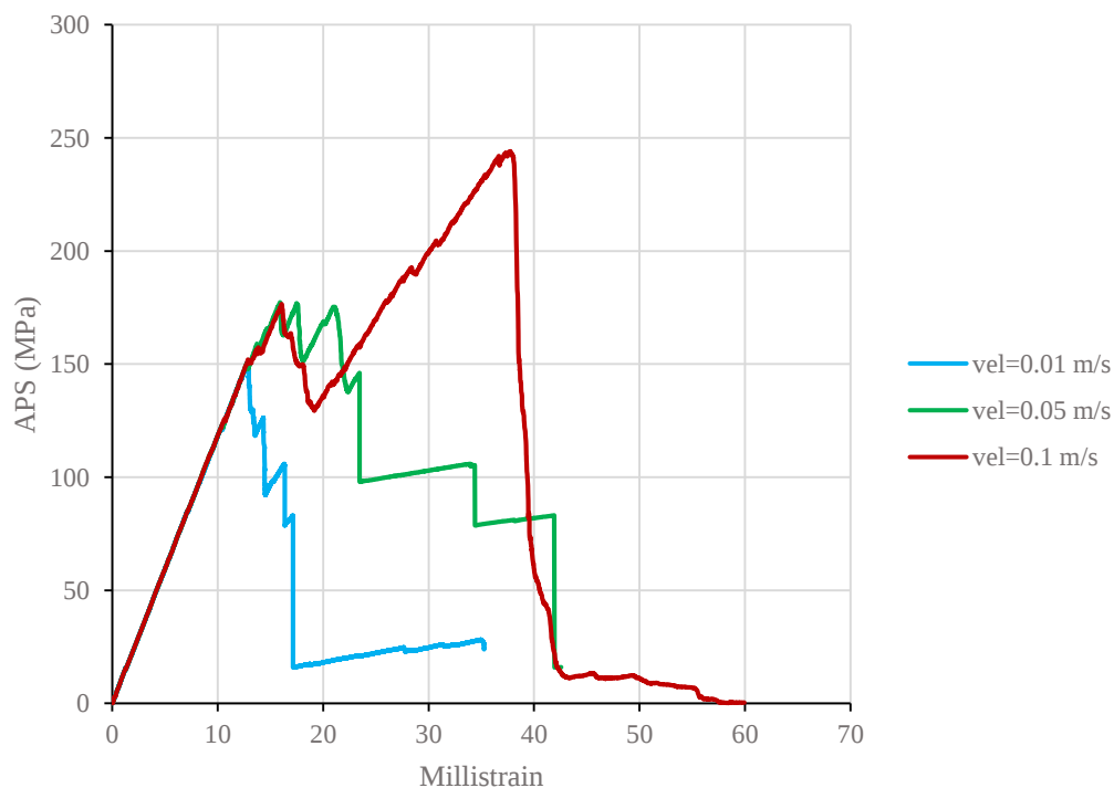
Figure 24: Loading velocity sensitivity: Average pillar stress vs. pillar strain curve
