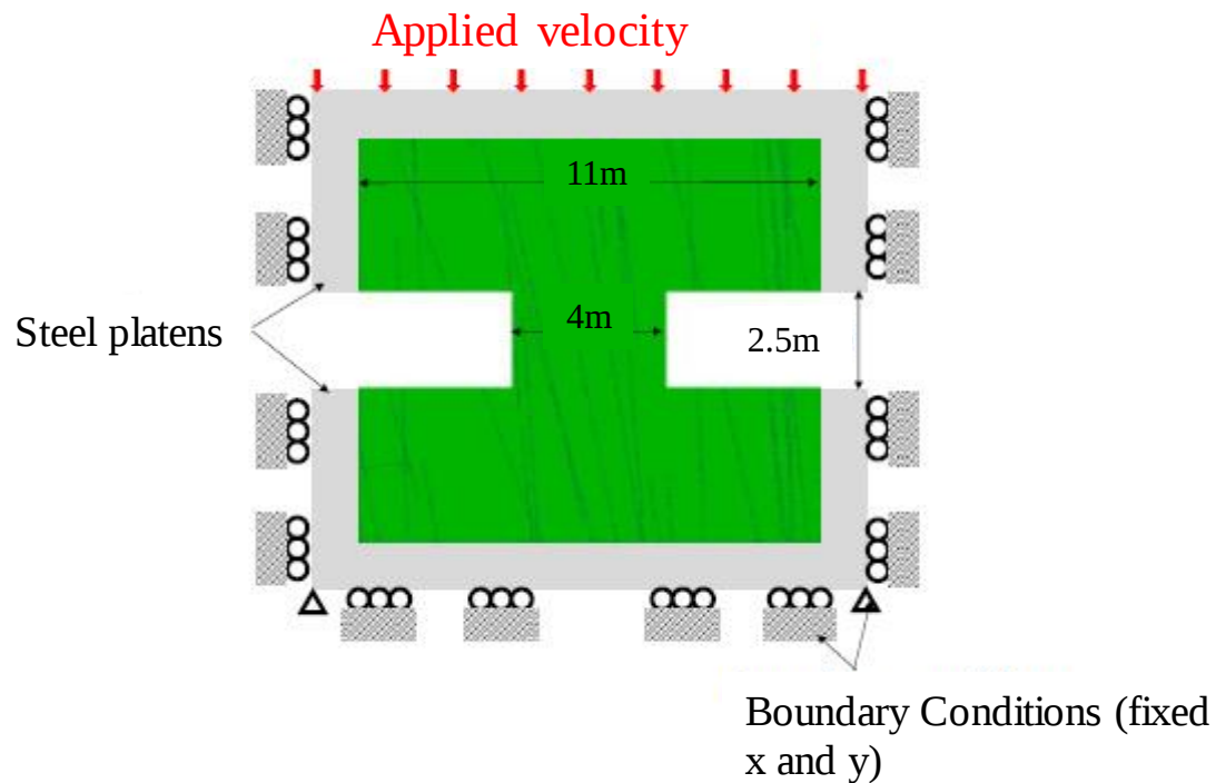
Figure 2: UDEC 4m pillar model
