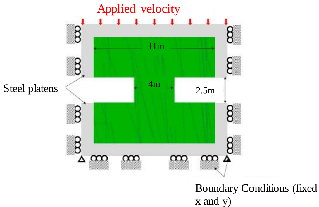
Figure 22: Typical Mine X jointed pillar model geometry – Dimensions and boundary conditions
