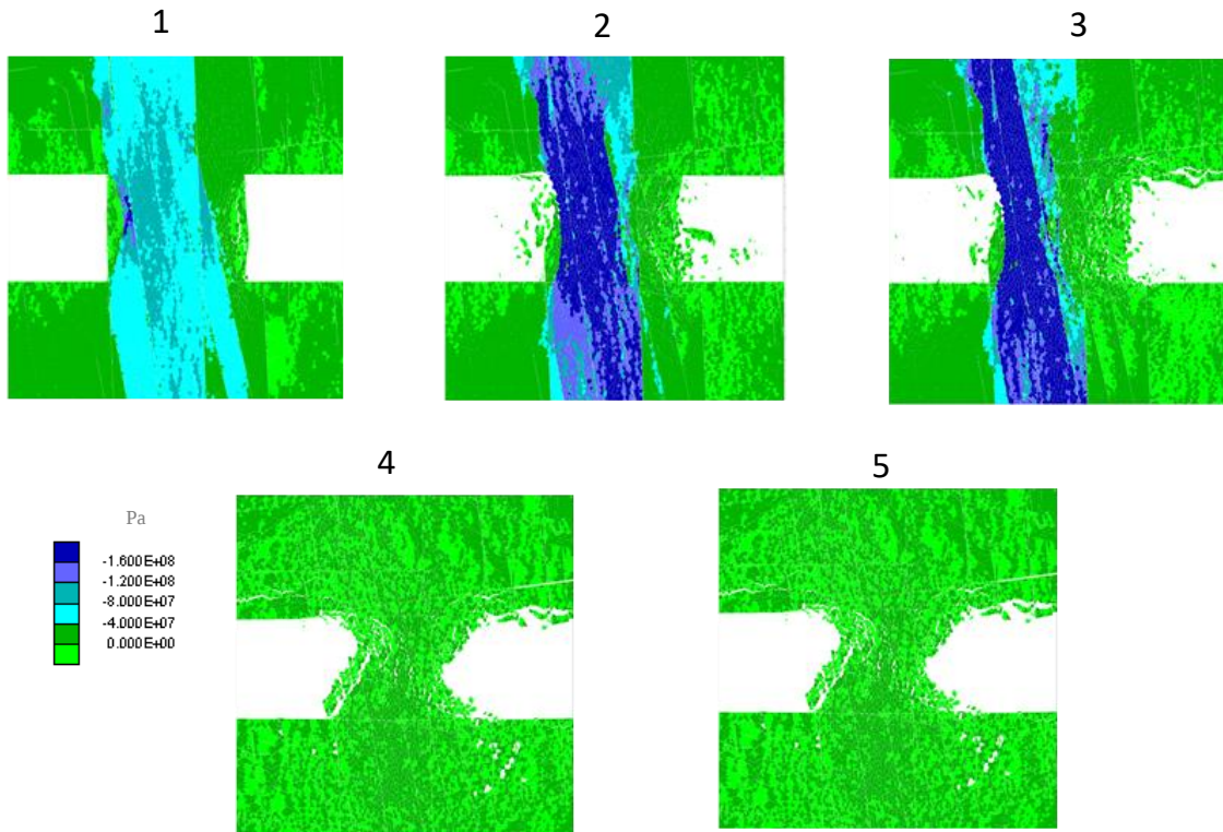
Figure 42: Progression of stresses for 4 m wide jointed pillar model for DFN 1
