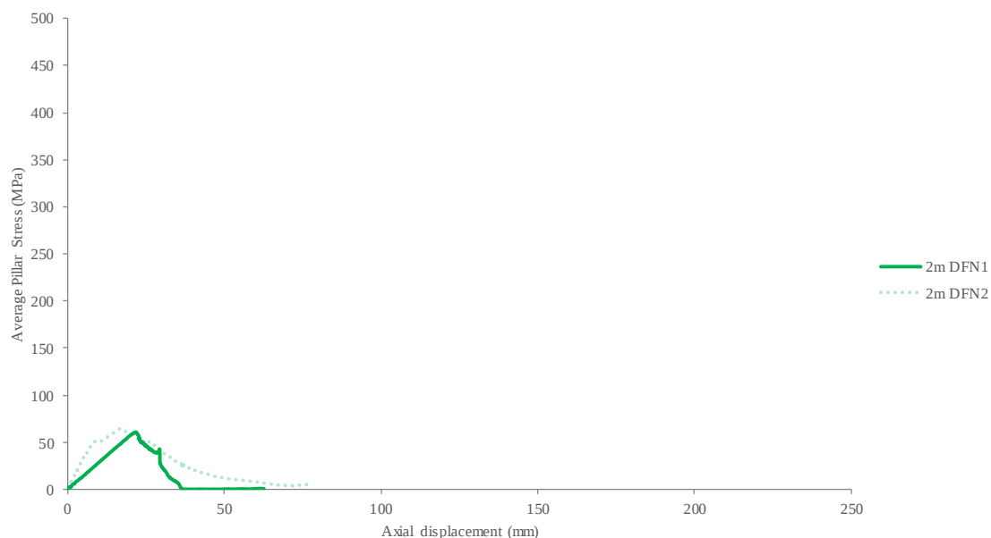
Figure 58: Pillar stress vs. axial displacement graphs of 2 m pillar models for DFN 1 with DFN 2 results in the background
