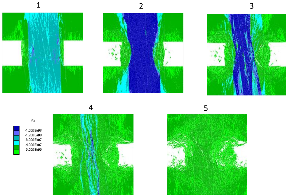
Figure 45: Progression of stresses for 6 m wide jointed pillar model for DFN 1
