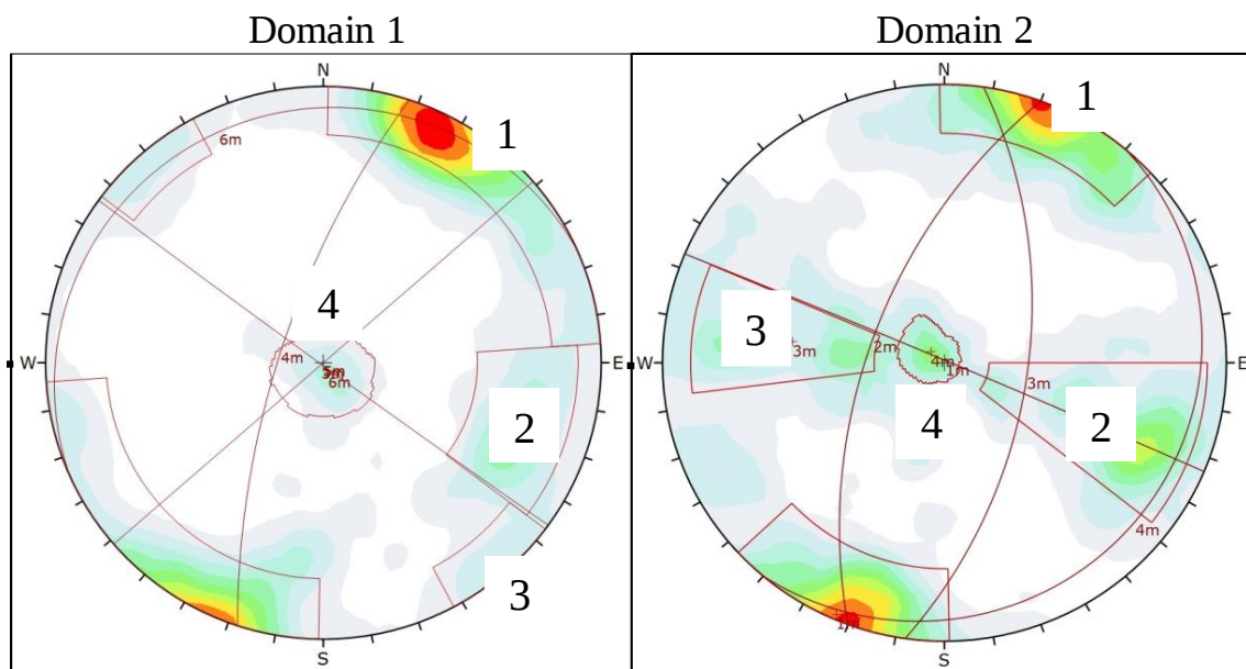
Figure 17: Stereonet plot of fractures mapped at Portal C (DIPS software)
