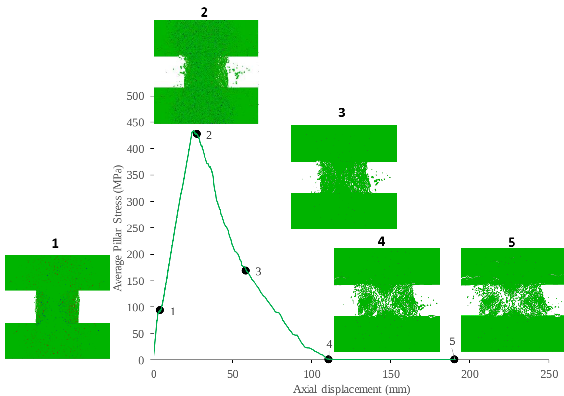
Figure 28: Average pillar stress versus axial displacement curve and failure mode for the intact 4 m pillar
