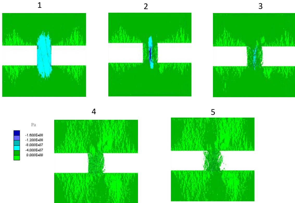
Figure 48: Progression of stresses for 2 m wide jointed pillar model for DFN 2
