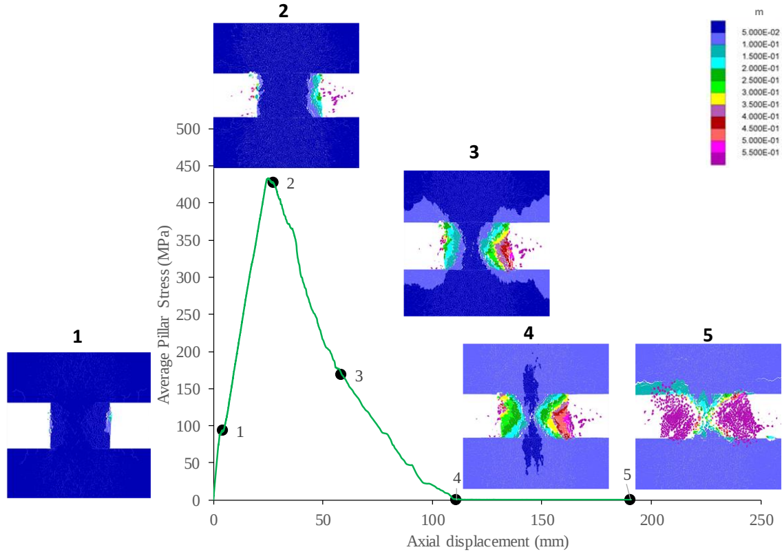
Figure 29: Average pillar stress versus axial displacement curve and displacement contours for the intact 4 m pillar.
