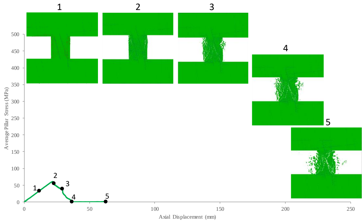
Figure 38: Average pillar stress versus axial displacement curve and associated failure mechanism for 2m wide pillar model for DFN 1
