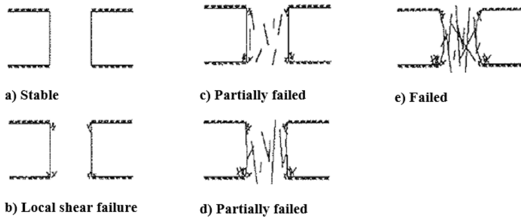
Figure 4: Schematic illustration of the evolution of fracture and failure in a pillar in massive rock (Lunder & Pakalnis, 1997)
