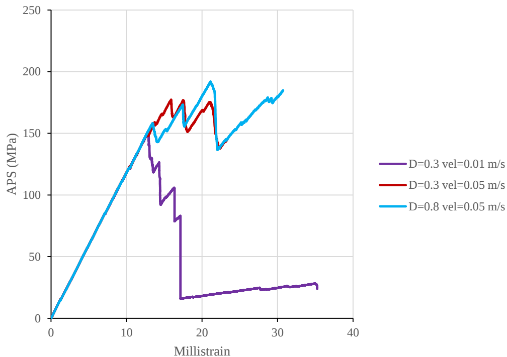
Figure 26: Damping sensitivity analysis: Average pillar stress vs. pillar strain curve
