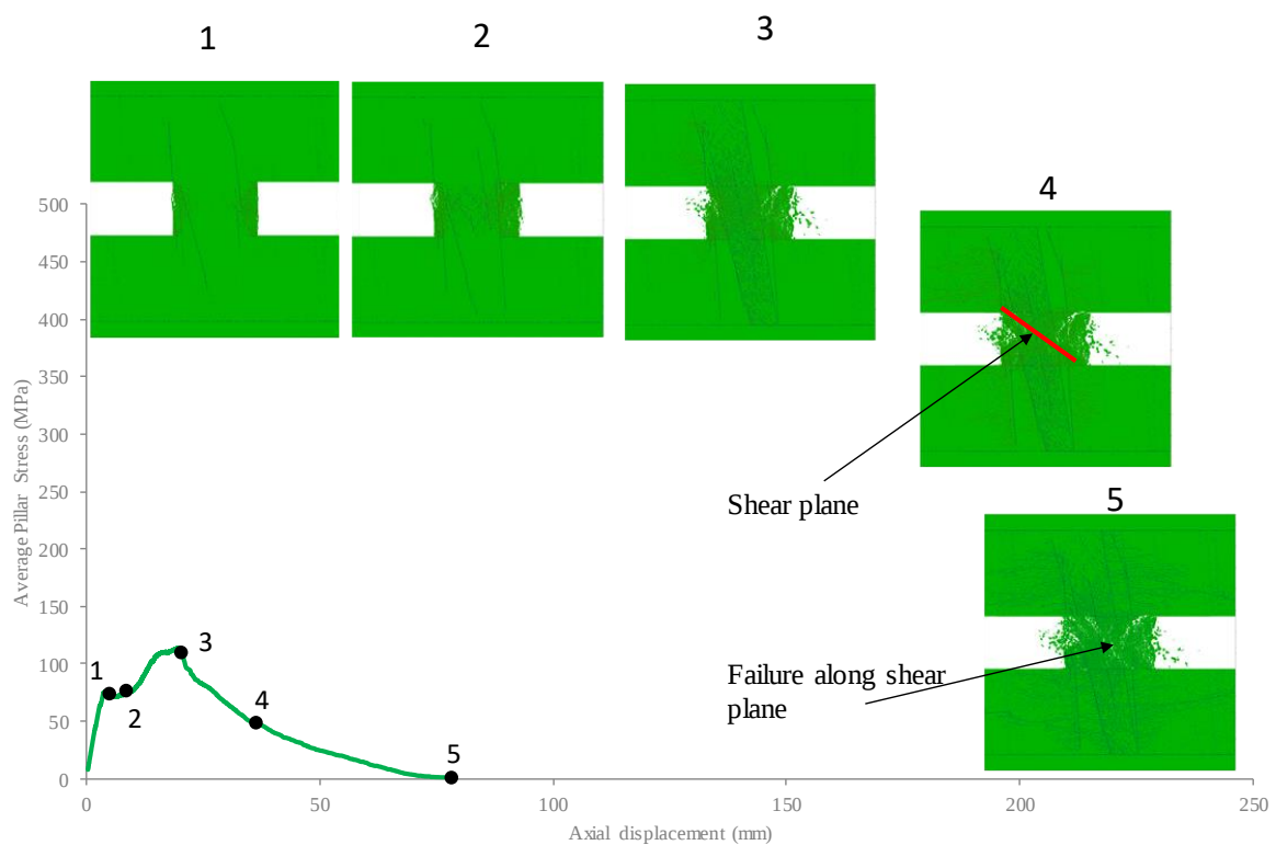
Figure 50: Average pillar stress versus axial displacement curve and associated failure mechanism for 4 m pillar for DFN 2
