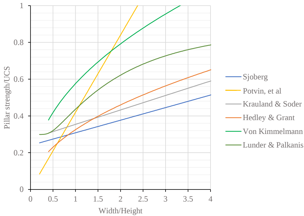
Figure 6: Empirical pillar strength formulas normalized to UCS ( after Martin and Maybee, 2000)
