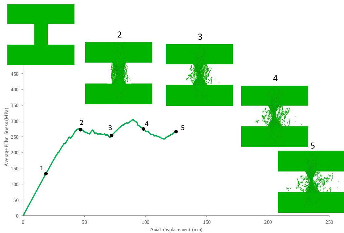
Figure 30: Average pillar stress versus axial displacement curve for the intact 2 m pillar
