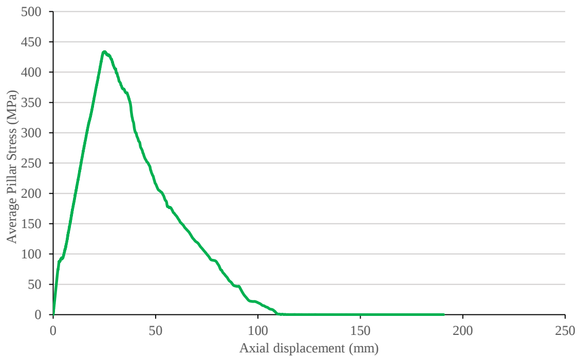
Figure 27: Average pillar stress versus axial displacement curve for the intact 4 m pillar
