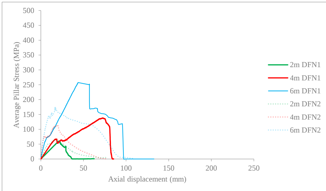
Figure 57: Average pillar stress versus axial displacement for DFN 1 and DFN 2 results in the background
