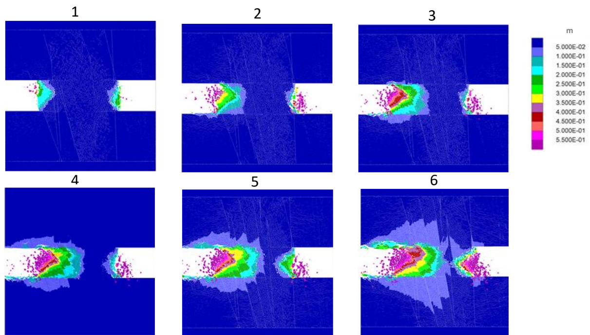
Figure 55: Progression of total displacement for 6 m wide jointed pillar model for DFN 2
