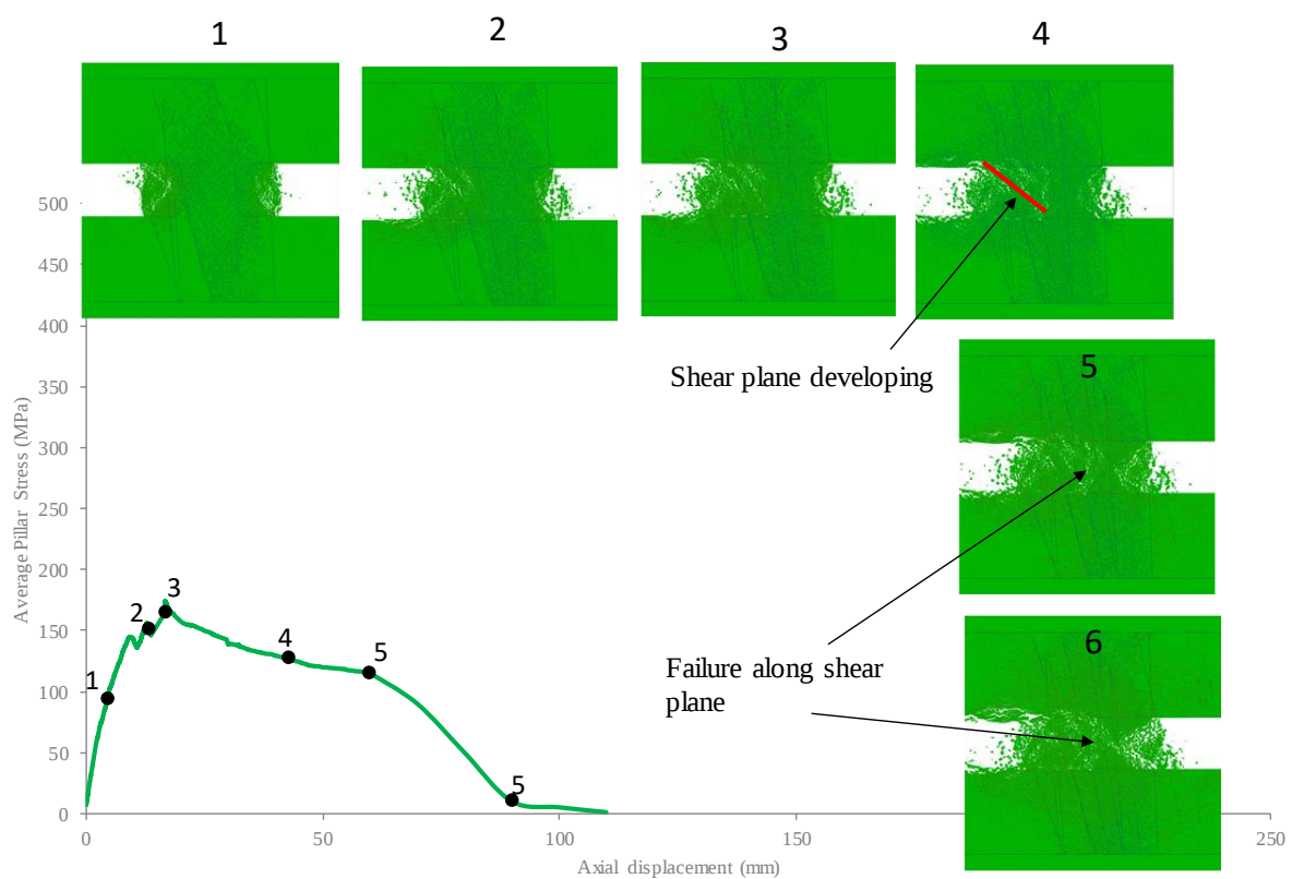
Figure 53: Average pillar stress versus axial displacement curve and associated failure mechanism for 6 m pillar for DFN 2
