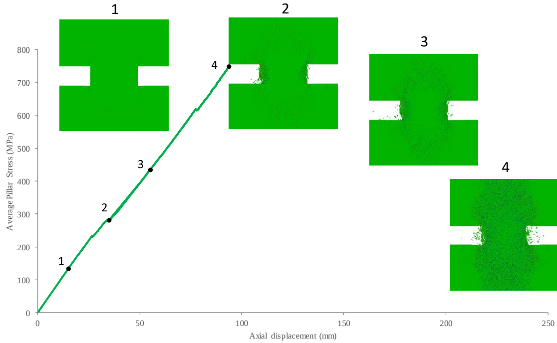
Figure 35: Average pillar stress versus axial displacement curve and failure mode for the intact 6 m pillar
