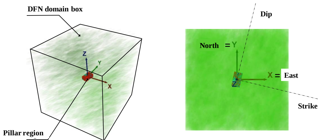
Figure 21: DFN domain and pillar region settings for P_C model in 3DEC, isometric view on the left and plane view on the right
