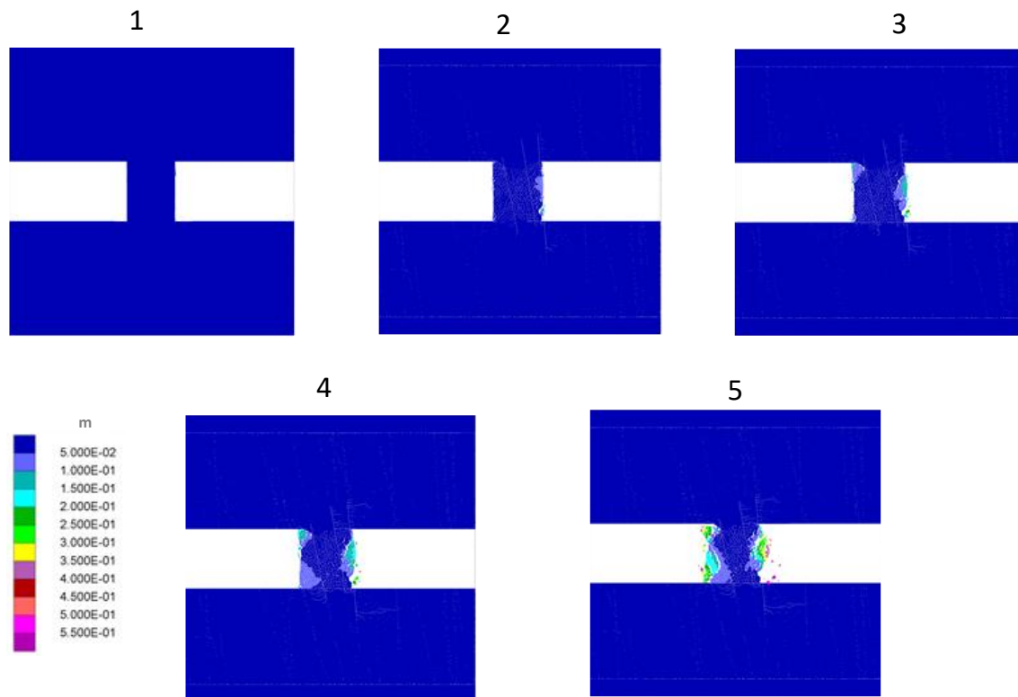
Figure 49: Progression of total displacement for 2 m wide jointed pillar model for DFN 2
