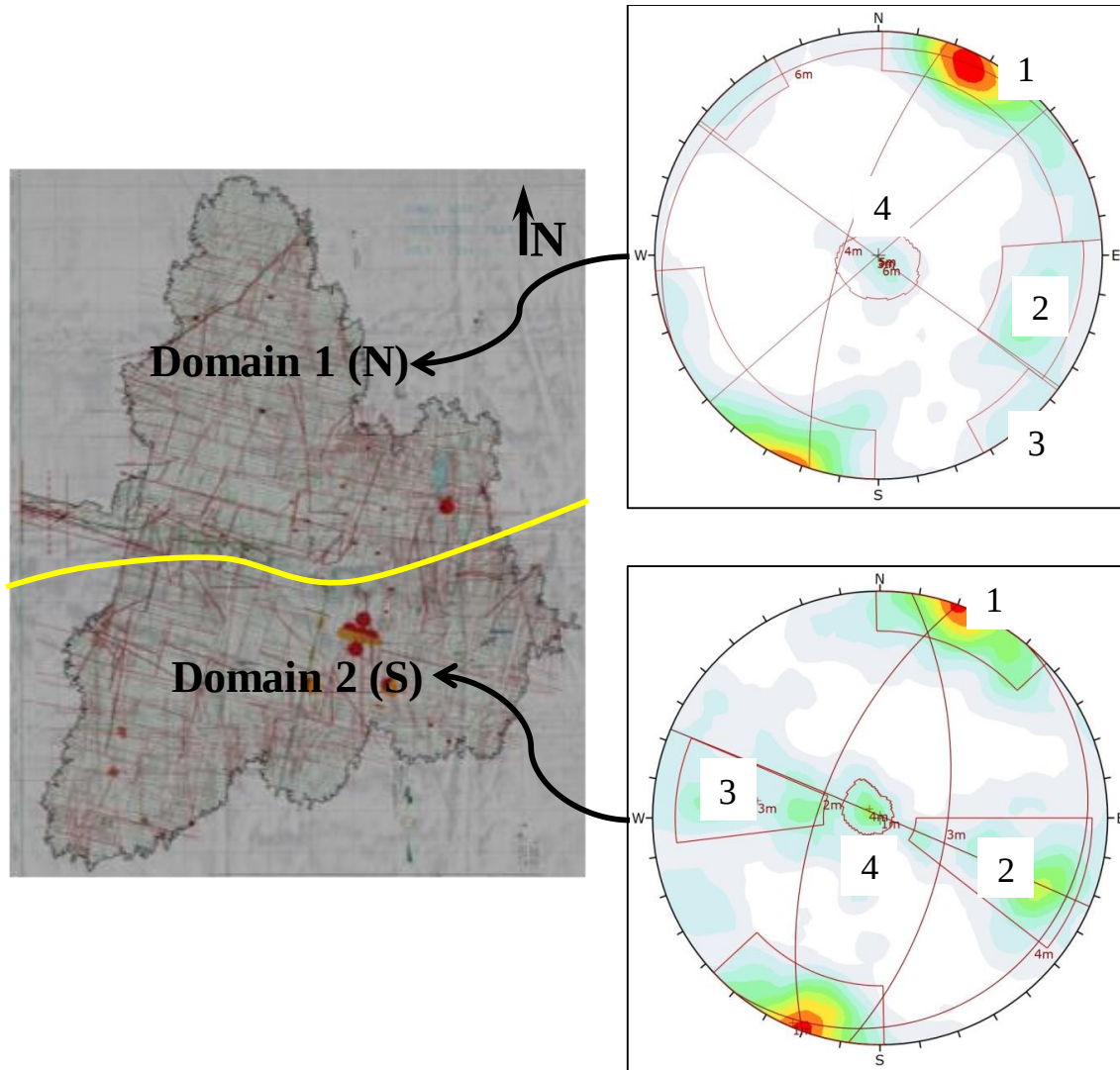
Figure 8: Fracture orientation in domain 1 and domain 2 (Mine X, 2016)
