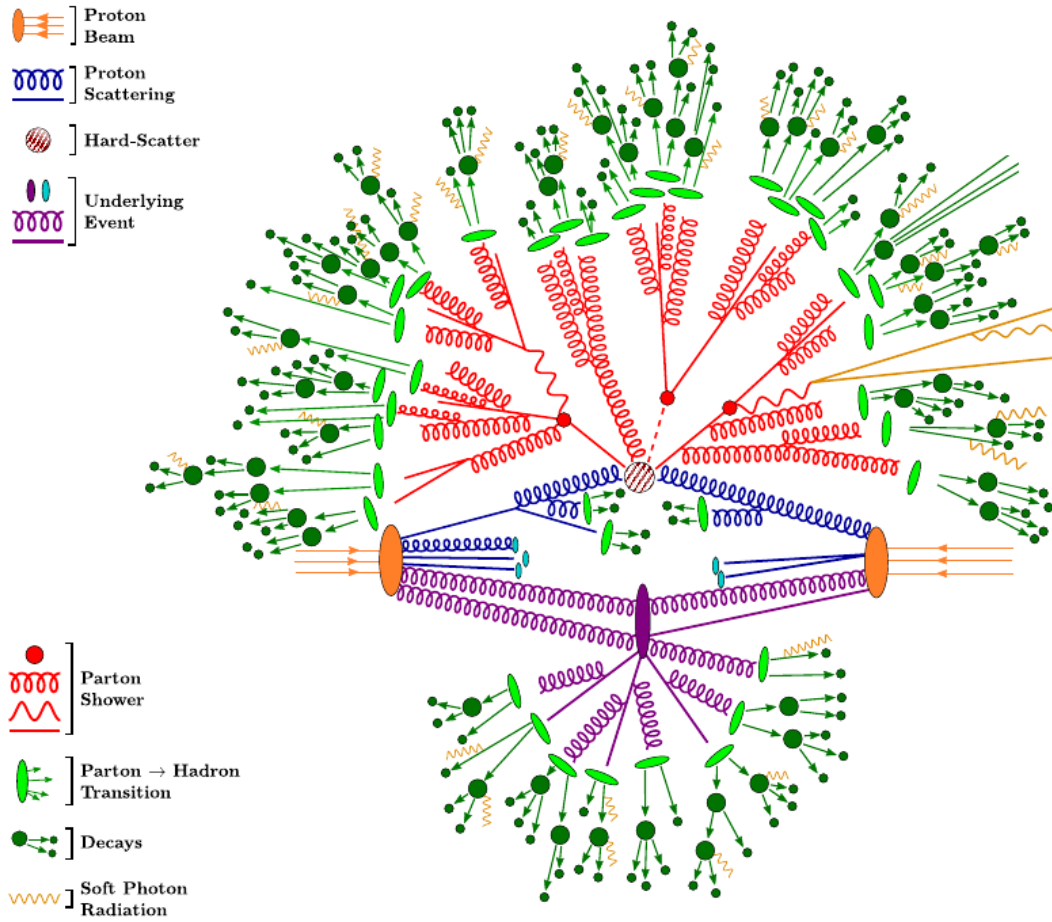
Figure 2.5: Sketch of a hadron-hadron collision as simulated by a Monte Carlo event generator. The red blob in the center represents the hard interaction, surrounded by a tree-like structure representing bremsstrahlung as simulated in parton showers. The purple blob represents a secondary hard multiple partons interaction. Hadronization process is represented by the light green blobs, dark green blobs indicate hadron decays, and yellow lines are soft photon radiation. [82]
