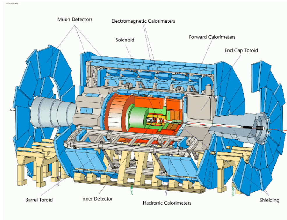
Figure 3.3: The ATLAS detector. [67]
