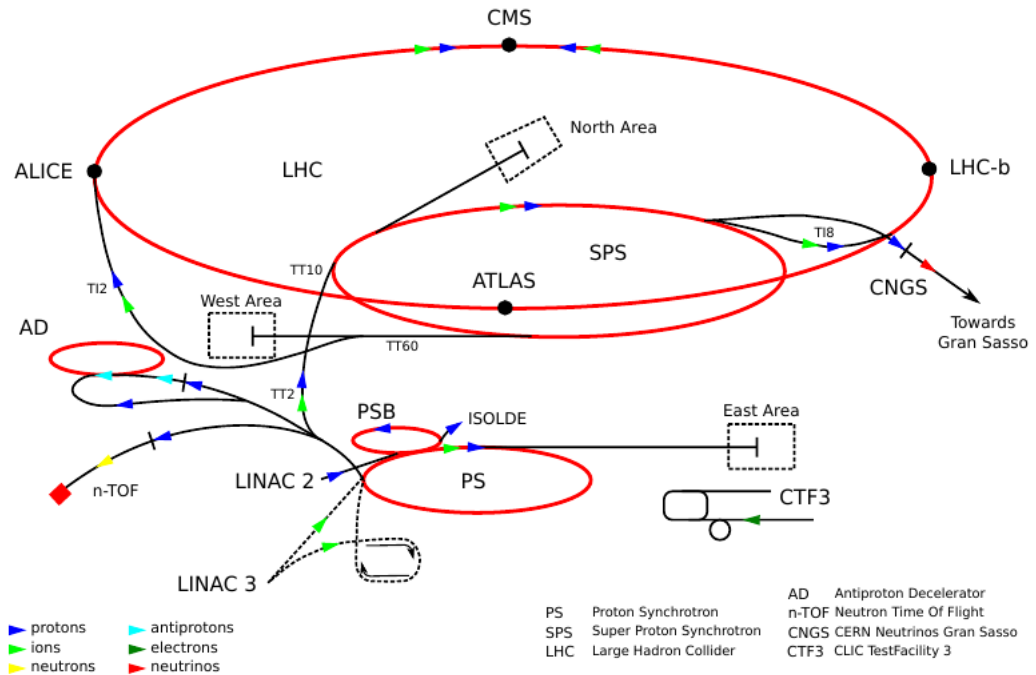
Figure 3.1: The accelerator complex at CERN. [21]
