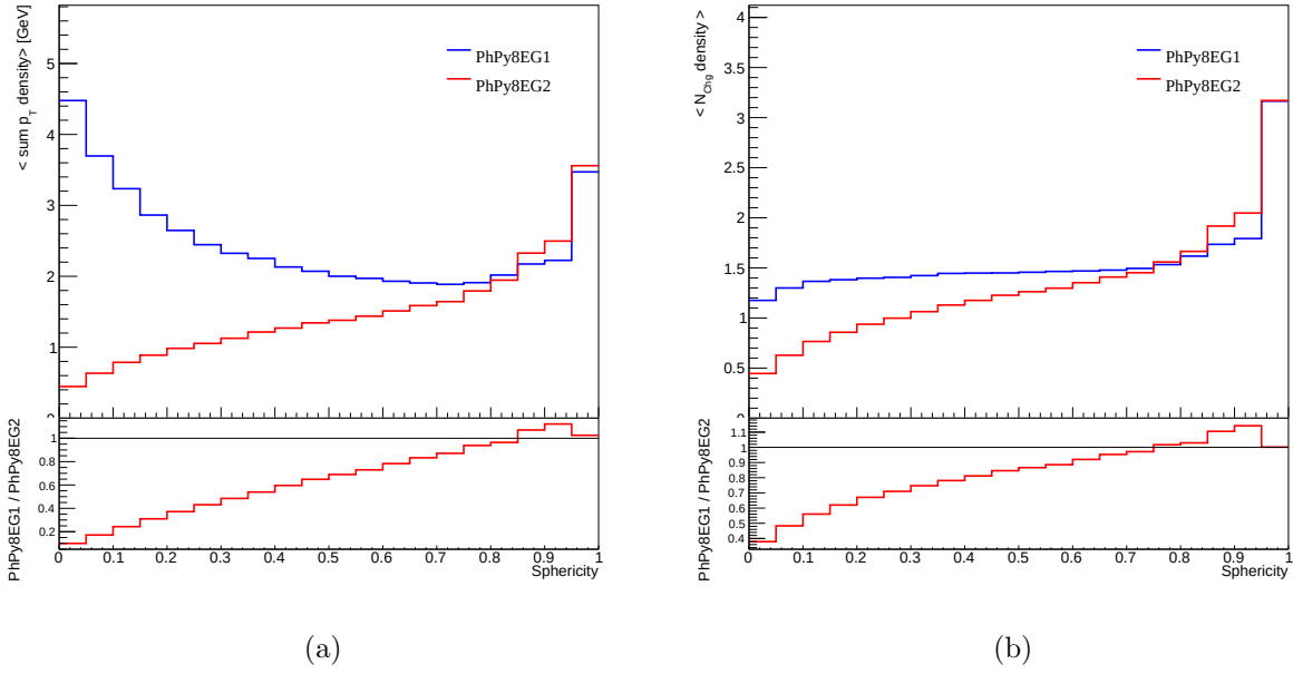
Figure 4.7: The mean of (a) the sum of the transverse momentum density \langle \text{sum } p_T \text{ density} \rangle , and (b) the mean of the multiplicity density \langle N_{Chg} \text{ density} \rangle of charged particles in the trans-min region as a function of the sphericity S . Two types of events were considered: for all events shown in blue, and for events for which the trans-min region is not contaminated by any jets, shown in red.
