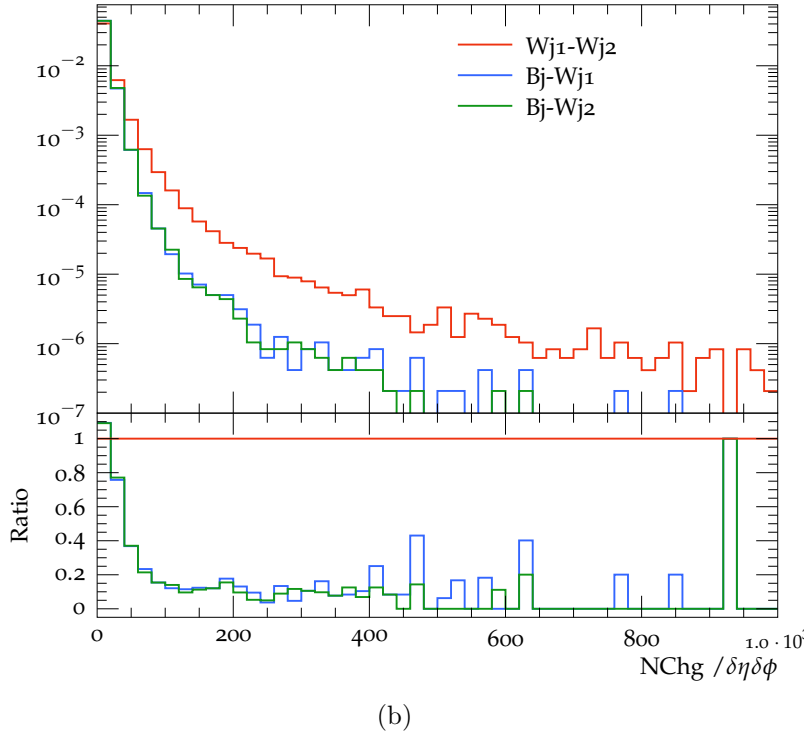
Figure 5.9: Distributions of (a) the sum of the transverse momentum density \sum p_T / \delta\eta\delta\phi , and (b) the multiplicity density NChg / \delta\eta\delta\phi of charged particles between these three pairs of jets. The bottom panel shows the ratio with respect to the pair Wj1-Wj2, where the blue line represents the ratio of the pair Wj1-Wj2 to the pair Bj-Wj1, and the green line represents the ratio of the pair Wj1-Wj2 to the pair Bj-Wj2.
