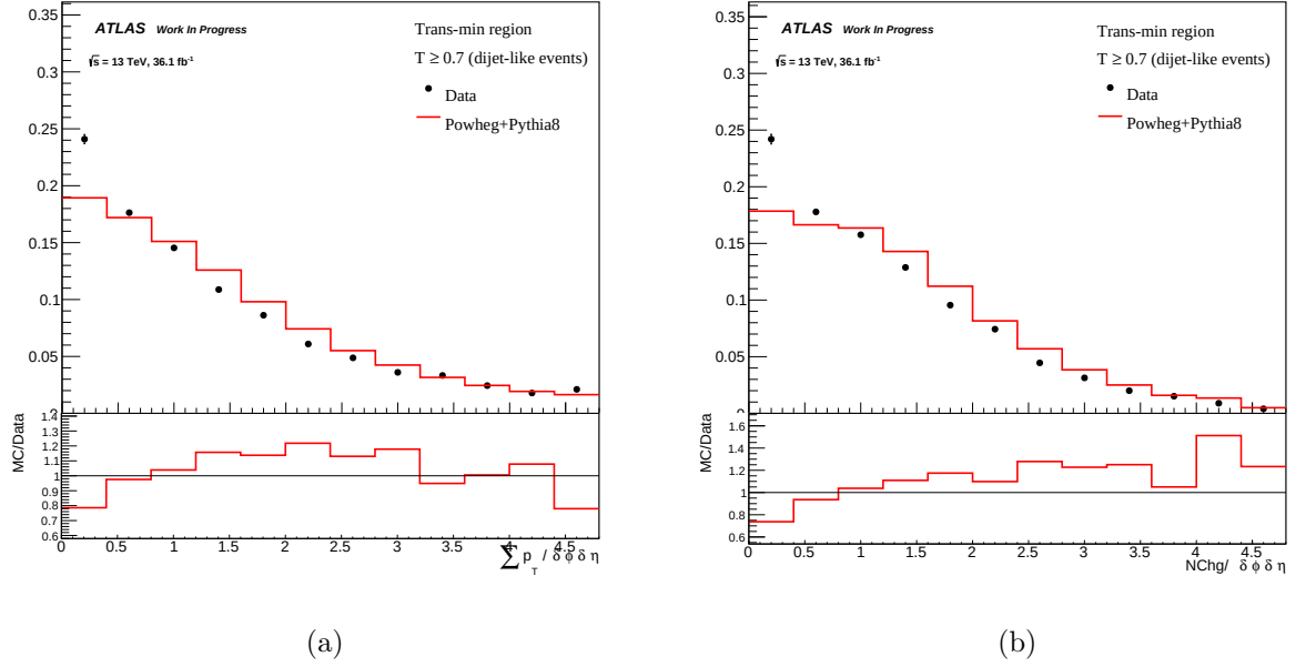
Figure 4.14: Distribution of (a) the sum of the transverse momentum density of charged particles \sum p_T / \delta\phi\delta\eta , and the (b) charged particles multiplicity density N_{Chg} / \delta\phi\delta\eta for events with T \geq 0.7 .
