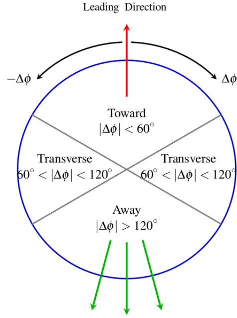
Figure 4.1: Definition of the UE regions as a function of the azimuthal angle with respect to the leading direction
