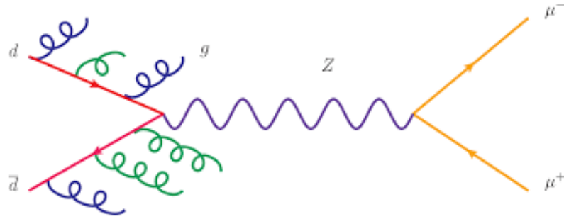
Figure 4.2: Feynman diagram of a Drell-Yan process producing a Z -boson decaying into muon pairs.
