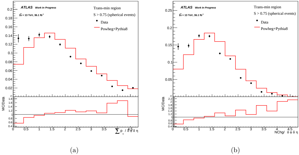
Figure 4.13: Distribution of (a) the sum of the transverse momentum density of charged particles \sum p_T / \delta\phi\delta\eta , and (b) the charged particles multiplicity density N_{Chg} / \delta\phi\delta\eta for events with S > 0.75 .
