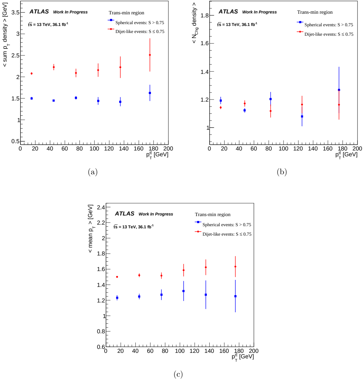
Figure 4.10: (a) The mean of the sum of the transverse momentum density \langle \text{sum } p_T \text{ density} \rangle , (b) the mean of the multiplicity density \langle N_{Chg} \text{ density} \rangle , and (c) the mean of the mean transverse momentum \langle \text{mean } p_T \rangle , of charged particles in the trans-min region for S > 0.75 and for S \leq 0.75 as a function of the p_T^{tt} .
