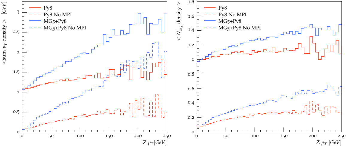
Figure 4.4: The mean of the sum of the transverse momentum density \langle \text{sum } p_T \text{ density} \rangle (left), and the mean of the multiplicity density \langle N_{Chg} \text{ density} \rangle (right) of charged particles in the toward region as a function of the momentum the Z -boson Z_{p_T} , both with MPI on and off for Pythia8 and Madgraph+Pythia8.
