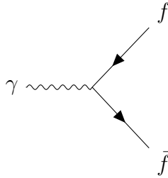
Figure 2.2: Feynman diagram of the QED interaction vertex.
