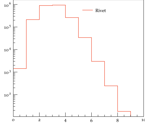
Figure 5.7: Distribution of the number of reconstructed anti- k_T R = 0.2 jets with p_T > 25 GeV inside an anti- k_T R = 1.0 jets with p_T > 200 GeV.
