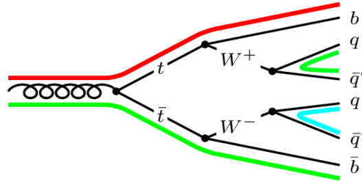
Figure 5.3: Feynman diagram of a t\bar{t} all hadronic channel (black lines) with QCD color propagation rule (colored lines).
