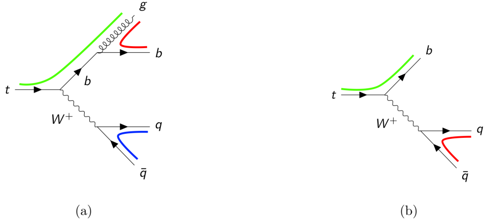
Figure 5.6: Feynman diagrams (black lines) of a t -quark decaying (a) with and (b) without additional radiative gluon from the b -quark, where the QCD color propagation rule are shown as the colored lines.
