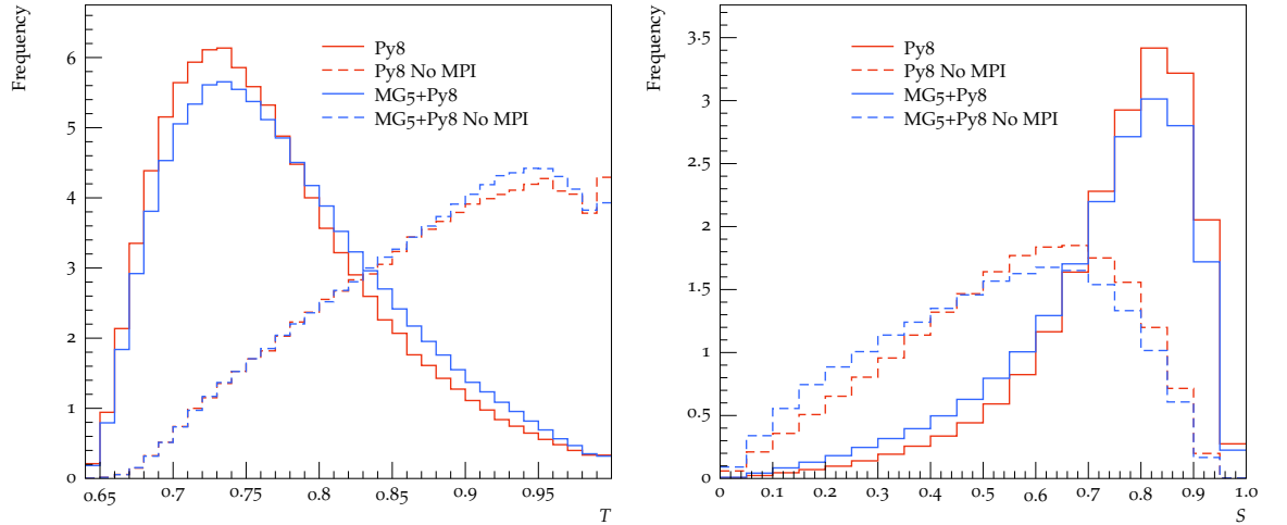
Figure 4.3: Transverse thrust T (left) and transverse sphericity S (right) distribution, both with MPI on and off for LO and multileg setups.
