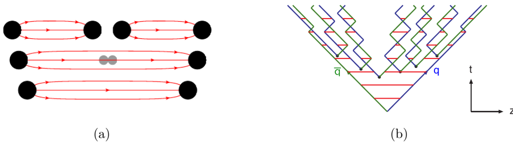
Figure 5.1: Illustration of (a) the string breaking by quark pair creation in the string field, and (b) the motion and breakup of a string system, with the two transverse degrees of freedom suppressed (diagonal lines are (anti)quarks, horizontal ones snapshots of the string field) [20].
