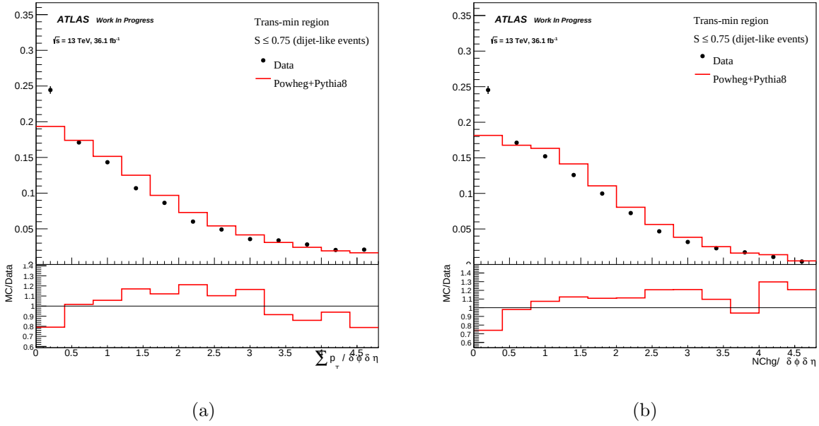
Figure 4.12: Distribution of (a) the sum of the transverse momentum density of charged particles \sum p_T / \delta\phi\delta\eta , and (b) the charged particles multiplicity density N_{Chg} / \delta\phi\delta\eta for events with S \leq 0.75 .
