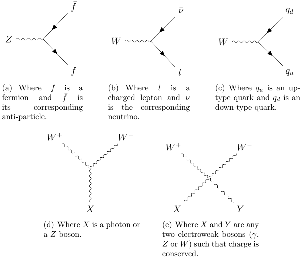
Figure 2.4: Feynman diagram of the weak interaction vertices.
