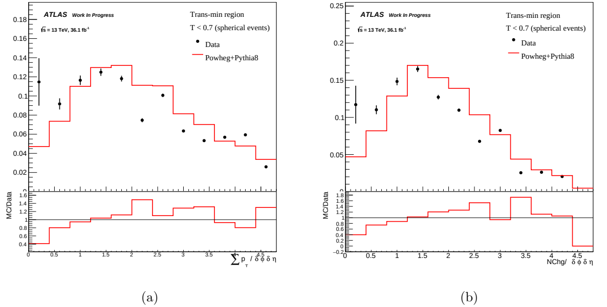
Figure 4.15: Distribution of (a) the sum of the transverse momentum density of charged particles \sum p_T / \delta\phi\delta\eta , and (b) the charged particles multiplicity density N_{Chg} / \delta\phi\delta\eta for events with T < 0.7 .
