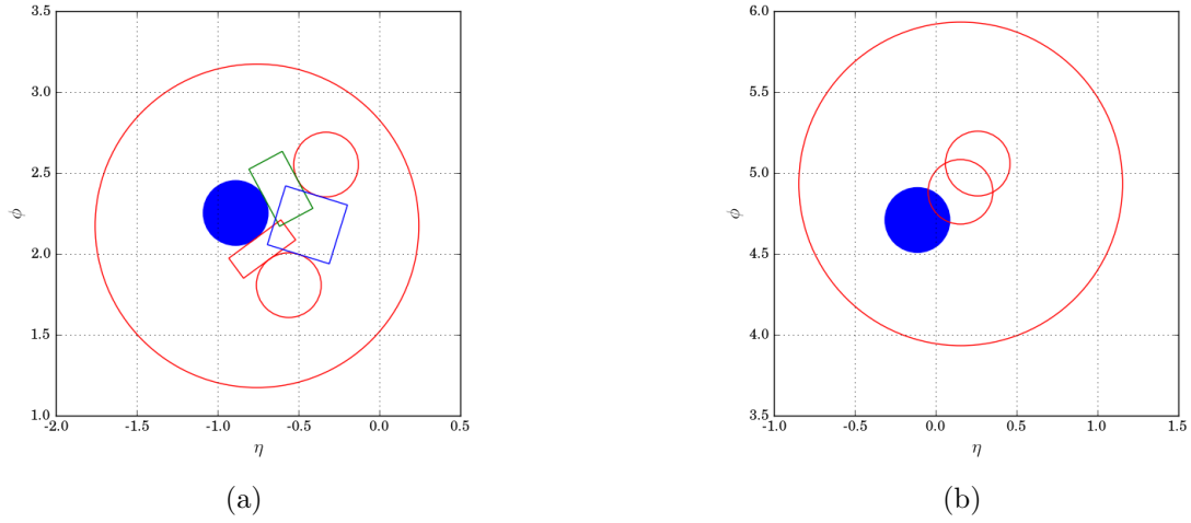
Figure 5.8: Examples of configurations of anti- k_t R = 0.2 jets inside an anti- k_t R = 1.0 jet. (a) A large radius jet where the three rectangular areas between the three anti- k_t R = 0.2 jets can all be defined. (b) A large radius jet where jet cones of the three anti- k_t R = 0.2 jets overlap.
