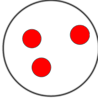
Figure 5.4: A representation of a large radius jet (black circles) with its subjets (red circle) in the \eta - \phi plane.
