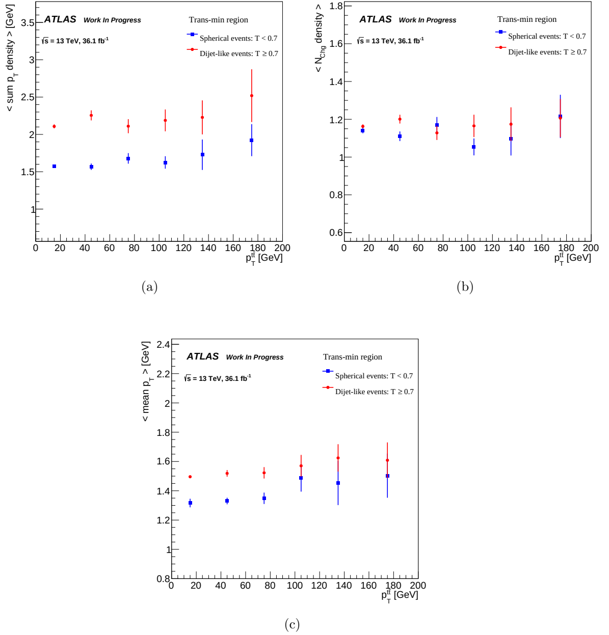
Figure 4.11: (a) The mean of the sum of the transverse momentum density \langle \text{sum } p_T \text{ density} \rangle , (b) the mean of the multiplicity density \langle N_{Chg} \text{ density} \rangle , and (c) the mean of the mean transverse momentum \langle \text{mean } p_T \rangle , of charged particles in the trans-min for T < 0.7 and for T \geq 0.7 as a function of the p_T^t .
