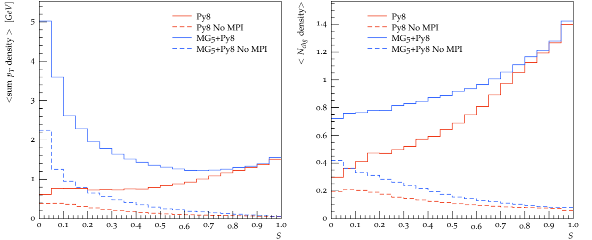
Figure 4.6: The mean of the sum of the transverse momentum density \langle \text{sum } p_T \text{ density} \rangle (left) and the mean of the multiplicity density \langle N_{Chg} \text{ density} \rangle (right) of charged particles in the toward region as a function of the sphericity S , both with MPI on and off for for Pythia8 and Madgraph+Pythia8.
