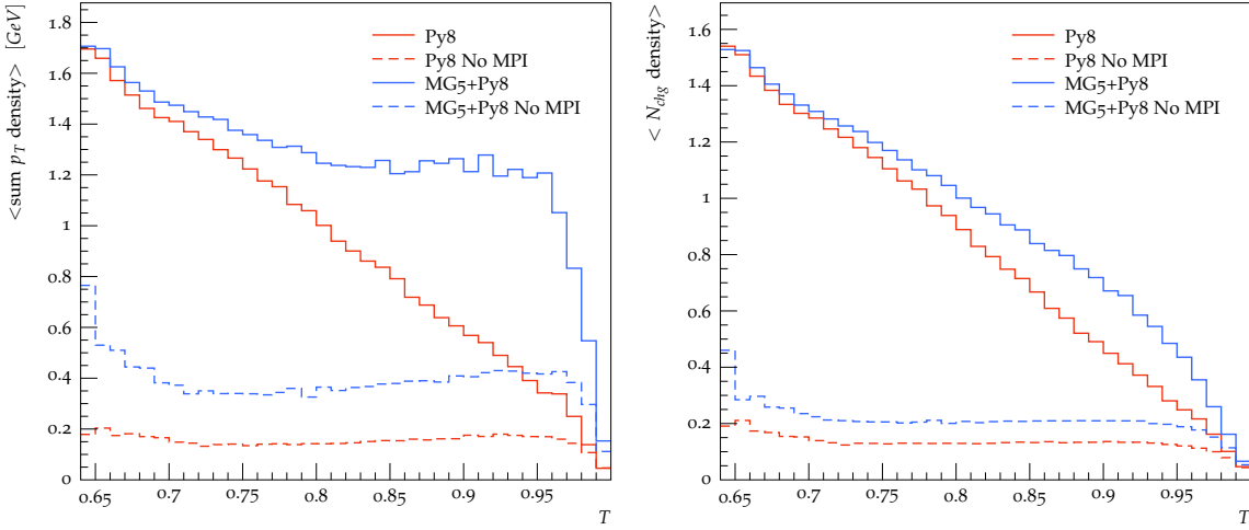
Figure 4.5: The mean of the sum of the transverse momentum density \langle \text{sum } p_T \text{ density} \rangle (left), and the mean of the multiplicity density \langle N_{Chg} \text{ density} \rangle (right) of charged particles in the toward region as a function of the the thrust T , both with MPI on and off for Pythia8 and Madgraph+Pythia8.
