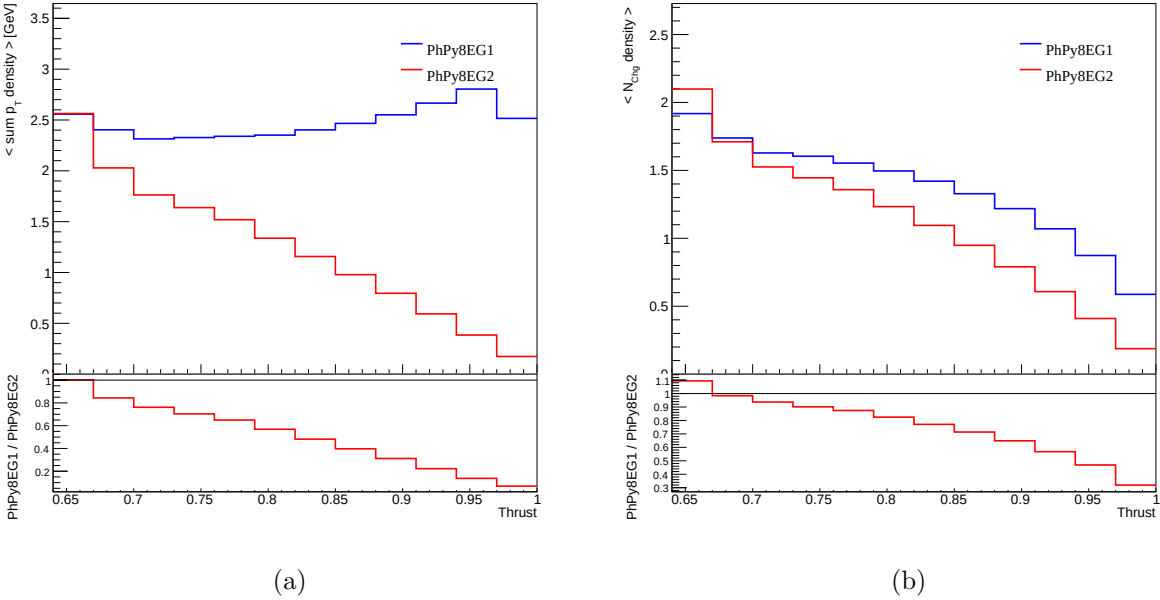
Figure 4.8: The mean of (a) the sum of the transverse momentum density \langle \text{sum } p_T \text{ density} \rangle , and (b) the mean of the multiplicity density \langle N_{Chg} \text{ density} \rangle of charged particles in the trans-min region as a function of the thrust T . Two types of events were considered: for all events shown in blue, and for events for which the trans-min region is not contaminated by any jets, shown in red.
