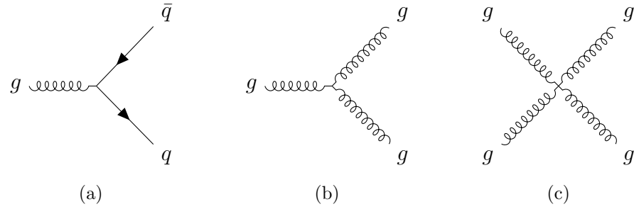
Figure 2.3: Feynman diagram of the QCD interaction vertices.
