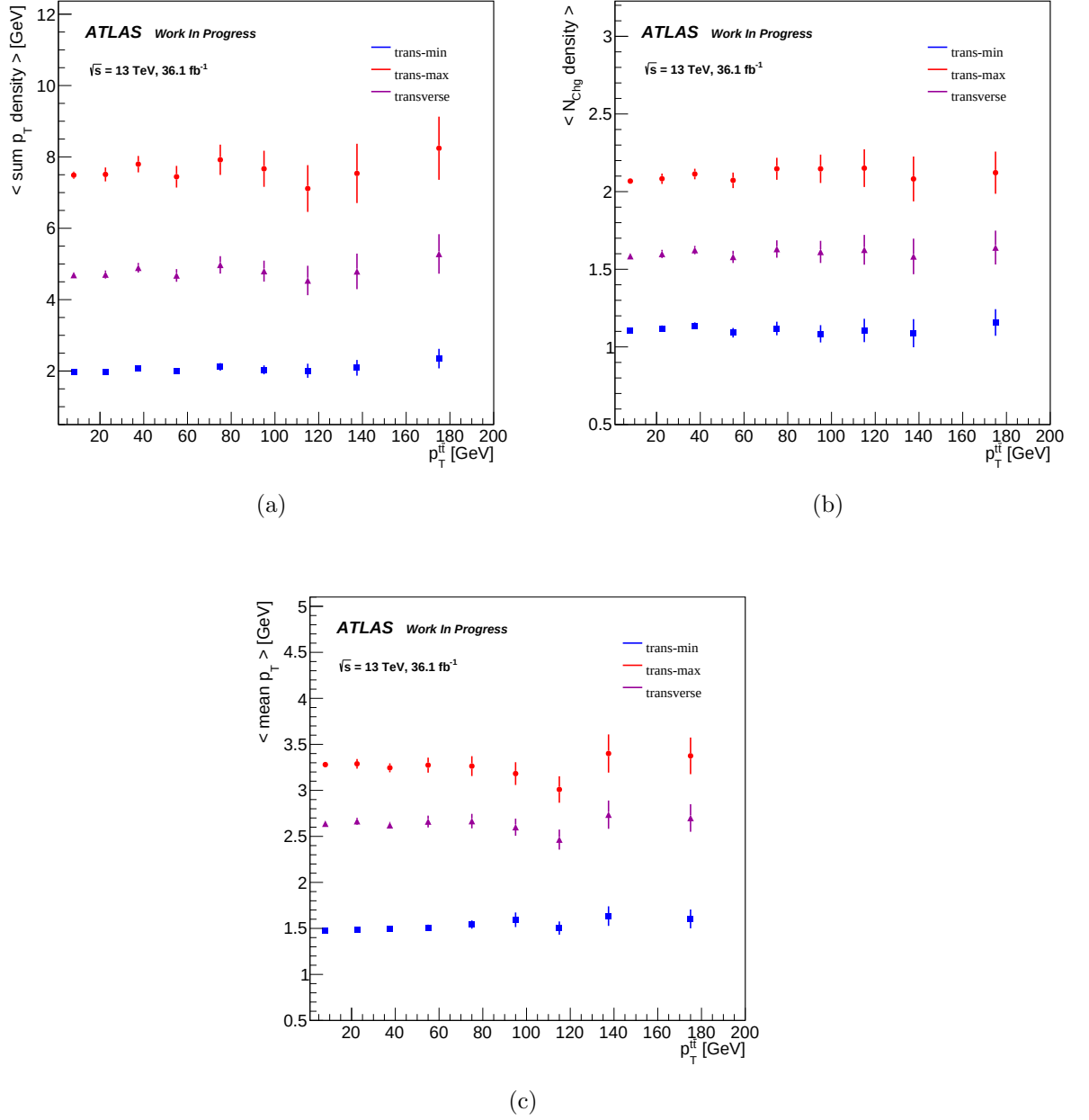
Figure 4.9: (a) The mean of the sum of the transverse momentum density \langle \text{sum } p_T \text{ density} \rangle , (b) the mean of the multiplicity density \langle N_{Chg} \text{ density} \rangle , and (c) the mean of the mean transverse momentum \langle \text{mean } p_T \rangle , of charged particles in the trans-min, trans-max and transverse region as a function of the p_T^{t\bar{t}} .
