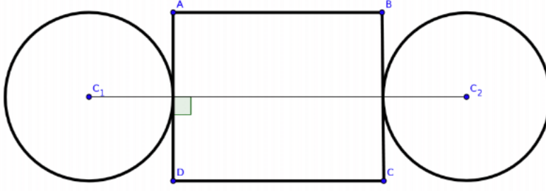
Figure 5.5: Diagram illustrating the rectangular region between jets.
