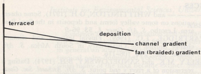
Figure 6. Gradients of braided and meandering channels.
