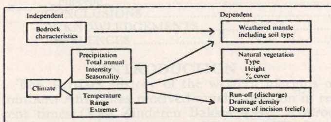
Figure 7. Environmental parameters affecting landform development.
