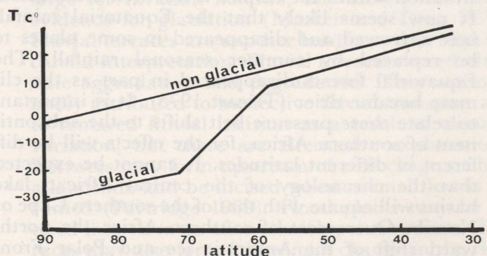
Figure 1. Present-day latitudinal mean temperature gradient compared to a glacial temperature gradient.
