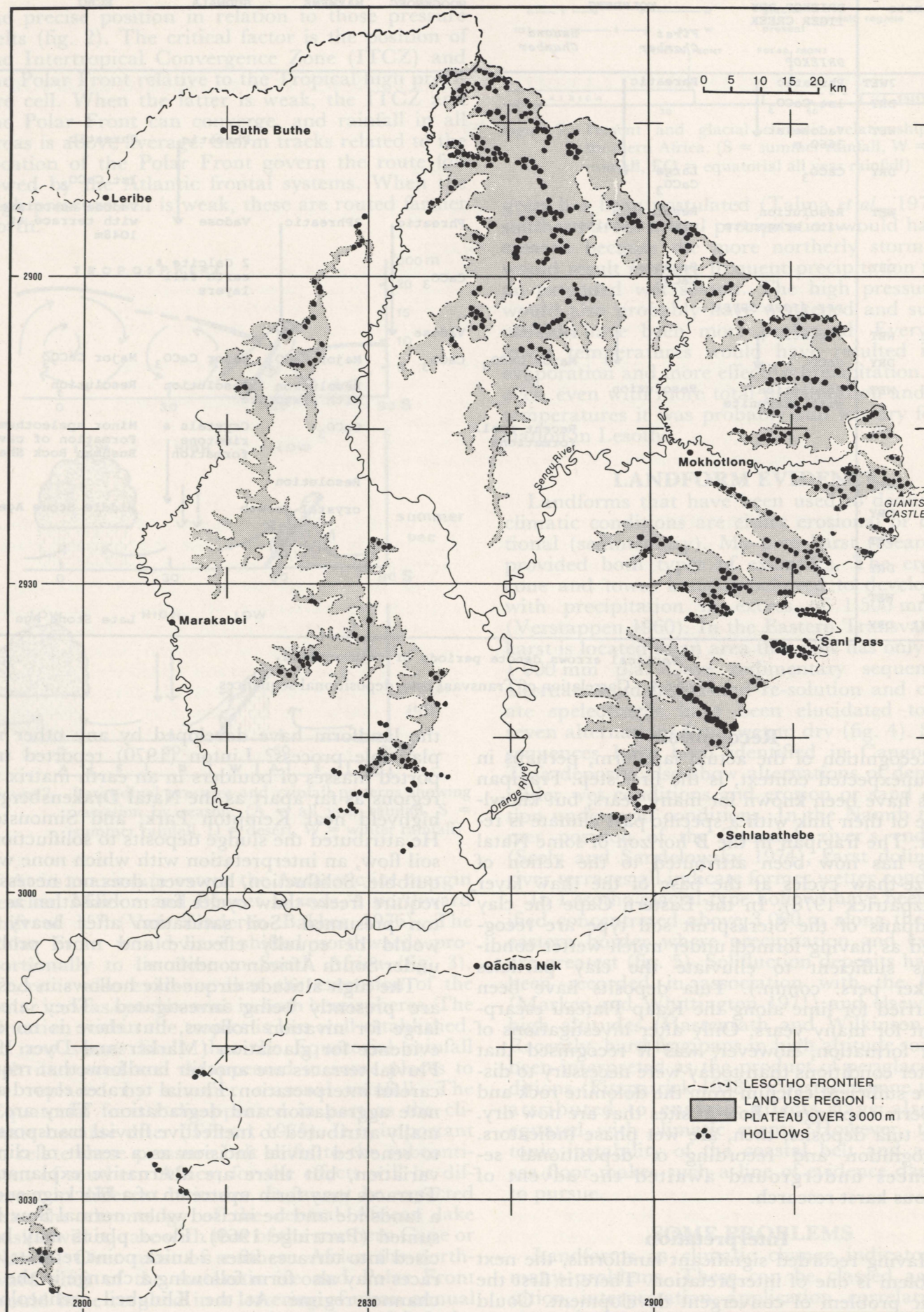
Figure 5. The distribution of high level hollows in Lesotho.
