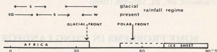
Figure 3. Present and glacial climatic relationships over southern Africa. (S = summer rainfall, W = winter rainfall, EQ = equatorial all year rainfall)
